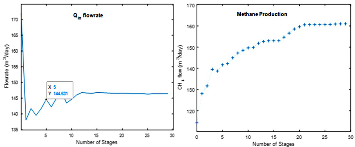
Figure 5.17: Flowrate in, q and how the resulting gas production changes during the simulation.
