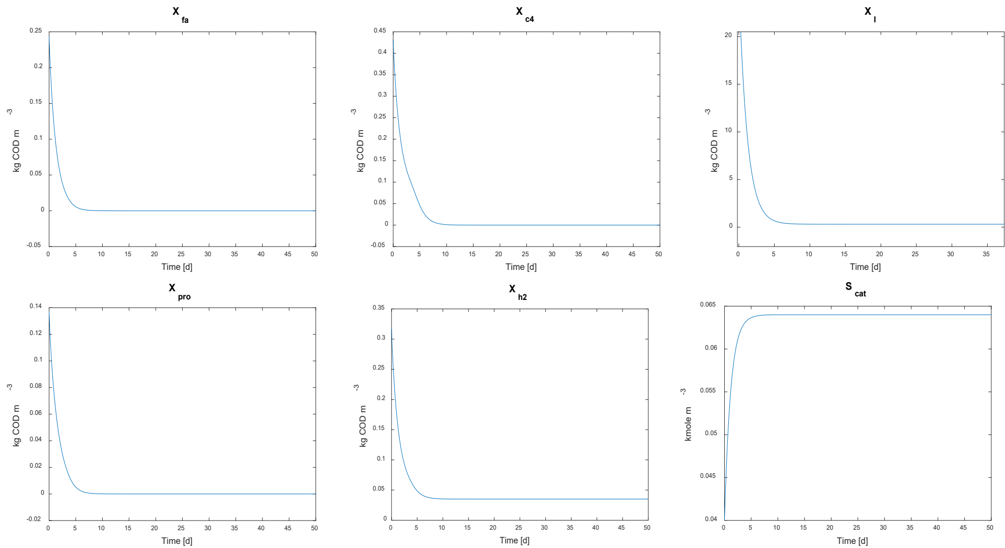
Figure 5.7: Model simulation component output, Substrate number output 20-25
