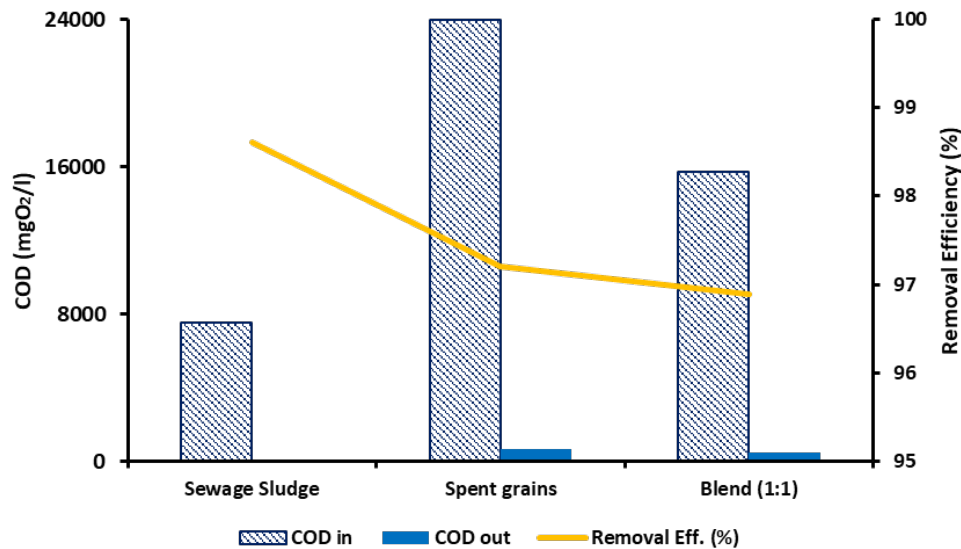
Figure 4.12: The COD of the feed and after the BMP study, and the COD removal efficiency
