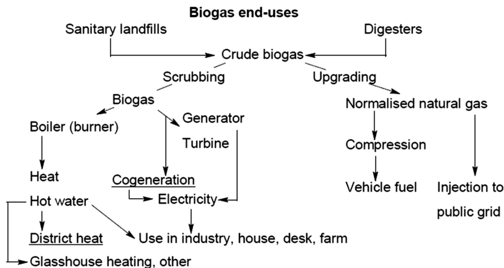
Figure 2.1: Applications and utilization of biogas
