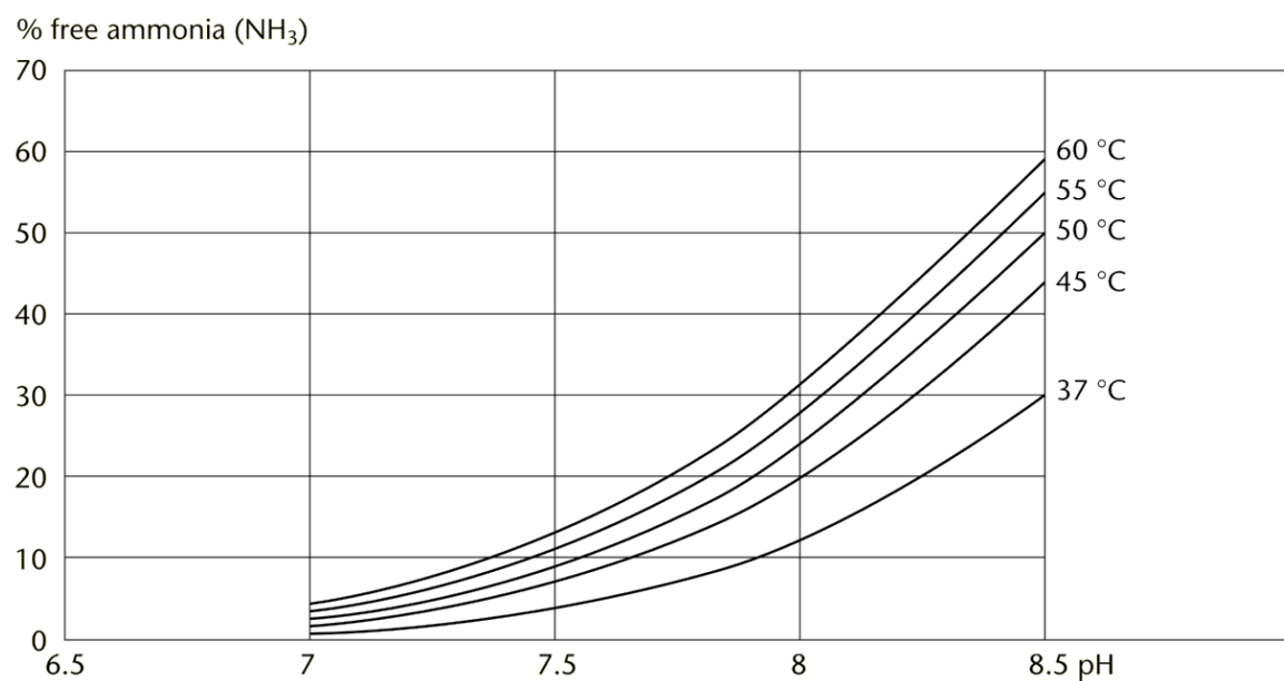
Figure 2.6: The influence of temperature and pH on the balance of ammonium ion and ammonia (Emerson, et al. 2015)
