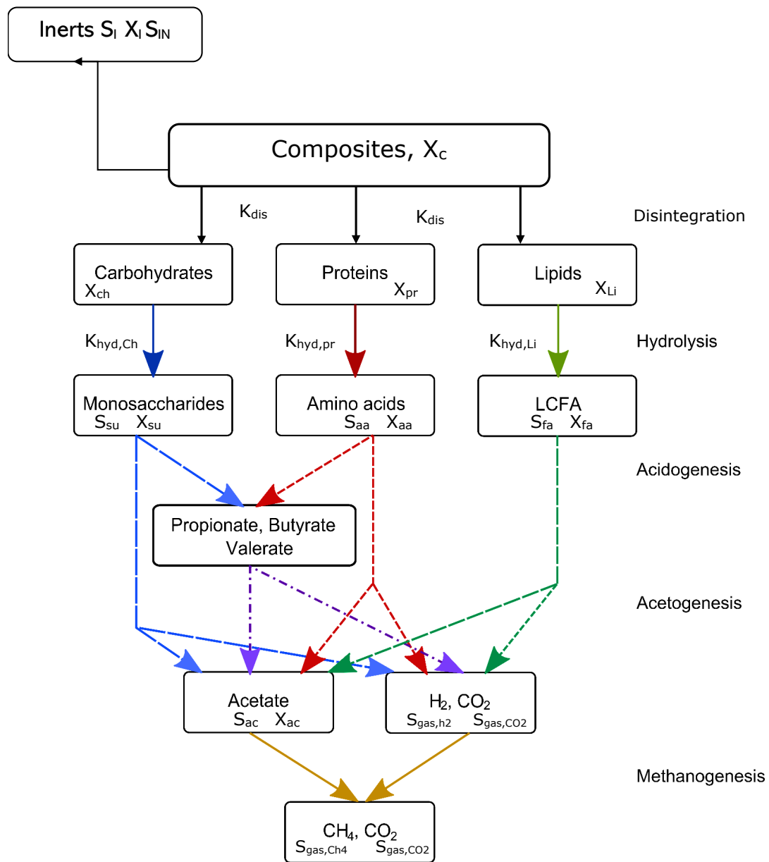
Figure 5.1: Anaerobic digestion process, composites degradation to inerts and hydrolysis reactants, through a disintegration step.
