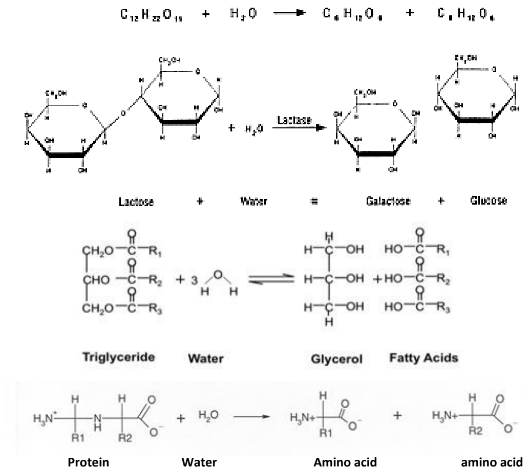
Figure 2.4: Simultaneous hydrolysis reaction. (i) Carbohydrates: Lactose, a polysaccharide, is hydrolyzed to produce galactose and glucose, both monosaccharides. (ii) Lipids: triglycerides are split into three fatty acids and glycerol in the presence of water molecules. (iii) Proteins: peptide bonds are broken to separate amino acids. Adapted from (Rea, 2014)
