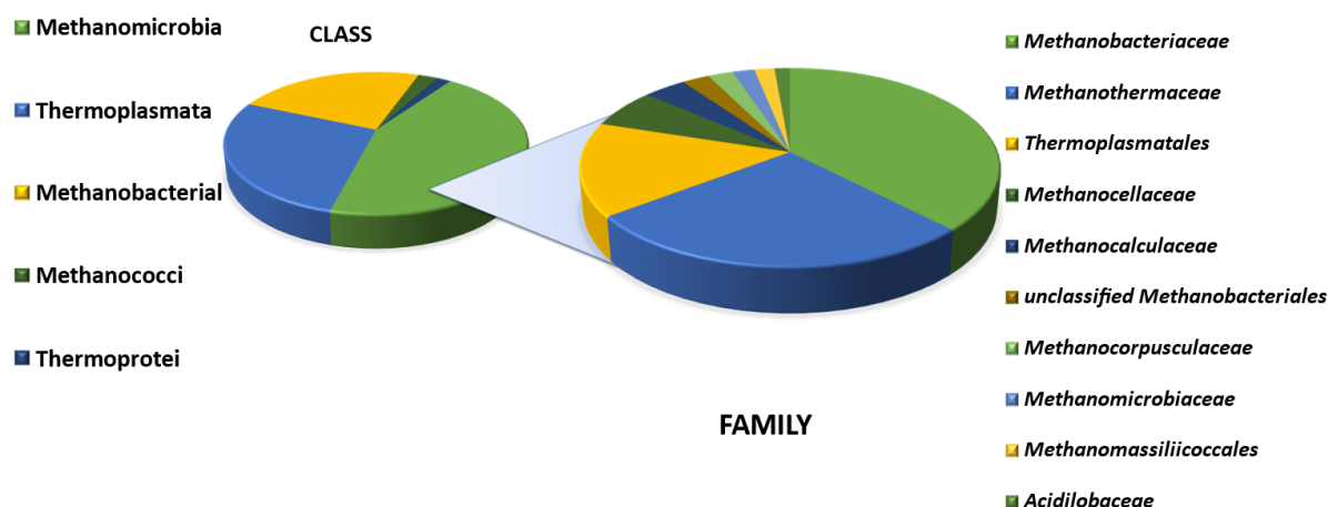
Figure 4.5: Kingdom Archaeal community composition in the classification of class and significant family.
