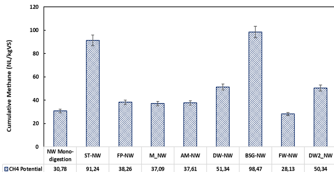
Figure 4.9: Methane production of Driefontein WWTW sludge and the co-substrates
