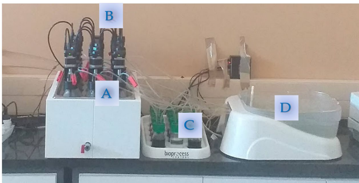
Figure 3.6: The biochemical methane potential test using the automatic methane potential test system (AMPTS II).
