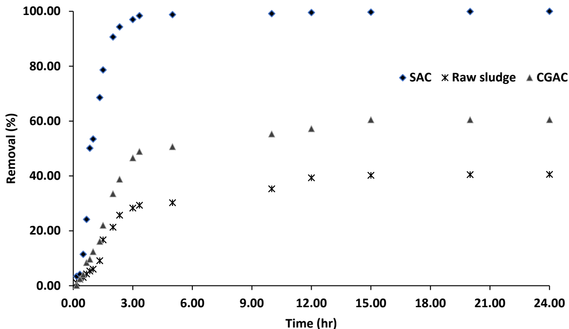
Figure 6.5: Adsorption of Cr(VI) by the sewage sludge-based activated carbon with time
