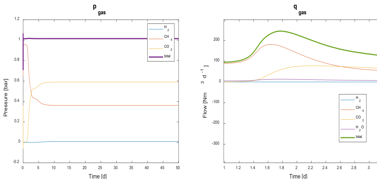
Figure 5.11: Component output for gas production, pressure, and flow rate.
