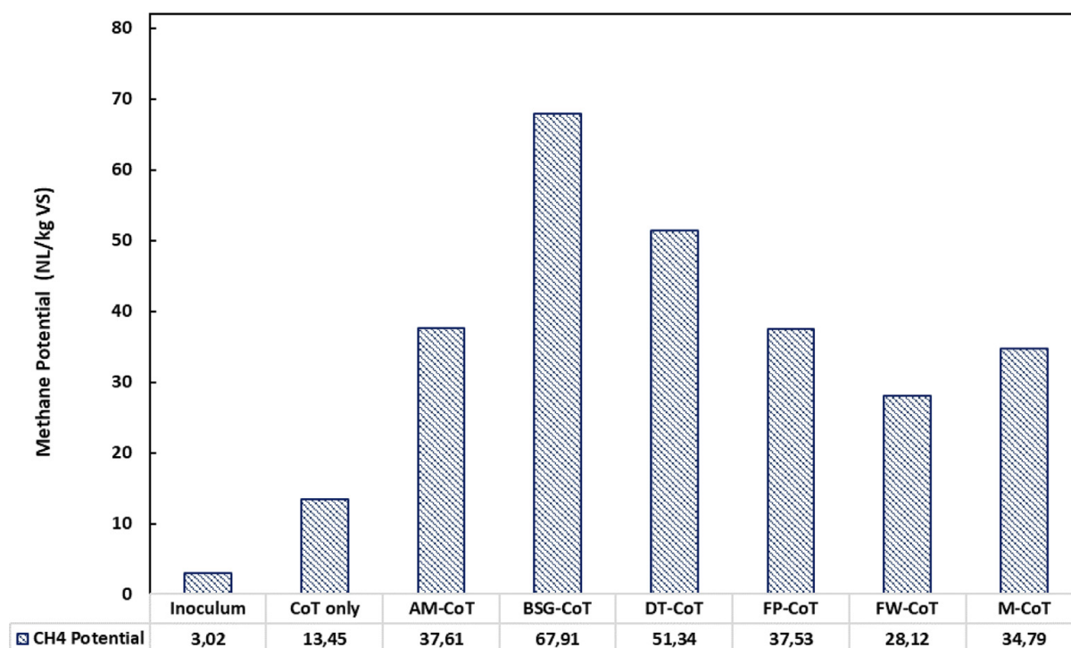
Figure 4.10: Methane production of Driefontein WWTW sludge and the co-substrates
