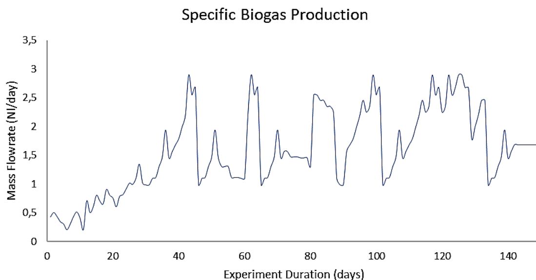
Figure 4.11: Semi-continuous biogas production per day
