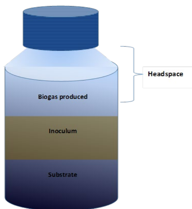
Figure 3.4: The Digester setup in the BMP setup Substrates & inoculum measurements
