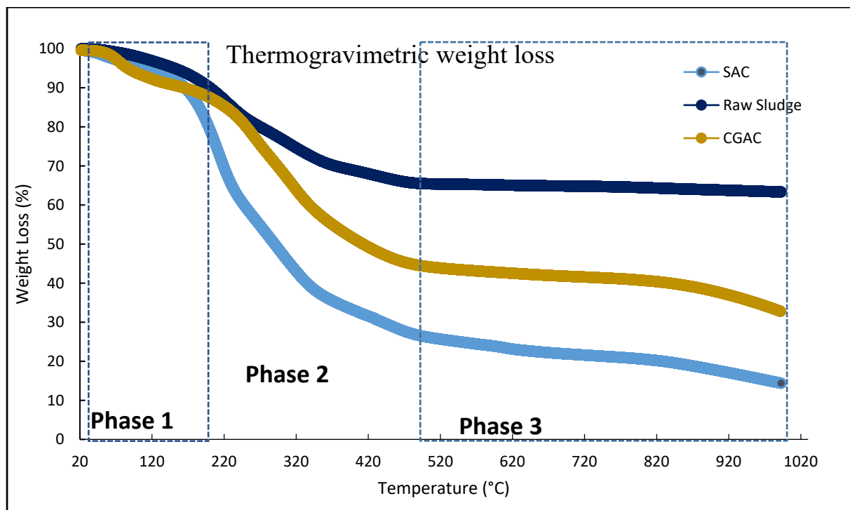
Figure 6.2: Thermal decomposition of raw sewage sludge and SAC
