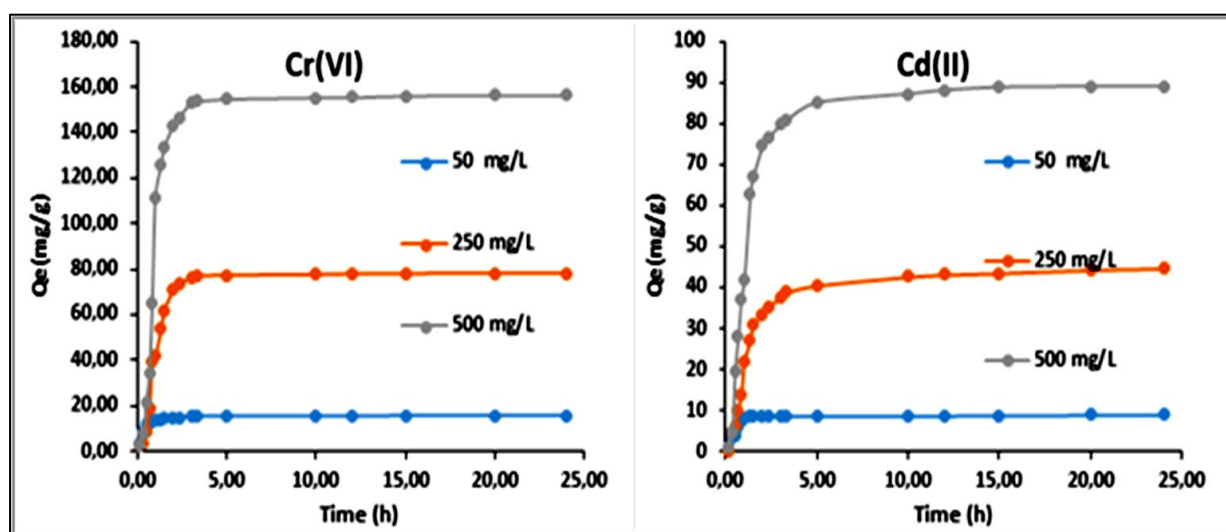
Figure 6.8: The adsorption uptake versus adsorption time at various initial concentrations at 30°C on sludge-based activated carbon.
