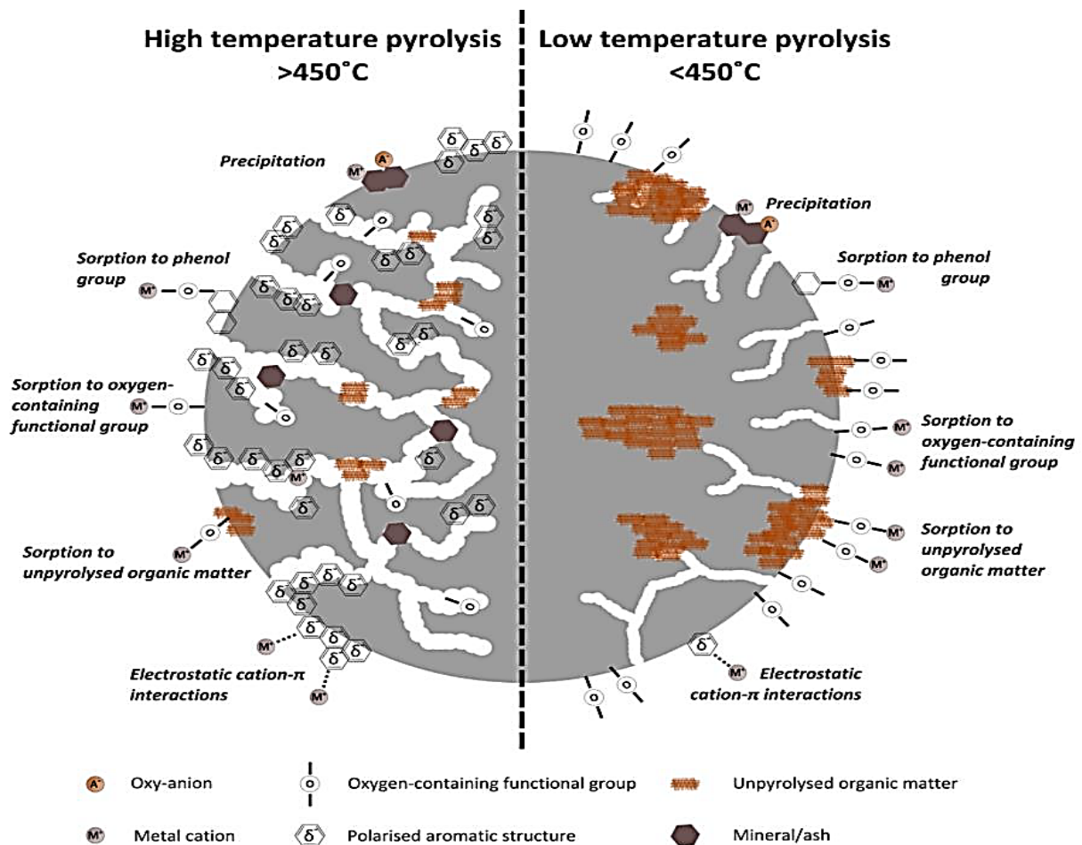
Figure 2.13: Adsorption mechanism on biochar surface in two temperature ranges (Ahmad et al., 2014)
