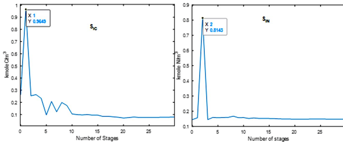
Figure 5.16: Optimal combination of S_{IC} and S_{IN} input variables propagates during a simulation
