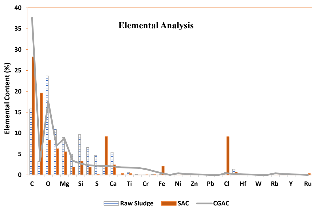
Figure 6.4: EDX spectra or Semi-quantitative XRF analysis of the raw sludge SAC and raw sludge samples
