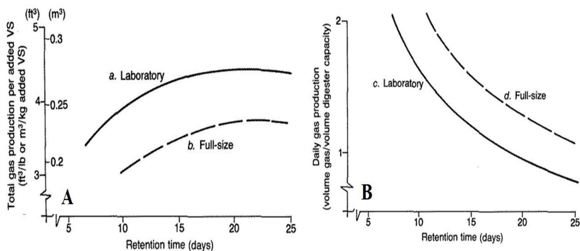
Figure 2.9: Effect of HRT on specific and daily biogas yield, (Masebinu, 2018)
