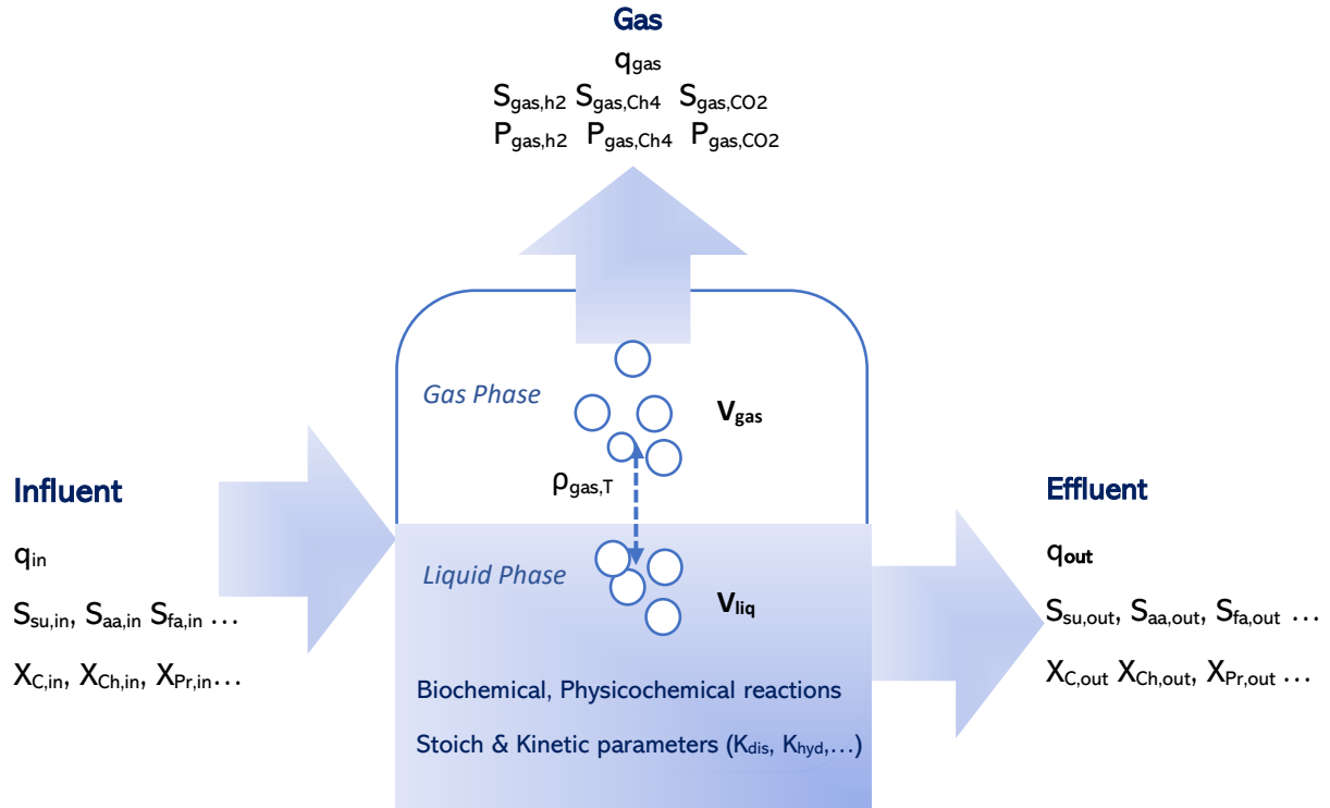
Figure 5.2: Mass balance boundary around CSTR in the anaerobic digestion system, adapted from Batstone et al (2002).
