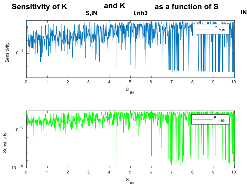
Figure 5.13: Variable dependence of sensitivity for two parameters. Sensitivity is constantly tested meanwhile a variable is changed. K_{S,IN} and K_{i,NH_3} are investigated as function of S_{IN}
