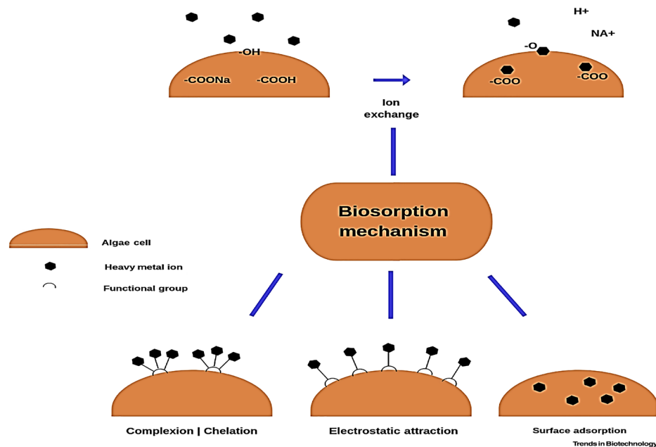
Figure 2.15: Pictorial definition of adsorption & Ion Exchange Process, (Gong, 2013).
