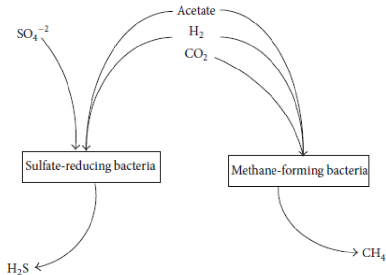
Figure 2.7: Sulphate-reducing bacteria compete for resources with the \text{CH}_4 -forming microbial community (Gerardi, 2003).
