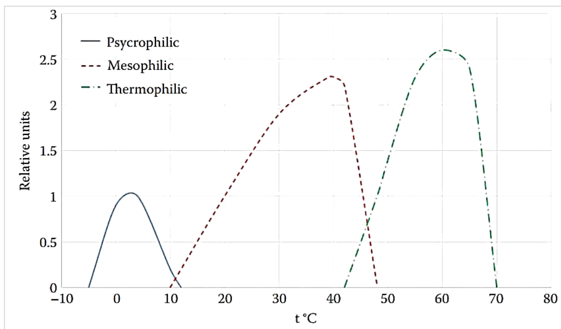
Figure 2.8: The efficiency of anaerobic bacterial growth at various temperature profiles (Rosato., 2008).
