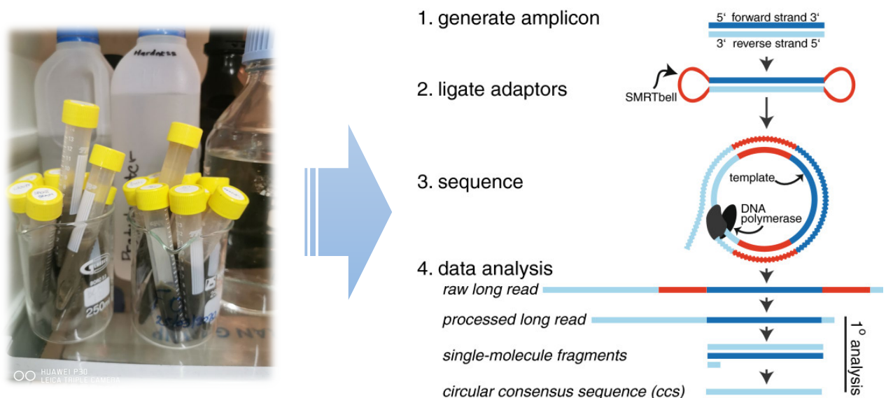
Figure 3.2: Illustration of Sample & PacBio sequence generation procedure, adapted from (PacBio, 2015)
