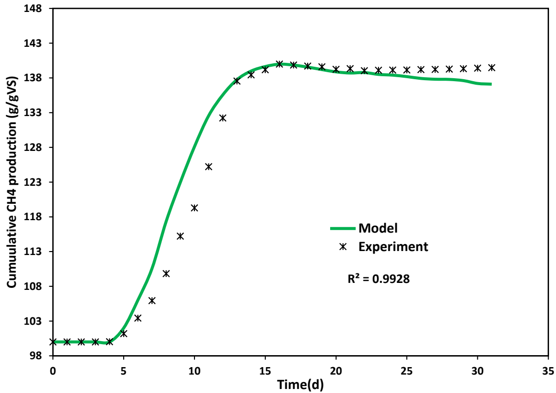
Figure 5.14: Comparison of the batch experimental and simulated methane production results.
