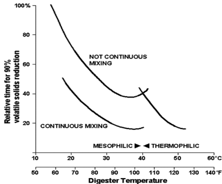
Figure 2.10: The effect of agitation on the degradation process of VS, volatile solids, Source (Meegoda et al., 2012)
