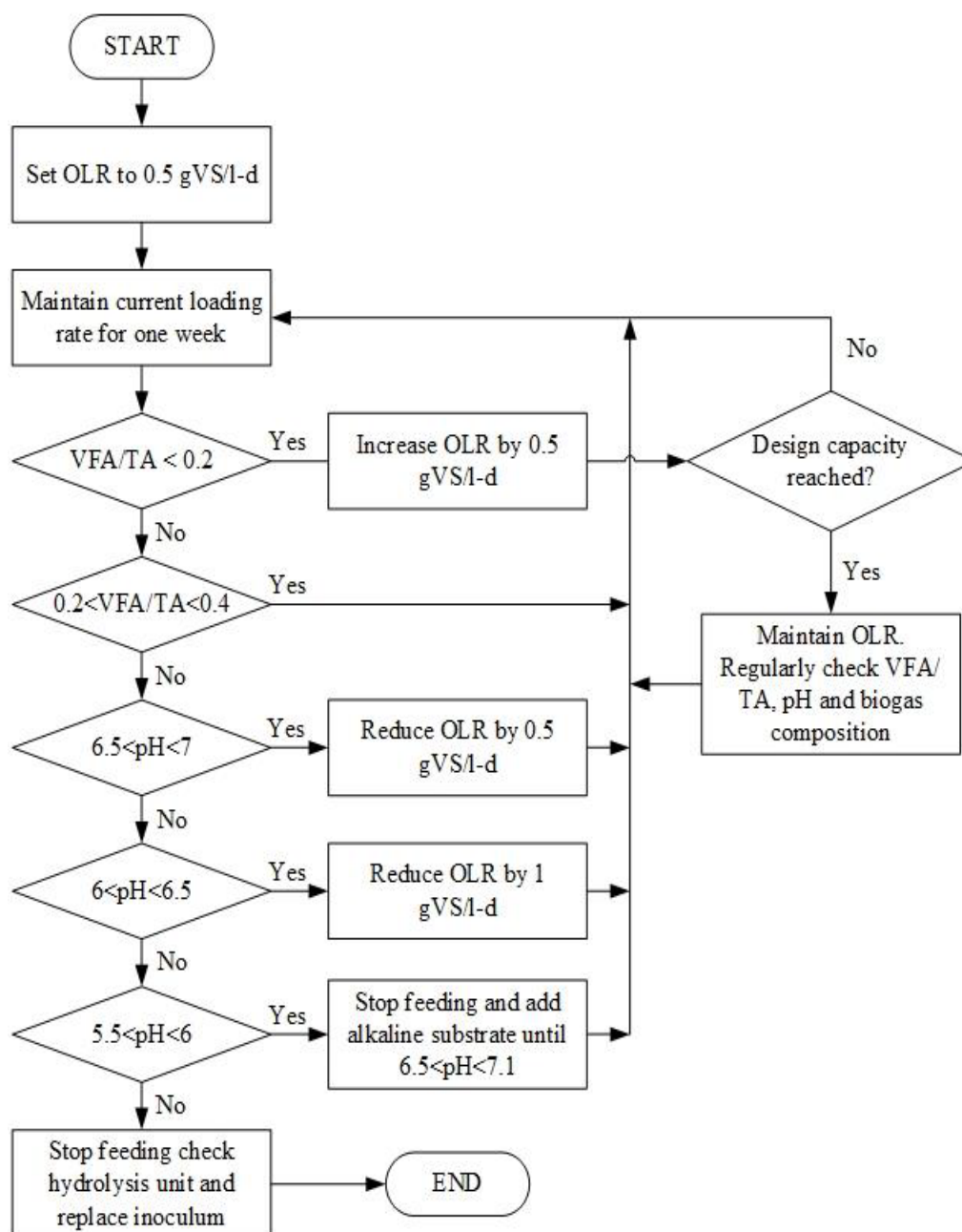
Figure 3.9: Procedure on how to adjust the OLR, adapted from Masebinu, (2018).
