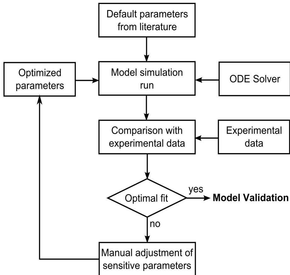
Figure 5.3: Flow chart for running the ADM1 model using Matlab/Simulink™
