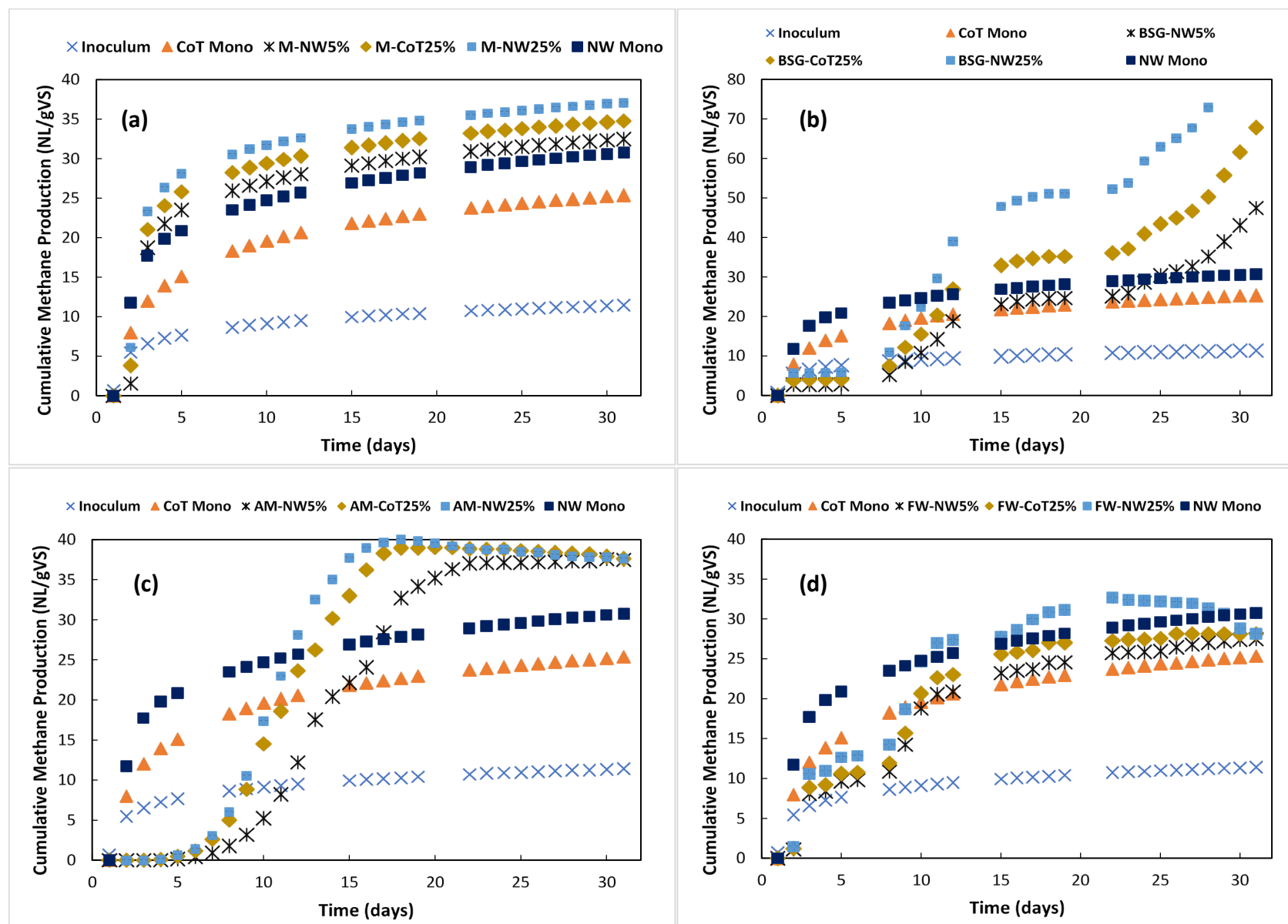
Figure 4.6: Cumulative methane production for co-digestion of sludge and (a) Molasses (b) BSG, spent grains (c) AM, animal manure (d) FW, food waste
