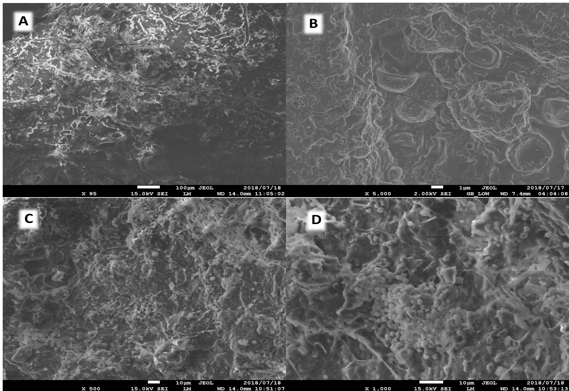
Figure 6.1: SEM micrographs, (A): Raw sludge; (B): SAC shows spherical carbon particles on the surface of carbonized.
