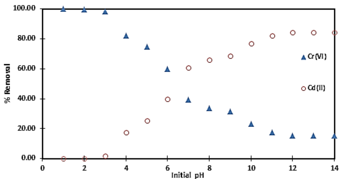
Figure 6.6: Effect of initial pH on adsorption of Cr (VI) and Cd (II)
