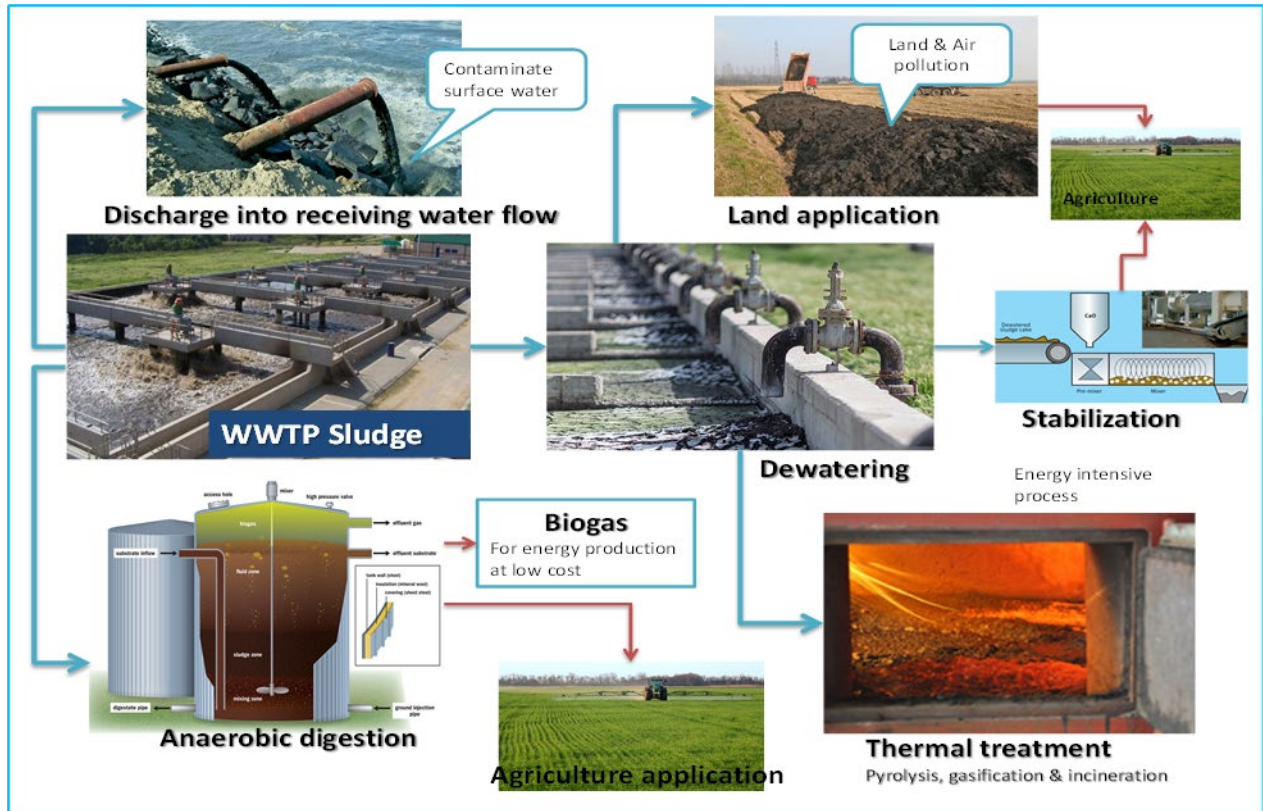
Figure 1.1: Current practice of sludge treatment in the municipality WWTP, adapted from (Department of Environmental Affairs, 2014; Department of Energy, 2019; Water Research Commission, 1997)
