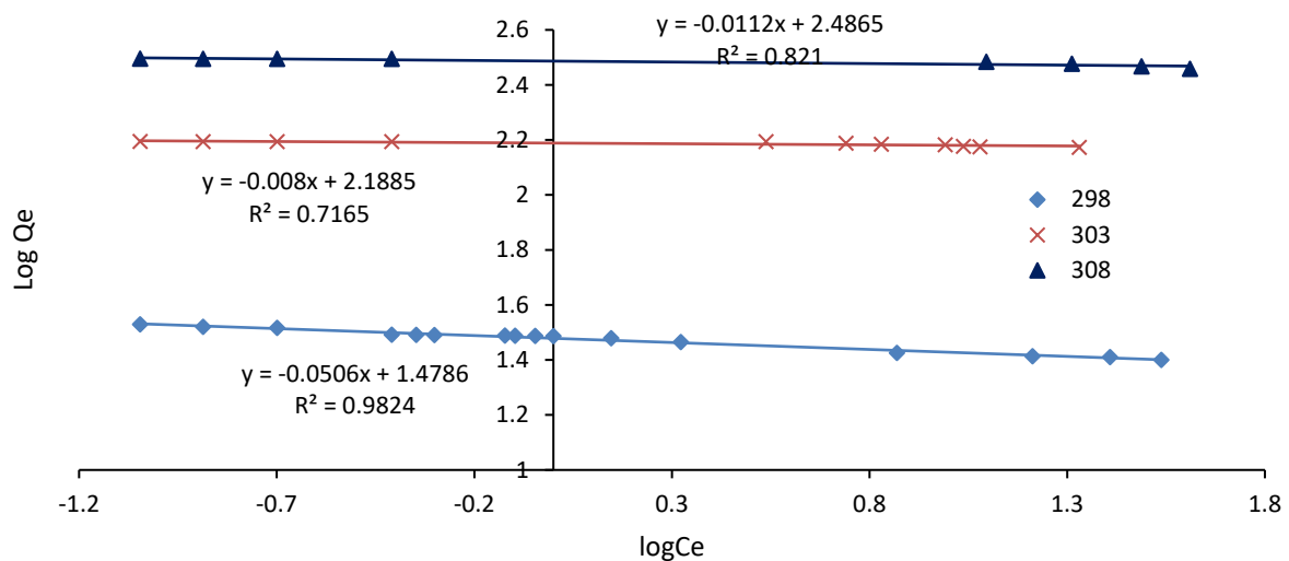
Figure 6.10: Linearized Freundlich isotherm for adsorption
