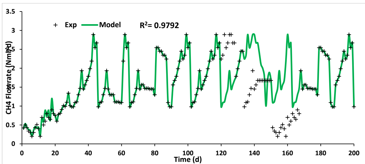
Figure 5.15: Comparison of the semi-continuous experimental and simulated methane production results.
