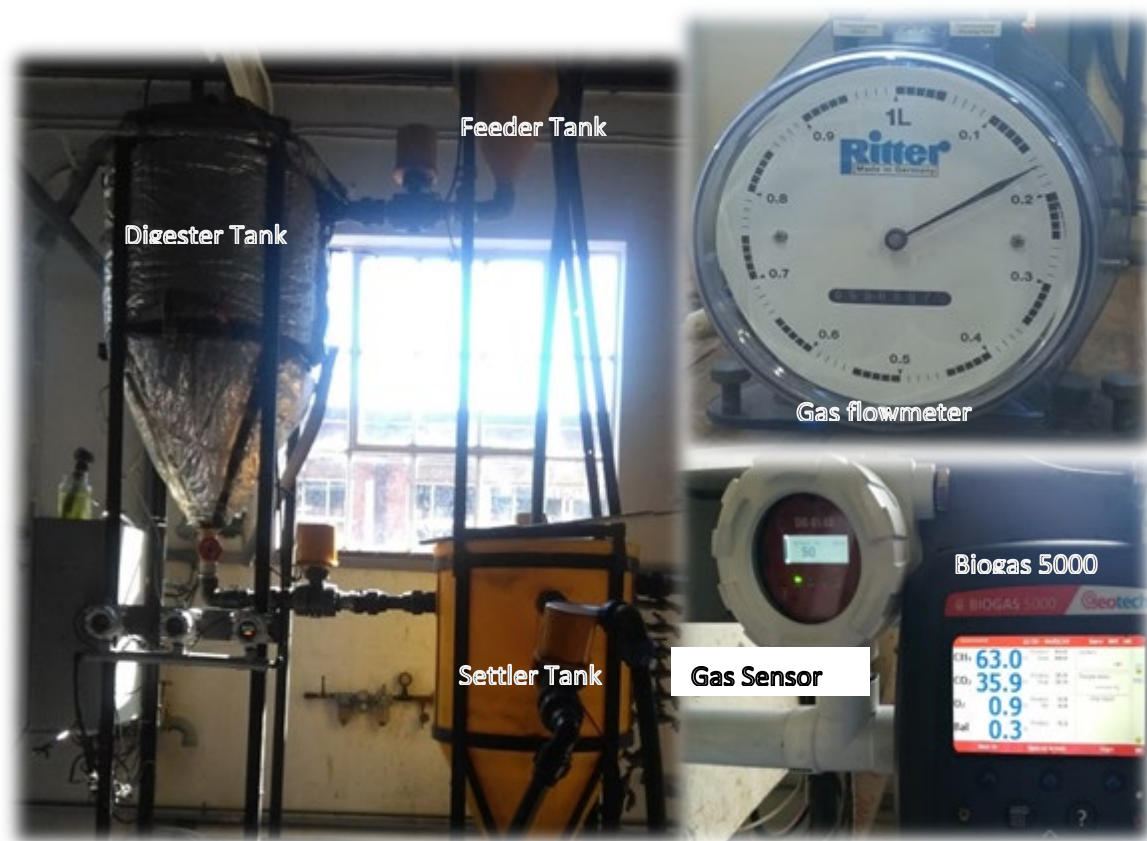
Figure 3.8: CSIR Semi-continuous Digester, Ritter gas flowmeter, and Geotech Biogas5000
