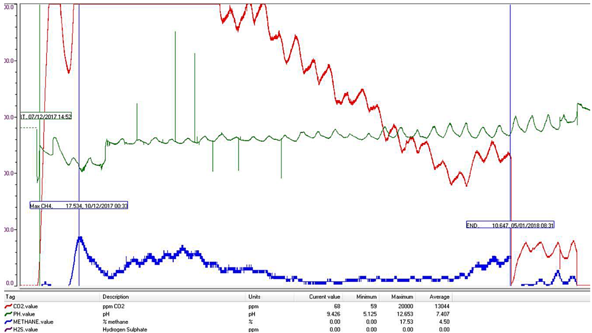
Figure 4.13: Pilot plant Trial 1, methane & carbon dioxide concentration and pH profile
