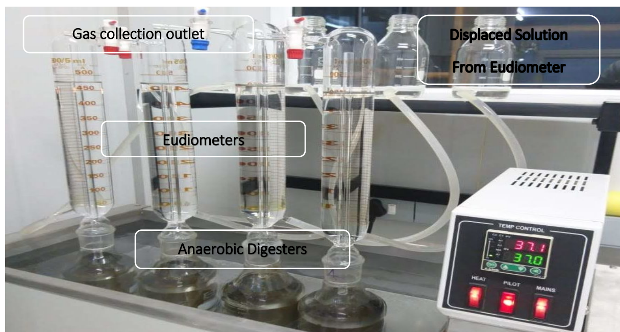
Figure 3.5: Eudiometer setup for estimating biogas from substrates
