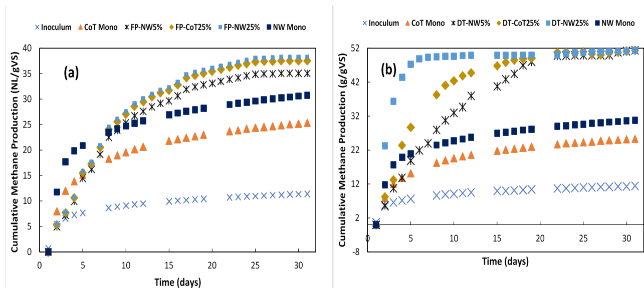
Figure 4.7: Methane cumulative results for co-digestion of sludge with (a) fresh produce and (b) dairy thick waste
