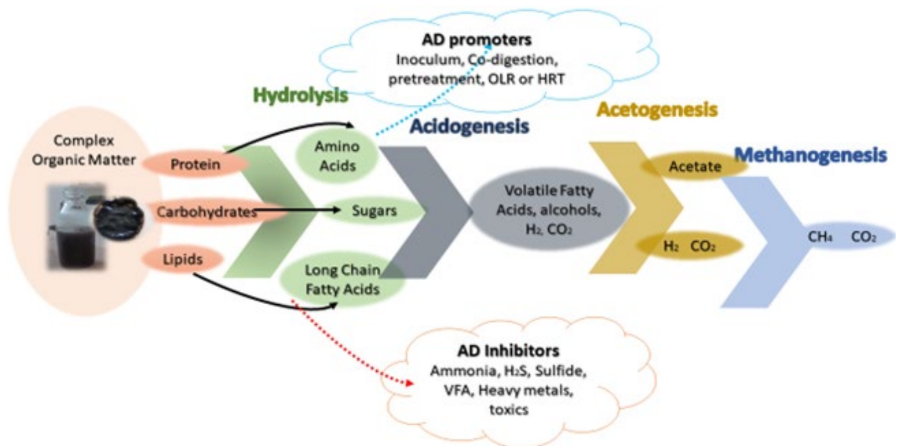
Figure 4.1: A simplified schematic presentation of the anaerobic digestion phases, adapted from (Salihi et al., 2018)
