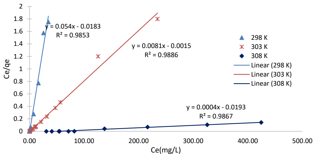
Figure 6.9: The Langmuir linear plots of C_e/Q_e versus C_e
