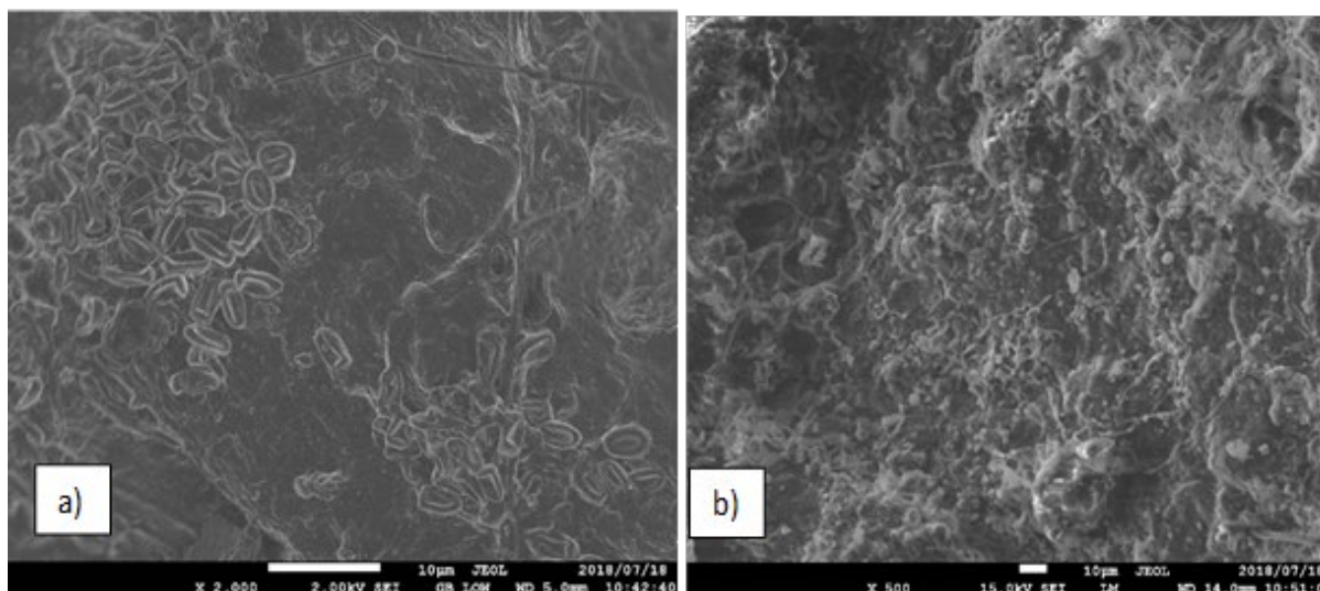
Figure 4.2: SEM micrographs of sewage sludge a) Raw sludge before anaerobic digestion b) Digested sewage sludge.
