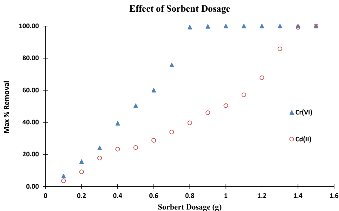
Figure 6.7: Effect of adsorbent dosage on adsorption of Cr (VI), Cd (II). Conditions: pH=10 for Cd (II); pH=2.0 for Cr (VI); 250 mg/L adsorbate concentration; 24 hrs. contact time
