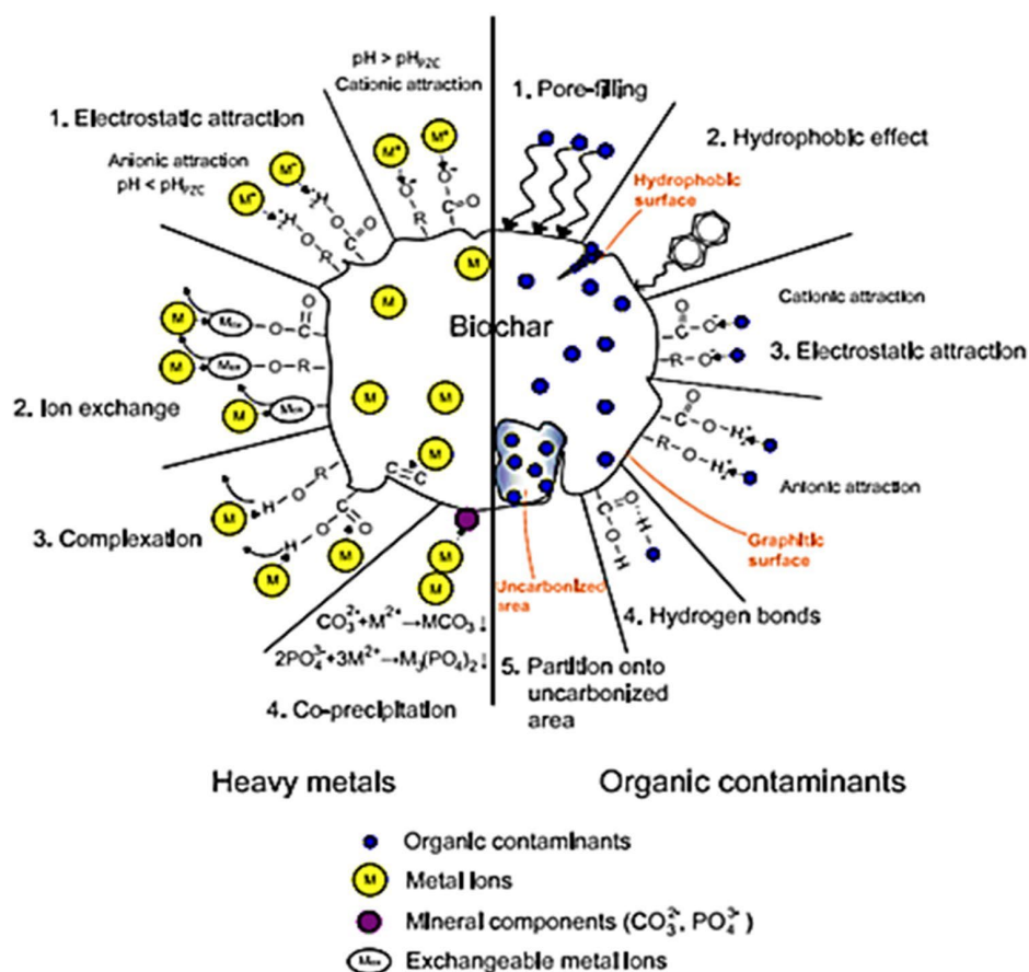
Figure 2.11: Adsorption mechanism of organic pollutant on biochar surface (Ahmad, et al. 2014).
