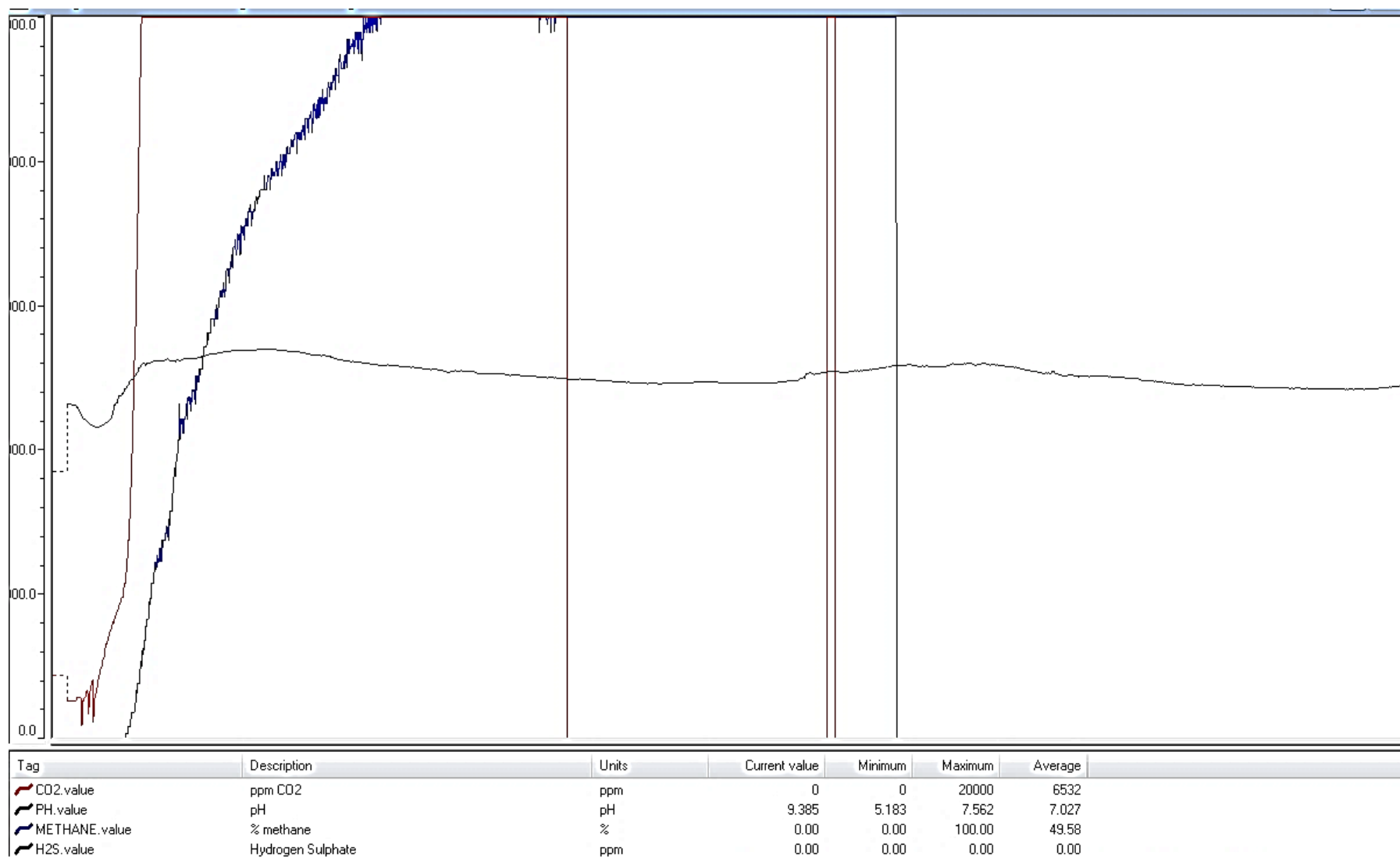
Figure 4.14: Pilot plant Trial 2 methane and carbon dioxide concentration and pH profile
