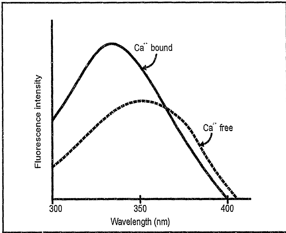
Figure 2.1 Excitation spectra of \text{Ca}^{2+} bound and \text{Ca}^{2+} free forms of fura-2 (emission wavelength = 510nm).
