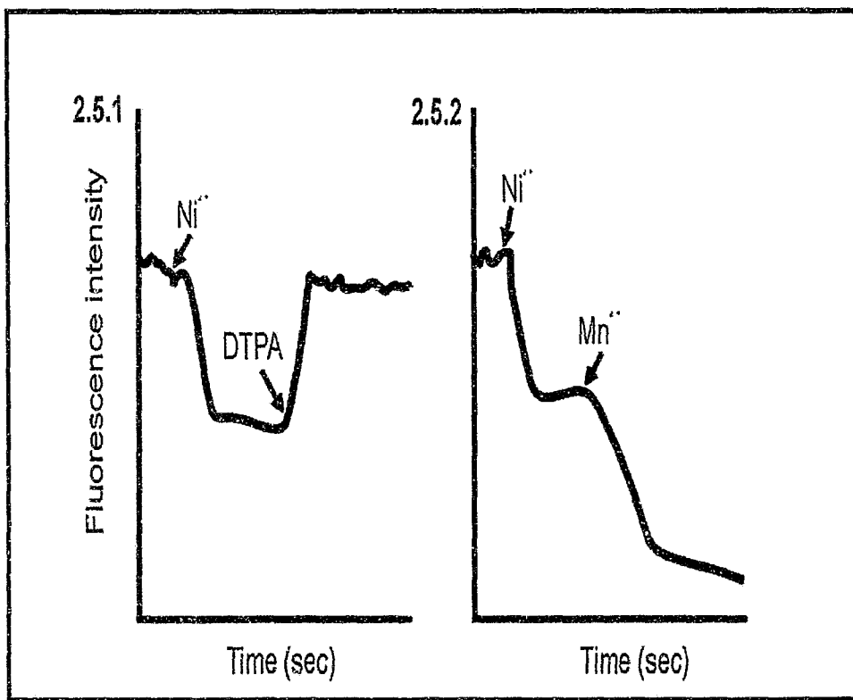
Figure 2.5 The effect of Ni^{2+} on the fura-2 fluorescence quench.
