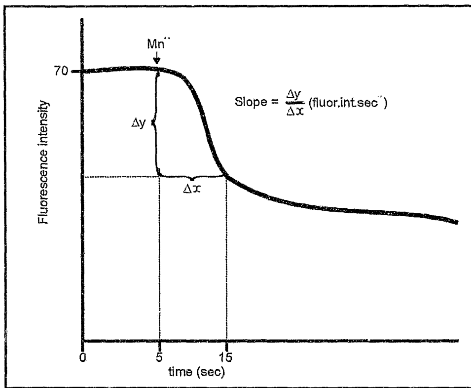
Figure 2.3 The calculation of Mn^{2+} influx into platelets by the rate of fura-2 fluorescence quenching.
