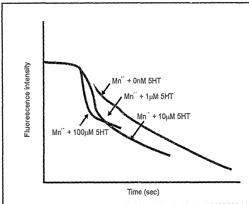
Figure 2.6 The effect of 5HT on the quenching rate of fura-2 by manganese.
