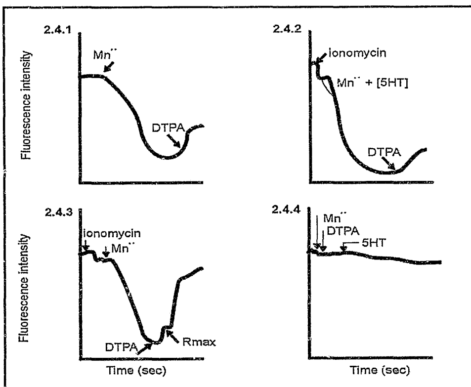
Figure 2.4 Evaluation of manganese influx into platelets.
