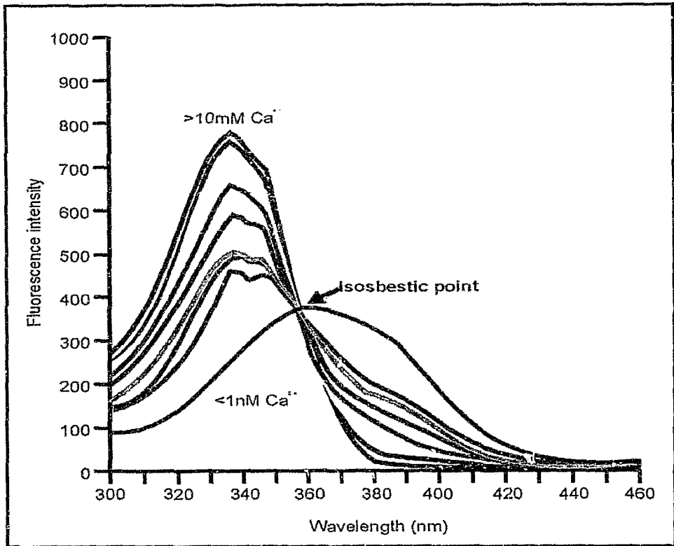
Figure 2.2 Excitation spectra for 4 \mu\text{M} fura-2-AM at 20°C in buffer with free \text{Ca}^{2+} values ranging from <1nM to >10mM.
