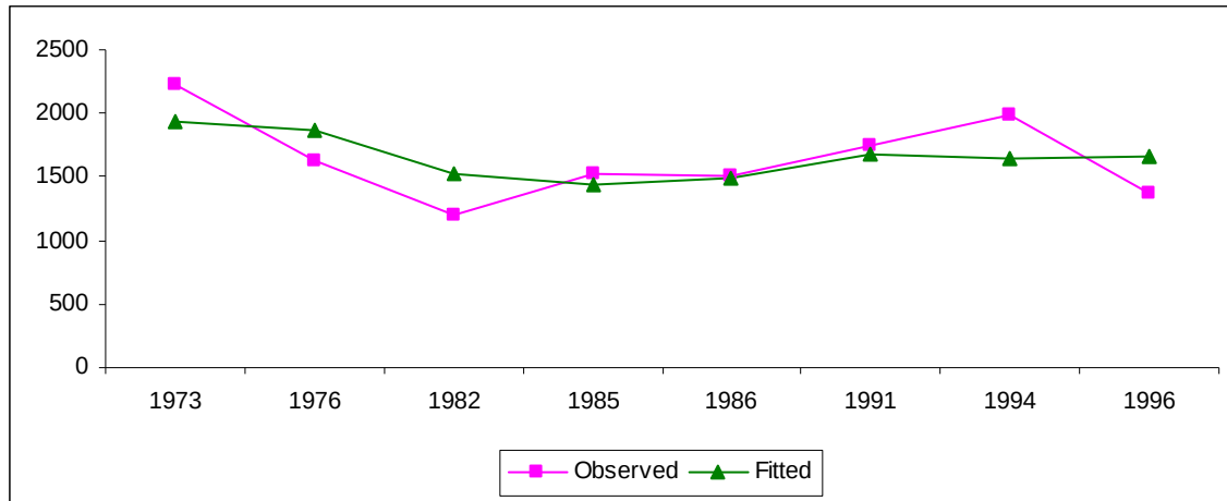
Figure 4.5: Plot of the bootstrap estimates of the true population sizes and the survey estimates for each of the eight surveys for 1000 replications
