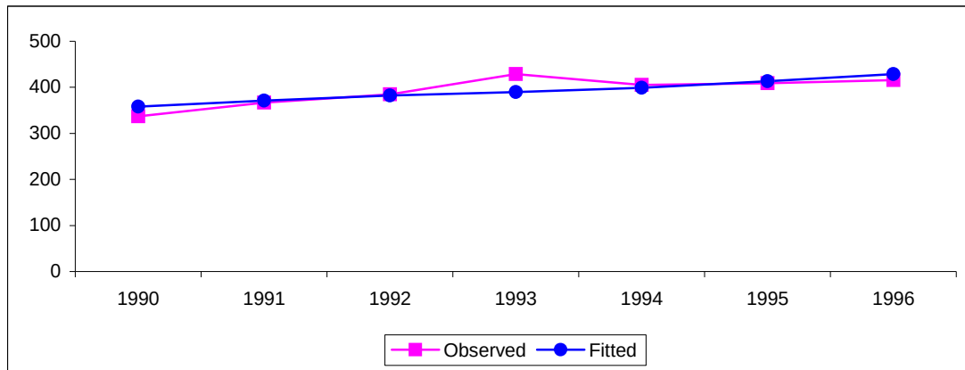
Figure 5.2: Plot of the bootstrap estimates of the true population sizes and the survey estimates for each of the seven surveys for 200 replications
