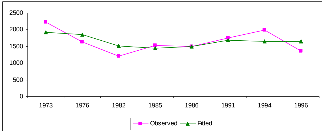
Figure 4.2: Plot of the bootstrap estimates of the true population sizes and the survey estimates for each of the eight surveys for 200 replications
