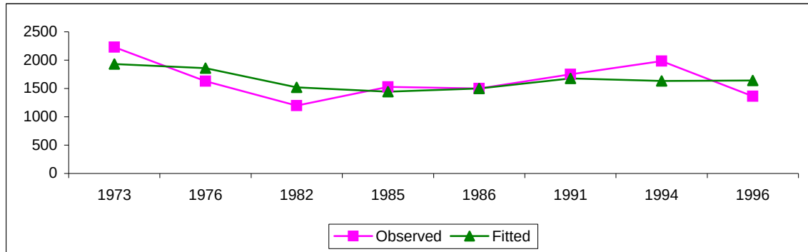
Figure 4.1: Plot of the estimated true population sizes and the survey estimates at each of the eight surveys
