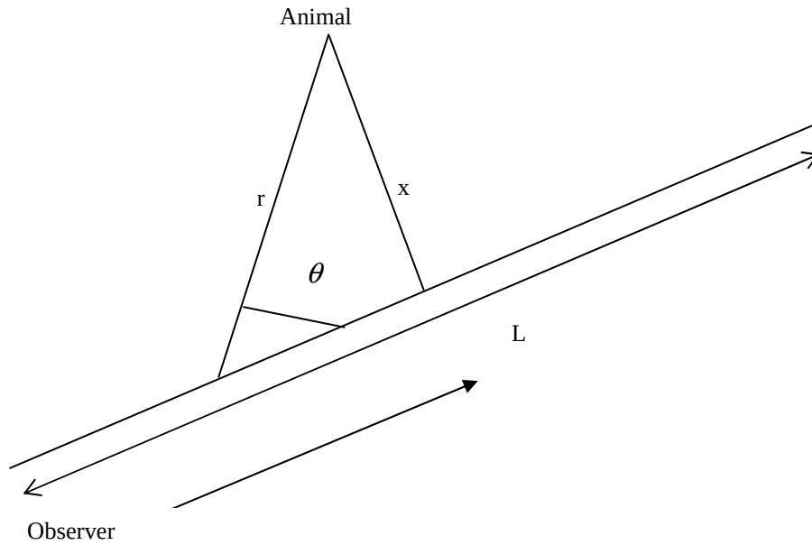
Figure 2.1: Example of line transect sampling and measurement
