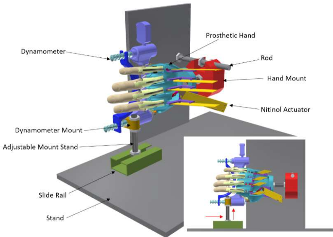
Figure 6.3: Finger Grip Strength Test Rig
