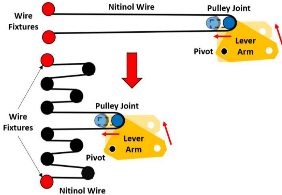
Figure 9.1: Modified Nitinol Actuator Layout
