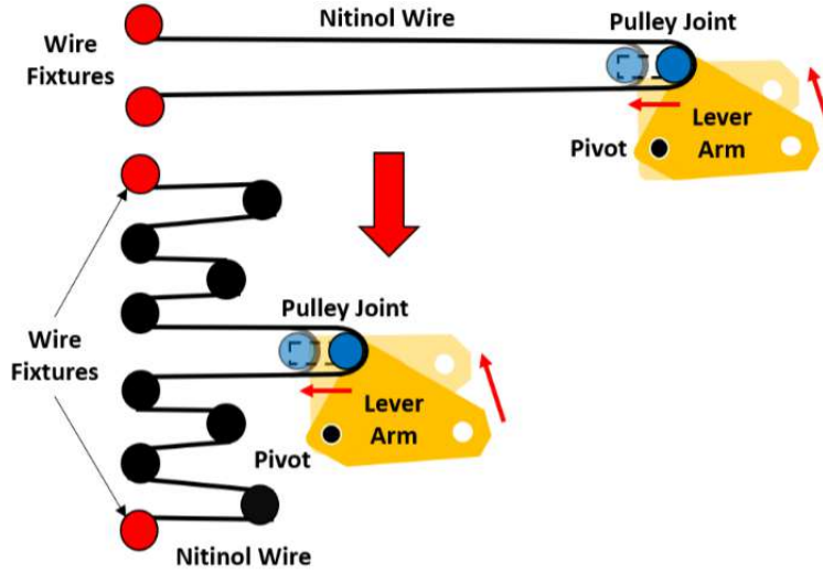
Figure 2.5: Modified Nitinol Actuator Layout
