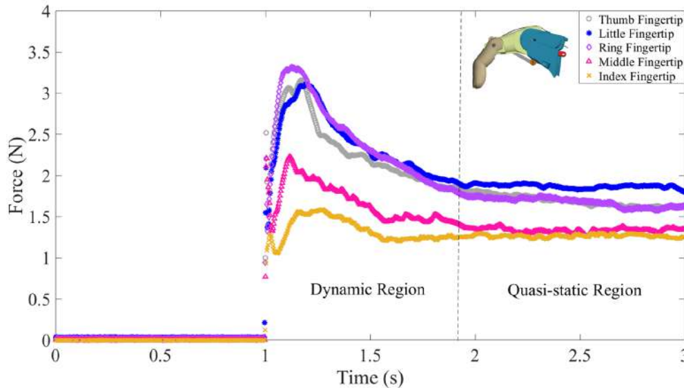
Figure 6.5: Fingertip Contact Force with a PIP Angle of 30^\circ
