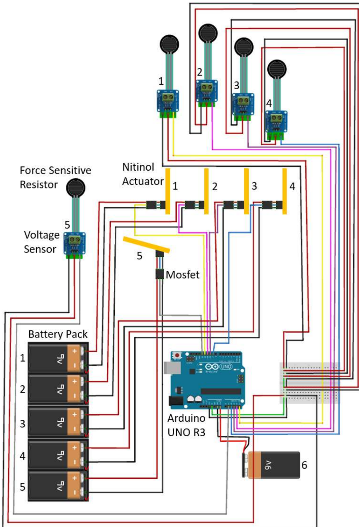
Figure 4.9: Prosthetic Hand Circuit
