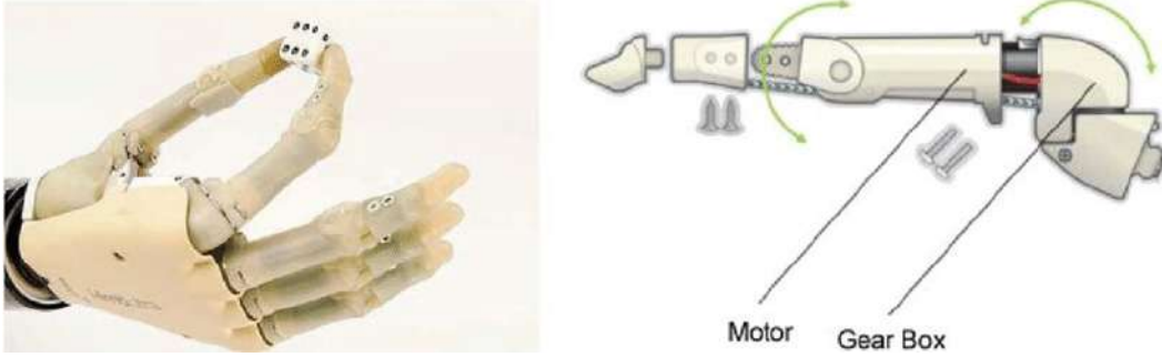
Figure 1.4: iLimb Hand [13]
