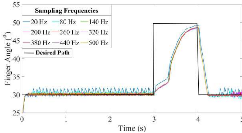
Figure 3.10: Step Signal with 6 V Input Voltage
