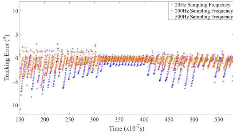
Figure 5.12: 11 V Ramp Signal Error
