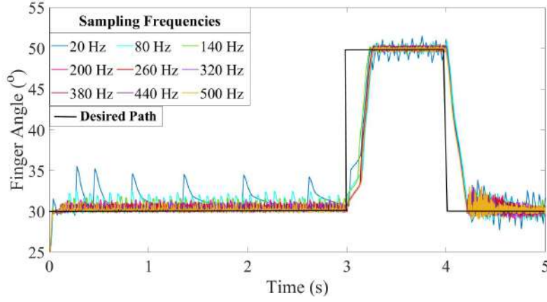
Figure 3.16: Step Signal with 12 V Input Voltage
