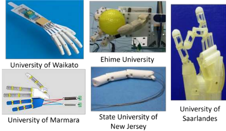
Figure 1.11: Past Nitinol Powered Prosthetic Hands [33, 34, 35, 36, 37]
