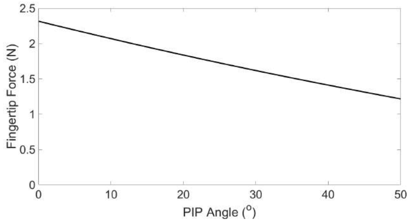
Figure 3.4: Fingertip Force vs PIP angle for Middle Prosthetic Finger
