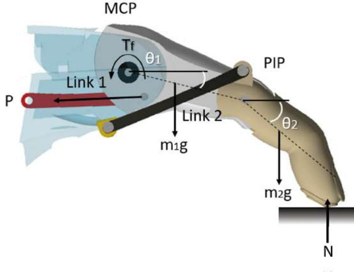
Figure 3.1: Free Body Diagram of Finger Mechanism
