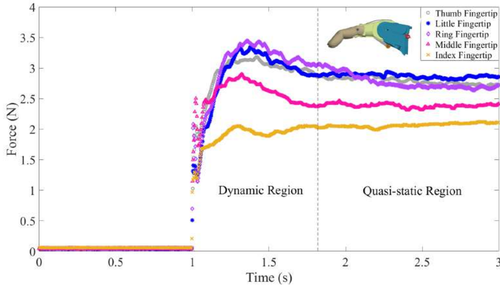
Figure 6.4: Fingertip Contact Force with a PIP Angle of 0^\circ
