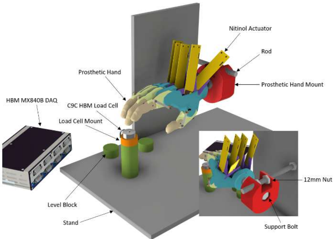
Figure 6.2: Fingertip Strength Test Rig
