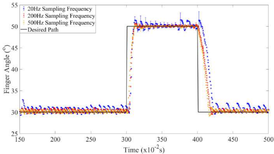
Figure 5.5: 9 V Step Signal
