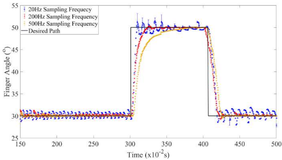
Figure 5.4: 7 V Step Signal
