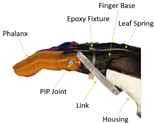
Figure 4.3: Finger Assembly Prototype
