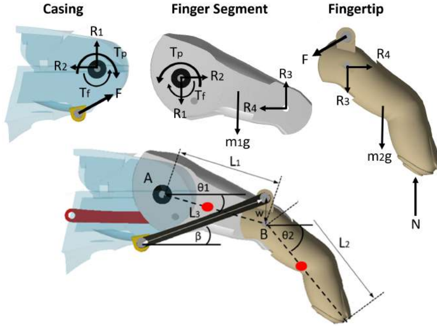
Figure 3.3: Detailed Free Body Diagrams of Finger Mechanism
