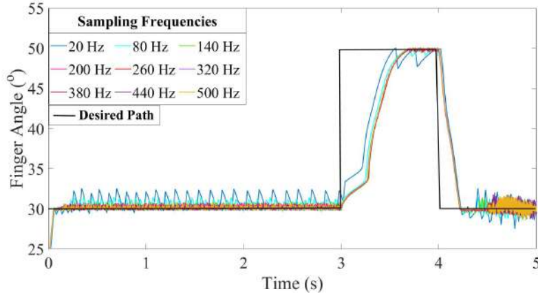
Figure 3.11: Step Signal with 7 V Input Voltage
