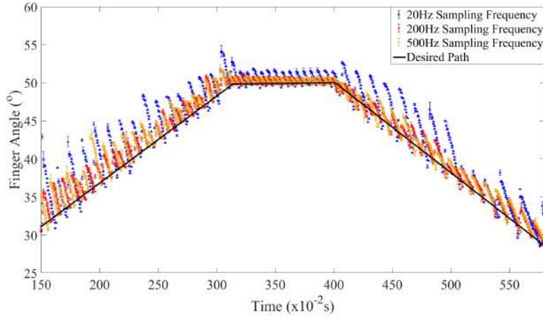
Figure 5.11: 11 V Ramp Signal
