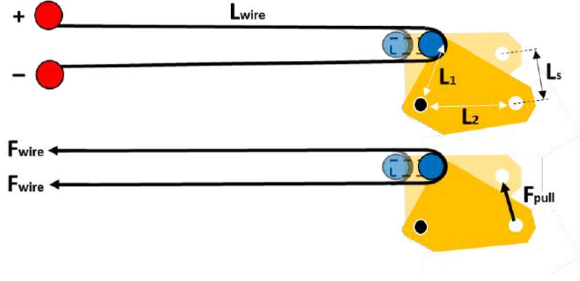
Figure 2.2: Nitinol Actuator Kinematic Diagram
