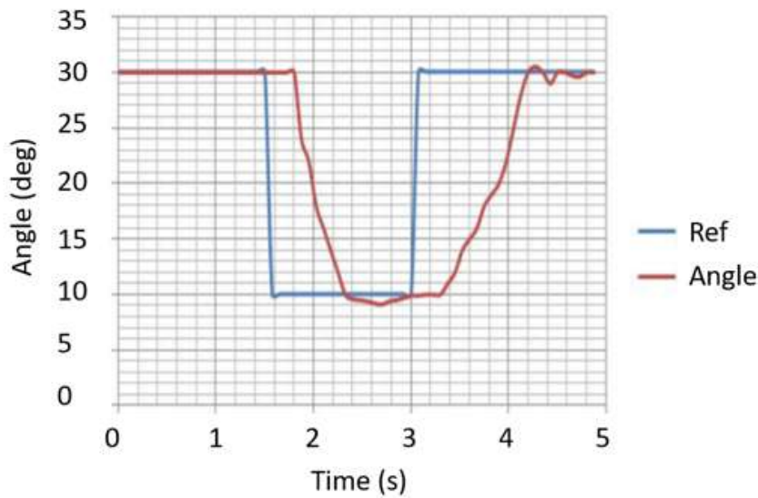
Figure 1.13: University of Marmara SMA Finger Response to Step Input [36]
