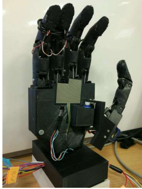
Figure 1.8: Wits prosthetic hand (Tact model) [6]
