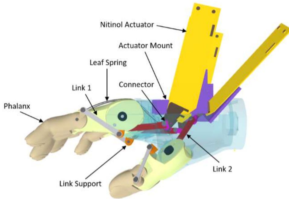
Figure 2.9: Actuation Scheme Configuration
