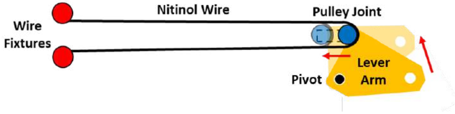
Figure 2.1: Nitinol Actuator Concept
