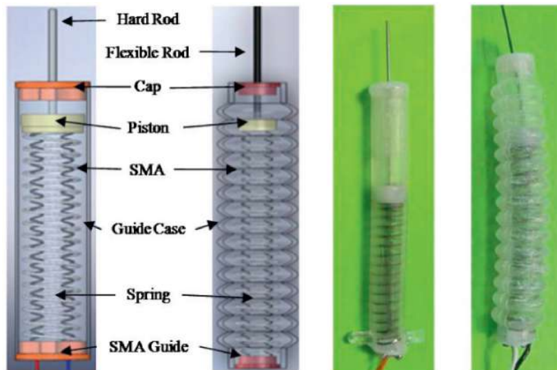
Figure 1.14: Tsuyama National College SMA Artificial Muscles [38]
