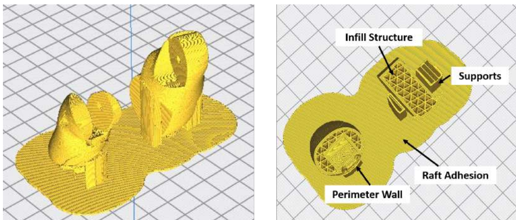
Figure 4.1: Sliced 3D Model for 3D Printing
