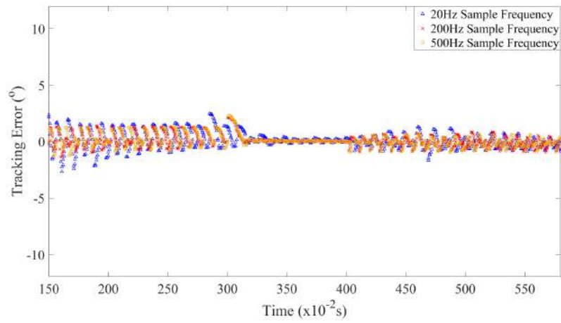
Figure 5.8: 7 V Ramp Signal Error
