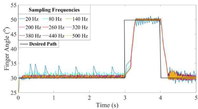
Figure 3.15: Step Signal with 11 V Input Voltage
