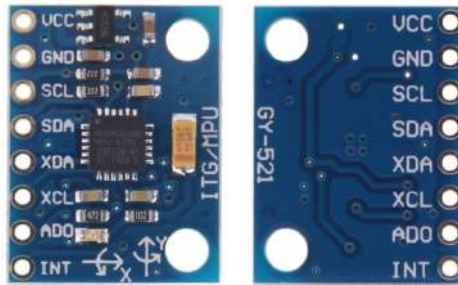
Figure 5.1: MPU6050 Sensor
