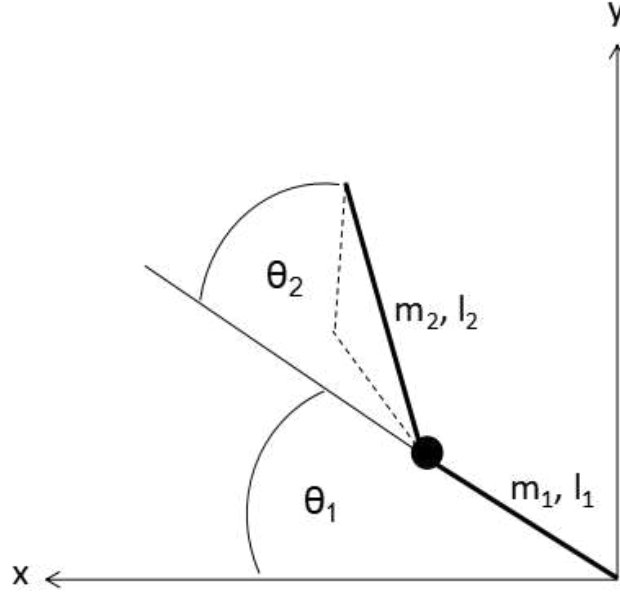
Figure 3.8: Simplified Link Diagram of Finger Mechanism
