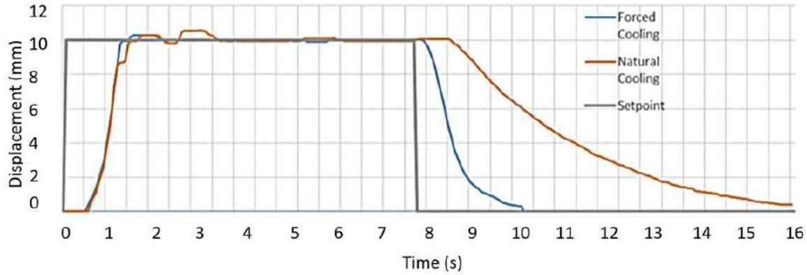
Figure 1.12: University of Waikato SMA Finger Response to Step Input [33]
