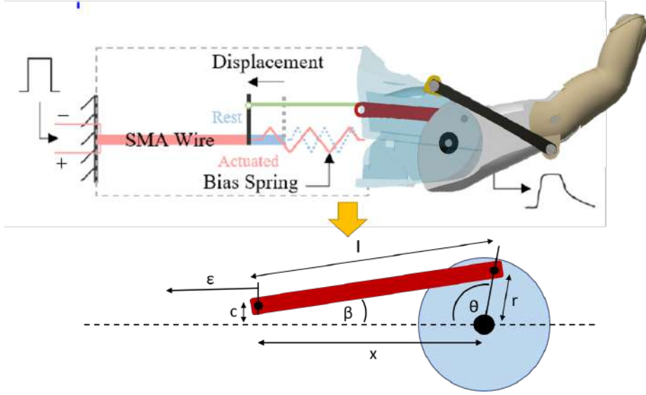
Figure 3.7: Crank-Slider Mechanism [43]
