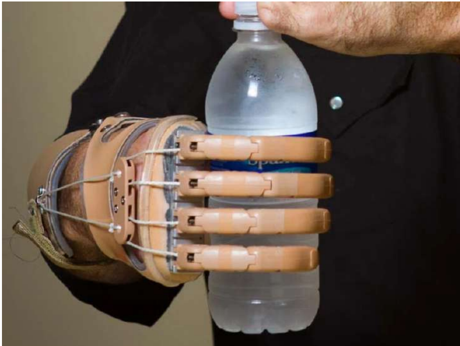
Figure 1.5: Body-Powered Prosthetic Hand [15]
