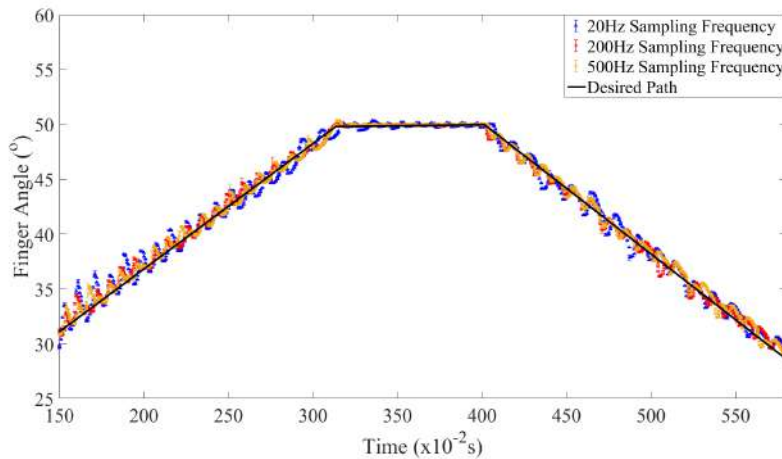
Figure 5.7: 7 V Ramp Signal
