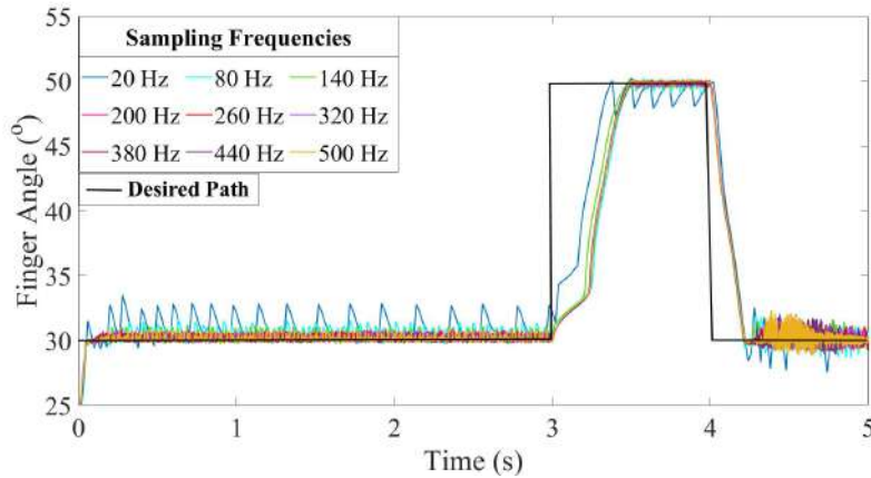
Figure 3.12: Step Signal with 8 V Input Voltage
