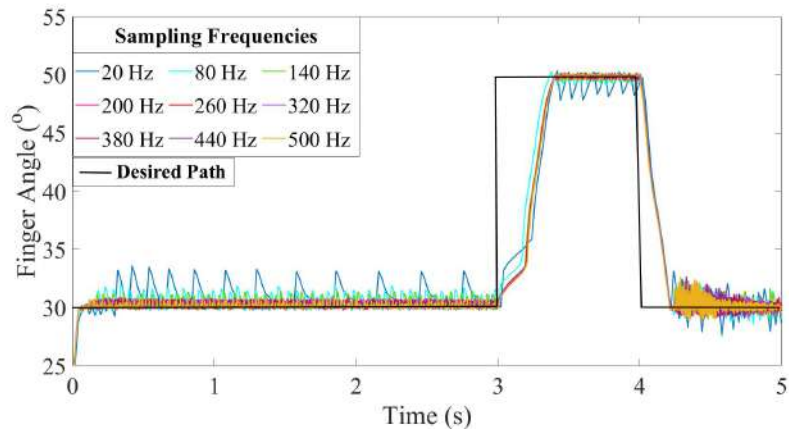
Figure 3.13: Step Signal with 9 V Input Voltage
