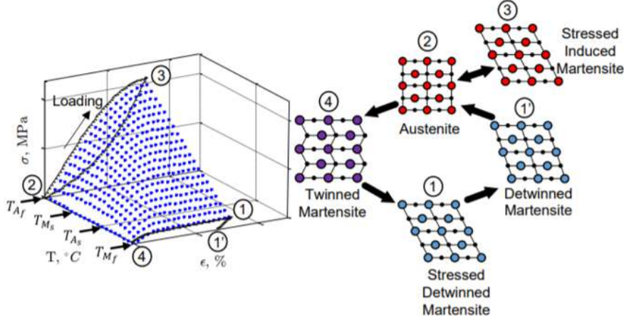
Figure 1.9: Stress-Strain-Temperature Curve [30]
