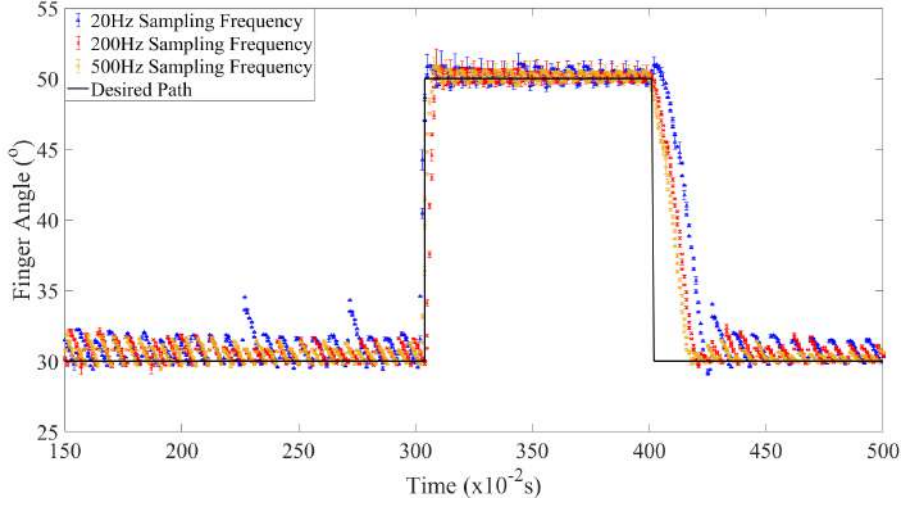
Figure 5.6: 11 V Step Signal
