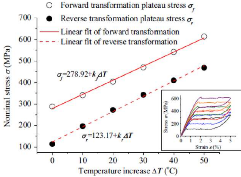
Figure 1.10: Temperature Dependence of the Isothermal Forward and Reverse Transformation Plateau Stresses ( k_f and k_r are constants with values 6.56 MPa/°C and 7.09 MPa/°C, respectively) [31]
