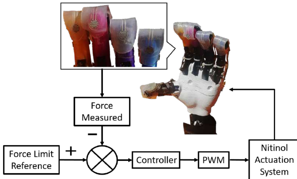
Figure 4.6: Adaptive Grip Control Loop
