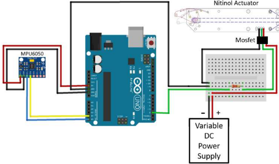
Figure 5.3: Finger Positioning Test Circuit
