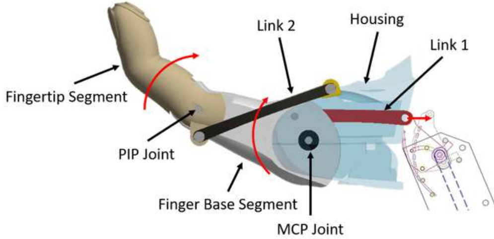
Figure 2.6: Two-Link Finger Mechanism
