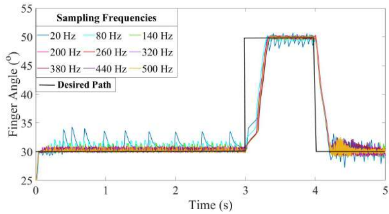
Figure 3.14: Step Signal with 10 V Input Voltage
