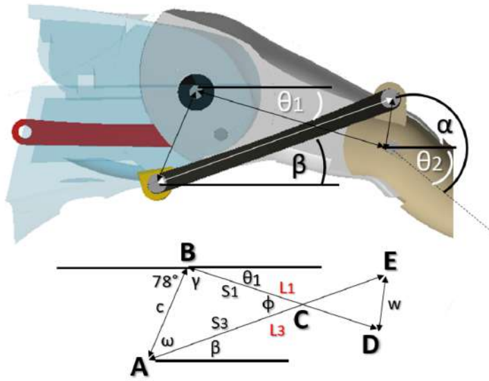
Figure 3.2: Link 2 Orientation with respect to the Finger Base Position Diagram
