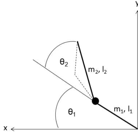
Figure C.1: Simplified Link Diagram of Finger Mechanism
