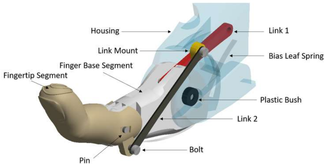
Figure 2.7: Two-link Finger Mechanism Assembly
