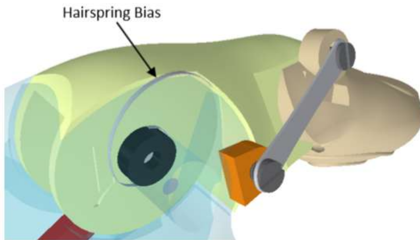
Figure 2.10: Hairspring Bias
