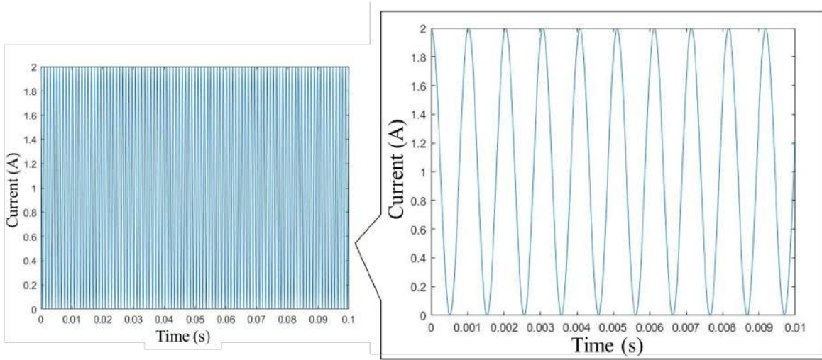
Figure 3.6: Input Current Signal with a 980 Hz PWM Frequency
