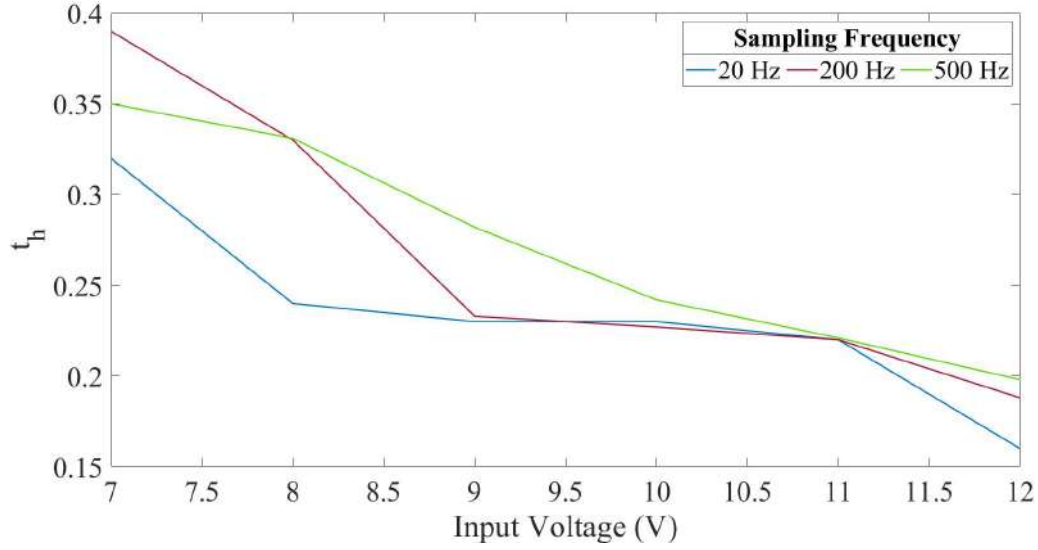
Figure 3.18: Time Constant (Heating) vs. Input Voltage
