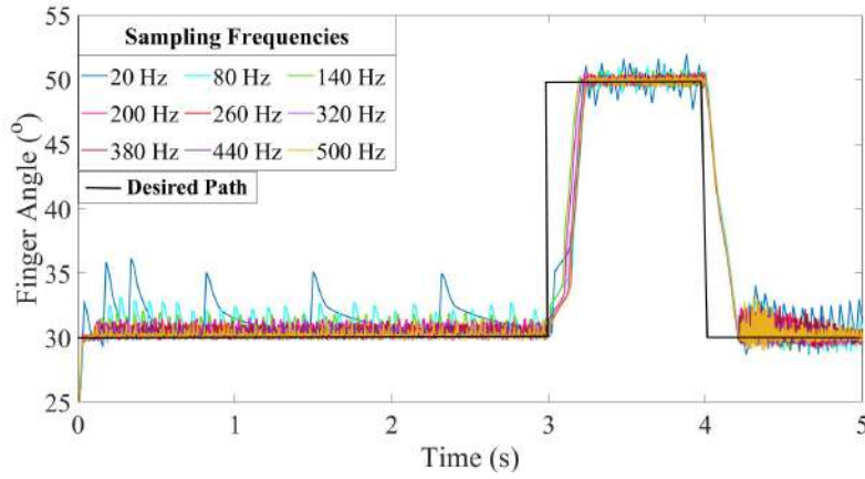
Figure 3.17: Step Signal with 13 V Input Voltage
