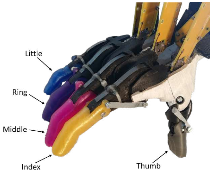
Figure 6.1: Labelled Prosthetic Fingers
