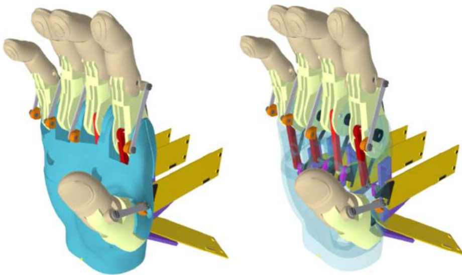
Figure 2.8: Prosthetic Hand Assembly
