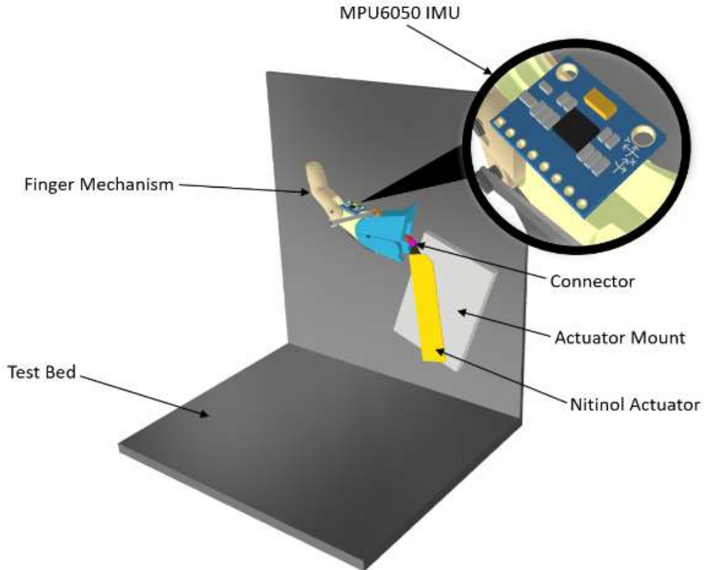
Figure 5.2: Finger Positioning Test Apparatus
