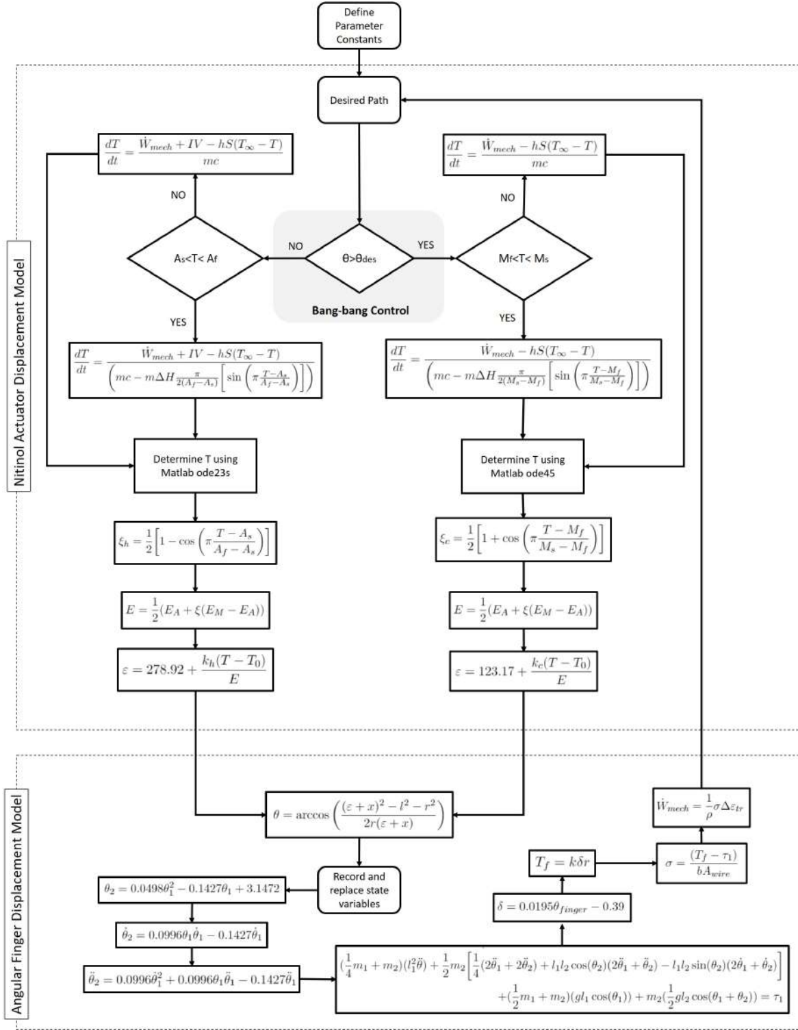
Figure 3.9: Matlab Code Architecture for Bang-Bang Controlled Nitinol-Driven Finger
