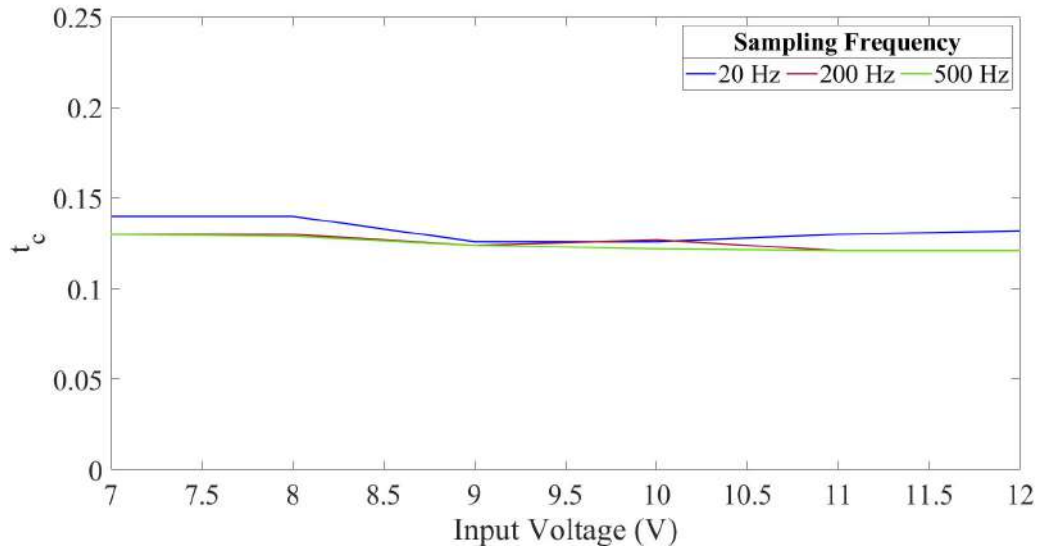
Figure 3.19: Time Constant (Cooling) vs. Input Voltage
