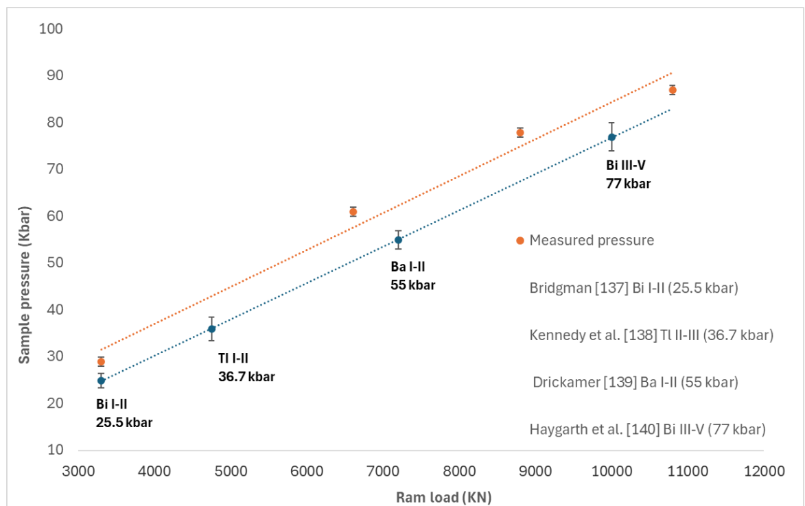
Figure 5.2: Comparison of the pressure calibration curve with reported values for fixed-point pressure transitions [18]
