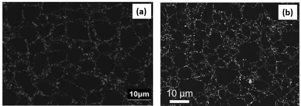
Figure 8.1: SEM-BSE images of PDC samples produced at: (a) calibrated pressure of 7 GPa, 1500°C and 20 minutes, (b) 5.5 GPa and 1450°C by Westraadt et al. [107], showing cobalt pools (medium grey contrast), diamond (dark contrast) and tungsten carbide (light grey contrast)
