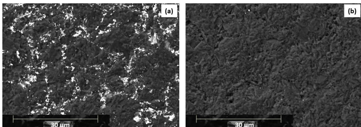
Figure 4.3: SEM-BSE images of the sintered PDC samples showing: (a) unleached and (b) leached, with cobalt pools (light contrast), porosity (dark contrast) and diamond (medium dark contrast). Experimental run conditions: 5 GPa, 1500°C and 25 minutes
