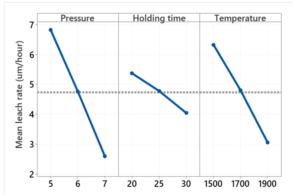
Figure 7.1: Main effects plot for leach rates of PDCs for pressure, holding time and temperature, horizontal dashed lines represent overall mean leach rate
