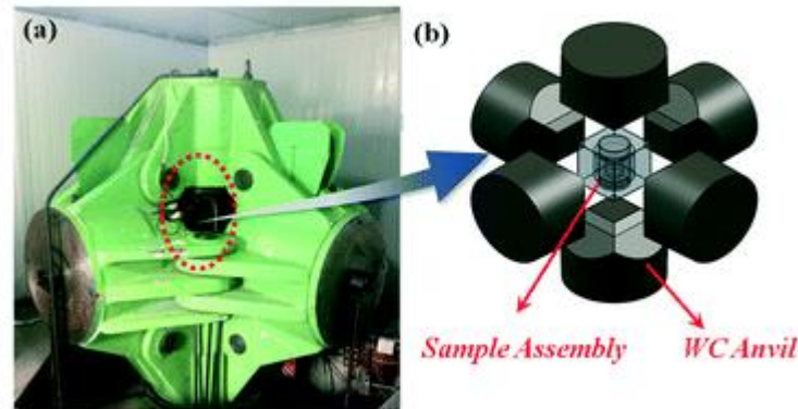
Figure 2.2: (a) HPHT press, (b) sample assembly [23]
