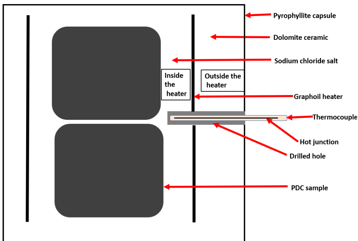
Figure 3.2: Schematic diagram of the sample assembly in the capsule with an S-type thermocouple inserted into the drilled hole on the side of the capsule
