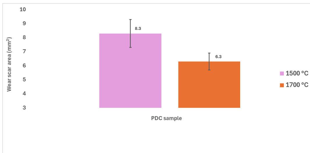
Figure 6.3: Wear scar area of leached PDC cutters sintered at different sintering temperatures
