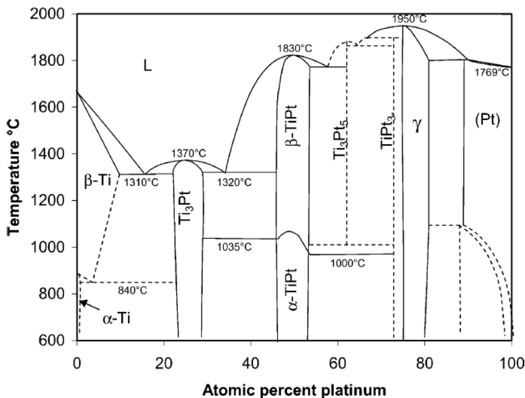
Figure 8.3: Ti–Pt phase diagram by Murray [141]
