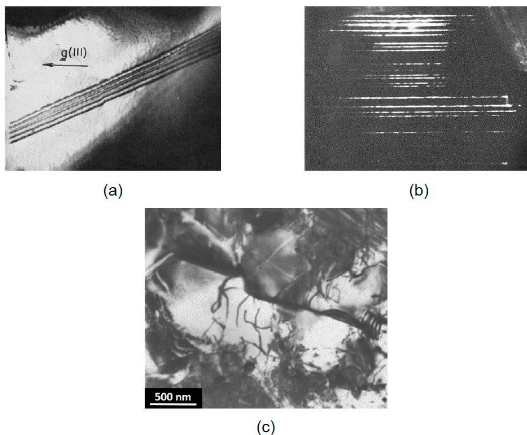
Figure 2.7: TEM micrographs showing: (a) stacking faults; (b) micro-twinning and (c) low dislocation density of diamond intergrowth [145]
