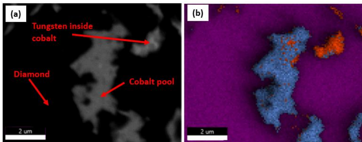
Figure 4.5: unleached sample: (a) SEM-BSE image showing diamond (dark), cobalt (medium grey) and tungsten (light) and (b) X-ray map showing cobalt (blue), tungsten (orange) and diamond (purple)
