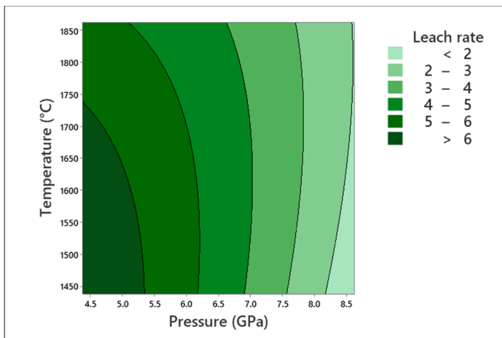
Figure 7.4: Contour plot for effect of pressure (GPa) and temperature (°C) on leach rate ( \mu\text{m/h} ) at a fixed holding time
