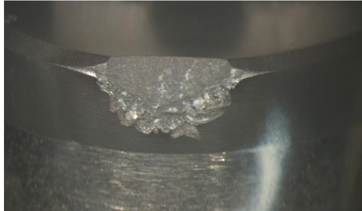
Figure 3.4: Typical image of a wear scar of the PDC after VTL test for the experimental run conditions: 5 GPa, 1500°C and 25 minutes
