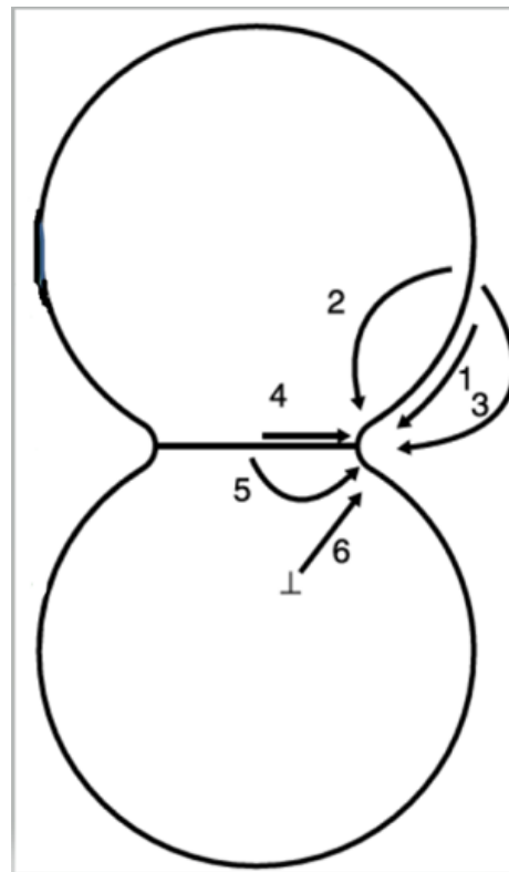
Figure 2.6: Sintering mechanisms for joining of two particles [32]
