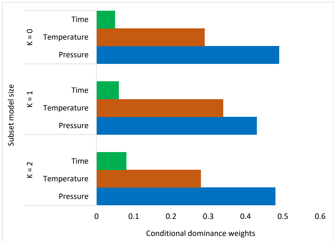
Figure 7.7: Conditional dominance weights for the of sintering variables at different subset size models
