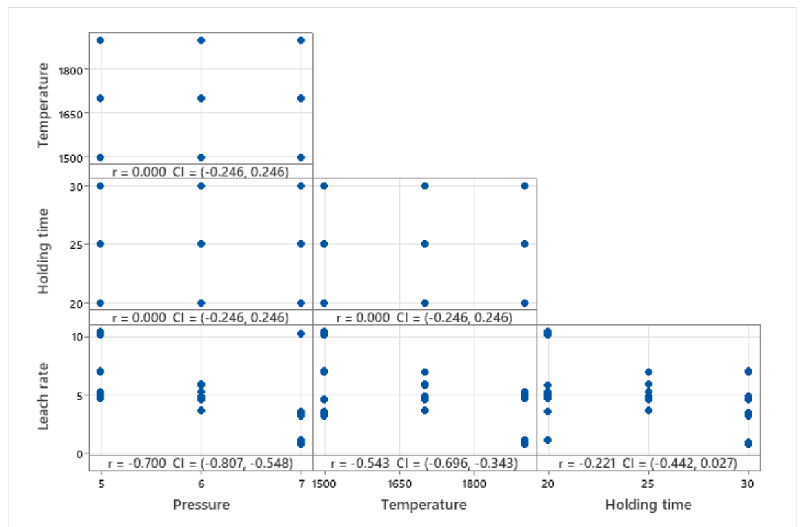
Figure 7.3: Correlation matrix showing the relationships between pressure (GPa), temperature (°C), holding time (minutes) and leach rate ( \mu\text{m/h} ), with Pearson correlation coefficients ( r ) and their 95% confidence intervals (CI) for each pair
