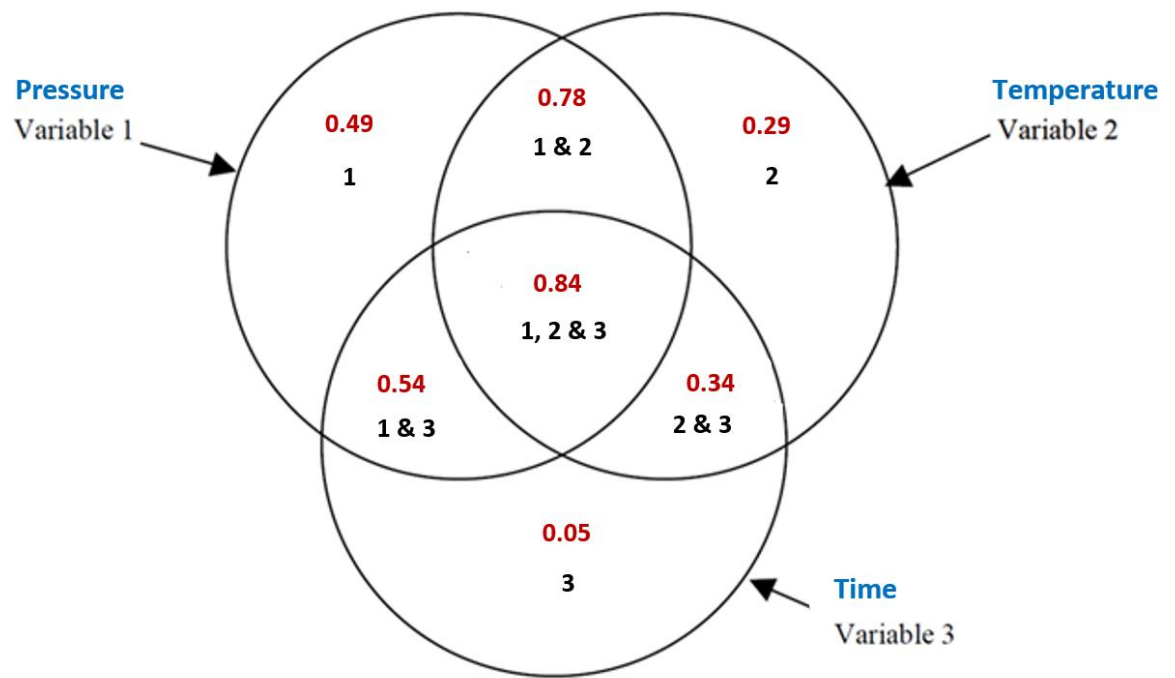
Figure 7.6: Venn diagram showing the complete dominance weights for the effect of sintering variables on the leachability of PDC
