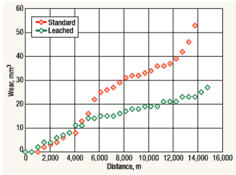
Figure 2.10 Wear behaviour for leached and non-leached PDCs subjected to a VTL test [66]
