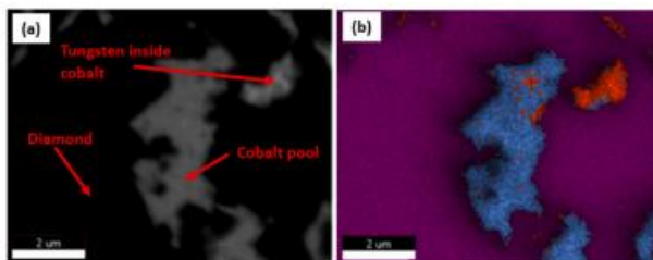
Fig. 2. 6 GPa sample: (a) SEM-BSE image showing diamond (dark), cobalt (medium grey) and tungsten (light) and (b) X-ray map showing cobalt (blue), tungsten (orange) and diamond (purple). (For interpretation of the references to colour in this figure legend, the reader is referred to the web version of this article.)
