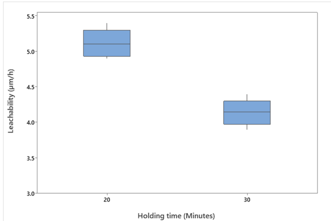
Figure 6.2: Boxplot analysis on the effect of holding time on leachability after 96 h leaching in HCl acid
