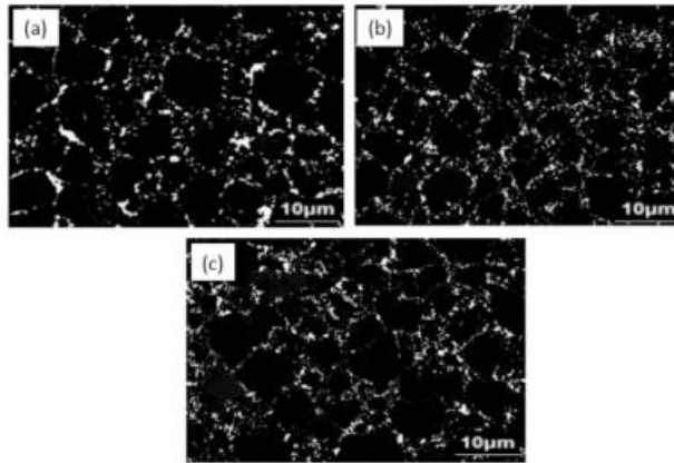
Fig. 3. SEM-EDS images of PDC binder pools at the top of the layer at different pressures: (a) 5 GPa, (b) 6 GPa and (c) 7 GPa, showing cobalt pools (light contrast) and diamond (dark contrast).
