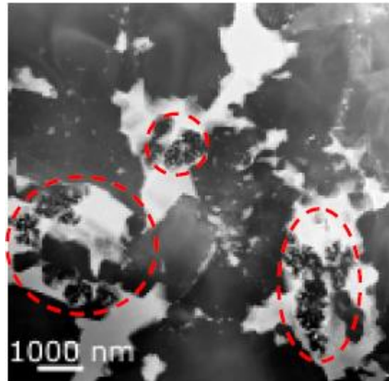
Figure 2.8: TEM image showing degraded cobalt pools after exposure to 700 °C for 2 h, with graphite outlined by red circles [28]
