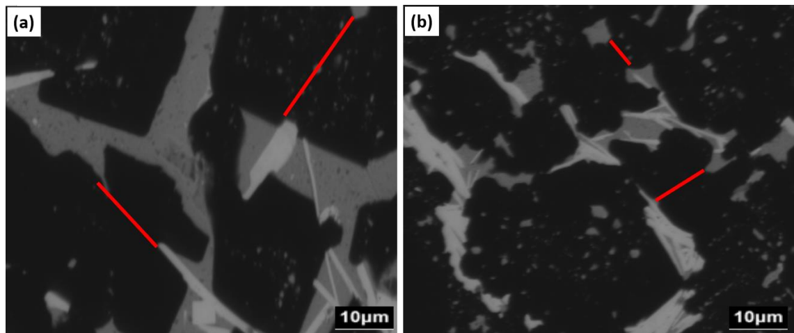
Figure 8.4: SEM-BSE images of PDC samples, taken from the bottom of the diamond layer near the interface, sintered for: (a) 20 minutes and (b) 30 minutes, showing cobalt pools (medium grey contrast), diamond (dark contrast) and tungsten carbide (light grey contrast). Red lines show interfaces between diamond grains. Sintering pressure and temperature were 7 GPa and 1500°C (Figure 4.1)
