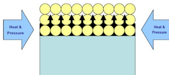
Figure 2.3: Cobalt binder migration [23]
