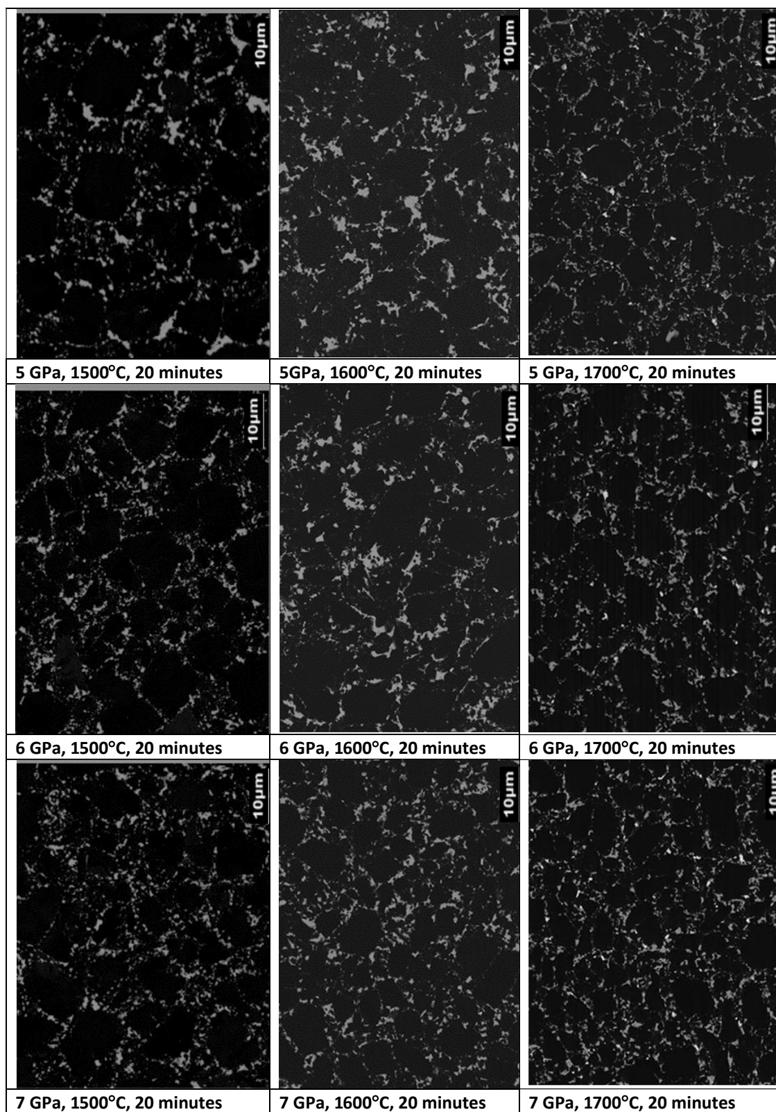
Figure 4.1: SEM-BSE images showing the effect of sintering variables on the microstructures of the diamond layer, showing: cobalt pools (medium grey contrast), diamond (dark contrast) and tungsten carbide (light grey contrast)
