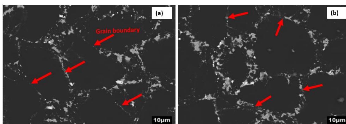
Figure 5.6: SEM-BSE images of the PDC samples sintered with two different thermocouple positions: (a) inside the heater (b) outside the heater, showing well-defined grain boundaries (red arrows), showing diamond (dark contrast), tungsten carbide (light contrast) and cobalt (medium grey contrast). The sintering conditions were 6 GPa, 1500°C and 20 minutes
