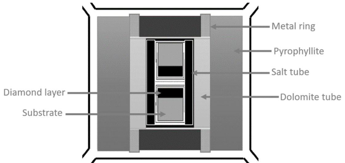
Figure 3.1: A cubic press capsule [22]
