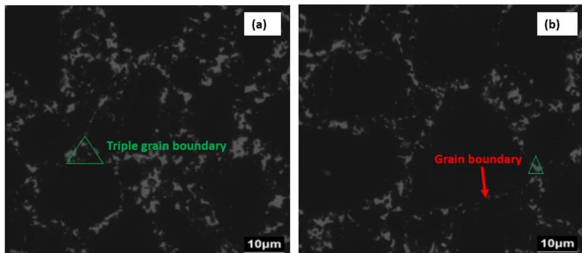
Figure 8.6: SEM-BSE images of PDC samples, taken from the middle of the diamond layer, sintered for: (a) 1500°C and (b) 1700°C, showing cobalt pools (medium grey contrast) and diamond (dark contrast) with well-defined grain boundaries (red arrow). Sintering pressure and holding time were 7 GPa and 20 minutes (Figure 4.1)
