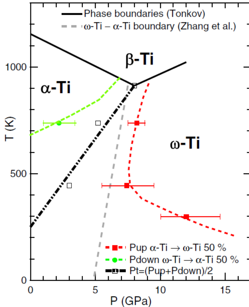
Figure 8.2: High-pressure phase diagram of titanium [108]
