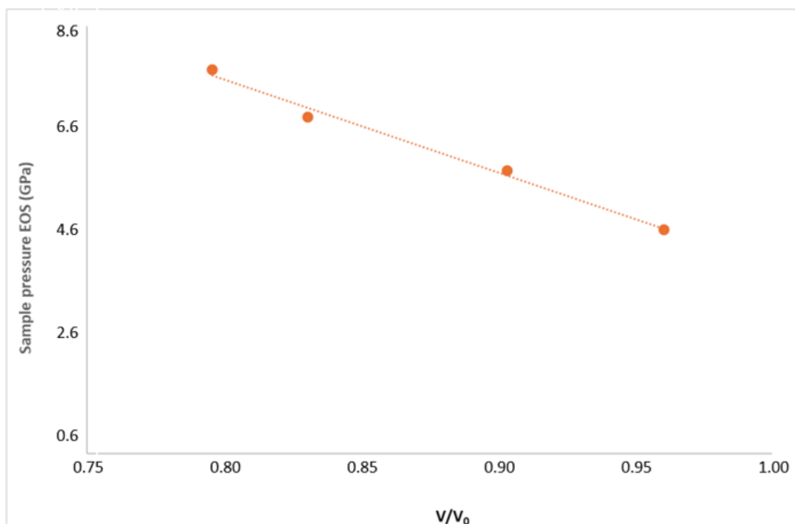
Figure 5.1: Relationship between sample pressure, calculated from the Murnaghan equation of state (EOS), and measured relative volume ( V/V_0 ) for the PDC samples. The dashed line is a linear fit to the calculated data
