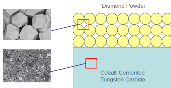
Figure 2.1: Diamond powder and WC substrate placed inside the sample assembly [23]
