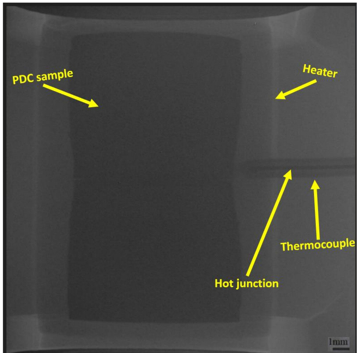
Figure 5.5: X-ray radiographic image of the sample assembly with a thermocouple inserted, showing heater (light line contrast), PDC sample (dark contrast), and hot junction (black line). (Figure 3.6 shows a line drawing of this sample assembly)
