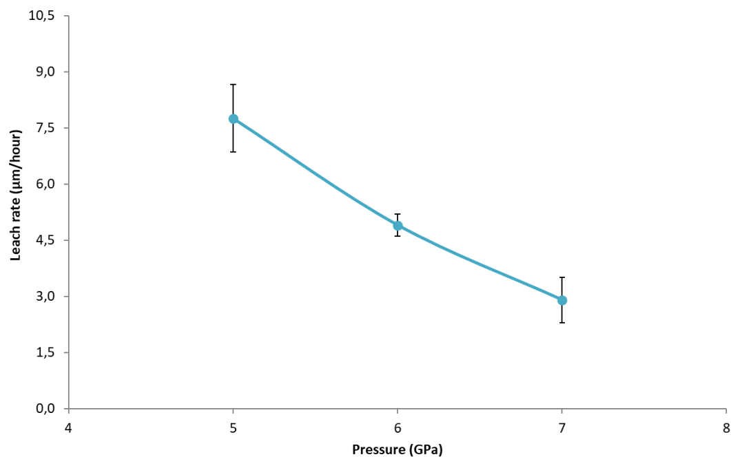
Figure 6.5: Relationship between leachability (leach rate) and sintering pressure after 96 h leaching in HCl acid
