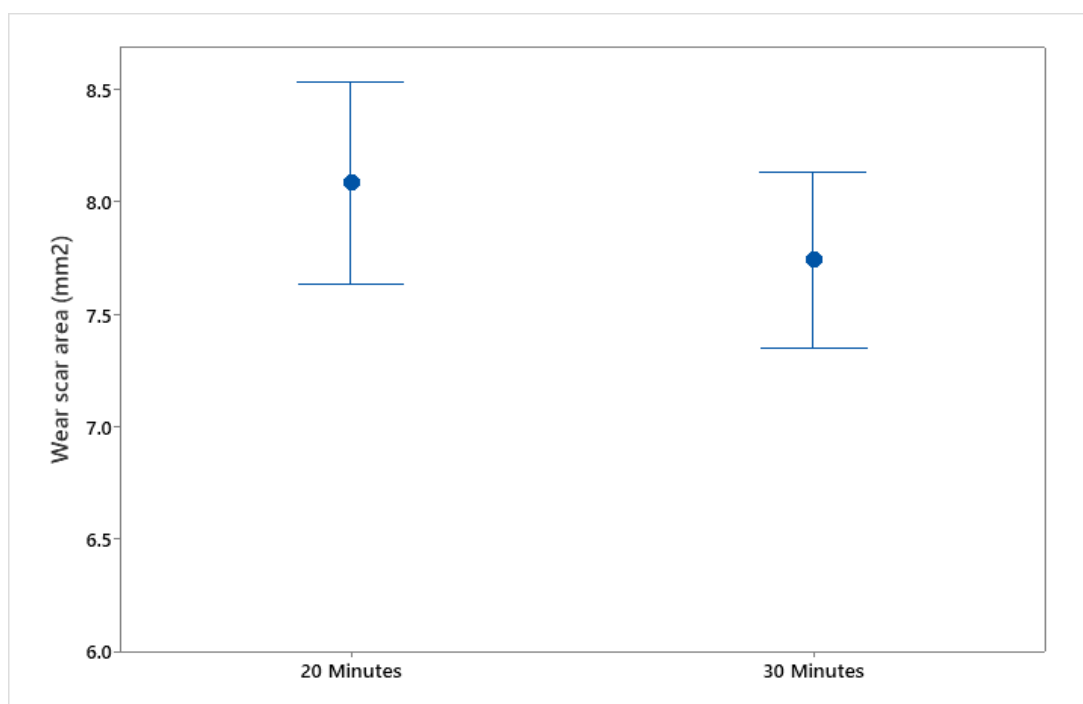
Figure 6.1: Wear scar areas of leached PDC cutters sintered at different holding times. Sintering pressure and temperature were fixed at 7 GPa and 1500°C
