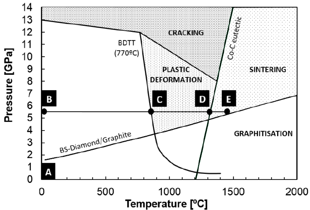
Figure 2.5: Sintering map for a cobalt based PDC [148]
