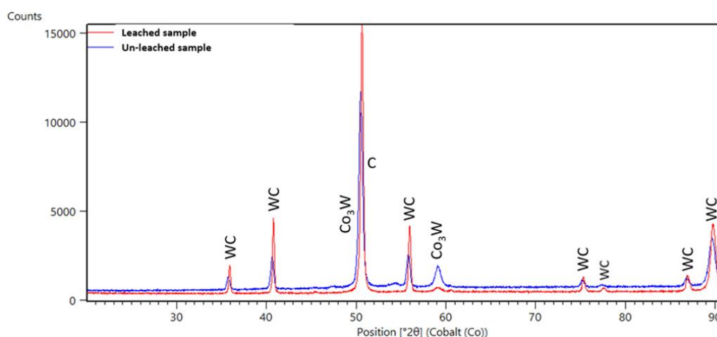
Figure 4.4: XRD patterns for the unleached and leached diamond layer samples.
