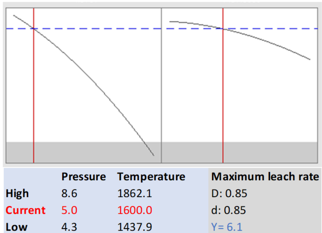
Figure 7.5: Optimisation plot showing the predicted leach rate ( \mu\text{m/h} ) as a function of pressure (GPa) and temperature ( ^{\circ}\text{C} ), showing maximum leachability achievable under the experimental boundary conditions tested, where: high = maximum value of the pressure and temperature, low = lowest value of the pressure and temperature and current = current value of the pressure and temperature
