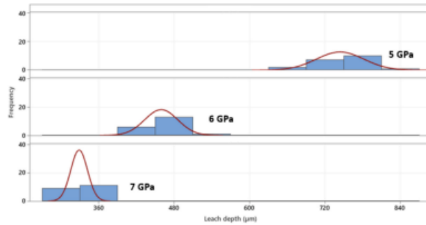
Fig. 5. ANOVA analysis of the leach depth measurements.
