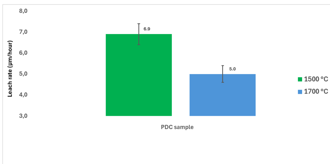
Figure 6.4: Effect of sintering temperature on leachability after 96 h leaching in HCl acid
