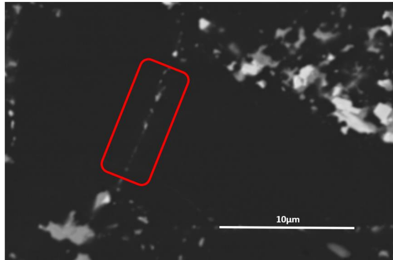
Figure 2.4: SEM-BSE image showing diamond-to-diamond bonding in PDC, showing cobalt pools (medium grey contrast), diamond (dark contrast) and tungsten carbide (light grey contrast) [28]
