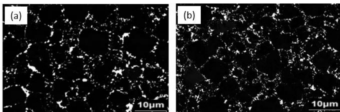
Figure 8.8: SEM-BSE images of PDC binder pools, taken from the middle of the diamond layer, sintered at different pressures: (a) 5 GPa and (b) 7 GPa, showing cobalt pools (light contrast), tungsten (grey contrast) and diamond (dark contrast). Sintering were 1500°C and 20 minutes (Figure 4.1)
