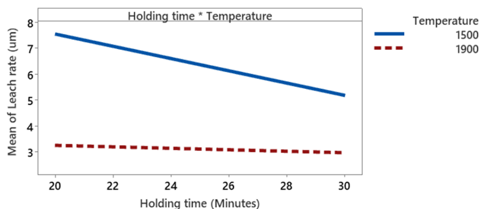
Figure 7.2: Interaction plot for holding time and temperature on leach rate
