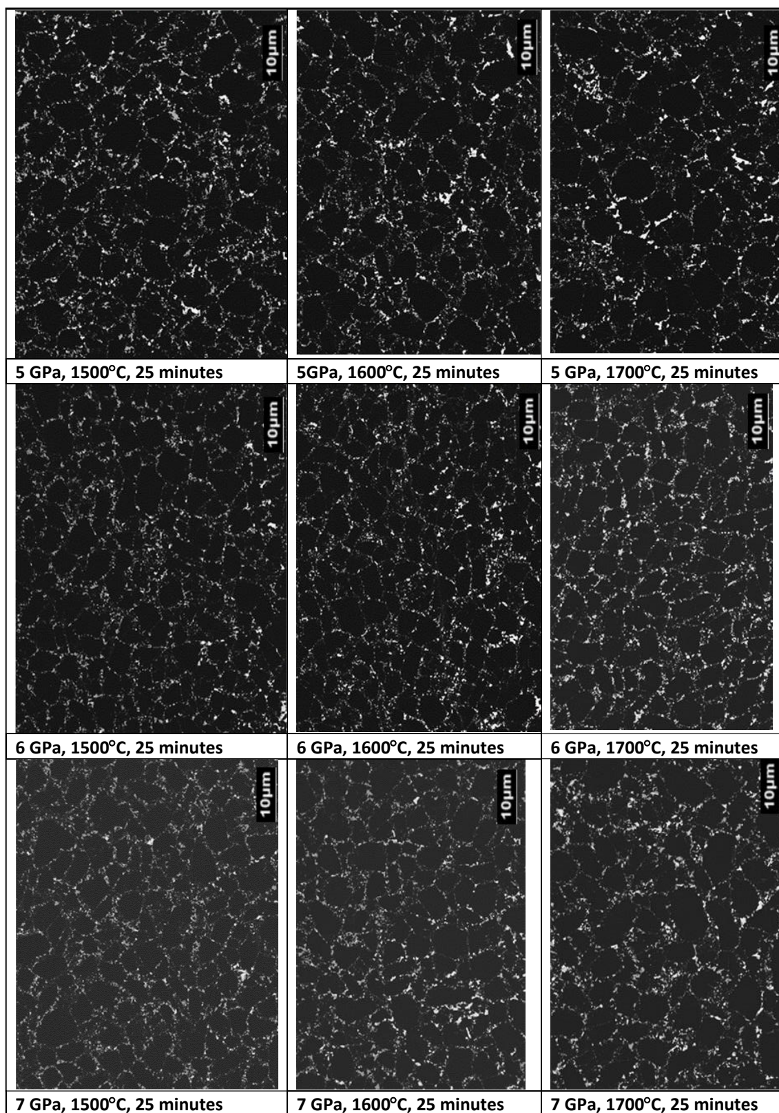
Figure 4.1 (continued): SEM-BSE images showing the effect of sintering variables on the microstructures of the diamond layer, showing: cobalt pools (medium grey contrast), diamond (dark contrast) and tungsten carbide (light grey contrast)
