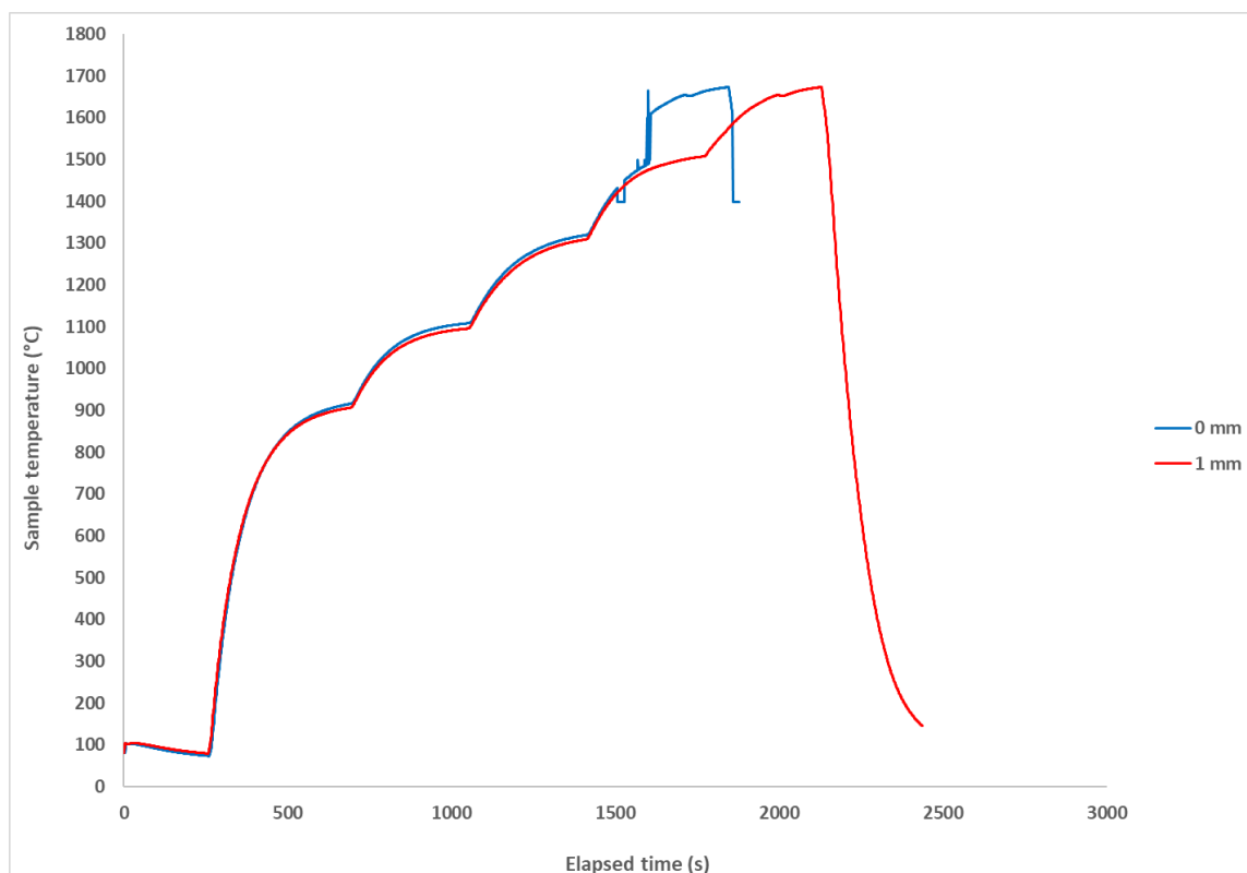
Figure 5.4: Effect of sample-thermocouple proximity on temperature measurement reliability
