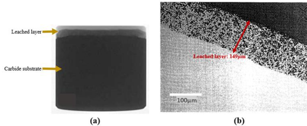
Figure 3.3: Leaching images showing: (a) X-ray tomography image of a leached sample and (b) Scanning electron microscope (SEM) image of the measured leached layer [13]
