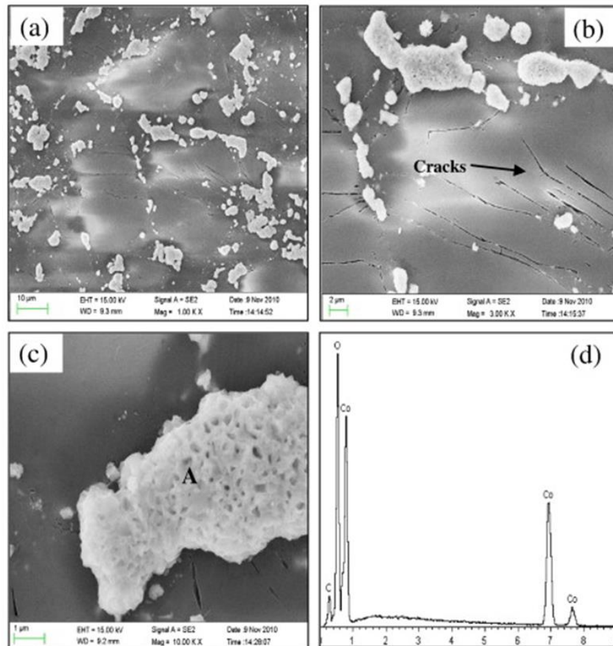
Figure 2.9: SEM-SE images of heat treated PDC at 900°C showing: (a) Co distribution, (b) micro-cracking, (c) Co 3 O 4 confirmed by (d) EDX analysis of cobalt [61]
