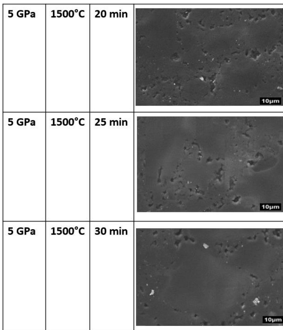
Figure 4.2 (continued): SEM-BSE images of leached and polished samples from nine experimental runs, showing: diamond (medium grey contrast), porosity (dark contrast) and tungsten carbide (light contrast)
