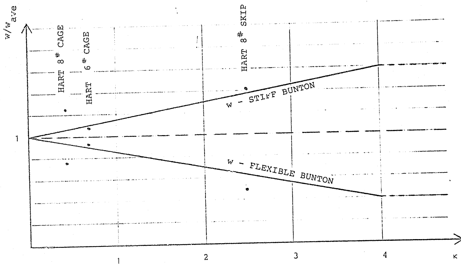
FIGURE 4.14 : Wheel load variation with buntion stiffness ratio
