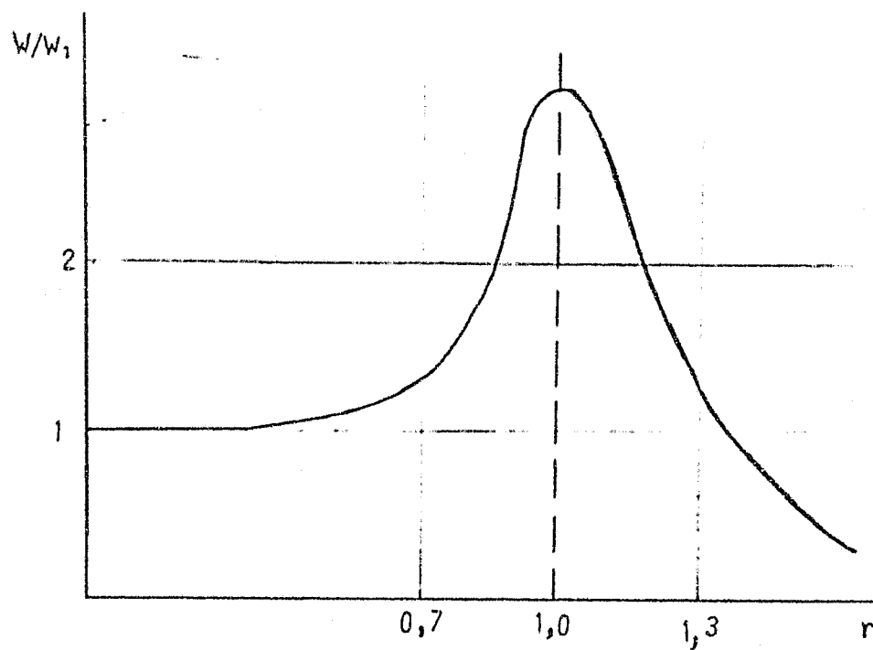
FIGURE 5.12 : Magnification Factor
