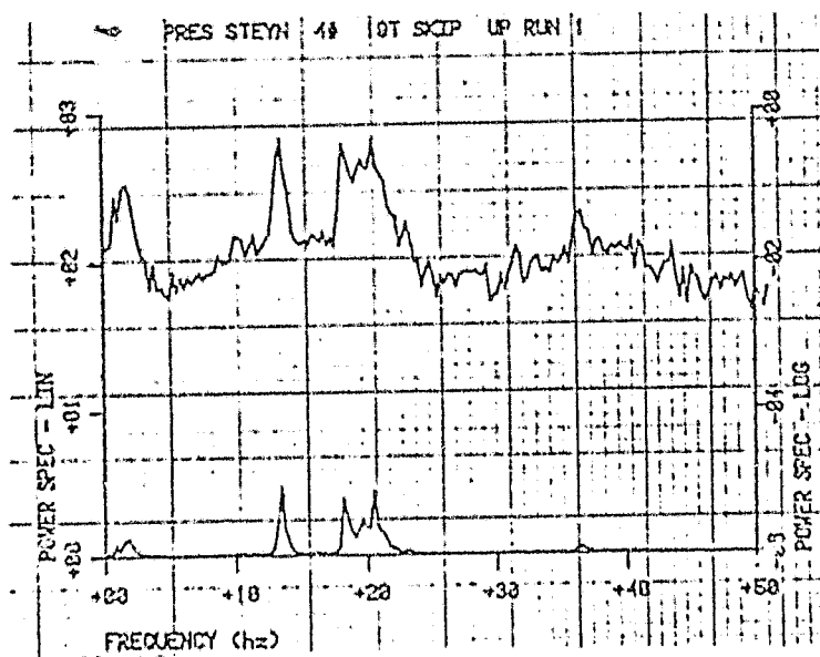
(c) Typical power spectrum of wheel loads
