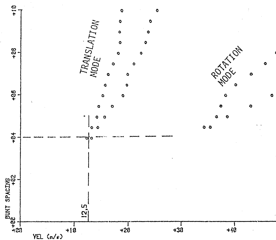
Figure 5.9 : Dynamic Magnification on Deelkraal No. 1 Shaft, 21 Tonne Skip.
