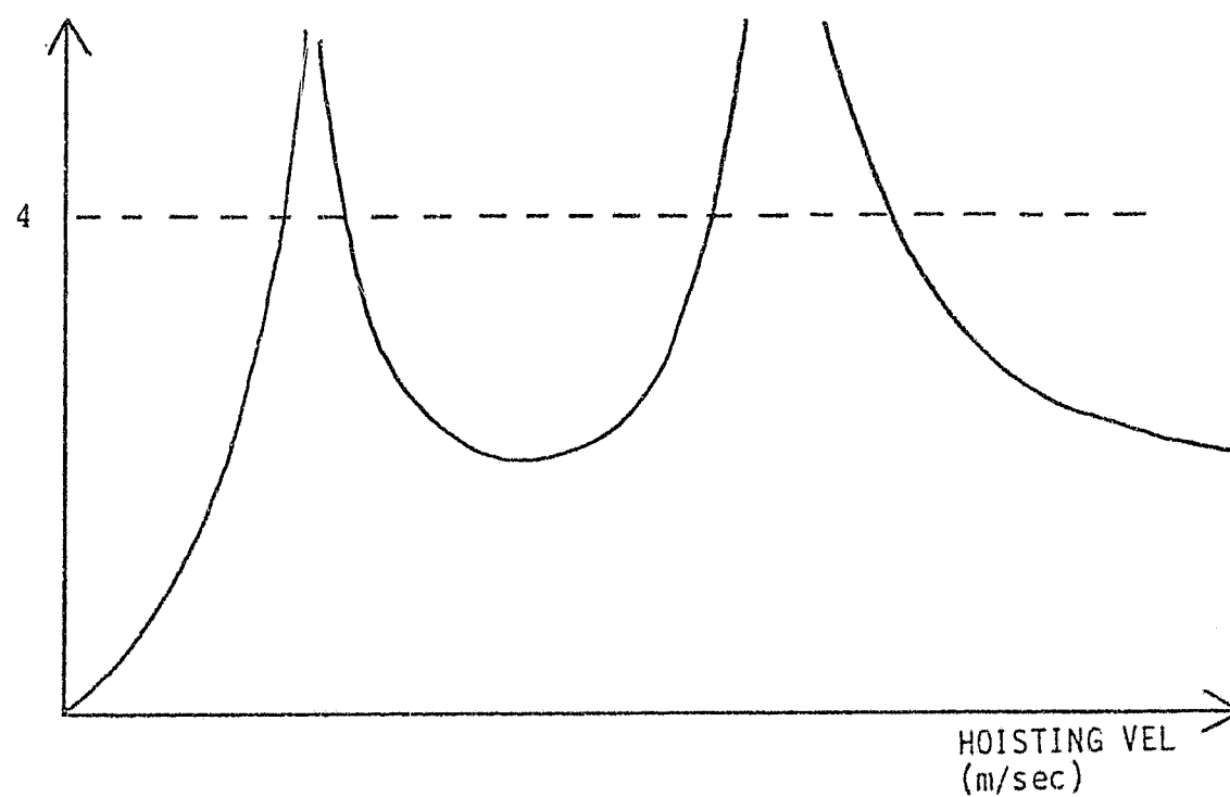
FIGURE 5.1 : Dynamic Magnification According to CSIR Report 9
