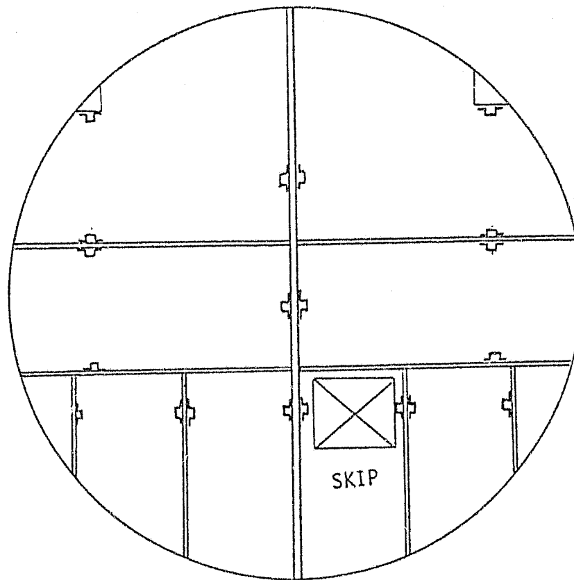
FIGURE 6.4 : Layout of Free State Geduld No. 5 Shaft
