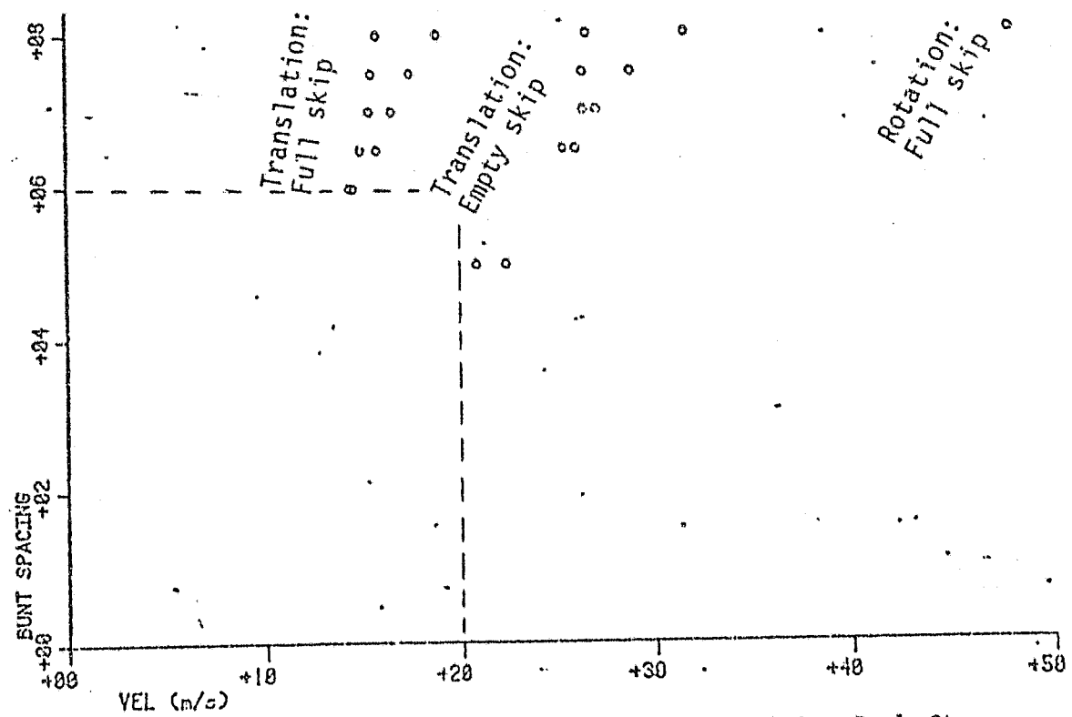
FIGURE 6.5 : DYNMAG dynamic predictions for F.S.G No. 5 shaft
