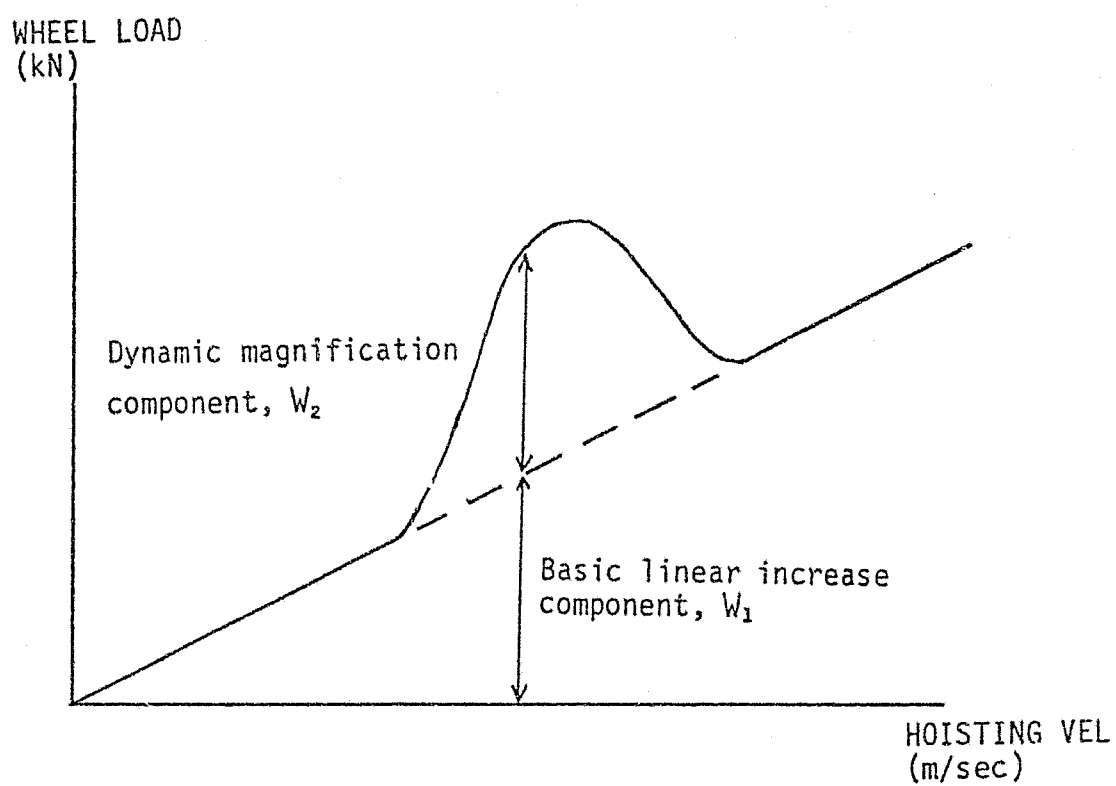
FIGURE 5.11: Dynamic Magnification Hump
