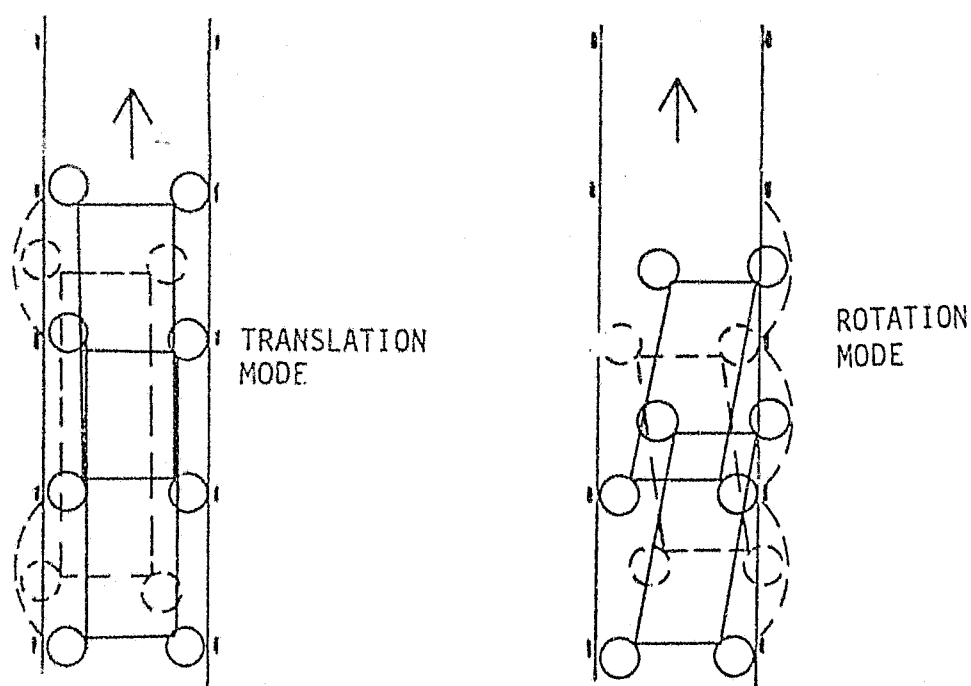
(a) LENGTH=(N) BUNTON SPACES (b) LENGTH=(N+½) BUNTON SPACES
