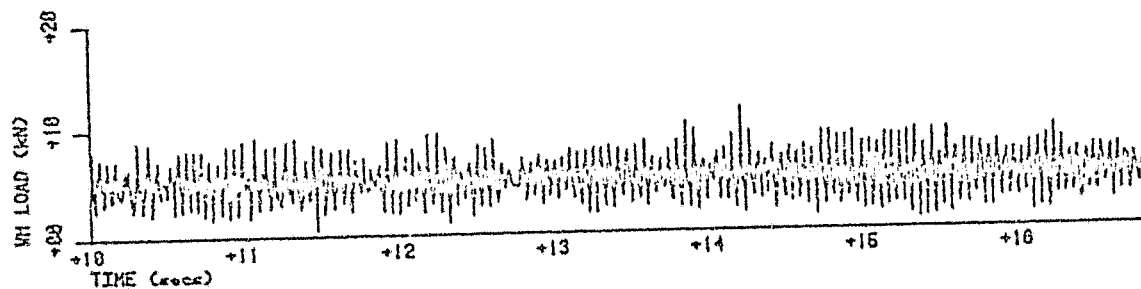
(b) Wheel loads on 10 tonne skip
