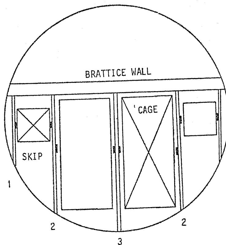
FIGURE 4.13 : Hartebeestfontein No. 8 shaft layout
