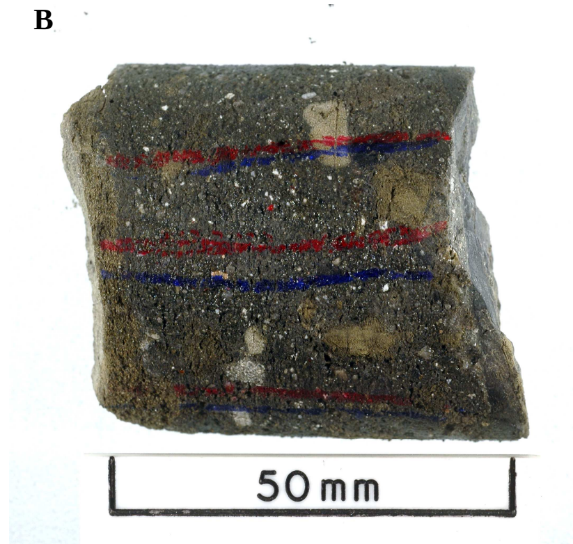
Sample RG7, Exmore Breccia, 1393.13 m. A) front view, B) back view.
