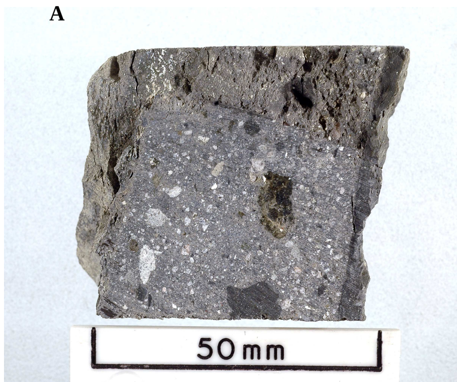
Sample RG7, Exmore Breccia, 1393.13 m. A) front view, B) back view.
