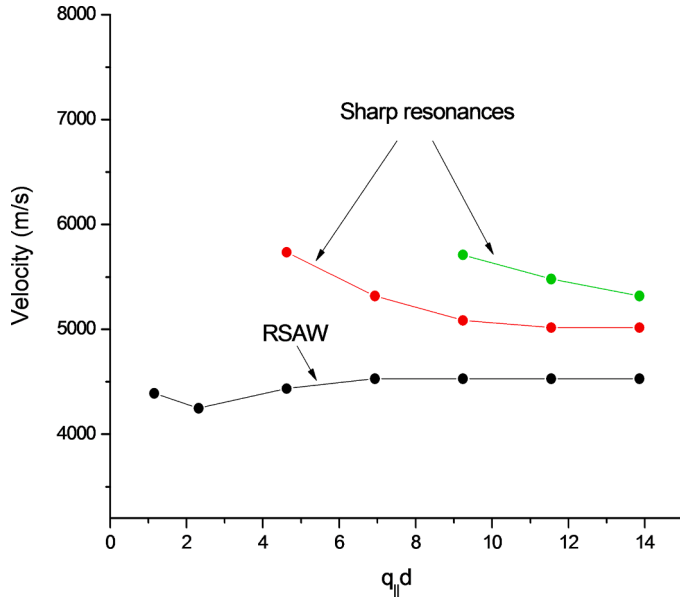
Fig. 4. Measured velocity dispersion of the modes vs. q_{||}d for the TiC/Si system. The dispersion was obtained by varying the layer thickness d while keeping q_{||} constant i.e., \theta_i was kept constant at 71^\circ .
