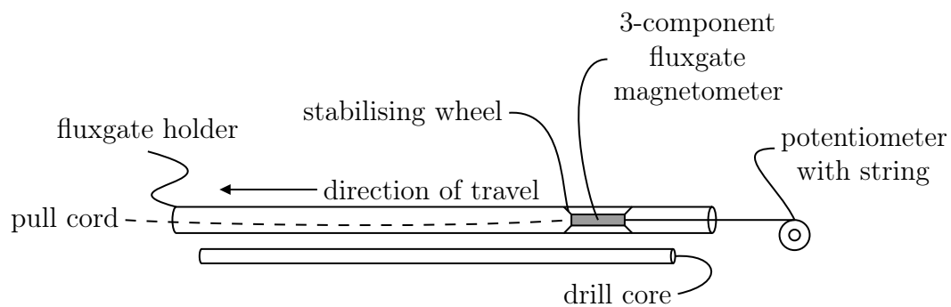
Figure 2.6: A measurement system for the determination of remanent and induced magnetisation along drill cores proposed by Foss, Leslie and Stuart (2015).
