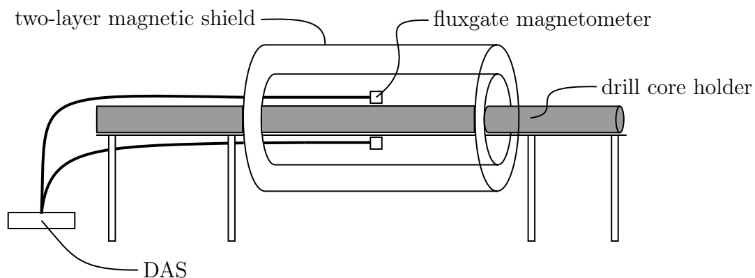
Figure 4.3: A diagram of the proposed measurement system with a second fluxgate magnetometer introduced to facilitate operation as a magnetic gradiometer.
