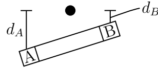
Figure 7.11: A diagram that illustrated how the position of a drill core, white rectangle with two regions of measurement (A and B), would alter the distance, d_A and d_B between the regions of measurement and the fluxgate magnetometer (black dot).
