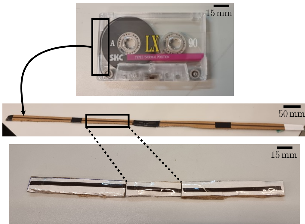
Figure 6.3: A diagram illustrating the process used to create synthetic drill cores from a cassette tape.
