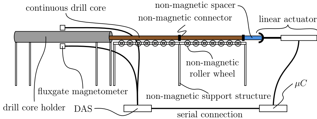
Figure 7.12: A simplified diagram, excluding the magnetic shield for clarity, of an automated version of the proposed measurement system where the only user intervention required is the loading of drill core and initiation of the measurement procedure.
