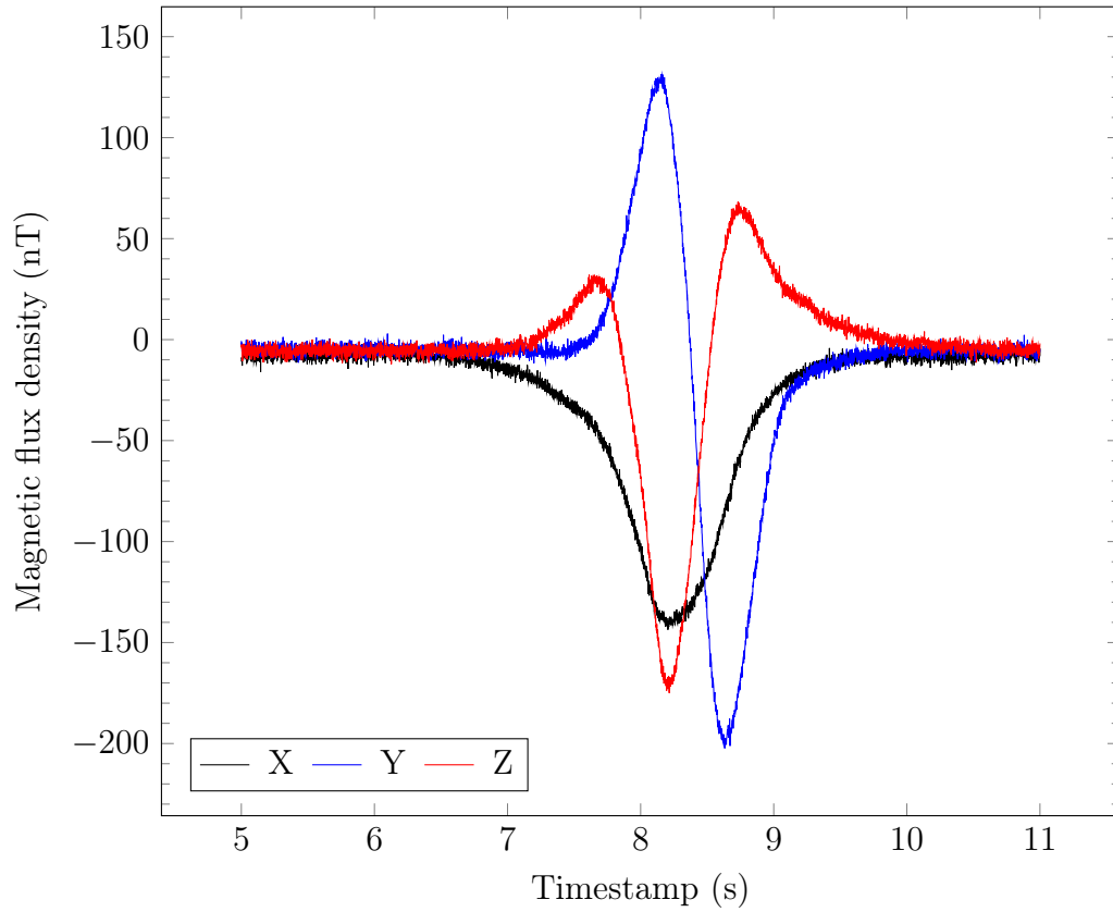
Figure 6.20: A plot of the three components of the magnetic flux density for a drill core, from the Critical Zone in the Eastern Lobe of the BIC. The effective sampling rate was 600 Hz.
