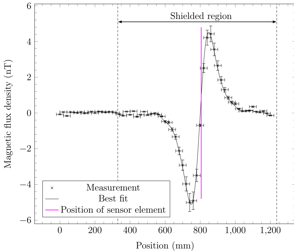
Figure 6.6: X component of the response of a fluxgate magnetometer to a magnetic dipole. The line of best fit, for positions between 540–1200 mm, was an eight-term Fourier model ( R^2 = 0.9984 , RMSE = 0.0886). The effective sampling rate was 8 Hz. The ‘shielded region’ annotation indicates the extent of the area enclosed by the magnetic shield.
