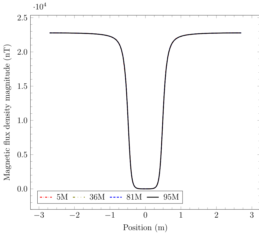
Figure 5.5: A line plot of the magnitude of the magnetic flux density along the main axis of a magnetic shield while varying the element count of the input mesh used in the FEA. The 0 m position corresponded to the midpoint of the main axis of the shield. The shield spanned from -0.447 m to 0.447 m in the plot.
