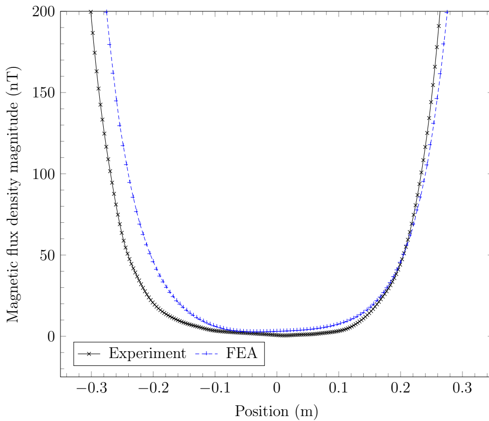
Figure 7.2: A small section of Figure 7.1 focuses on the midpoint of the main axis of the magnetic shield, comparing the FEA and experimental results for the magnetic flux density.
