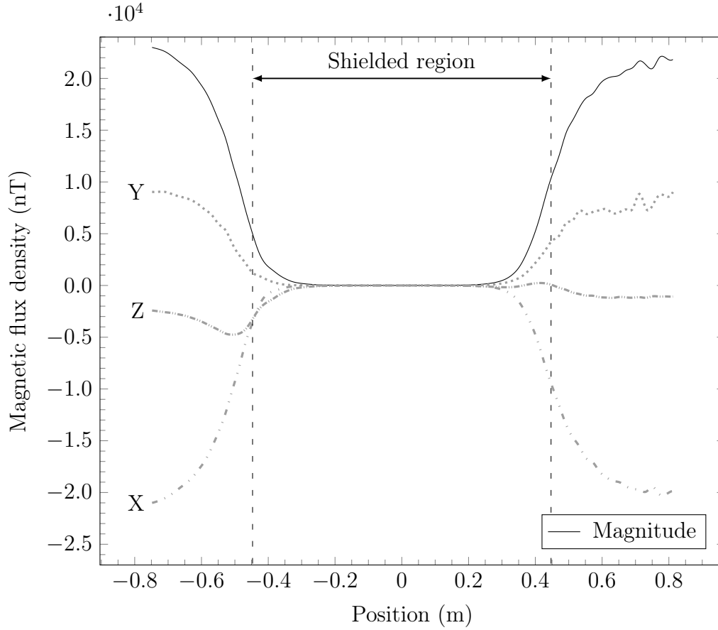
Figure 6.4: Magnetic flux density as a function of position along the main axis of a two-layer magnetic shield. The 0 m position corresponds to the midpoint of the main axis of the shield. The area marked "Shielded region" corresponds to measurements taken inside the magnetic shield.
