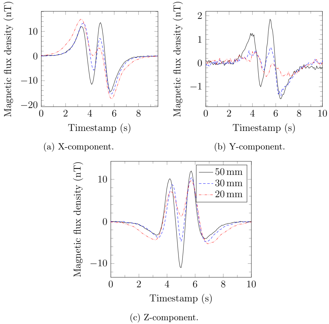
Figure 6.10: Three sets of fluxgate magnetometer outputs were collected using three synthetic drill cores passed under the sensor, with the length of the centre standard varied each run. The effective sampling rate was 10 Hz. The legend in Figure 6.10c applies to Figures 6.10a and 6.10b.
