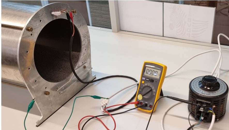
Figure 6.2: The setup used to degauss the magnetic shield. The magnetic shield is on the left side of the image, while the multimeter is in the centre and the variable autotransformer is on the right.
