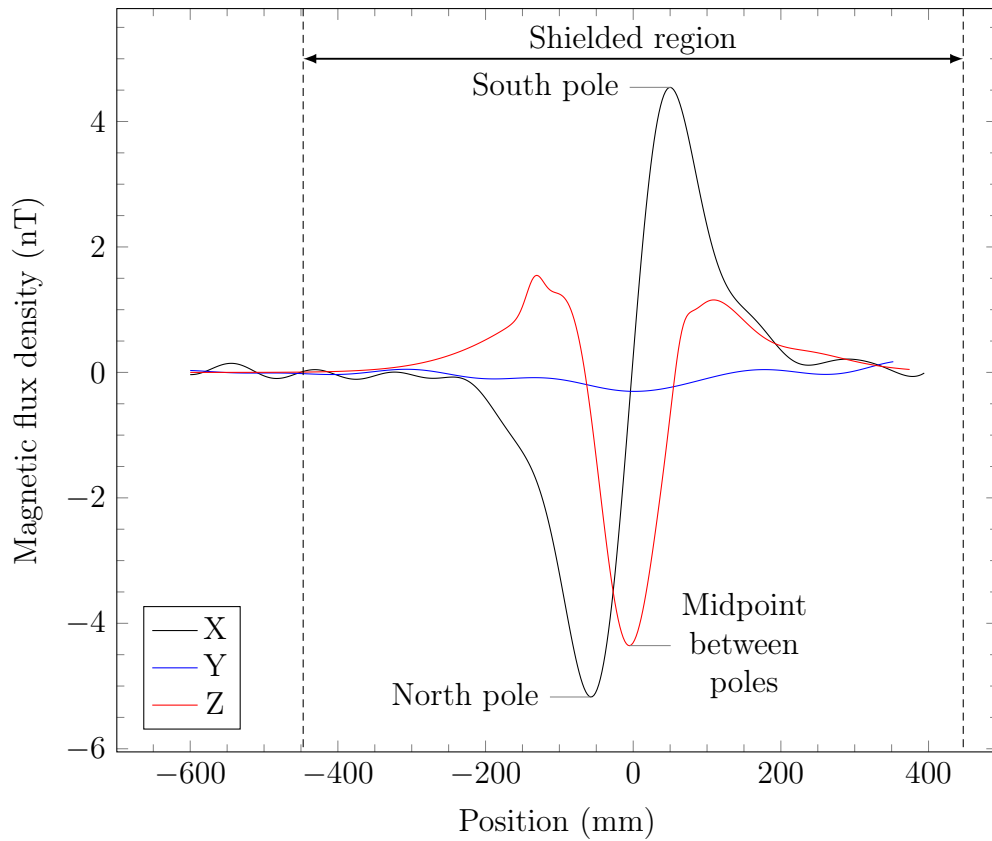
Figure 7.5: The three components of the response of a fluxgate magnetometer to a magnetic dipole as the dipole was moved closer to the fluxgate, directly under the fluxgate, at 0 m, and then away from the fluxgate. The lines of best fit, depicted here, are derived from the measurement points in Figures 6.6, 6.7, and 6.8. The positions of each set of results were adjusted so that at 0 m, all responses corresponded to the dipole being directly under the corresponding sense element inside the magnetometer. The space enclosed by the shield is indicated on the plot as the “shielded region”.
