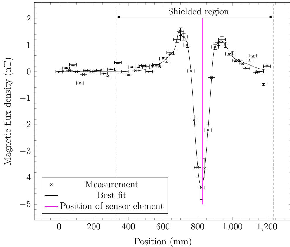
Figure 6.8: Z component of the response of a fluxgate magnetometer to a magnetic dipole. The line of best fit was a six-term Gaussian model ( R^2 = 0.9818 , RMSE = 0.1708). The effective sampling rate was 8 Hz. The ‘shielded region’ annotation indicates the extent of the area enclosed by the magnetic shield.
