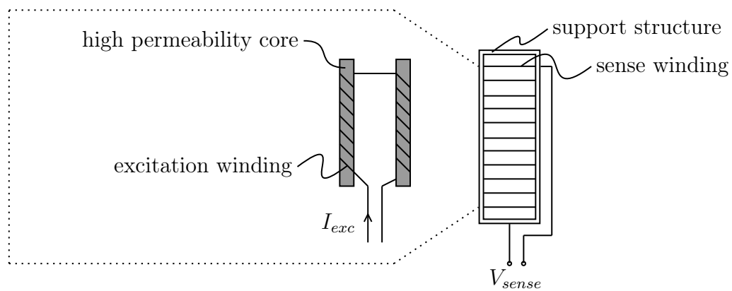
Figure 2.3: A simplified diagram of a single-component Vacquier-type fluxgate magnetometer. The high-permeability cores and excitation winding have been separated from the sense winding for visibility. In a real device, the sense winding is wrapped around both the high-permeability cores and the excitation winding. Source: Adapted from Figure 3.4b in Ripka (2021).
