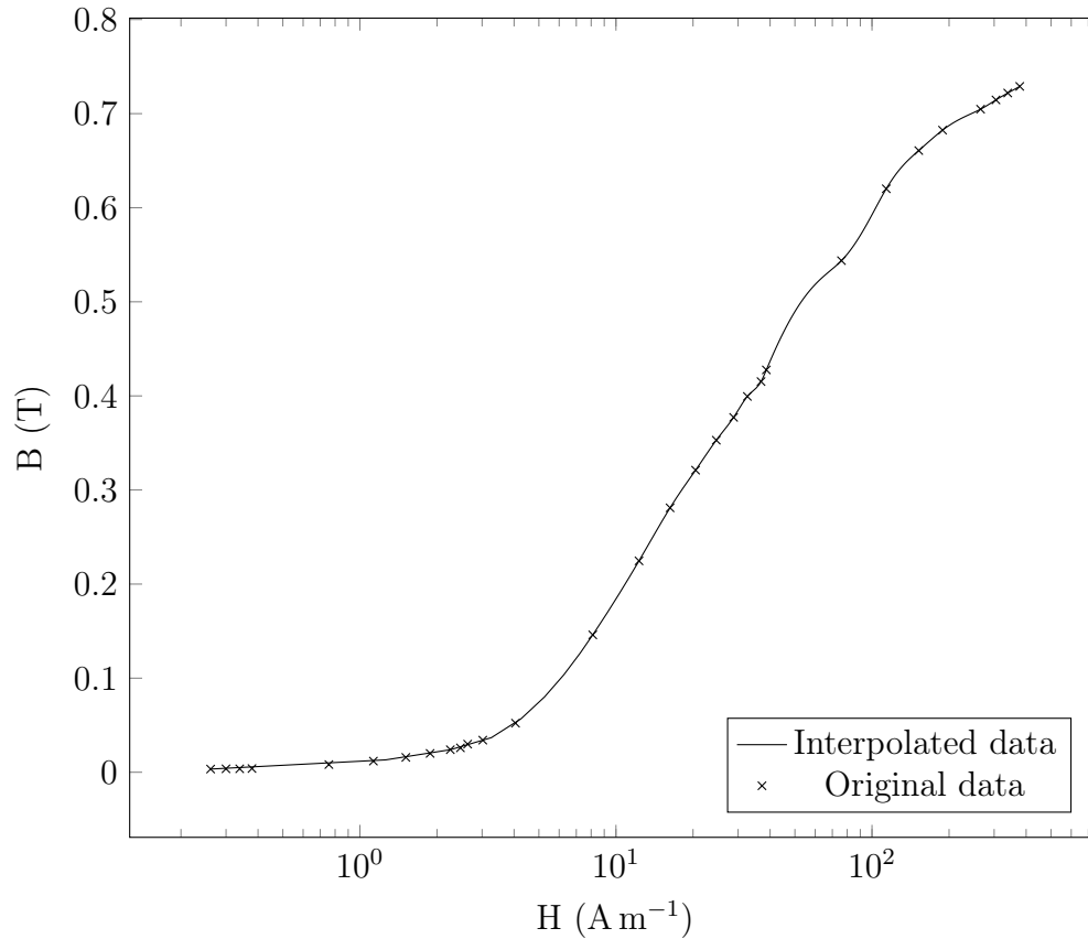
Figure B.1.1: A semi-log plot of the original B-H points measured by Arpaia et al. for 1.4mm thick ASTM A753 Alloy 4 and a line plot derived from fitting a cubic spline to the original data.
