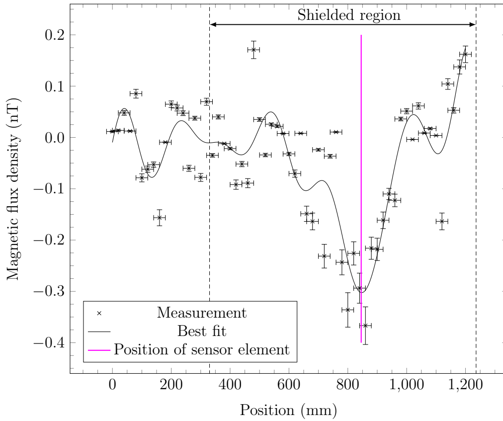
Figure 6.7: Y component of the response of a fluxgate magnetometer to a magnetic dipole. The line of best fit was an eight-term Fourier model ( R^2 = 0.7203 , RMSE = 0.0727). The effective sampling rate was 8 Hz. The ‘shielded region’ annotation indicates the extent of the area enclosed by the magnetic shield.
