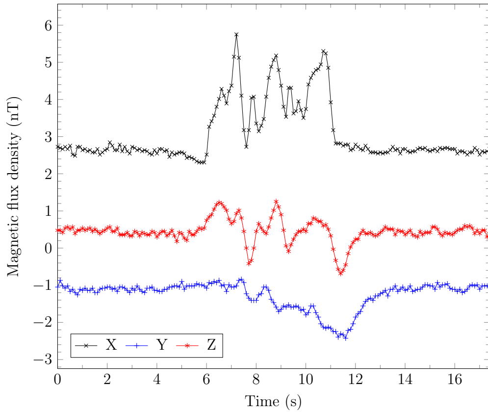
Figure 6.15: A plot of the three components of the magnetic flux density for the drill core with ID 4/3, from the Main Zone of the BIC, that contained little magnetic minerals, passed through the measurement system used in the investigation. The effective sampling rate was 10 Hz.
