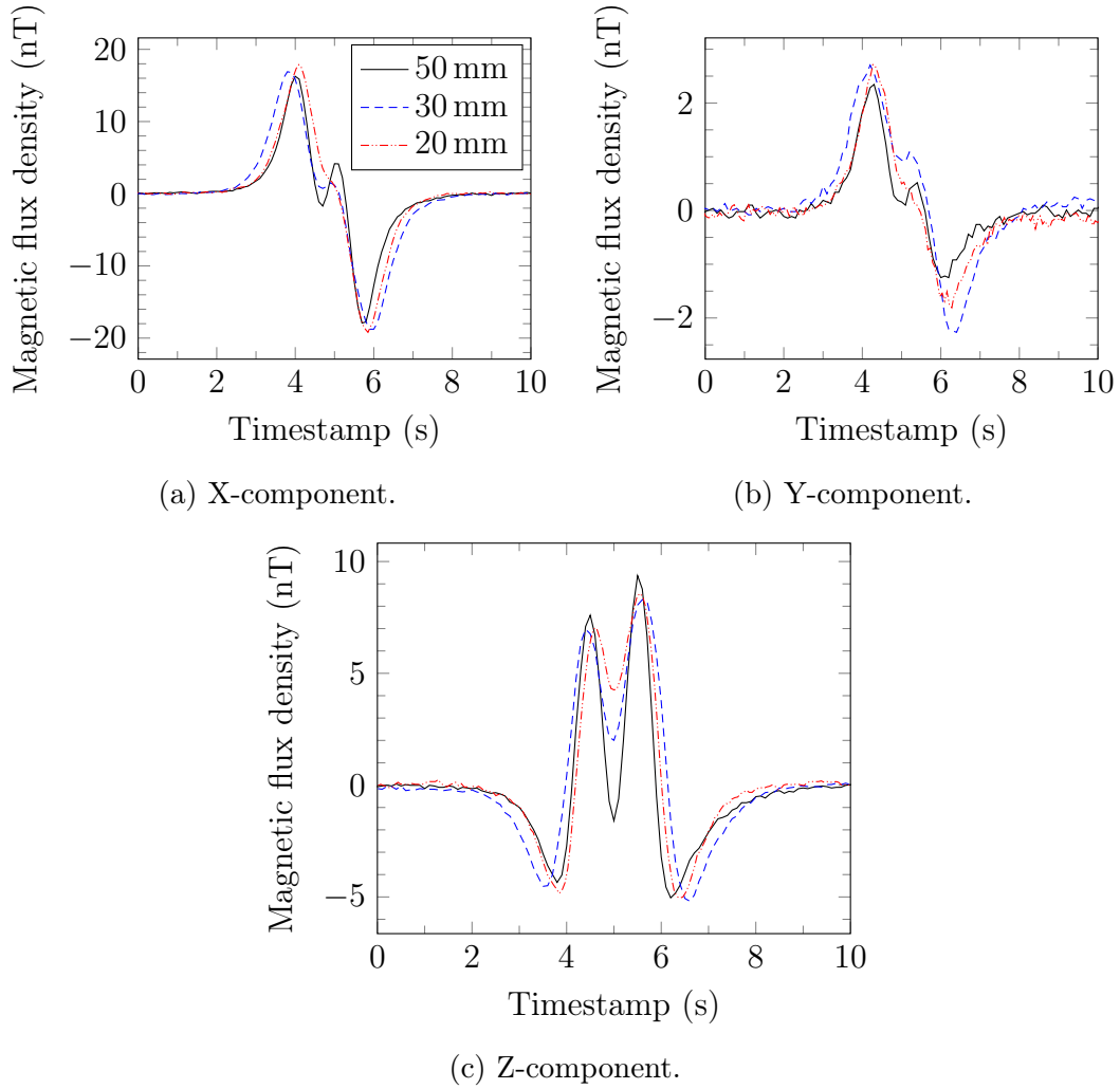
Figure 6.11: Three sets of fluxgate magnetometer outputs were collected using two synthetic drill cores, separated by a gap, passed under the sensor, with the length of the gap varied each run. The effective sampling rate was 10 Hz. The legend in Figure 6.11a applies to Figures 6.11b and 6.11c.
