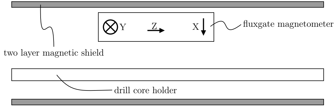
(a) Cross-section of the proposed measurement system indicating the orientation of the fluxgate magnetometer.
