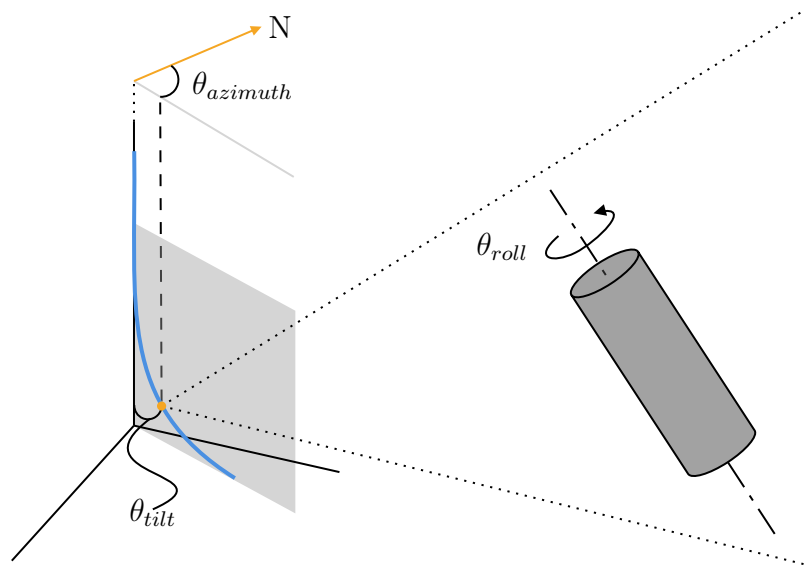
Figure 7.10: A diagram depicting the two angles used to describe the trajectory, blue line, of a borehole in three-dimensional space and a third angle, \theta_{roll} , that describes the direction that the drill core faces. The borehole is constrained to the grey plane, which is parallel to the vertical axis and not orthogonal to either horizontal axis. Borehole trajectory diagram adapted from Figure 3 in [59].
