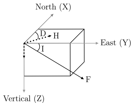
Figure 7.6: A diagram illustrating how the geomagnetic field of the Earth is expressed in spherical coordinates. The diagram is adapted from Lowrie (2007).
