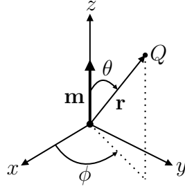
Figure 2.1: A diagram depicting a magnetic dipole moment \mathbf{m} positioned along the z-axis and an arbitrary measurement point Q . The diagram is adapted from Griffiths (2023) and represents the geocentric axial dipole of the average magnetic field of the Earth [14].
