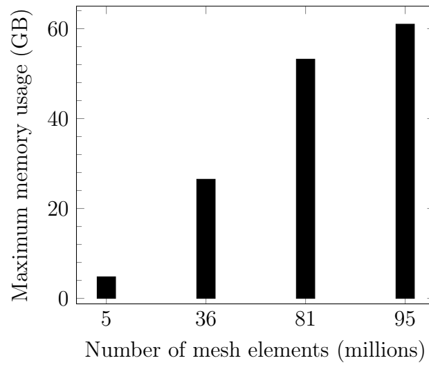
Figure C.2.2: A bar graph of the number of elements in an input mesh, to an FEA, and the maximum memory usage, per compute node, during execution of the FEA code.
