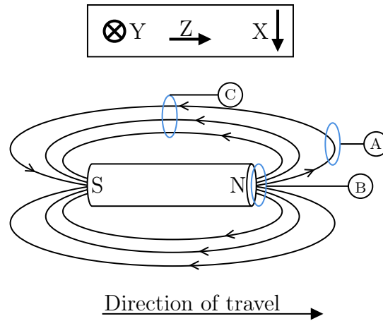
Figure 7.4: A not-to-scale diagram of a synthetic drill core passed under a fluxgate magnetometer, with component orientations depicted. Idealised field lines around the drill core are displayed.
