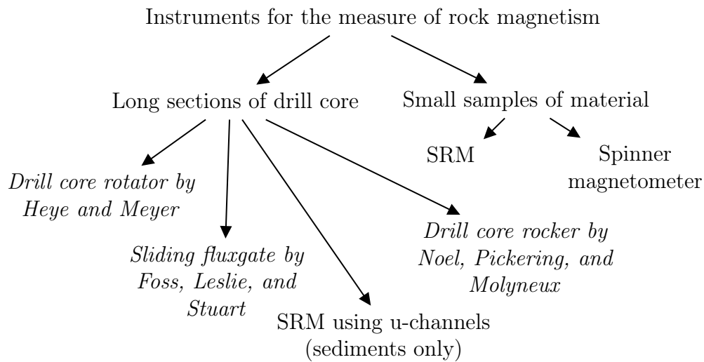
Figure 2.2: Instruments used for the measure of magnetism in rock samples. An italicised name indicated a prototype instrument that was not commercially available. Diagram compiled from the works of Heye and Meyer (1972) and Noel, Pickering and Molyneux (1989), Butler (1992), Weeks et al. (1993), Goree (2007), Foss, Leslie and Stuart (2015), and Ripka (2021).
