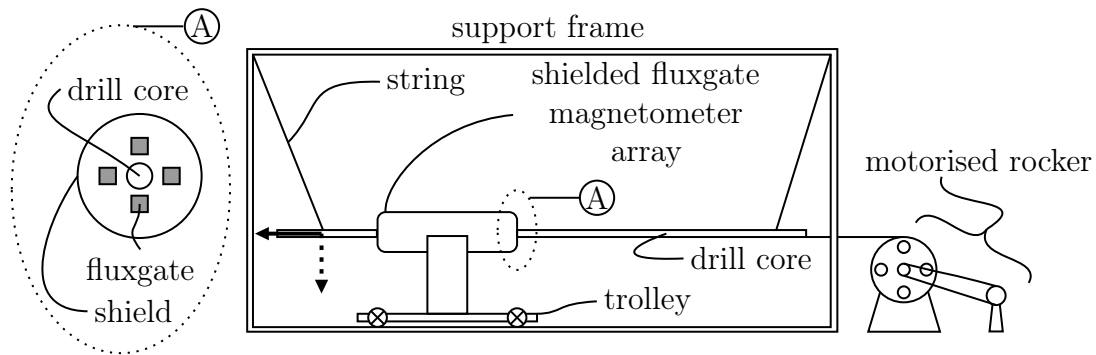
Figure 2.5: A diagram of a measurement system designed for the measurement of axial remanent magnetisation of long sediment cores. The directions of the radial and axial components of magnetisation are illustrated by the vertical dashed arrow and bold horizontal arrow, respectively. Source: Adapted from Figure 1b in Noel, Pickering and Molyneux (1989).
