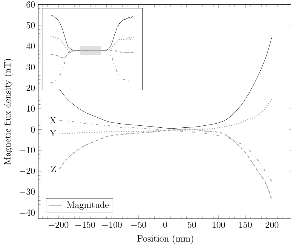
Figure 6.5: A small section of Figure 6.4, centred around the midpoint of the main axis of the magnetic shield used in the investigation. The grey rectangle in the inset graph indicates where the enlarged section was taken from Figure 6.4.
