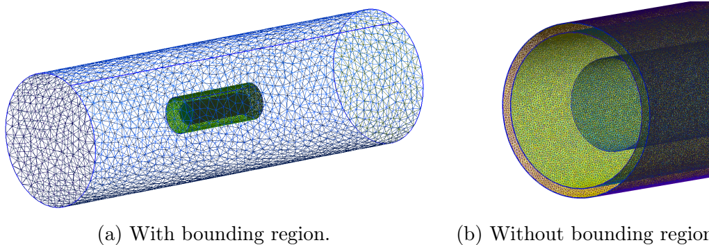
Figure 5.3: Different views of the mesh representing the two-layer magnetic shield used in the FEA. For visibility, only the 2D mesh elements are shown. The innermost cylinder in (b) is the region referred to as the “internal transition region”.
