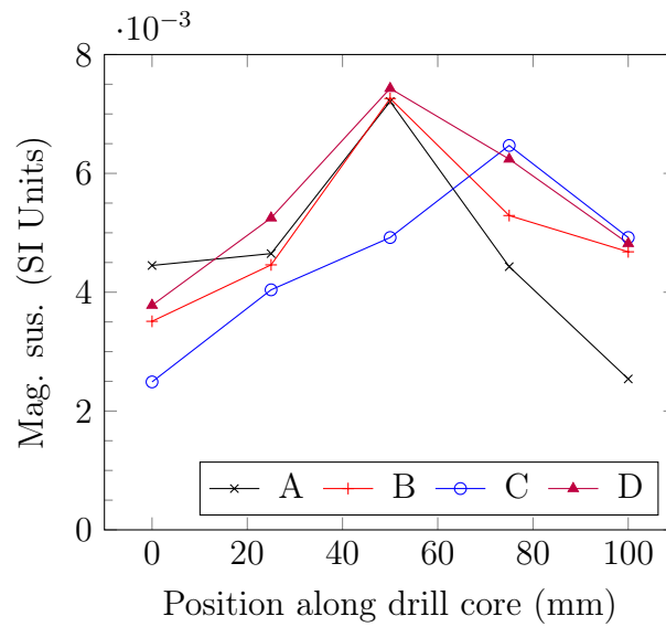
Figure 6.19: Magnetic susceptibility measurements as a function of position along the drill core recovered near the Atok mine, recorded by the GDD MPP instrument. The letters in the legend correspond to four different profiles taken along the length of the drill core. Each profile was a 90^\circ rotation about the main axis from the other.
