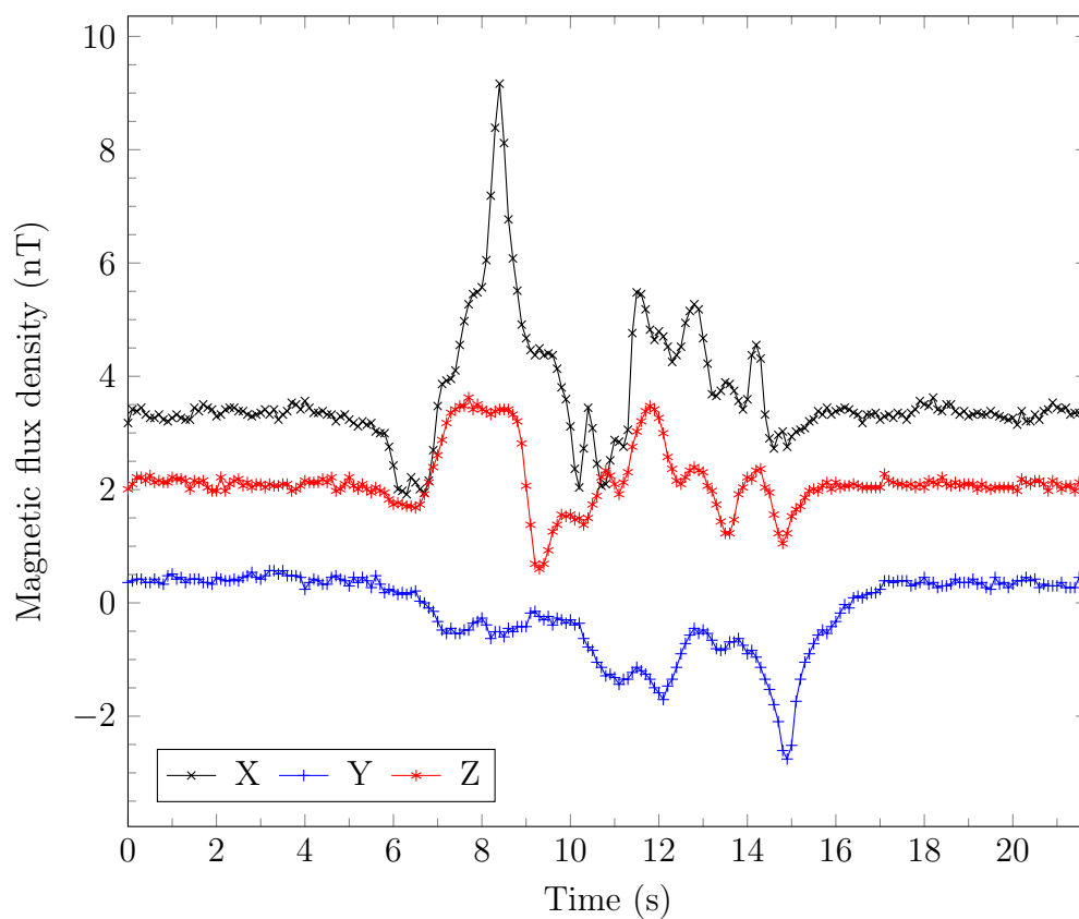
Figure 6.16: A plot of the three components of the magnetic flux density for the drill core with ID 4/4, from the Main Zone of the BIC, that contained little magnetic minerals, passed through the measurement system used in the investigation. The effective sampling rate was 10 Hz.
