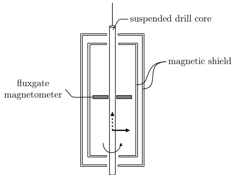
Figure 2.4: A diagram of a measurement system designed for the measurement of the radial component of magnetisation present in a drill core. The directions of the radial and axial components of magnetisation are illustrated by the bold horizontal arrow and vertical dashed arrow, respectively. Source: Adapted from Figure 1 in Heye and Meyer (1972).
