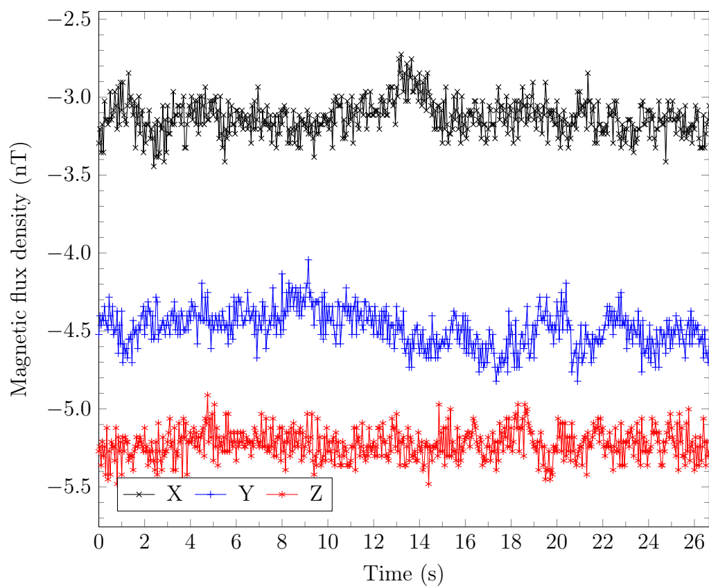
Figure 6.14: A plot of the three components of the magnetic flux density recorded for drill core with ID 4/3, from the Main Zone of the BIC, that contained little magnetic minerals, passed through the measurement system used in the investigation. The effective sampling rate was 20 Hz.
