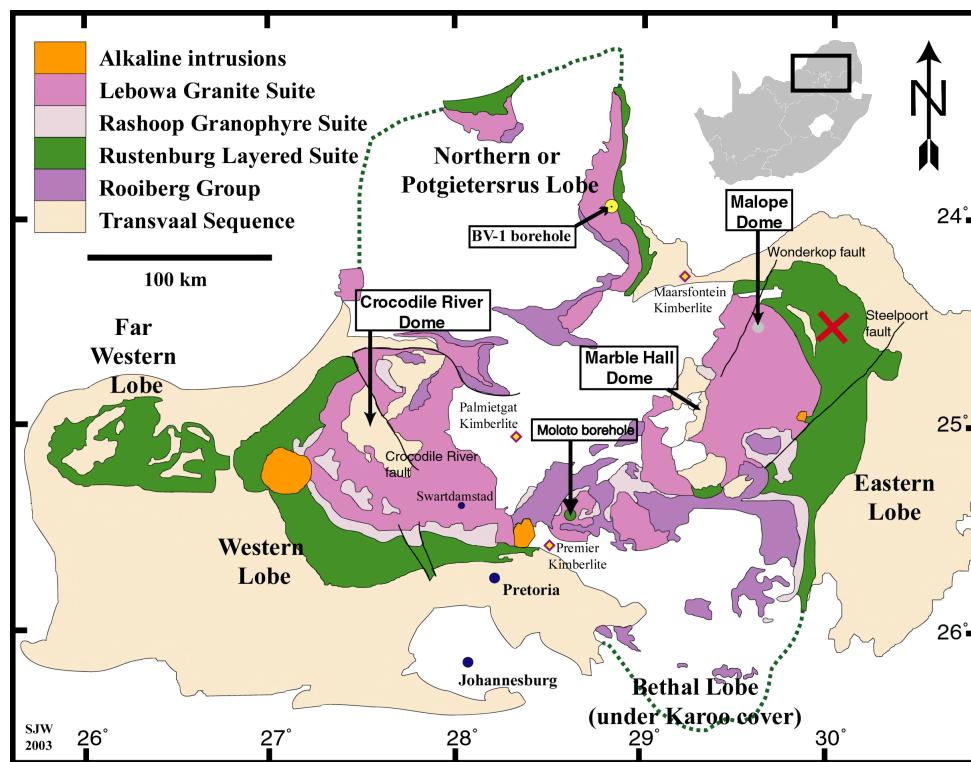
Figure 1.1: A simplified geologic map of the Bushveld Igneous Complex (BIC) in South Africa. The red cross on the Eastern Lobe indicates the location of the Bushveld Drilling Project (BVDP) borehole. Map of the BIC modified and used with permission, from Webb et al. (2004). The blank map of South Africa, by Wikimedia user “Clapsus”, is used under license (CC BY-SA 3.0)
