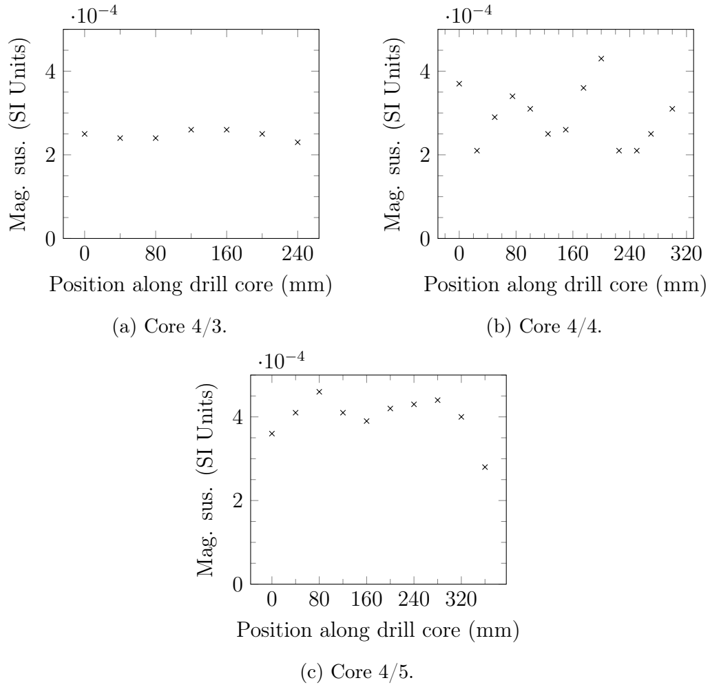
Figure 6.13: Magnetic susceptibility measurements, as a function of position along drill core 4/3, 4/4, and 4/5, recorded with the GDD MPP instrument.
