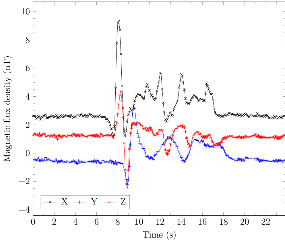
Figure 6.17: A plot of the three components of the magnetic flux density for the drill core with ID 4/5, from the Main Zone of the BIC, that contained little magnetic minerals, passed through the measurement system used in the investigation. The effective sampling rate was 10 Hz.
