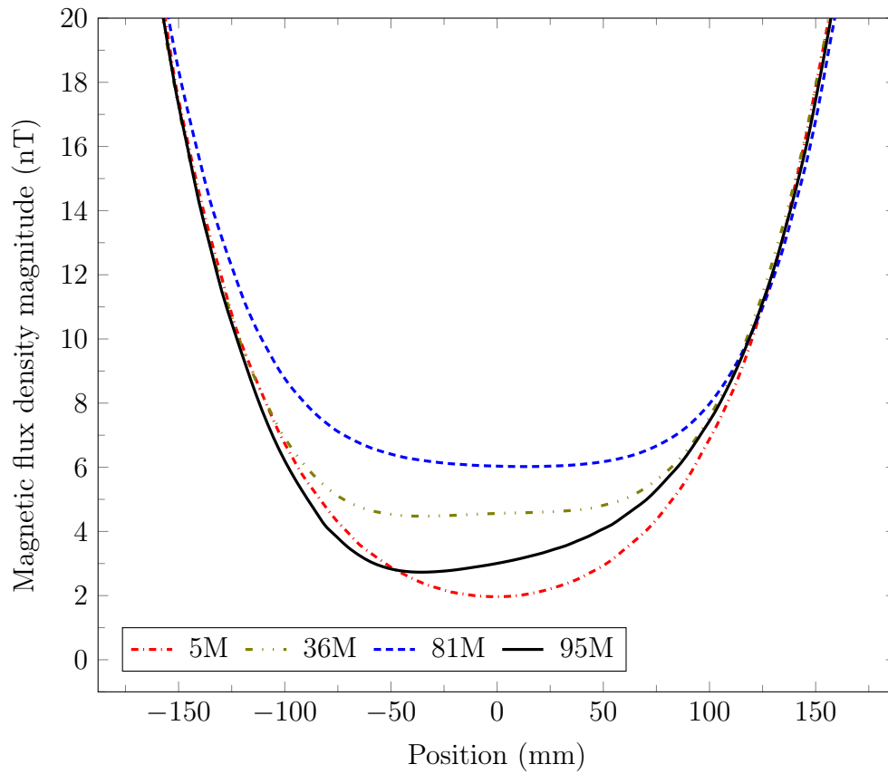
Figure 5.6: A plot of a small section of Figure 5.5, centred around the midpoint of the main axis of the magnetic shield.
