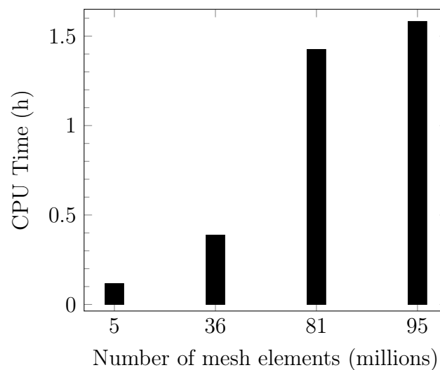
Figure C.2.1: A bar graph of the number of elements in an input mesh, to an FEA, and the amount of CPU time taken for the FEA code to reach the convergence criterion.
