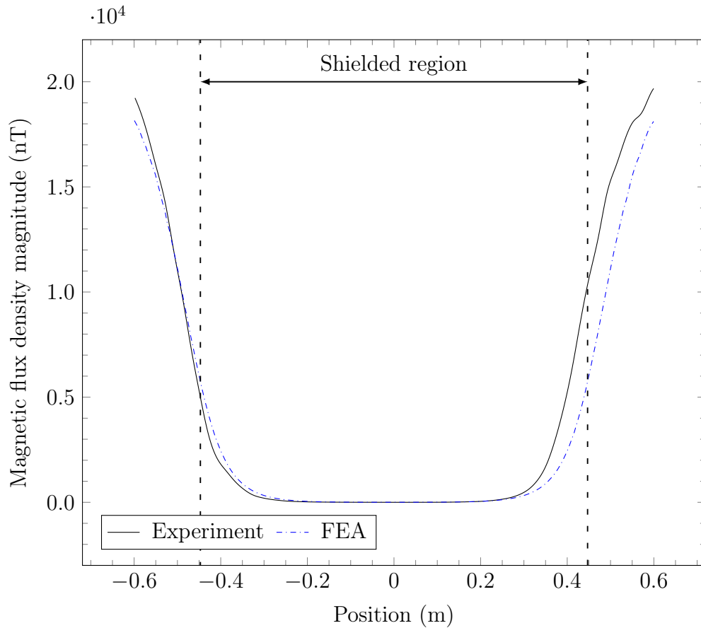
Figure 7.1: A line plot comparing the FEA and experimental results for the magnetic flux density along the main axis of the magnetic shield used in the investigation. The centre of the shield, along the main axis, is found at the 0 m position and the space enclosed by the shield is indicated on the plot as the “shielded region”.
