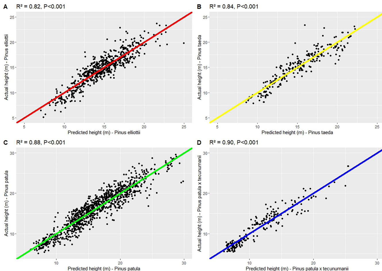
Fig. 2. Comparison of tree dominant height growth from multiple linear regression model predictions to the actual measured dominant height values for (A) Pinus elliottii (red), (B) Pinus taeda (yellow), (C) Pinus patula (green), and (D) Pinus patula x Pinus tecunumanii (blue) trees.
