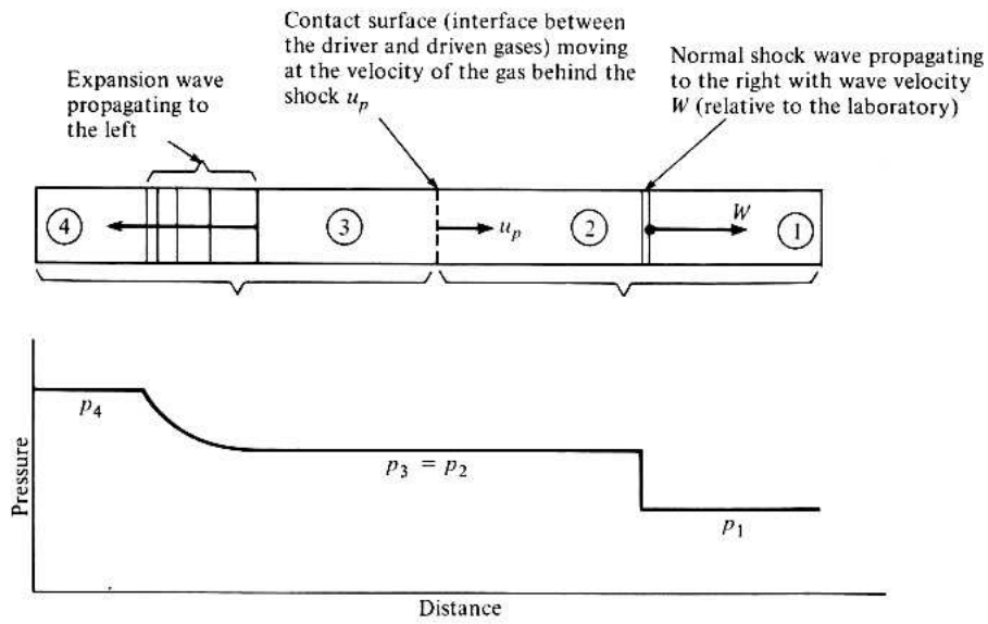
Figure 2.2: Shock tube after diaphragm burst [3]
