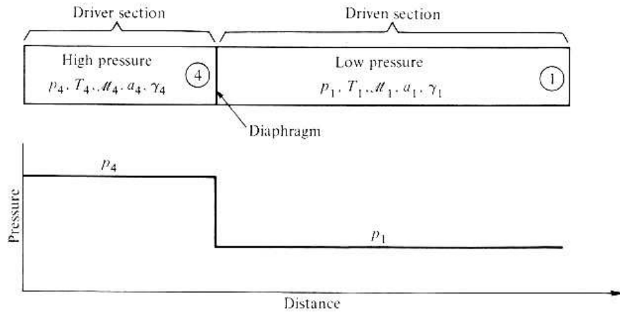
Figure 2.1: Shock tube initial conditions before diaphragm burst [3]
