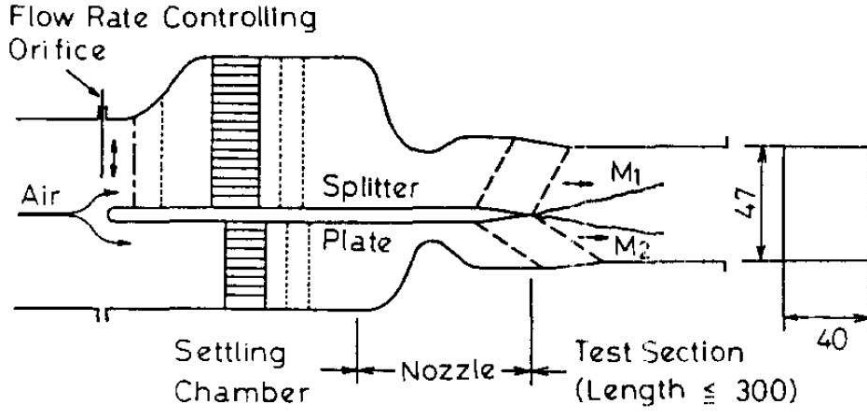
Figure 2.14: Experimental apparatus ( M_2 = 1.4 test conditions) [21]
