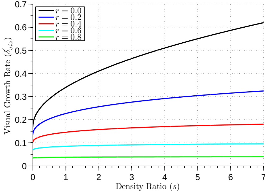
Figure 6.40: Visual Growth Rate ( \delta'_{viz} ) vs Density Ratio ( s )
