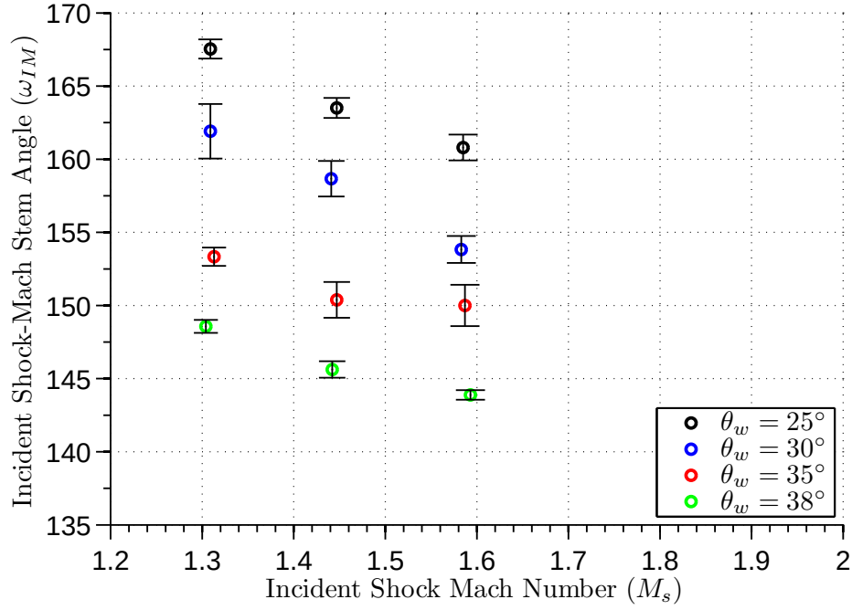
Figure 6.14: \omega_{IM} vs M_s
