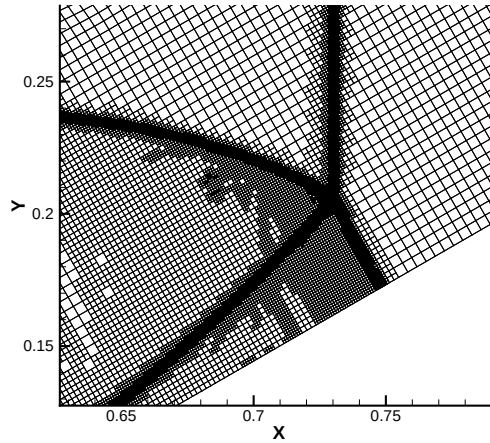
Figure 5.2: Refined mesh in the vicinity of the triple point for a 30° Wedge, M_s = 1.46
