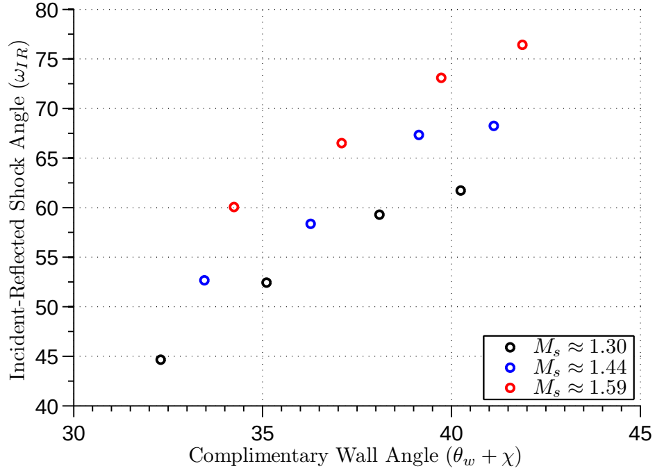
Figure 6.17: \omega_{IR} vs \theta_w + \chi
