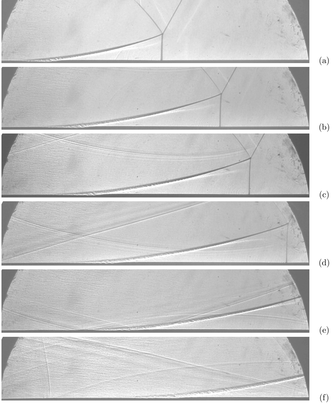
Figure 6.2: Shear layer development for the 30° Wedge. M_s = 1.44 . (a) 3000 \mu s , (b) 3100 \mu s , (c) 3150 \mu s , (d) 3200 \mu s , (e) 3300 \mu s , (f) 3400 \mu s
