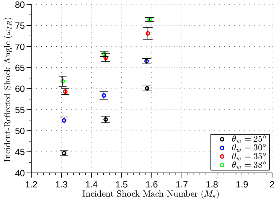
Figure 6.12: \omega_{IR} vs M_s
