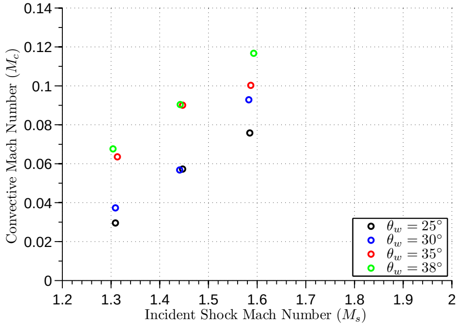
Figure 6.34: Convective Mach Number
