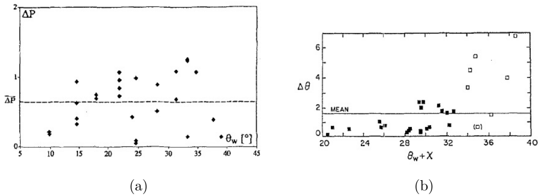
Figure 1.19: Normalised minimum experimental error values with mean value indicated by a dashed line[12] (a) Pressure difference (b) \theta difference
