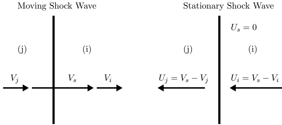
Figure 1.1: Galilean transformation of a shock wave from the laboratory to stationary shock reference frame [1]
