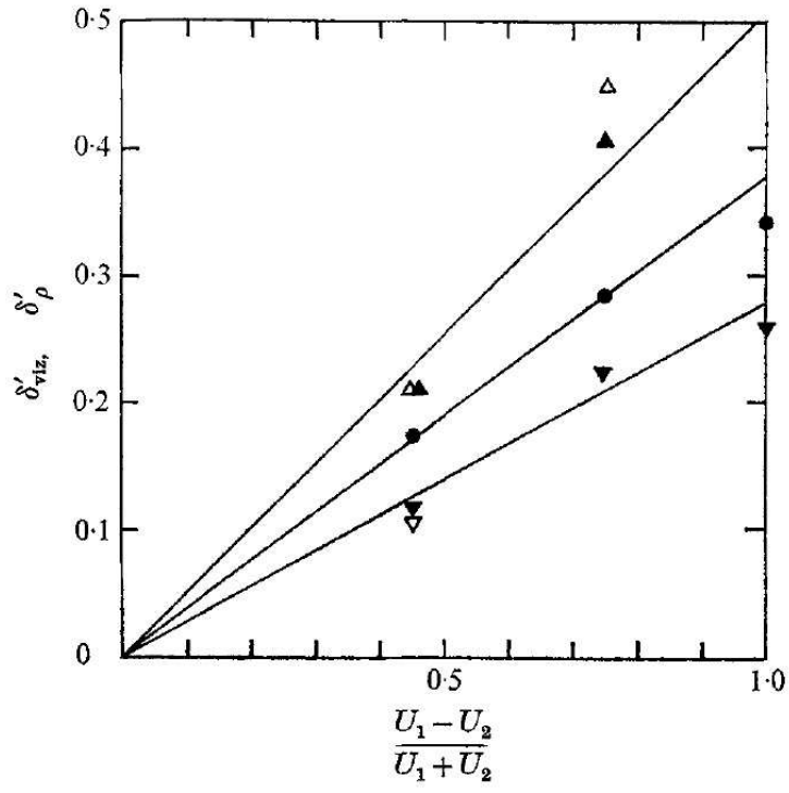
Figure 2.8: Shear layer growth rates (filled symbols represent visual growth rates from experimental photographs) [17]
