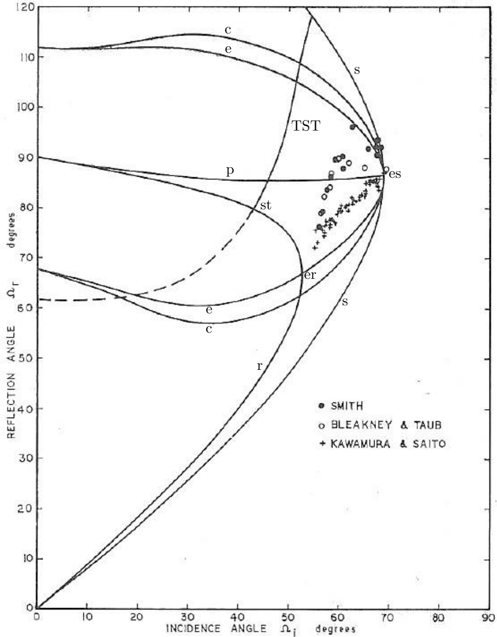
Figure 1.13: Variation of incidence angle with reflection angle for \xi = 0.8 [8]
