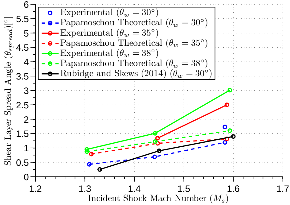
Figure 6.42: Spread angle comparison to theory from Papamoschou and Roshko[22]
