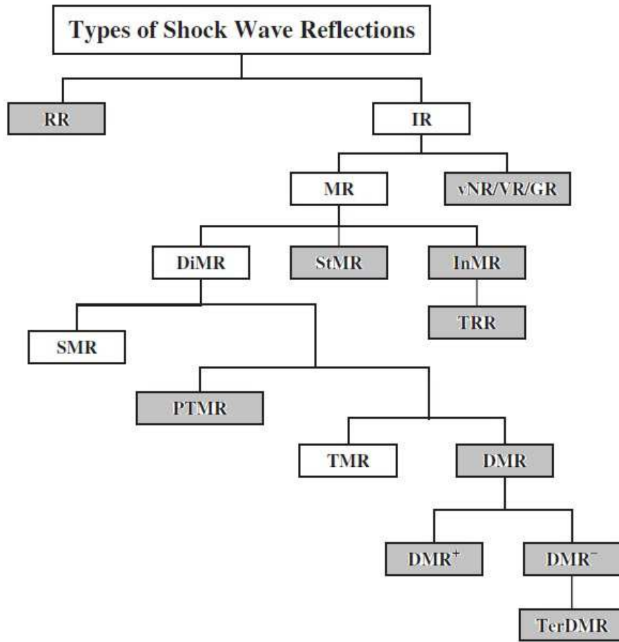
Figure 1.2: Possible shock wave reflections as classified in Ben-Dor [1]
