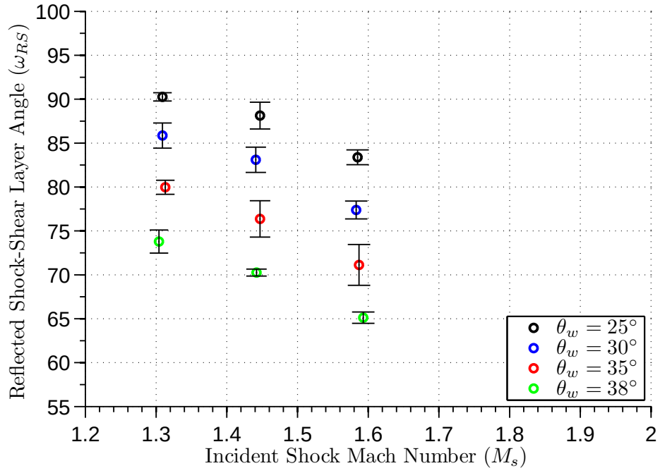
Figure 6.13: \omega_{RS} vs M_s
