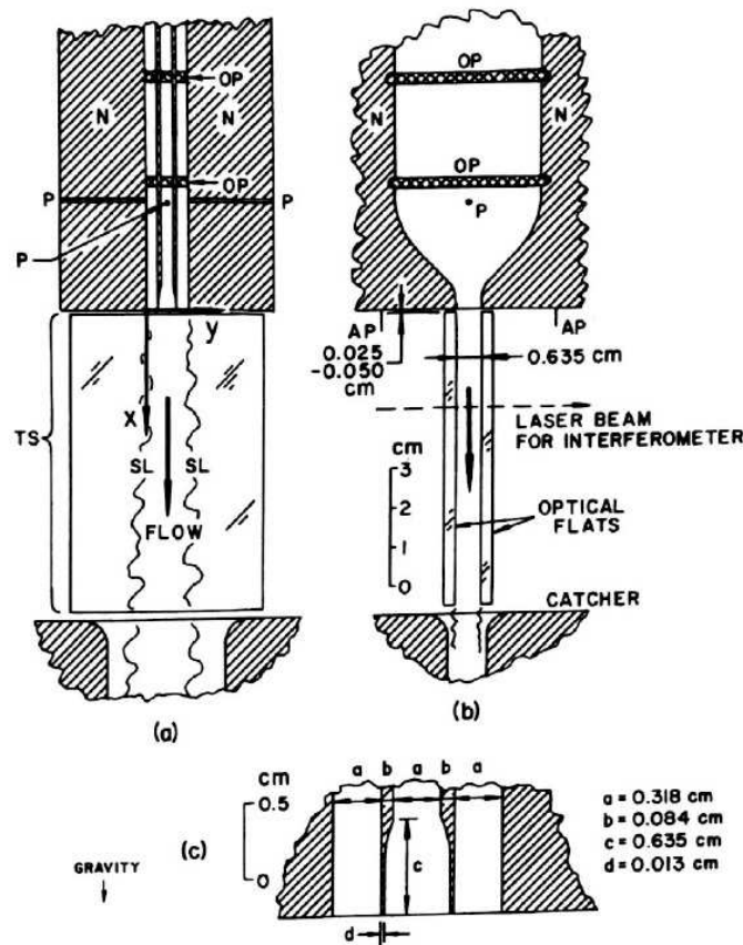
Figure 2.10: Experimental apparatus (a) Parallel to shear layers (b) Normal to shear layers (c) Magnification of nozzle exits [19]
