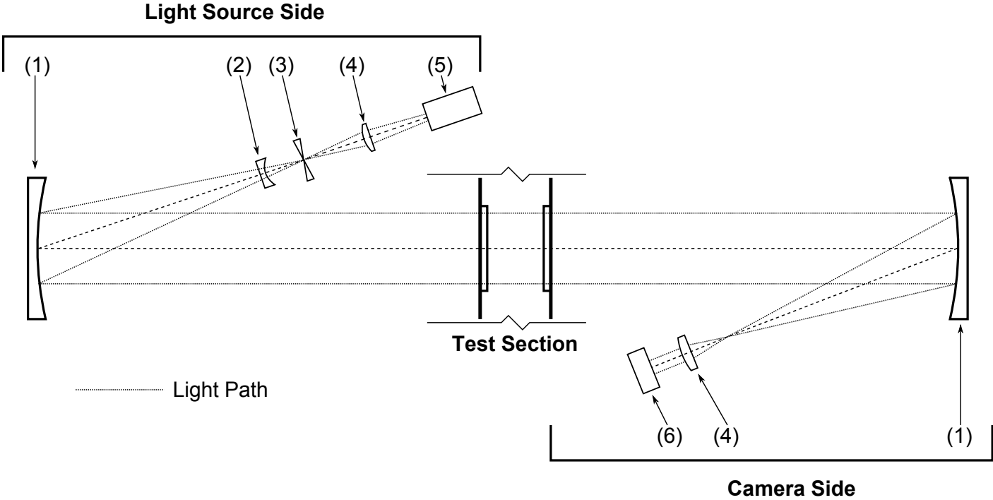
Figure 4.3: Flow Visualisation Layout
