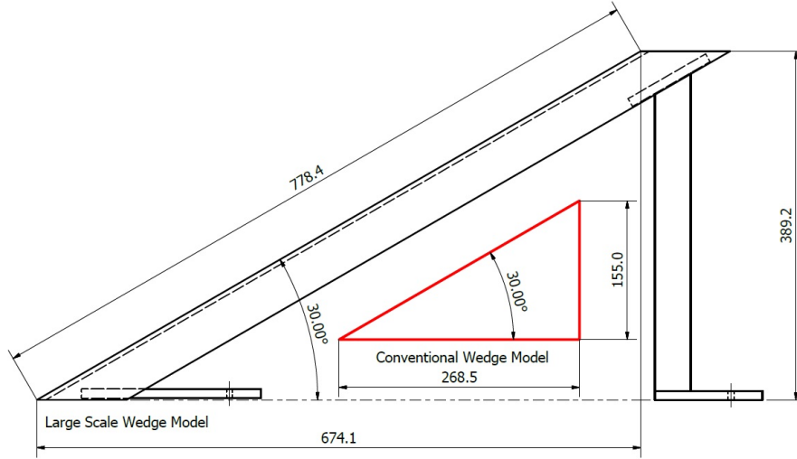
Figure 6.19: Comparison of facility wedge sizes (dimensions in mm)
