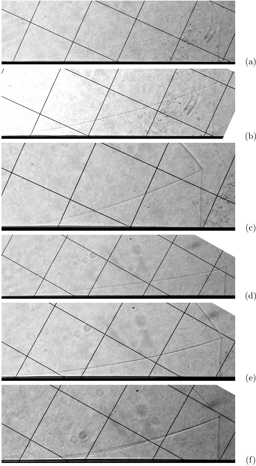
Figure 6.6: Shear layer development for the 25^\circ Wedge. Corresponding Incident Shock Mach number and time delay: (a) M_s = 1.309 , 1925\mu s (b) M_s = 1.447 , 1750\mu s (c) M_s = 1.585 , 1550\mu s . Shear layer development for the 30^\circ Wedge: (d) M_s = 1.309 , 1900\mu s (e) M_s = 1.441 , 1700\mu s (f) M_s = 1.583 , 1550\mu s
