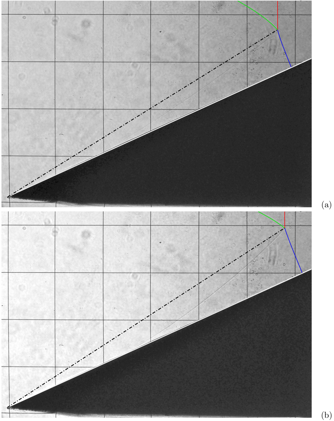
Figure B.1: Single Mach Reflection with highlighted features for the \theta_w = 25^\circ wedge ( Incident Shock , Reflected Shock , Mach Stem , Triple Point Trajectory - Black, Wedge Surface - White): (a) M_s = 1.309 , Time Delay: 1925\mu s (b) M_s = 1.447 , Time Delay: 1750\mu s
