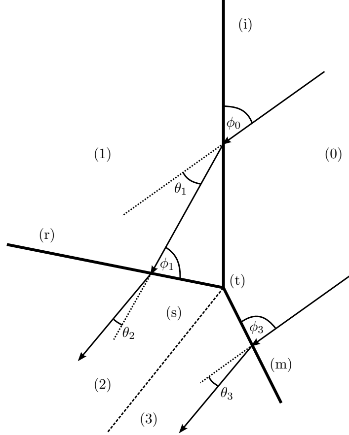
Figure 1.11: Three Shock Theory schematic with definition of parameters
