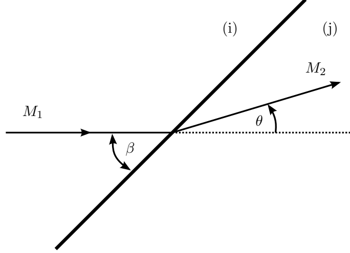
Figure 1.9: Oblique shock wave parameters[1]
