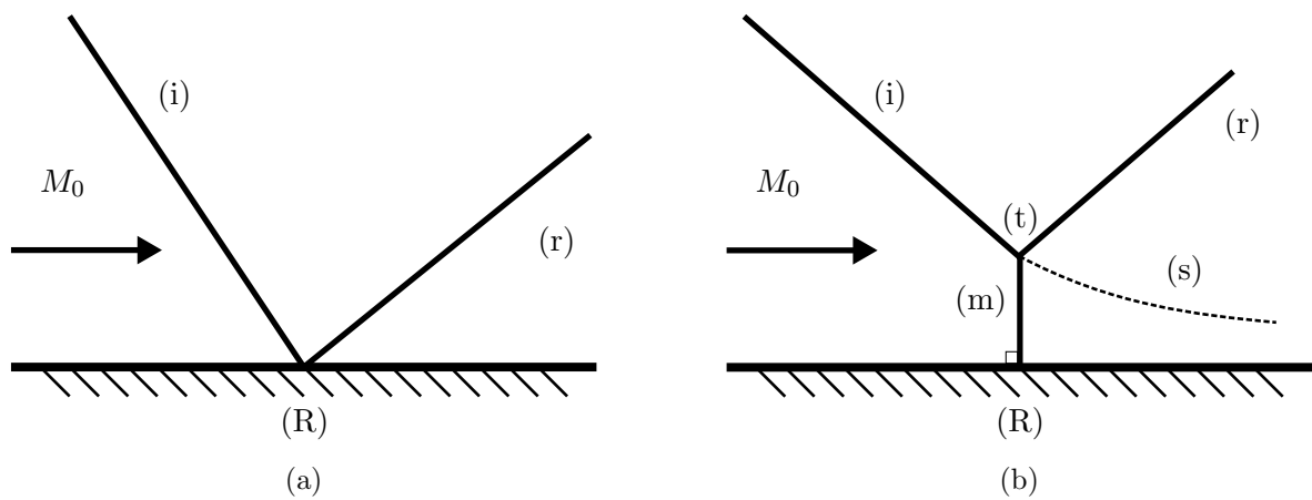
Figure 1.3: (a) Regular Reflection (RR), (b) Mach Reflection (MR)
