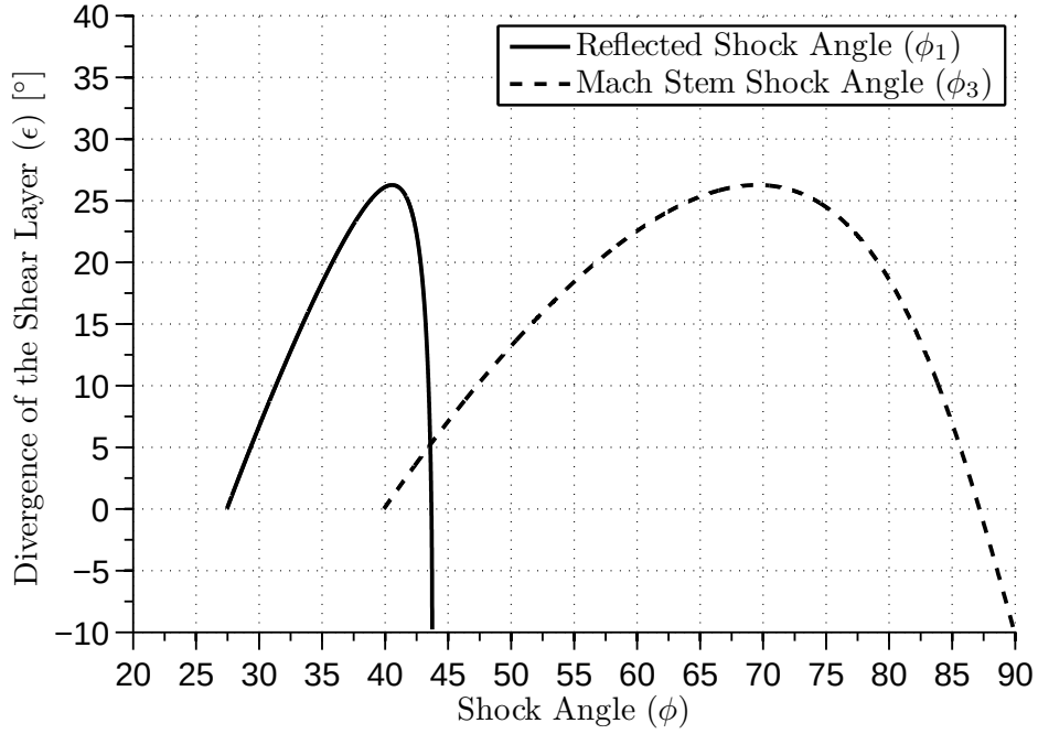
Figure 6.23: Shock Angle ( \phi ) vs Shear Layer Divergence ( \epsilon )
