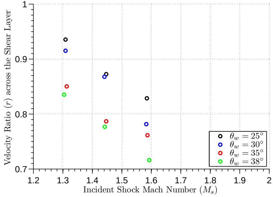
Figure 6.35: Velocity Ratio across the Shear Layer
