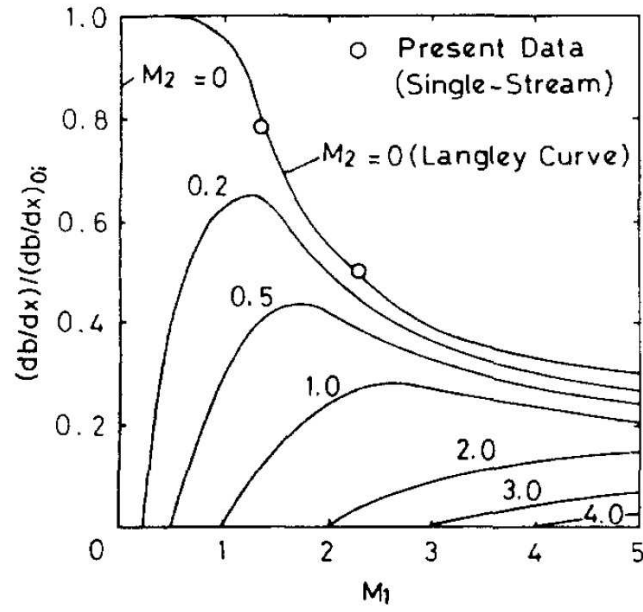
Figure 2.15: Spreading rate variation with M_1 [21]
