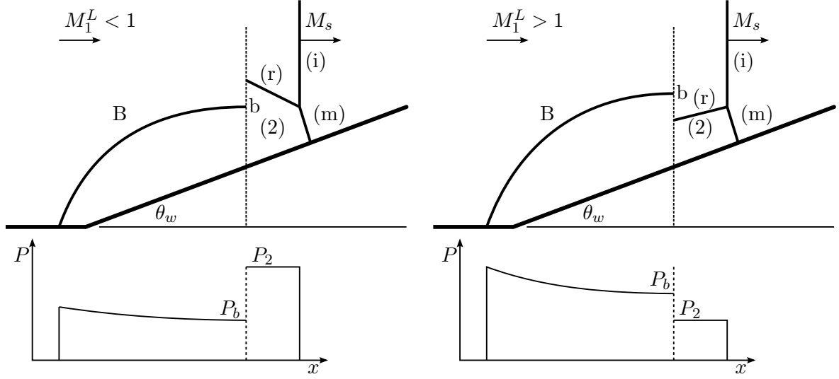
Figure 1.5: The shock wave reflection process model[1]. Schematic showing effect of M_1^L on the pressure jump
