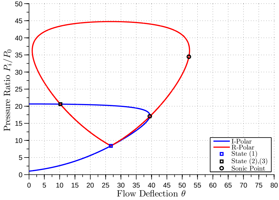
Figure 6.22: Shock Polar representation of Ben-Dor's data
