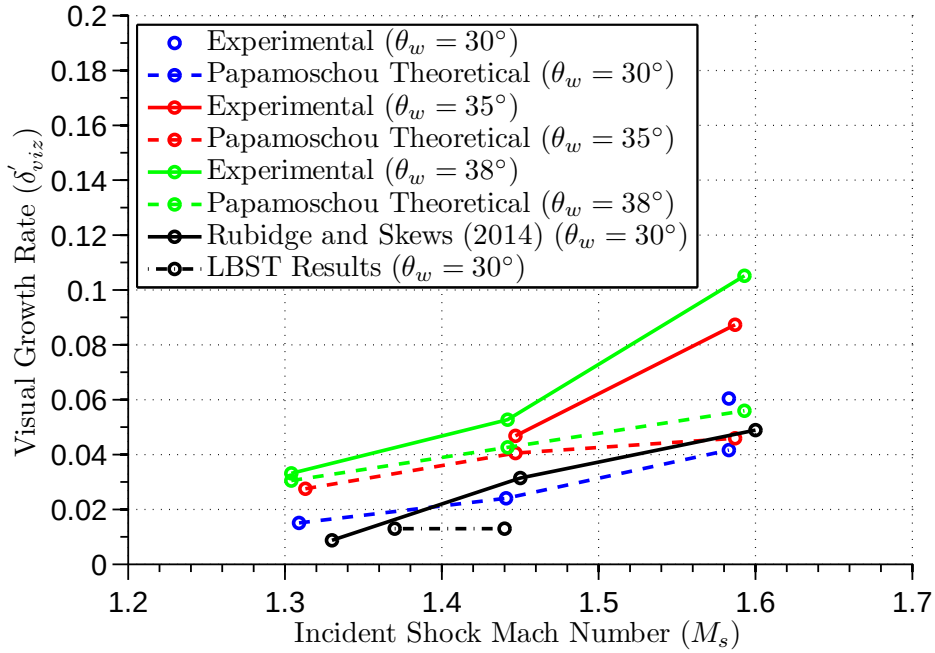
Figure 6.41: Visual Growth Rate ( \delta'_{viz} ) comparison to theory from Papamoschou and Roshko[22]
