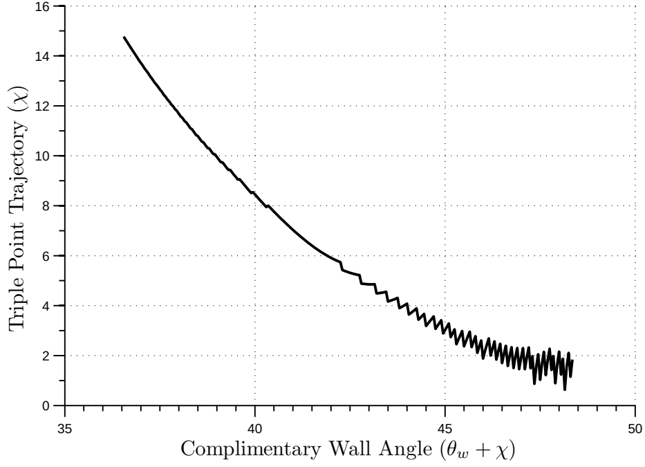
Figure C.1: Triple Point Trajectory ( \chi ) vs Complimentary Wall Angle ( \theta_w + \chi ) for M_s = 1.44
