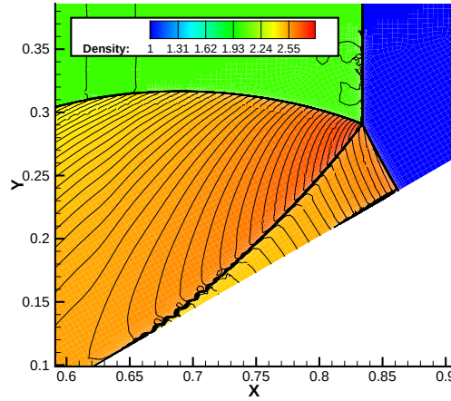
Figure 5.3: Contours of density of a Single Mach Reflection occurring on a 30^\circ Wedge, M_s = 1.61
