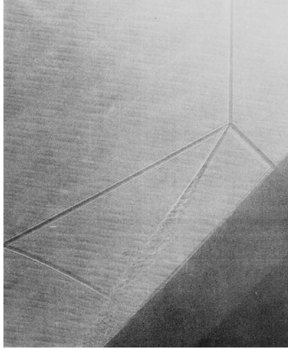
Figure 1.16: Zoomed in shadowgraph of the DMR analysed by Ben-Dor[10, 11]. M_s = 2.71 \pm 0.01 , \theta_w = 47.1^\circ , T_0 = 296\text{K} , p_0 = 760 \text{ torr} and \chi = 3^\circ \pm 0.5^\circ .
