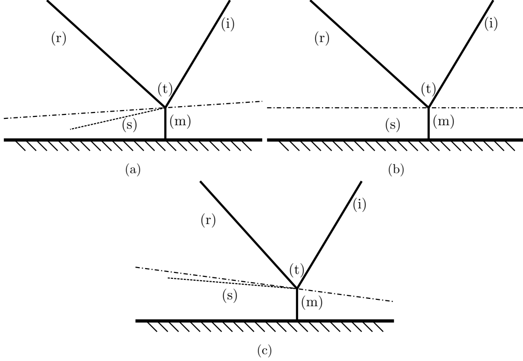
Figure 1.4: Illustration of MR types (a) Direct Mach Reflection (DiMR) (b) Stationary Mach Reflection (StMR) (c) Inverse Mach Reflection (InMR), adapted from Ben-Dor [1]
