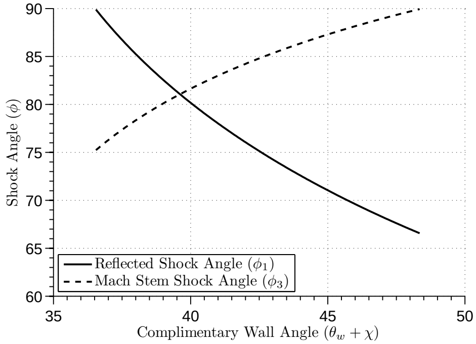
Figure C.5: Shock Angle ( \phi ) vs Complimentary Wall Angle ( \theta_w + \chi ) for M_s = 1.44
