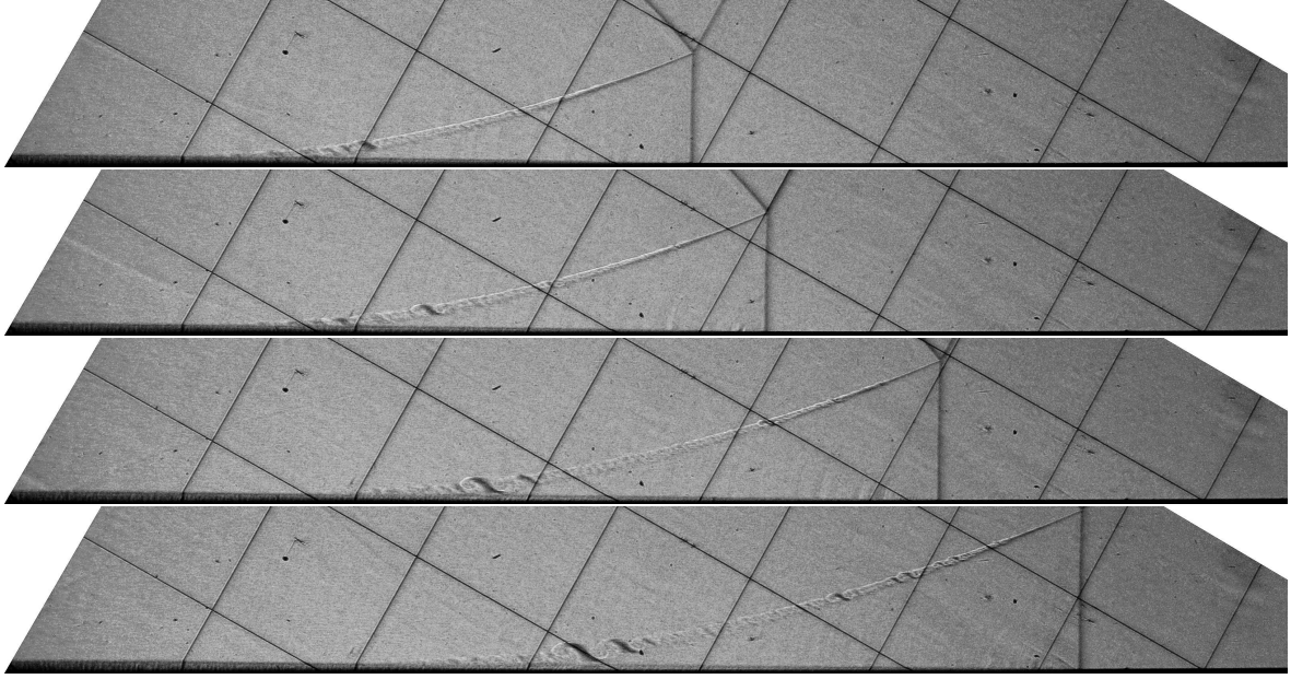
Figure 1.23: KHI occurring along a Mach reflection shear layer for a 30° wedge, M_s = 1.61 [13]
