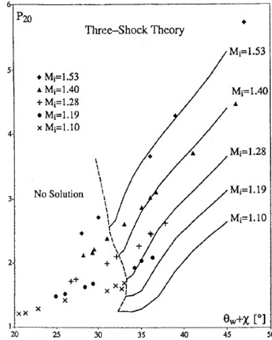
Figure 1.17: Pressure behind the reflected shock ( P_{20} ) vs Complimentary Wall Angle ( \theta_w + \chi ) as a function of Mach number. Solid lines indicate Three Shock Theory calculated theoretically[12]
