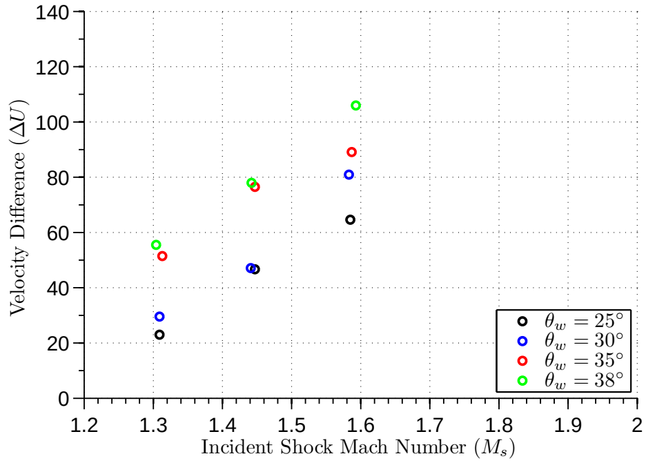
Figure 6.33: Velocity difference across the Shear Layer
