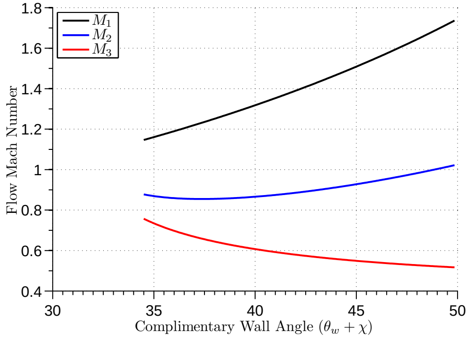
Figure C.4: Flow Mach Number vs Complimentary Wall Angle ( \theta_w + \chi ) for M_s = 1.585
