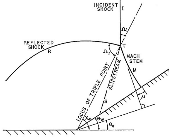
Figure 1.12: Definition of parameters used in Skews[8]
