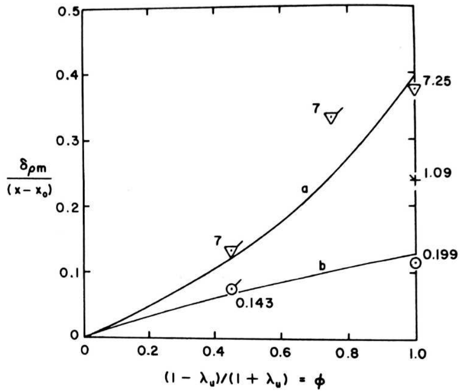
Figure 2.11: Shear layer spreading rates \delta_{\rho m} vs \phi with \lambda_{\rho} as a parameter [19]
