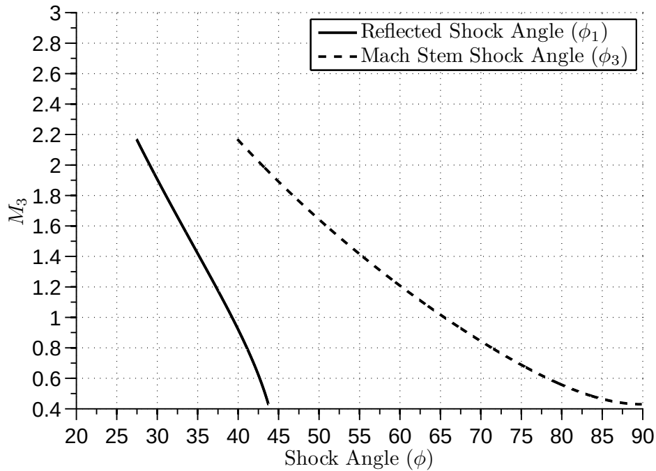
Figure 6.24: Shock Angle ( \phi ) vs M_{03}
