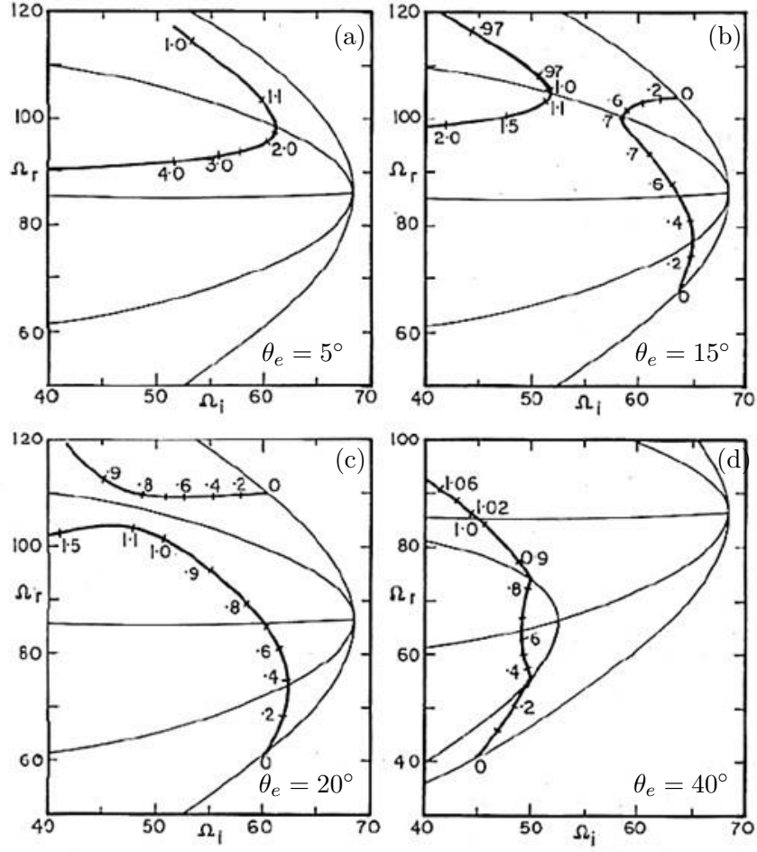
Figure 1.14: Various solution types for values of F with \theta_e as a parameter[8]
