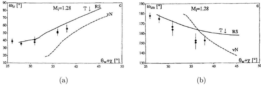
Figure 1.20: Measured shock angles with dashed line calculated from three shock theory and line T from the modified theory[12] (a) \omega_{IR} (b) \omega_{IM}
