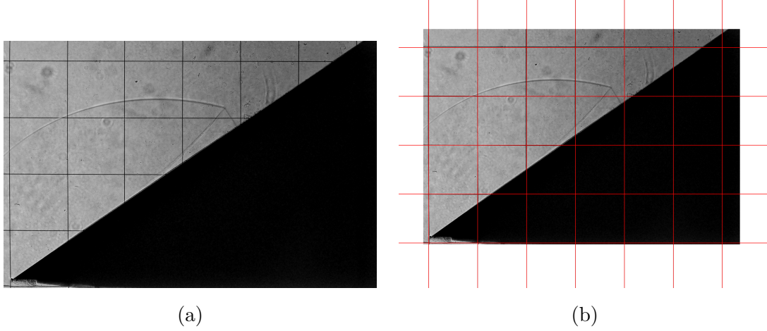
Figure 6.9: (a) \theta_w = 35^\circ , M_s = 1.587 Original Image (b) Image corrected for grid distortion with virtual grid overlaid in red
