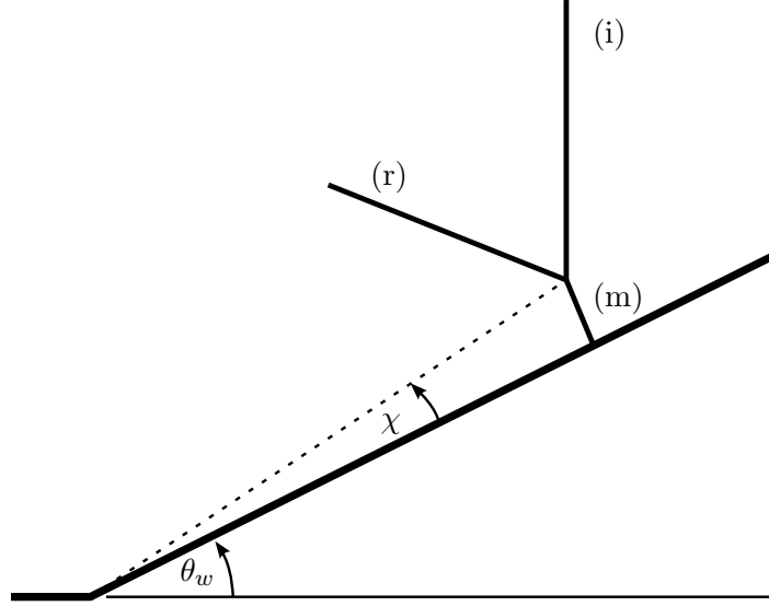
Figure 1.10: Mach Reflection occurring on a plane wedge
