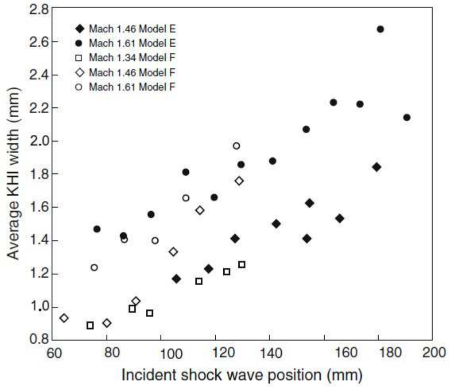
Figure 1.24: Shear layer average width [13]
