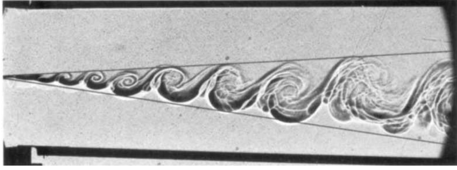
Figure 2.6: Shadowgraph of mixing layer showing measurement of growth rate [17]
