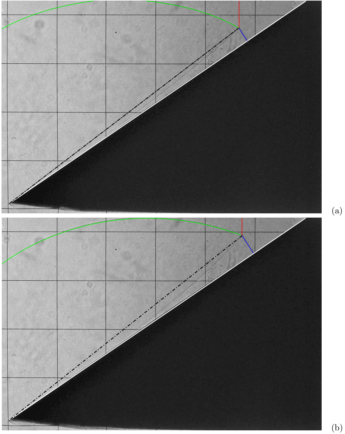
Figure B.3: Single Mach Reflection with highlighted features for the \theta_w = 35^\circ wedge ( Incident Shock , Reflected Shock , Mach Stem , Triple Point Trajectory - Black, Wedge Surface - White): (a) M_s = 1.313 , Time Delay: 1925\mu s (b) M_s = 1.447 , Time Delay: 1750\mu s
