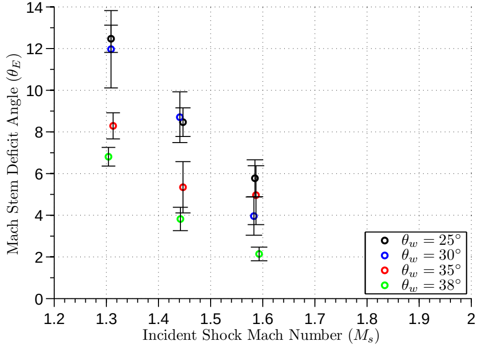
Figure 6.16: \theta_E vs M_s
