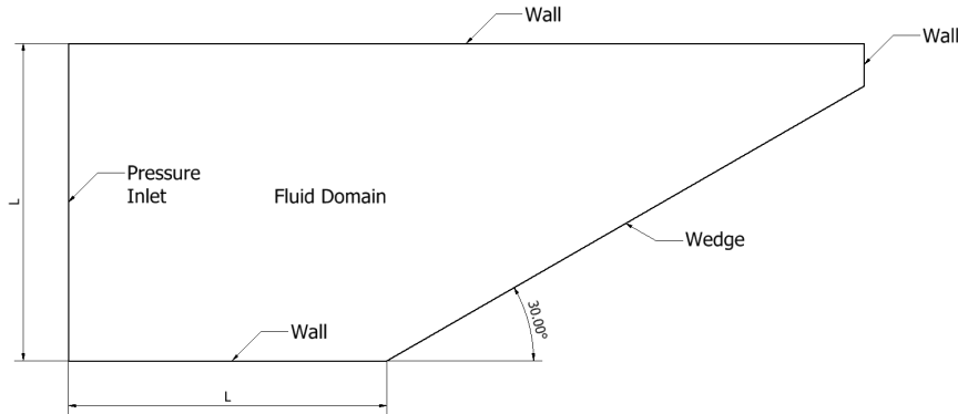
Figure 5.1: A typical geometry for a 30^\circ Wedge
