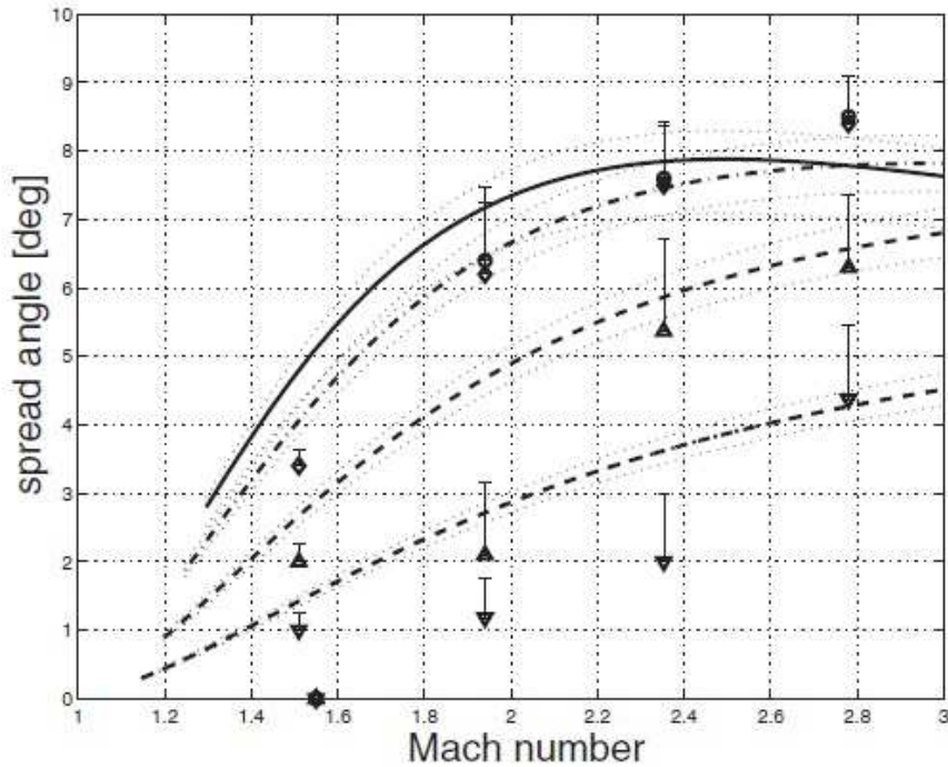
Figure 2.21: Spread angle of the shear layer as a function of Mach number [14]
