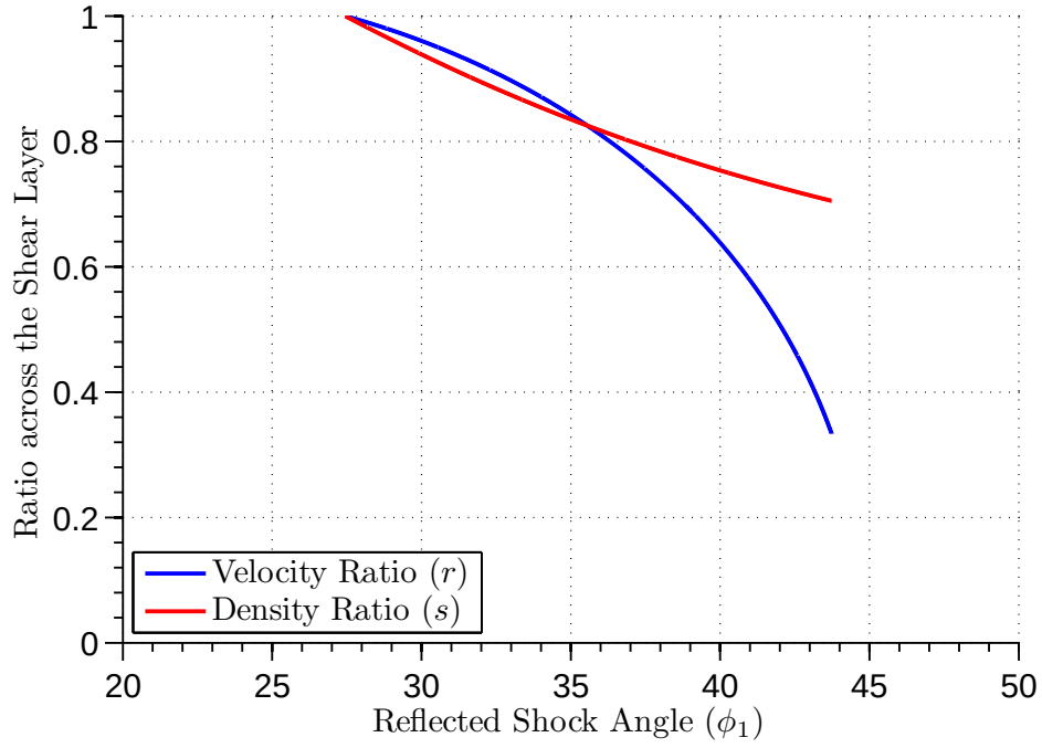
Figure 6.25: Reflected Shock Angle ( \phi_1 ) vs Velocity and Density Ratio
