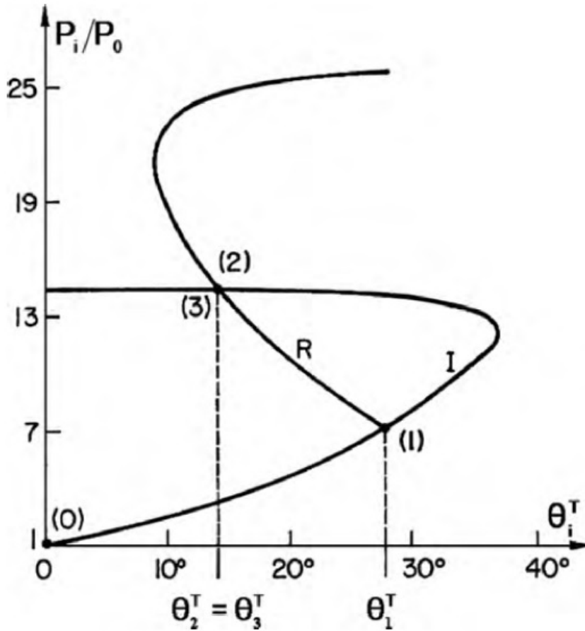
Figure 1.22: Shock Polar solution of a Single Mach Reflection[1]
