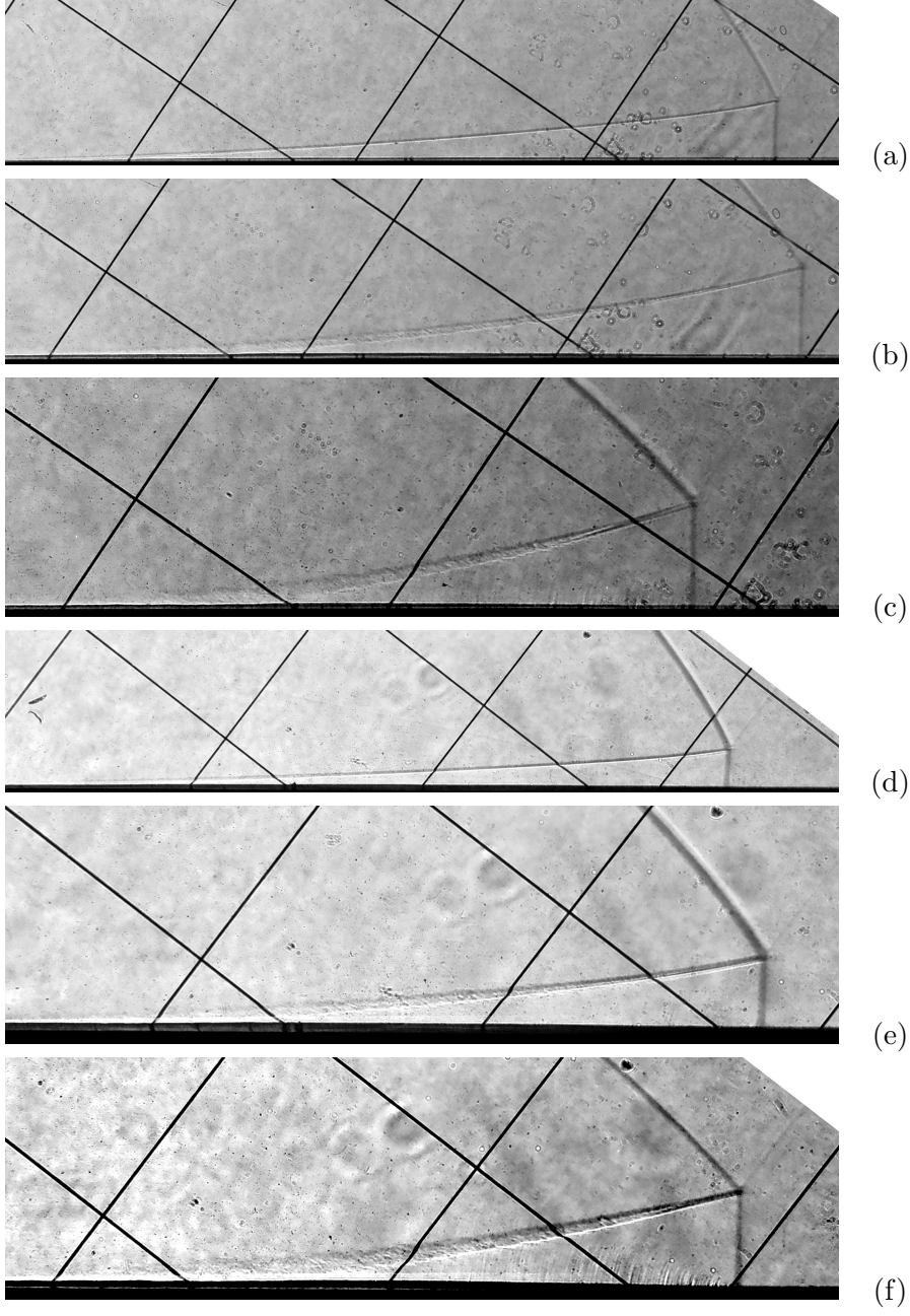
Figure 6.8: Shear layer development for the 35^\circ Wedge. Corresponding Incident Shock Mach number and time delay: (a) M_s = 1.313 , 1925\mu s (b) M_s = 1.447 , 1750\mu s (c) M_s = 1.587 , 1550\mu s . Shear layer development for the 38^\circ Wedge: (d) M_s = 1.304 , 1850\mu s (e) M_s = 1.442 , 1650\mu s (f) M_s = 1.593 , 1500\mu s
