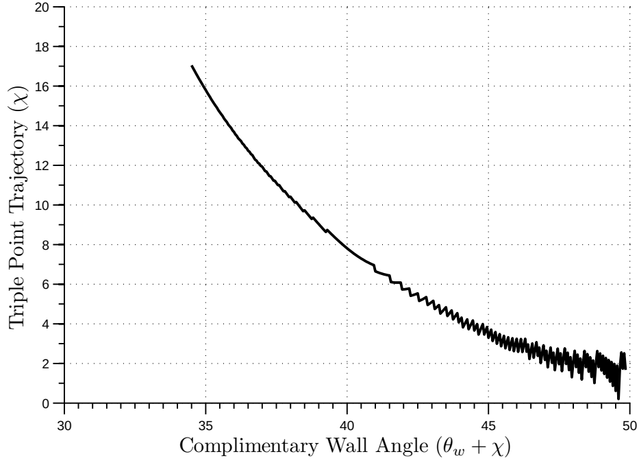
Figure C.2: Triple Point Trajectory ( \chi ) vs Complimentary Wall Angle ( \theta_w + \chi ) for M_s = 1.585
