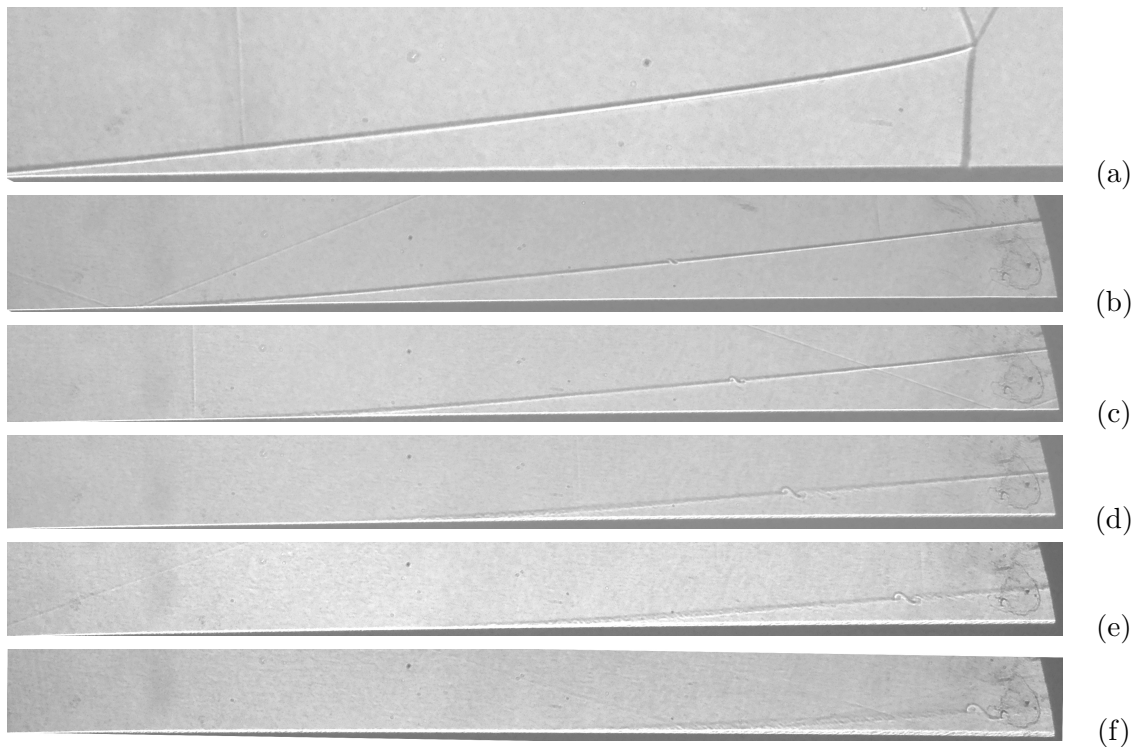
Figure 6.4: Shear layer development for the 30° Wedge. M_s = 1.27 . (a) 3800\mu s , (b) 4000\mu s , (c) 4200\mu s , (d) 4400\mu s , (e) 4600\mu s , (f) 4800\mu s
