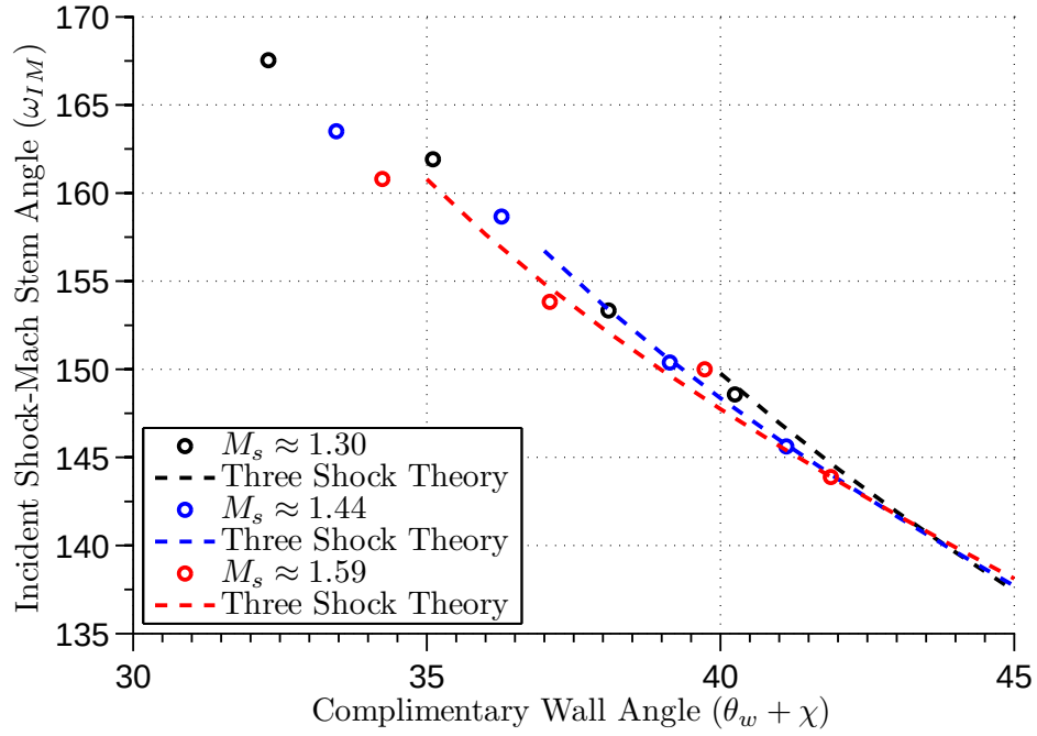
Figure 6.27: Comparison of experimental shock angles to Three Shock Theory for \omega_{IM}
