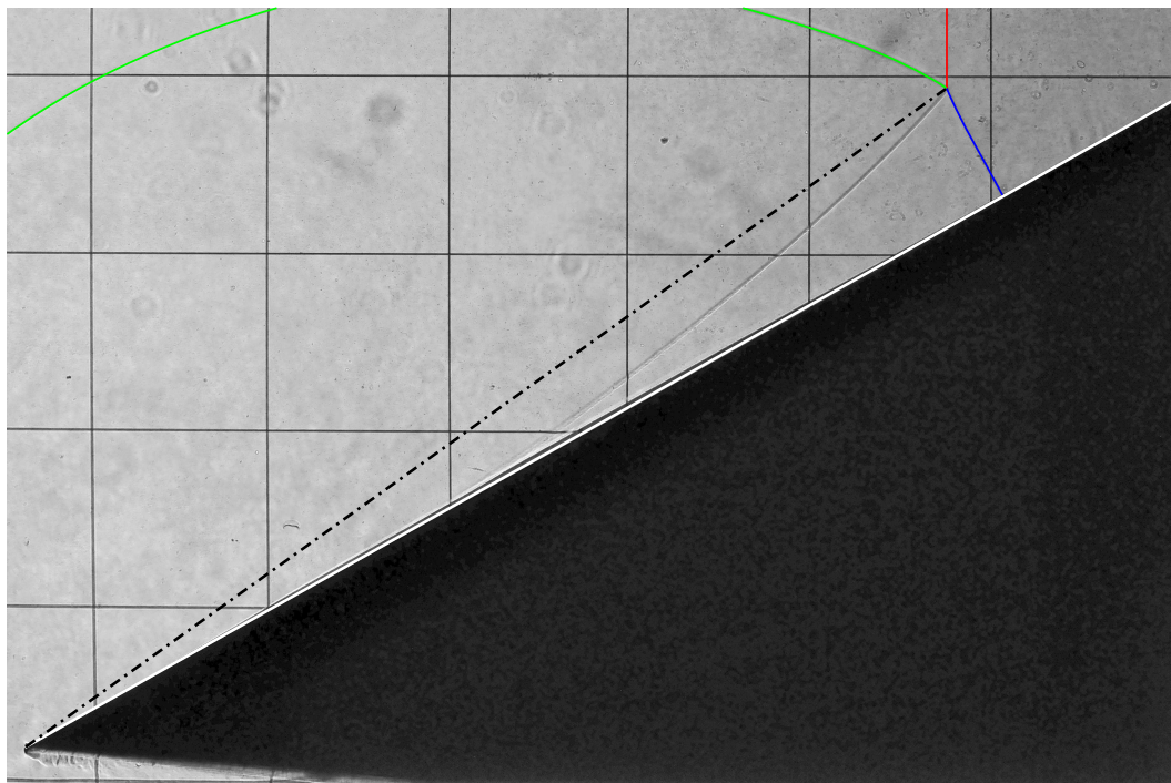
Figure B.2: Single Mach Reflection with highlighted features for the \theta_w = 30^\circ wedge ( Incident Shock , Reflected Shock , Mach Stem , Triple Point Trajectory - Black, Wedge Surface - White): (a) M_s = 1.309 , Time Delay: 1900\mu s (b) M_s = 1.441 , Time Delay: 1700\mu s
