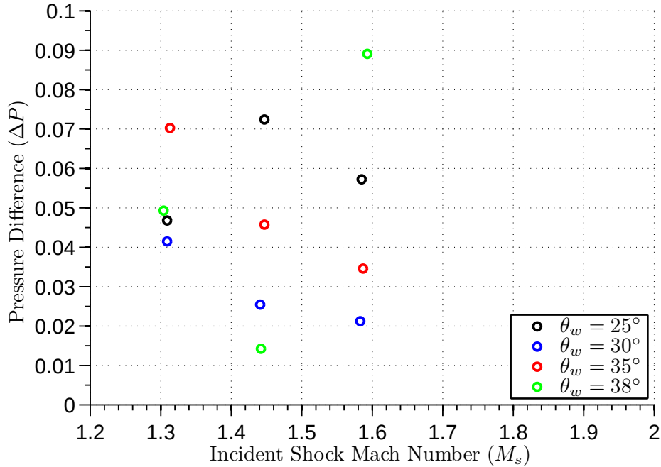
Figure 6.31: Pressure difference across the shear layer
