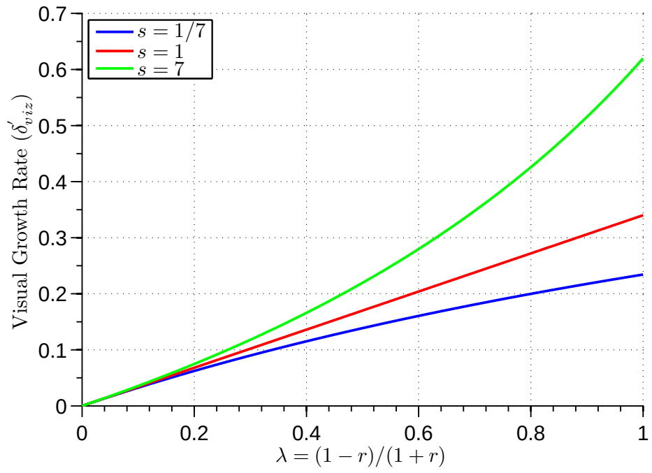
Figure 6.37: Visual Growth Rate ( \delta'_{viz} ) vs \lambda
