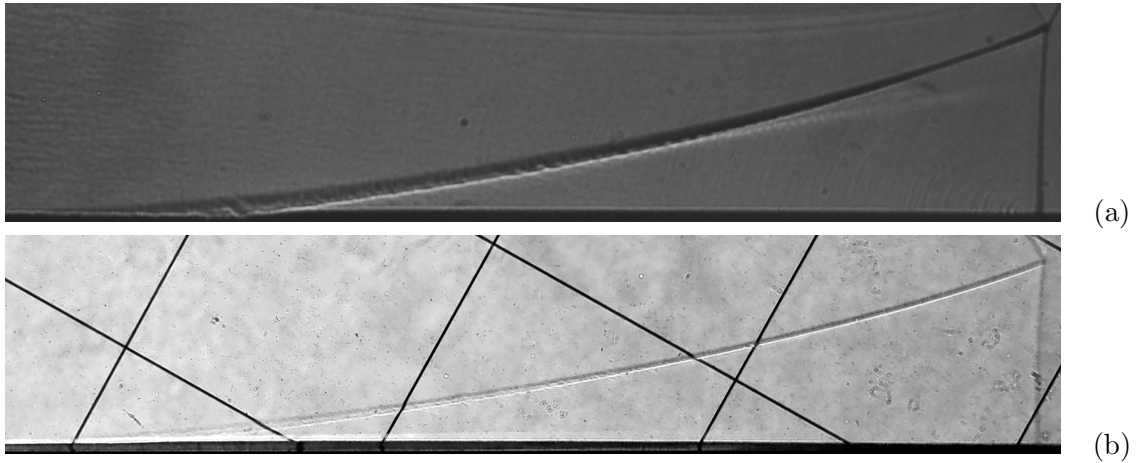
Figure 6.20: Comparison of SMR's obtained at M_s = 1.44 in the (a) LBST (b) MSAST
