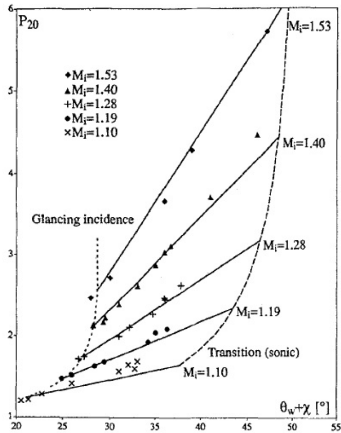
Figure 1.21: Modified three shock theory proposed by Olim and Dewey[12]
