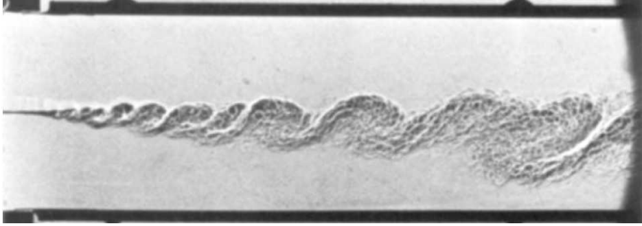
Figure 2.7: Shadowgraph of mixing layer for density ratio of 7 [17]
