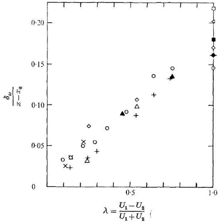
Figure 2.9: Vorticity thickness vs \lambda for s = 1 [17]
