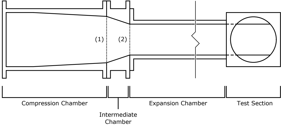
Figure 4.2: Schematic of the Michael Seitz Automated Shock Tube (MSAST)
