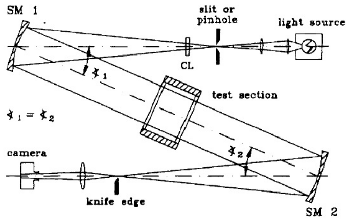
Figure 2.3: Schematic layout of a typical monochrome schlieren visualisation system (adapted from Kleine[16])
