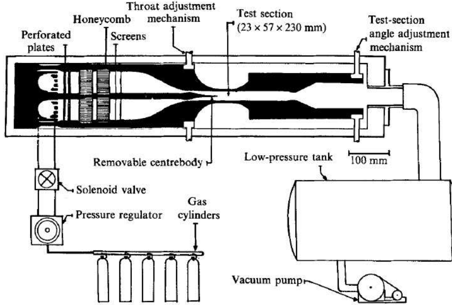
Figure 2.17: Experimental apparatus [22]
