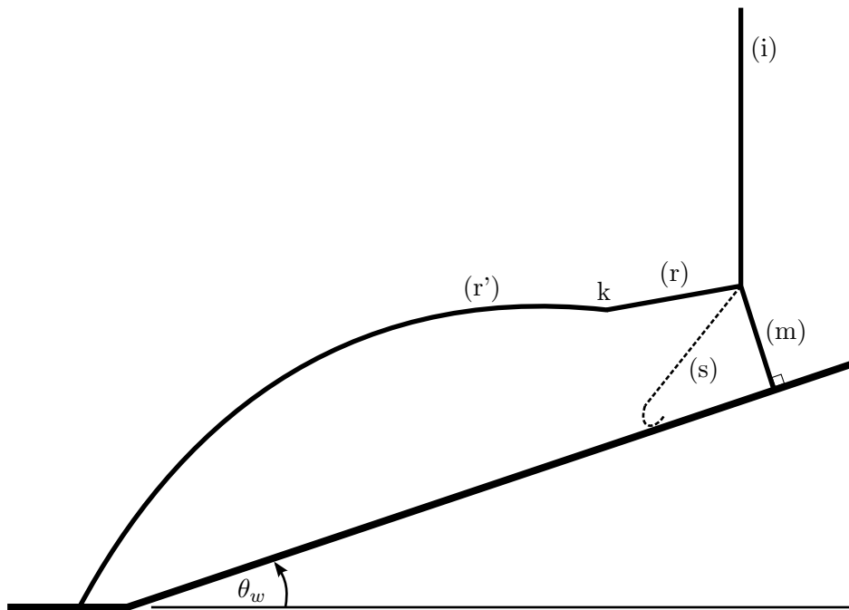
Figure 1.7: Transitional Mach Reflection (TMR)[1]
