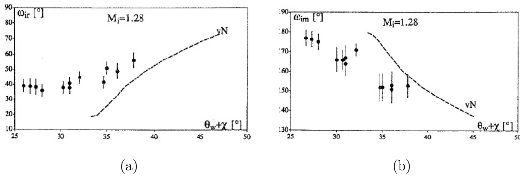
Figure 1.18: Measured shock angles with dashed line calculated from three shock theory[12] (a) \omega_{IR} (b) \omega_{IM}
