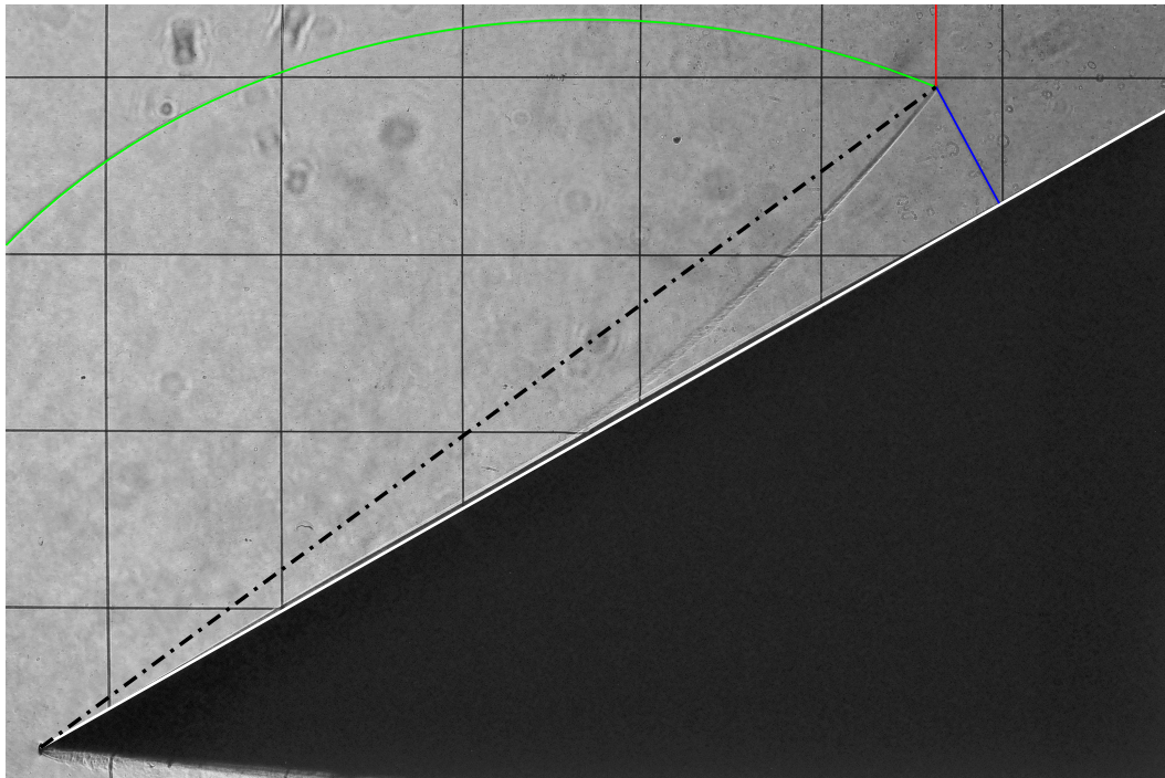
Figure 6.5: Single Mach Reflection with highlighted features ( Incident Shock , Reflected Shock , Mach Stem , Triple Point Trajectory - Black, Wedge Surface - White): (a) \theta_w = 25^\circ . M_s = 1.585 , Time Delay: 1550\mu s (b) \theta_w = 30^\circ . M_s = 1.583 , Time Delay: 1550\mu s
