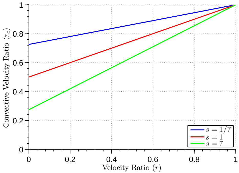
Figure 6.38: Convective Velocity Ratio ( r_c ) vs Velocity Ratio ( r )
