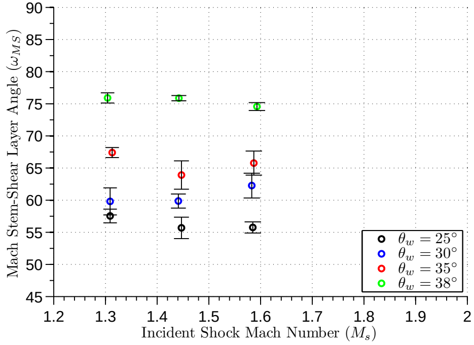
Figure 6.15: \omega_{MS} vs M_s
