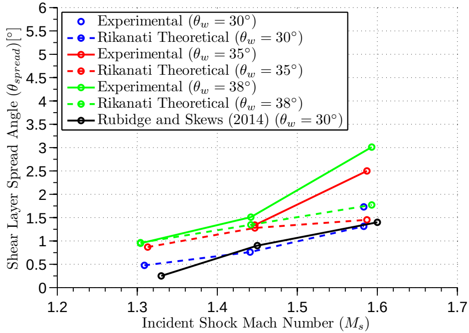
Figure 6.43: Spread angle comparison to theory from Rikanati et al.[14]
