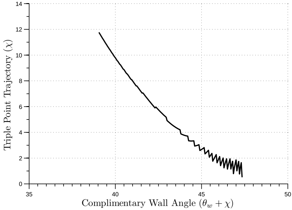
Figure 6.28: Triple Point Trajectory ( \chi ) vs Complimentary Wall Angle ( \theta_w + \chi ) for M_s = 1.30
