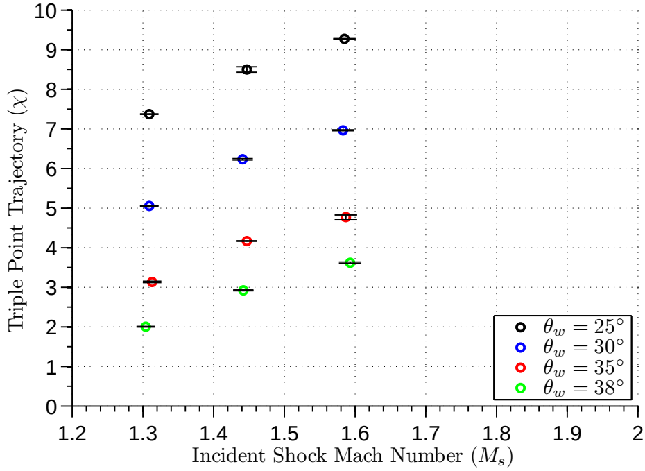
Figure 6.11: \chi vs M_s
