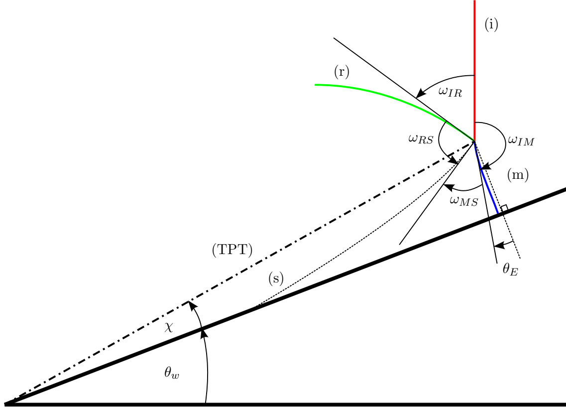
Figure 6.10: Schematic of measured angles
