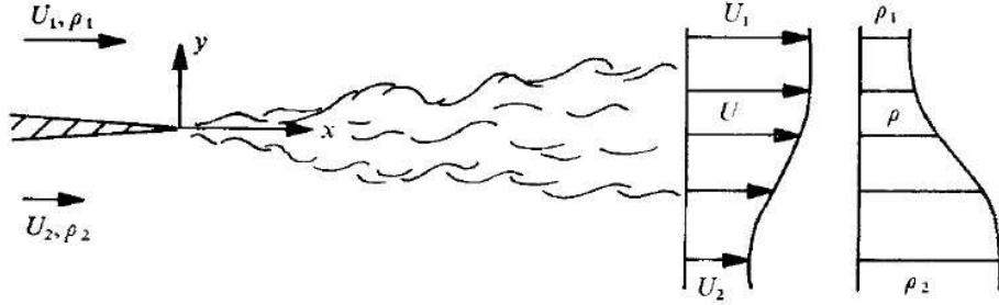
Figure 2.5: Plane mixing layer [17]
