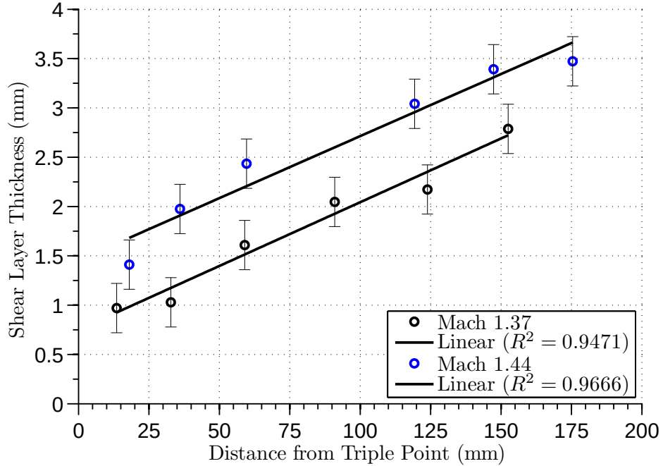
Figure 6.3: Measured Shear Layer Thickness from the LBST
