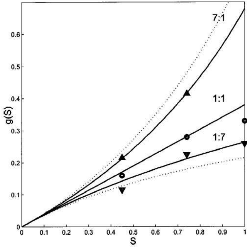
Figure 2.20: Growth rates as a function of S [24] with data from Brown and Roshko[17]. Dotted lines from Dimotakis[20]
