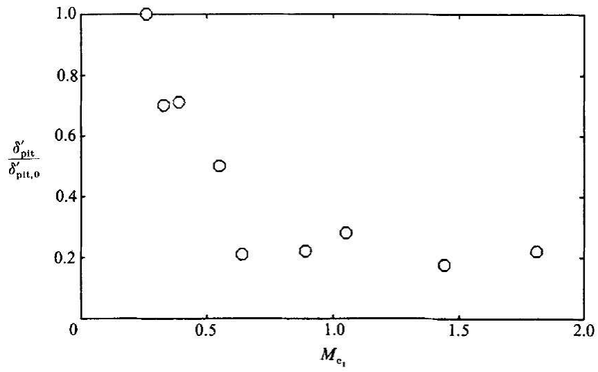
Figure 2.19: Normalised pitot thickness growth rate versus M_{c_1} [22]
