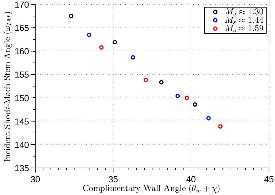
Figure 6.18: \omega_{IM} vs \theta_w + \chi
