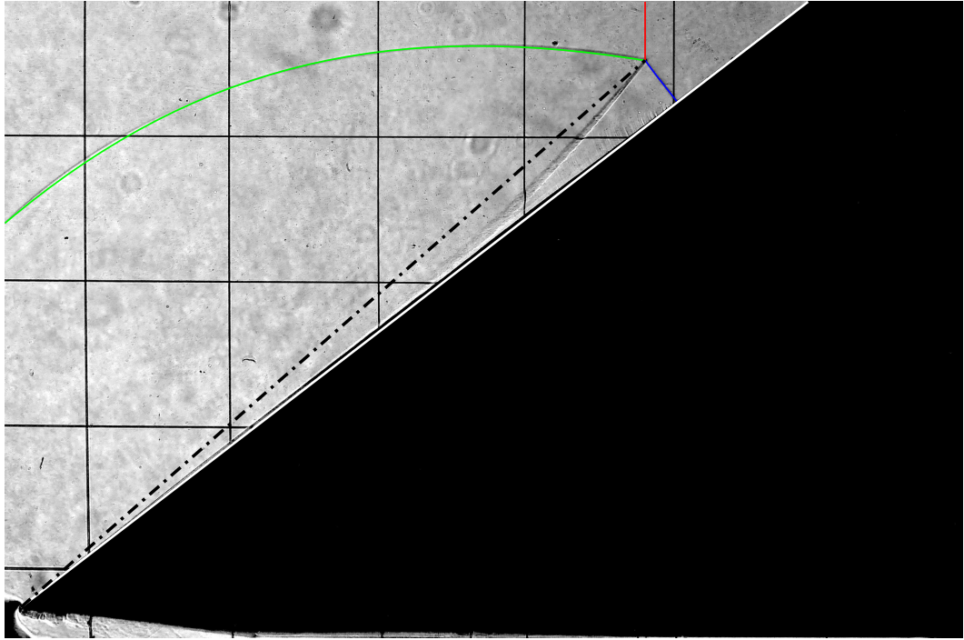
Figure 6.7: Single Mach Reflection with highlighted features ( Incident Shock , Reflected Shock , Mach Stem , Triple Point Trajectory - Black, Wedge Surface - White): (a) \theta_w = 35^\circ . M_s = 1.587 , Time Delay: 1550\mu s (b) \theta_w = 38^\circ . M_s = 1.593 , Time Delay: 1500\mu s
