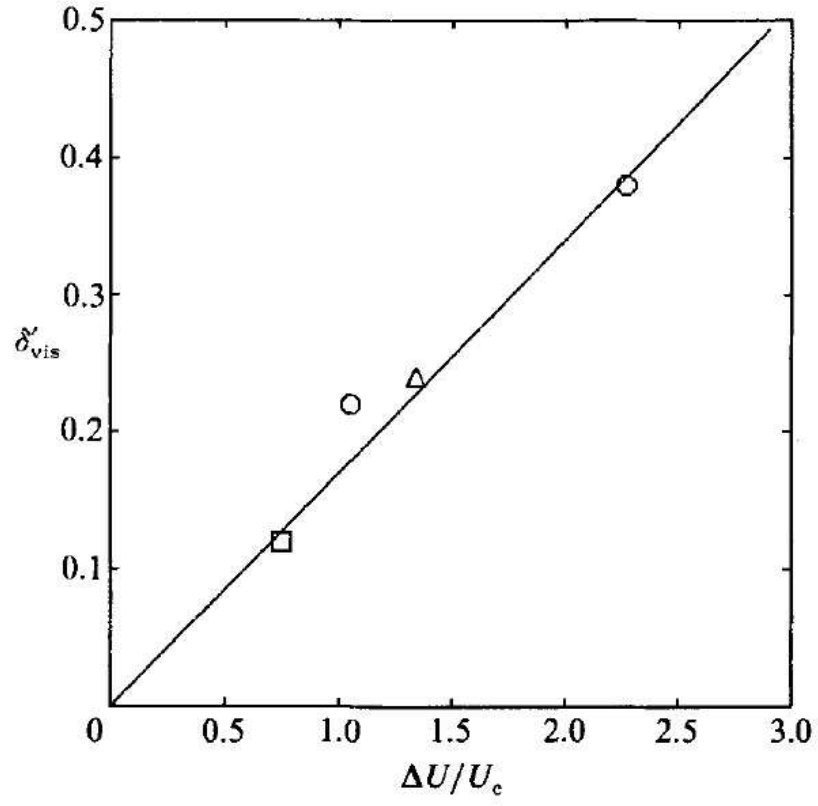
Figure 2.18: Visual thickness growth rate versus \Delta U/U_c [22]
