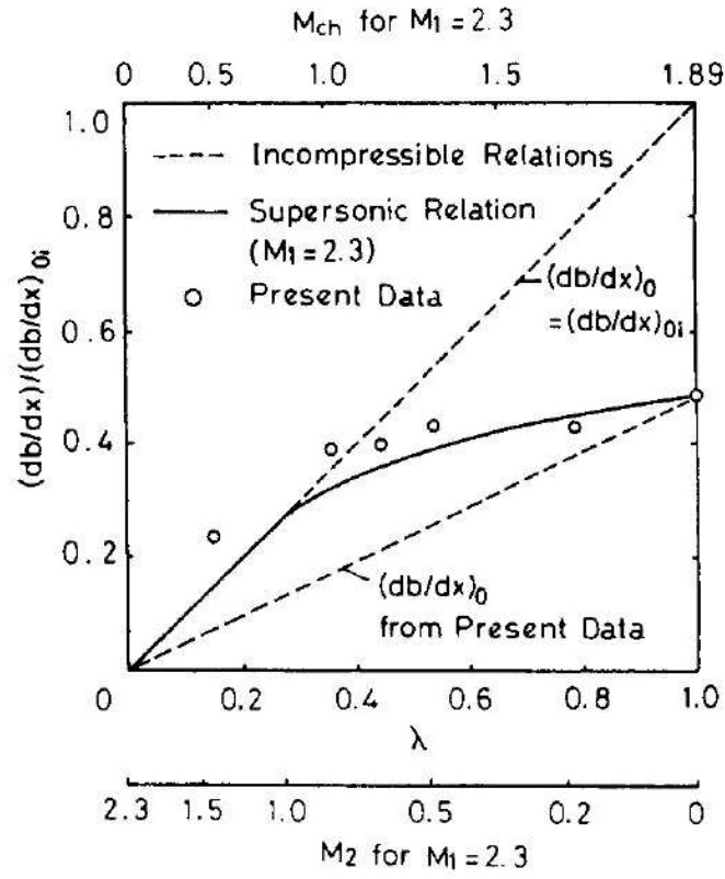
Figure 2.16: Spreading rate variation with \lambda [21]
