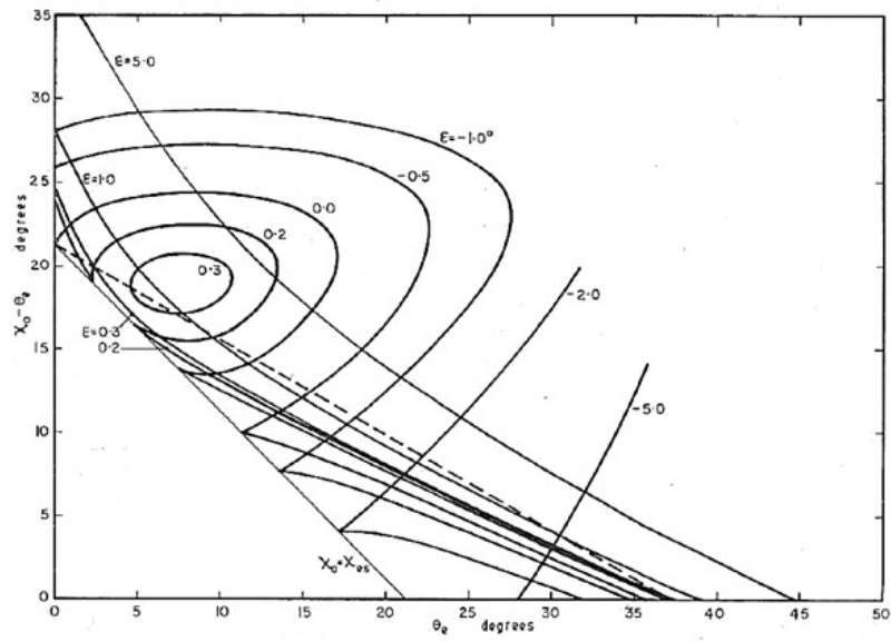
Figure 1.15: Limit curves for values of \epsilon [8]
