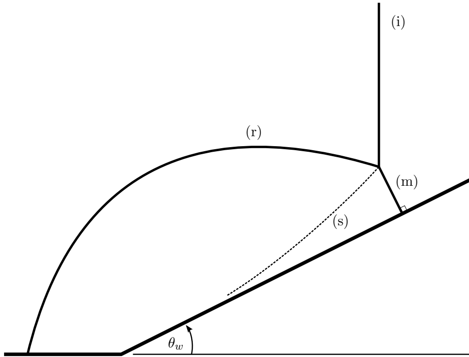
Figure 1.6: Single Mach Reflection (SMR)[1]
