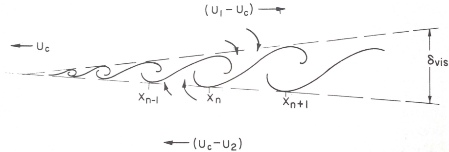
Figure 2.12: Vortex reference frame showing large structures and induced velocities [20]
