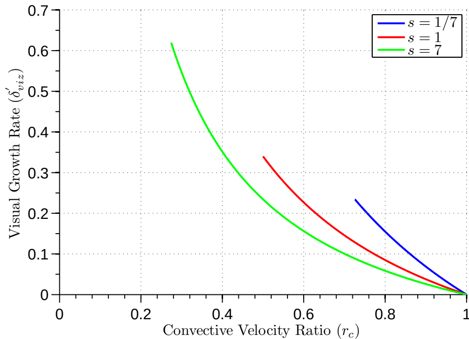
Figure 6.39: Visual Growth Rate ( \delta'_{viz} ) vs Convective Velocity Ratio ( r_c )
