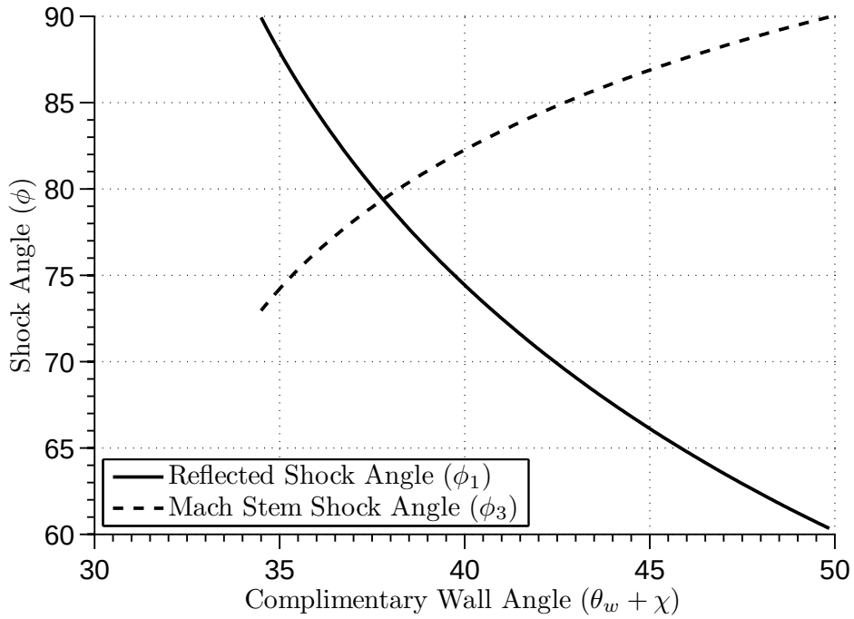
Figure C.6: Shock Angle ( \phi ) vs Complimentary Wall Angle ( \theta_w + \chi ) for M_s = 1.585
