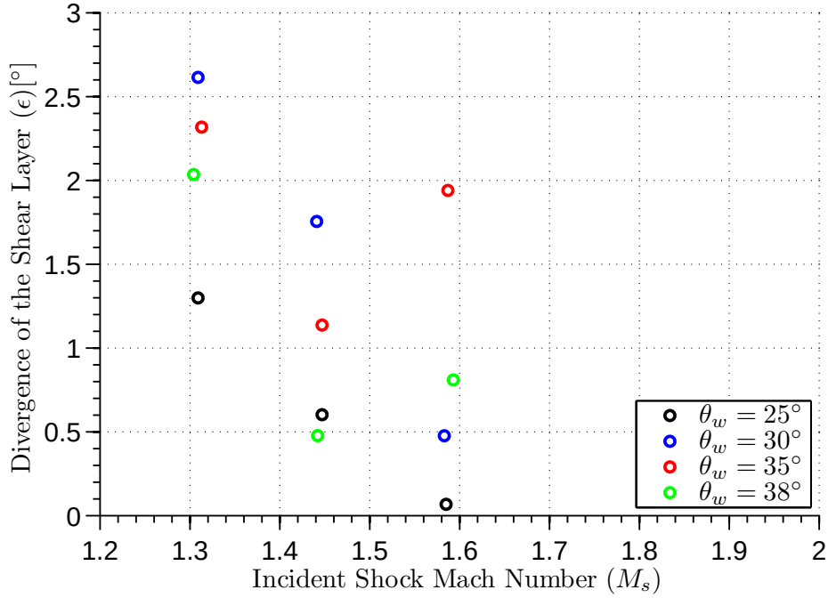
Figure 6.32: Divergence across the Shear Layer
