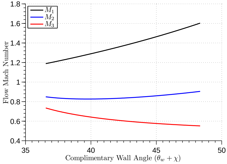
Figure C.3: Flow Mach Number vs Complimentary Wall Angle ( \theta_w + \chi ) for M_s = 1.44
