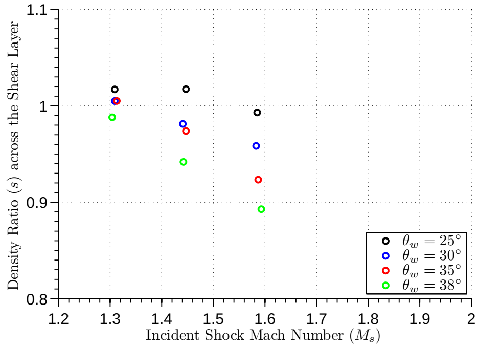
Figure 6.36: Density Ratio across the Shear Layer
