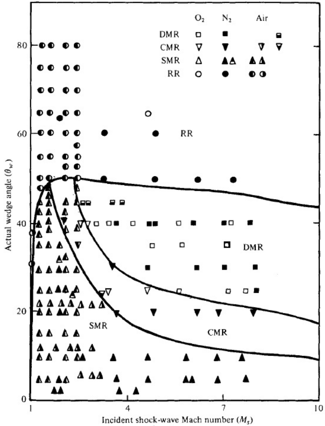
Figure 1.8: Experimental verification of analytical transition criteria for imperfect Nitrogen and other gases. P_0 = 15 torr, T_0 = 300\text{K} [2]
