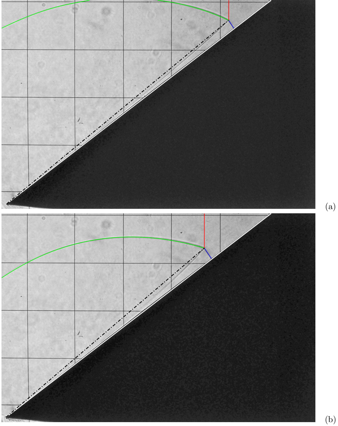
Figure B.4: Single Mach Reflection with highlighted features for the \theta_w = 38^\circ wedge ( Incident Shock , Reflected Shock , Mach Stem , Triple Point Trajectory - Black, Wedge Surface - White): (a) M_s = 1.304 , Time Delay: 1850\mu s (b) M_s = 1.442 , Time Delay: 1650\mu s
