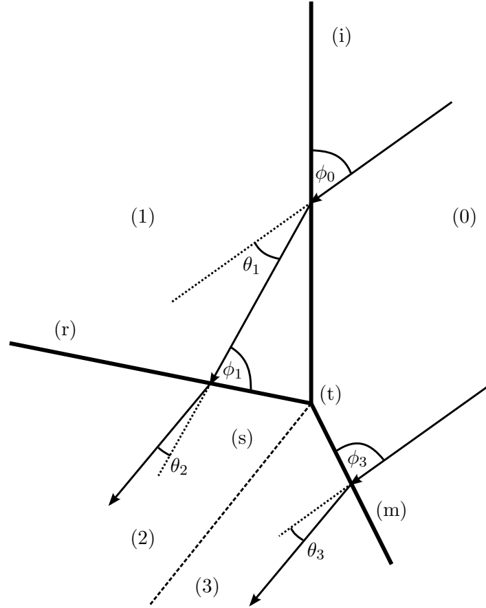
Figure 6.21: Confluence of three shocks at the triple point of a Mach Reflection with definition of angles and flow regions
