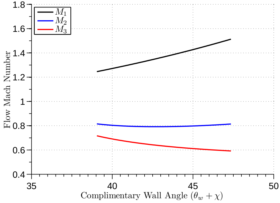
Figure 6.29: Flow Mach Number vs Complimentary Wall Angle ( \theta_w + \chi ) for M_s = 1.30
