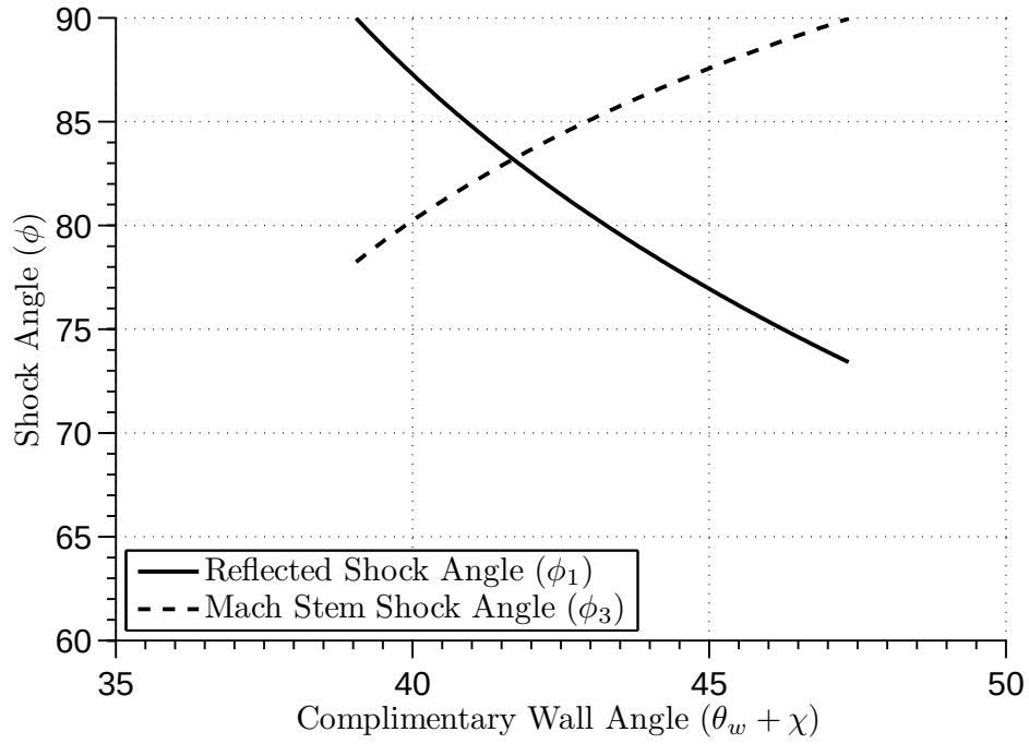
Figure 6.30: Shock Angle ( \phi ) vs Complimentary Wall Angle ( \theta_w + \chi ) for M_s = 1.30
