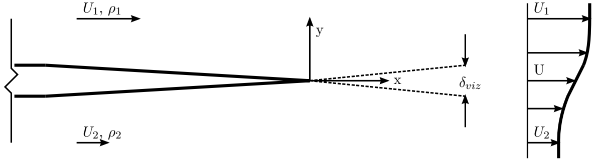
Figure 2.4: Schematic of a plane shear layer with definition of some parameters (adapted from Brown and Roshko[17])
