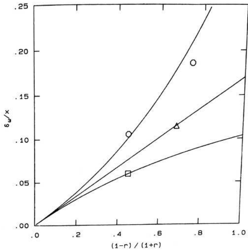
Figure 2.13: Vorticity (maximum slope) thickness for s = 1/7, 1, 7 [20]
