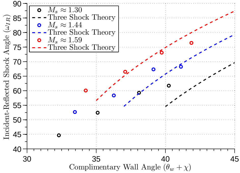
Figure 6.26: Comparison of experimental shock angles to Three Shock Theory for \omega_{IR}
