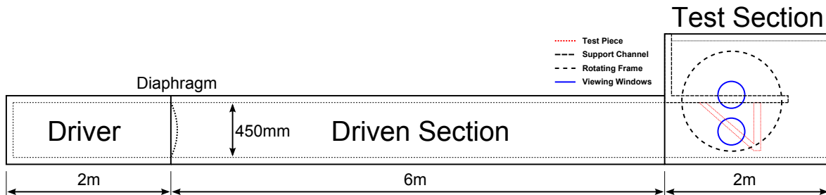
Figure 4.1: Large Blue Shock Tube Schematic
