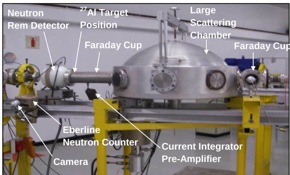
Figure 3.3 Part of the C-line experimental set-up to measure neutron yield from the ^{27}\text{Al}(\text{p},\text{n})^{27}\text{Si} reaction.
