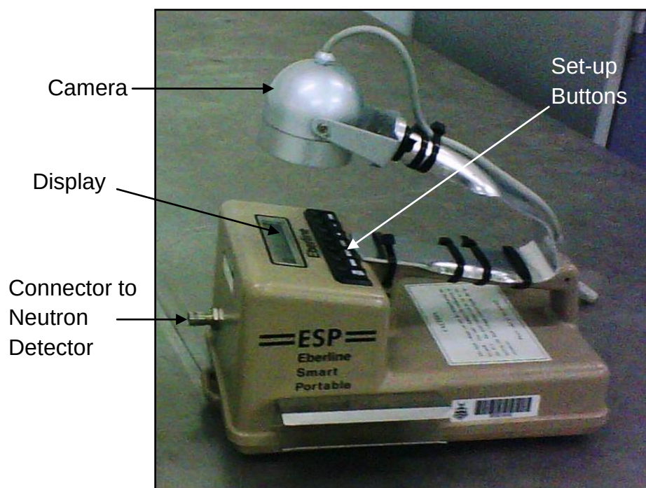
Figure 3.5 Photograph of the Eberline Smart Portable (ESP1) neutron counter which was used in the ^{27}\text{Al}(p,n)^{27}\text{Si} reaction.
