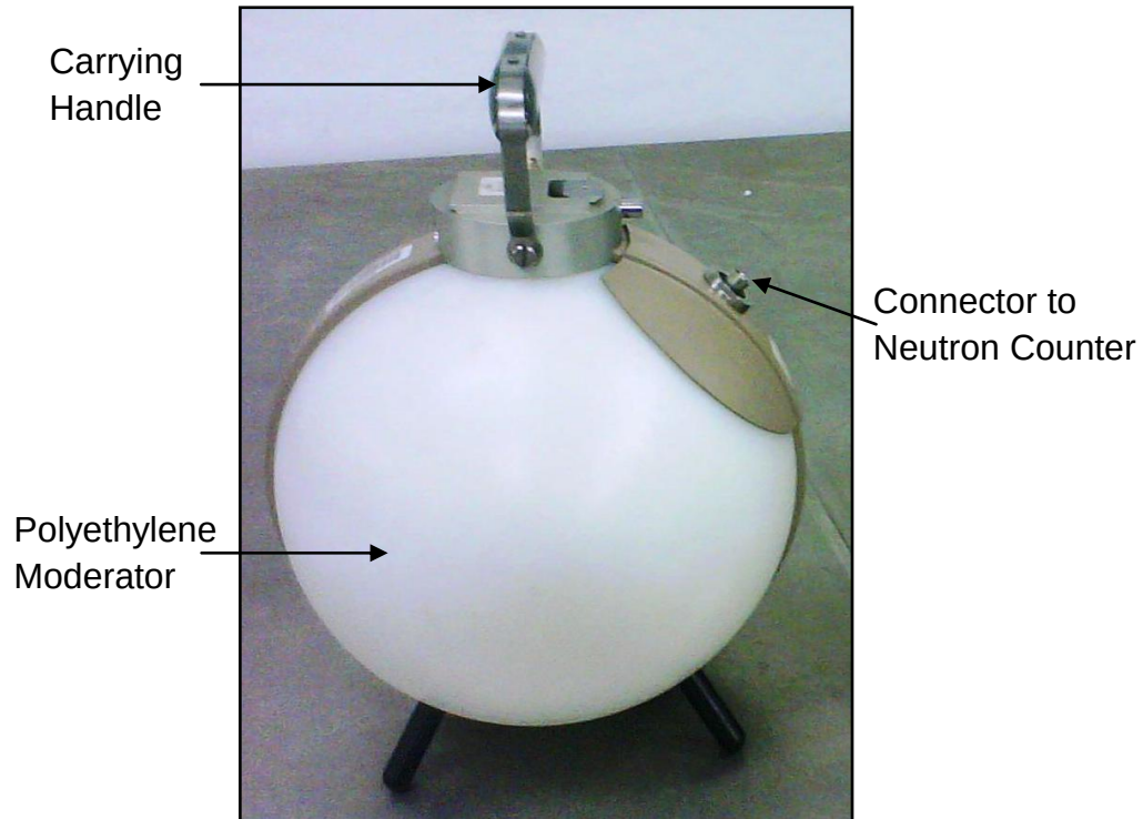
Figure 3.4 Photograph of the Eberline Neutron Rem Detector which was used to detect neutrons in the ^{27}\text{Al}(p,n)^{27}\text{Si} reaction.
