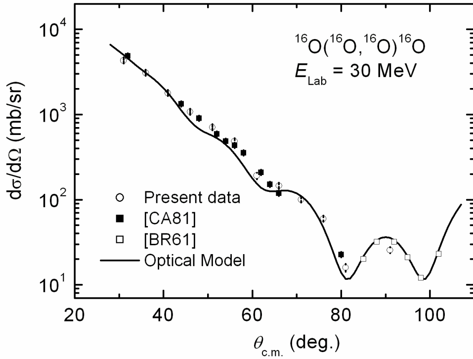
Figure 3.14 Angular distribution for the elastic scattering of ^{16}\text{O} from ^{16}\text{O} at E_{\text{Lab}} = 30 \text{ MeV} . The solid curves show Upper : the symmetrised ratio-to-Mott optical model calculations using the parameters shown in Table 3.4. Lower : symmetrised optical model prediction.
