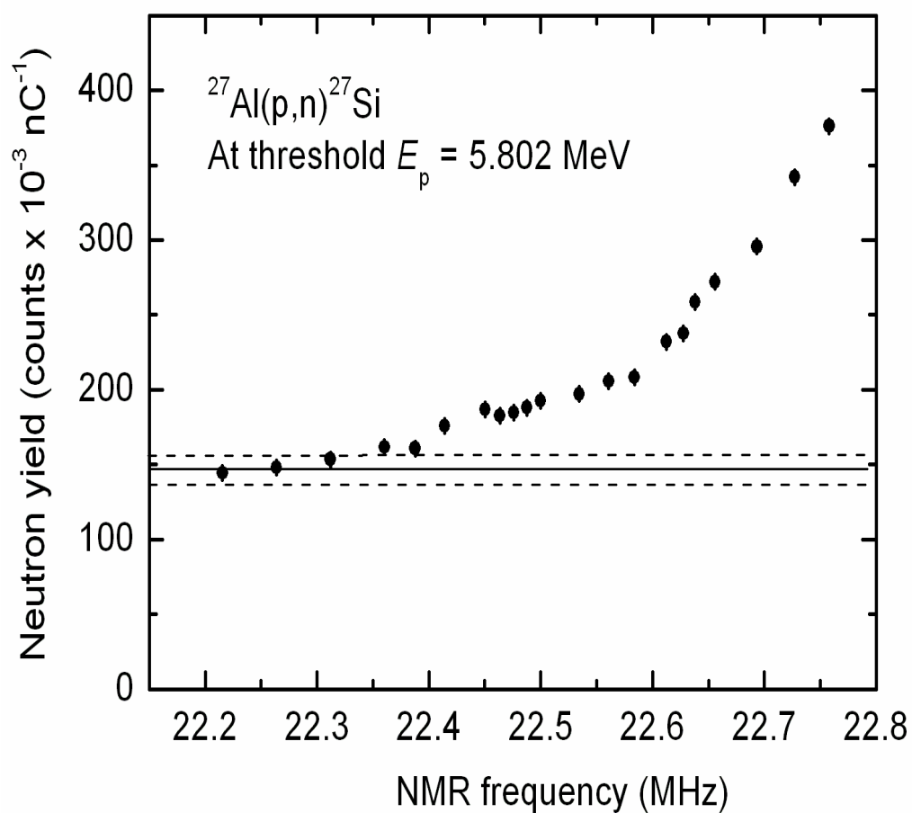
Figure 3.6 Normalised neutron yield for the ^{27}\text{Al}(p,n)^{27}\text{Si} reaction, plotted as a function of NMR frequency. The constant background is shown by the solid line with the upper and lower limits indicated by the dashed lines.
