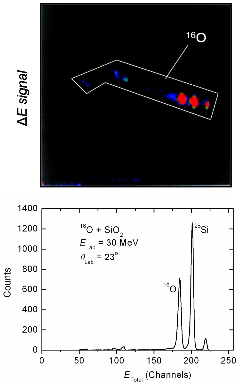
Figure 3.13 Upper: Two-dimensional \Delta E versus E_{\text{Total}} spectrum of ^{16}\text{O} + \text{SiO}_2 . Lower: Projected one-dimensional spectrum at E_{\text{Lab}} = 30 \text{ MeV} and \theta_{\text{Lab}} = 23^\circ .
