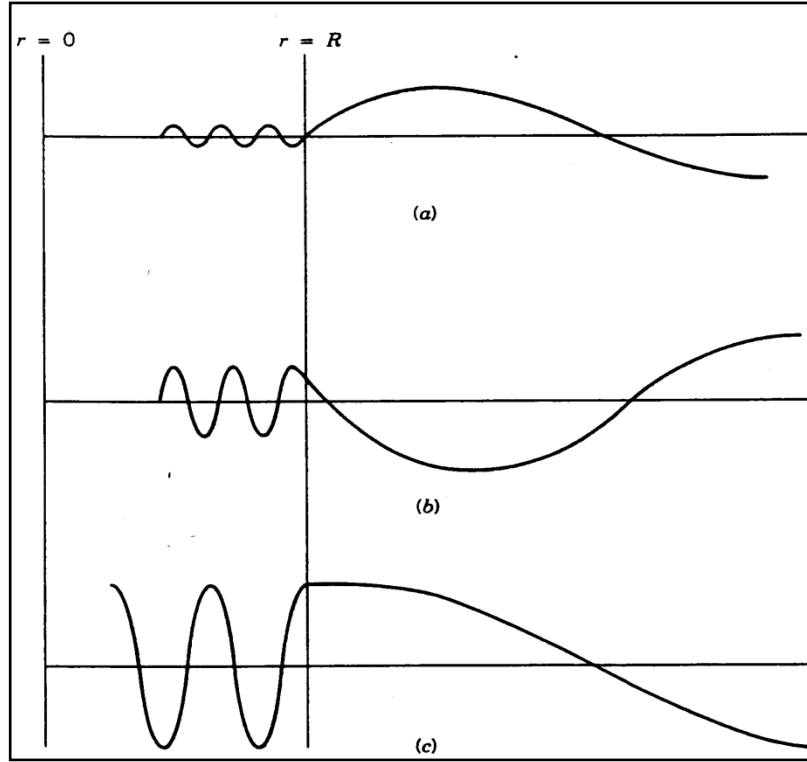
Figure 2.3 (a) Far from resonance, the exterior and interior wave-functions match badly, and little penetration of the nucleus occurs. (b) As the match improves, there is a higher probability to penetrate. (c) At resonance the amplitudes match exactly, the incident particle penetrates easily, and the cross-section rises to a maximum [KR88].
