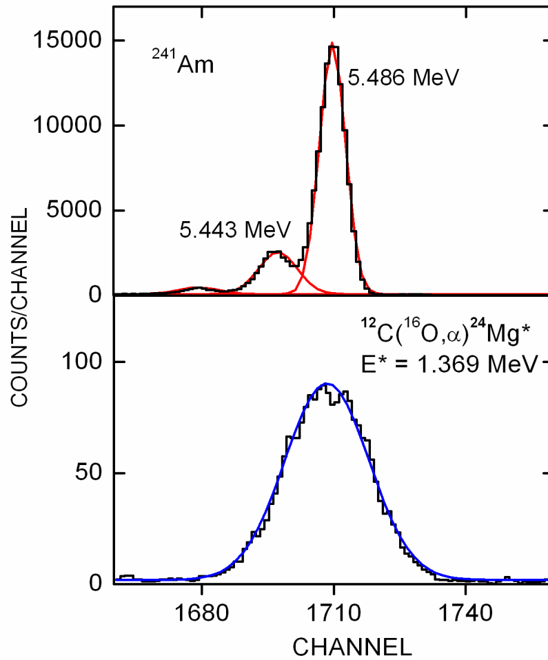
Figure 3.10 Upper: Main peaks from an ^{241}\text{Am} \alpha -source. Lower: Enlarged view of the alpha group for the ^{24}\text{Mg}^* level at 1.369 MeV of excitation. Gaussian curve fittings are shown around each peak.
