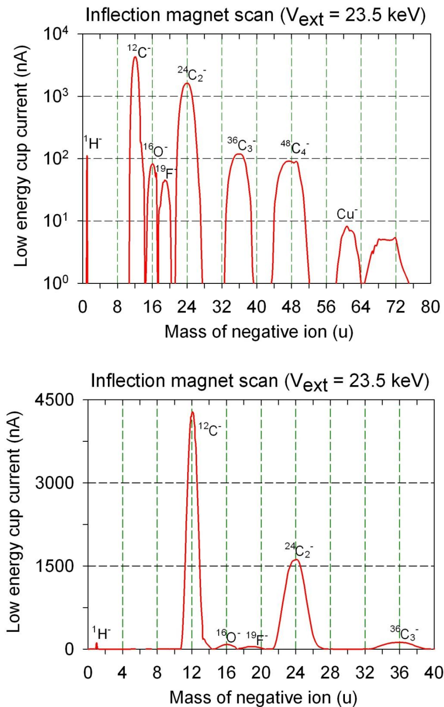
Figure 3.2 Upper: Log plot of ion source species identified, using a graphite target in an 860C negative sputter ion-source with source extraction voltage ( V_{\text{ext}} = 23.5 keV). Lower: Linear plot of ion source species identified, using a graphite target in an 860C negative sputter ion-source with source extraction voltage ( V_{\text{ext}} = 23.5 keV).
