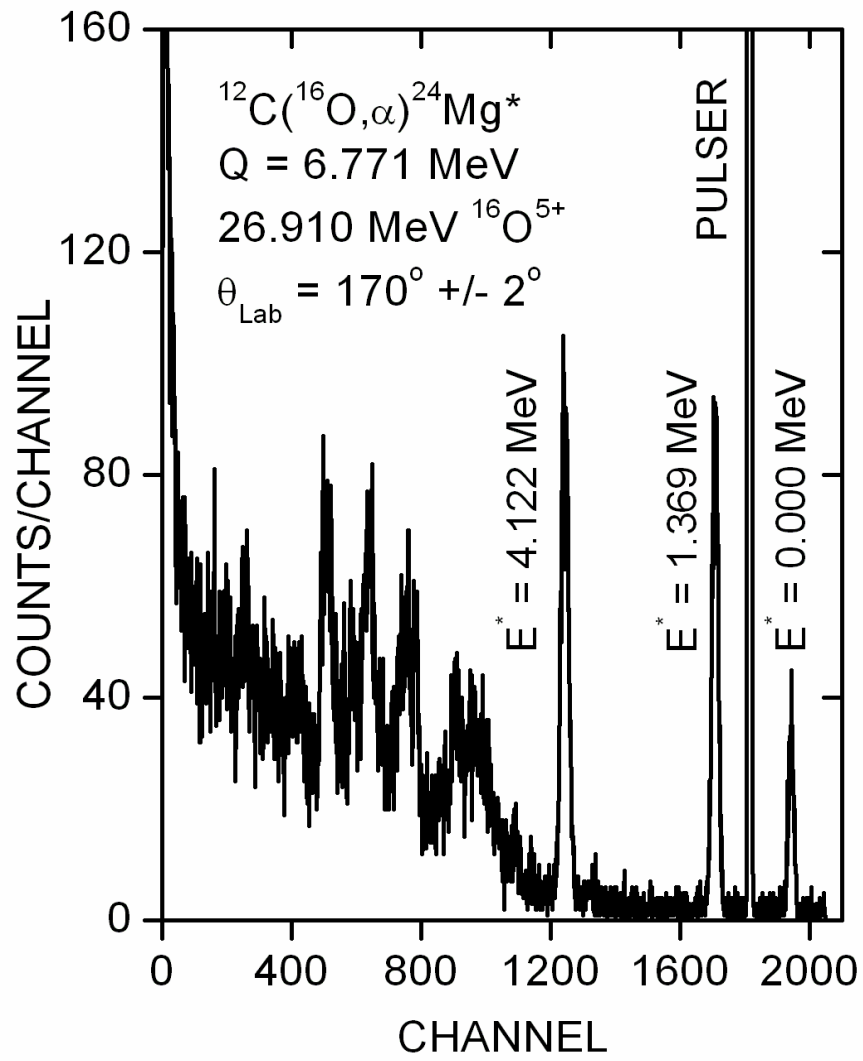
Figure 3.9 Measured energy spectrum from the ^{12}\text{C}(^{16}\text{O},\alpha)^{24}\text{Mg}^* reaction.
