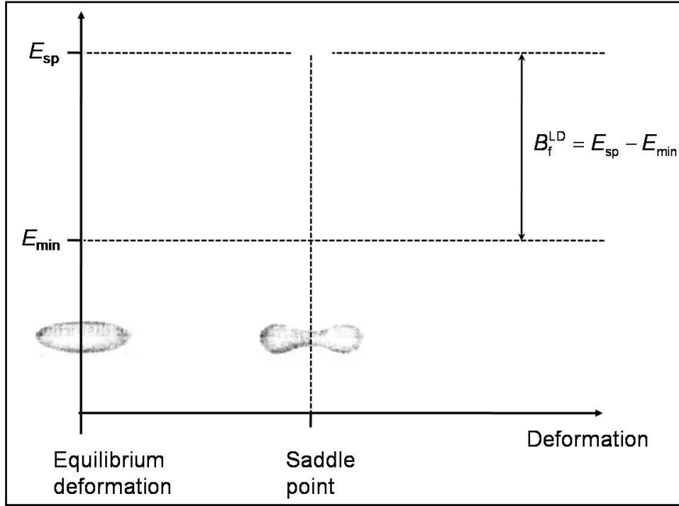
Figure 2.2 An illustration of fission decay of a compound nucleus.
