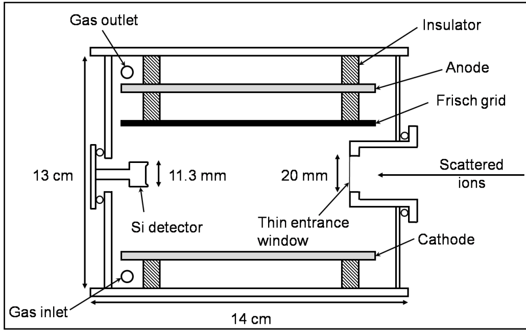
Figure 3.11 Schematic diagram of the \Delta E - E gas-ionisation detector.
