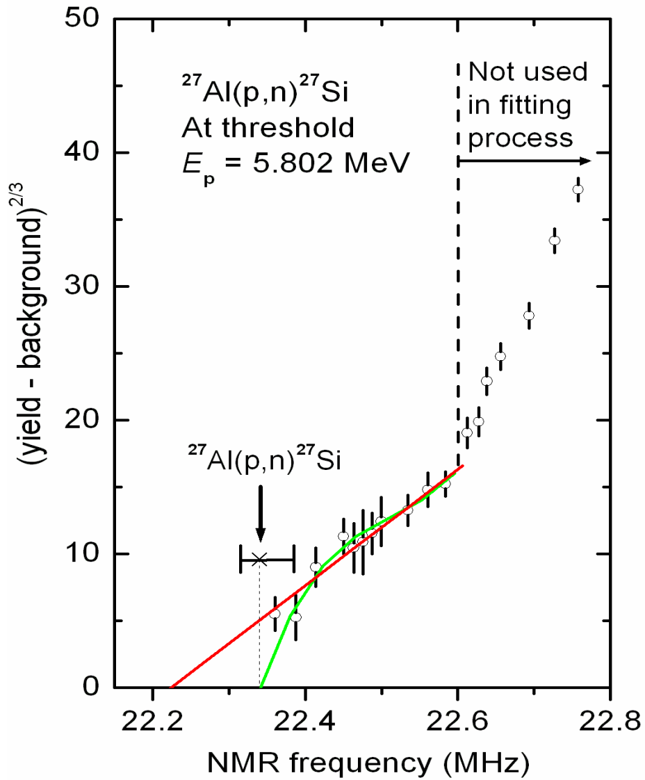
Figure 3.7 Threshold curve for the ^{27}\text{Al}(p,n)^{27}\text{Si} reaction, showing (Y-B)^{2/3} , where Y is the neutron yield and B is the mean background, plotted as a function of NMR frequency. The error bar on the ^{27}\text{Al}(p,n)^{27}\text{Si} measurement is determined by the upper and lower limits of background subtraction (see Fig. 3.6).
