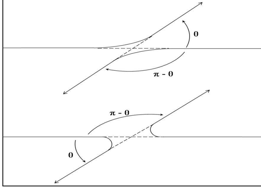
Figure 2.4 Identical particle scattering resulting in two indistinguishable events.
