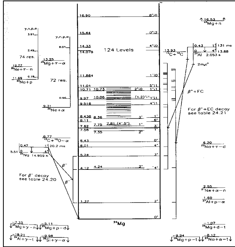
Figure 3.8 Energy levels of ^{24}\text{Mg} [EN90].
