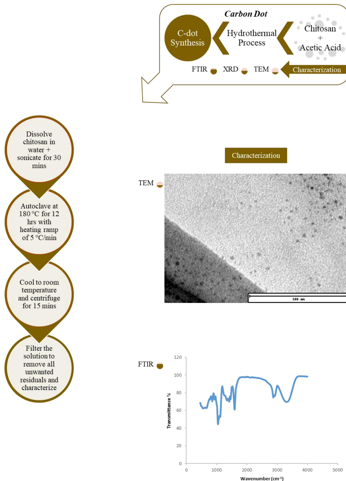
Figure 3.2 The flow diagram of C-dot synthesis and its characterization
