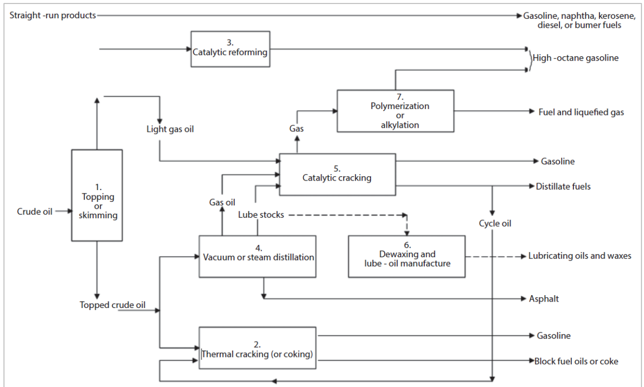
Figure 2.8 Basic Refinery Operations (Coker, 2021)
