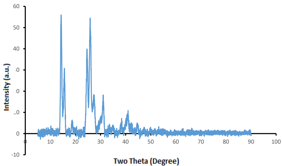
Figure A.3 XRD of h-BN synthesized by CVD method calcined at 700 °C
