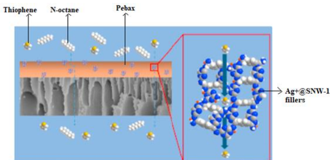
Figure 2.28 Facilitated transport of Thiophenic compounds through Pebax MMM (Pan et al., 2018 )
