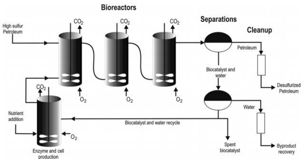
Figure 2.24 Biodesulfurization Process Operations (Boniek et al. 2015)
