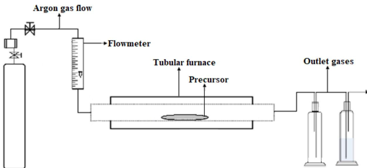
Figure 3.6 Horizontal CVD method for h-BN synthesis
