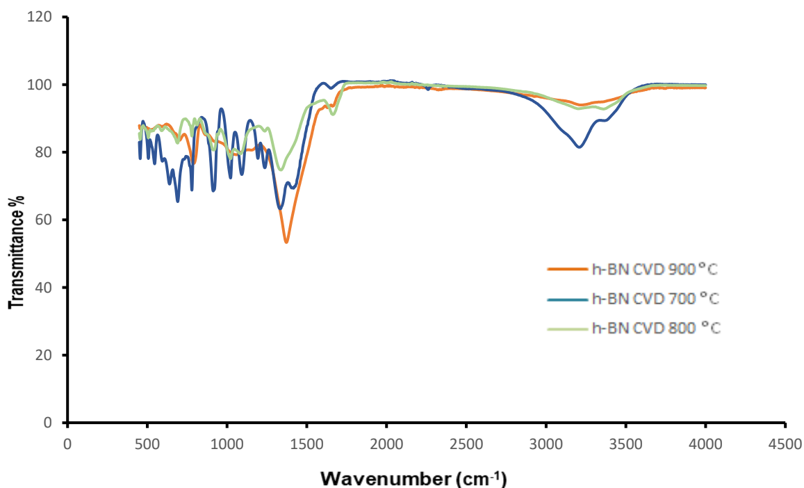
Figure 3.10 FTIR spectra of h-BN synthesized using CVD method at different temperatures
