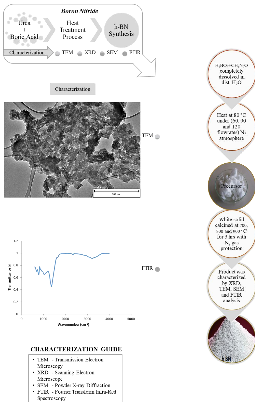
Figure 3.1 The flow diagram of h-BN synthesis and its characterization
