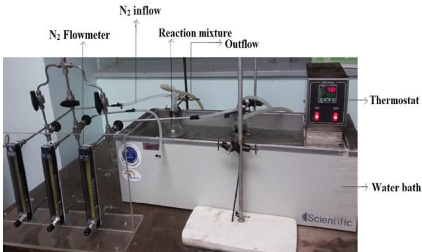
Figure 3.5 Water bath set up for precursor preparation
