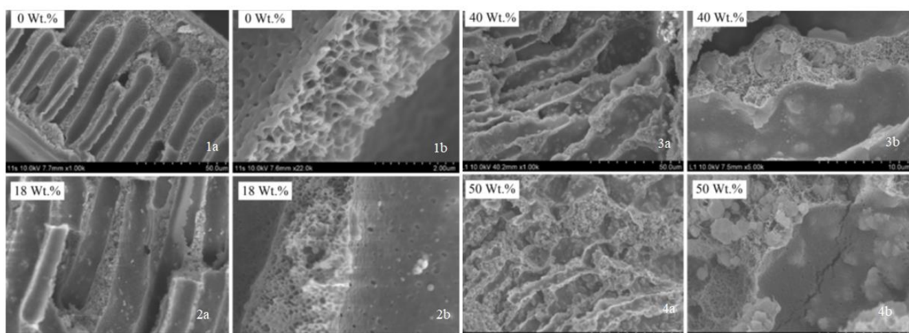
Figure 2.26 FESEM images of cross-sections of raw PI and zeolites/PI MMMs adsorbents: (1) 0 wt.%, (2) 18 wt.%, (3) 40 wt.%, and (4) 50 wt.% (Lin et al., 2012)
