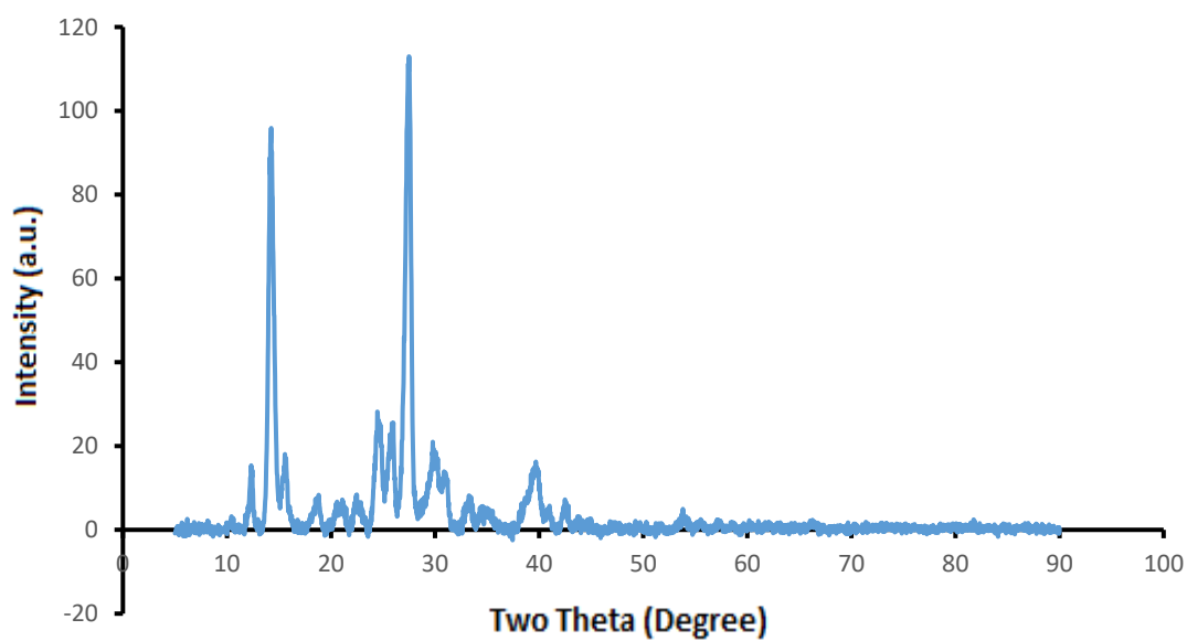
Figure A.2 XRD of h-BN synthesized by HTF method calcined at 800 °C
