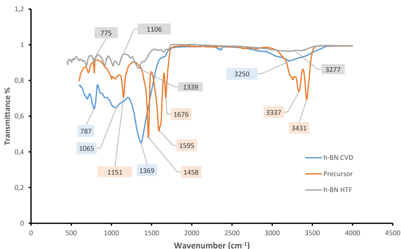
Figure 3.11 The FTIR spectra of precursor formed from urea, boric acid before heat treatment and final h-BN product from CVD and HTF methods heated at 900 °C
