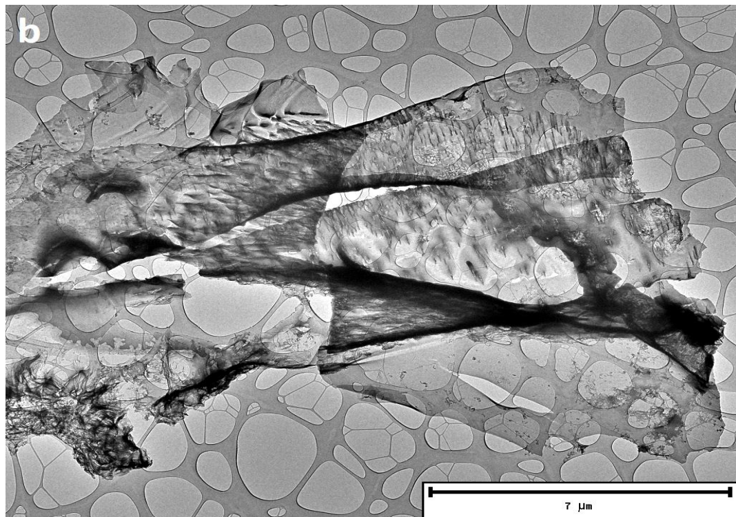
Figure 3.12 TEM images of h-BN CVD (900 °C) (a) showing stacked layer like structures, and (b) h-BN with multiple crumpled layers
