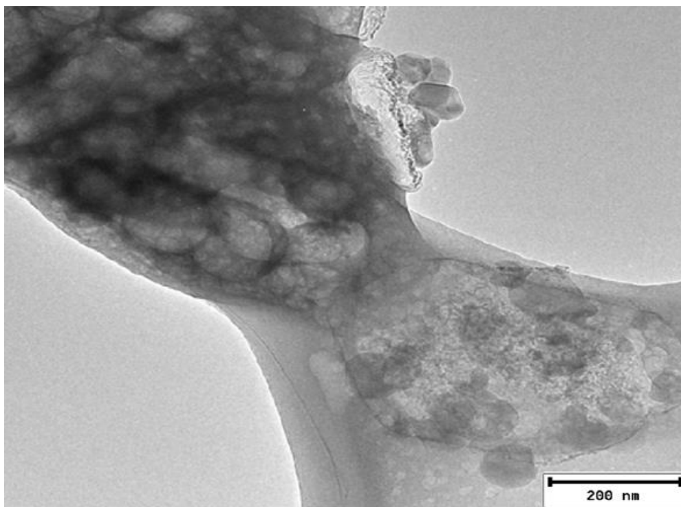
Figure A.5 TEM image of h-BN calcined by HTF (800 °C)
