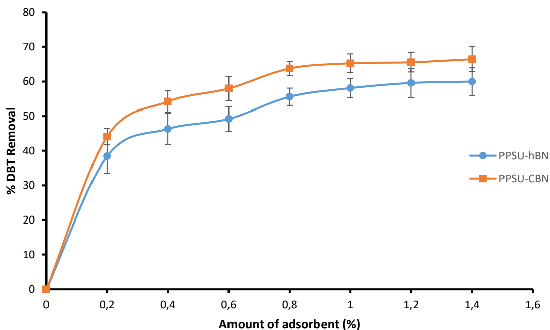
Figure 5.3 Desulfurisation behaviour with adsorbent amount
