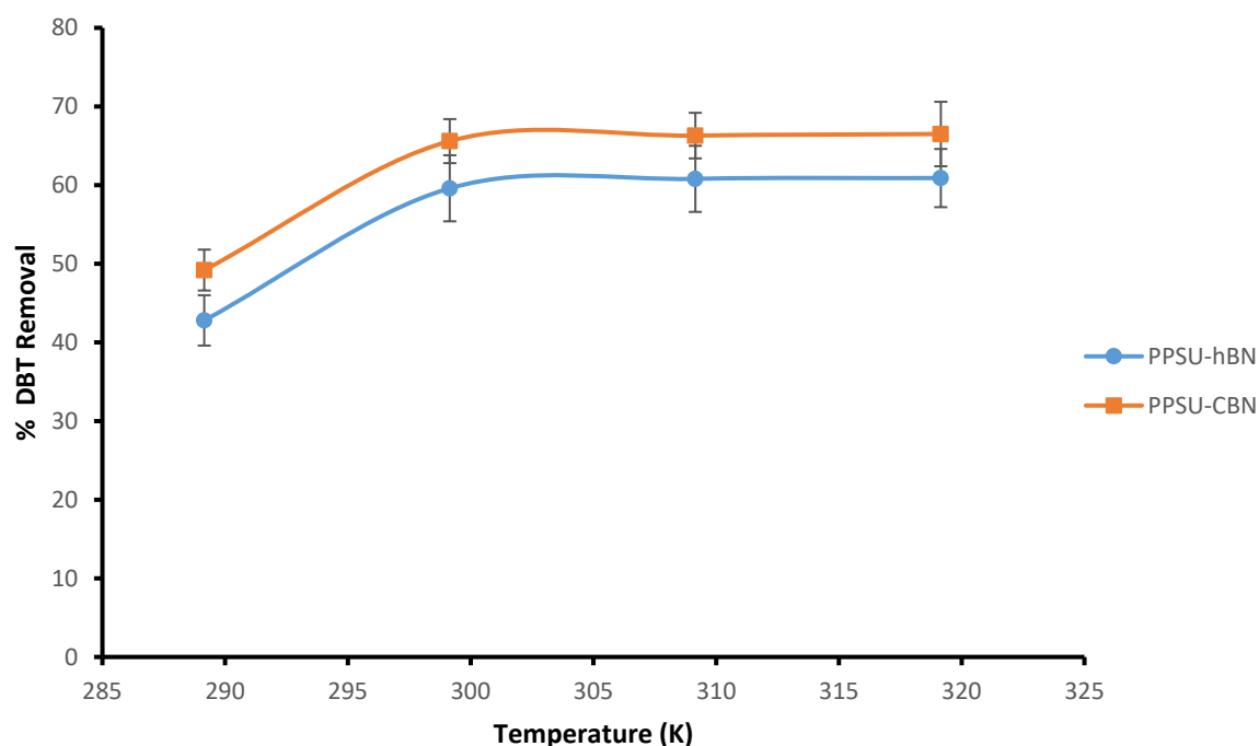
Figure 5.4 Desulfurisation behaviour with temperature
