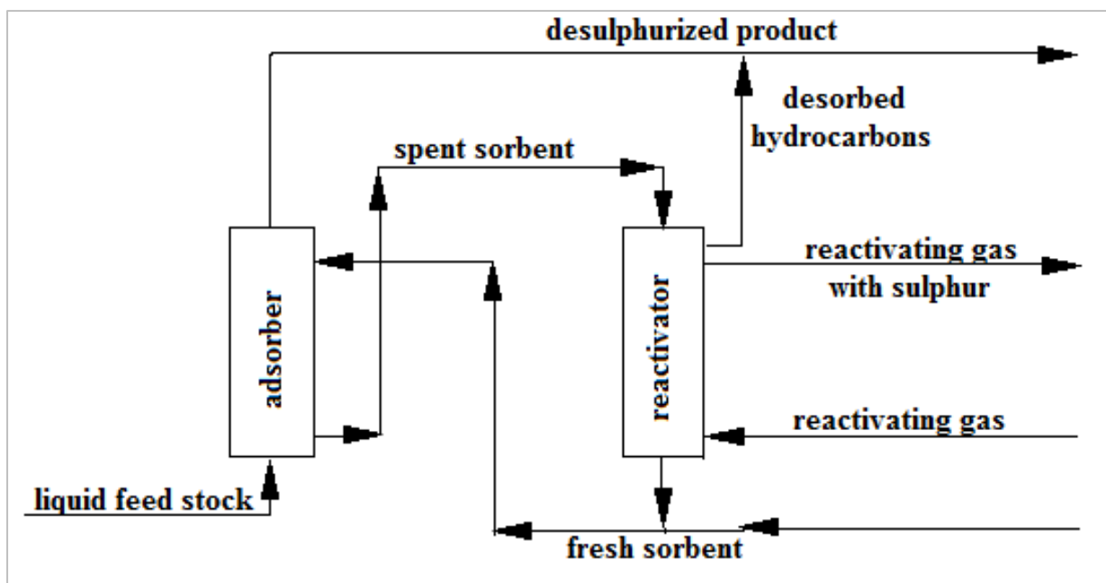
Figure 2.25 Simplified adsorptive desulfurization flow process (Babich and Moulijin, 2003)
