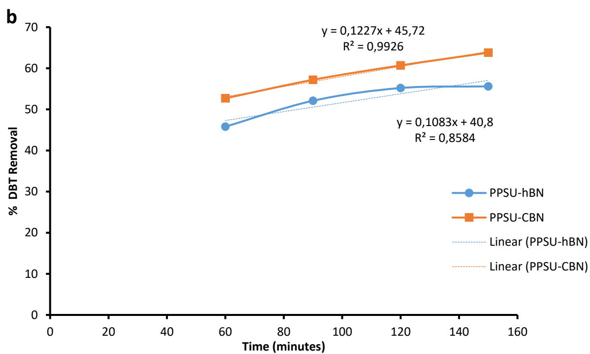
Figure 5.5 Graphs showing adsorption behaviour for varying contact time at (a) rapid phase and (b) slow phase
