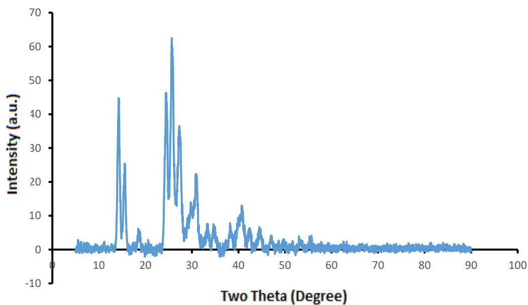
Figure A.1 XRD of h-BN synthesized by HTF method calcined at 700 °C
