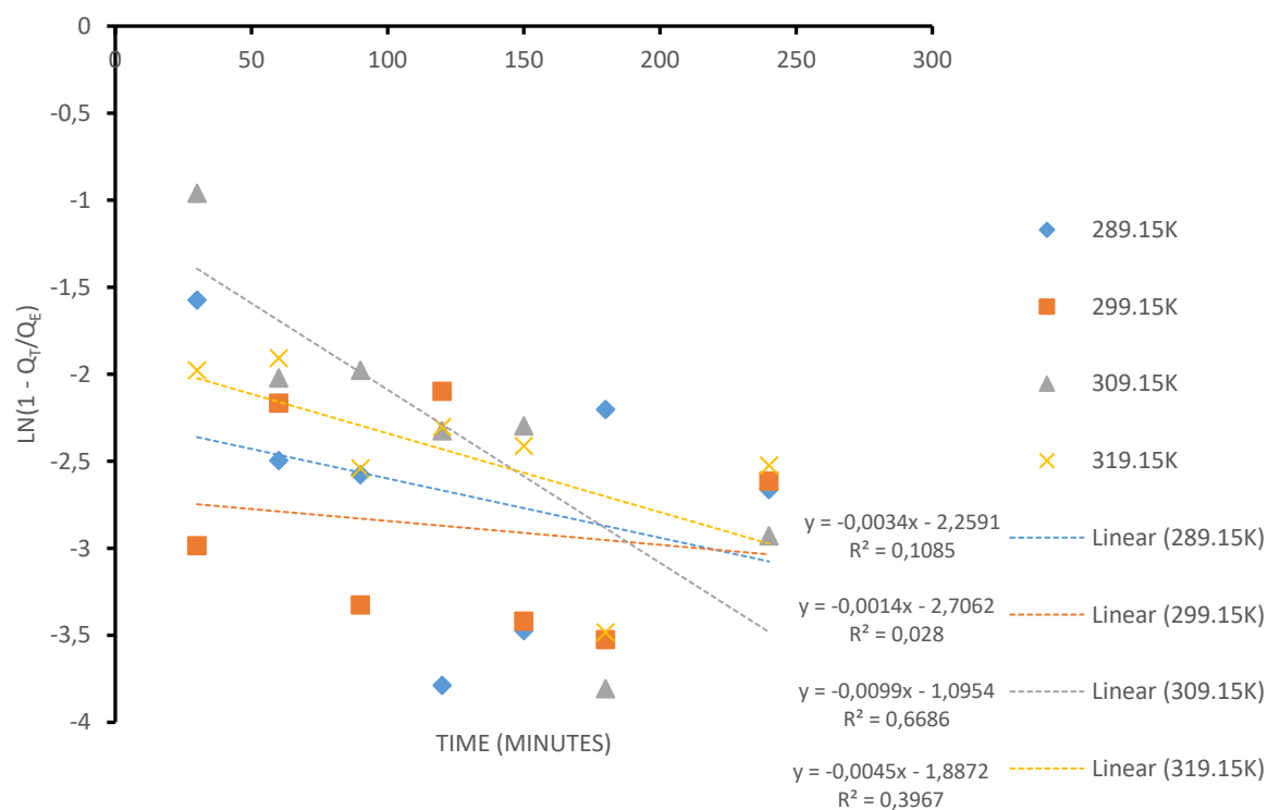
Figure 6.11 Film diffusion model
