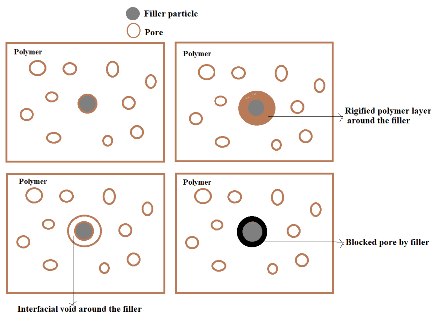
Figure 2.27 Image of various structures at the polymer/filler interface region (Moore and Koros, 2005)
