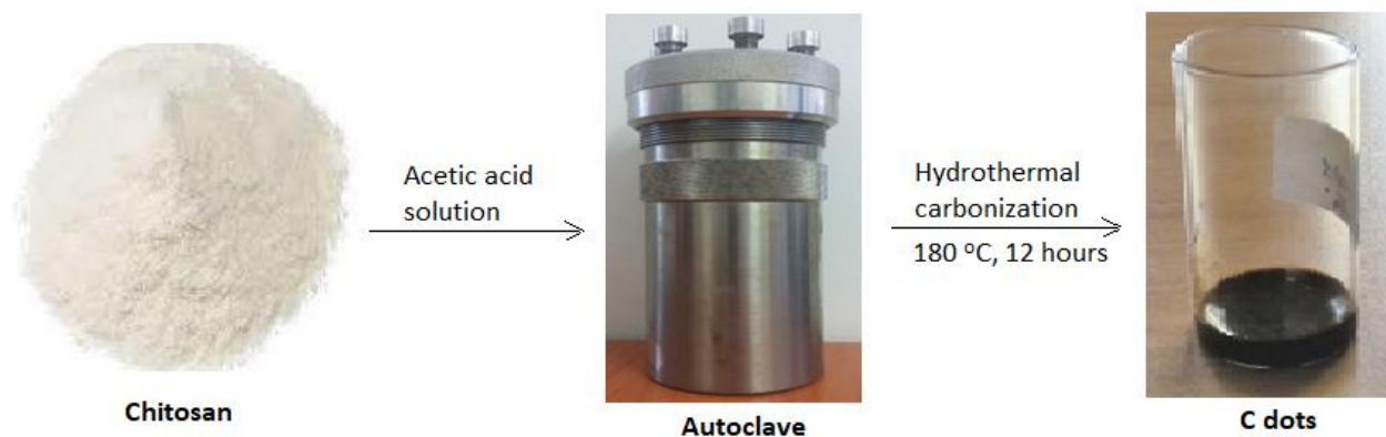
Figure 3.7 Hydrothermal synthesis of Carbon dots
