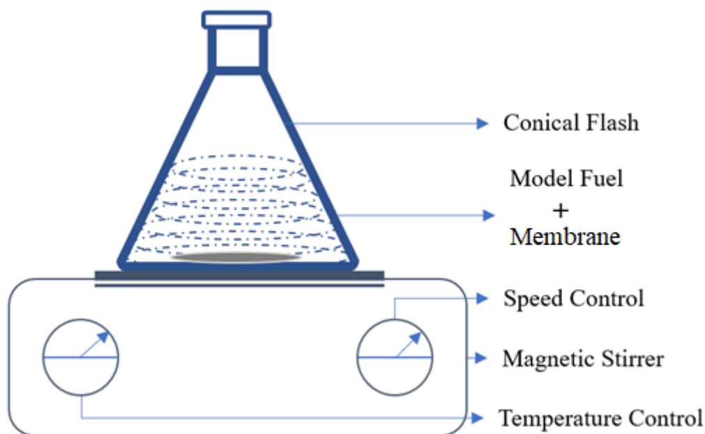
Figure 5.1 Batch adsorption process set-up for sulfur removal using MMM embedded with h-BN and CBN
