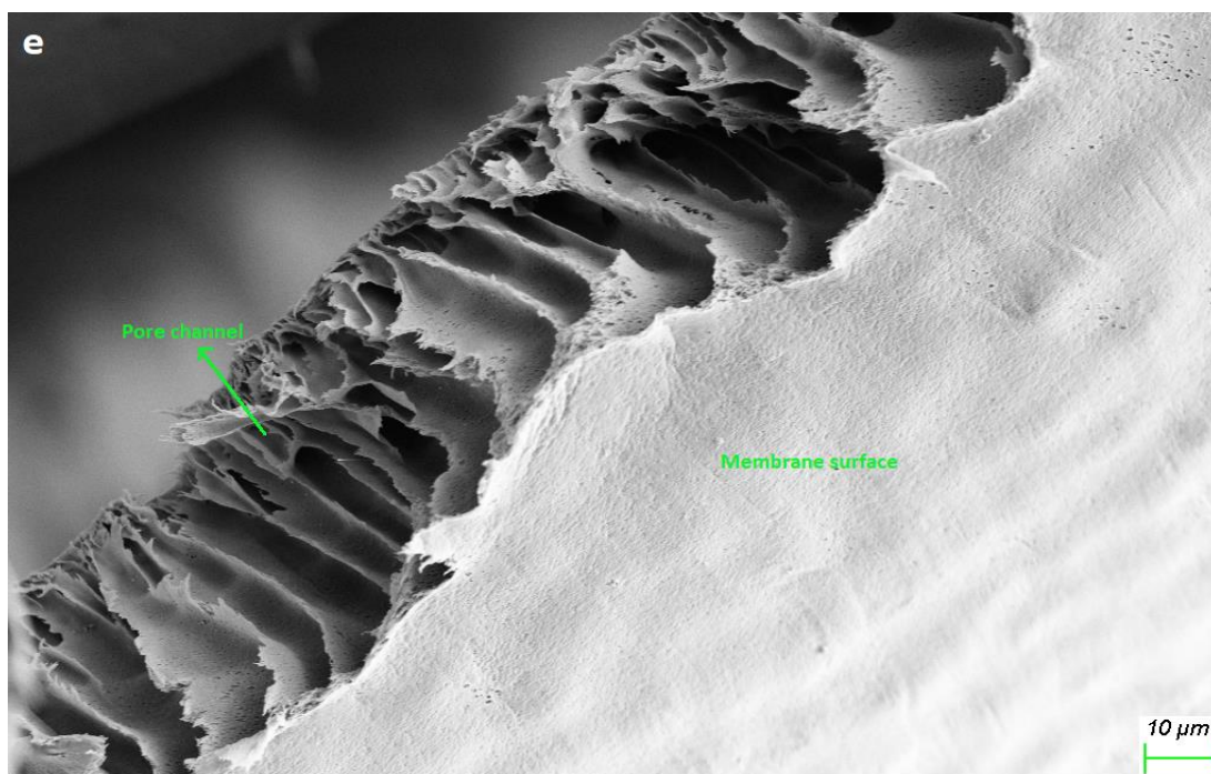
Figure 4.4 (a) PPSU membrane surface (b) cross section of PPSU membrnae, (c) cross section of PPSU-CBN (1.2 wt.%) membrane, (d), PPSU-CBN (1.2 wt.%) membrane surface showing surface layer thickness and (e) porous network channels of PPSU-CBN (0.8 wt.%) membrane
