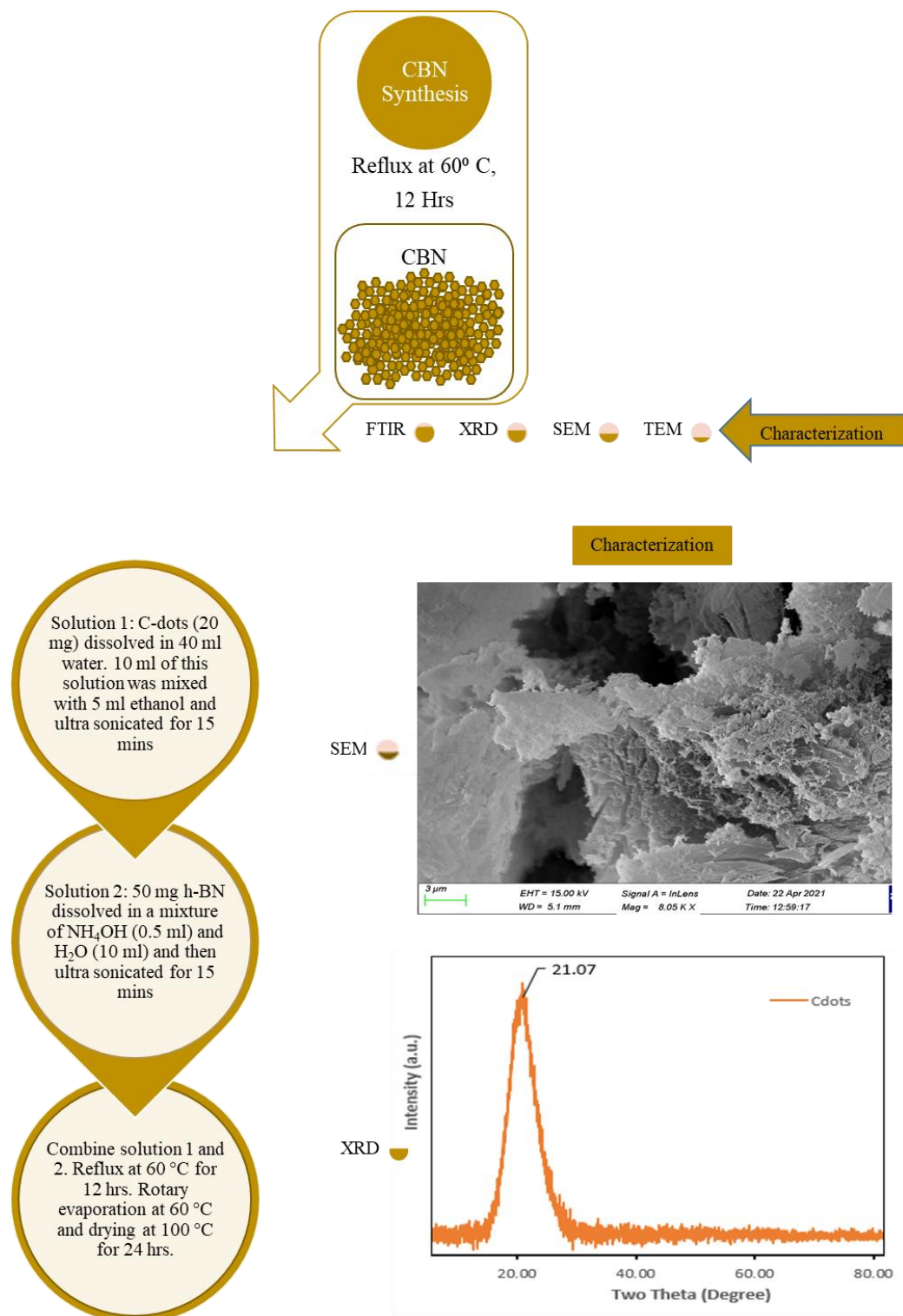
Figure 3.3 The flow diagram of C-dot doped on h-BN and its characterization
