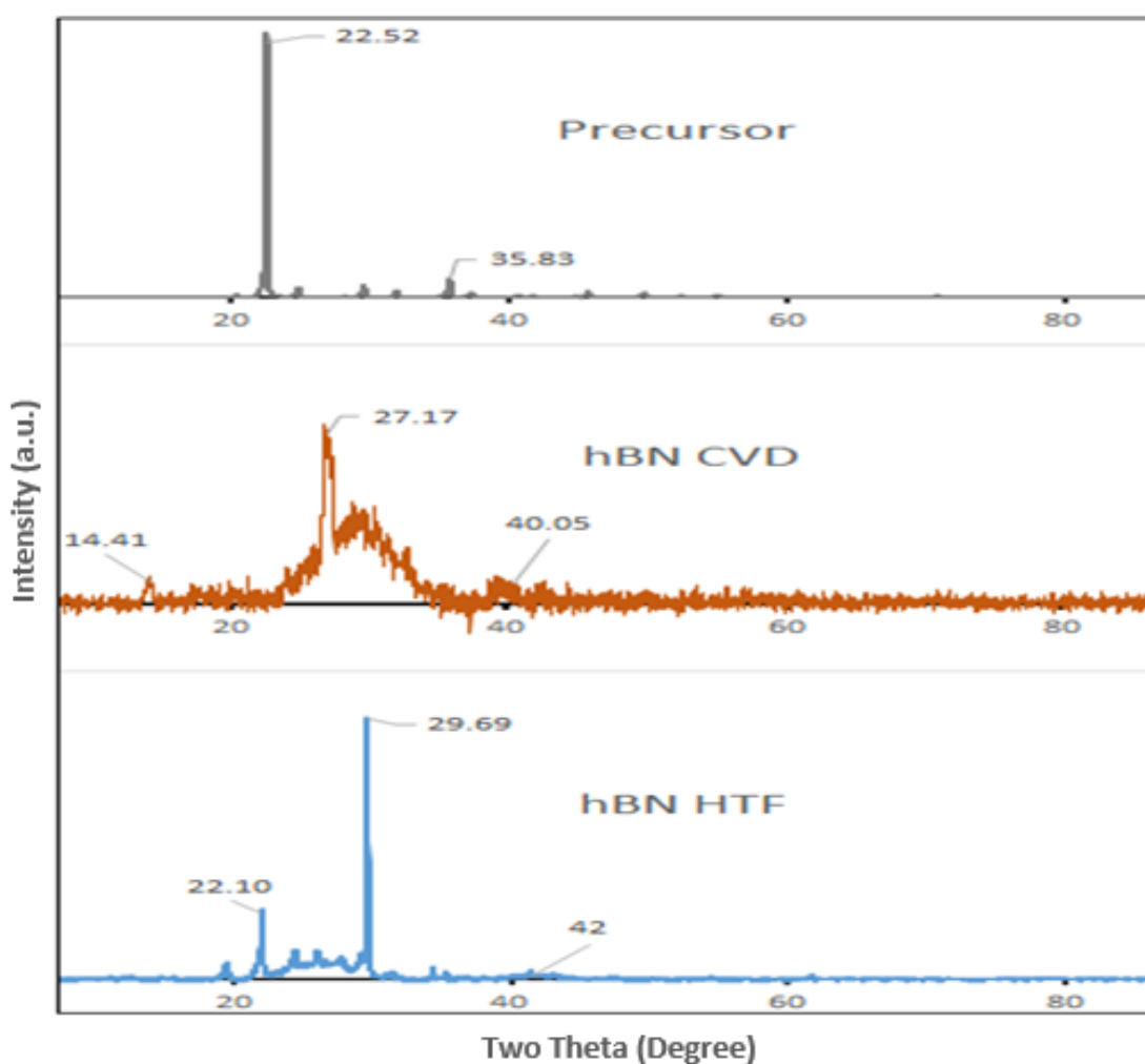
Figure 3.14 Image showing XRD peaks of precursor, synthesized h-BN by CVD (900 °C) method and HTF (900 °C) method
