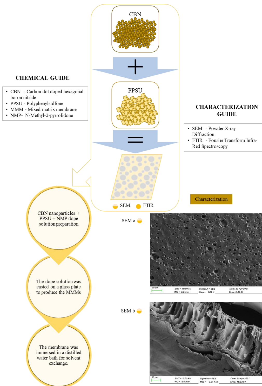
Figure 4.1 Development of PPSU MMM with CBN nanoparticles
