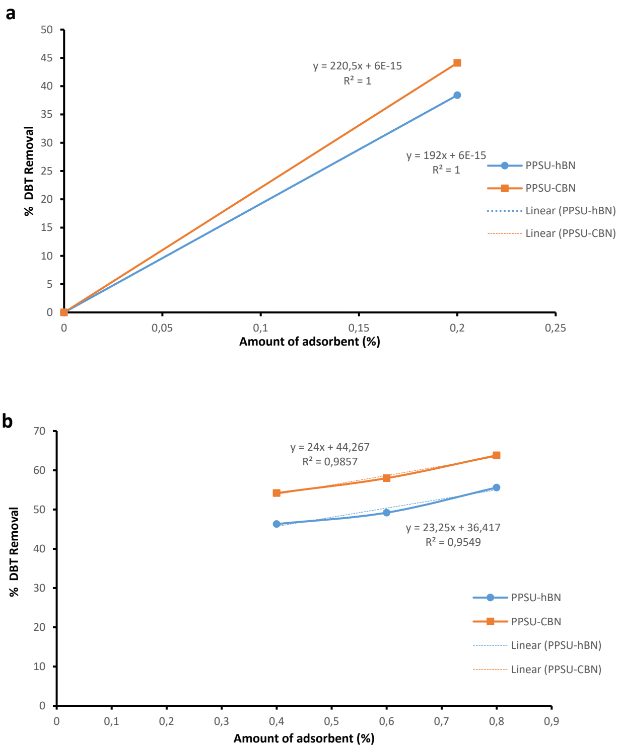
Figure 5.6 Graphs showing adsorption behaviour for varying adsorbent amount at (a) rapid phase and (b) slow phase
