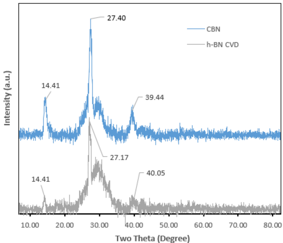
Figure 3.21 XRD image of CBN and h-BN CVD
