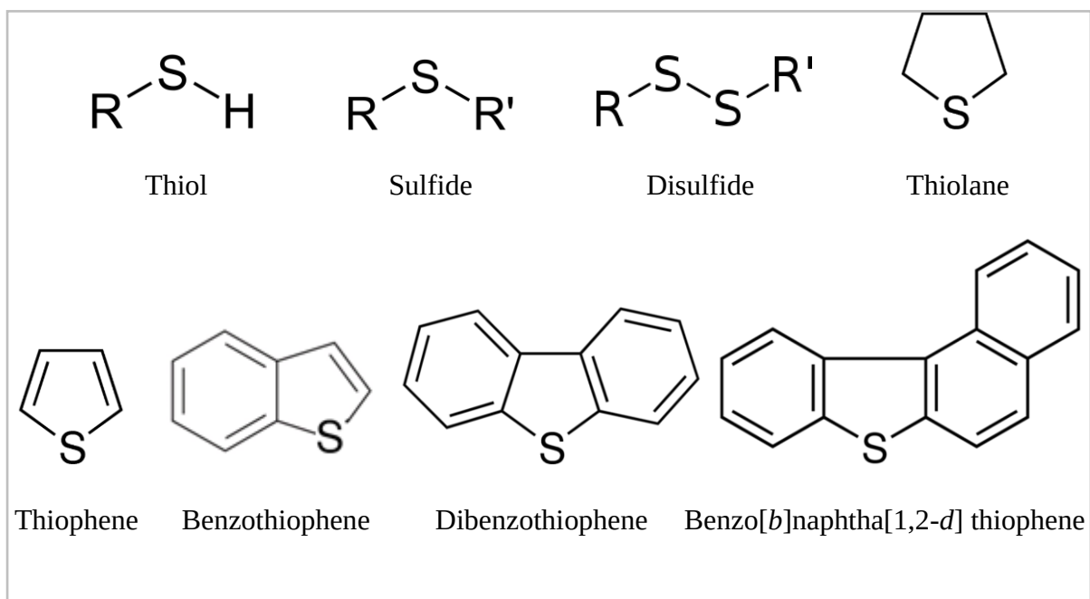
Figure 2.9 Crude oil sulfur compounds (R=alkyl) (Javadli and De Klerk, 2012)
