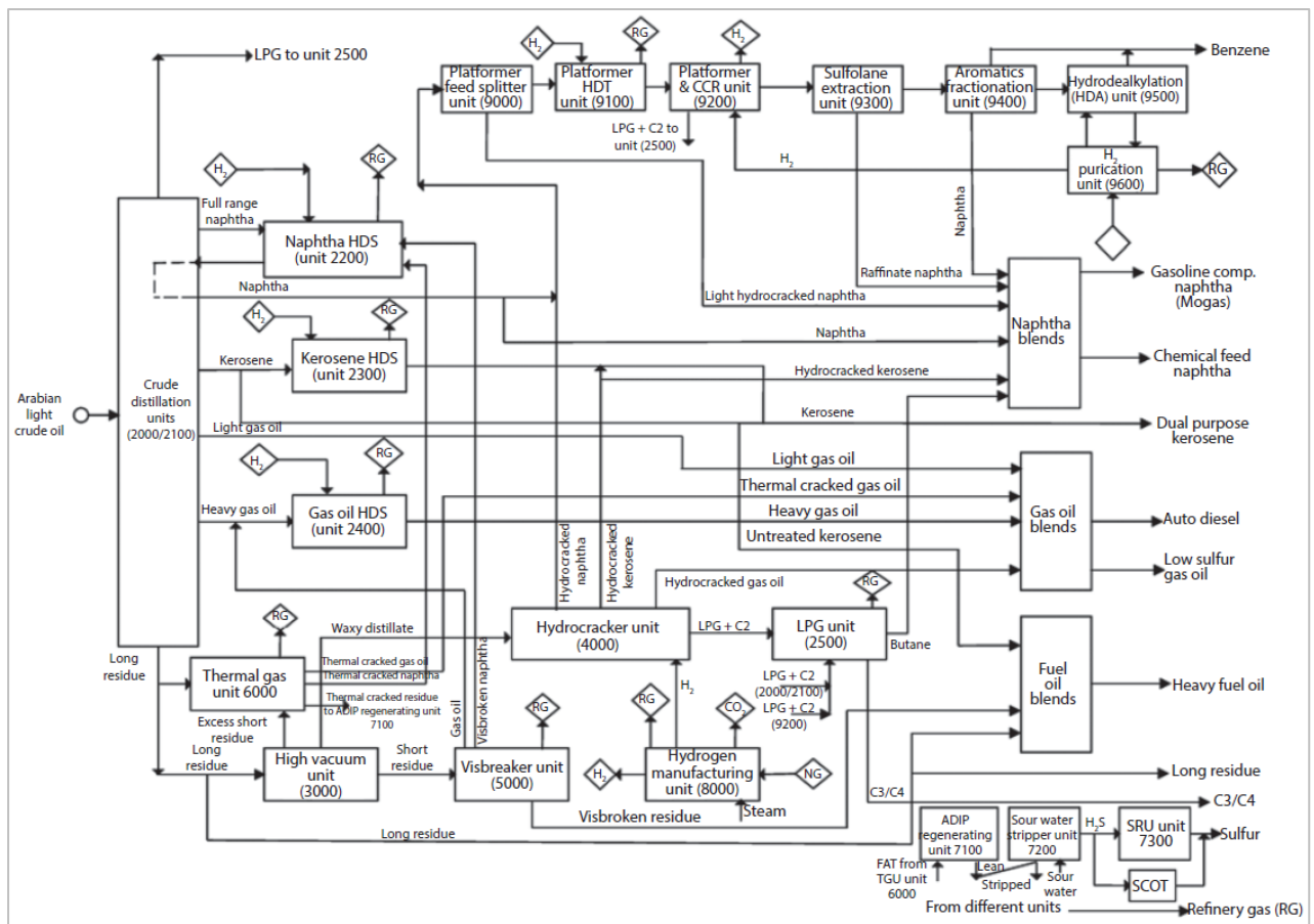
Figure 2.10 Complex Refinery Operations (Coker, 2021)
