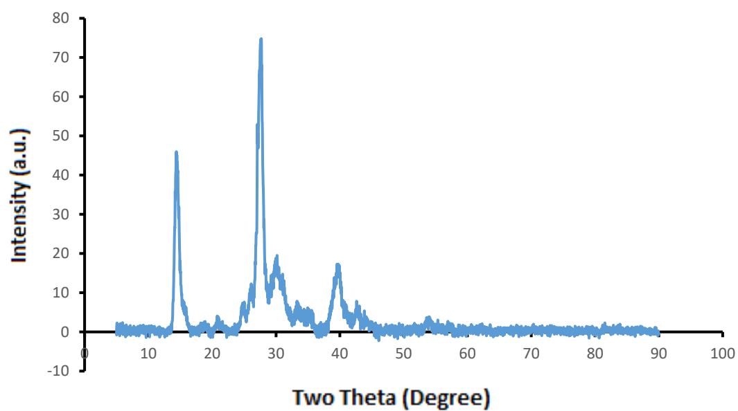
Figure A.4 XRD of h-BN synthesized by CVD calcined at 800 °C
