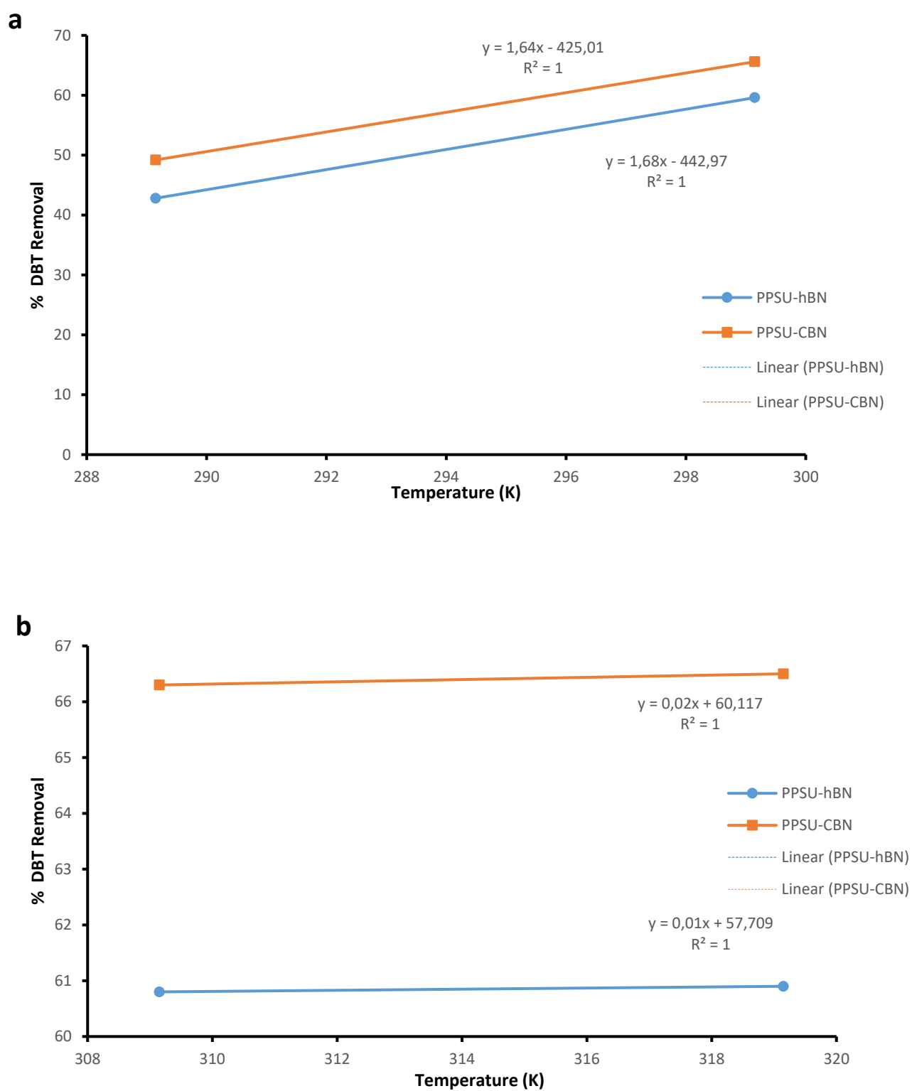
Figure 5.7 Graphs showing adsorption behaviour for varying temperature at (a) rapid phase and (b) slow phase
