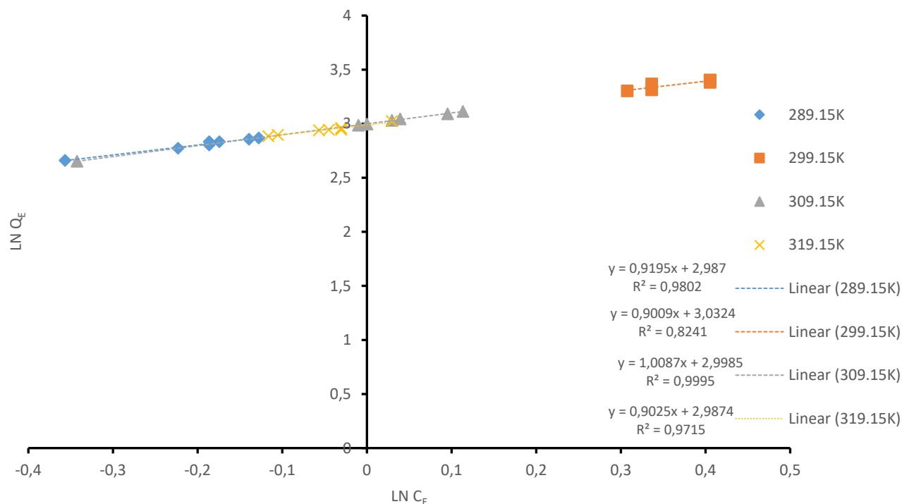
Figure 6.2 Freundlich adsorption isotherm
