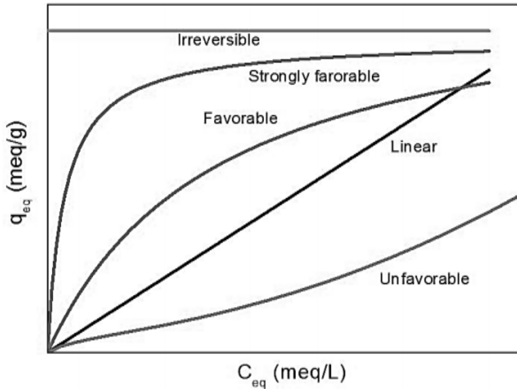
Figure 5.9 Adsorption isotherms (Barros et al., 2013)
