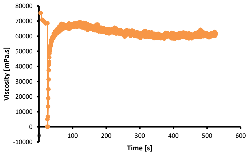
Figure 4.10: Shear thinning over time for 1.0 w% NCC mud sample over time at 25°C
