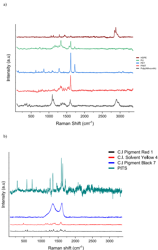
Fig. 6. Raman spectra of detected a) polymers (HDPE, PU, PET, PA6T, and Poly (AM-co-AA)) and b) additives (C.I. Pigment Red 1, C.I. Solvent Yellow 4, C.I. Pigment Black 7, and Potassium indigotetrasulphonate (PITS)). (For interpretation of the references to colour in this figure legend, the reader is referred to the Web version of this article.)
