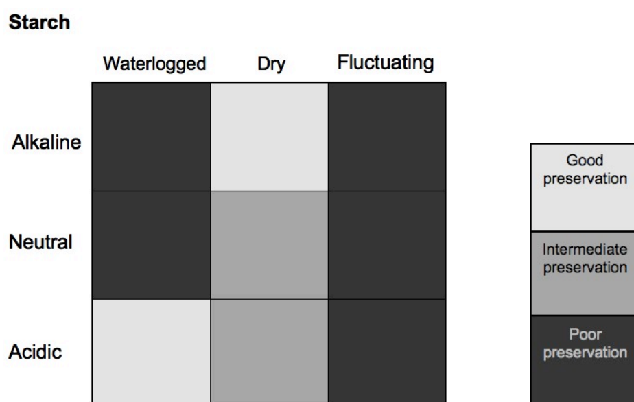
Figure 3.3: The quality of preservation of starch in a variety of environments at moderate temperatures (Based on information from the paragraphs above and from (Crow 2008, Figure 5, 2272)).
