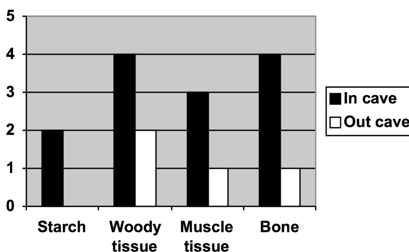
Figure 4.1: Preservation index for the Sterkfontein samples that were exposed for one year.
