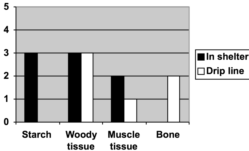
Figure 4.6: Preservation index for the Sibudu samples that were buried for one year. Note that the bone sample, inside the shelter was not recovered.
