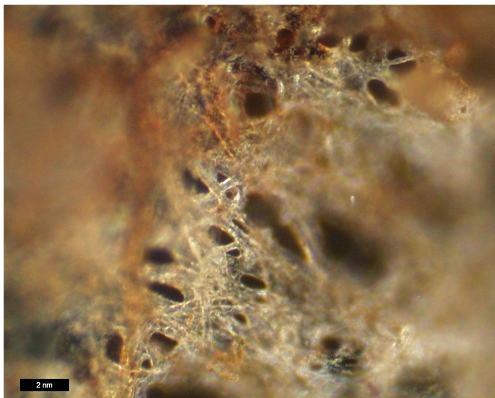
Figure B.130: Gelatinous hyphae. Thick hyphae deposits can be extremely similar to muscle tissue residues. The organic shapes and the holes are sometimes strikingly similar. Magnification 500, brightfield polarised light.
