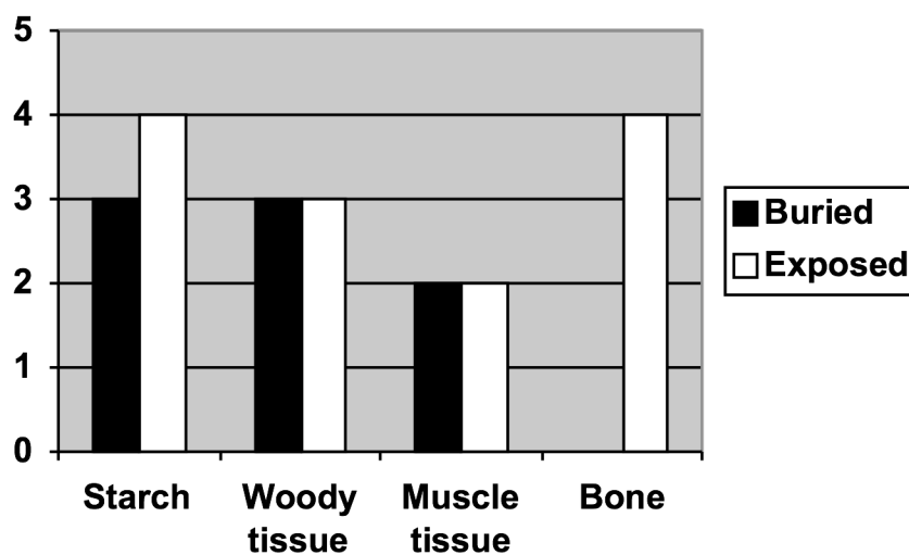
Figure 4.7: Preservation index for the Sibudu samples that were deposited inside the shelter for one year. Note that the buried bone sample was not recovered.
