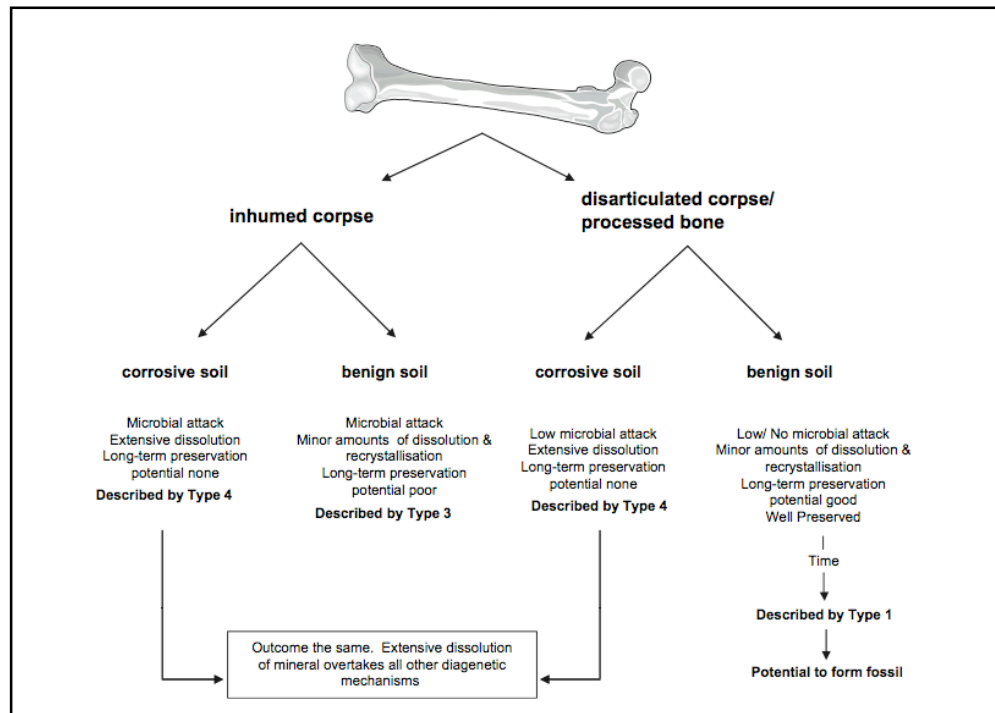
Figure 3.1: Diagenetic end-points for bones in terrestrial environments, taking into account the effects of burial environment and taphonomy (From Nielsen-Marsh et al. 2007, 1529). Smith et al. (Smith et al. 2007) recognise four types of preserved bone: Type 1: Is well preserved bone. It contains a high percentage protein, has a high Oxford Histology Index score, a high C/P ratio and a low Mineral Crystallinity Index and low porosity values. Type 2: Underwent accelerated collagen or protein hydrolysis. It contains a low percentage protein, a highly altered mineral index, but with a high Oxford Histology Index score, a low C/P ratio, a high Mineral Crystallinity Index and increased porosity with small pores. Type 3: Is microbially attacked bone. In this type protein tends to decrease, there is a decreased Oxford Histology Index score, occasional hyper-mineralised edges and mineral alteration, an increasing Mineral Crystallinity Index and an increase in porosity with medium pores. Type 4: Underwent catastrophic mineral dissolution. It contains a low percentage protein, has a low Oxford Histology Index score, a low C/P ratio, high Mineral Crystallinity Index and high porosity values with large pores.
