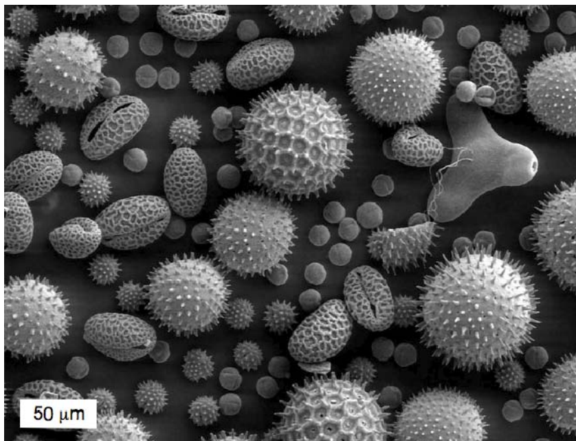
Figure A.30: SEM image of pollen from sunflower ( Helicantus annuus ), morning glory ( Ipomoea purpurea ), hollyhock ( Sildalcea malviflora ), lily ( Lilium auratum ), primrose ( Oenothera fruticosa ) and castor bean ( Ricinus communis ). Magnification 500. Image by Dartmouth Electron Microscope Facility, Dartmouth College (2004), Wikimedia Commons.
