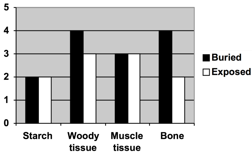
Figure 4.3: Preservation index for the Sterkfontein samples that were deposited inside the cave for one year.
