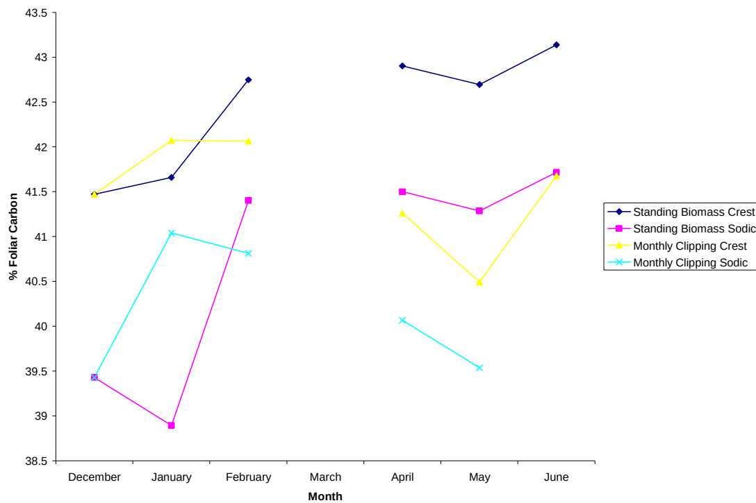
Figure 4.11: Change in percentage foliar carbon through the growing season in monthly clipped treatments inside the enclosure and standing biomass (seasons 2 and 3 combined)
