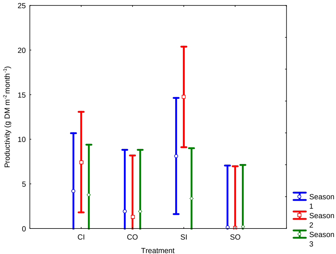
Figure 4.1: Grass biomass productivity ( \text{g DM m}^{-2} \text{ month}^{-1} ) within each treatment per sampling season 1 (December 2002 – June 2003), season 2 (December 2003 – June 2004) and season 3 (December 2004 – June 2005). Treatment codes refer to the terrain – crest (C) and sodic patch (S) – and position relative to the enclosure – inside (I) and outside (O). Points denote means and vertical bars denote 0.95 confidence intervals
