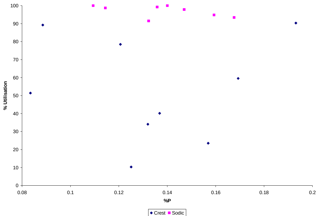
Figure 4.18: Relationship between percentage foliar phosphorus and percentage forage utilised in the sodic patch ( r=-0.45 , p>0.05 ) and crest patch ( r=0.05 , p>0.05 ) over seasons 2 and 3
