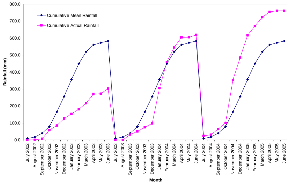
Figure 3.2: Mean cumulative and actual cumulative rainfall (mm) from July 2002 to June 2005 for the Skukuza Meteorological Station
