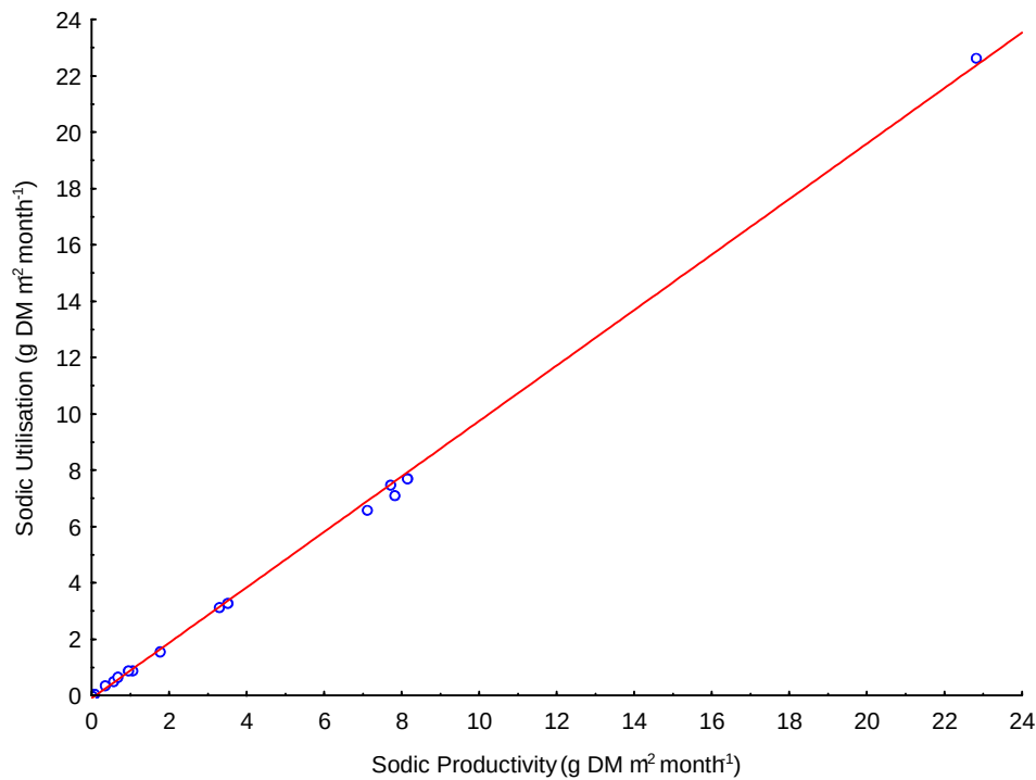
Figure 4.16: Relationship between the monthly means of sodic productivity (g DM m -2 month -1 ) and utilisation over three seasons ( r=0.99 , p<0.05 )
