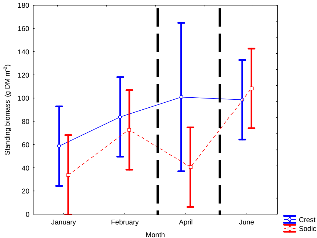
Figure 4.4: Standing biomass (g DM m -2 ) accumulated in the crest (C) and sodic patch (S) inside the enclosure over time (months accumulated over sampling seasons 2 and 3). Points denote means and vertical bars denote 0.95 confidence intervals. The bold dashed vertical line-breaks indicate missing values for the months of March and May
