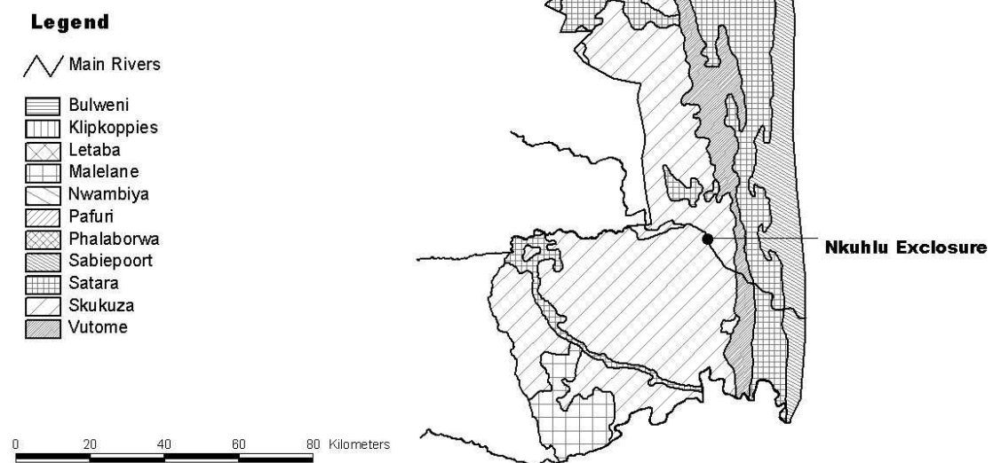
Figure 2.2: Land systems of the Kruger National Park (Venter 1990), indicating the position of the study area (the Nkuhlu Research Exclosure)
