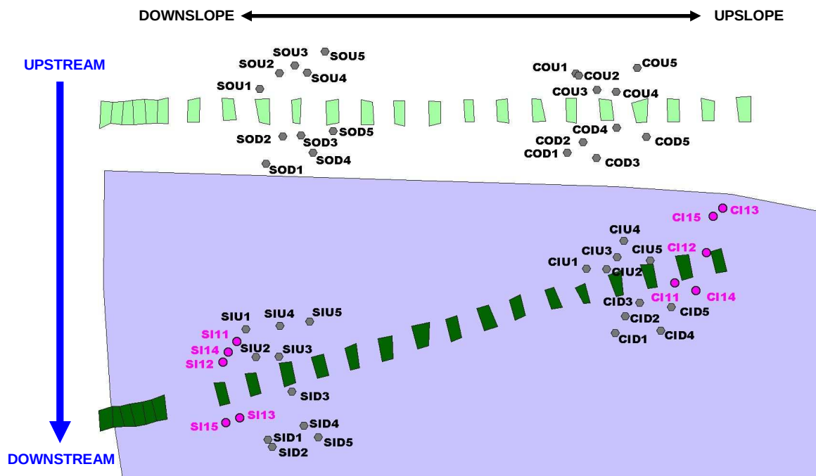
Figure 3.10: Diagram of the sampling area indicating the position of transect 6 (light green) outside the exclosure (white background), transect 7 (dark green) inside the exclosure (light blue background) and the location of biomass plots with plot reference names (CIU for instance, is an abbreviation for “Crest Inside Upstream”; SOD = “Sodic Outside Downstream”). Plots in pink added in Feb 2004. Crest plots occupy an upslope position relative to sodic plots. The schematised blue arrow on the left of the diagram indicates the position and flow direction of the Sabie River
