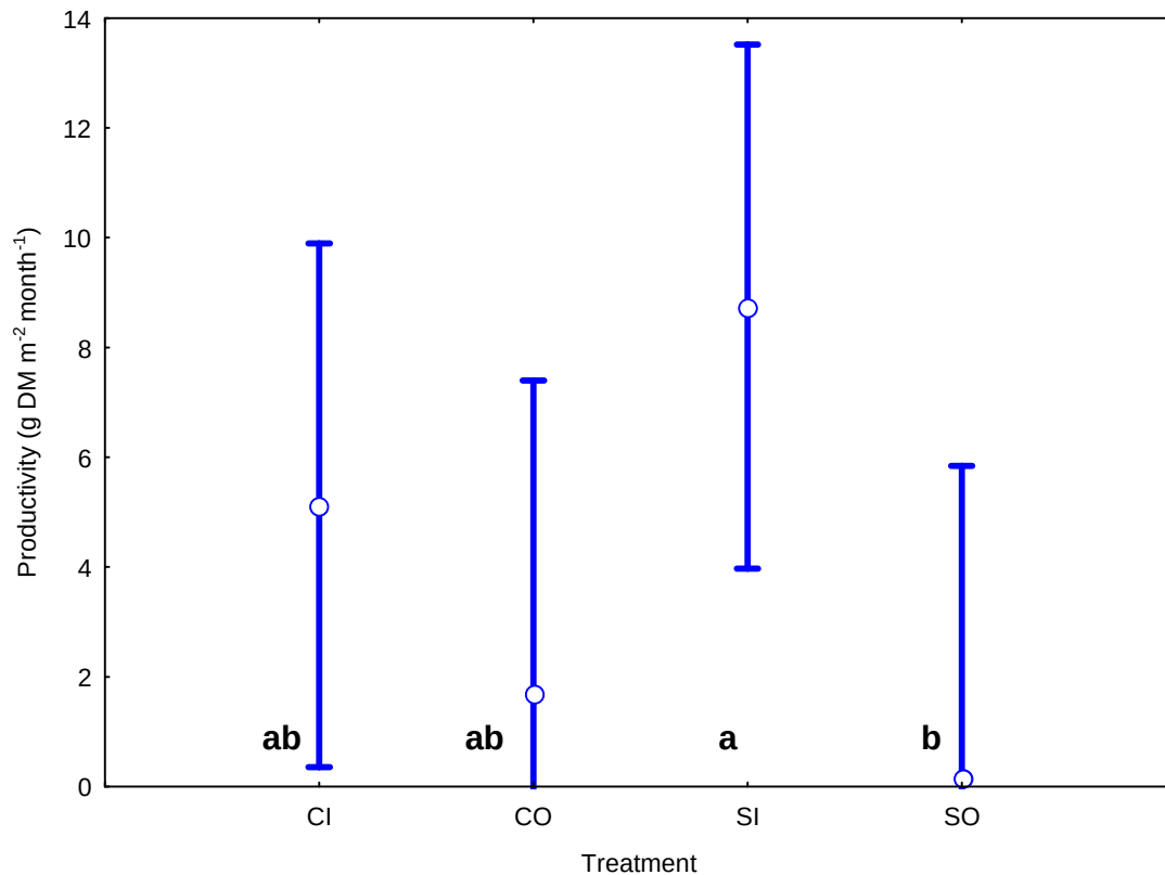
Figure 4.2: Grass biomass productivity (g DM m -2 month -1 ) in each treatment for three growing seasons (2002 – 2005). Treatment codes refer to the terrain – crest (C) and sodic patch (S) – and position relative to the enclosure – inside (I) and outside (O). Points denote means and vertical bars denote 0.95 confidence intervals. Data with similar letters are not significantly different
