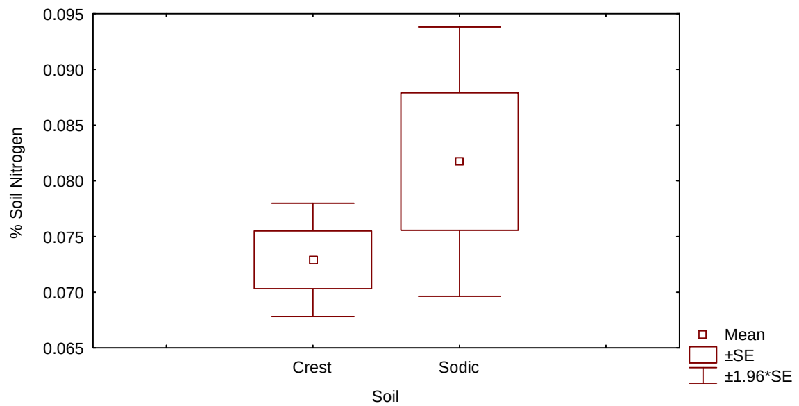
Figure 4.25: Percentage soil nitrogen in crest (n=20) and sodic (n=20) soils in Season 3
