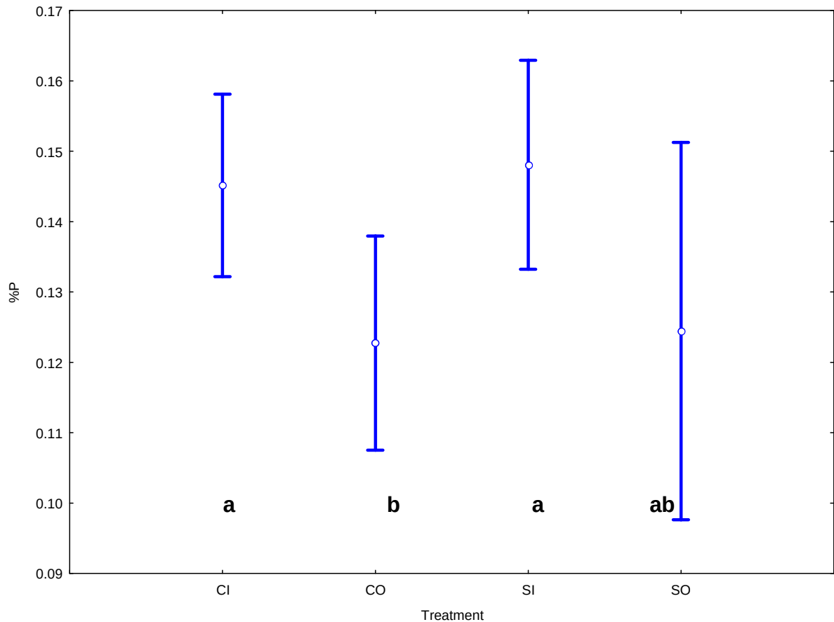
Figure 4.10: Percentage foliar phosphorus across all treatments over seasons 2 and 3. Treatment codes refer to the terrain – crest (C) and sodic patch (S) – and position relative to the exclosure – inside (I) and outside (O). Points denote means and vertical bars denote 0.95 confidence intervals. Data with similar letters are not significantly different
