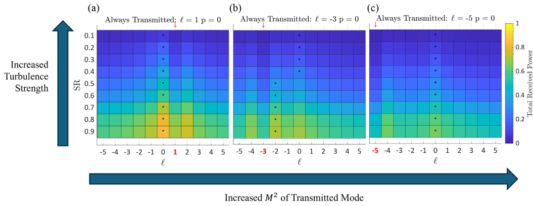
Fig. 3. Total powers received when an OAM beam is both transmitted and received with other beams at different turbulence strengths using simulations. The red arrow shows the transmitted mode, and the asterisks show with which mode a transmitted mode should be combined to maximize power. In (a) the transmitted mode is \ell = 1 , which has the lowest M^2 , in (b) \ell = -3 , and in (c) \ell = -5 (highest M^2 ). At lower M^2 and turbulence strengths, the optimal mode combination involves the neighboring mode, whereas at higher M^2 and turbulence strengths the optimal mode is the Gaussian beam.
