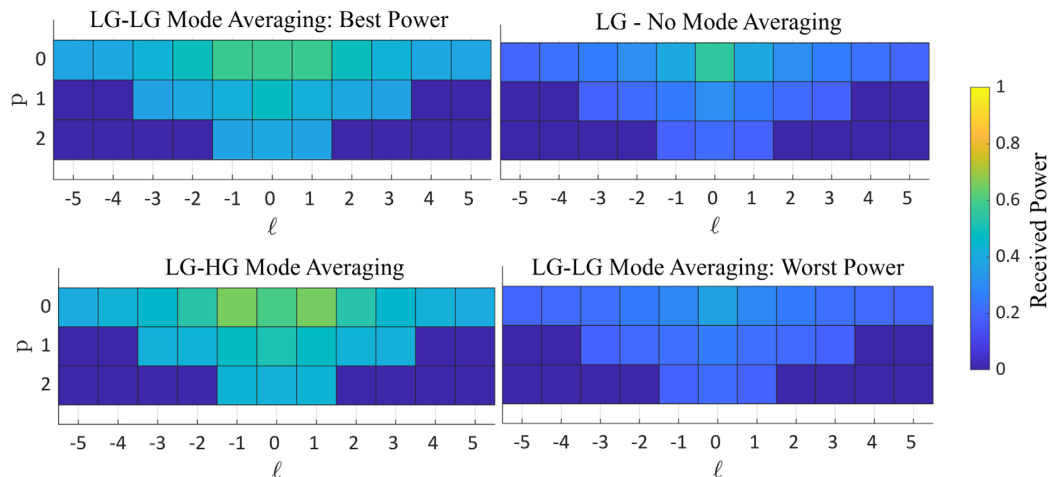
Fig. 7. Maximum received power for each transmitted LG mode at an SR of 0.6, comparing four scenarios: (a) mode averaging with the optimal LG-LG mode combination, (b) mode averaging with the optimal LG-HG mode combination, (c) no mode averaging, and (d) mode averaging with an LG-LG combination that minimizes power. It can be seen that mode averaging using the optimal LG-LG and LG-HG mode combinations perform better than no mode averaging. However, if the least optimal modes are used, the resulting power from mode averaging may be worse than without mode averaging.
