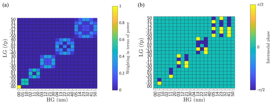
Fig. 1. (a) The power weightings and (b) the phases of HG modes making up different LG modes determined using Eqs. (4) and (5).
