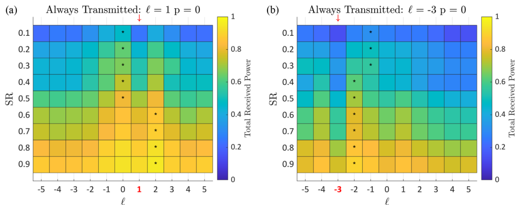
Fig. 4. Total powers received when a chosen OAM beam is both transmitted and received with other beams in an experiment. In (a) the transmitted mode is \ell = 1 whereas in (b) the transmitted mode is \ell = -3 . In (a) the optimal mode is always the neighboring mode, whereas in (b) the optimal mode changes from the neighboring modes to an \ell = -1 mode as the turbulence strength increases. These results are slightly different to the simulation results.
