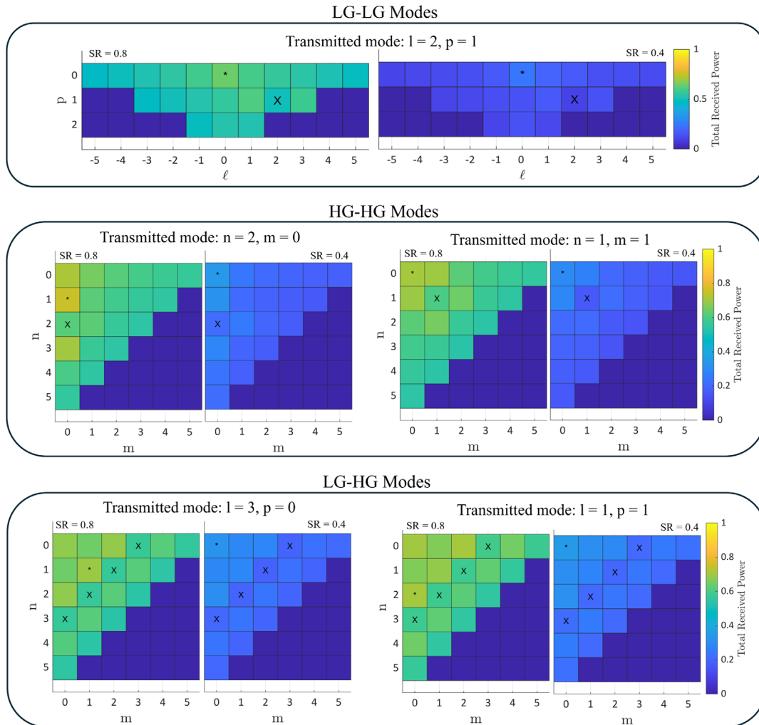
Fig. 5. Total powers received for an LG-LG mode combination, two HG-HG mode combinations, and two LG-HG mode combinations at an SR of 0.8 and 0.4. The “X” marks the chosen mode, and the “*” indicates which mode is the mode with which the transmitted mode should be combined to maximize power in a mode averaging system. It can be seen that the best mode is either a neighboring mode or a Gaussian beam, similar to the OAM modes. The definition of “neighboring mode” varies for different mode combinations.
