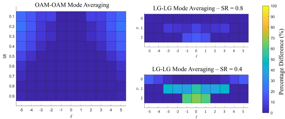
Fig. 8. The percentage difference between the power acquired when the optimal mode is used and the power acquired when the neighboring mode is used for OAM-OAM and LG-LG mode combinations in the simulations. At low turbulence strengths the difference is low; however, as the turbulence strength increases the percentage becomes significant. This is, particularly, the case for LG modes with larger p values. It must be noted that when the percentage is 0% the optimal mode is the neighboring mode.
