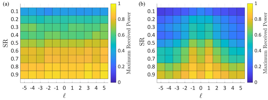
Fig. 6. The maximum average received power for different OAM modes at various turbulence strengths in a system using (a) optimal mode combinations in receiver and transmitter mode averaging, and (b) no mode averaging. Mode averaging improves the received power for most modes, particularly at higher turbulence strengths.
