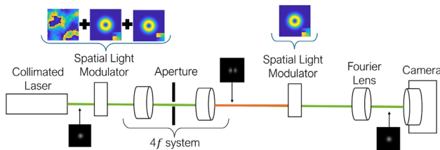
Fig. 2. The setup used to create beams, propagate the beams, and perform modal decomposition on the beams. Experimentally, propagation occurs between the 4f system and the second SLM as shown by the orange line. The insets show an example of the intensity of the beam along the setup, and the diagrams above SLMs show what is displayed without the grating on the SLM.
