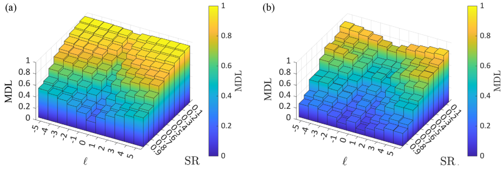
Fig. 9. The MDL of the beams measured using (a) simulations and (b) experiments. MDL must be considered when choosing optimal modes, as it increases with M^2 and turbulence strength, contributing to the average powers. The differences between the two figures explain the discrepancies between the experimental and simulation results for best mode combinations.
