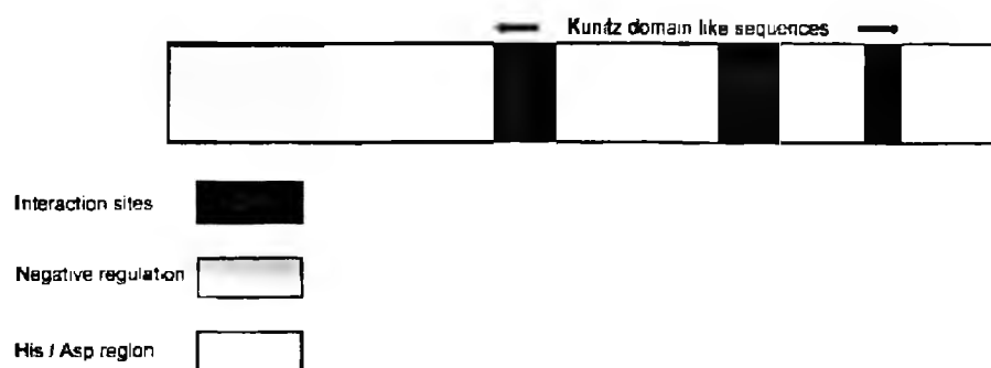
Figure 6. Schematic representation of the characteristic regions in the HBV X protein
