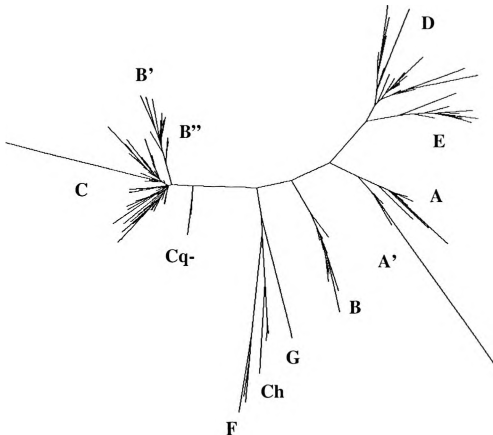
Figure 56. Neighbor tree (UPGMA option) of 175 core gene sequences
