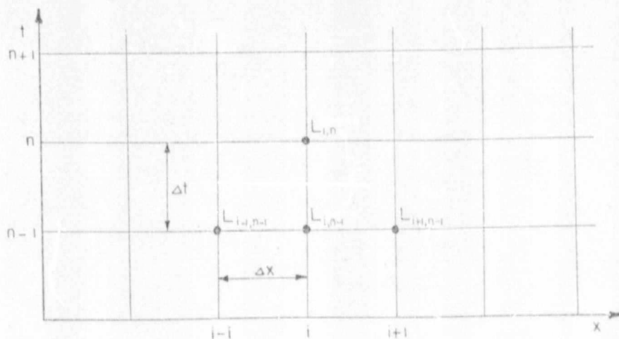
Fig. A2.1 Finite difference grid for solution of the BOD-DO partial differential equations
