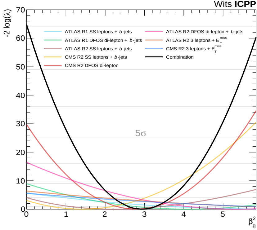
Figure 2.6: The negative 2 times the logarithm of the profile likelihood ratios for each of the individual fit results considered in this article, overlaid with that of their combination [9].
