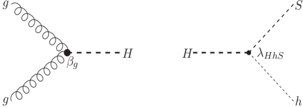
Figure 2.5: Feynman diagrams showing the dominant production mechanism of the heavy scalar, gg \rightarrow H , and its decay mode, H \rightarrow Sh .
