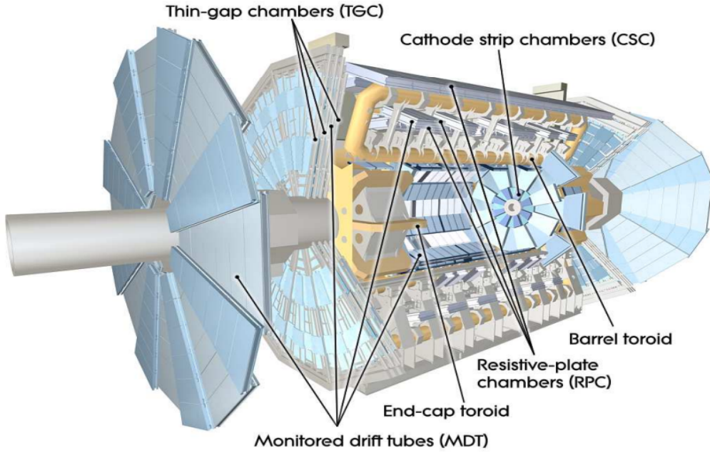
Figure 3.7: An overview of the Muon system [44].
