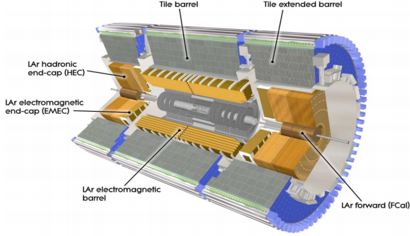
Figure 3.4: An overview of the calorimeter system [64].
