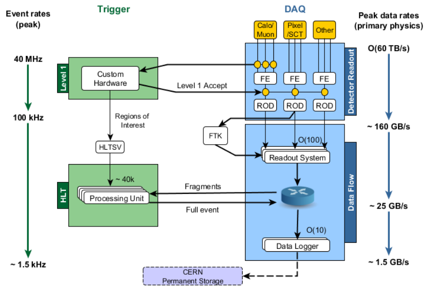
Figure 3.8: ATLAS Trigger and DAQ systems, with the expected peak rates and bandwidths for each component [68].
