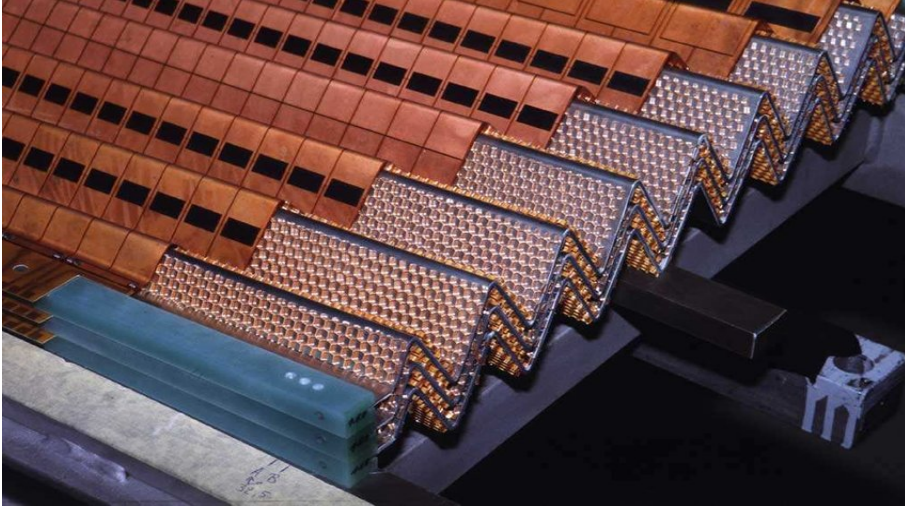
Figure 3.5: Accordion-shaped geometry of the LAr calorimeter [44].
