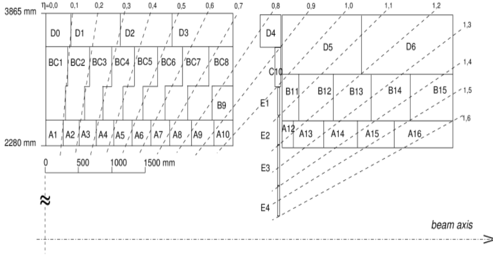
Figure 3.6: Segmentation in radial depth and pseudorapidity of the tile-calorimeter modules in the central (left) and extended (right) barrels. The bottom of the picture corresponds to the inner radius of the tile calorimeter and is parallel to the beam pipe. The tile calorimeter is symmetric about the interaction point at the origin [44].
