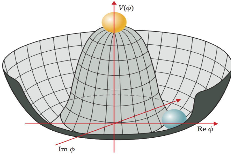
Figure 2.2: Mexican hat shape of Higgs potential that leads to “symmetry breaking”.
