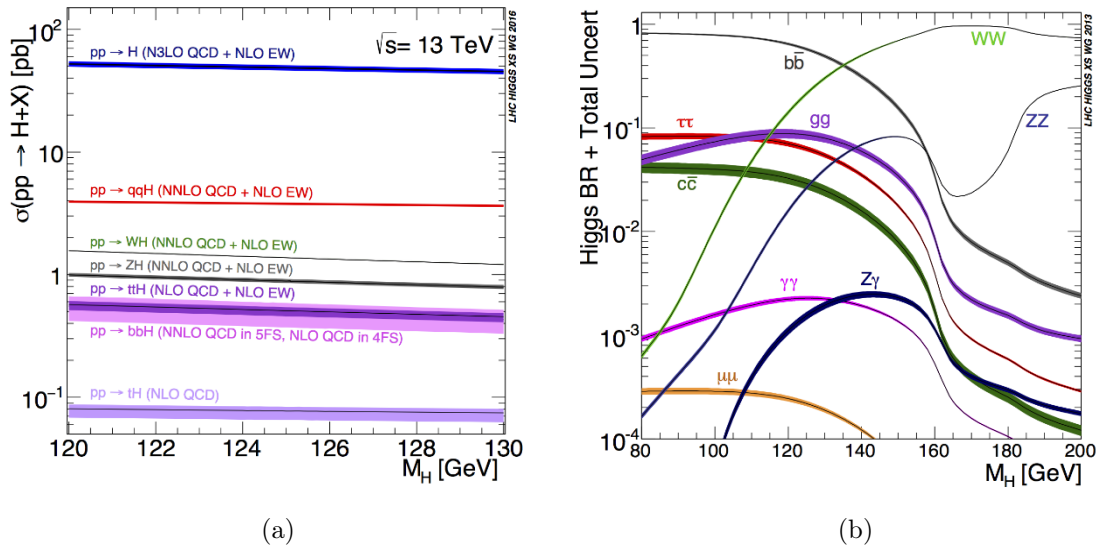
Figure 2.4: Cross sections for the h boson production as a function of its mass for a low mass range, with bands representing theoretical uncertainties with the observed mass, m_h , of 125 GeV, left, and the branching ratios as a function of its mass for a wide mass range [25], right.
