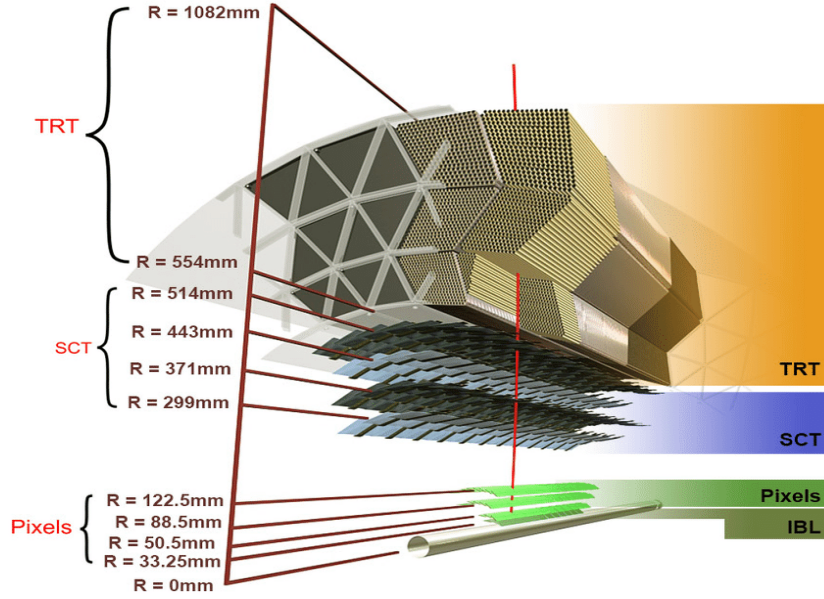
Figure 3.3: A schematic cross-section of the ID in the barrel section of the ATLAS detector, depicting the layers of the subsystems and the distance at which they are located from the interaction point [56].
