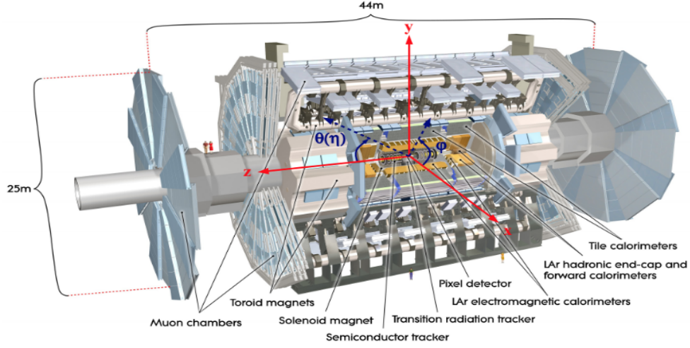
Figure 3.2: An overview of a full ATLAS detector and coordinate system [44–47].
