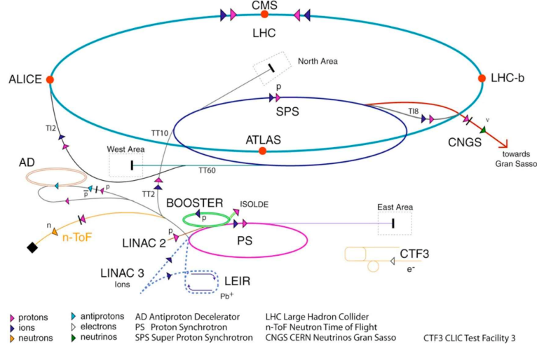
Figure 3.1: The CERN accelerator complex comprising of the multi-stage system of injectors that are used to increase the proton energy. A subset of the many experiments supported by these accelerators is also presented [51].
