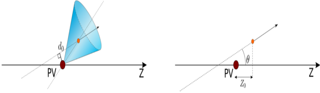
Figure 5.1: Definitions of the d_0 , z_0 \sin \theta track reconstruction parameters. PV denotes the primary vertex of the pp collisions.
