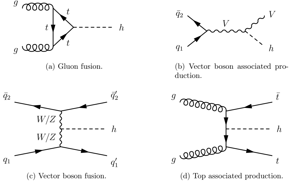
Figure 2.3: Feynman diagrams for the dominant Higgs boson production modes in high energy pp collisions.
