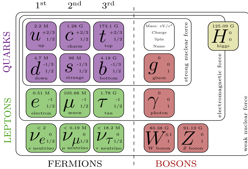
Figure 2.1: The SM of elementary particles, with three generations of matter in the first three columns in purple and green. The gauge bosons in the fourth column in red and the Higgs boson at the far top right corner in yellow.
