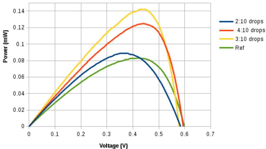
Figure 5.19: P-V characteristics fabricated device with varied concentration of Ag NPs in PEDOT:PSS .
