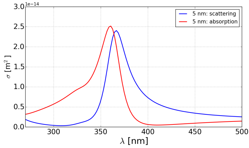
Figure 5.3: Scattering/absorption cross-section for a spherical Ag NPs of a diameter 5 nm in a simple plane surface.
