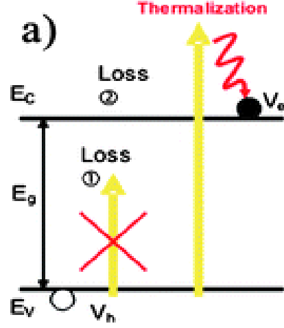
Figure 2.2: (a) Description of the absorption and thermalization losses occurring in a solar cell [45].
