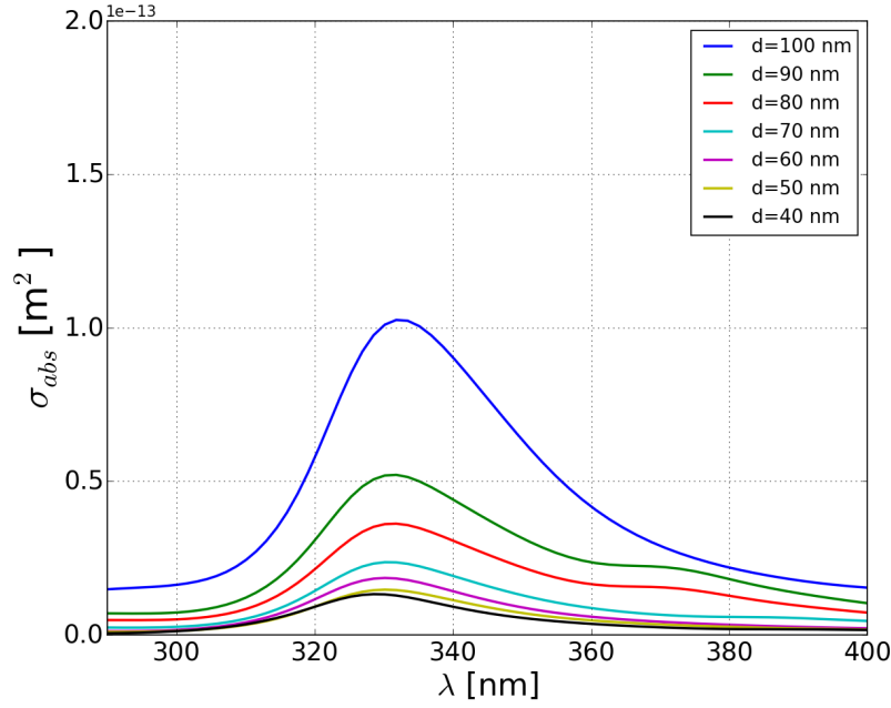
Figure 5.2: The absorption cross-section for a simple plane surface with silver spheres of different diameters.
