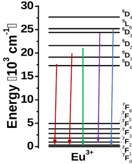
Figure 5.23: Energy level diagram for \text{Eu}^{3+} ions.
