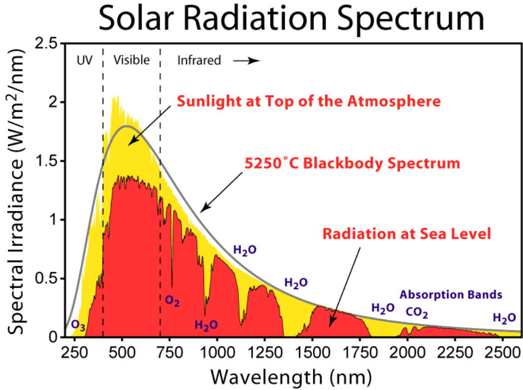
Figure 2.1: A solar emission spectrum [43]
