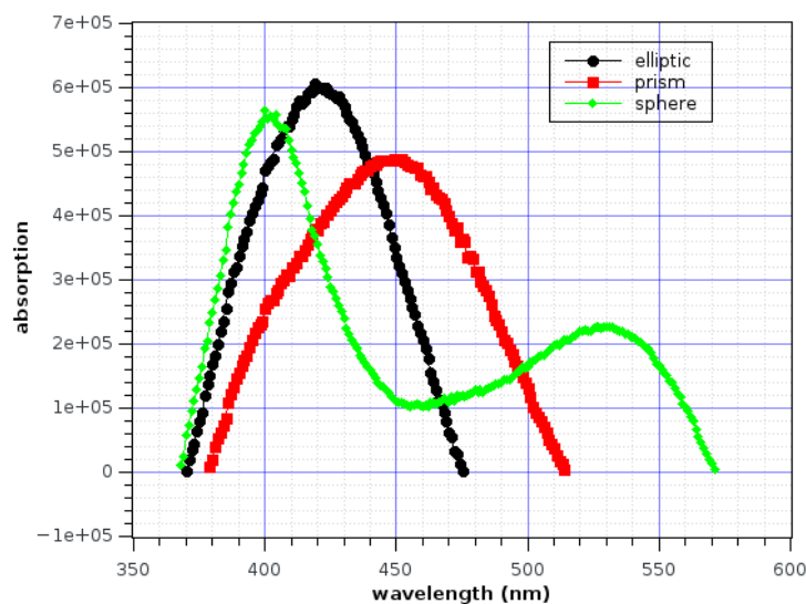
Figure 5.13: Absorption spectrum of Ag NPs fabricated at varied reaction times
