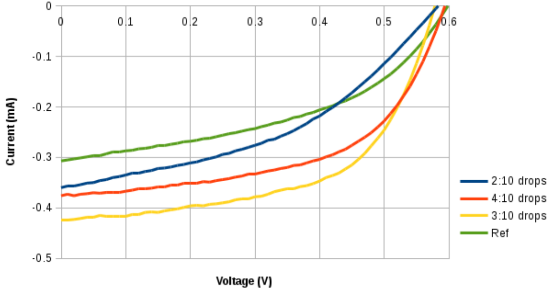
Figure 5.16: I–V characteristics of fabricated devices with different concentration of Ag NPs
