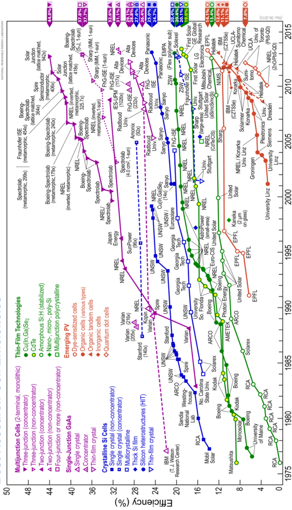
Figure 1.2: The efficiency road map of diverse families of solar cell technologies [6].
