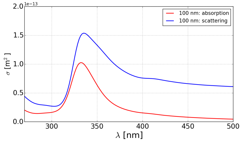
Figure 5.4: Scattering/absorption cross-section for a spherical Ag NPs of a 100 nm diameter in a simple plane surface.
