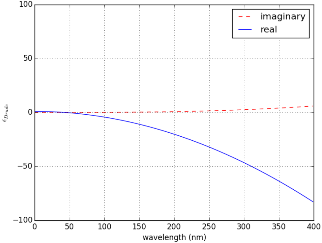
Figure 3.2: Real and imaginary part of the dielectric constant for silver according to the Drude-Sommerfeld free-electron model
