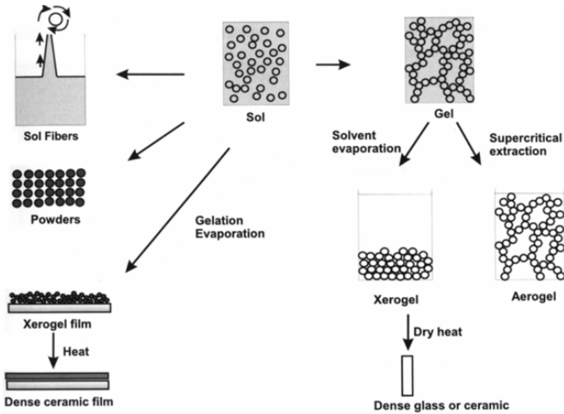
Figure 4.3: Sol-gel processing options [107]
