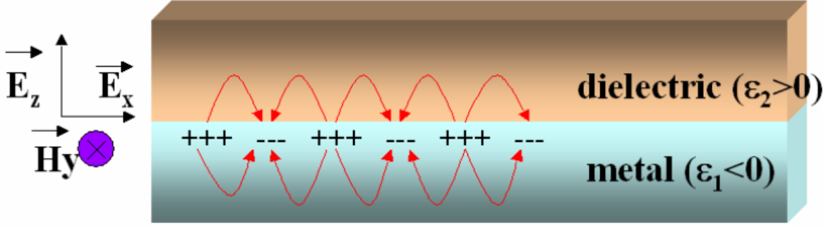
Figure 3.1: Two media with dielectric function separated at interface [82]
