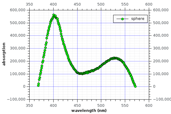
(a) Absorption spectra for spherical Ag NPs
