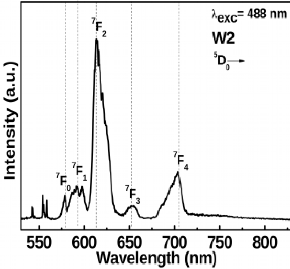
Figure 5.24: Room temperature photoluminescence spectrum of \text{Eu}^{3+} doped \text{SiO}_2 - \text{HfO}_2 .
