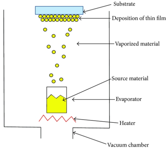
Figure 4.1: Schematic of thermal evaporation [103]
