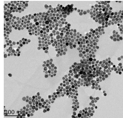
(b) TEM image for spherical Ag NPs
