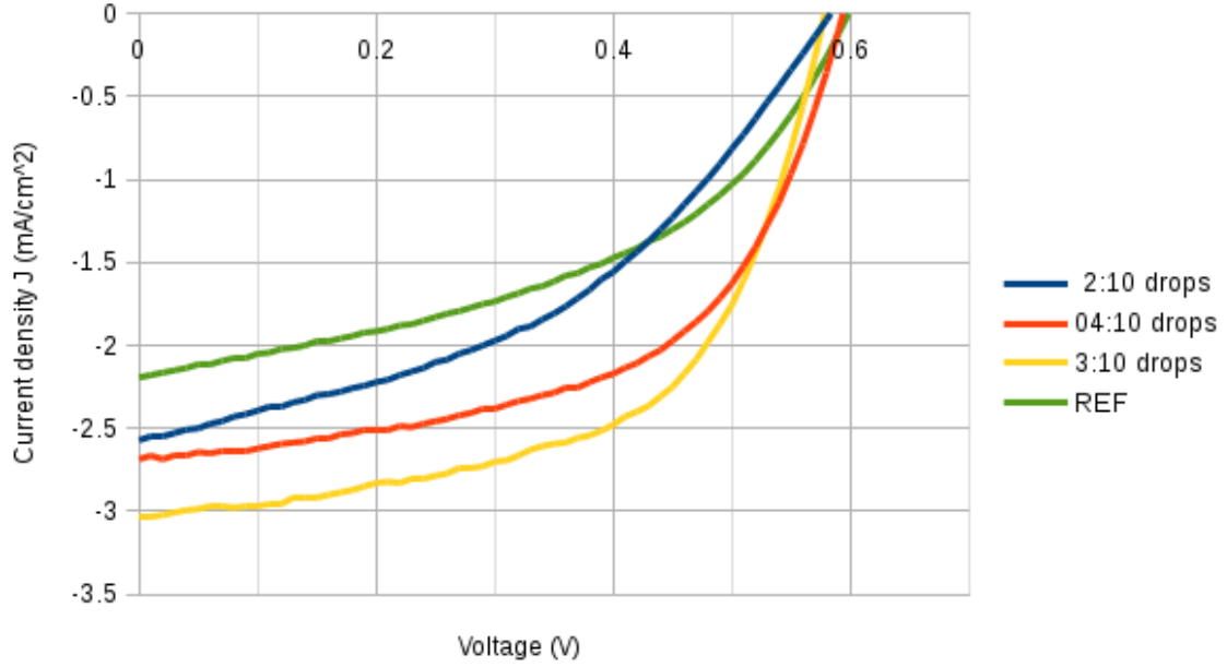
Figure 5.18: J-V characteristics fabricated device with varied concentration of Ag NPs in PEDOT:PSS.
