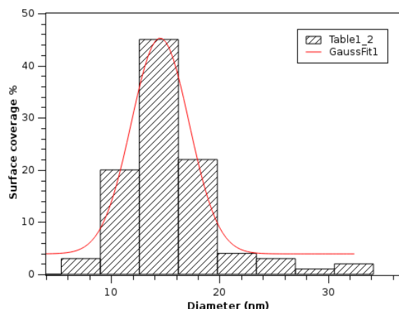
Figure 5.6: Histogram showing Ag spherical NPs of an average diameter of 15 nm.
