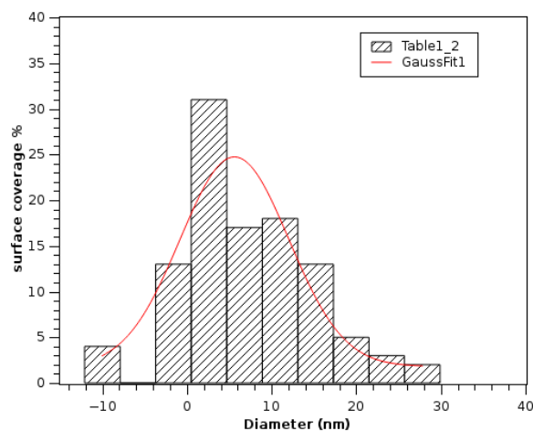
Figure 5.10: Histogram showing agglomerated Ag NPs average diameter of 16 nm.
