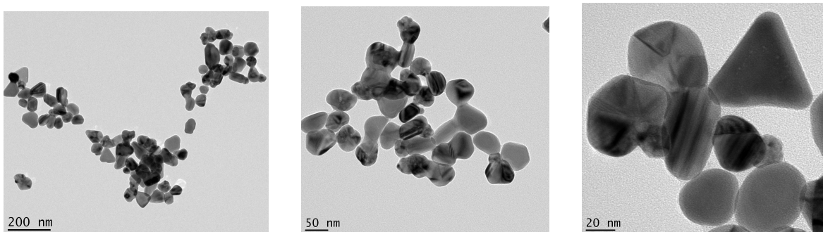
Figure 5.9: TEM images showing nucleated prism Ag NPs.
