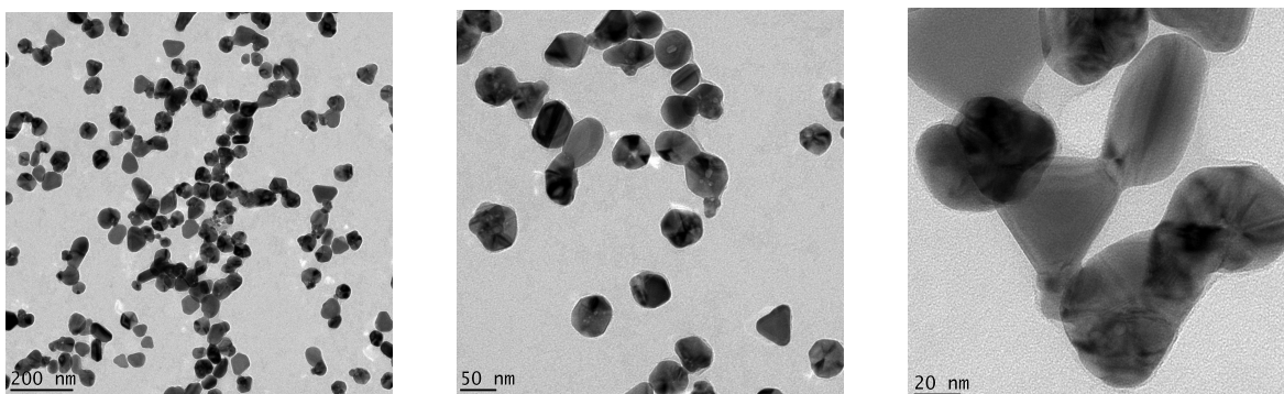
Figure 5.7: TEM images showing prism like Ag NPs.
