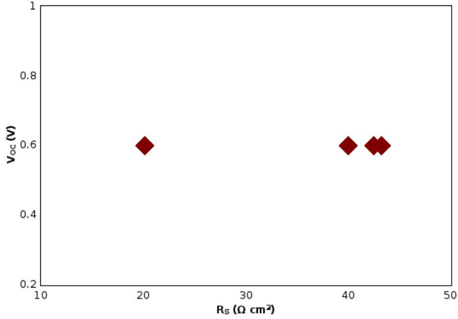
Figure 5.17: Shunt resistance increase at constant open circuit voltage.
