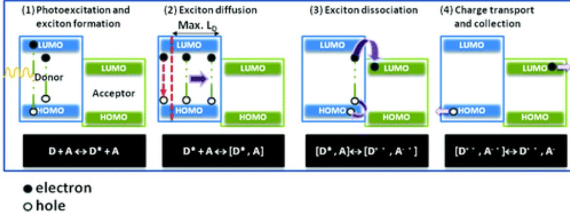
Figure 2.3: (1) Photoexcitation of the donor to generate a bound electron hole pair, called an exciton. (2) Exciton diffusion to the D-A interface. A distance longer than the maximum diffusion length (max DL) will lead to relaxation of the exciton. (3) Bound exciton dissociation at the D-A interface to form a geminate pair. (4) Free charge transportation and collection at electrodes [51].
