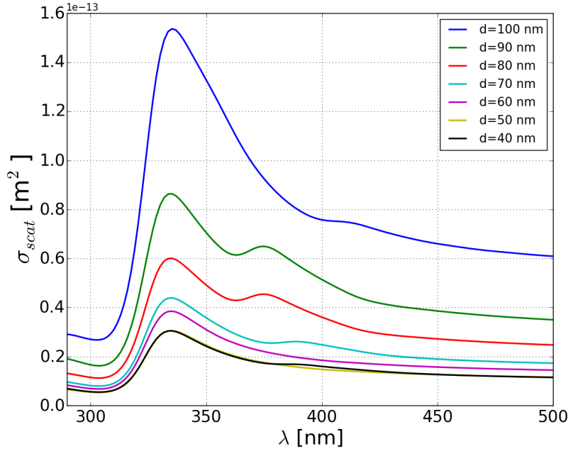
Figure 5.1: The scattering cross-section for silver spheres of different diameters.
