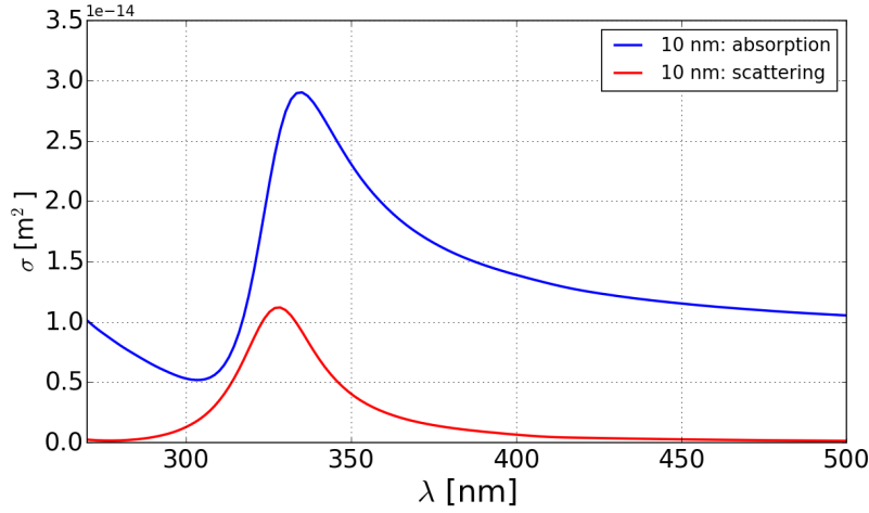
Figure 5.15: Absorption spectra for Ag spherical NPs of 10 nm diameter with MEEP simulation.
