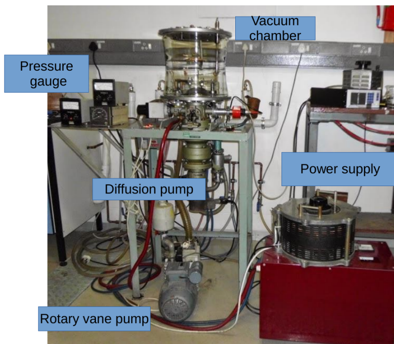
Figure 4.2: The experimental set-up of the thermal evaporation system used in the present study.
