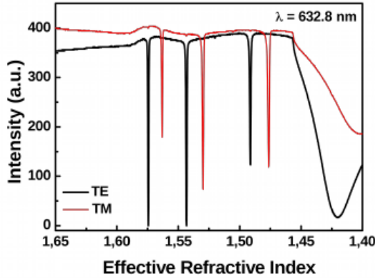
Figure 5.22: M-line measurement for both modes TE and TM
