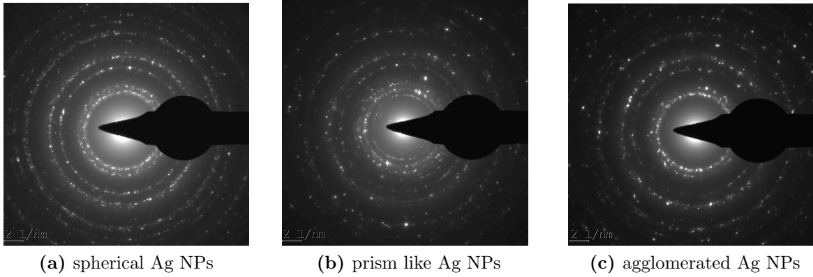
Figure 5.11: SAED patterns of Ag NP synthesized at varied reaction time
