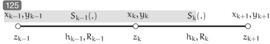
Figure 2.1: Configuration of notations, on two consecutive intervals, on the income axis.
