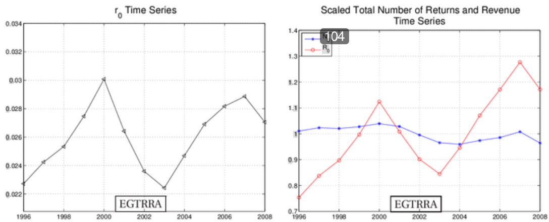
Figure 3.8: r_0 and scaled R_0, N_0 time series.
