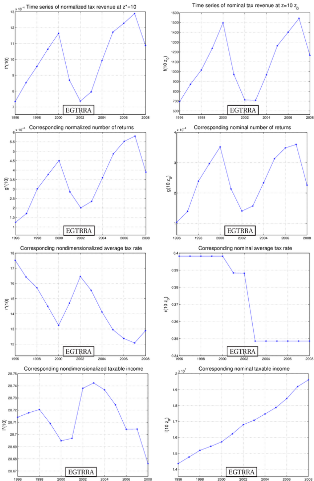
Figure 3.14: Time series at very high income levels, at z = 10 z_0 .
