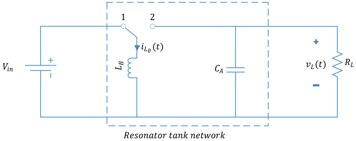
Figure 1-3: Ideal Buck-Boost Converter (Adapted from [12] )
