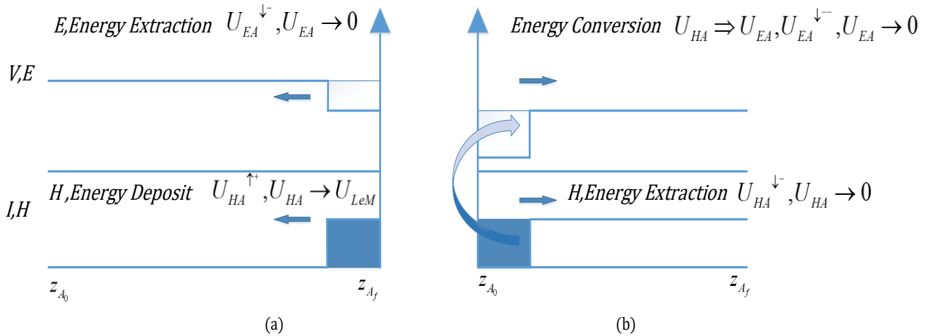
Figure 3-21: Electromagnetic Energy Interactions on C_r , Wave Propagation Towards (a) z_{A0} (b) z_{Af} .
