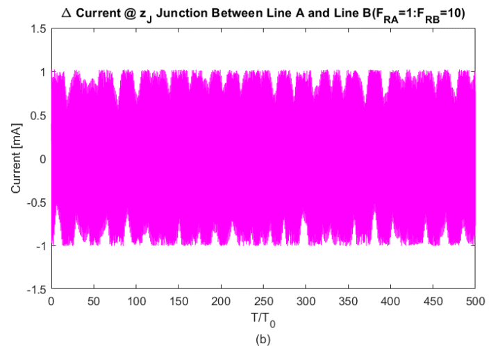
Figure 6-38: Current Differences at z_{B_f} and z_J a) \Delta i(z_{B_f}, t) b) \Delta i(z_J, t) ( F_{RA} = 1, F_{RB} = 10 )
