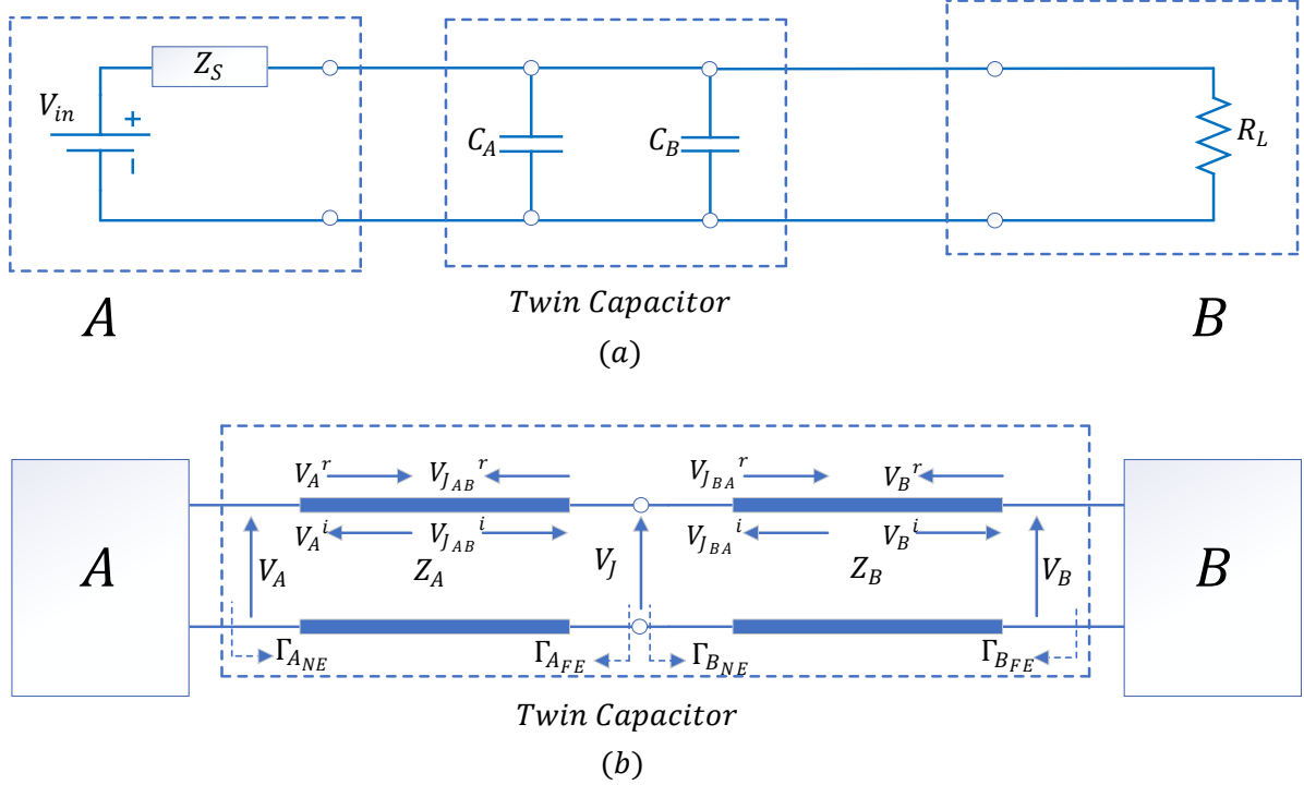
Figure 3-9: Switched Capacitor Converter System a) Coupled System b) Decoupled System
