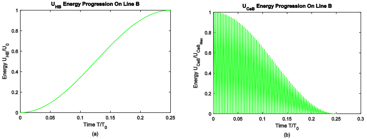
Figure 3-26: Normalized Energy Progressions Line B (a) U_{HB} (b) U_{CeB}
