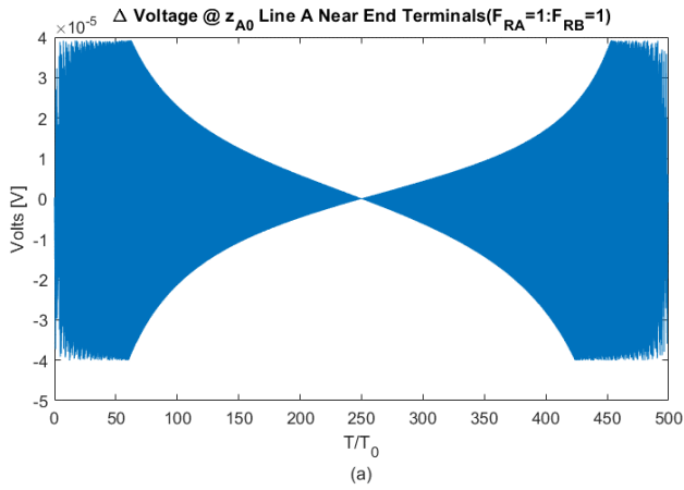
Figure 6-33: Voltage Differences at z_{A_0} and z_J a) \Delta v(z_{A_0}, t) b) \Delta v(z_{B_f}, t) ( F_{RA} = 1, F_{RB} = 1 )
