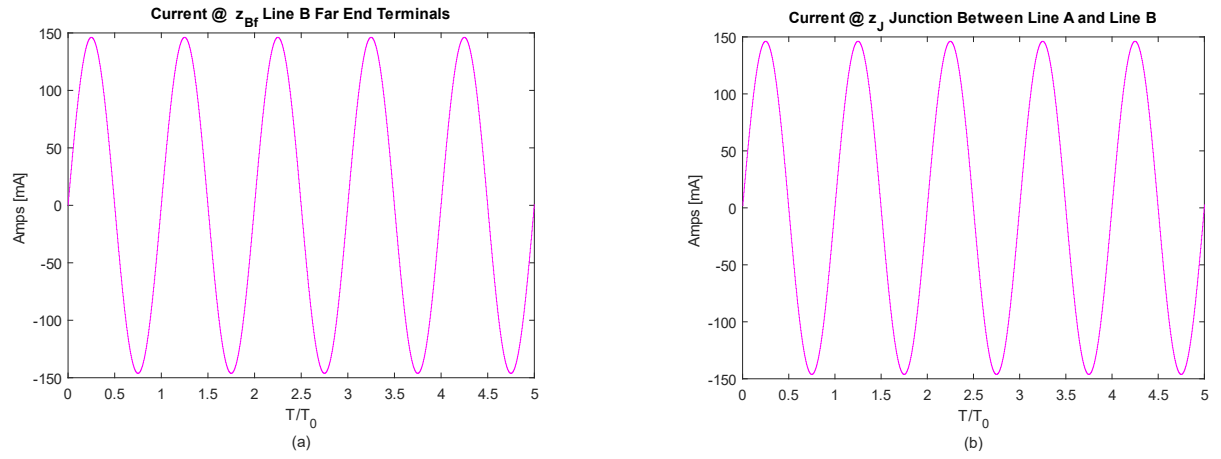
Figure A-5: LC Resonator Junction and Terminal Currents a) i_B(z_{Bf}, t) b) i_B(z_J, t)
