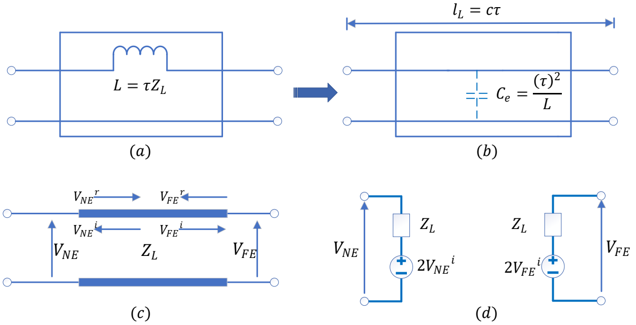
Figure 3-5: Series Inductor Models a) Lumped Element b) Self-Capacitance c) Link-Line d) Thevenin Equivalent
