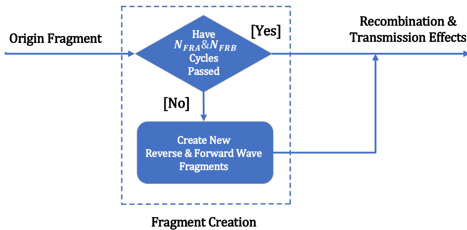
Figure 4-5: Algorithm Determining Fragment Creation At The Junction Or Discontinuity
