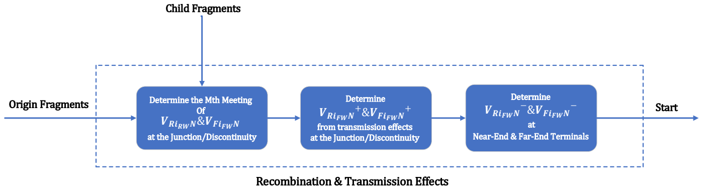
Figure 4-6: Algorithm Detailing Recombination Effects At The Junction Or Discontinuity
