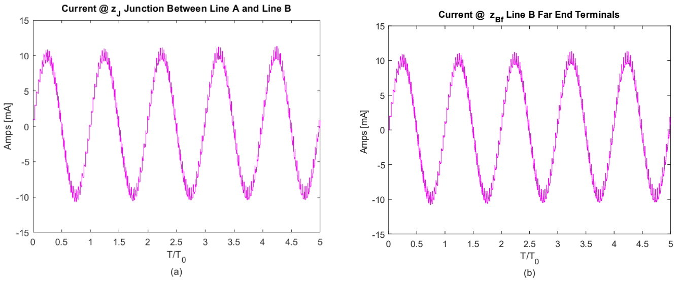
Figure 6-36: Generated Current Waveforms a) i(z_J, t) b) i_B(z_{Bf}, t) ( F_{RA} = 1, F_{RB} = 10 )
