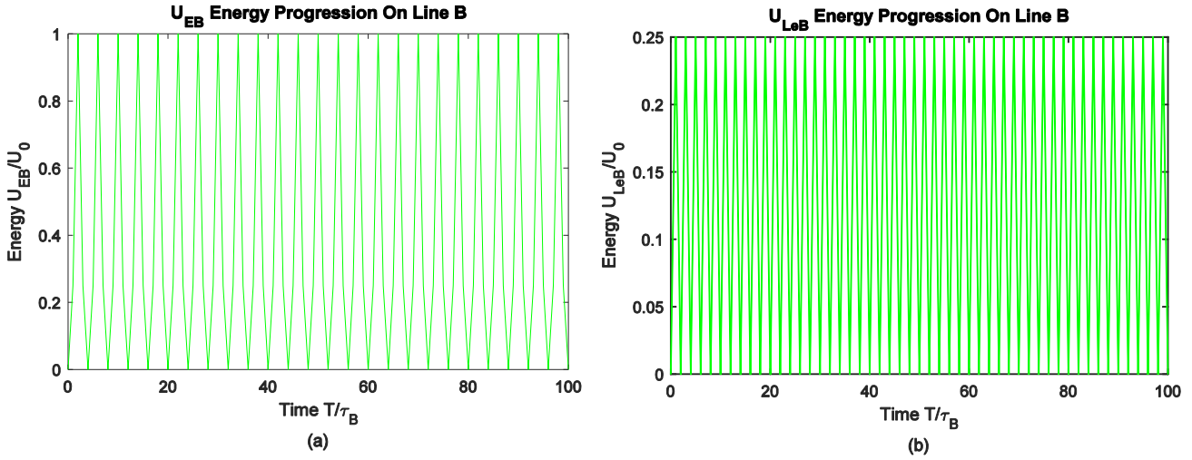
Figure 3-18: Line B ( C_B ) Energy Progressions a) U_{EB} b) U_{LeB}
