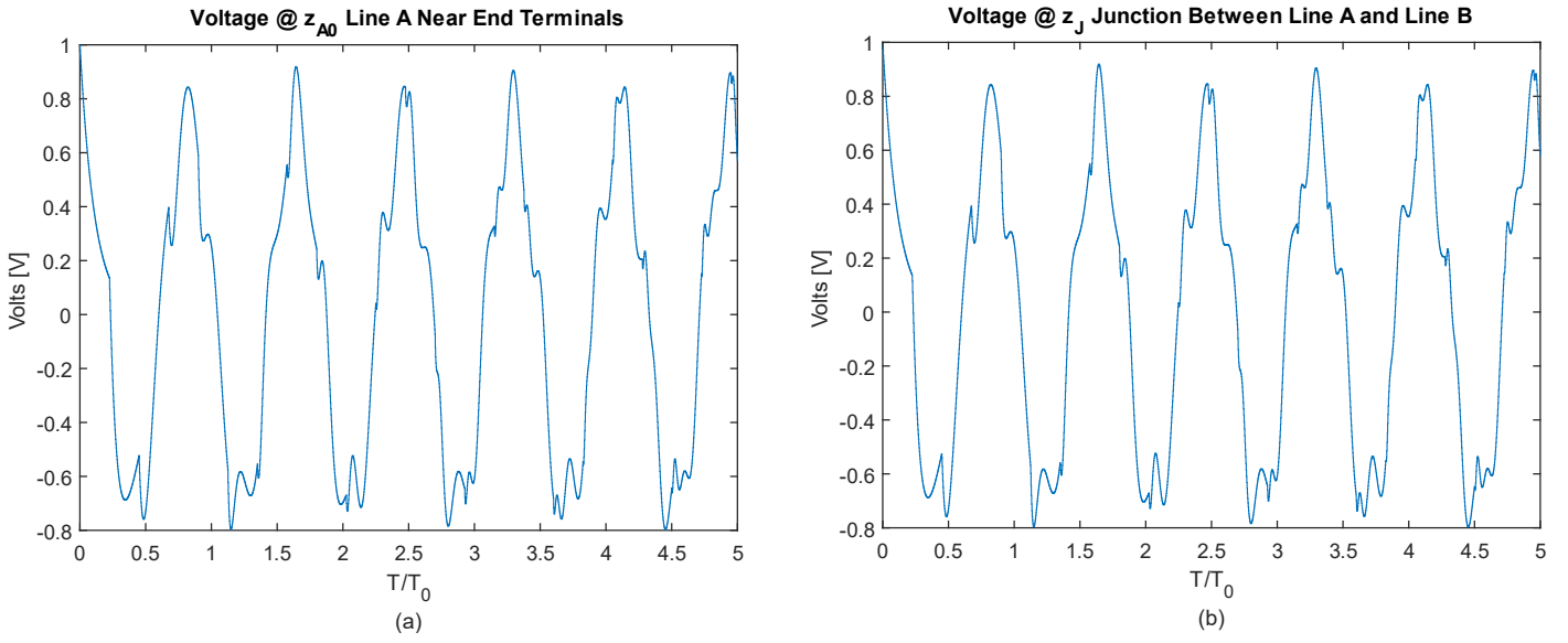
Figure 6-39: Generated Voltage waveforms a) v_A(z_{A0}, t) b) v(z_J, t) ( F_{RA} = 1, F_{RB} = 100 )
