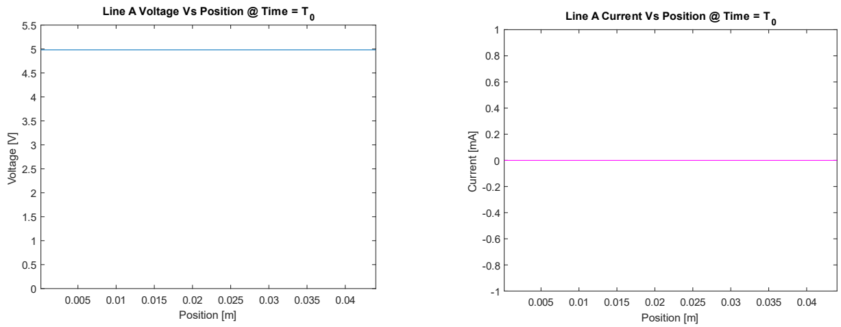
Figure A-6: LC Resonator Line A Voltage and Current @ T_0 ( v_A(z, T_0) , i_A(z, T_0) )
