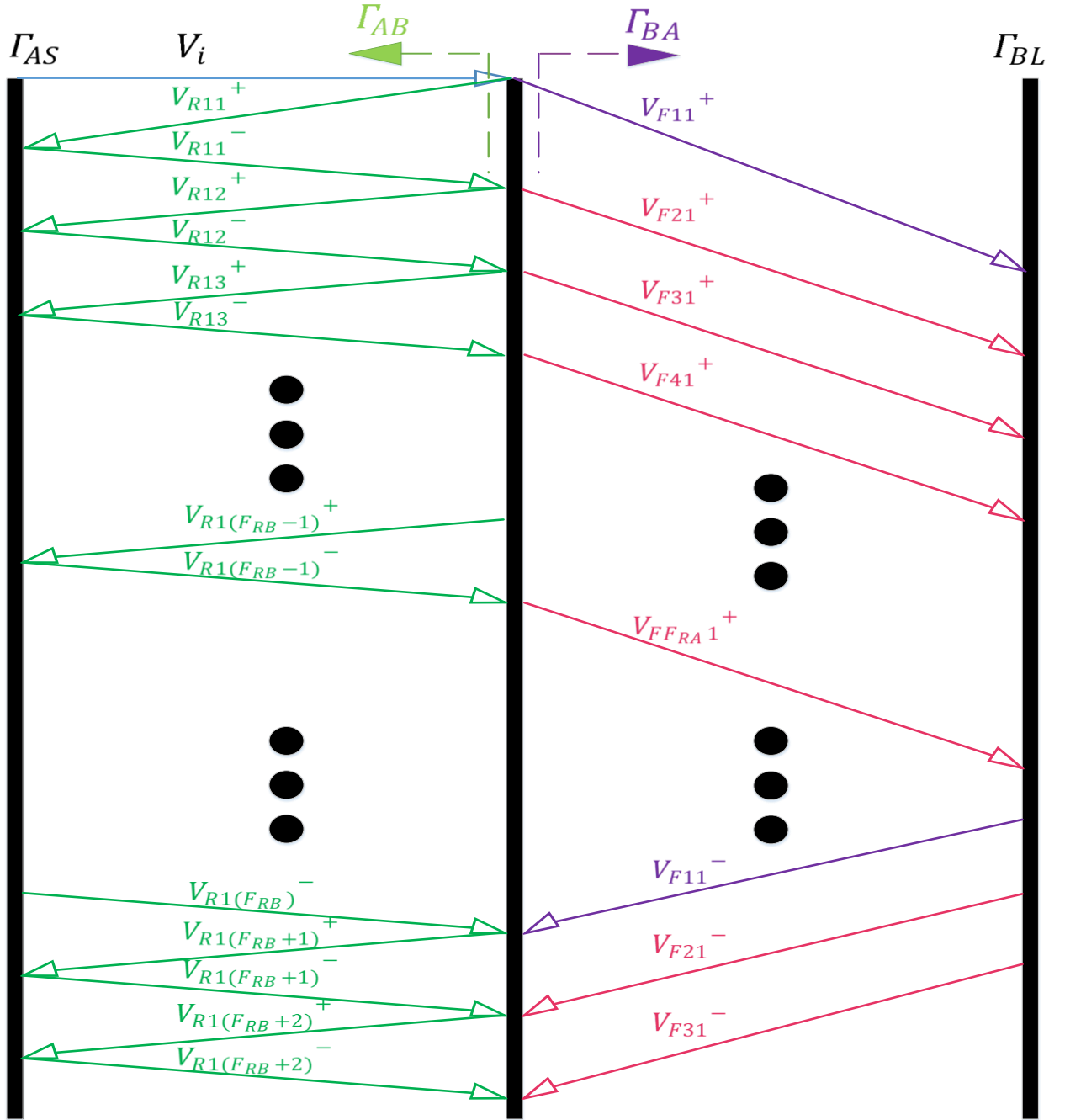
Figure 4-8: Finite Fragment Generation 1: k (FFGIMD)
