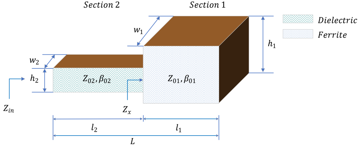
Figure A-1: Parallel Planar LC Resonant Structure (Adapted from [20])
