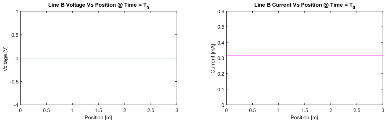
Figure 6-23: LC Resonator Line B Voltage and Current @ T_0 ( v_B(z, T_0) , i_B(z, T_0) )
