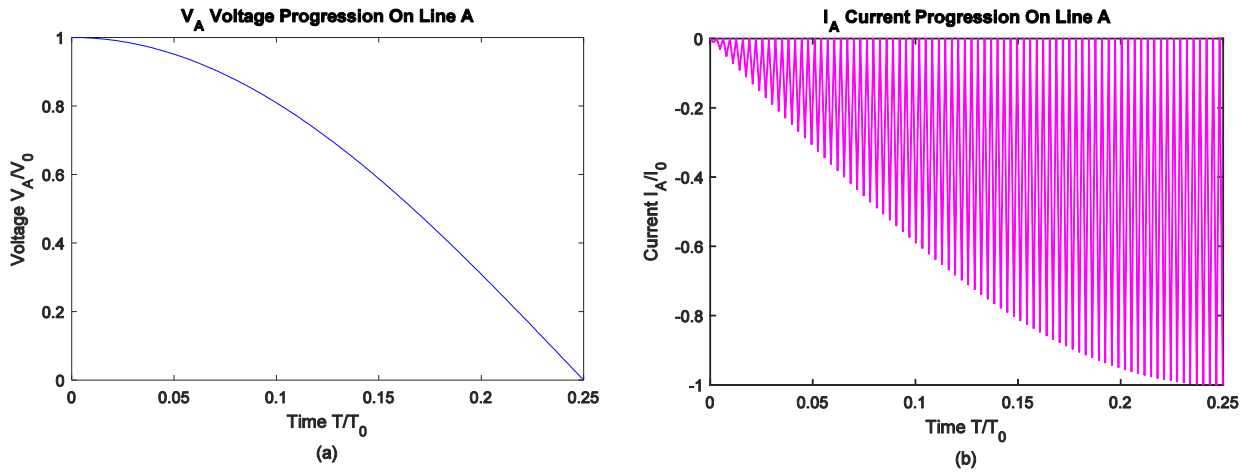
Figure 3-22: Line A ( C_r ) Voltage and Current Progressions (a) Voltage ( V_A \rightarrow 0 ) (b) Current ( I_A \rightarrow -I_0 )
