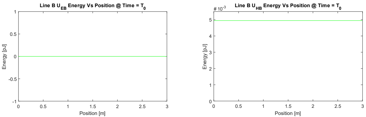
Figure 6-24: LC Resonator Line B Electric and Magnetic Energies @ T_0 ( U_{EB}(z, T_0) , U_{HB}(z, T_0) )
