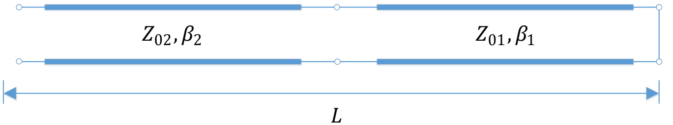
Figure 2-6: Transmission Line Model of Parallel LC Resonant Structure (Adapted from [20])
