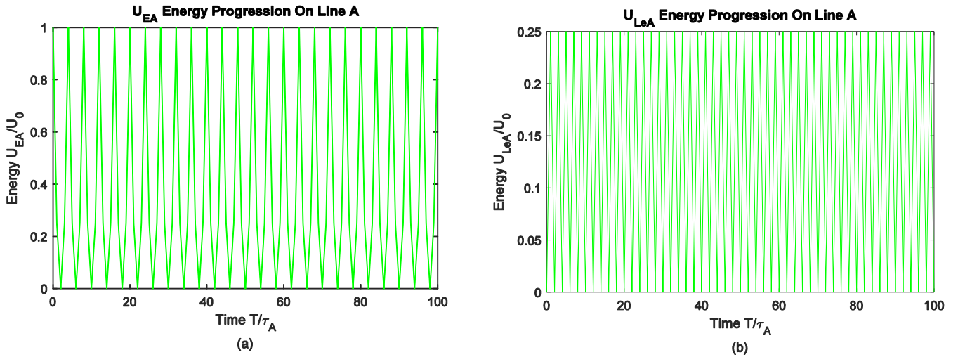
Figure 3-17: Line A ( C_A ) Energy Progressions a) U_{EA} b) U_{LeA}
