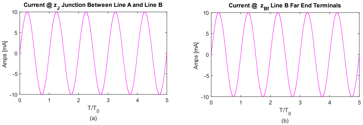
Figure 6-20: LC Resonator Junction and Terminal Currents a) i_B(z_J, t) b) i_B(z_{B_f}, t)
