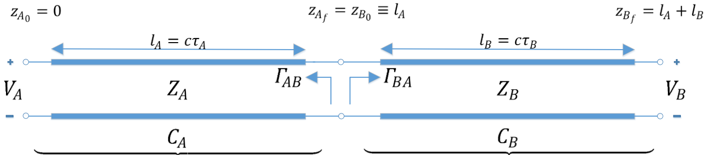
Figure 3-12: Twin Capacitor Link-Line Model (Switch Closed)
