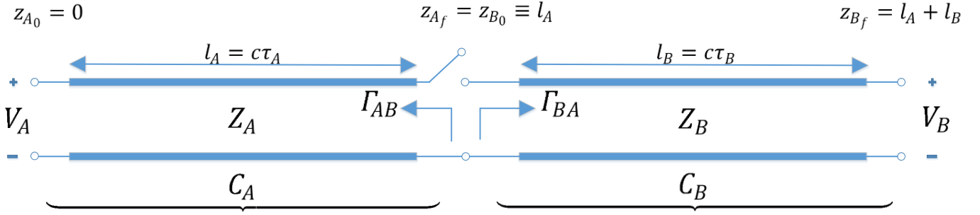
Figure 3-11: Twin Capacitor Link-Line Equivalent Model (Switch Open)
