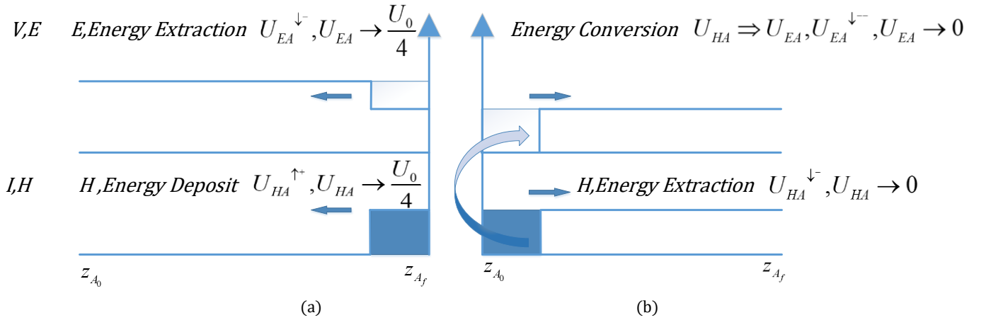
Figure 3-13: Energy Interactions on C_A Wave Propagation Towards a) z_{A0} b) z_{Af}
