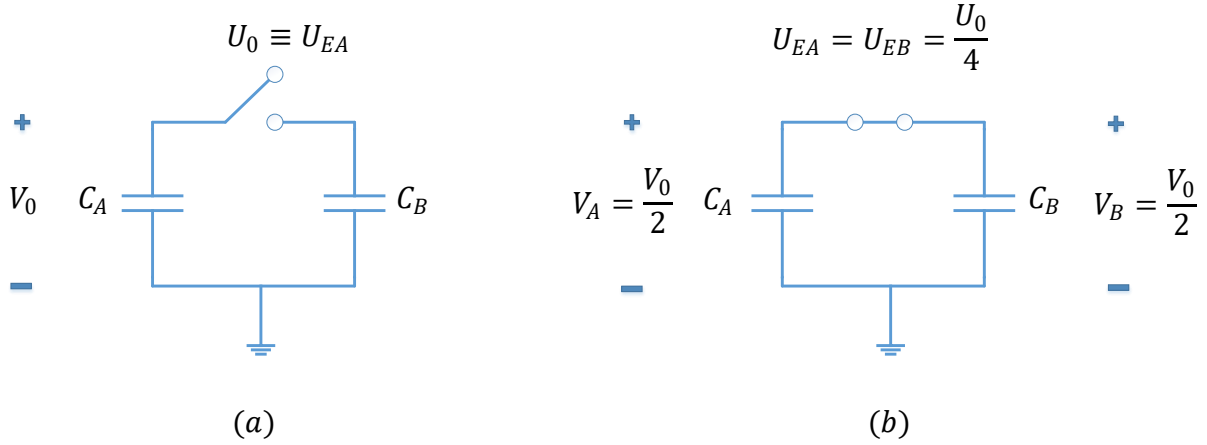
Figure 2-1: Twin Capacitor a) Initial State b) Equilibrium State
