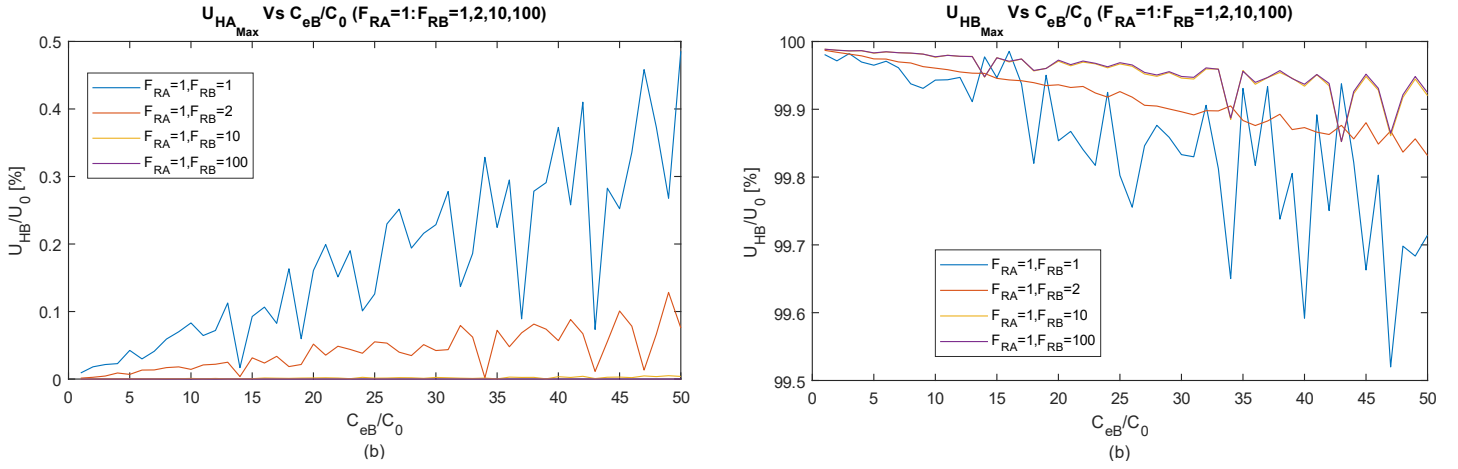
Figure 6-29: LC Resonator Max Magnetic Line Energies vs. Self-Capacitance (FFGIMD) a) U_{HA\_Max} b) U_{HB\_Max}
