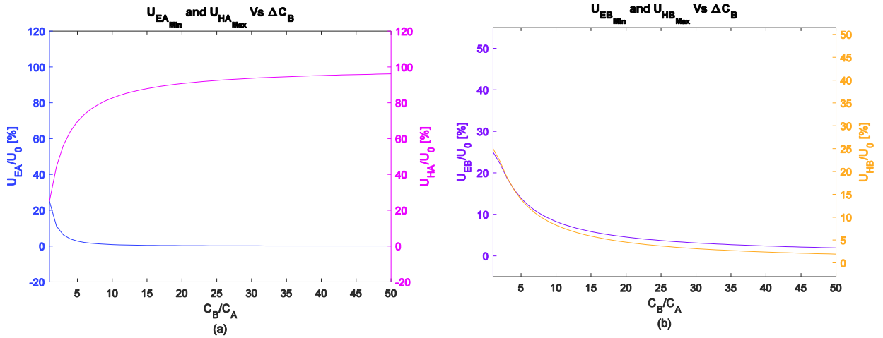
Figure 6-4: Min Electrical and Max Magnetic Line Energies Vs. Capacitance
