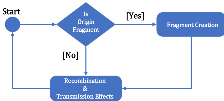
Figure 4-4: High Level Algorithm for Establishing Fragmentation Generation Cases
