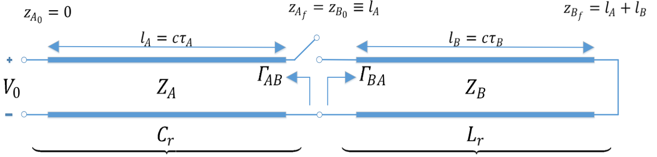
Figure A-2: Resonator Tank Link-Line Equivalent Model (Switch Open)
