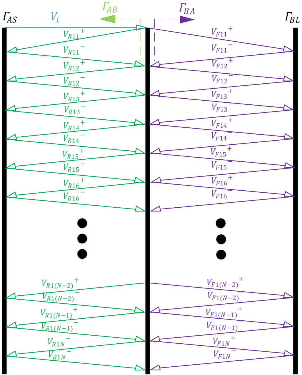
Figure 4-9: Finite Fragment Generation 1:1 (FFGMD)
