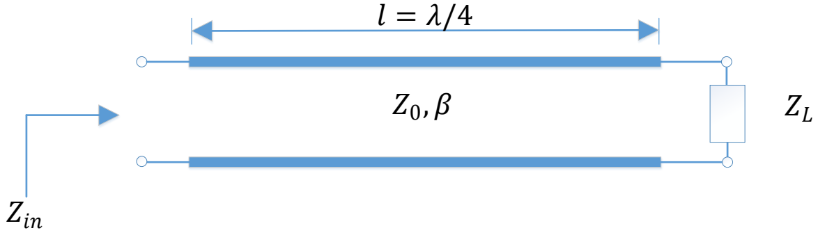
Figure 2-4: General \lambda/4 Transmission Line terminated by load Z_L (Adapted from [20])
