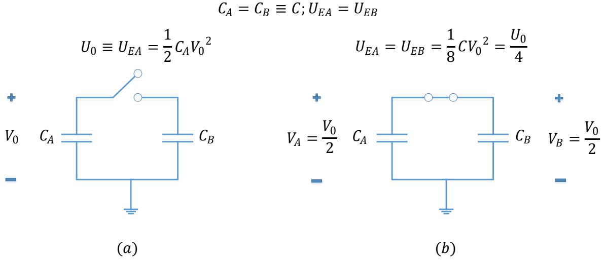
Figure 3-10: Twin Capacitor Paradox a) Initial Charged State b) Equilibrium State
