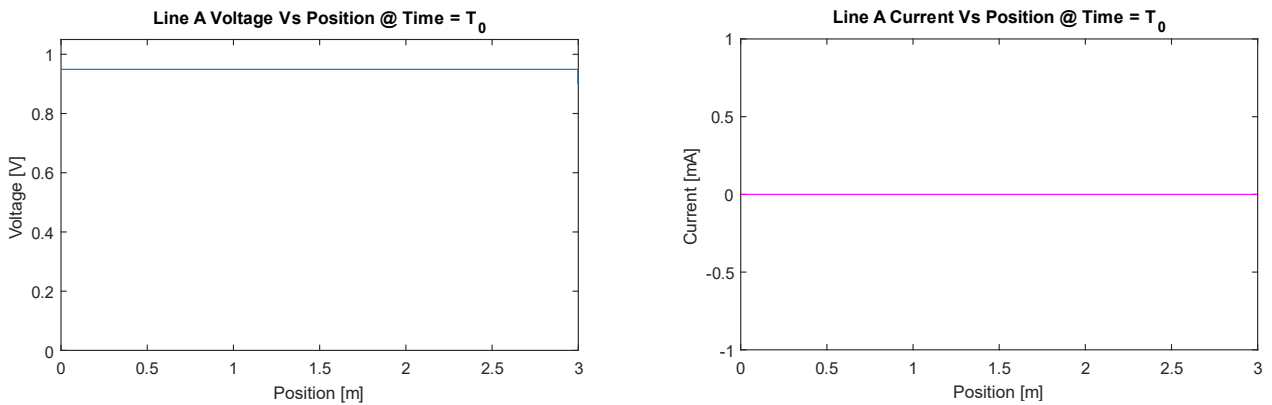
Figure 6-21: LC Resonator Line A Voltage and Current @ T_0 ( v_A(z, T_0) , i_A(z, T_0) )
