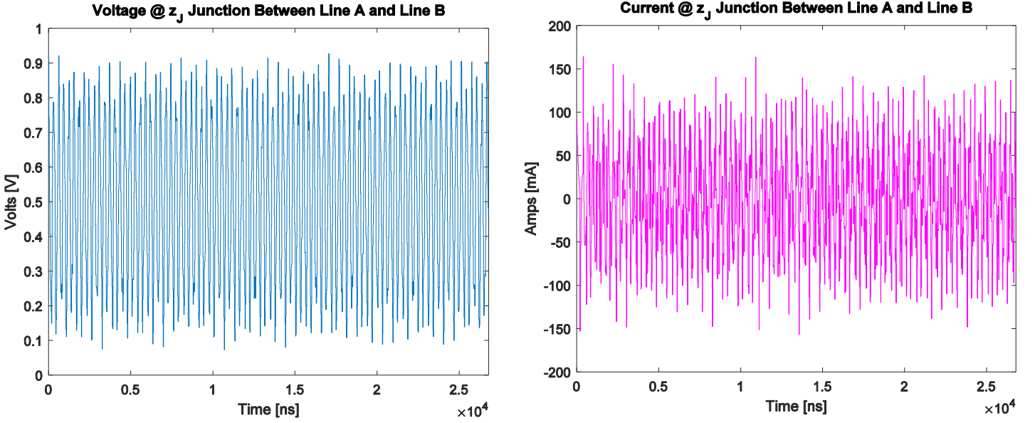
Figure 6-13: Junction Voltage and Current a) v(z_J, t) b) i(z_J, t) ( F_{RA} = 1, F_{RB} = 10 )
