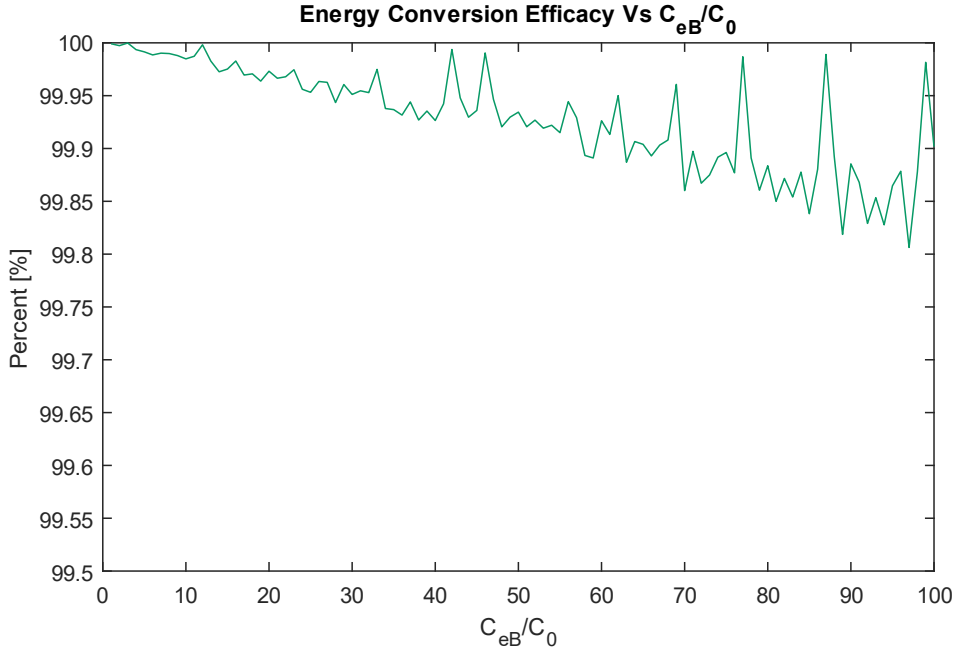
Figure A-12: LC Resonator Energy Conversion Efficacy Vs. Self-Capacitance
