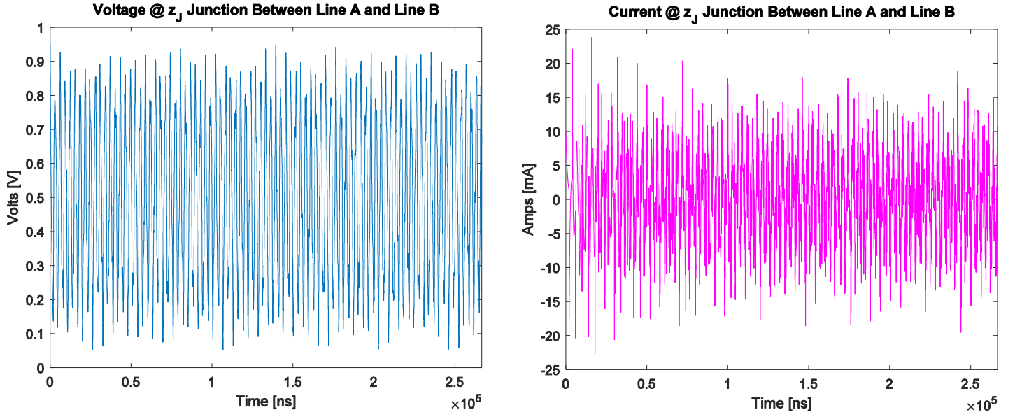
Figure 6-15: Junction Voltage and Current a) v(z_J, t) b) i(z_J, t) ( F_{RA} = 1, F_{RB} = 100 )
