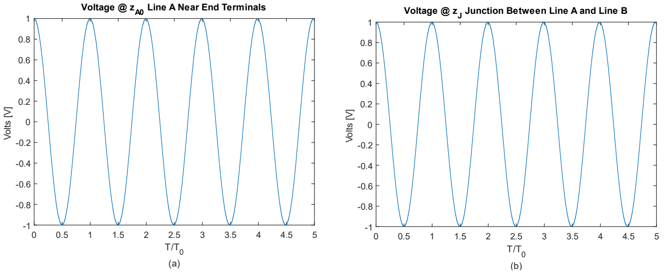
Figure 6-35: Generated Voltage waveforms a) v_A(z_{A0}, t) b) v(z_J, t) ( F_{RA} = 1, F_{RB} = 10 )
