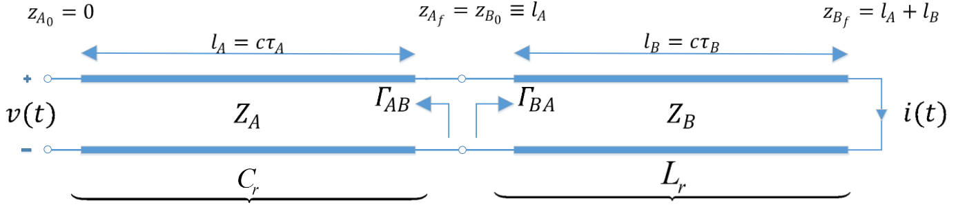
Figure 3-20: Resonator Tank Link-Line Equivalent Model (Switch Closed)
