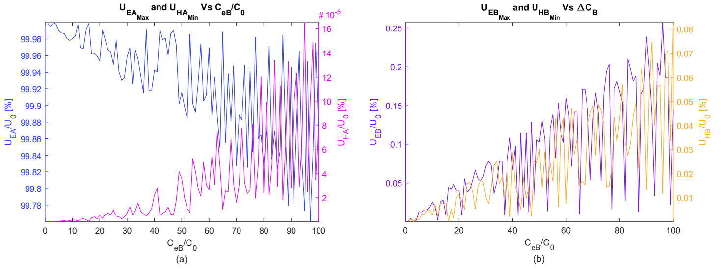
Figure A-10: LC Resonator Max Electrical and Min Magnetic Line Energies Vs. Self-Capacitance
