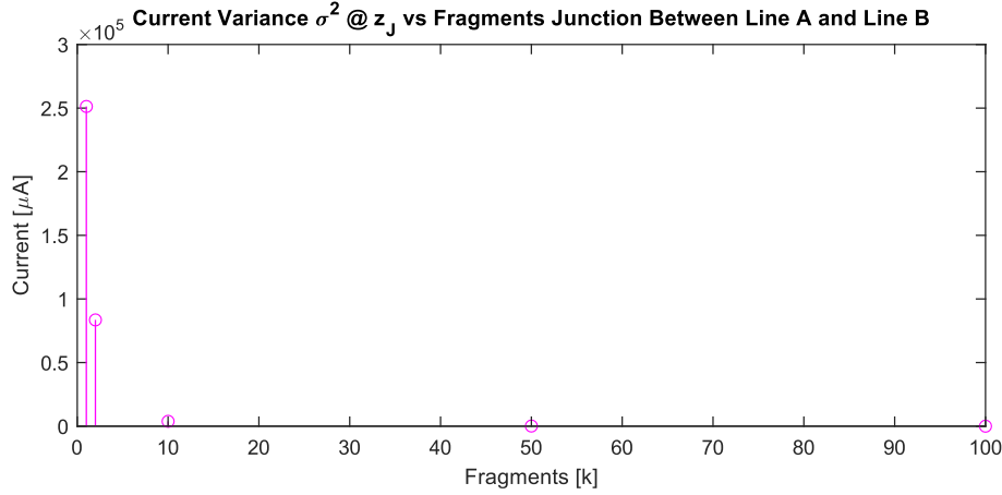
Figure 6-17: Junction Current Variance Var(i(z_J, t)) ( F_{RA} = 1, F_{RB} = 1, 2, 10, 50, 100 )
