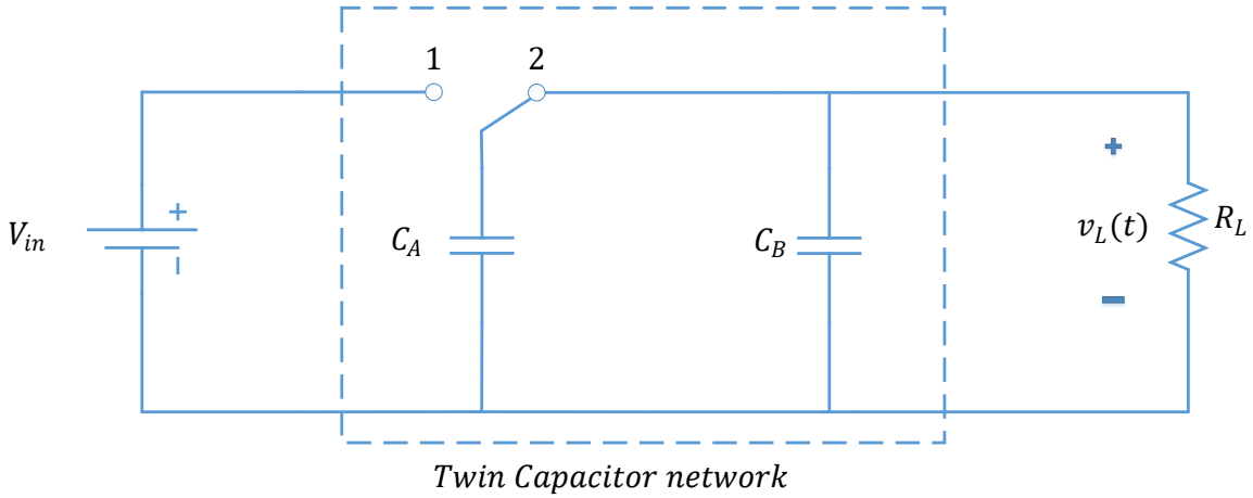
Figure 1-2: Switched-Capacitor Converter
