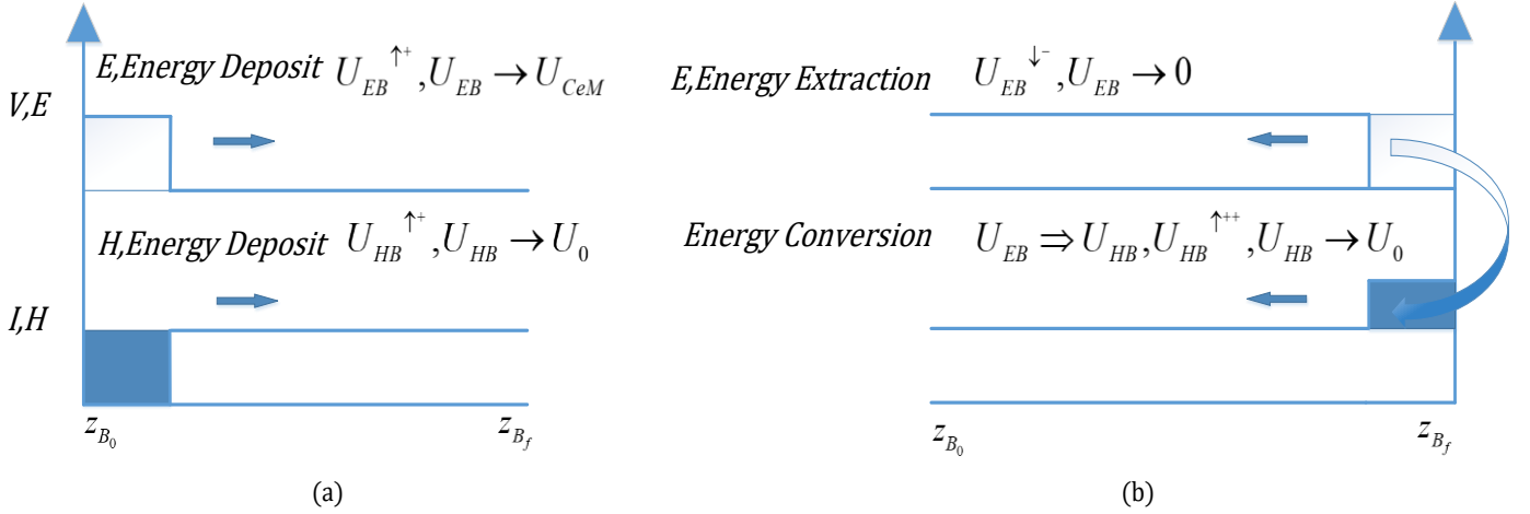
Figure 3-24 Electromagnetic Energy Interactions on L_r , Wave Propagation Towards (a) z_{B_f} (b) z_{B_0}
