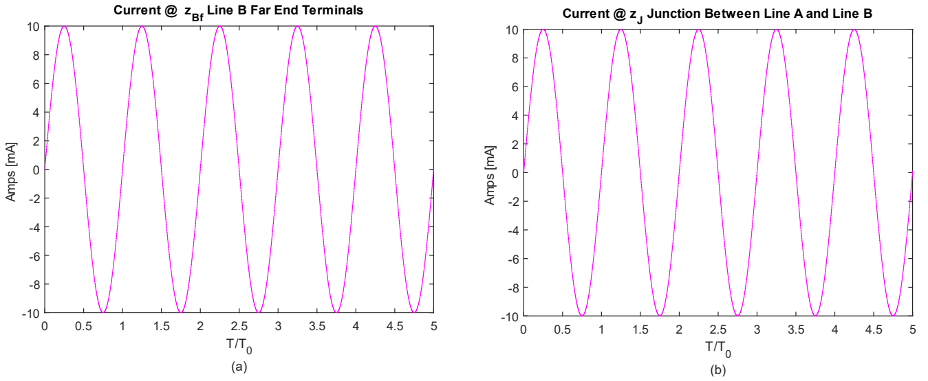
Figure 6-32: Generated Current Waveforms a) i_B(z_{B_f}, t) b) i(z_J, t) ( F_{RA} = 1, F_{RB} = 1 )
