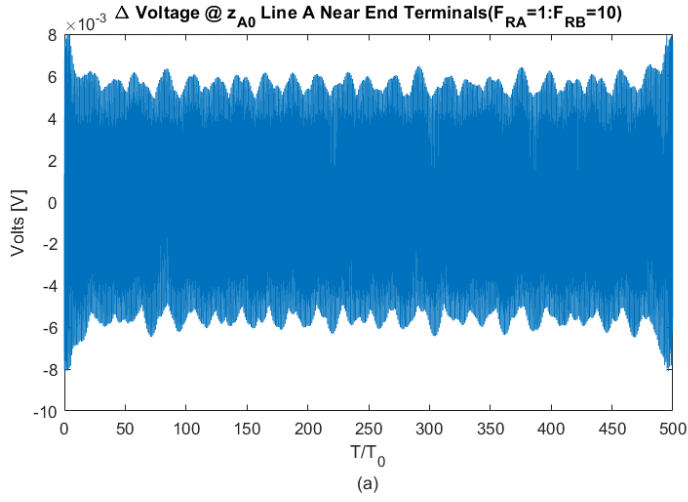
Figure 6-37: Voltage Differences at z_{A_0} and z_J a) \Delta v(z_{A_0}, t) b) \Delta v(z_{B_f}, t) ( F_{RA} = 1, F_{RB} = 10 )
