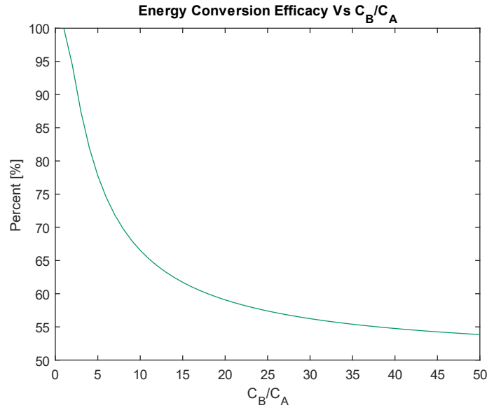
Figure 6-5: Energy Conversion Efficacy Vs. Capacitance
