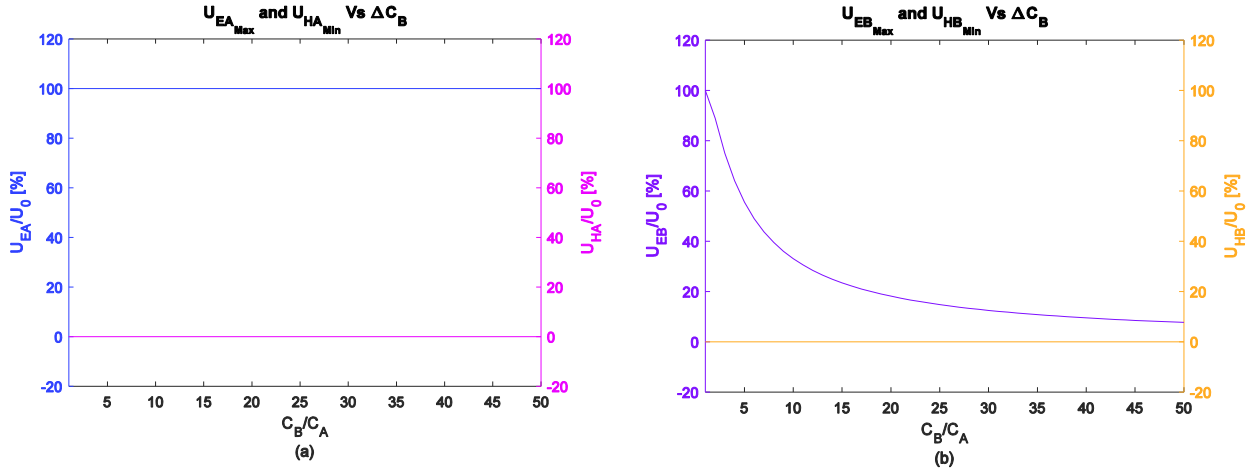
Figure 6-3: Max Electrical and Min Magnetic Line Energies Vs. Capacitance
