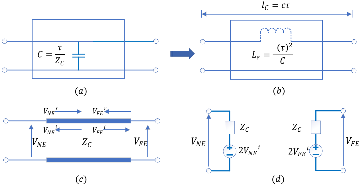
Figure 3-6: Shunt Capacitor Models a) Lumped Element b) Self-Inductance c) Link-Line d) Thevenin Equivalent
