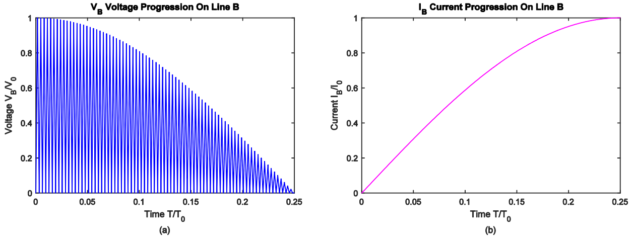
Figure 3-25: Line B Voltage and Current Progressions (a) Voltage ( V_B \rightarrow 0 ) (b) Current ( I_B \rightarrow I_0 )
