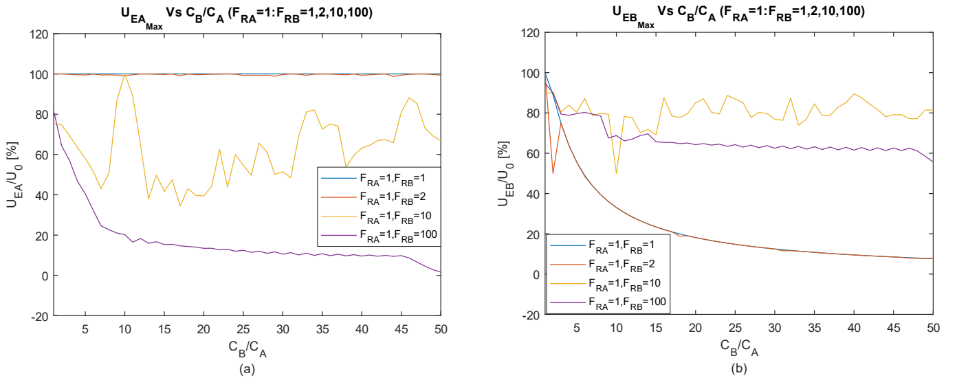
Figure 6-6: Maximum Electrical Energies vs. Changing Capacitance (FFGIMD) a) U_{EA_{Max}} b) U_{EB_{Max}}
