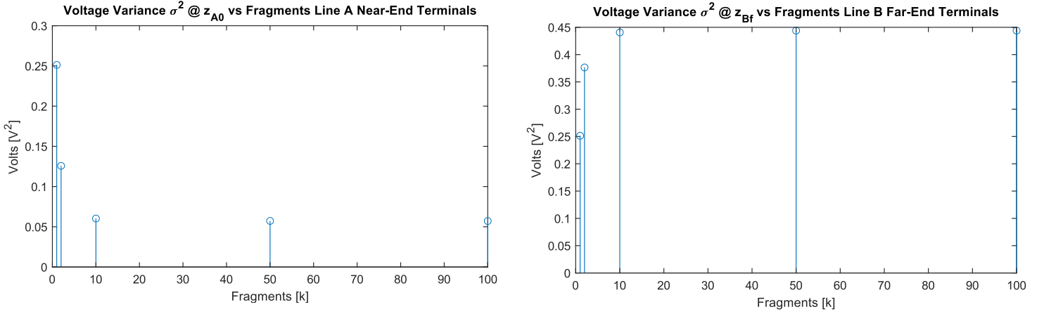
Figure 6-16: Terminal Voltage Variance a) Var(v(z_{A_0}, t)) b) Var(v(z_{B_f}, t)) ( F_{RA} = 1, F_{RB} = 1, 2, 10, 50, 100 )
