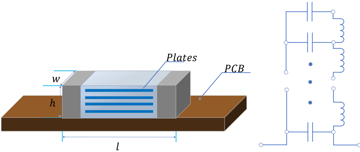
a) Physical Structure of MLC Capacitor
