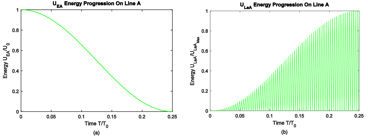
Figure 3-23: Normalized Energy Progressions Line A (a) U_{EA} (b) U_{LaA}
