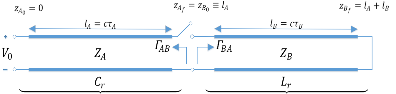
Figure 3-19: Resonator Tank Link-Line Equivalent Model (Switch Open)
