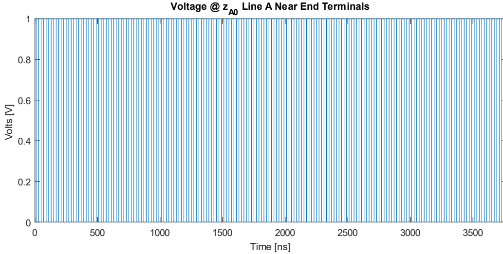
Figure 6-8: Line A Voltage at z_{A_0} terminals ( F_{RA} = 1, F_{RB} = 1 )
