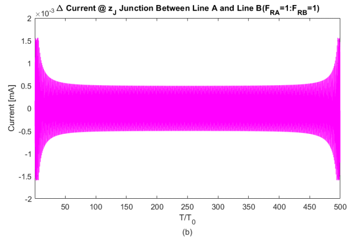
Figure 6-34: Current Differences at z_{B_f} and z_J a) \Delta i(z_{B_f}, t) b) \Delta i(z_J, t) ( F_{RA} = 1, F_{RB} = 1 )
