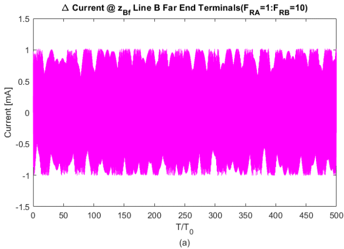
Figure 6-38: Current Differences at z_{B_f} and z_J a) \Delta i(z_{B_f}, t) b) \Delta i(z_J, t) ( F_{RA} = 1, F_{RB} = 10 )
