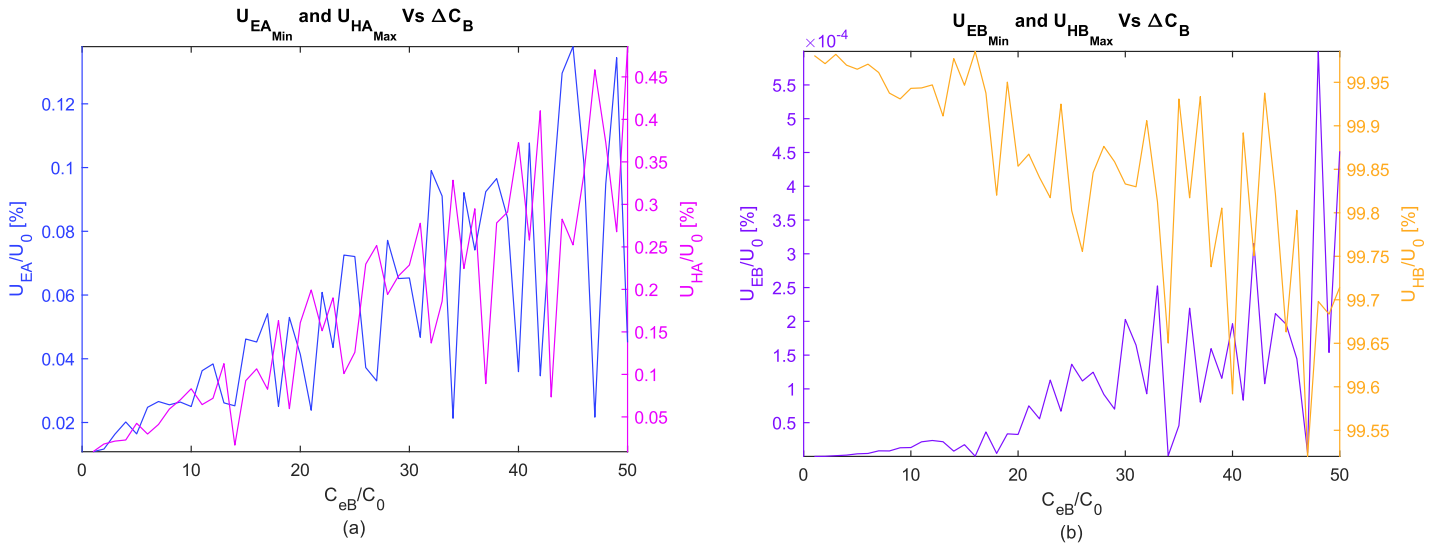
Figure 6-26: LC Resonator Min Electrical and Max Magnetic Line Energies Vs. Self-Capacitance
