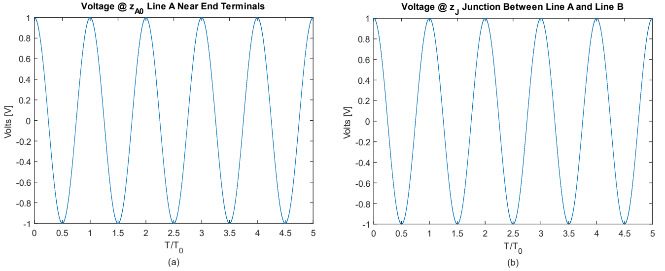
Figure 6-31: Generated Voltage Waveforms a) v_A(z_{A_0}, t) b) v(z_J, t) ( F_{RA} = 1, F_{RB} = 1 )
