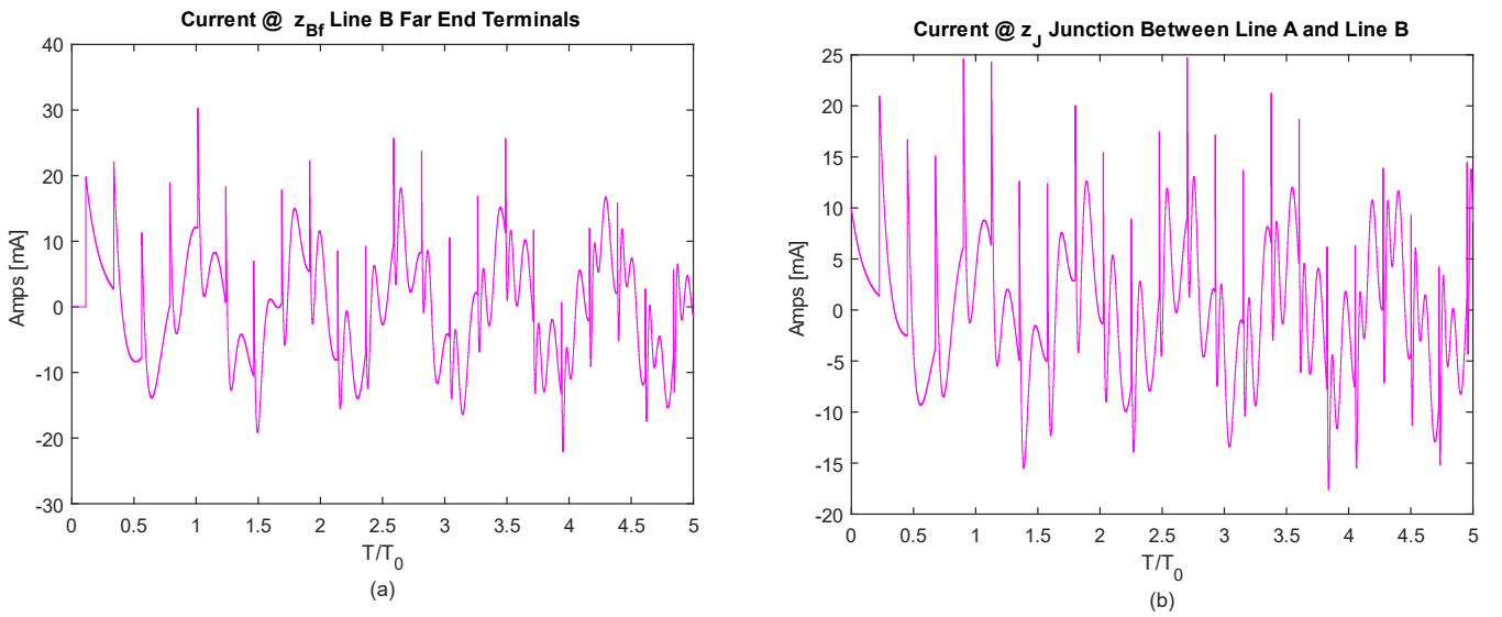
Figure 6-40: Generated Current Waveforms a) i_B(z_{Bf}, t) b) i(z_J, t) ( F_{RA} = 1, F_{RB} = 100 )
