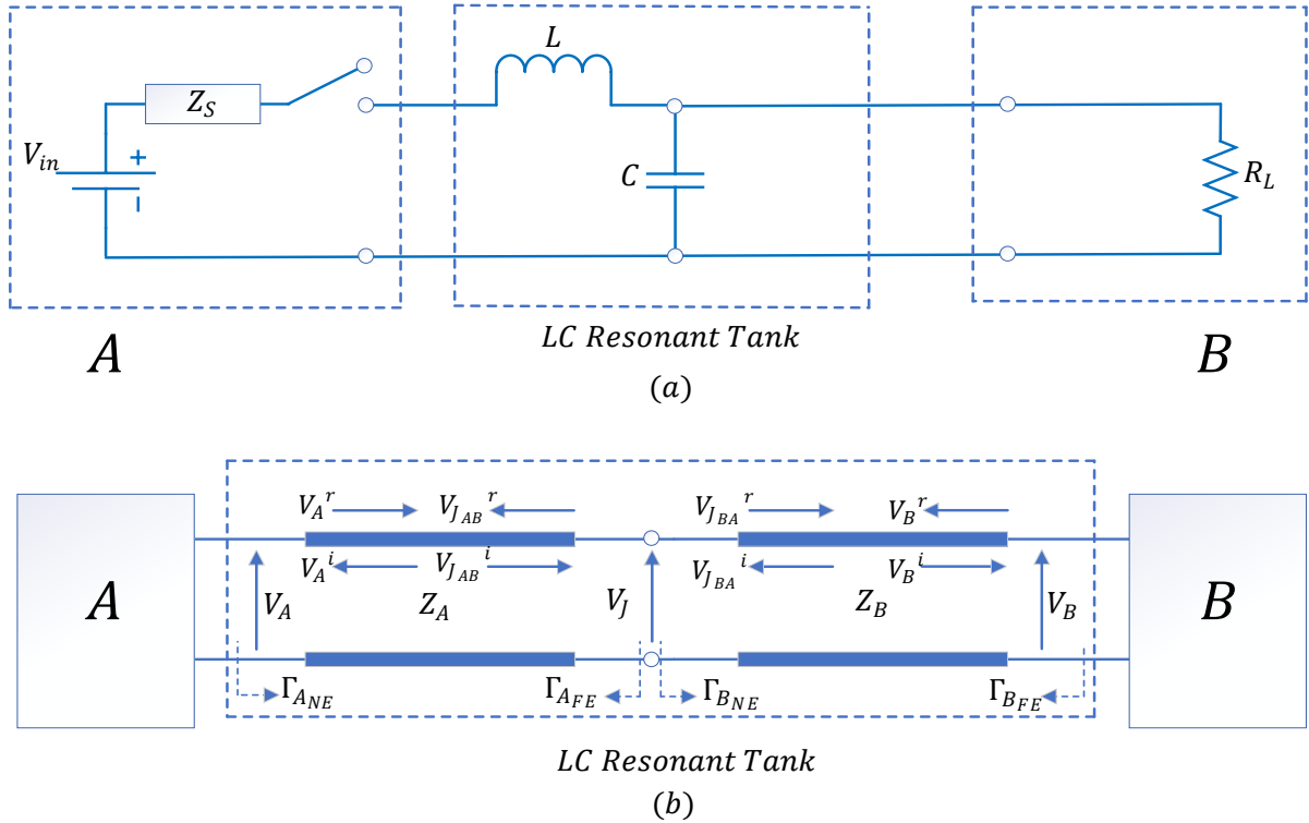
Figure 3-8: SMPS Converter System a) Coupled System b) Decoupled System
