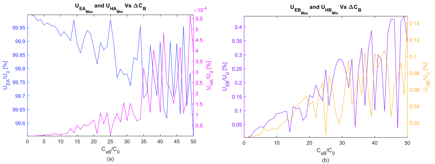
Figure 6-25: LC Resonator Max Electrical and Min Magnetic Line Energies Vs. Self-Capacitance
