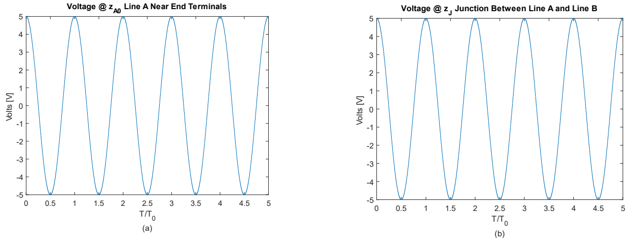
Figure A-4: LC Resonator Terminal and Junction Voltages a) v_A(z_{A0}, t) b) v_A(z_J, t)
