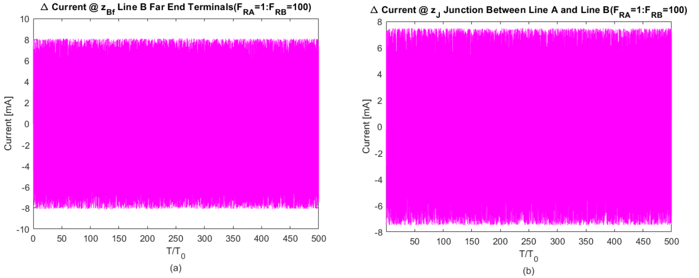
Figure 6-42: Current Differences at z_{B_f} and z_J a) \Delta i(z_{B_f}, t) b) \Delta i(z_J, t) ( F_{RA} = 1, F_{RB} = 100 )
