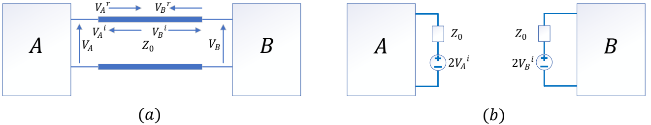
Figure 3-7: Decoupled Systems via a) Link-Line model b) Thevenin Equivalent model (Adapted from [39])
