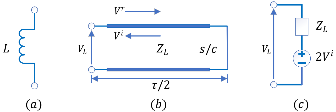
Figure 3-4: Inductor Models a) Lumped Element b) TLM Stub c) Thevenin Equivalent Circuit
