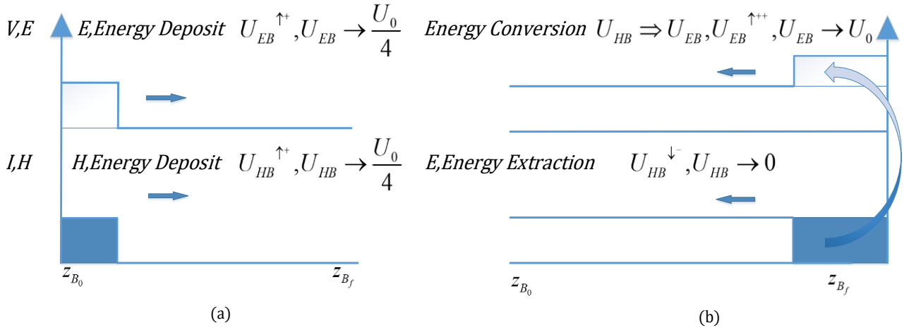
Figure 3-14: Energy Interactions on C_B Wave Propagation Towards a) z_{A0} b) z_{Af}
