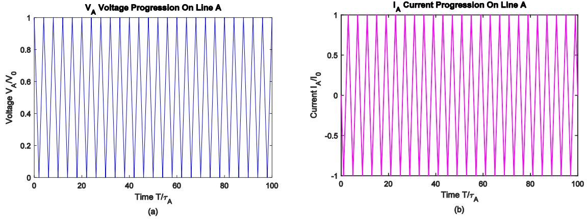
Figure 3-15: Line A ( C_A ) Voltage and Current Progressions a) Voltage b) Current
