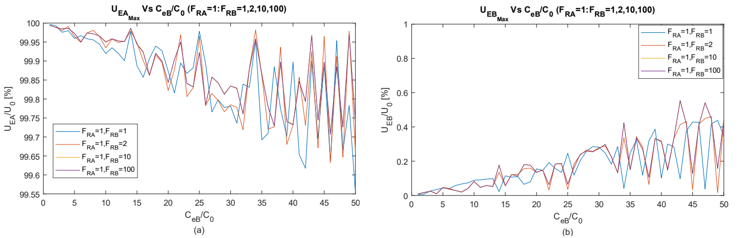
Figure 6-28: LC Resonator Max Electrical Energies vs. Self-Capacitance (FFGIMD) a) U_{EA_{Max}} b) U_{EB_{Max}}
