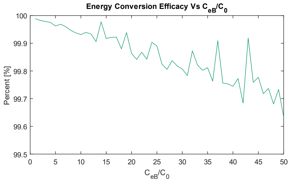
Figure 6-27: LC Resonator Energy Conversion Efficacy Vs. Self-Capacitance
