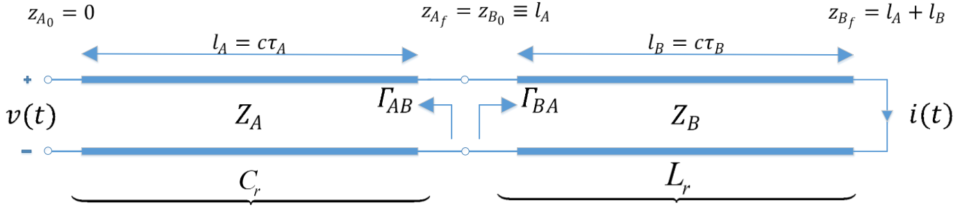
Figure A-3: Resonator Tank Link-Line Equivalent Model (Switch Closed)
