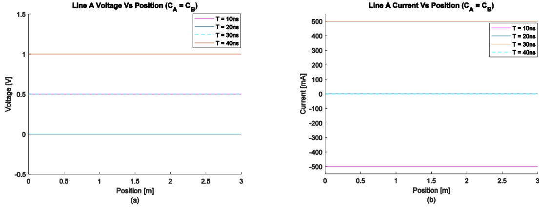
Figure 6-1: FFGMD Line A Distributions ( C_A = C_B ) a) Voltage b) Current
