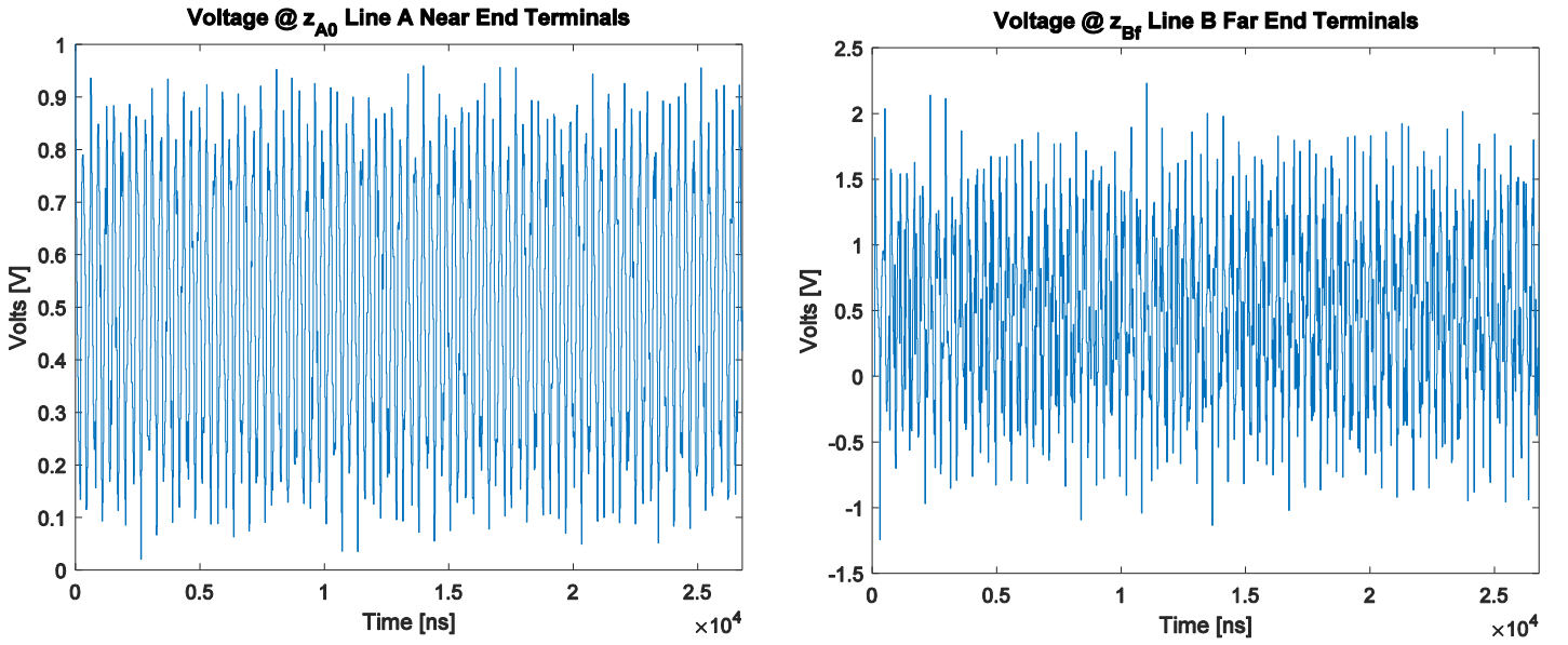
Figure 6-14: Terminal Voltages a) v(z_{A0}, t) b) v(z_{Bf}, t) ( F_{RA} = 1, F_{RB} = 100 )
