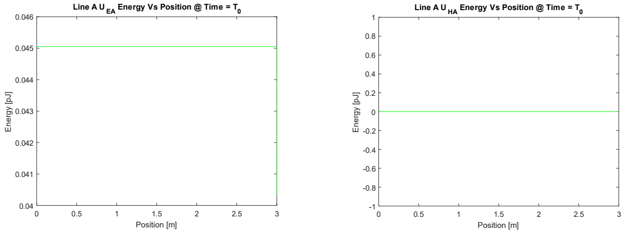
Figure 6-22: LC Resonator Line A Electric and Magnetic Energies @ T_0 ( U_{EA}(z, T_0) , U_{HA}(z, T_0) )
