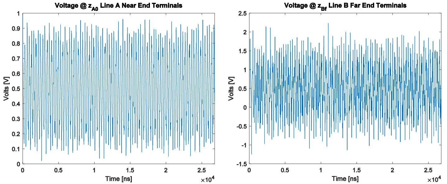
Figure 6-12: Terminal Voltages a) v(z_{A_0}, t) b) v(z_{B_1}, t) ( F_{RA} = 1, F_{RB} = 10 )
