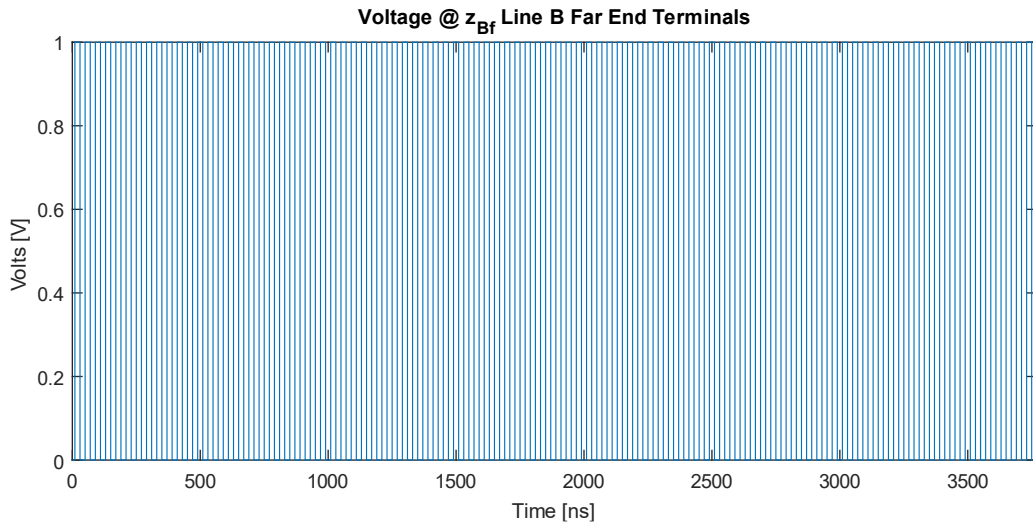
Figure 6-9: Line B Voltage at z_{B_f} terminals ( F_{RA} = 1, F_{RB} = 1 )
