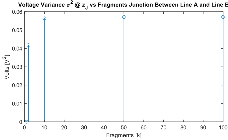
Figure 6-18: Junction Voltage Variance Var(v(z_J, t)) ( F_{RA} = 1, F_{RB} = 1, 2, 10, 50, 100 )
