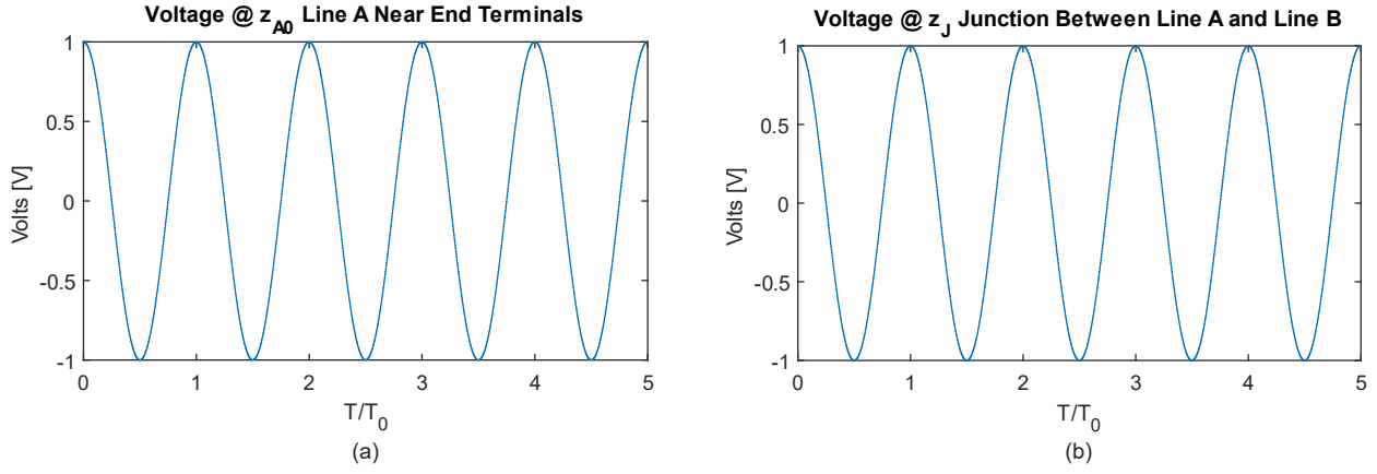
Figure 6-19: LC Resonator Terminal and Junction Voltages a) v_A(z_{A_0}, t) b) v_A(z_J, t)
