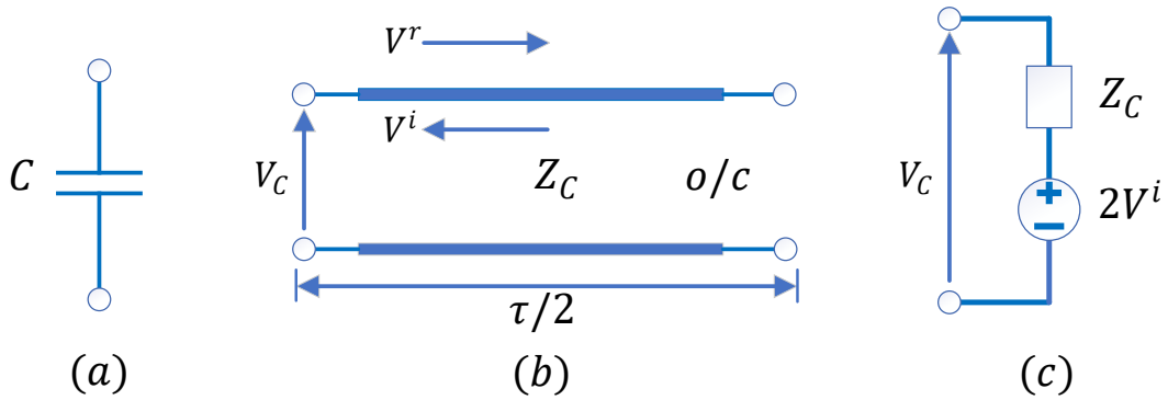
Figure 3-3: Capacitor Models a) Lumped Element b) TLM Stub c) Thevenin Equivalent Circuit
