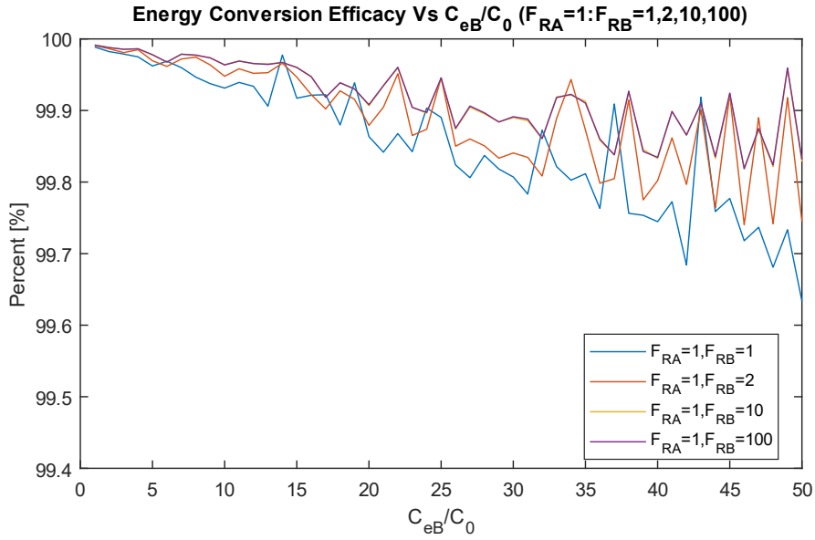
Figure 6-30: Energy Conversion Efficacy vs. Self-Capacitance (FFGIMD)
