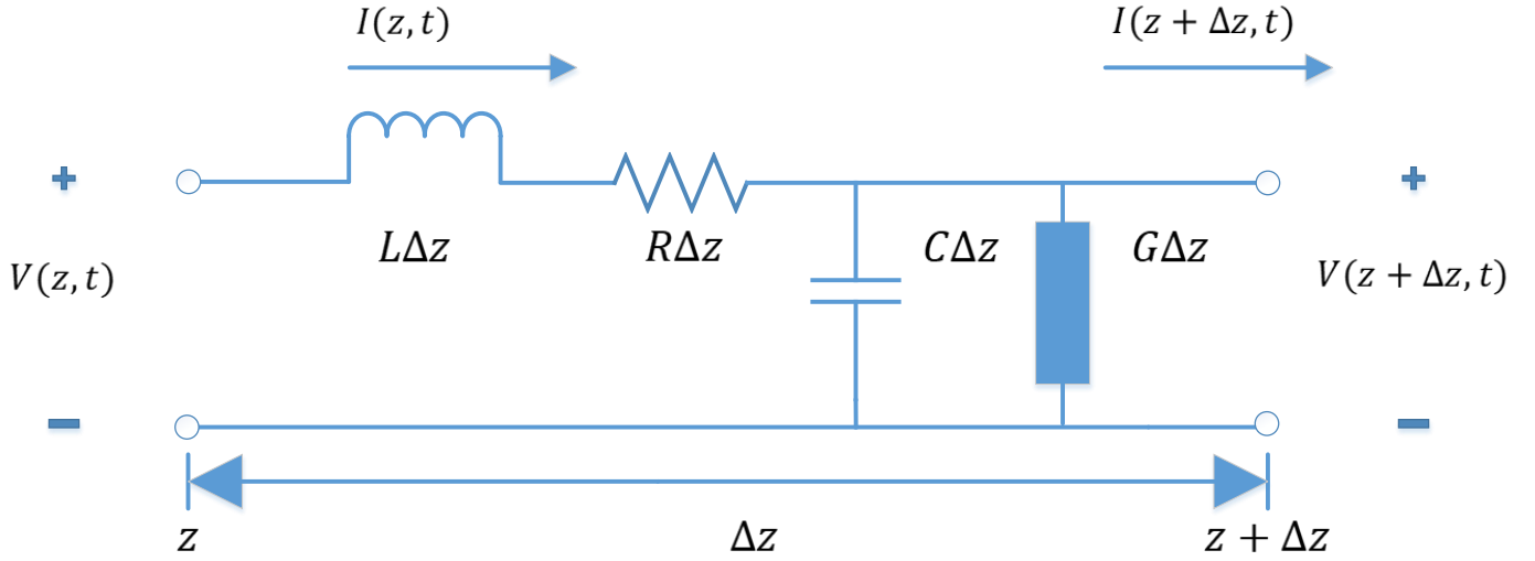
Figure 3-2: Per-Unit Length Distributed Parameter Segment
