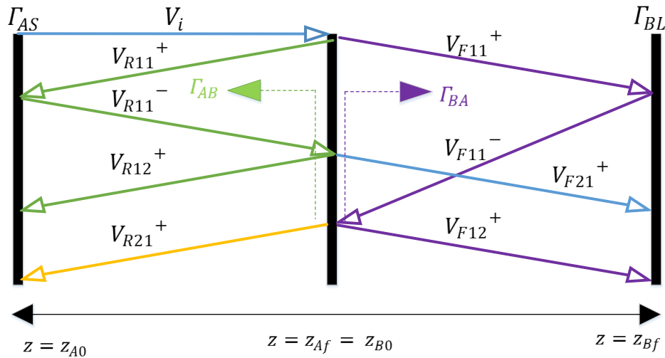
Figure 4-1: Fragmentation Bounce Diagram
