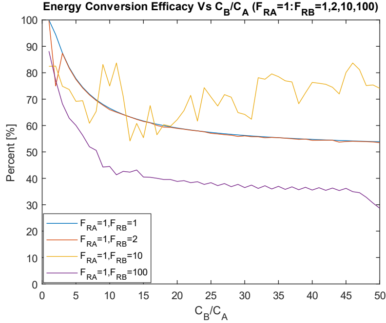
Figure 6-7: Energy Conversion Efficacy vs. Changing Capacitance (FFGIMD)
