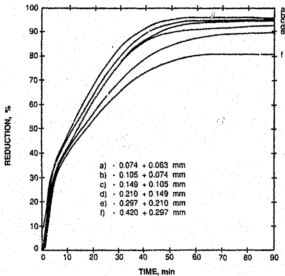
Figure 4.7 The effect of particle size on the reduction of the Mamatwan manganese ore at 1350 °C.
