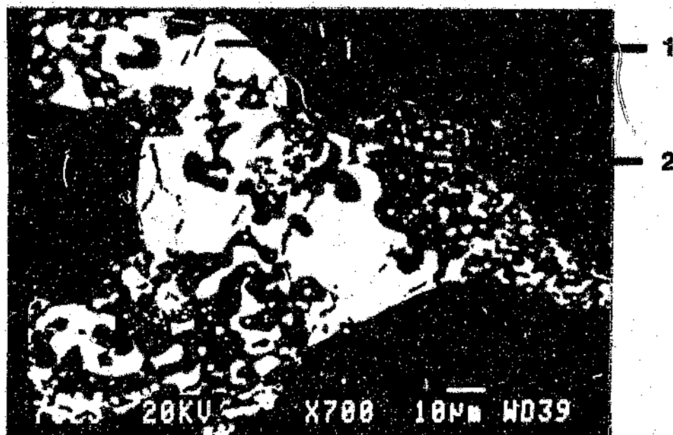
Figure 4.22 A Mamatwan manganese ore grain subjected to 82.45 percent reduction for 90 minutes at 1300 °C. Mag. 700X
