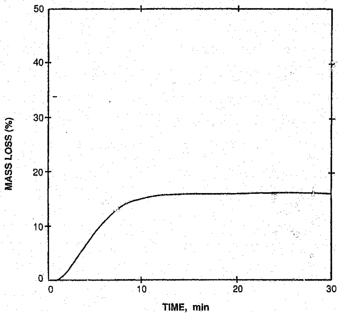
Figure 4.1 The effect of preheating on the Mamatwan manganese ore at 1000 °C.
