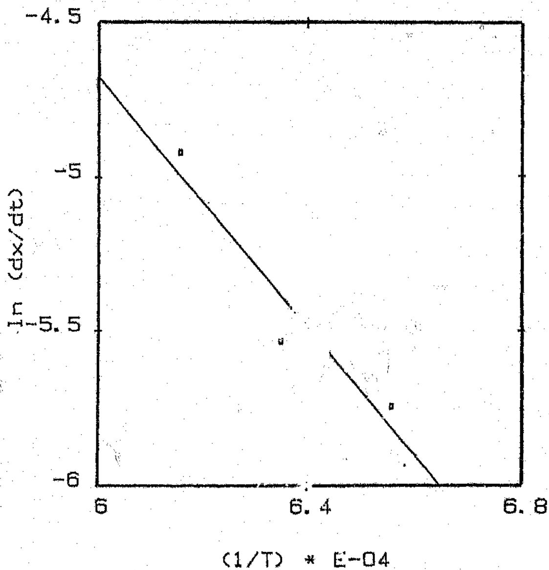
Figure 5.4 Arrhenius plot of the second stage kinetic data.
