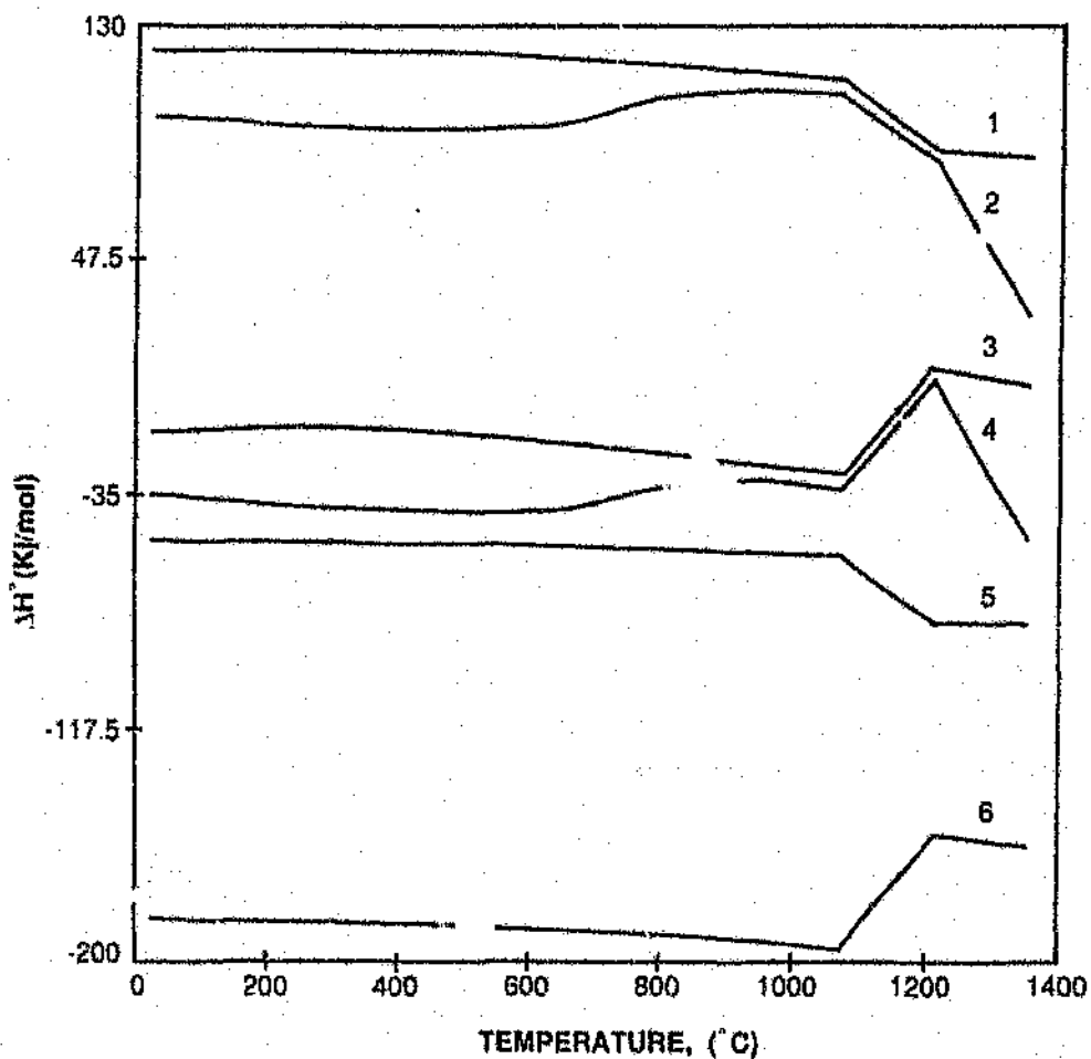
Figure 2.16 Enthalpy change as a function temperature for some \text{Mn}_2\text{O}_3 and \text{Mn}_3\text{O}_4 reduction reactions.
