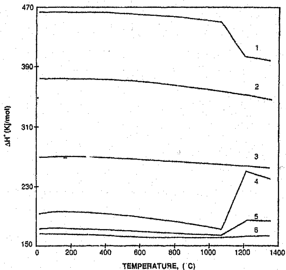
Figure 2.18 Entalphy change as a function temperature for some manganese oxides dissociation reactions.
