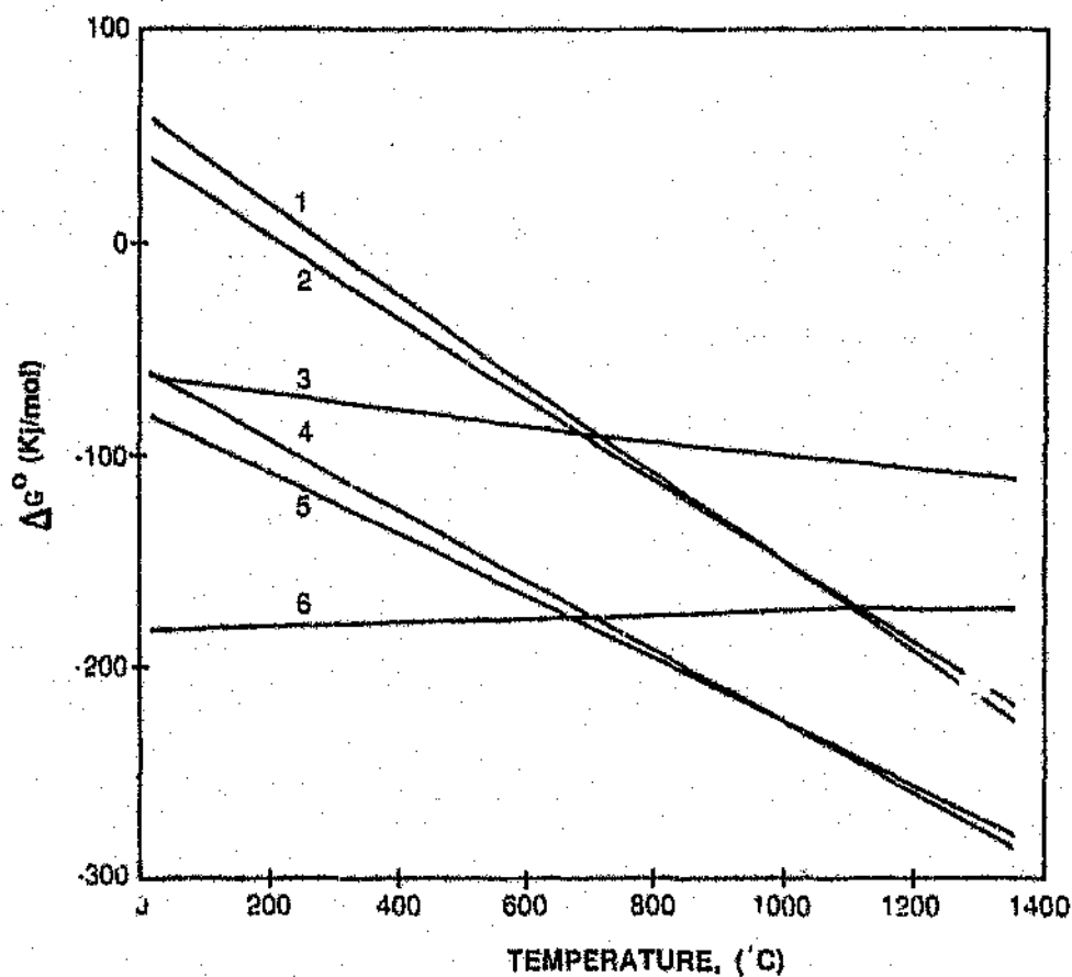
Figure 2.15 Free energy change as a function temperature for some \text{Mn}_2\text{O}_3 and \text{Mn}_3\text{O}_4 reduction reactions.
