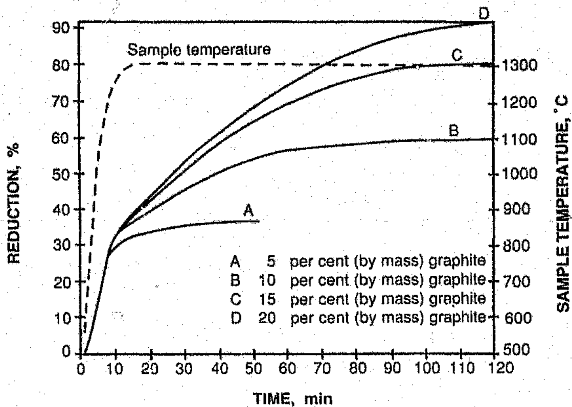
Figure 2.8 The effect of carbon amount on the reduction of Mamatwan manganese ore by graphite (after Grimsley, 1980).
