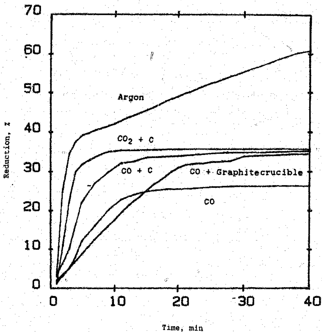
Figure 4.12 Reduction of the Mamatwan manganese ore under CO and CO 2 atmospheres at 1300 °C.
