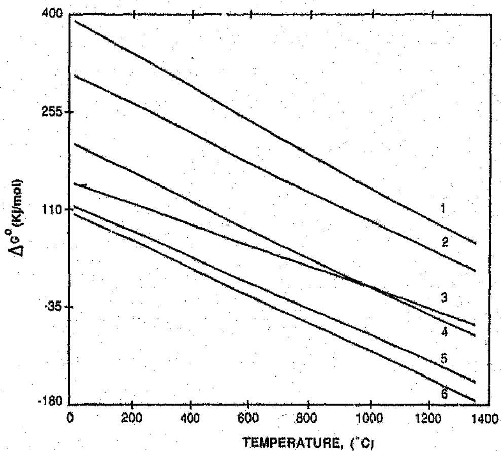
Figure 2.17 Free energy change as a function temperature for some manganese oxides dissociation reactions.
