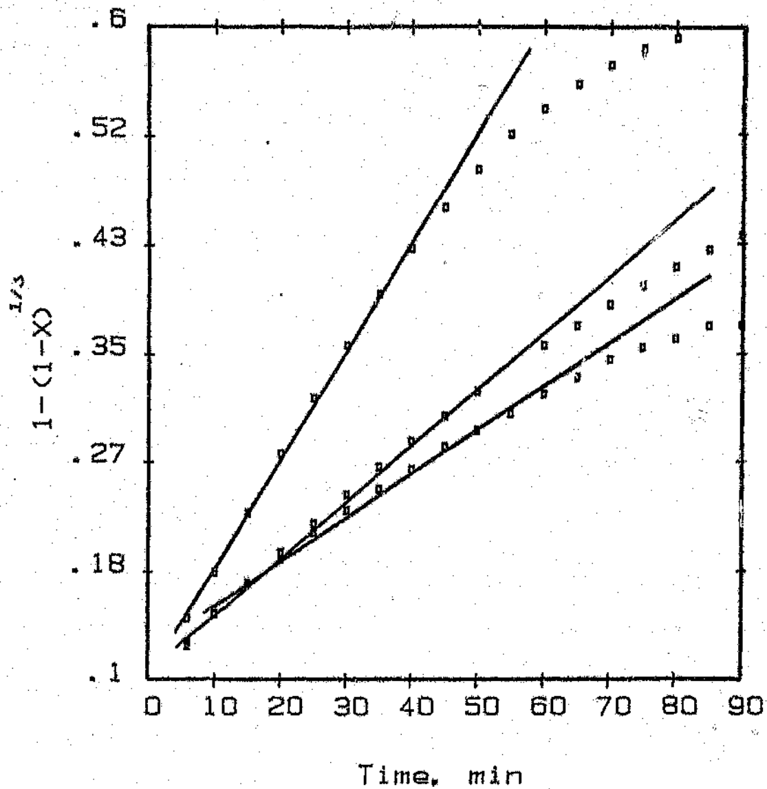
Figure 5.2 Application of kinetic data to Equation 5.9 after first stage of the reduction.
