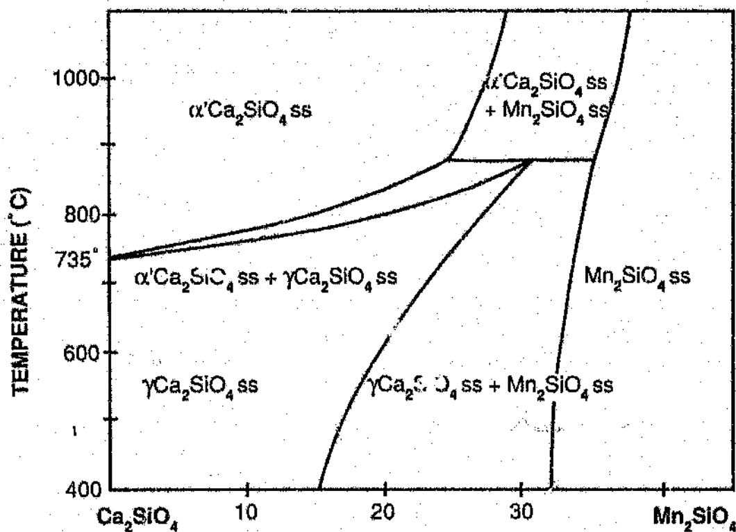
Figure 2.20 Phase relations in the system CaO-MnO-SiO 2 below 1000°C. (after Glosser, 1962).
