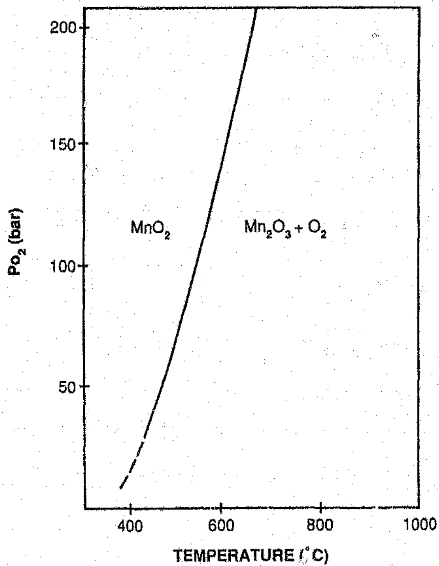
Figure 2.9 System Mn-O; univariant equilibrium curve between \text{MnO}_2 and \text{Mn}_2\text{O}_3 (after Klingsberg, 1960).
