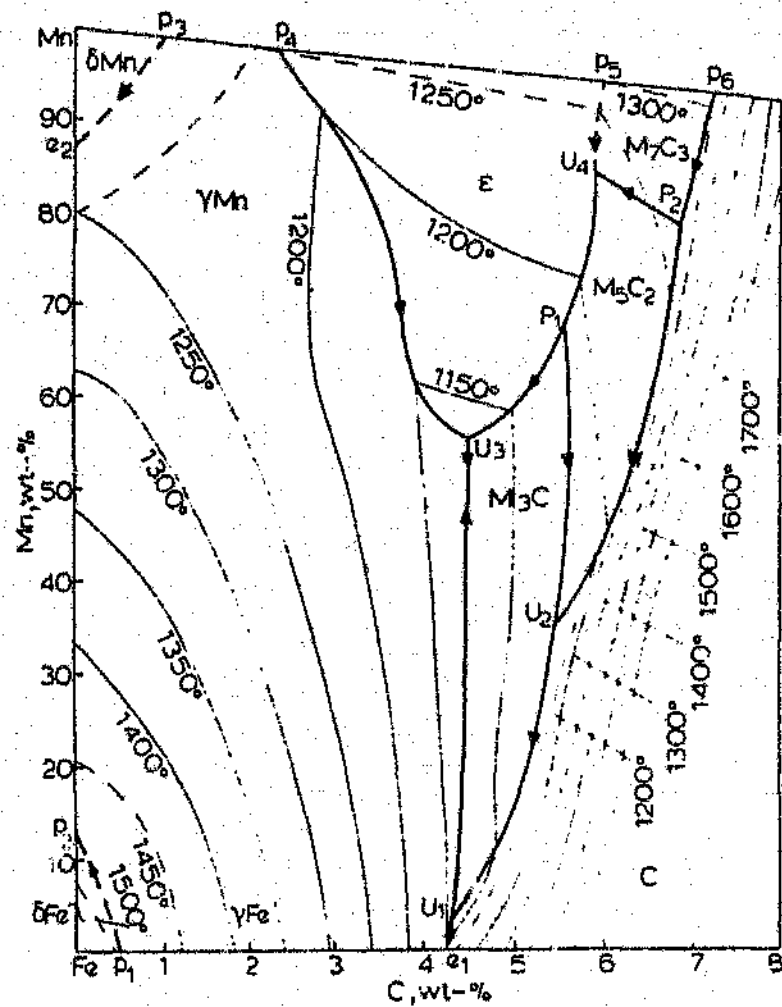
Figure 2.24 Liquidus projection of C-Fe-Mn system. (after Schurmann, 1977; Schenck and et al, 1963; Chipman, 1952).
