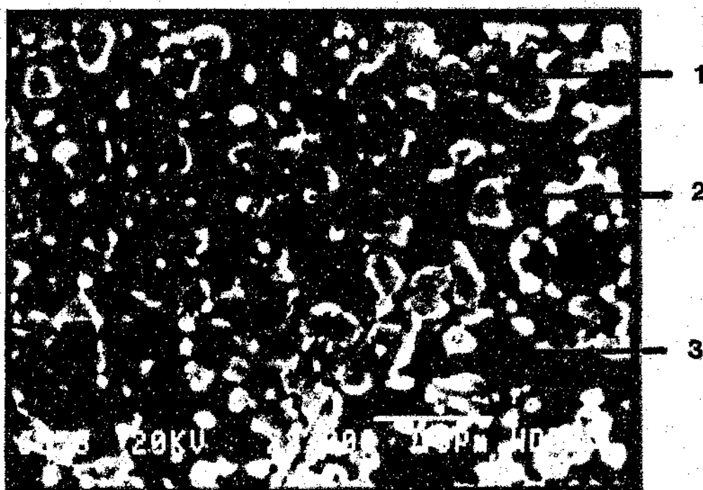
Figure 4.14 A Mamatwan manganese ore grain subjected to 38.14 percent reduction for 6 minutes at 1350 °C. Mag. 2000X
