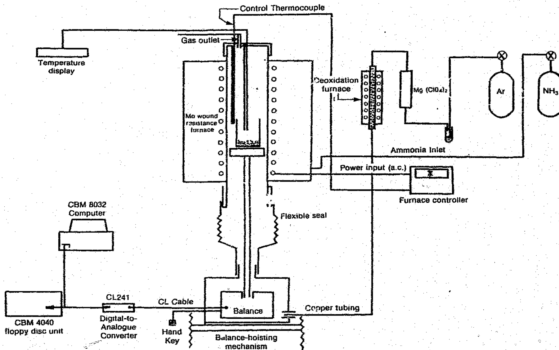
Figure 3.2 Schematic representation of experimental apparatus
