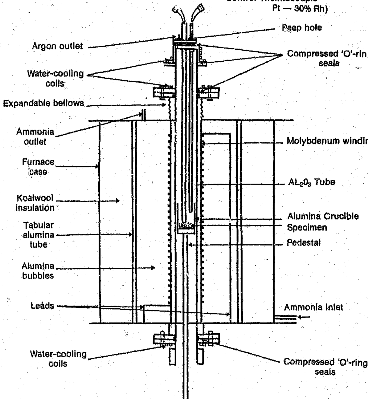
Figure 3.1 The vertical molybdenum-wound resistance furnace.
