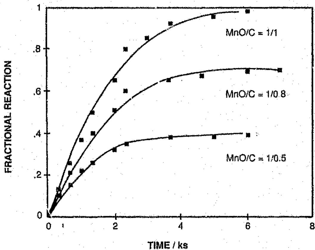
Figure 2.5 The effect of MnO-to-C ratio on the reduction of MnO by graphite (after Terayama, 1985).
