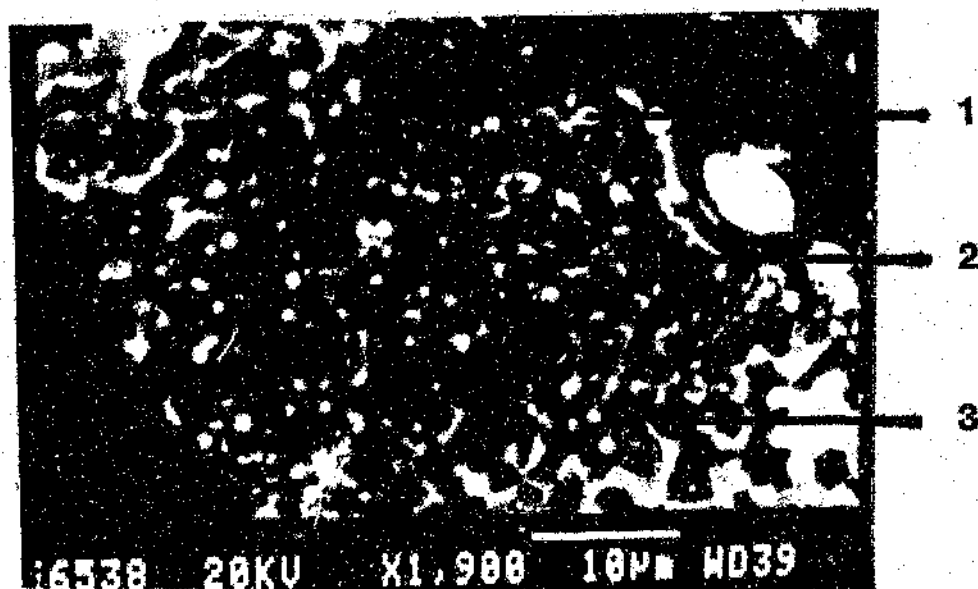
Figure 4.15 A Mamatwan manganese ore grain subjected to 45.54 percent reduction for 10 minutes at 1350 °C. Mag. 1900X
