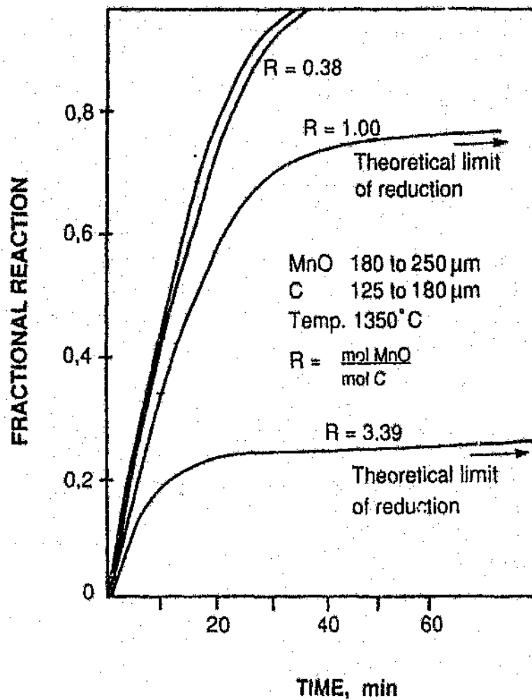
Figure 2.1 The effect of MnO-to-C ratio on the reduction of MnO by carbon (after Rankin, 1987)
