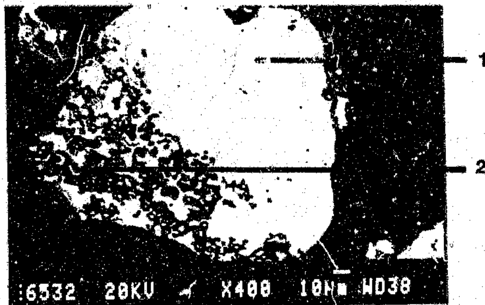
Figure 4.19 A Mamatwan manganese ore grain subjected to 92.15 percent reduction for 70 minutes at 1350 °C. Mag. 400X
