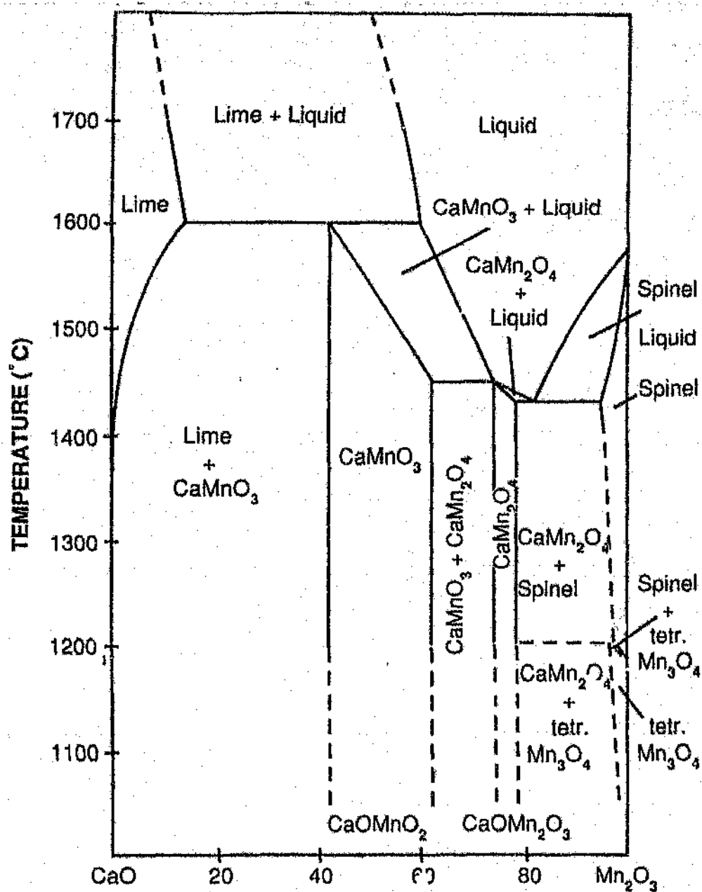
Figure 2.19 Phase relations in the system CaO-manganese oxide above 1100°C. (after Ribound and et al, 1963).
