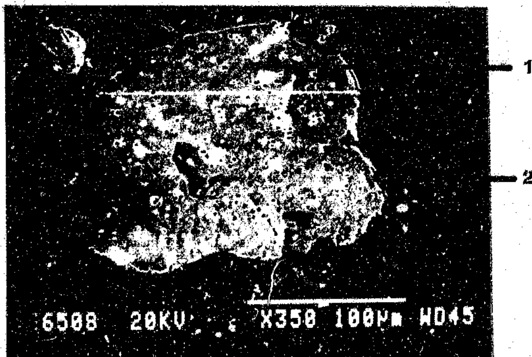
Figure 4.20 A Mamatwan manganese ore grain subjected to 94.01 percent reduction for 90 minutes at 1350 °C. Mag. 350X.
