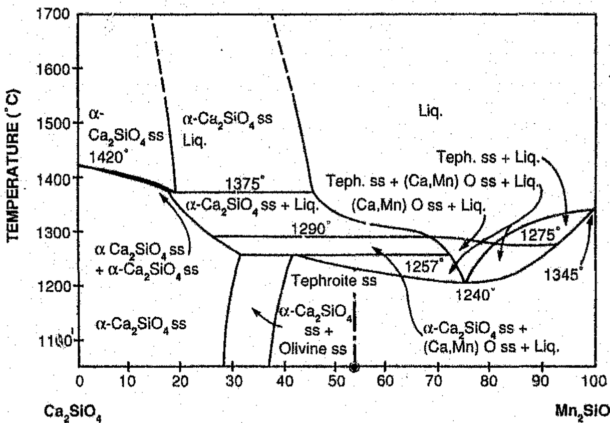
Figure 2.21 Phase relations in the system \text{CaO-MnO-SiO}_2 above 1000^\circ\text{C} . (after Glosser, 1962).
