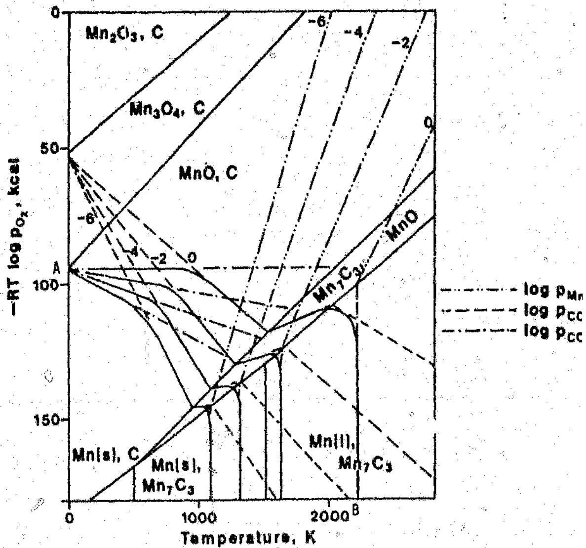
Figure 2.25 Pourbaix diagram for the Mn-O-C system. (after Downing, 1963).
