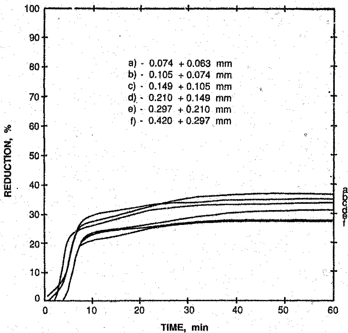
Figure 4.4 The effect of particle size on the reduction of the Mamatwan manganese ore at 1100 °C.
