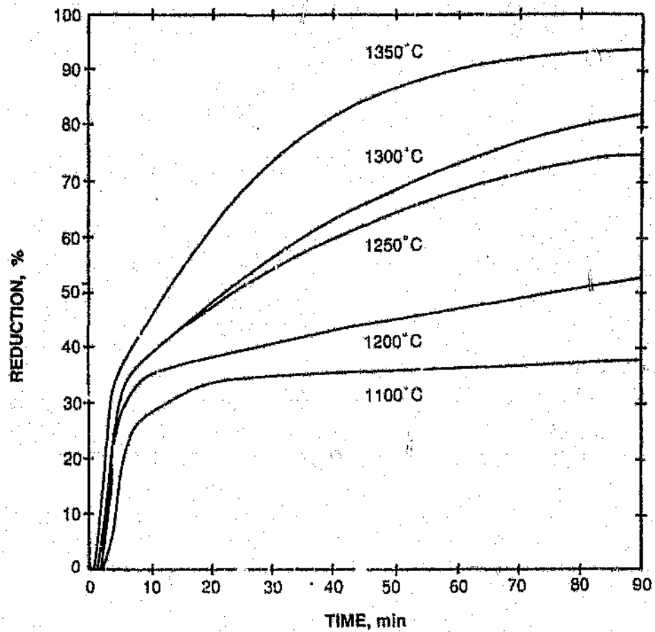
Figure 4.2 The effect of temperature on the reduction of the Maratwan manganese ore. (The ore is -0.42 mm).
