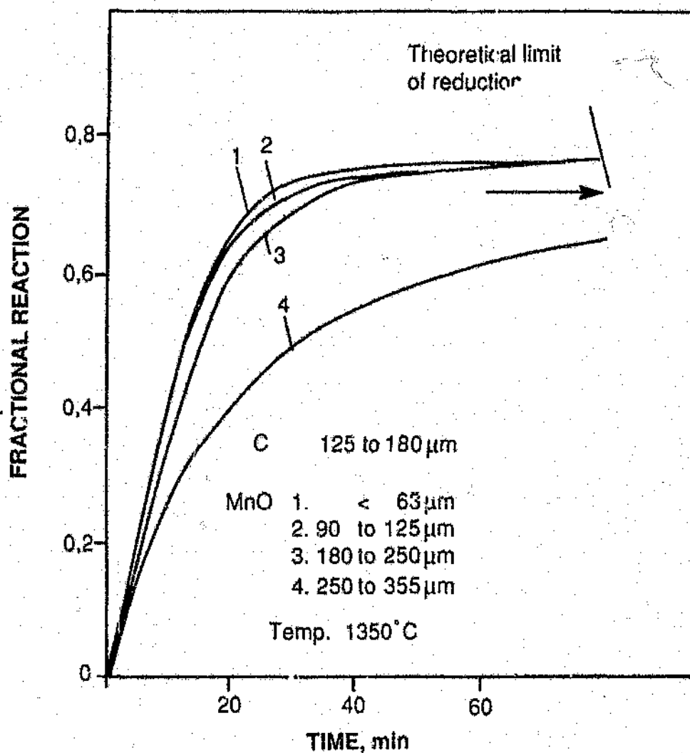
Figure 2.3 The effect of particle size of MnO on the reduction of MnO by graphite (after Rankin, 1980).
