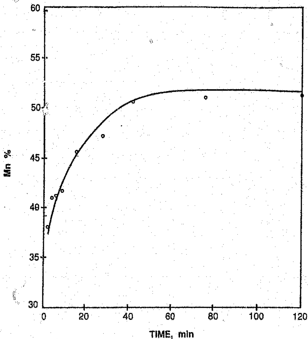
Figure 4.31 Manganese content variation of the reaction mixture during the reduction at 1350 °C.
