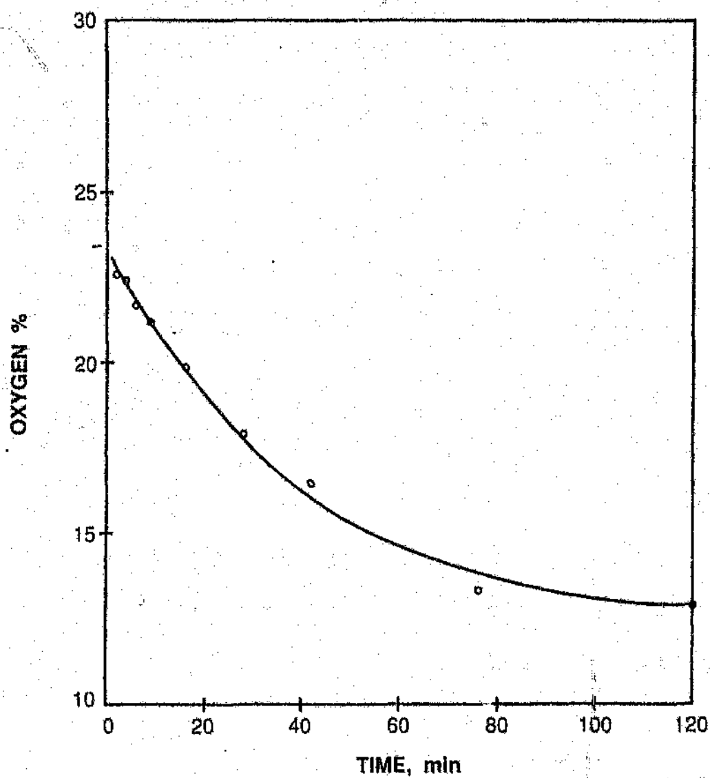
Figure 4.30 Oxygen content variation of the reaction mixture during the reduction at 1350 °C.
