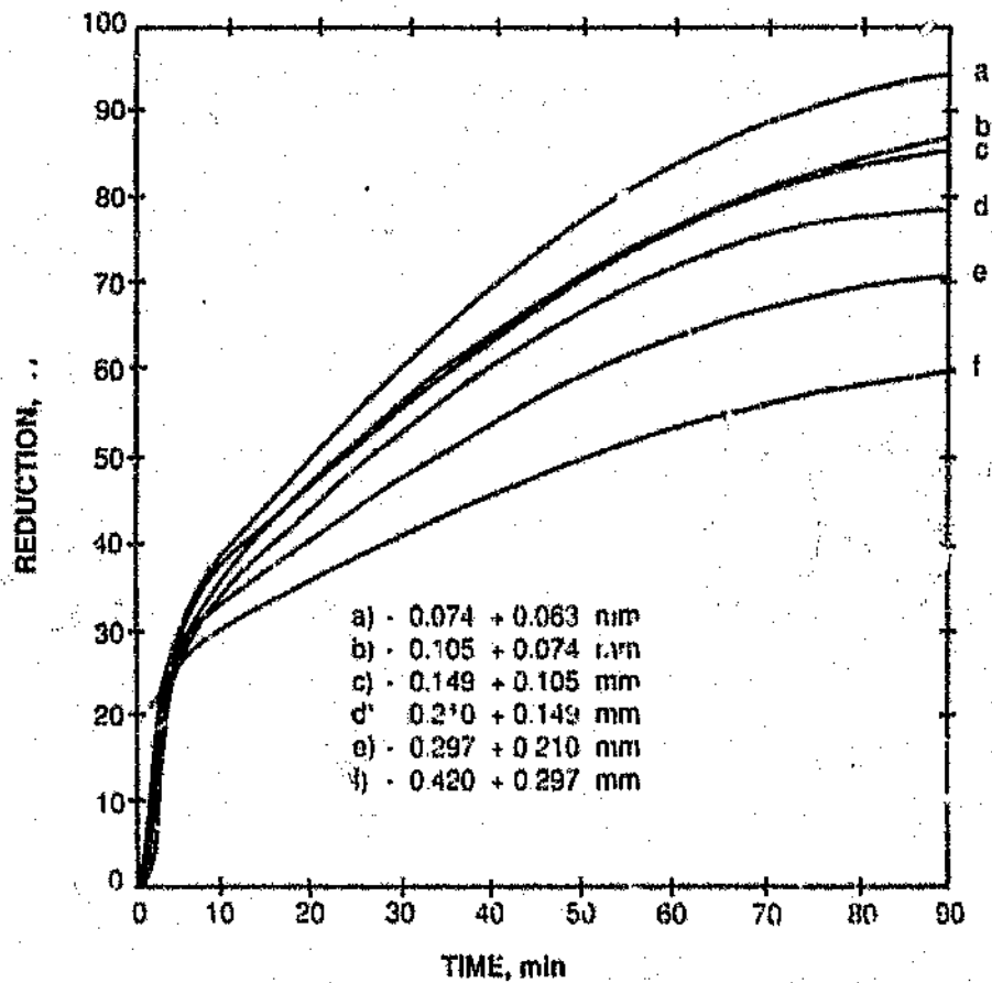
Figure 4.6 The effect of particle size on the reduction of the Mamatwan manganese ore at 1300 °C.
