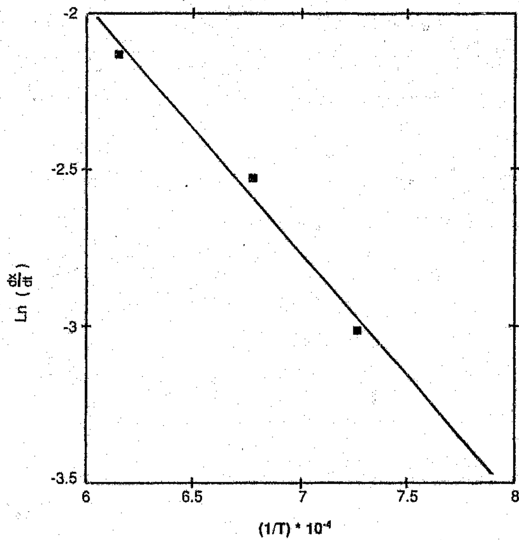
Figure 5.1 Arrhenius plot of the first stage kinetic data.
