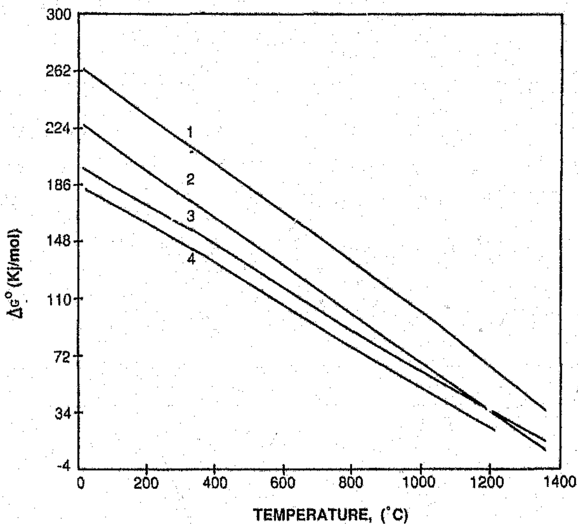
Figure 2.13 Free energy change as a function temperature for some MnO reduction reactions.
