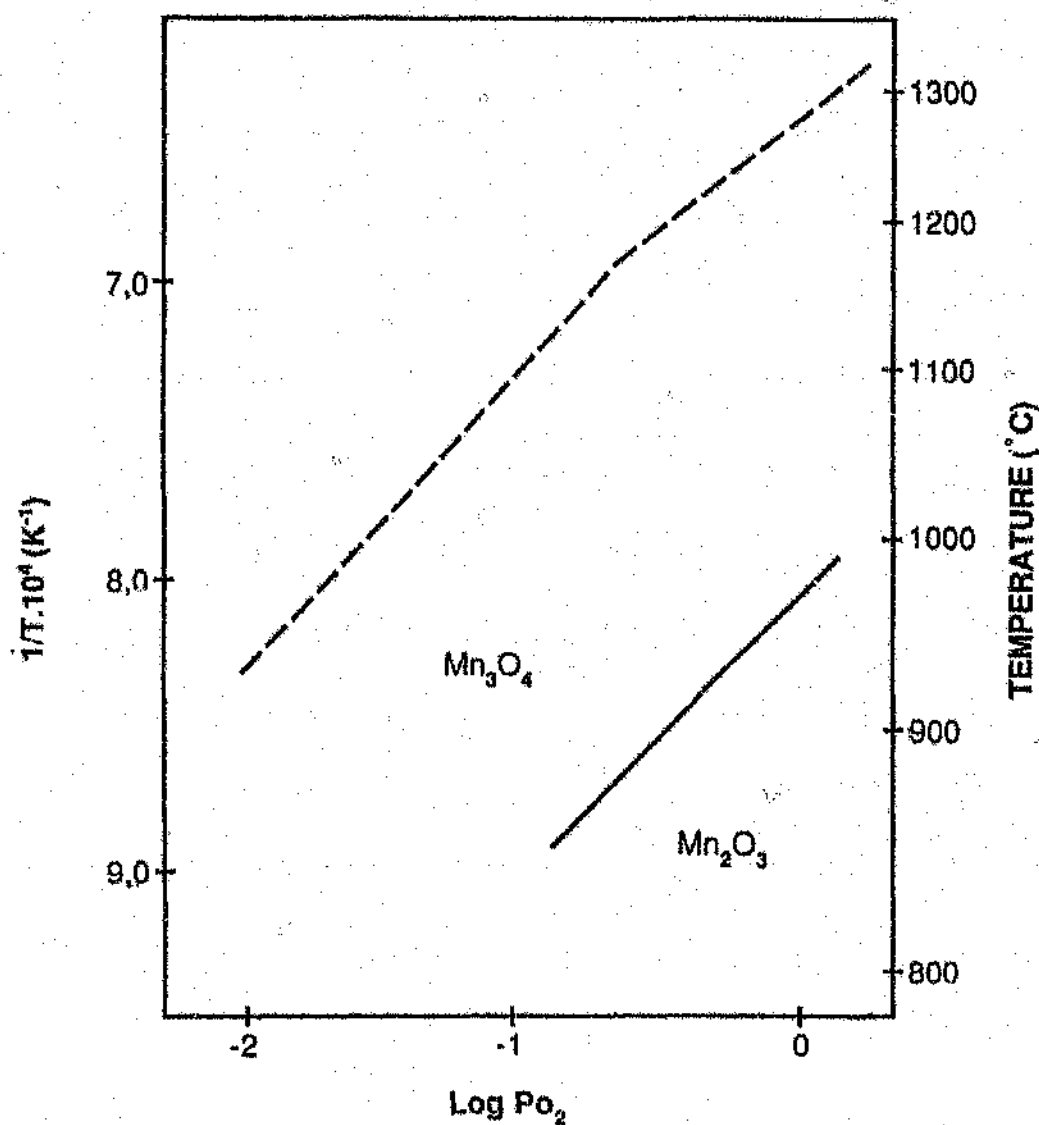
Figure 2.11 System \text{Mn}_2\text{O}_3 - \text{Mn}_3\text{O}_4 as a function of oxygen pressure and temperature (after Hahn and et al, 1960).
