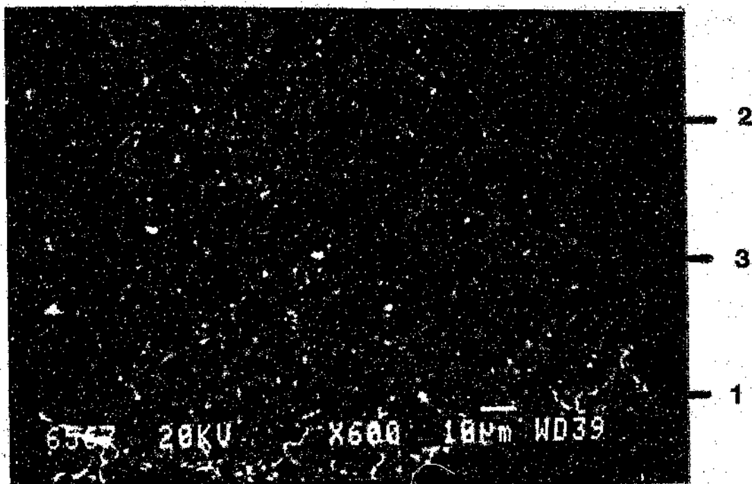
Figure 4.13 A Mamatwan manganese ore grain subjected to 26.64 percent reduction for 3 minutes at 1350 °C. Mag. 600X
