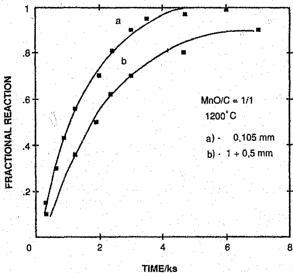
Figure 2.6 The effect of particle size of MnO on the reduction of MnO by graphite (after Teramachi, 1985).
