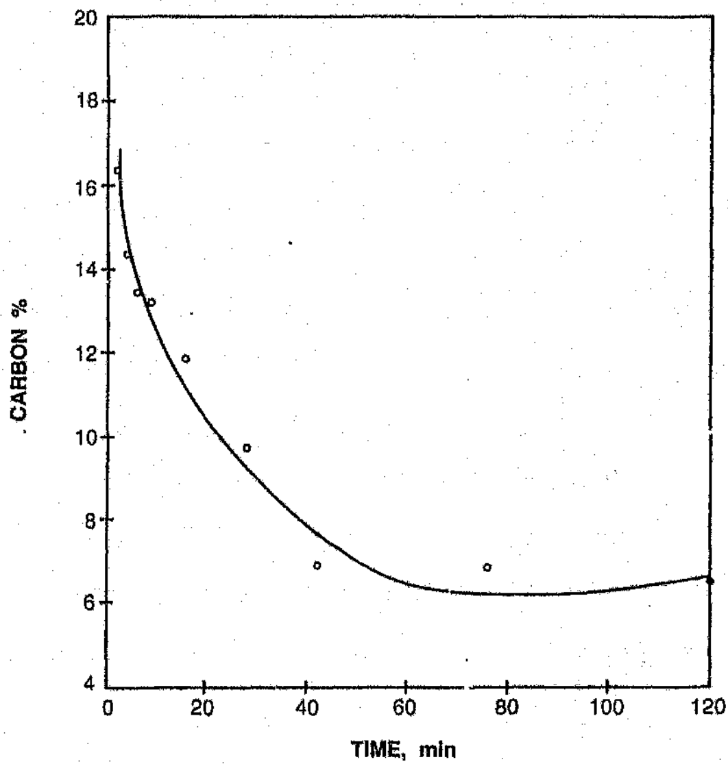
Figure 4.29 Carbon content variation of the reaction mixture during the reduction at 1350 °C.
