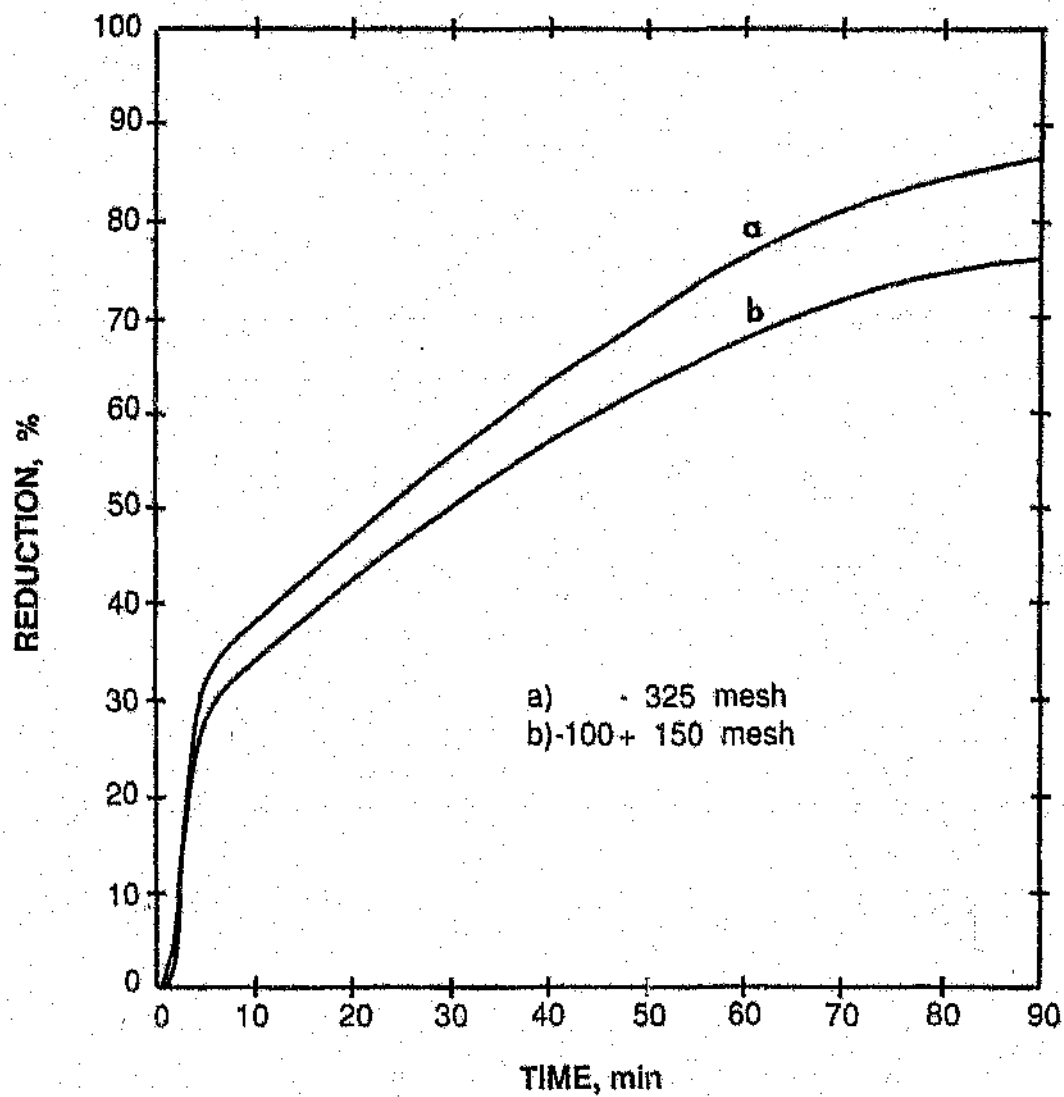
Figure 4.10 The effect of carbon particle size on the reduction of the Mamatwan manganese ore at 1300 °C.
