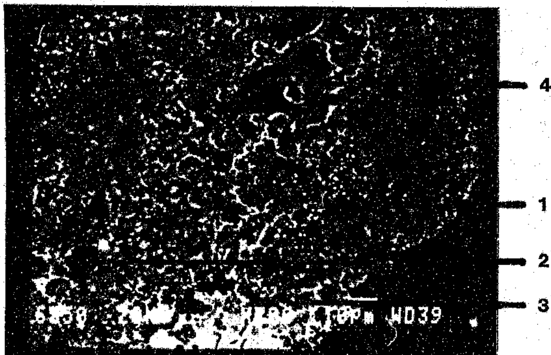
Figure 4.24 A Mamatwan manganese ore grain subjected to 37.81 percent reduction for 90 minutes at 1100 °C. Mag. 700X
