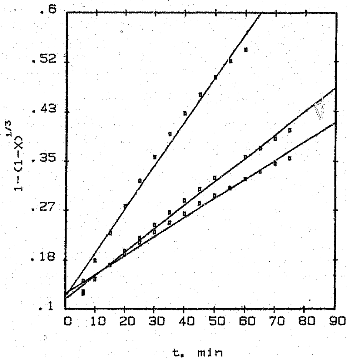
Figure 5.3 Regression analysis of the second stage kinetic data.
