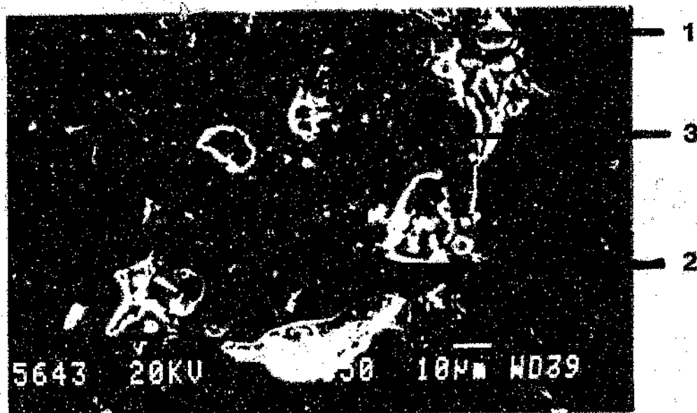
Figure 4.17 A Mawatwan manganese ore grain subjected to 78.03 percent reduction for 35 minutes at 1350 °C. Mag. 650X
