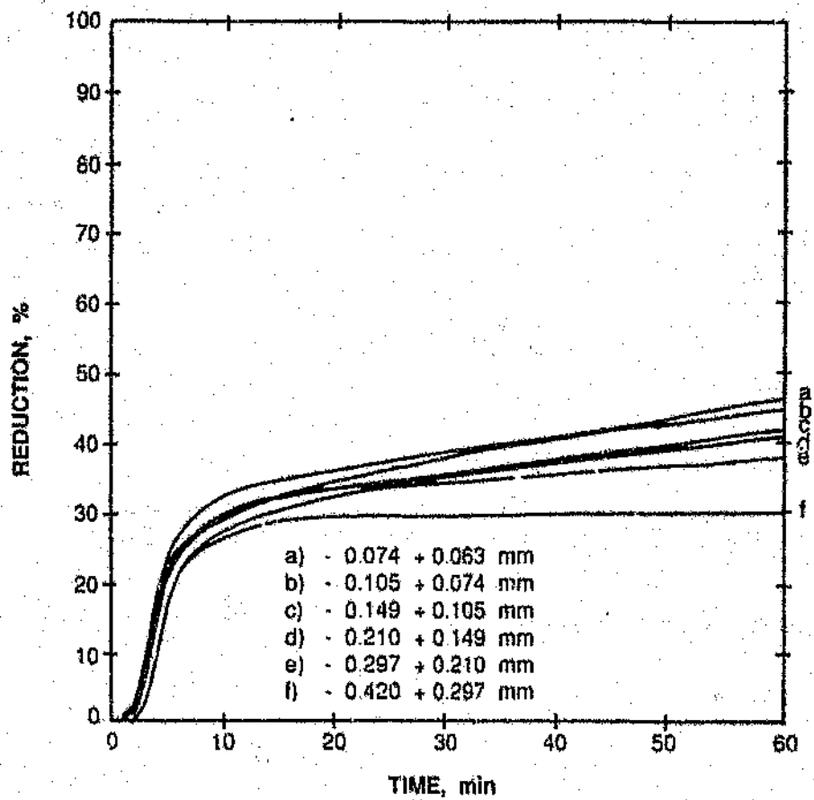
Figure 4.5 The effect of particle size on the reduction of the Mamatwan manganese ore at 1200 °C.
