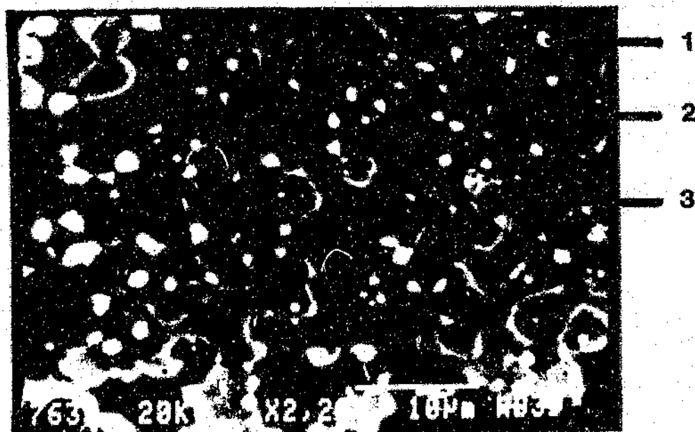
Figure 4.23 A Mamatwan manganese ore grain subjected to 53.09 percent reduction for 90 minutes at 1200 °C. Mag. 2200X
