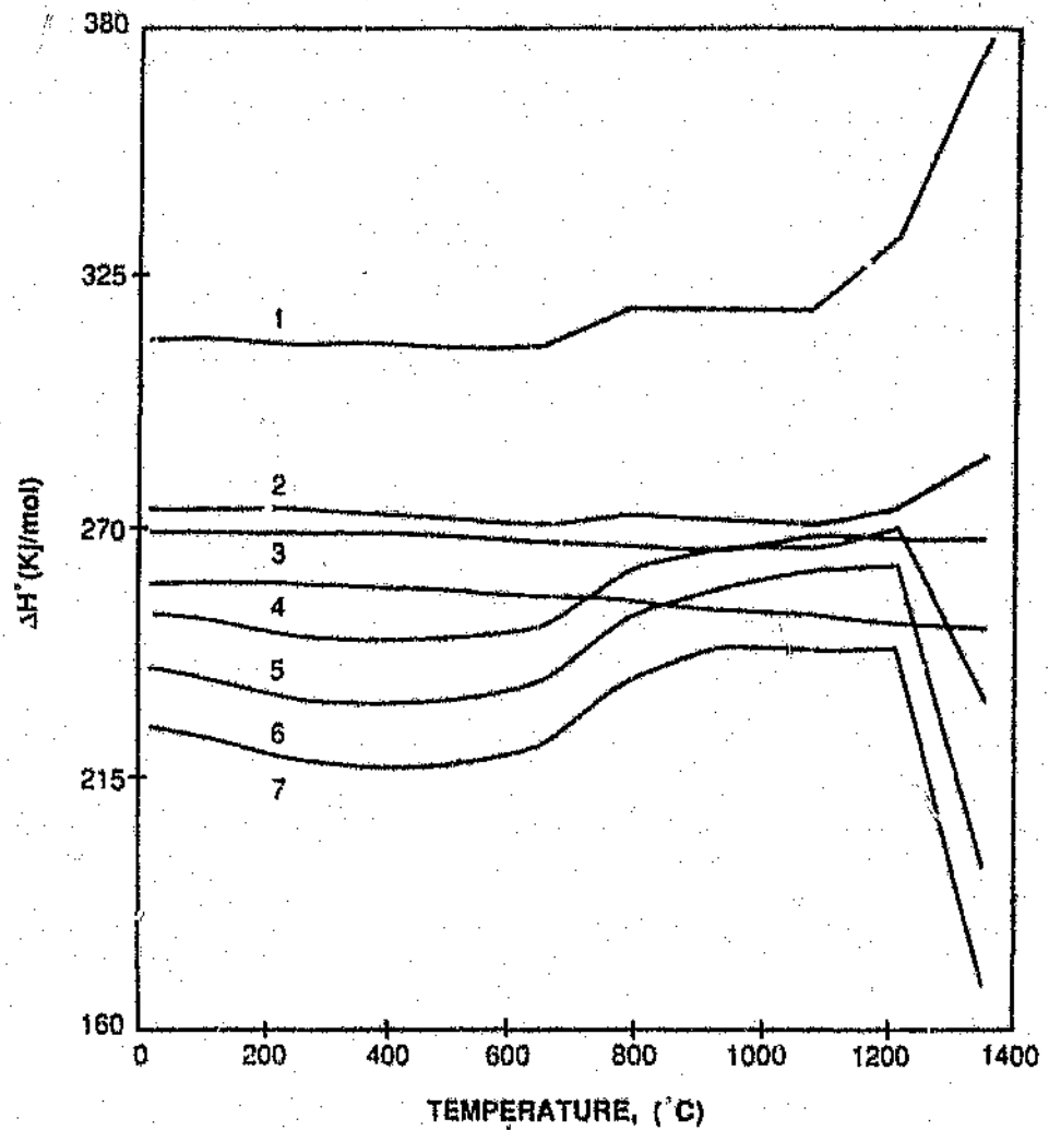
Figure 2.14 Enthalpy change as a function temperature for some MnO reduction reactions.
