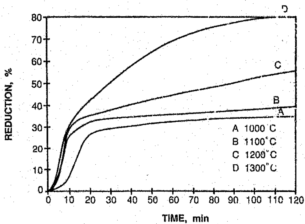
Figure 2.7 The effect of temperature on the reduction of Mamatwan manganese ore by graphite (after Grimsley, 1977).
