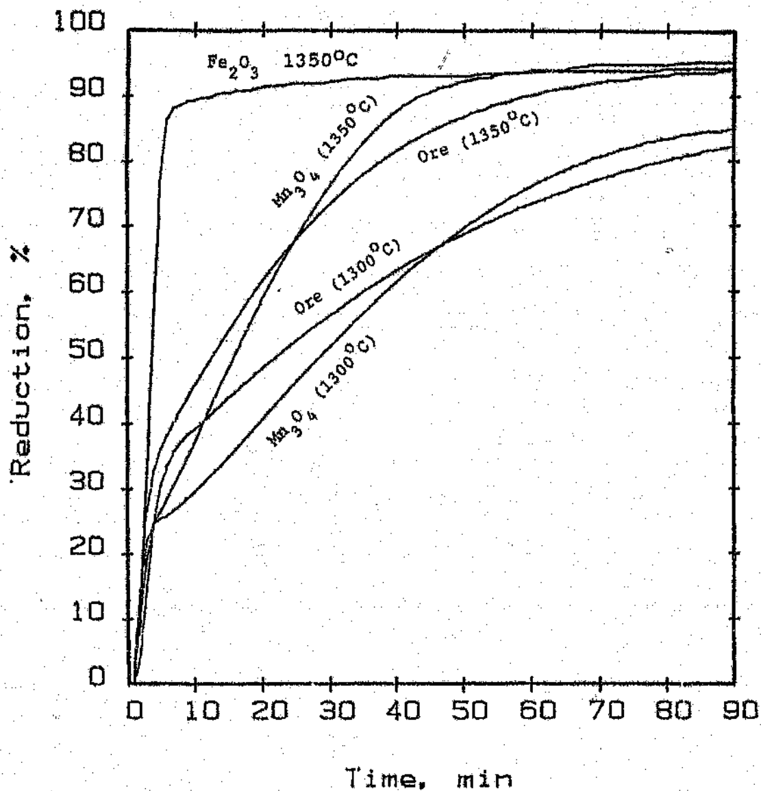
Figure 4.11 The effect of temperature on the reduction of pure \text{Mn}_3\text{O}_4 and \text{Fe}_2\text{O}_3 .
