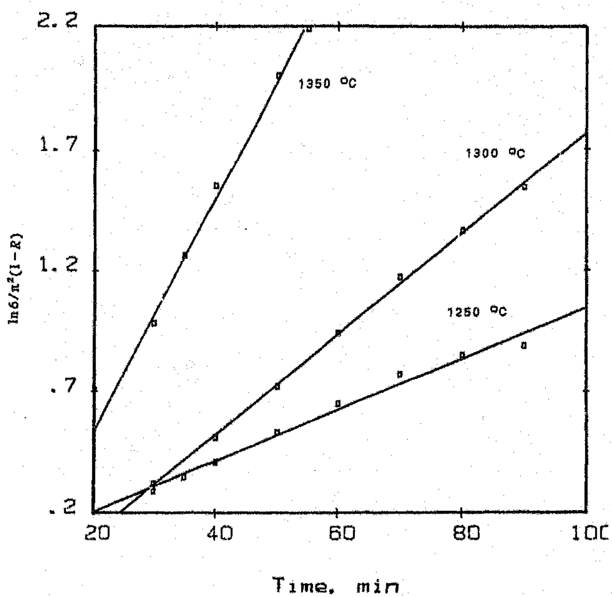
Figure 5.5 Application of equation 5.8 to the third stage kinetic data.
