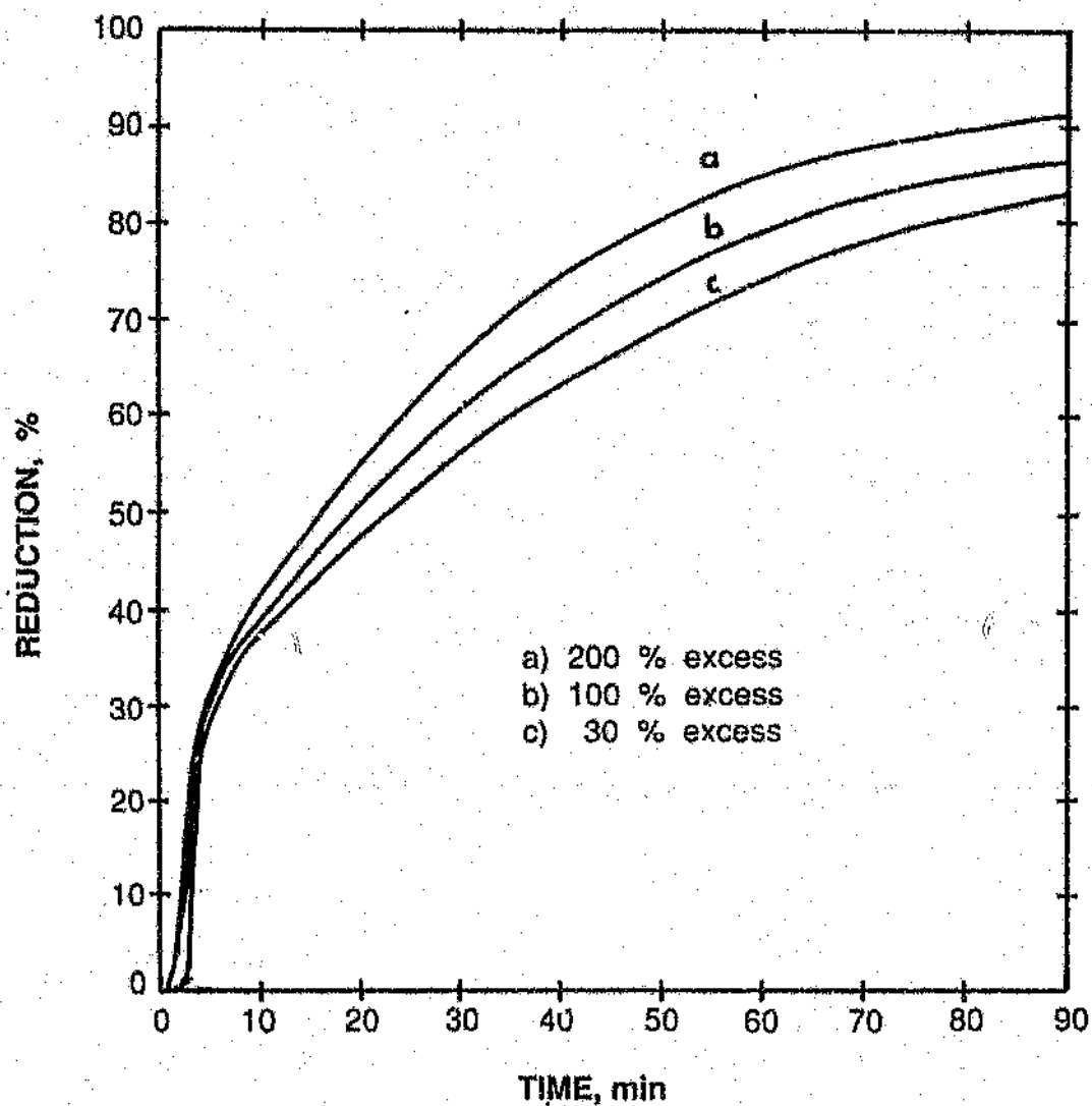
Figure 4.9 The effect of carbon amount on the reduction of the Mamatwan manganese ore at 1300 °C.
