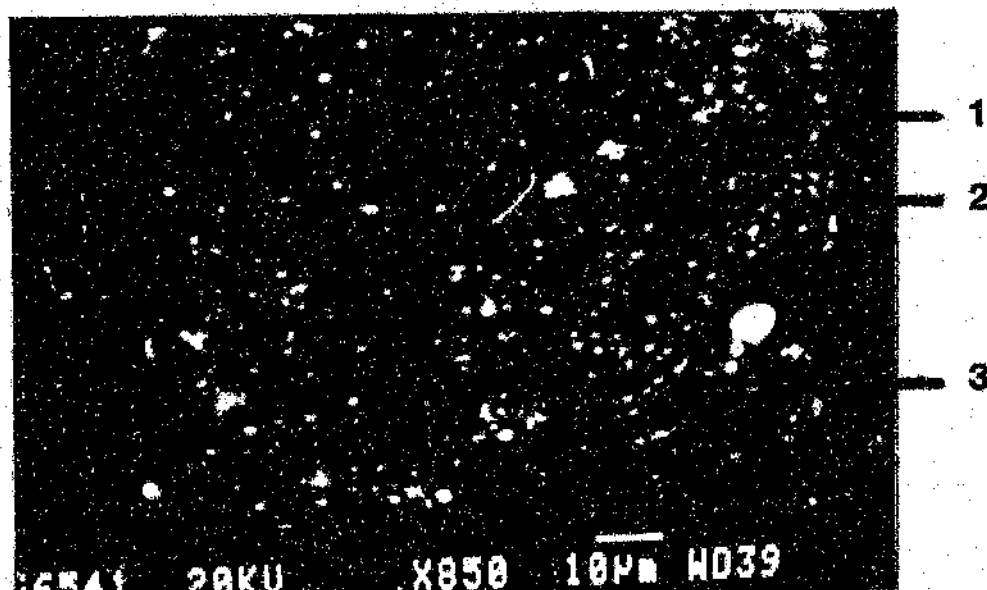
Figure 4.16 A Mamatwan manganese ore grain subjected to 68.09 percent reduction for 25 minutes at 1350 °C. Mag. 850X
