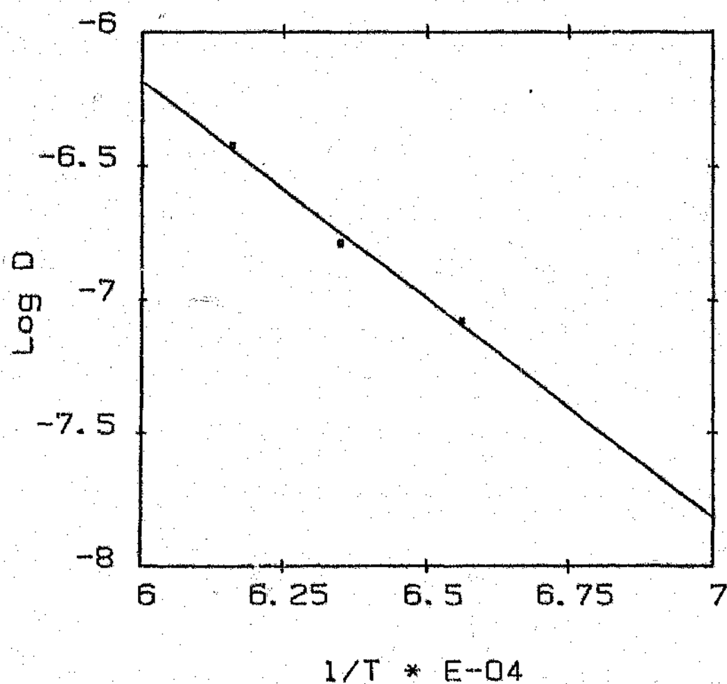
Figure 5.6 Arrhenius plot of the third stage kinetic data.
