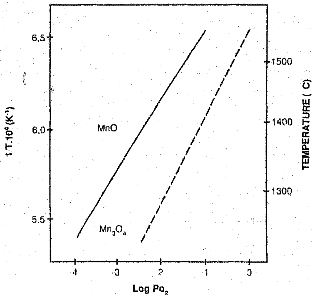
Figure 2.12 System MnO-Mn 3 O 4 as a function of oxygen pressure and temperature (after Hahn and et al, 1960).
