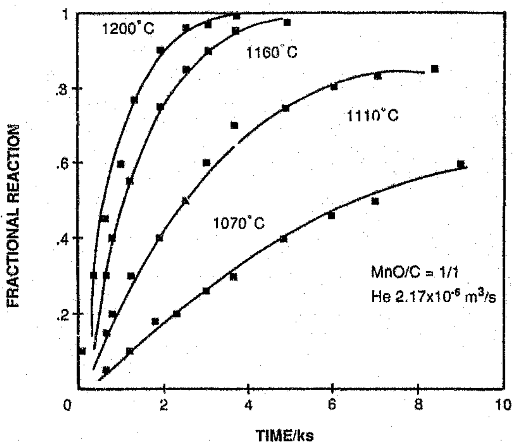
Figure 2.4 The effect of temperature on the reduction of MnO by graphite (after Terayama, 1985).
