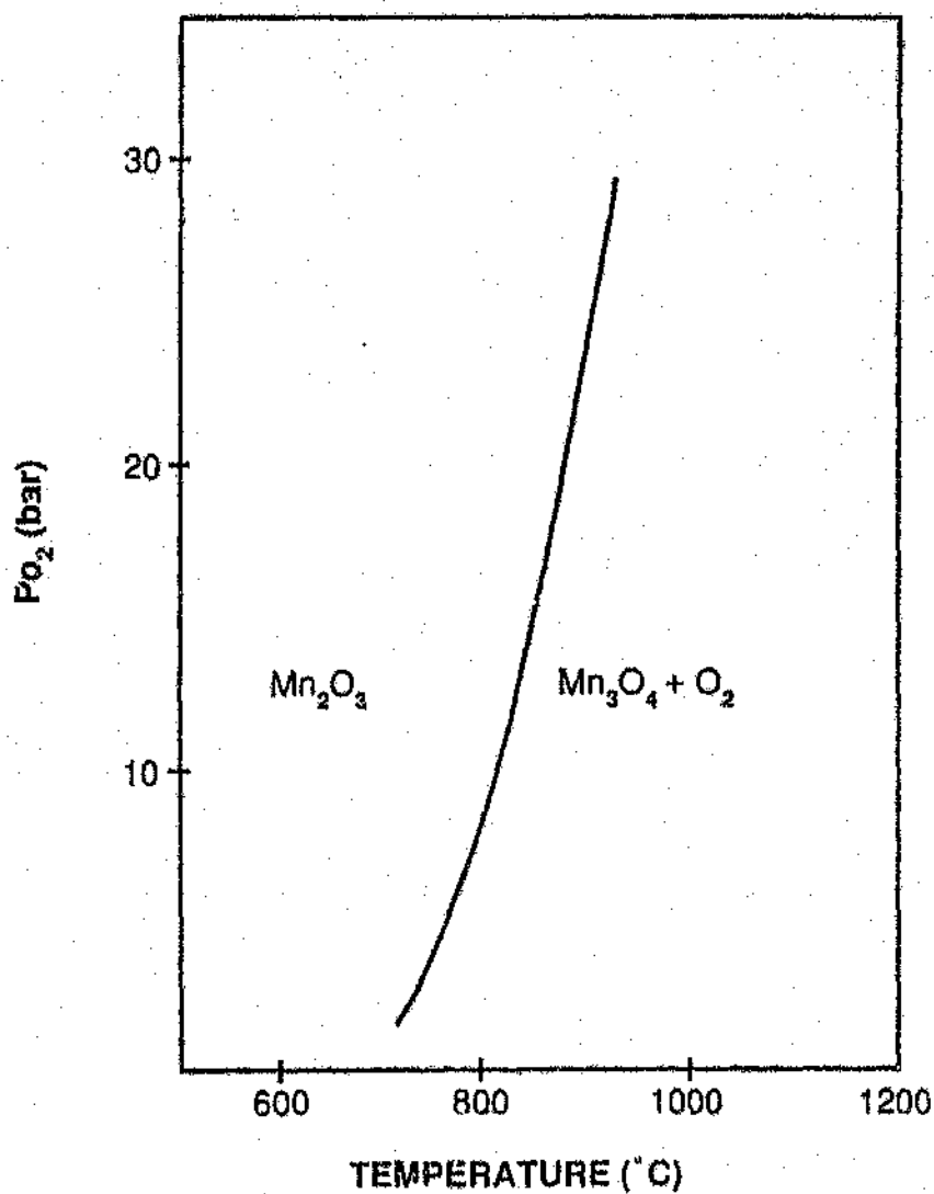
Figure 2.10 System Mn-O; univariant equilibrium curve between \text{Mn}_2\text{O}_3 and \text{Mn}_3\text{O}_4 (after Klingsberg, 1960).
