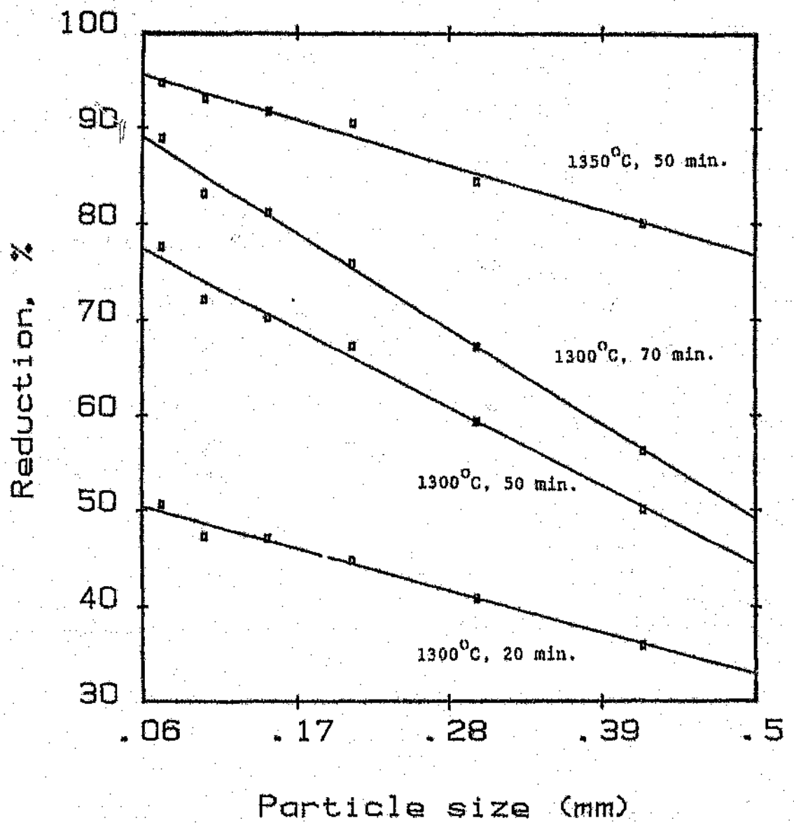
Figure 4.8 The effect of particle size on the reduction of the Mamatwan manganese ore after 20, 50, 70 minutes retention times at 1300°C and 1350°C.
