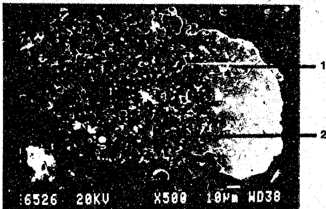
Figure 4.18 A Mamatwan manganese ore grain subjected to 86.83 percent reduction for 50 minutes at 1350 °C. Mag. 500X
