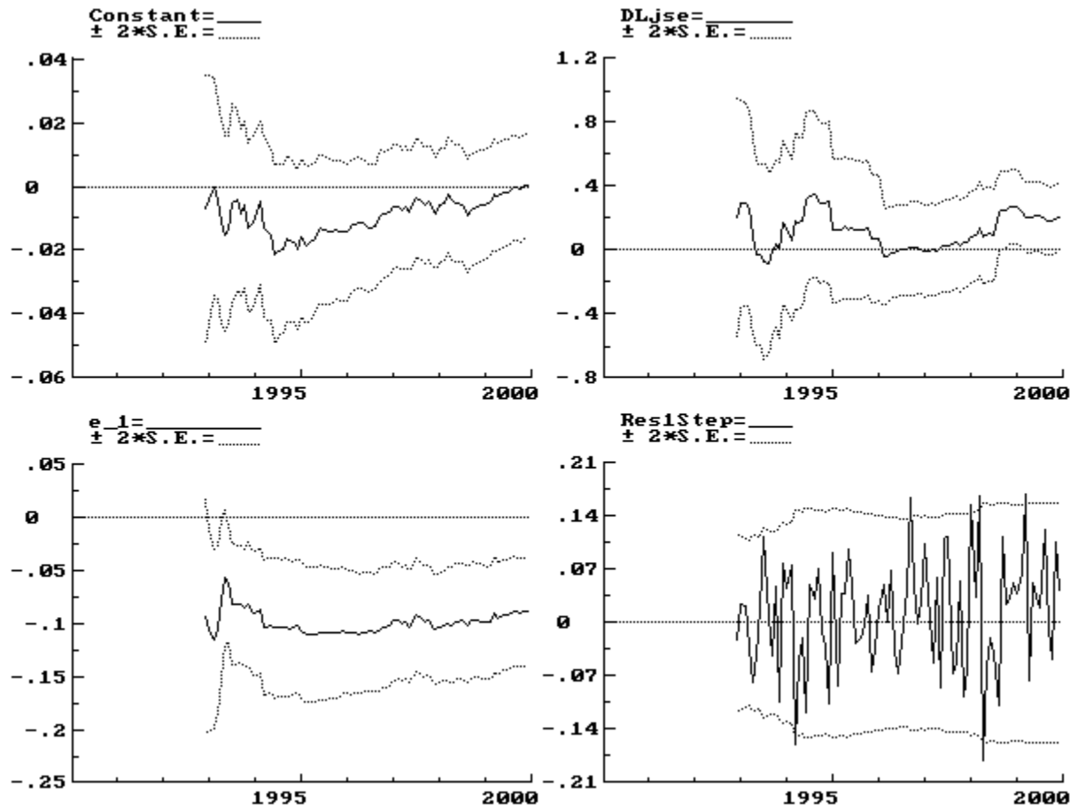
Figure 3: RECURSIVE GRAPHICS
