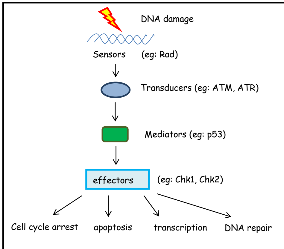
Figure 1.3: An outline of the DNA damage response signal-transduction pathway. This pathway consists of sensors, transducers, mediators and effectors. (Adapted from Zhou & Elledge, 2000).
