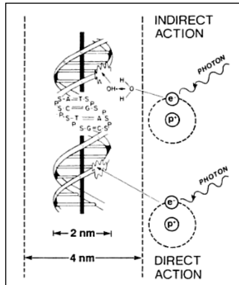
Figure 1.2: The two types of radiation damage on DNA: Direct action - direct damage to the biologic macromolecule; and Indirect action - damage to the biologic macromolecule through the ionisation of water (Hall & Giaccia, 2012).
