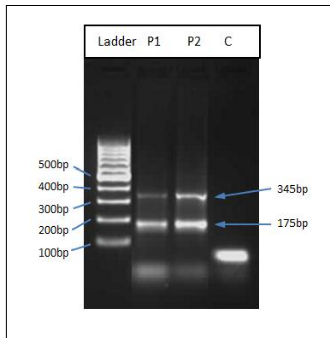
Figure 2.3: PCR showing centromeric sequenced products of 175 bp and 345 bp. P1 and P2 indicates the PCR products and C indicates the negative control. The bottom bands in all lanes indicate primer dimers.
