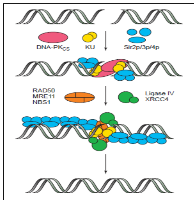
Figure 1.6: The process of NHEJ involves the use of various proteins to bind the two fragmented DNA strands together (Kanaar, Hoeijmakers & van Gent, 1998).
