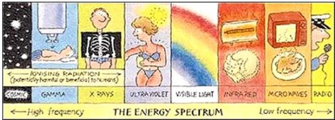
Figure 1.1: Examples of IR are gamma rays, X-rays and cosmic rays (World Health Organisation).
