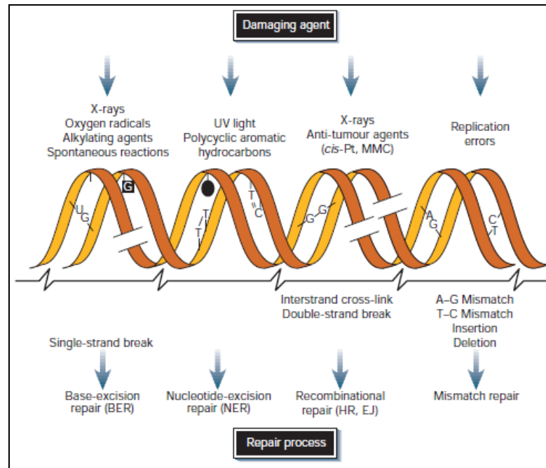
Figure 1.4: Different types of DNA repair mechanisms caused by ionising radiation and other agents (Hoeijmakers, 2001)
