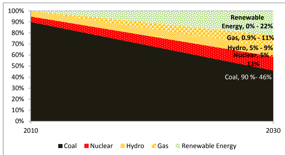
Figure 3: Change in electricity generation technology mix (Source: South Africa 2011b)
