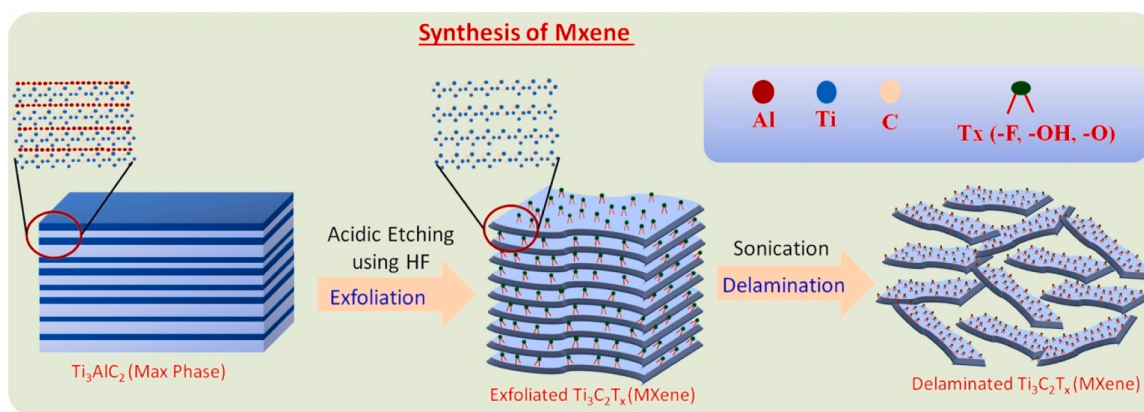
Fig. 3. Illustration of the process of MXene synthesis process [41]. Cullied with permission from Elsevier.
