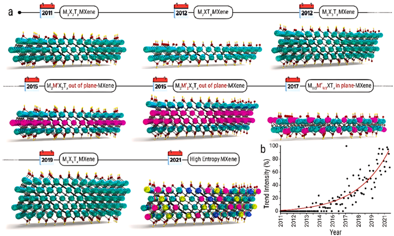
Fig. 2. (a) The structures of MXenes. (b) The data collected over the decade from users' engagement with the word "MXene." [34]. Culled with permission from Elsevier.
