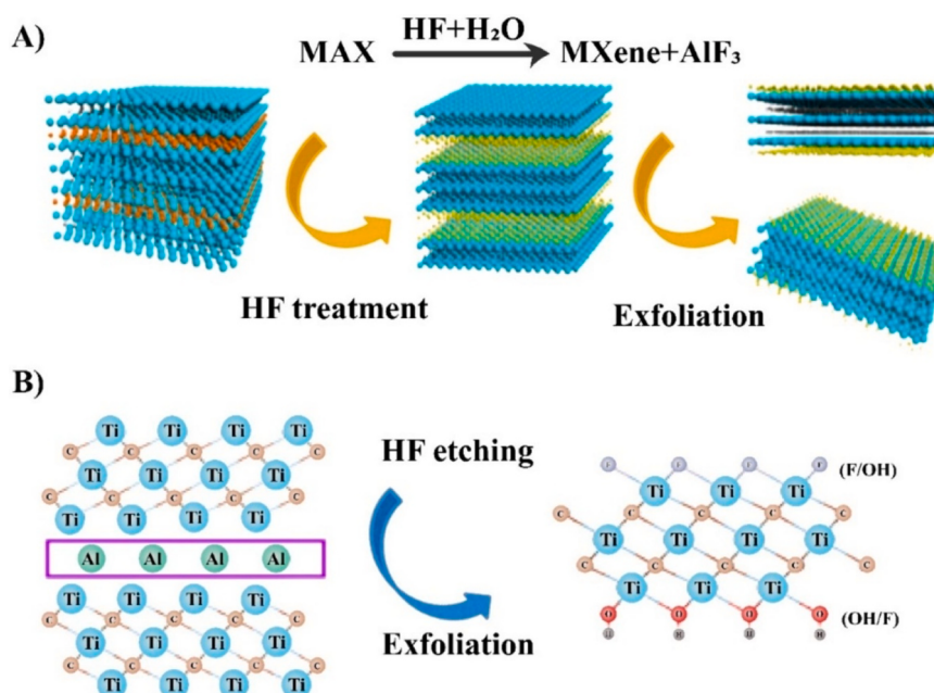
Fig. 4. Schematic illustration of selective etching of the MXenes with hydroxyl and fluorine atoms [8]. Cullied with permission from Elsevier.
