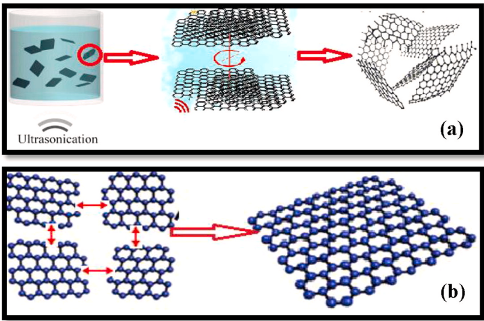
Fig. 1. (a) Liquid phase exfoliation, (b) joining of graphene flakes [24]. Culled with permission from Elsevier.
