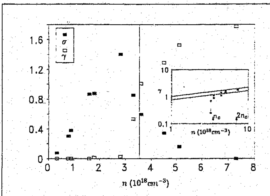
Figure 4.8: The average values of \sigma and \gamma , from figs. 4.7, in a single plot to compare the relative behaviour. The insert shows \gamma in the metallic phase, together with predictions of the free-electron model with two different effective masses.
