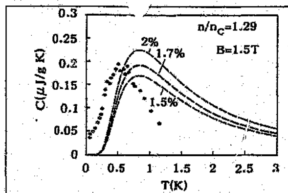
Figure 2.14: Comparisons with the specific heat data in the metallic phase. Reproduced from the publication in §2.7.
