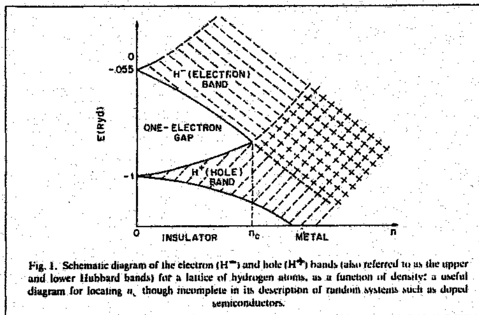
Figure 1.3: Energy level diagram showing the Mott transition. Reproduced from [3].
