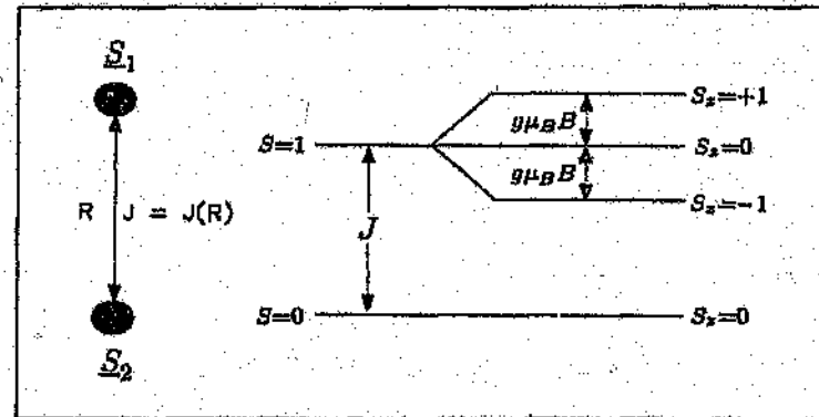
Figure 2.2: A spin-pair, with exchange coupling J , and corresponding energy levels.
