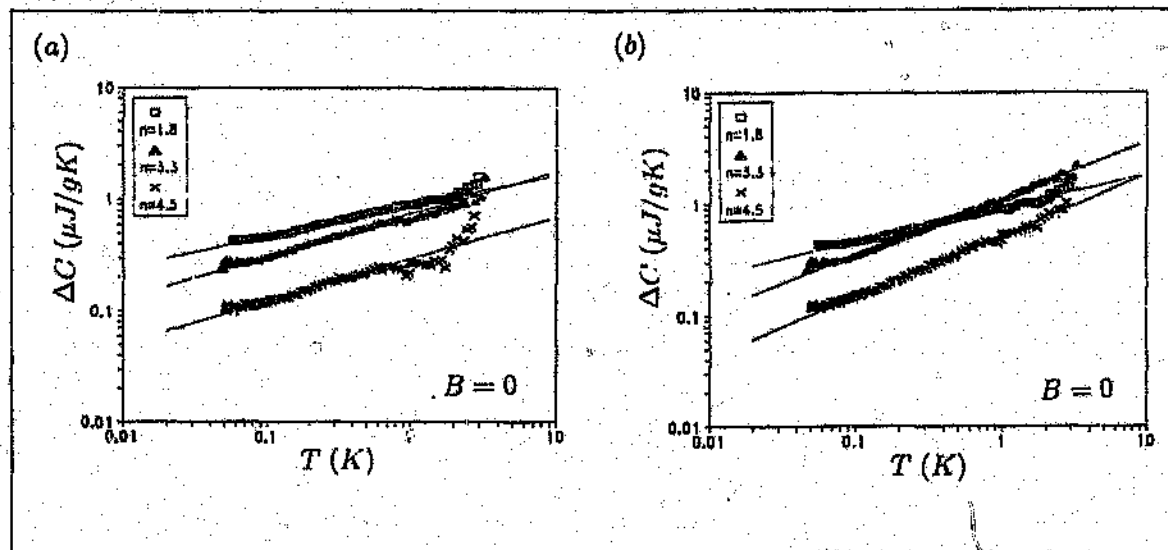
Figure 4.9: The excess specific heat \Delta C obtained using (a) procedure 1, and (b) procedure (2). The power law form predicted by the model is shown by the straight lines.
