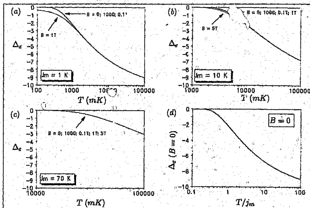
Figure C.7: Plots of the correction function \Delta_\epsilon .
