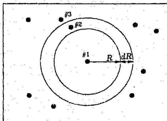
Figure B.1: A random spatial distribution of spins.
