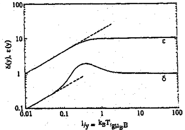
FIG. 1. The coefficients \delta and \varepsilon , as defined in Eqs. (6), vs k_B T / g\mu_B B . The dashed lines show the low-temperature asymptotic behavior where \delta, \varepsilon \sim y^{-\alpha} .
