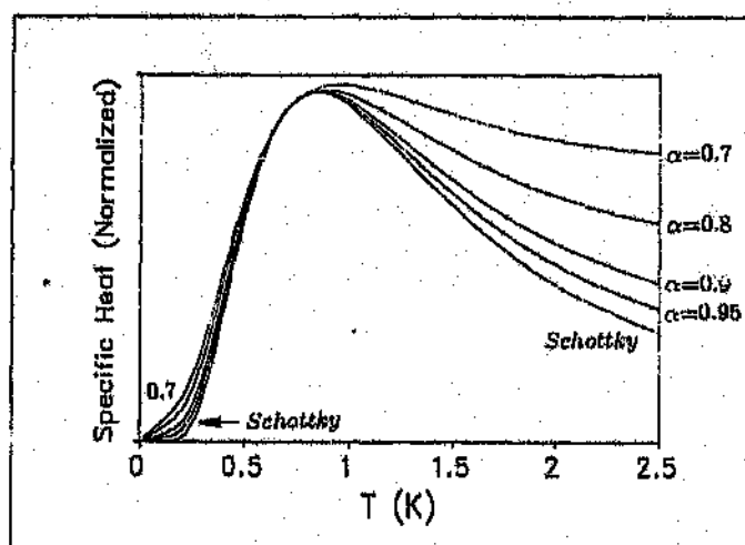
Figure C.9: The normalized specific heat for various \alpha values, together with the Schottky specific heat, for comparison.
