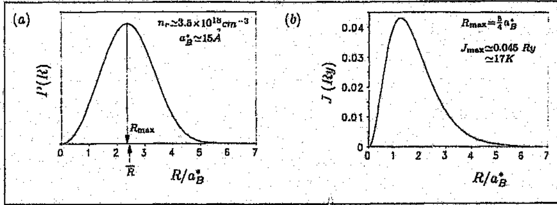
Figure 2.1: Plot of (a) the Poisson distribution function P(R) , using the Si:P values for a_B^* and n = n_c , and (b) the Herring-Flicker expression for the exchange coupling. The point (R_{\max}, J_{\max}) denotes the maximum in this function.
