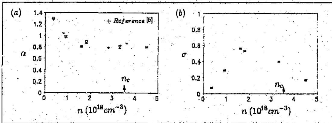
Figure 4.2: Values obtained for \alpha and \sigma from fitting the zero-field data of various donor concentrations n .
