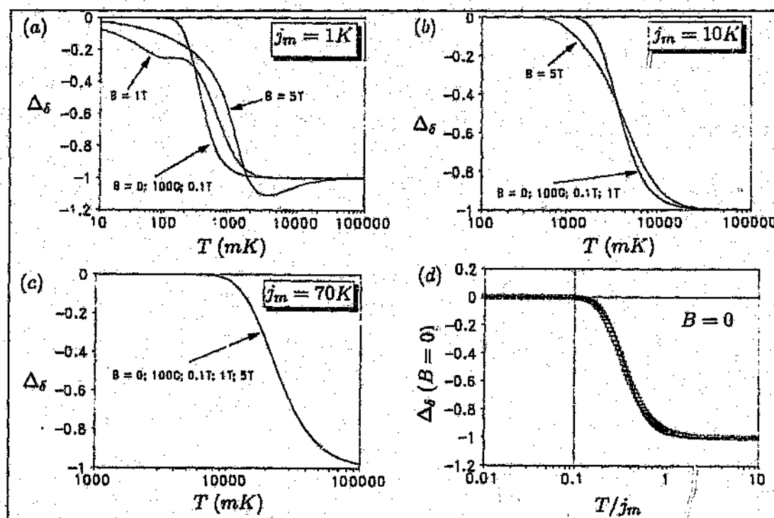
Figure C.6: Plots of the correction function \Delta_\delta .
