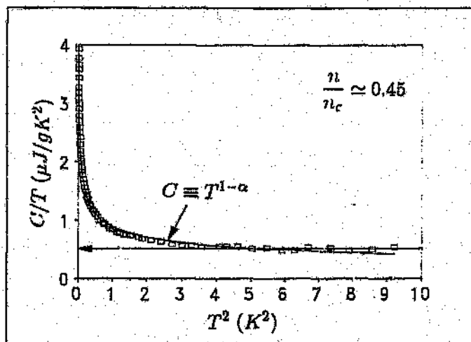
Figure 4.11: The zero-field specific heat data for n = 1.6 \times 10^{18} \text{ cm}^{-3} , as shown in fig. 4.10a, plotted as C/T versus T^2 . This plot shows the apparent constant contribution at high T attributed to the itinerant component in the "standard" method (§4.2.1).
