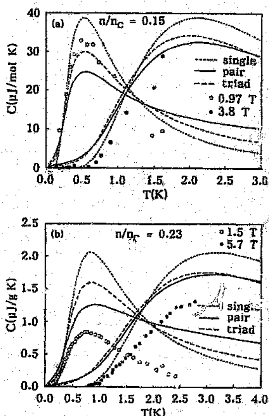
FIG. 3. Specific-heat predictions for Si:P as a function of concentration, temperature, and magnetic field for the single-spin, pair, and triad models. The experimental data of (a) are taken from Kobayashi et al. (Ref. 3), while those of (b) are taken from Lakner and Löhneysen (Ref. 4).
