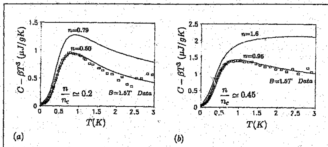
Figure 5.1: The B = 1.5T specific heat data for the concentrations (a) n = 0.79 \times 10^{18} \text{ cm}^{-3} and (b) n = 1.6 \times 10^{18} \text{ cm}^{-3} . The upper curves are the predictions of the spin-pair model, while the lower curves show these results when the concentrations are scaled down.
