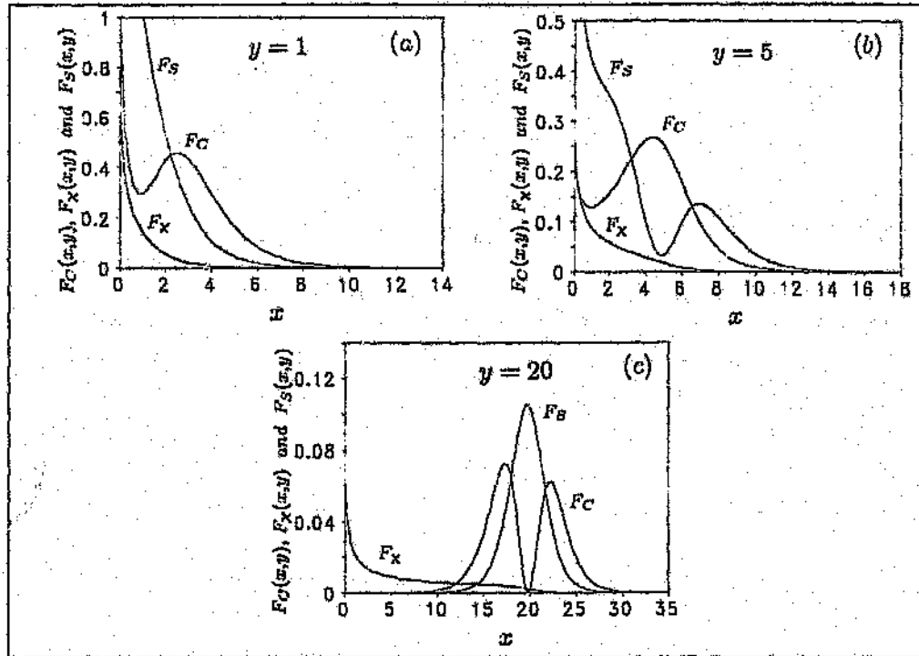
Figure C.3: Plots of the integrands F_C(x, y) , F_X(x, y) , and F_S(x, y) , for various values of y , to determine a suitable upper cutoff for the integration.
