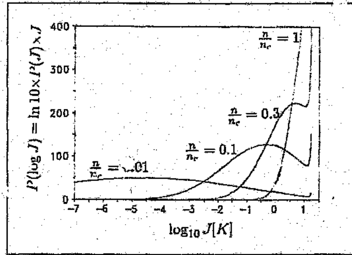
Figure 2.5: The distribution P(\log J) of \log J values.
