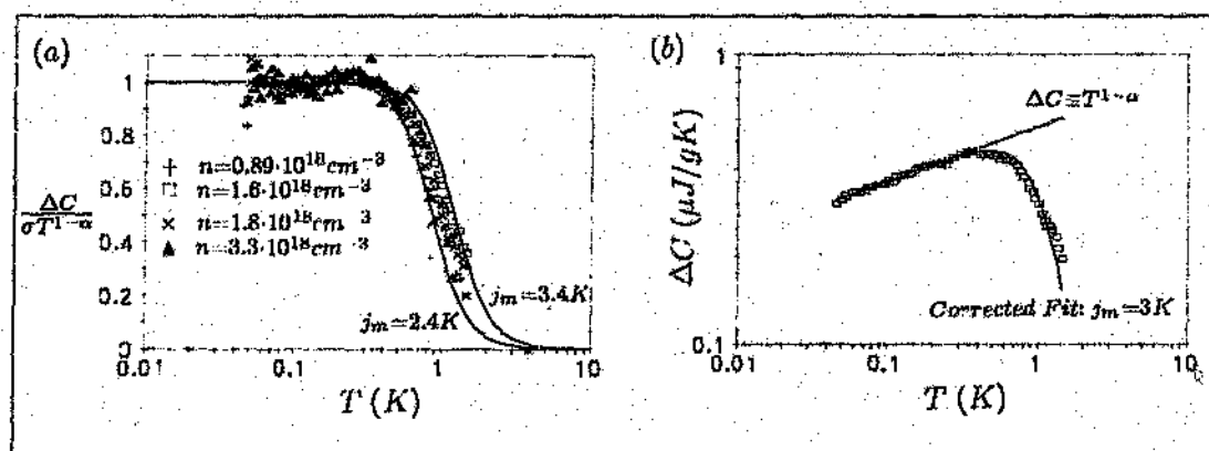
Figure 4.3: The excess specific heat \Delta C for B = 0 , with (a) a plot of \Delta C/\sigma T^{1-\alpha} versus T , together with fits of eqn. (4.19), while (b) shows a plot of \Delta C for n = 1.6 \times 10^{18} \text{ cm}^{-3} , indicating the power law form as well as the corrected fit given by eqn. (4.18).
