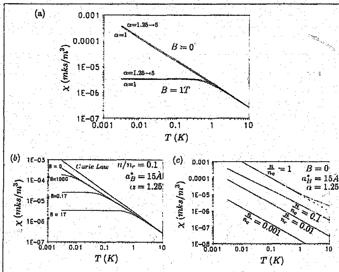
Figure 2.12: Dependence of the spin-triad susceptibility \chi on (a) the parameter \alpha , (b) the magnetic field B , and (c) the concentration n .
