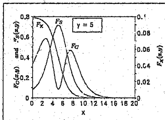
Figure C.2: Plots of the integrands F_C(x, y) , F_x(x, y) , and F_S(x, y) to show the exponentially decaying tails.
