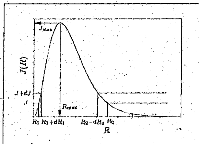
Figure B.2: Graphical aid to the determination of P(J) , showing a plot of the Herring-Flicker exchange coupling J_{HF}(R) .
