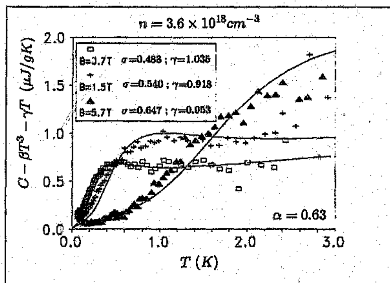
Figure 4.13: The excess specific heat \Delta C for a just-metallic sample. The curves are fits of \sigma \delta(y) T^{1-\alpha} , with the parameters used shown in the figure.
