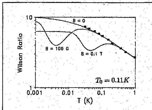
Figure 3.4: The magnetic field dependence of the Wilson Ratio.
