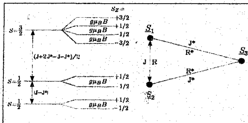
Figure 2.10: The energy level diagram for the spin-triad shown.
