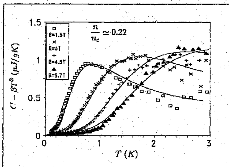
Figure 4.14: The electronic specific heat for n = 3.3 \times 10^{18} \text{cm}^{-3} (refer to fig. 4.12). The curves are fits of eqn. (4.22) with \gamma = 0 . The value of \alpha = 0.4 is much lower than expected.
