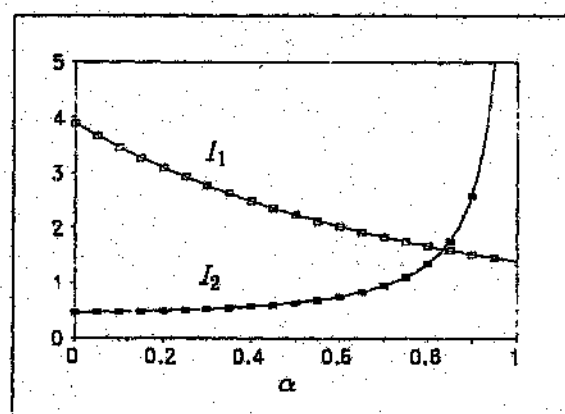
Figure C.1: A plot of the terms I_1 and I_2 .
