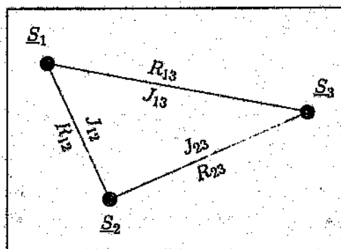
Figure 2.9: A spin-triad, where R_{ij} is the separation and J_{ij} the exchange coupling between spins i and j .
