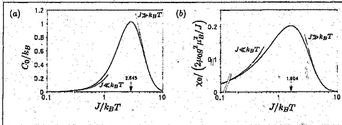
Figure 2.3: The (a) specific heat C_0 and (b) susceptibility \chi_0 of a single J -coupled spin-pair. The peak positions and asymptotic forms are also included.
