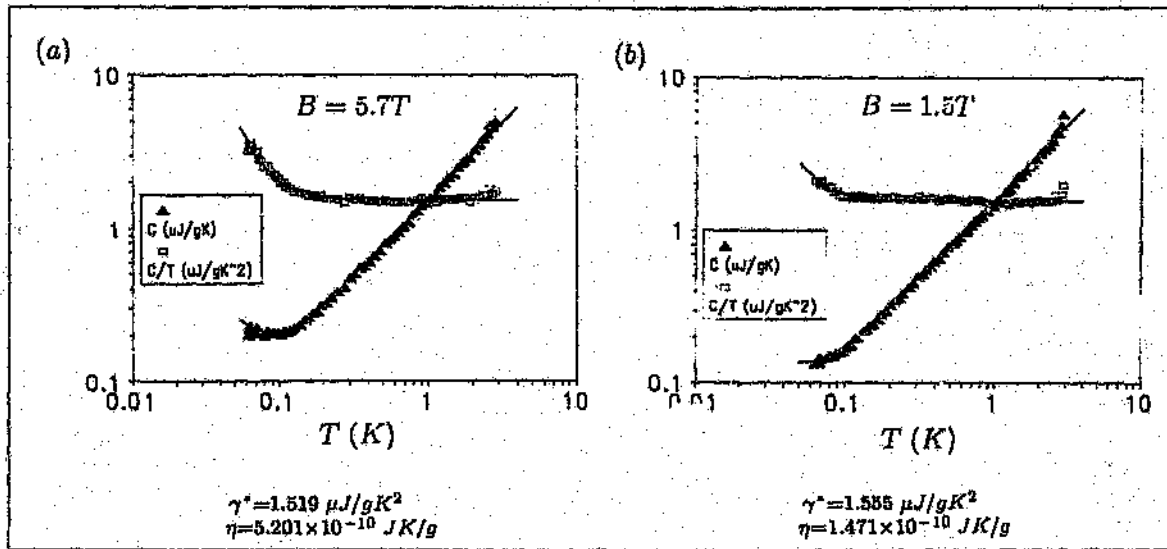
Figure 4.19: Plots of C and C/T versus T for n = 7.3 \times 10^{18} cm^{-3} , in two magnetic fields. The curves are fits of (4.26) and (4.27). The low T anomaly is clearly visible as the upturn in the data.
