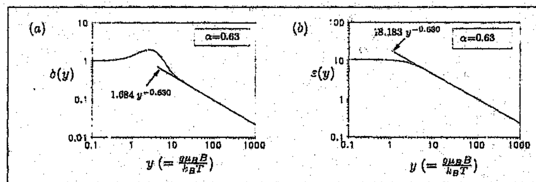
Figure D.1: Plots of the functions (a) \delta(y) , and (b) \varepsilon(y) , versus y . Also shown are the determined asymptotic forms.
