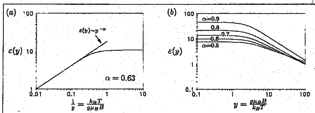
Figure 3.2: A plot of (a) the function \varepsilon(y) versus 1/y , for \alpha = 0.63 , with (b) showing its dependence on the parameter \alpha .
