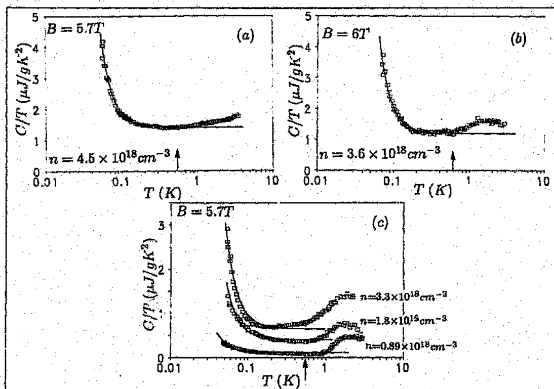
Figure 4.20: Plots of C/T versus T for various concentrations, with the curves being fits of eqn. (4.27). The arrows indicate the predicted temperature up to which this expression should describe the data.
