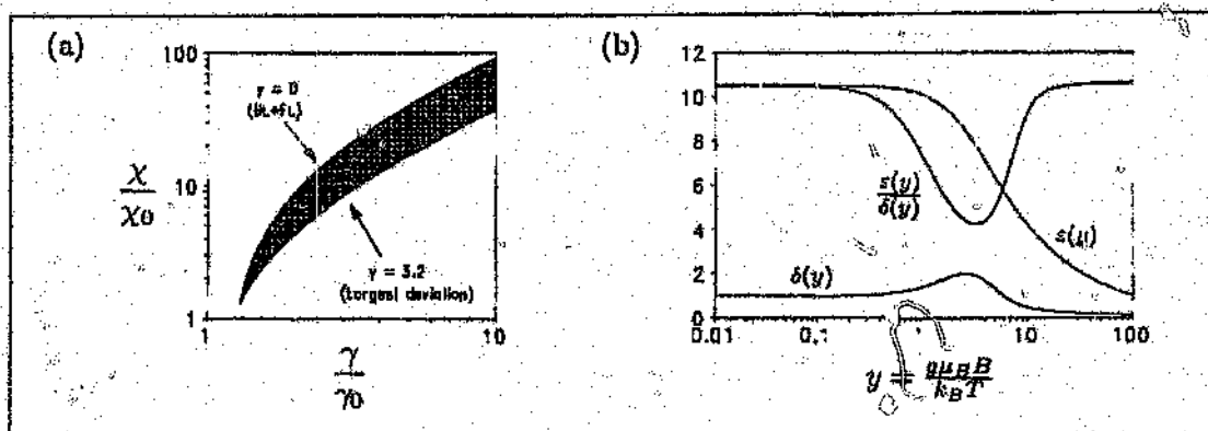
Figure 3.5: The (a) surface of allowed (\gamma/\gamma_0, \chi/\chi_0) values predicted by the extended two fluid model, and (b) a plot of \epsilon(y)/\delta(y) , which determines this surface.
