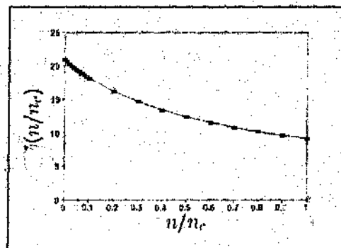
Figure B.3: A plot of the factor I(n/n_c) appearing in expression (B.18), which was evaluated numerically.
