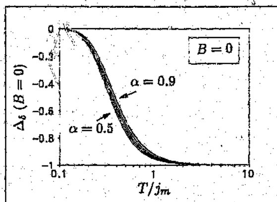
Figure C.8: The dependence of the zero-field correction \Delta_s on the parameter \alpha .
