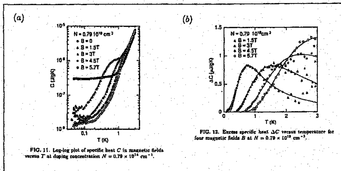
Figure 4.4: Plots of (a) the total specific heat C of an insulating sample in various magnetic fields, with (b) showing the corresponding excess specific heat \Delta C obtained with the use of eqn. (4.11). Reproduced from [5].
