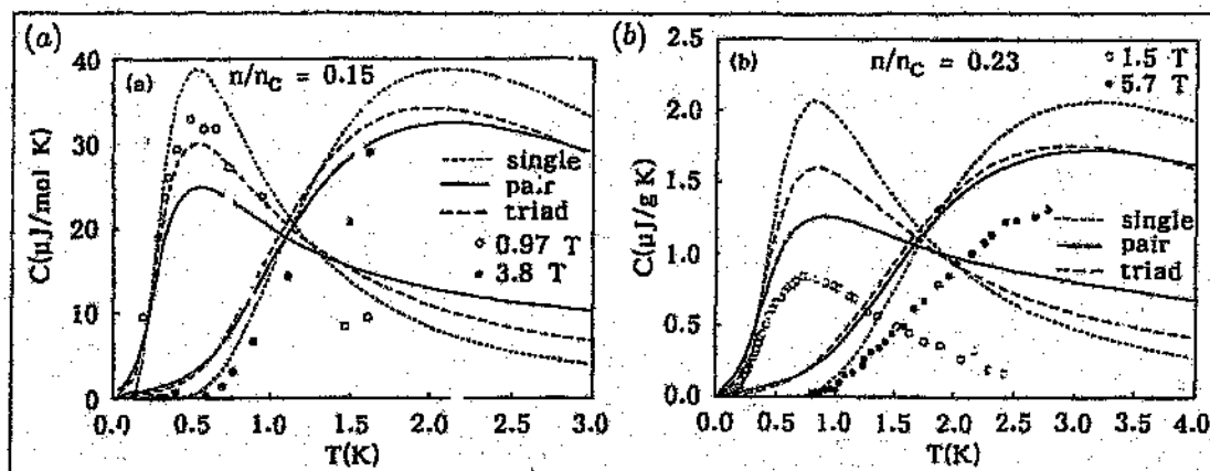
Figure 2.13: Comparisons with the specific heat data in the insulating phase. Reproduced from the publication in §2.7.
