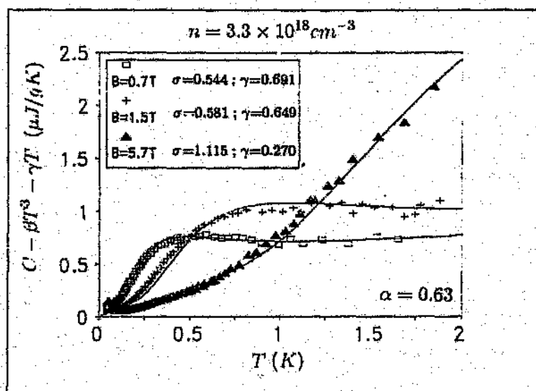
Figure 4.12: The excess specific heat \Delta C for a just-insulating sample. The curves are fits of \sigma \delta(y) T^{1-\alpha} , with the parameters used shown in the figure.
