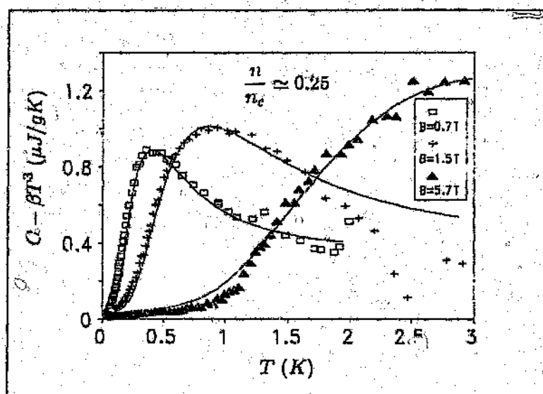
Figure 4.16: The electronic specific heat for n = 0.89 \times 10^{18} \text{ cm}^{-3} . The curves are fits of (4.22), with no itinerant contribution ( \gamma = 0 ), and \alpha = 0.83 . The value of \sigma = 0.275 was used for all fields. The B = 1.5T deviation for T \gtrsim 2K could be attributed to the larger uncertainties in the data occurring at these temperatures [5].
