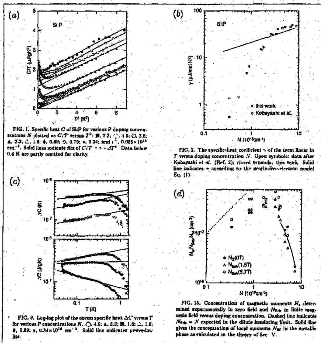
Figure 1.6: Plots of (a) C/T versus T^2 for B = 0 , (b) \gamma versus n obtained from the analysis of (a), and (c) the corresponding excess specific heat \Delta C obtained from (a). The effective concentration of localized moments obtained from the B \neq 0 specific heat analysis is shown in (d). Reproduced from [5].
