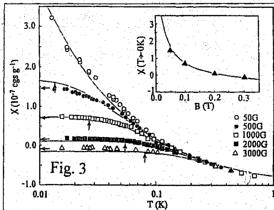
Figure 4.24: Comparisons to the susceptibility data in higher fields for a just-metallic sample. Reproduced from the publication in §4.7.
