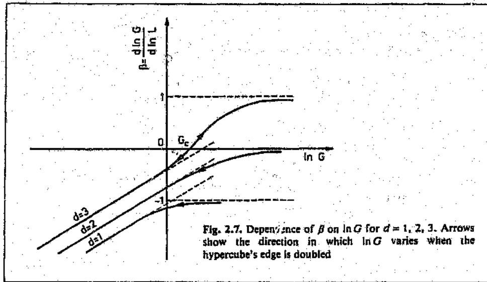
Figure 1.5: The scaling parameter \beta(g) . Reproduced from [4].
