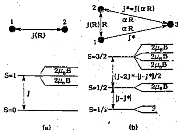
FIG. 1. Energy-level diagram for the (a) spin pair and (b) spin triad in a magnetic field B . J is the exchange coupling between a pair of spins, and \alpha is a parameter which is a little greater than unity.
