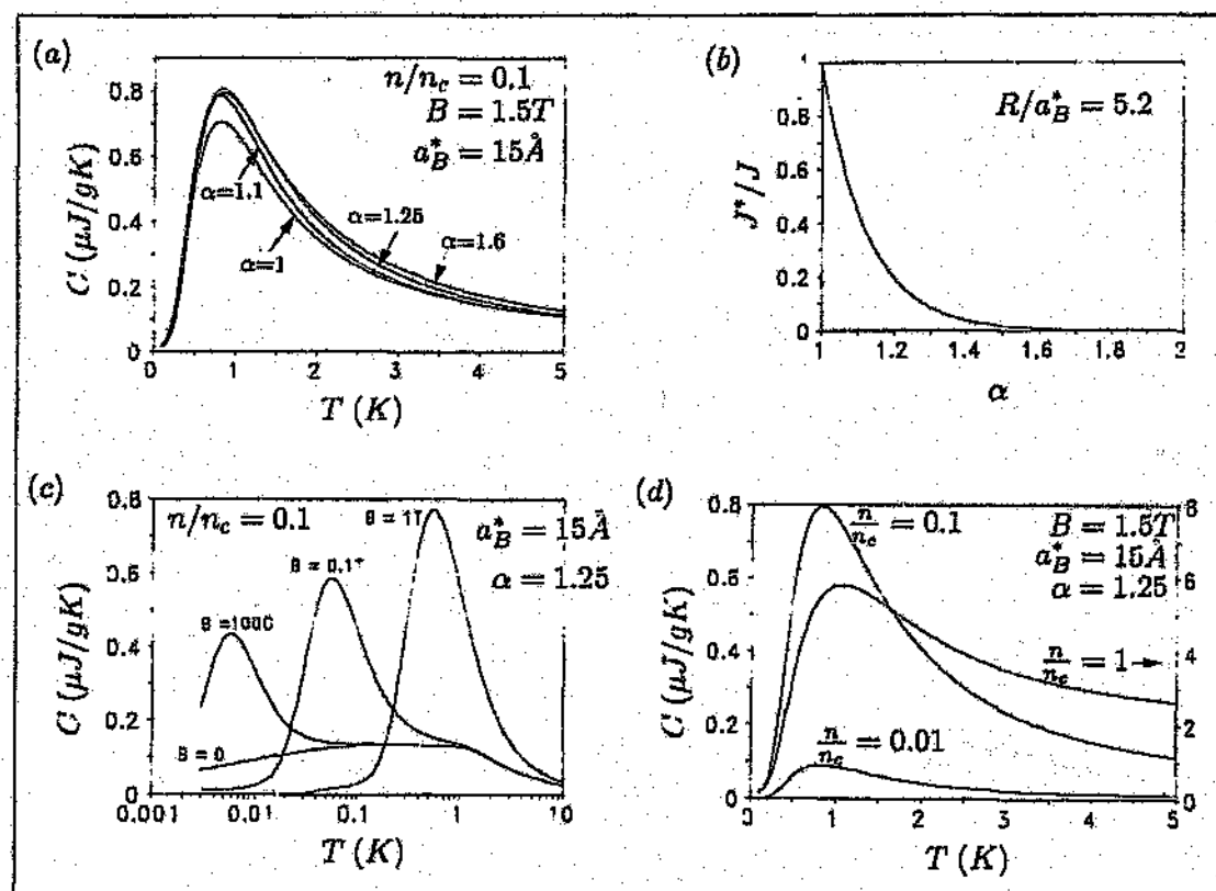
Figure 2.11: Dependence of the spin-triad specific heat C on (a) the parameter \alpha , (c) the magnetic field B , and (d) the concentration n . Figure (b) plots J^*/J versus \alpha as an aid to fig. (a).
