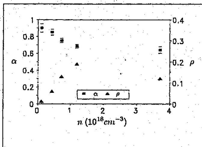
Figure 4.23: Plot of the values of \alpha and \rho obtained from the fittings in figs. 4.22.
