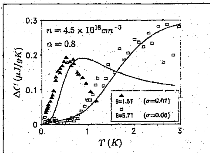
Figure 4.6: Predictions of the extended two-fluid model to the n = 4.5 \times 10^{18} \text{ cm}^{-3} specific heat data in fig. 4.1b.
