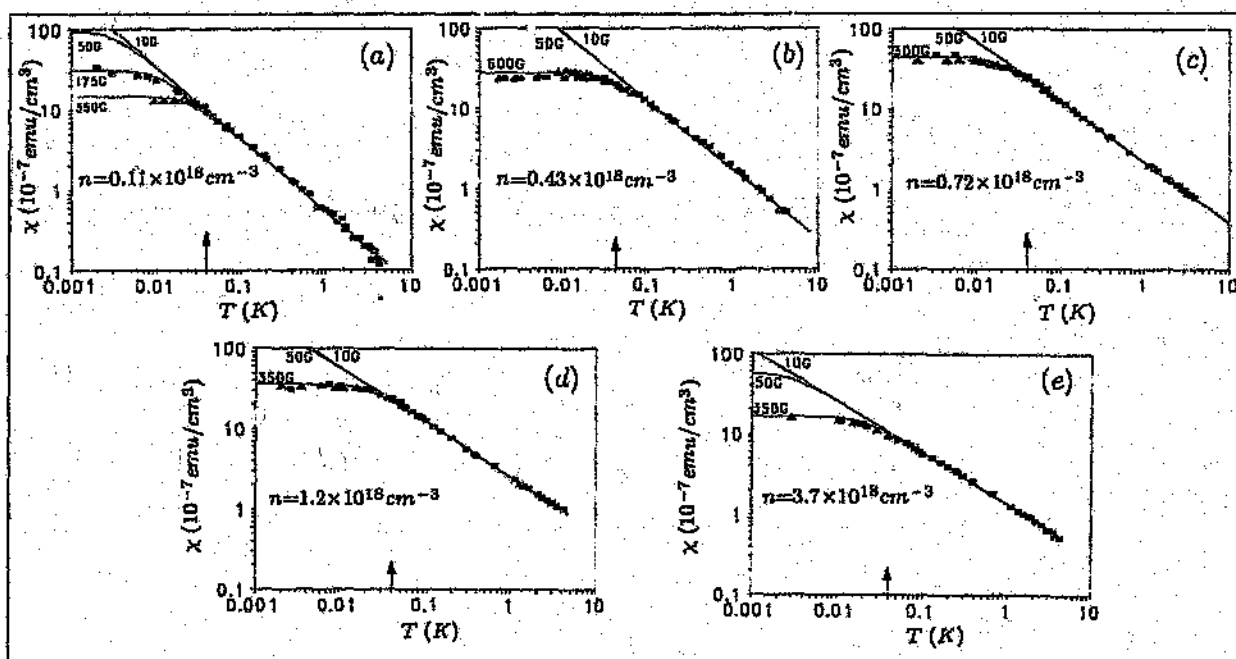
Figure 4.22: Fits of the prediction in eqn. (4.30) to the low magnetic field susceptibility \chi , for various concentrations in the insulating phase. The arrows indicate the temperature above which we predict the T^{-\alpha} power law form. The magnetic fields used for each curve are shown. For the data we use "■" and "▲" for B = 10G and 50G respectively.
