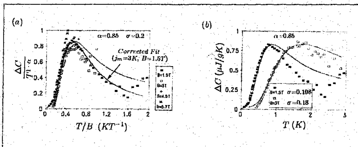
Figure 4.5: The specific heat data for n = 0.79 \times 10^{18} \text{ cm}^{-3} from fig. 4.4b, together with the predictions of the extended two-fluid model.
