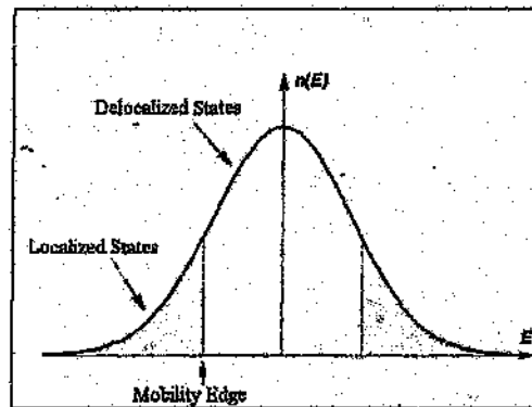
Figure 1.4: Density of states n(E) in the Anderson model.
