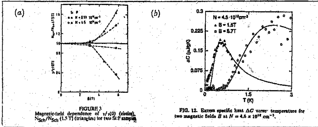
Figure 4.1: Plots showing (a) the field-dependence of the effective localized moment concentration N_{Sch} and itinerant contribution \gamma(B) , and (b) the excess specific heat \Delta C in non-zero fields for a metallic sample. Reproduced from (a) [20] and (b) [5].
