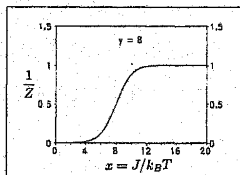
Figure C.5: A plot of 1/Z versus x , giving the probability of the singlet state of the spin-pair being occupied.
