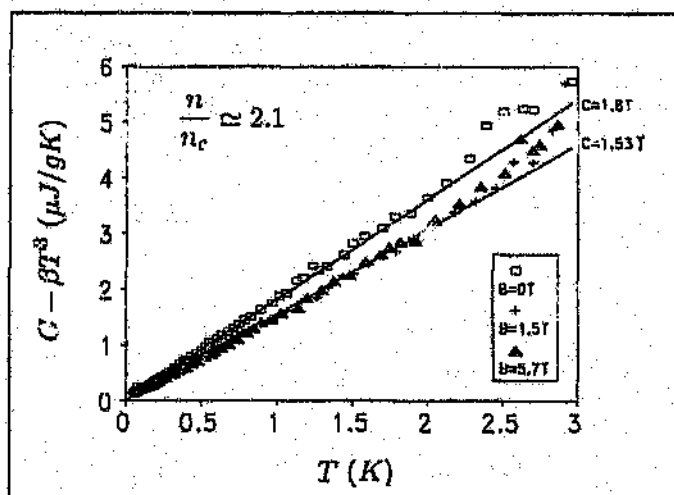
Figure 4.18: The electronic specific heat for n = 7.3 \times 10^{18} \text{ cm}^{-3} in various magnetic fields. The curves are linear fits to the data.
