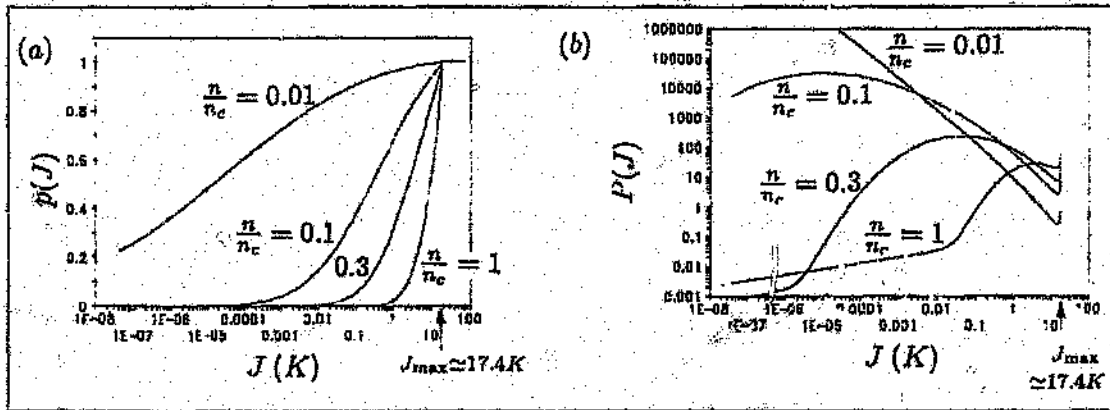
Figure 2.4: Plot of (a) the function p(J) = \int_0^J P(J)dJ , and (b) the distribution function P(J) = p'(J) .
