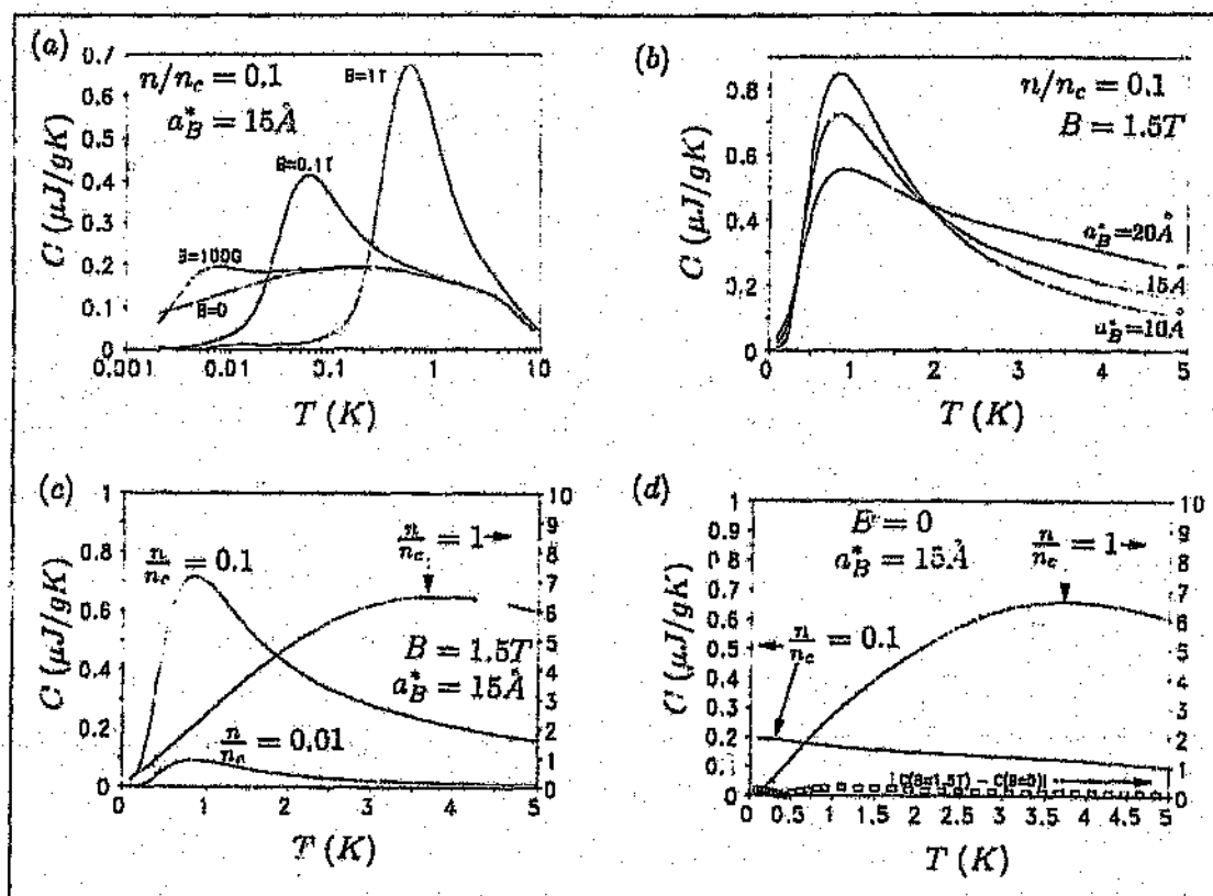
Figure 2.7: The dependence of the spin-pair system specific heat C on (a) the magnetic field B , (b) the Bohr radius a_B^* , and (c) the concentration n . Fig. (d) is shown to explain a feature of fig. (c).
