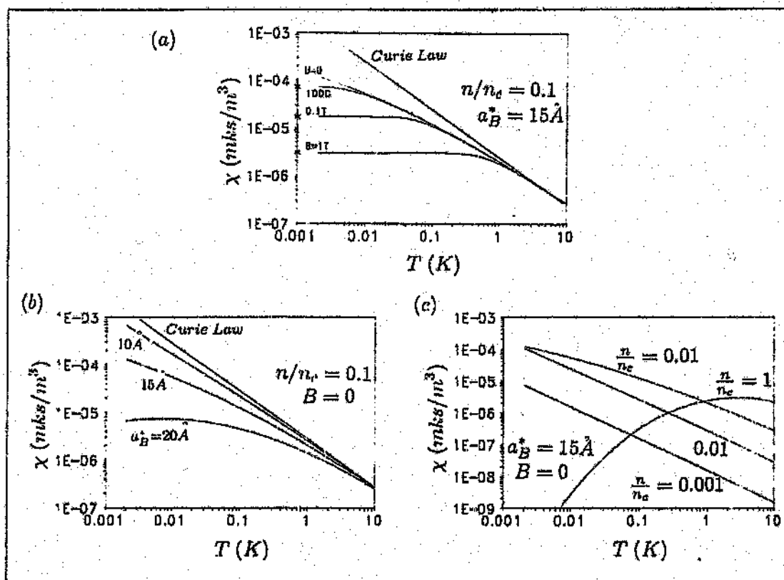
Figure 2.8: The dependence of the spin-pair system susceptibility \chi on (a) the magnetic field B , (b) the Bohr radius a_B^* , and (c) the concentration n .
