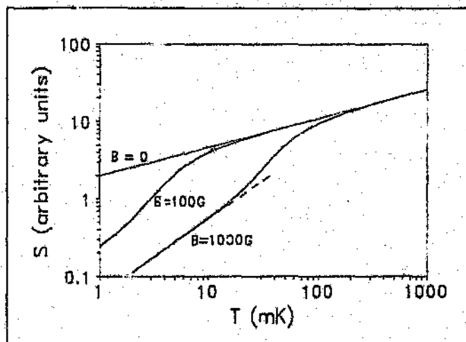
Figure 3.3: The entropy S , in arbitrary units, for various magnetic fields.
