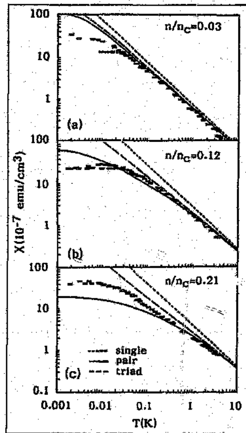
Figure 2.15: Comparisons with the susceptibility data. Reproduced from the publication in §2.7.
