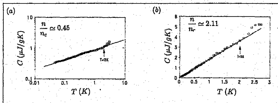
Figure 4.10: The zero-field specific heat, with the phonon contribution subtracted from the data, for an (a) insulating, and (b) metallic sample. The straight lines indicate the form of the data.
