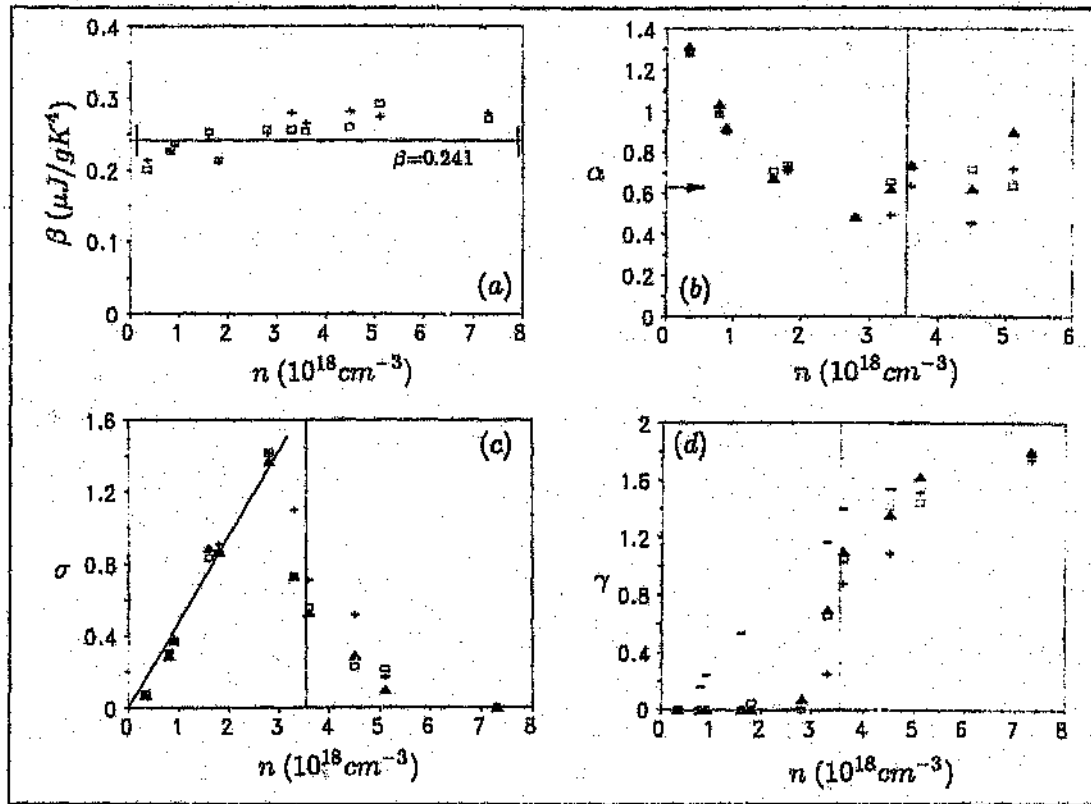
Figure 4.7: Plots of the values obtained for \beta , \alpha , \sigma , and \gamma from the fitting of eqn. (4.20) to the zero-field specific heat data.
