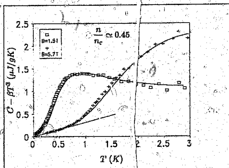
Figure 4.17: The electronic specific heat for n = 1.6 \times 10^{18} cm^{-3} . The curves are fits of (4.22), with no itinerant contribution ( \gamma = 0 ), and \alpha = 0.7 . The values of \sigma = 0.64 and 0.71 were used for B = 1.5 T and 5.7 T . The low temperature behaviour, predicted by (4.2), is also shown.
