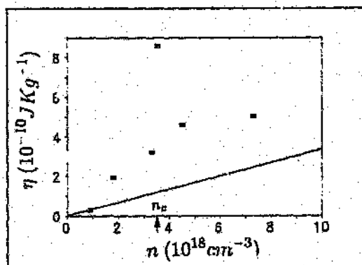
Figure 4.21: Plot of the nuclear contribution \eta versus the donor concentration n . The curve gives the expected value (eqn. (4.25)) for a non-interacting ^{31}\text{P} nuclear system.
