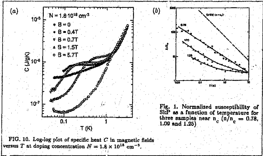
Figure 1.2: Plot of (a) Specific heat of 'insulating' Si:P for various magnetic fields, and (b) normalized susceptibility of Si:P on both sides of the MI transition ( \chi_0 is the Pauli value). Reproduced from [5] and [6] respectively.
