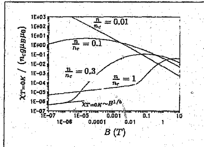
Figure 2.6: The magnetic field dependence of the absolute zero susceptibility \chi_{T=0K} .
