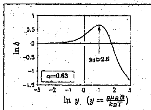
Figure C.10: A plot of \ln(\delta) versus \ln(y) , for \alpha = 0.63 . Indicated is the position y_0 of the maximum.
