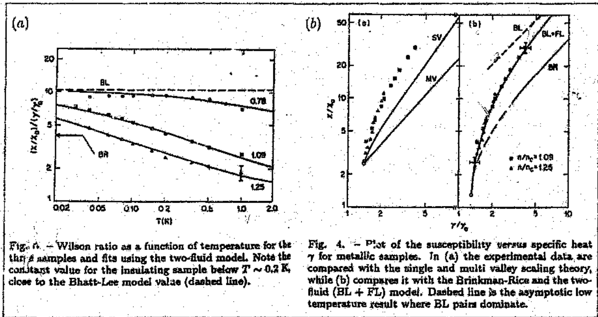
Figure 1.7: The (a) Wilson ratio and (b) \chi/\chi_0 versus \gamma/\gamma_0 plots, reproduced from [11].
