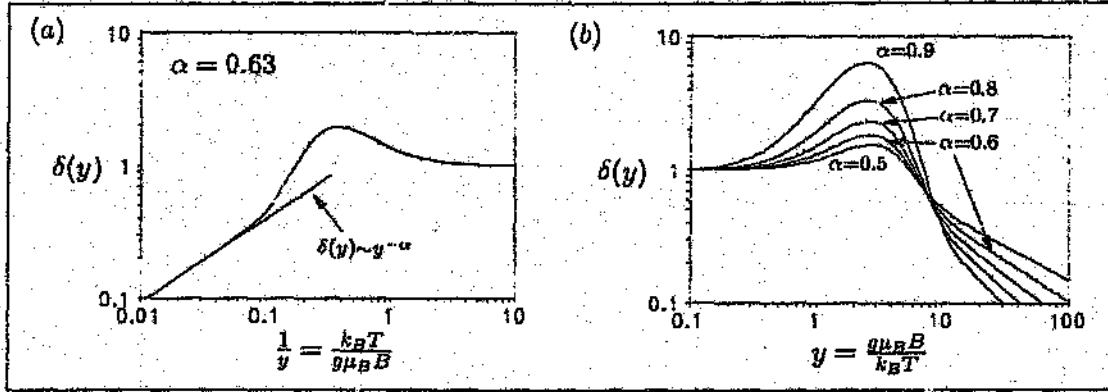
Figure 3.1: A plot of (a) the function \delta(y) versus 1/y , for \alpha = 0.63 , with (b) showing its dependence on the parameter \alpha .
