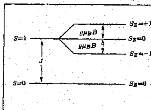
Figure C.4: Spin-pair energy levels.
