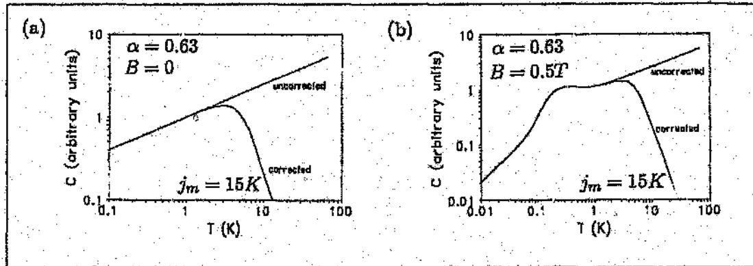
Figure 3.6: Plots of the specific heat C for a (a) zero, and (b) non-zero magnetic field, showing the effects of introducing the corrections to the extended two-fluid model.
