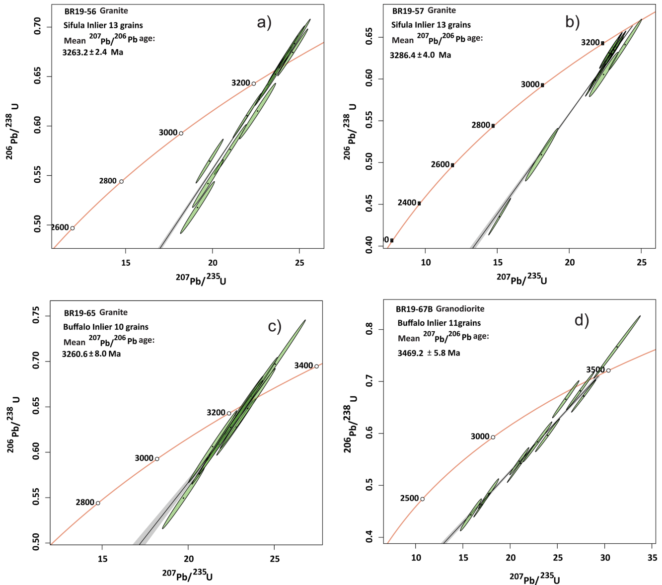
Fig. 17. U-Pb (Wetherill) concordia diagrams for zircons recovered from the granitoids of the Buffalo River Greenstone Belt. Data ellipses correspond to 1-sigma analytical uncertainties. Age calculations and data display were conducted using IsoplotR (Vermeesch, 2018).
