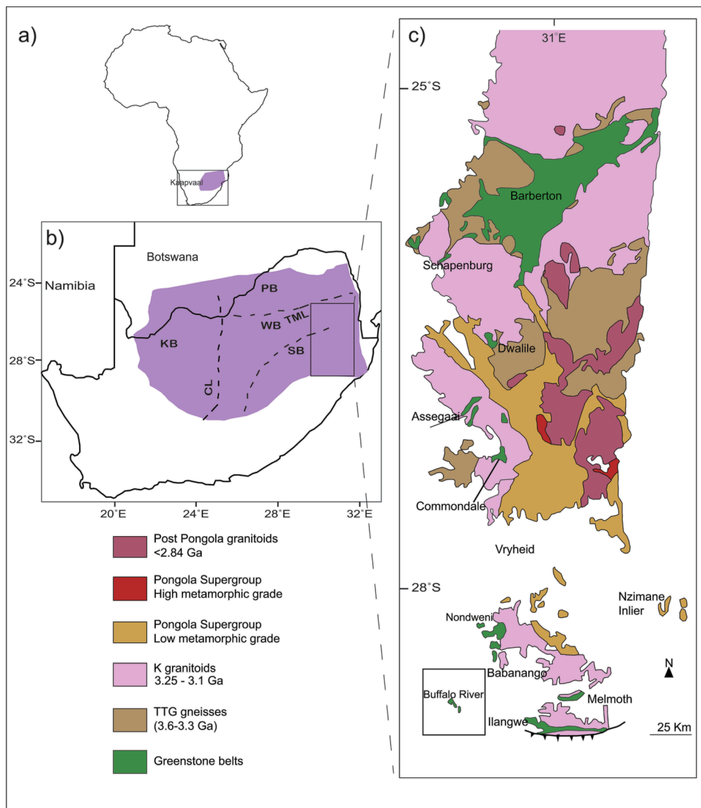
Fig. 1. Location of the Kaapvaal Craton (a) and (b) associated subdomains and structural features. KB Kimberley Block, SB Swaziland Block, WB Witwatersrand Block; PB Pietersburg Block, CL Colesburg lineament, TML Thabazimbi-Murchison Lineament; (c) geological map of the south-east region of the Kaapvaal craton, showing the distribution of Archean granitoid and greenstone belt remnants (after Hofmann et al., 2019). The Paleoproterozoic Buffalo River Greenstone Belt is located at the southern boundary of the Kaapvaal craton with the Mesoproterozoic Natal thrust belt.
