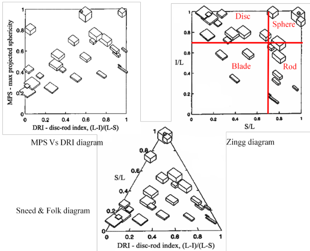
Figure 3.6 Examples of MPS vs. DRI, Sneed & Folk and Zingg shape diagrams used in this research. Adjusted from Illenberger (1991).
