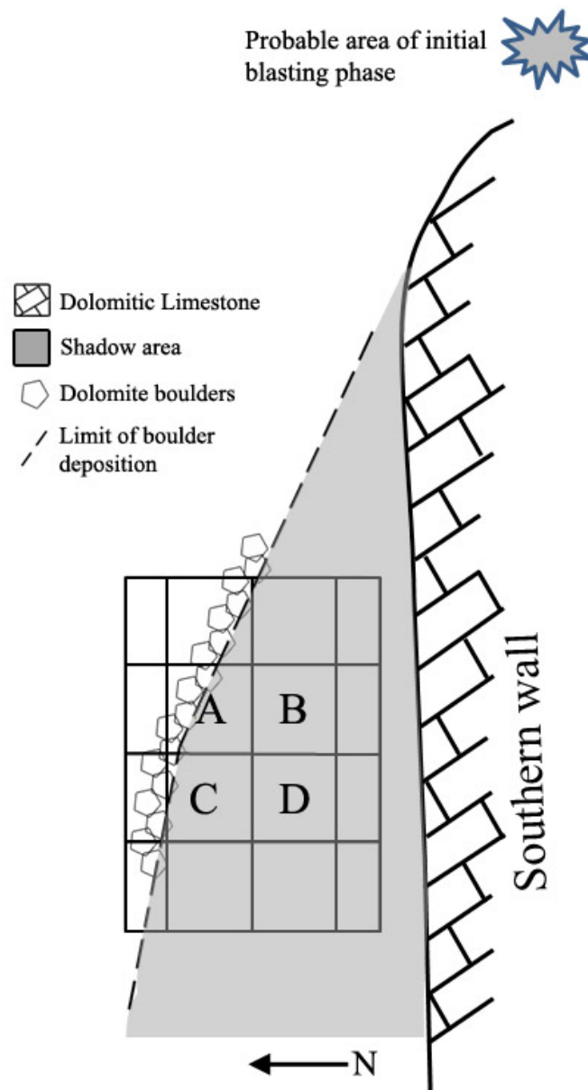
Figure 5.5 Plan view schematic of the STK-MH1 site with plotted dolomitic boulders deposited during the initial blasting phase. The area of initial blasting is indicated by the depositional pattern manifested by the fractured dolomite boulders.
