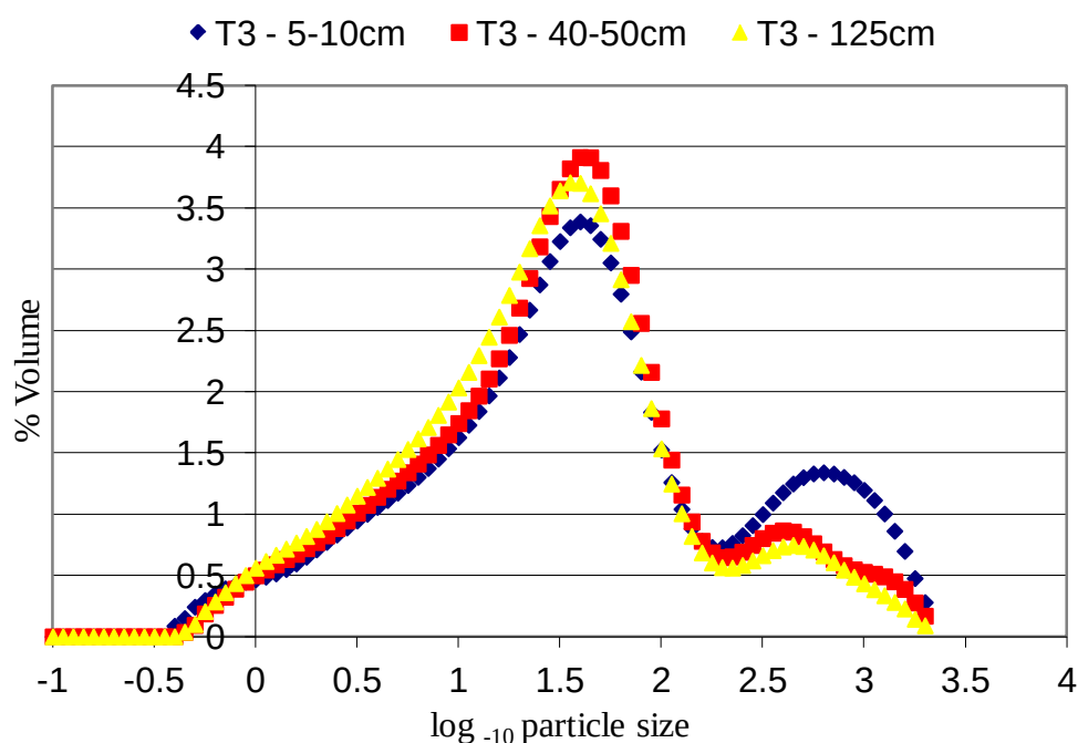
Figure 5.32 T3 combined particle size distribution curves. Stated sample depths are relative to deposit surface.
