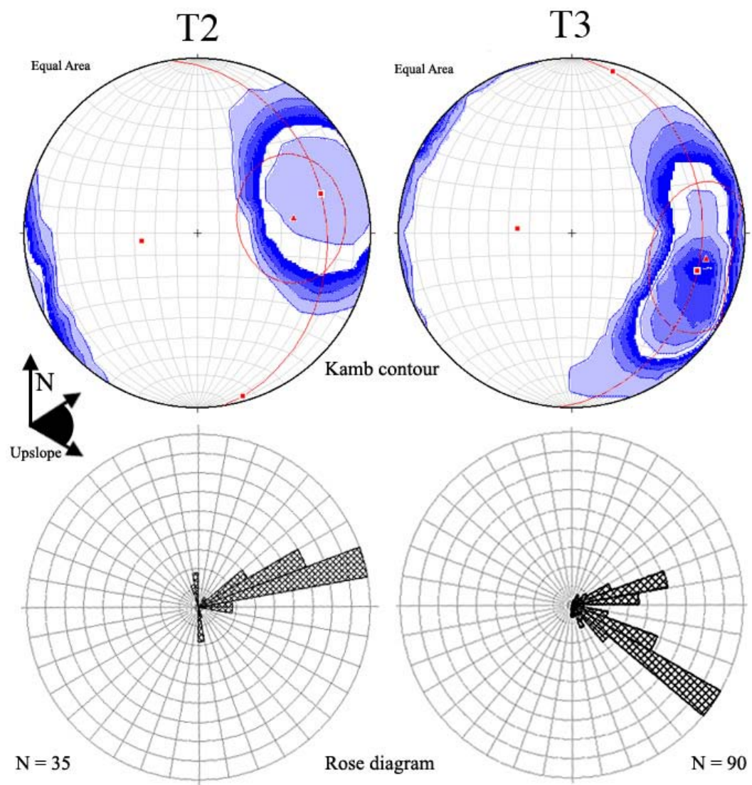
Figure 5.49 MH1 Fabric analysis models. Only T2 and T3 provided data for fabric analysis.
