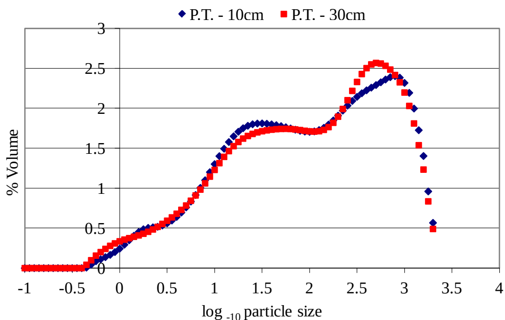
Figure 6.21 P.T. combined particle size distribution curves.
