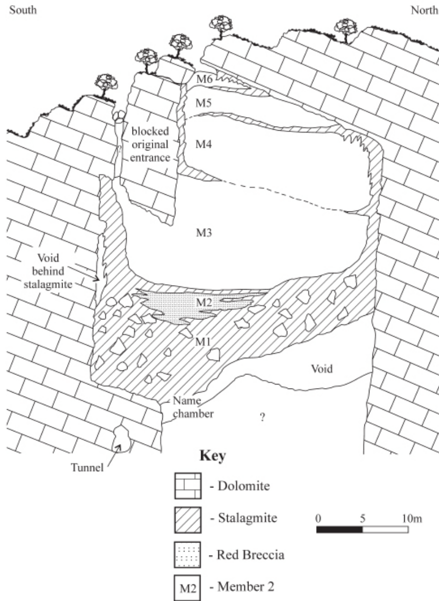
Figure 2.3 Clarke's Sterkfontein stratigraphy. Schematic north-south section of Sterkfontein to show general relationship of breccias with suggested original openings and possible surface topography. From Clarke (2006).
