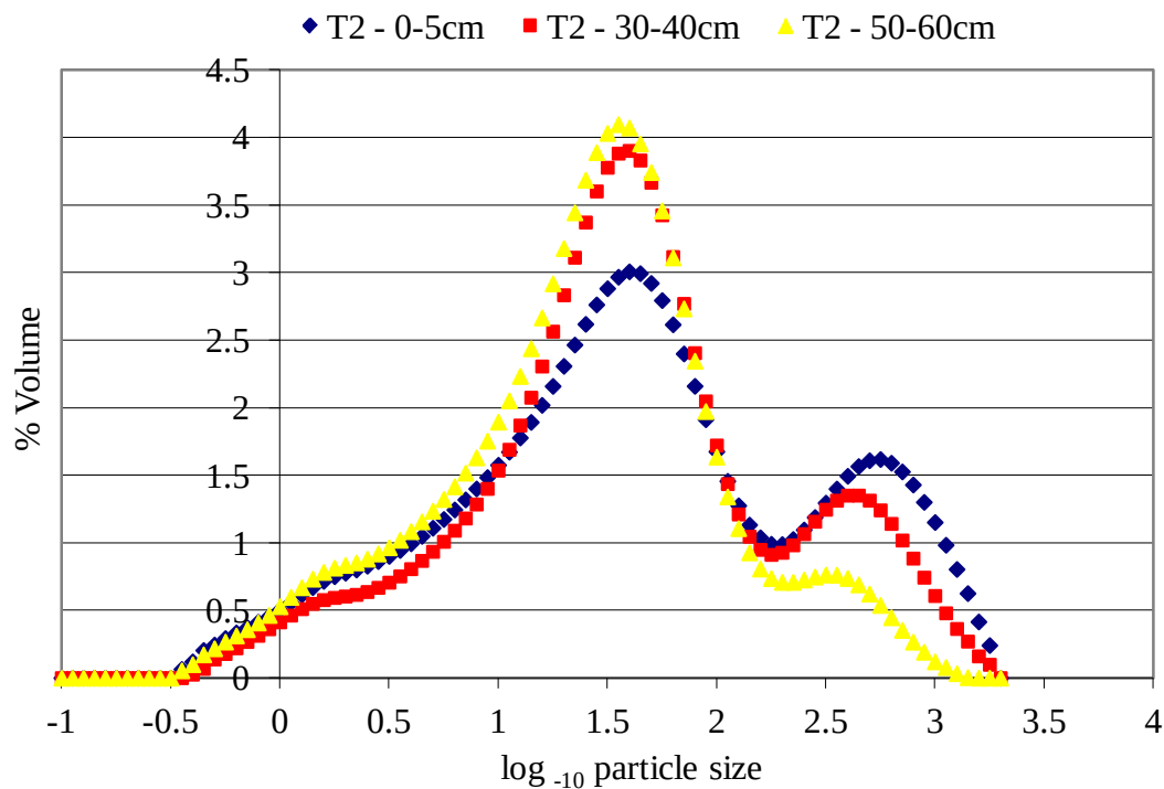
Figure 5.17 T2 combined particle size distribution curves. Stated sample depths are relative to deposit surface.
