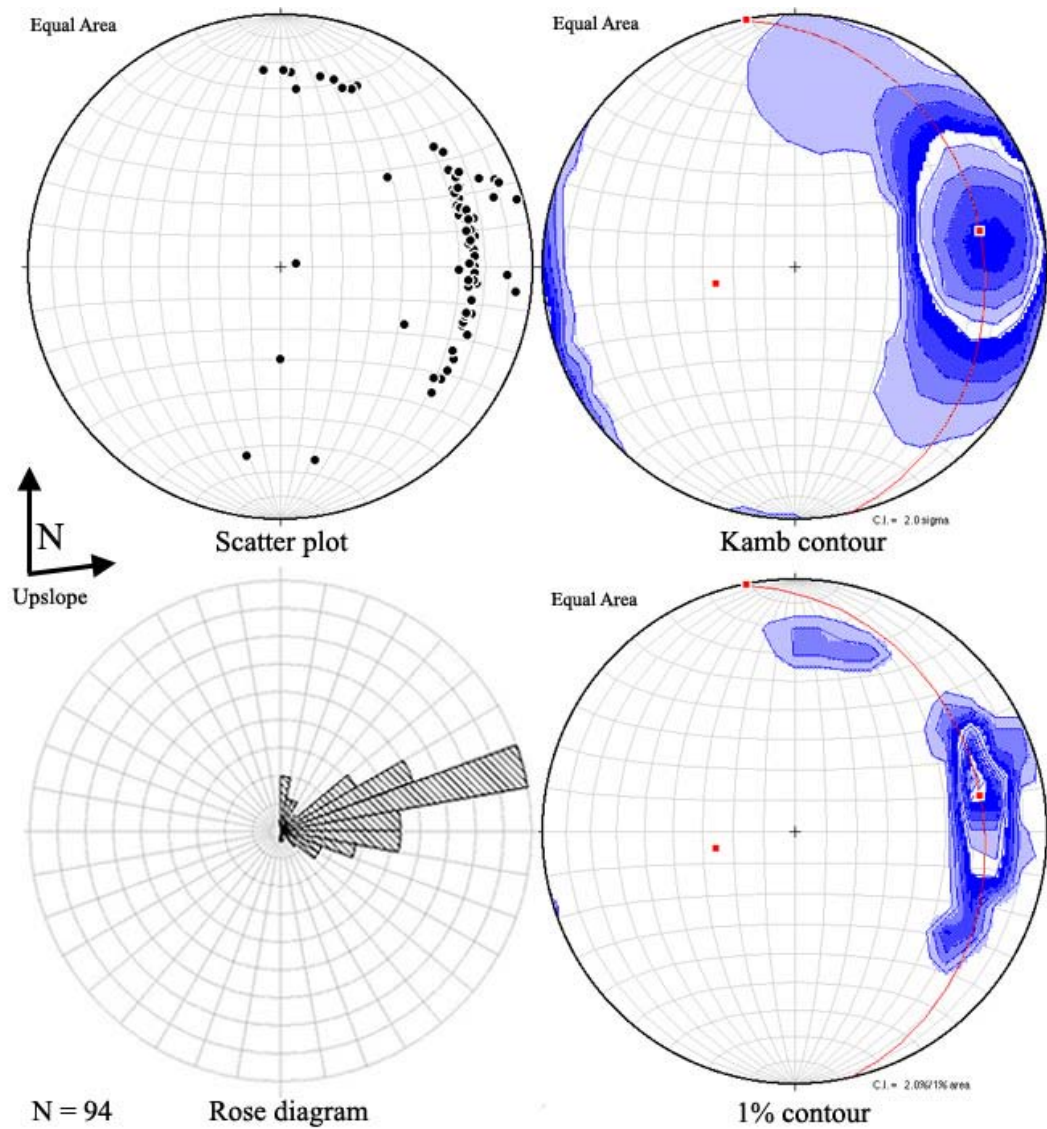
Figure 6.10 S.T. fabric analysis models. Kamb contouring has a contour interval of 2.0 sigma. The 1% contour plot has a contour interval of 1%. All stereographic projections show best the best fit plain and cone. The rose diagram sections represent 10°.
