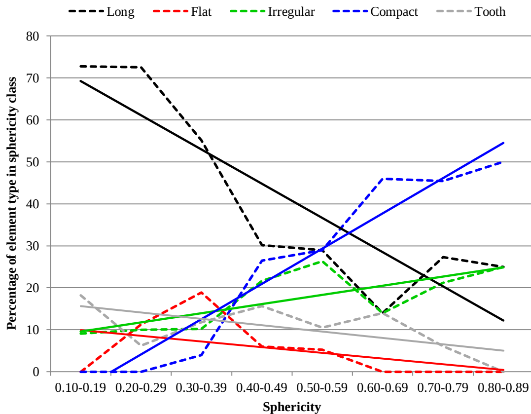
Figure 4.2 Relative proportions of different elements across sphericity classes. The dashed lines represent the actual data. The solid lines represent linear trend lines.
