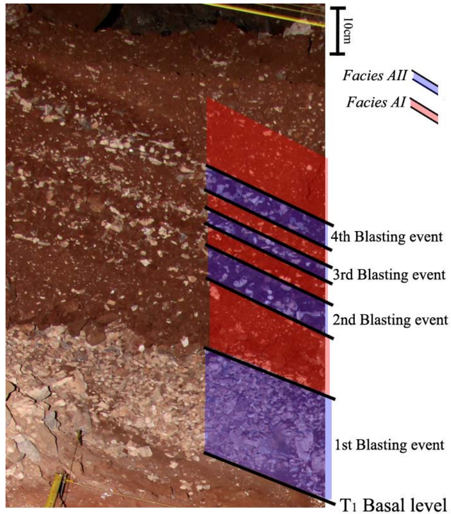
Figure 5.4 Stratigraphic profile of the southern wall of the T1 deposit. T1 basal level travertine stratum lies directly on the surface of T2.
