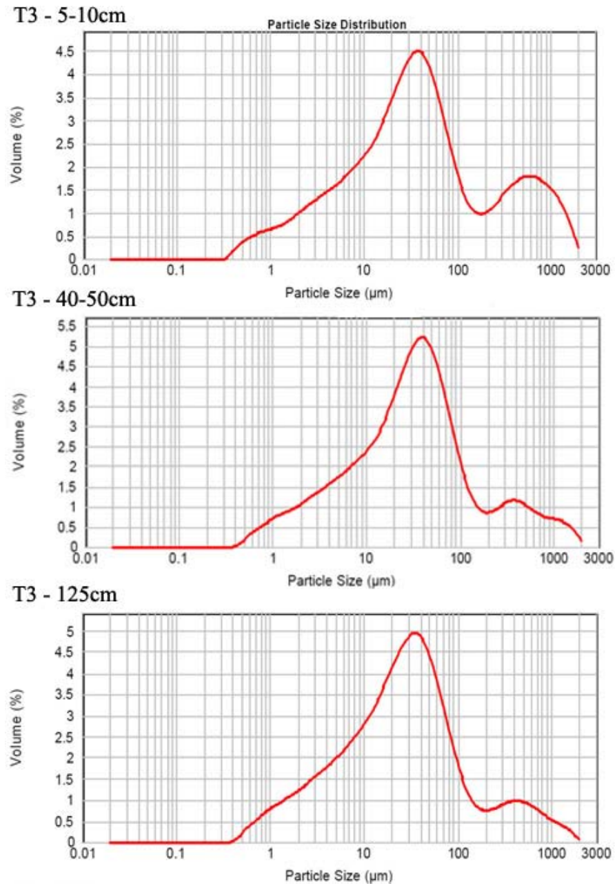
Figure 5.31 T3 particle size distribution curves for three samples taken at the surface, middle and base of the T3 deposit.
