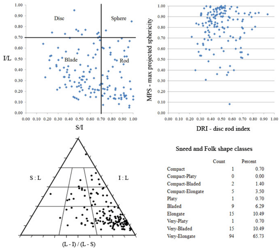
Figure 5.35 T3 particle shape indices.
