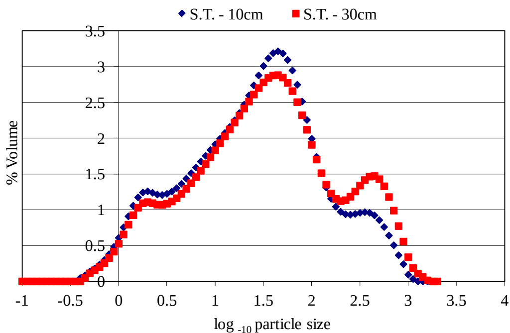
Figure 6.9 S.T. combined particle size distribution curves.
