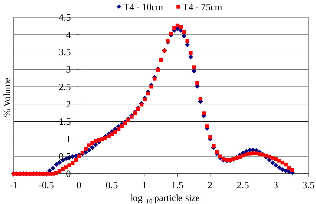
Figure 5.46 T4 combined particle size distribution curves. Stated sample depths are relative to deposit surface. The x-axis is a log scale.
