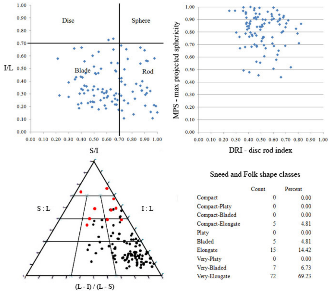
Figure 6.11 S.T. particle shape indices. The red points on the Sneed & Folk diagram represent natural clasts collected during excavation. The natural clasts are not included in the shape class table.
