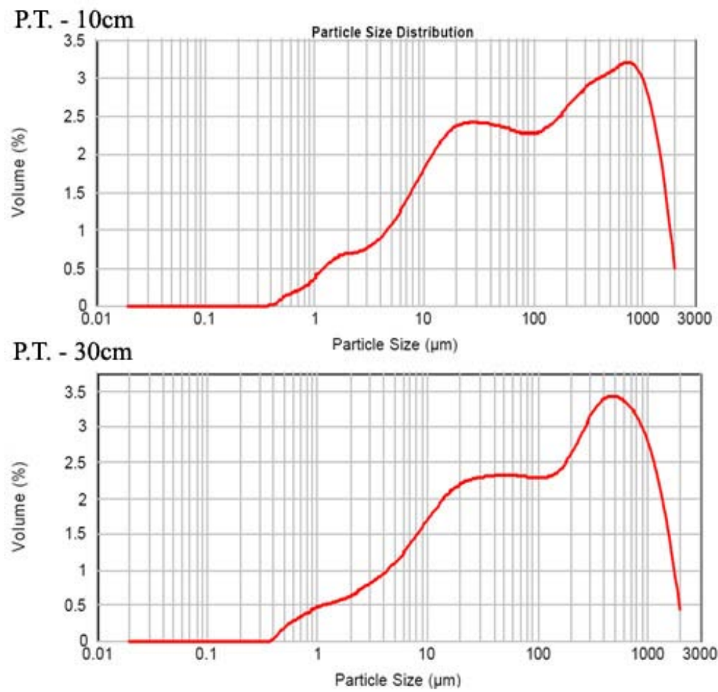
Figure 6.20 P.T. particle size distribution curves for two samples taken at top of the deposit and base of the excavation.
