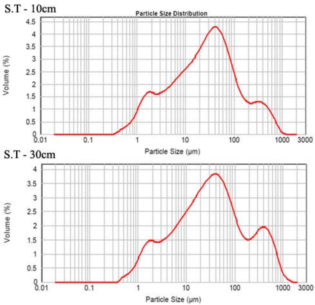
Figure 6.8 S.T. particle size distribution curves for two samples taken at upper and base of the matrix-supported sediments in the Secondary Talus deposit.
