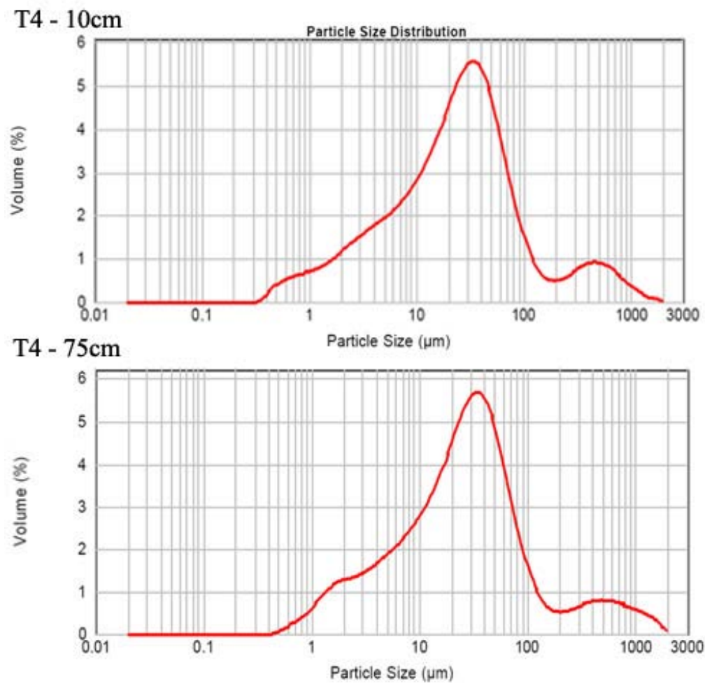
Figure 5.45 T4 particle size distribution curves for two samples taken at the surface and lowest point reached in the T4 deposit.
