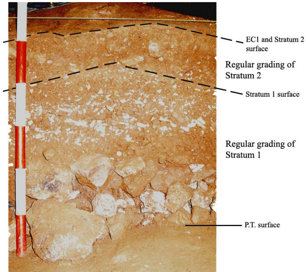
Figure 6.5 S.T. eastern wall excavation profile. The consolidated surface of the P.T. ( Facies 0 ) can be seen at the base of the picture. The staff segments measure 10cm.
