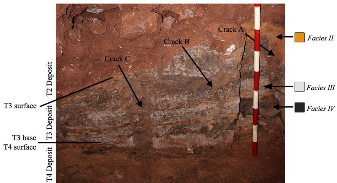
Figure 5.28 STK-MH1 eastern wall profile of T2, T3 and T4. The three main cracks A, B and C are labelled. The facies described in the text are also indicated. The segments on the range staff measure 10cm.
