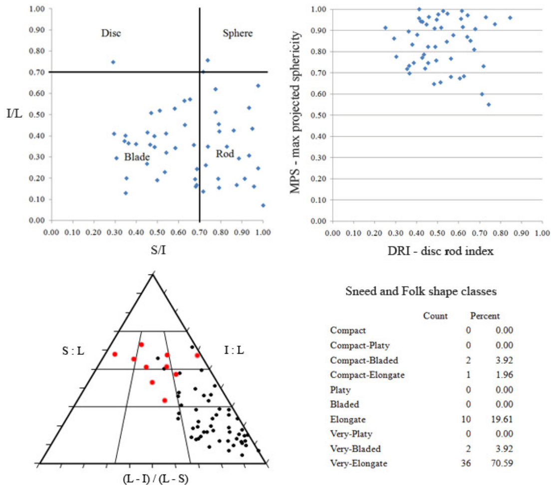
Figure 5.19 T2 particle shape indices. The red points on the Sneed & Folk diagram represent natural clasts excavated from the T2 deposit. The natural clasts are not included in the shape class table.
