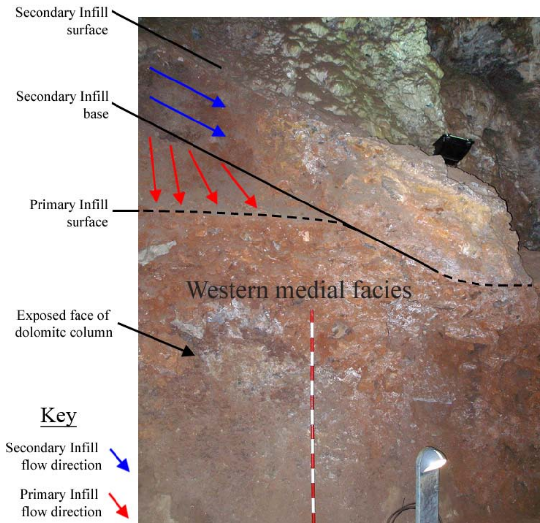
Figure 7.15 STK-MH2 truncated profile showing the western medial facies, the Primary Infill surface and the Secondary Infill boundaries. The arrows represent the different sediment flow directions in each deposit. The range staff segments measure 10cm.
