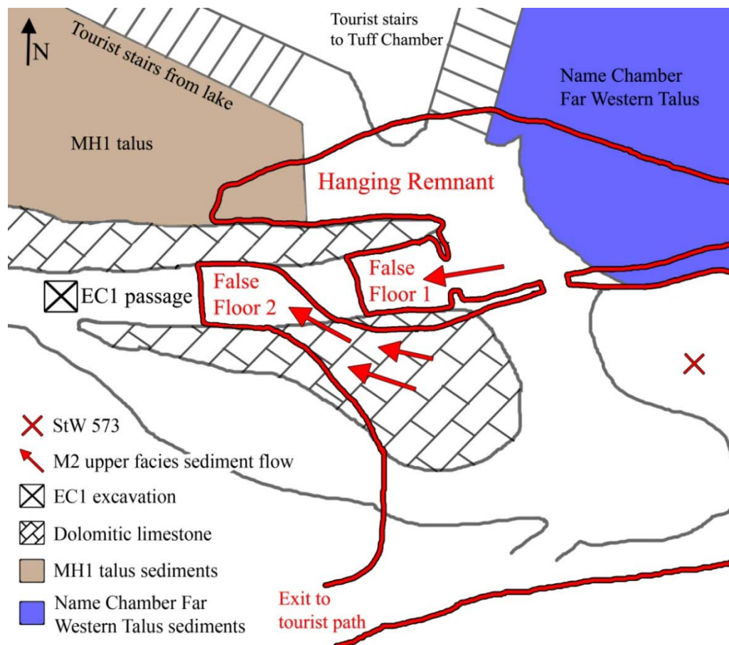
Figure 6.3 Schematic plan view of the Silberberg Grotto sediments exiting the Silberberg Grotto chamber into the EC1 passage, forming two false floor breccia bodies. The Red line represents the limits of the Silberberg Grotto and the current limits of the M2 sediments. The grey line represents the cave morphology of the underlying chambers and passages. The general sediment flow trend creating the false floors found in the EC1 passage is illustrated. Diagram is not to scale.
