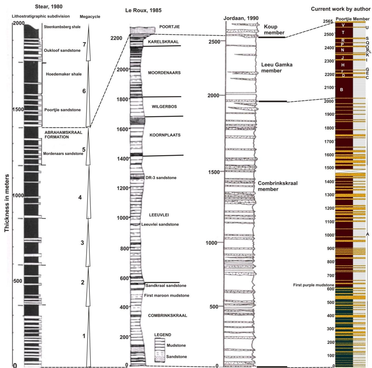
Figure 5.1: Comparison of Stear (1980), Le Roux, 1985, Jordaan (1990) and current work by author.
