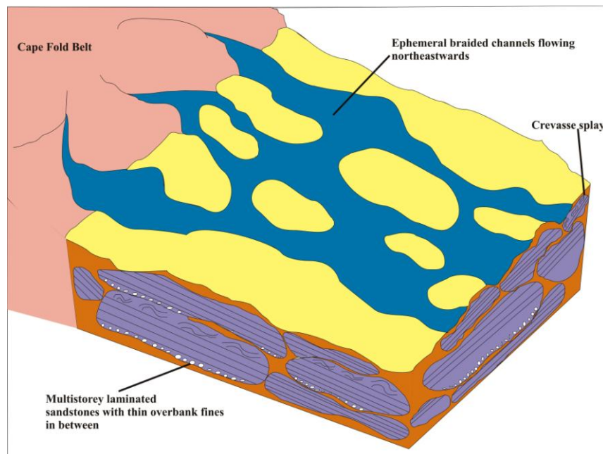
Figure 5.2: Palaeoenvironmental reconstruction of the Abrahamskraal Formation from the Ecc-a-Beaufort contact to the top of arenaceous unit A (0-2075m). Braided palaeoenvironment affected by the Cape Orogeny resulting in a high energy depositional environment leading to the formation of thick sandstone beds with less mudstone interbeds (drawing modified from Tucker, 2011).
