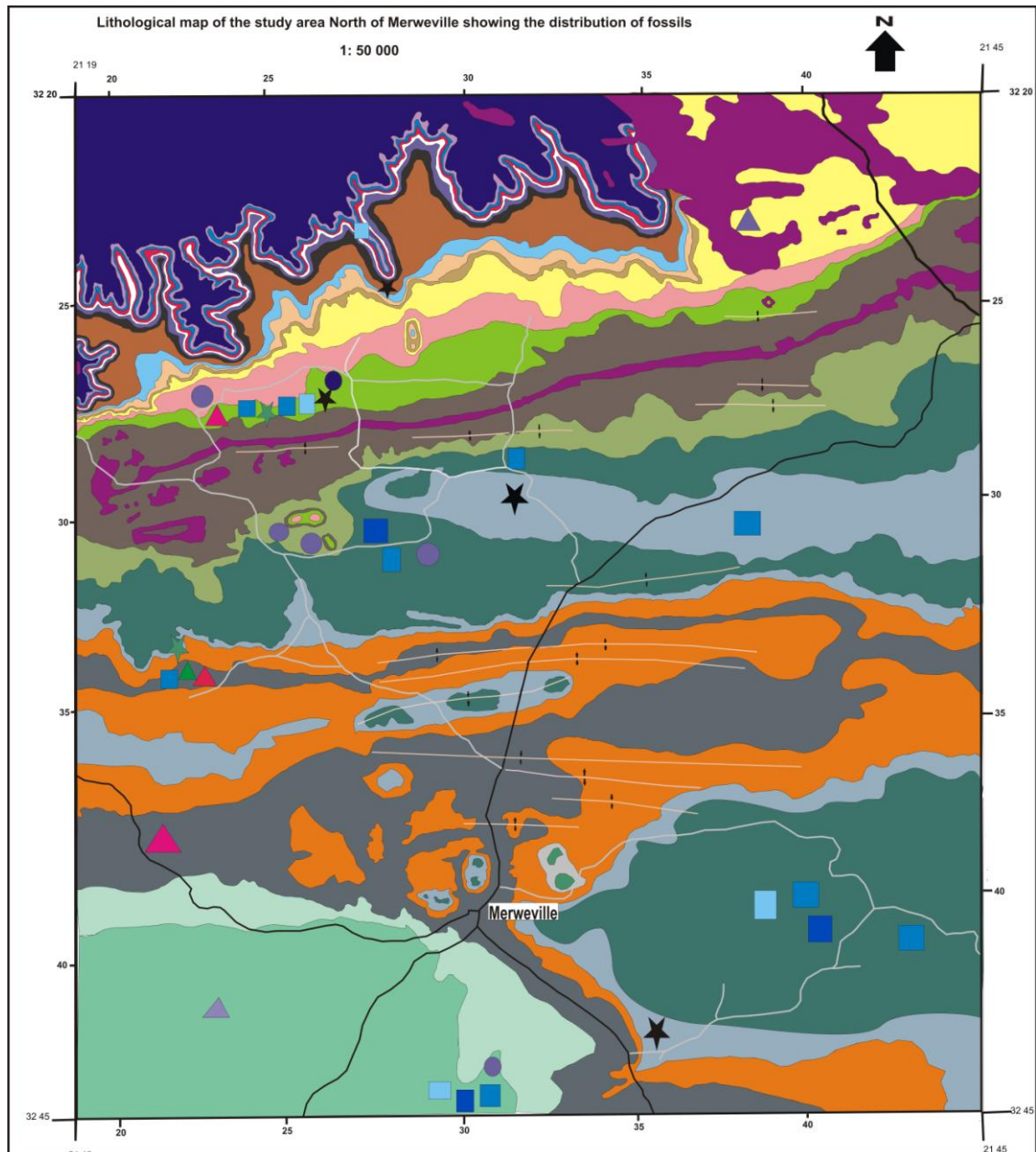
Figure 3.1c: Lithological map of the study area from Merweville up to the base of the Poortjie Member at the Escarpment. Fossil localities are also included. Legend on Figure 3.1b.
