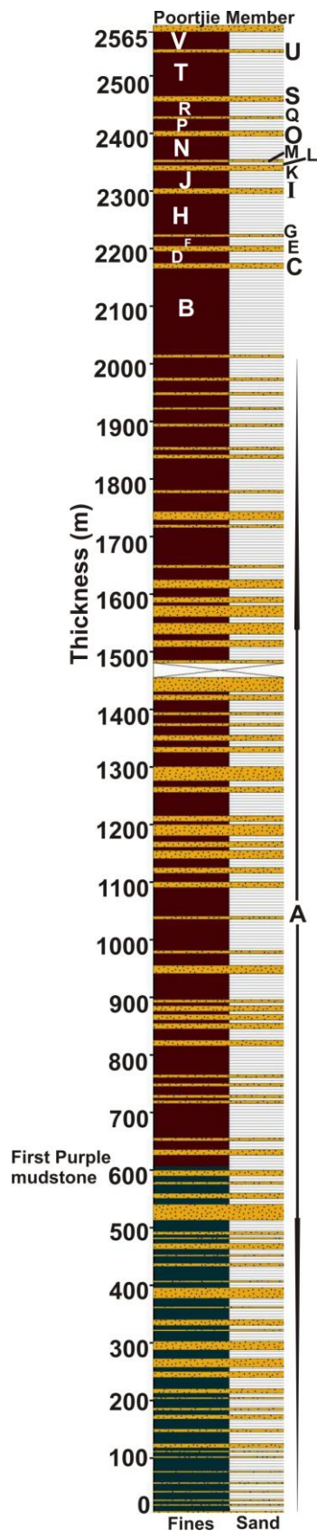
Figure 3.1a: Simplified stratigraphic section of the Abrahamskraal Formation in the study area showing different lithological units coded A-U. See Appendix A for a comprehensive stratigraphic section.
