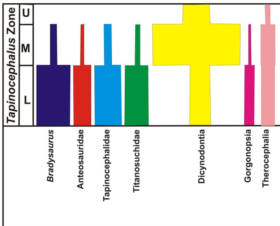
Figure 1.4: Biostratigraphic scheme of Boonstra (1969) showing a threefold subdivision of the Tapinocephalus biozone into Lower, Middle and Upper subdivisions) and illustrating relative numbers of various taxa during Tapinocephalus Zone times.
