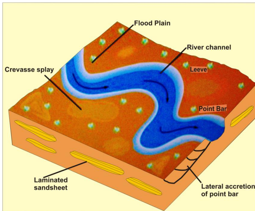
Figure 5.3: Palaeoenvironmental reconstruction of the stratigraphic succession from mudstone B till the base of the Poortjie Sandstone (2075m- 2565m). This was a meandering fluvial environment with thicker overbank fines relative to sandstone units. (drawing modified from Tucker, 2011).
