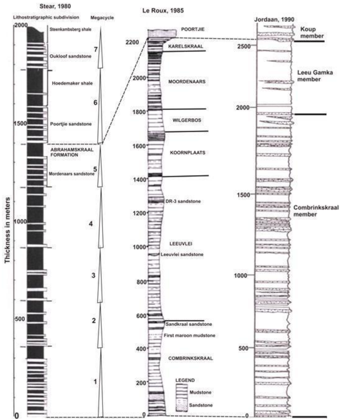
Figure 1.3: Comparison of the lithostratigraphic schemes for the Abrahamskraal Formation Stear 1980: (section measured in the Moordenaarskaro); Le Roux, 1985: (section measured north of Merweville); & Jordaan's 1990: (section measured on the farm Combinkskraal, south of Leeu Gamka).
