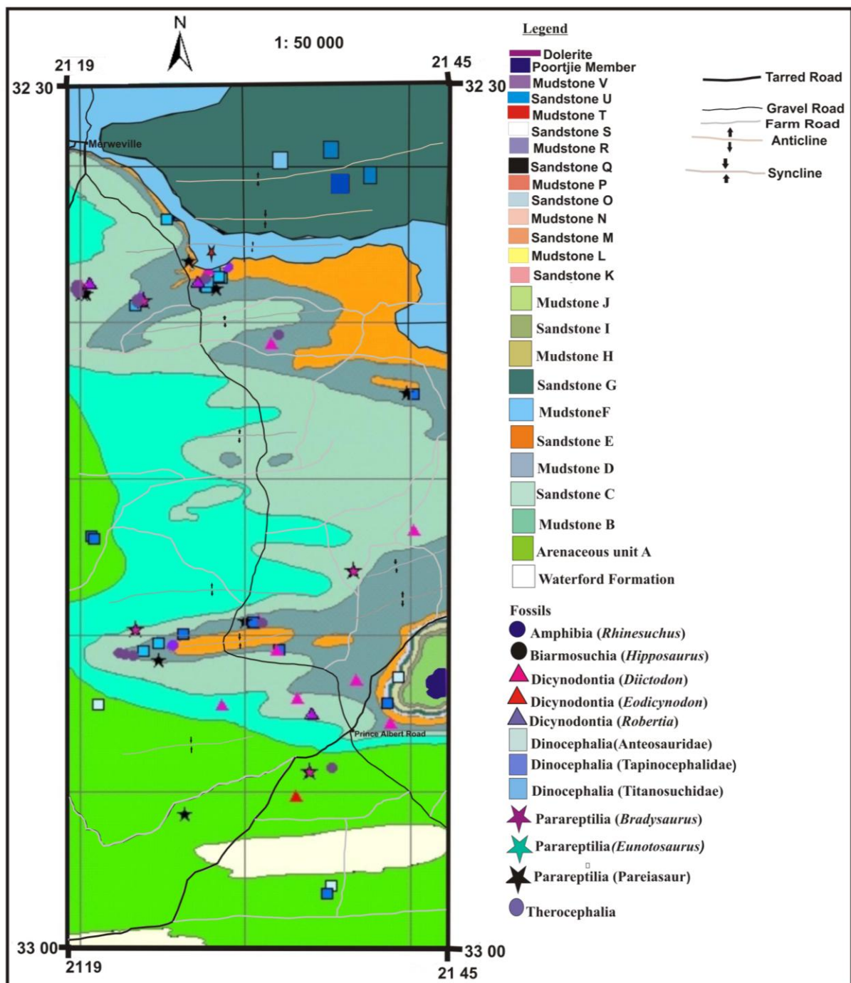
Figure 3.1b: Lithological map from the Eccra – Beaufort contact near Prince Albert Road till sandstone G at Merweville. The map also shows the distribution of different fossil taxa. (Scale 1: 50 000)
