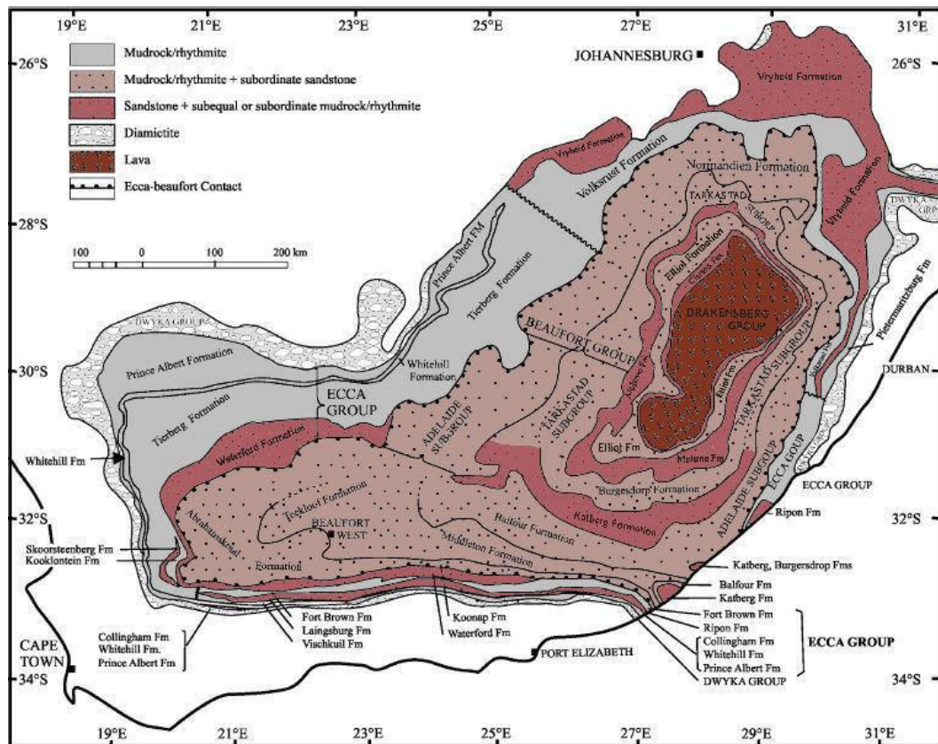
Figure 1.1: Map of the lithostratigraphic units of the Karoo Supergroup of South Africa (after Catuneanu et al. , 2005).
