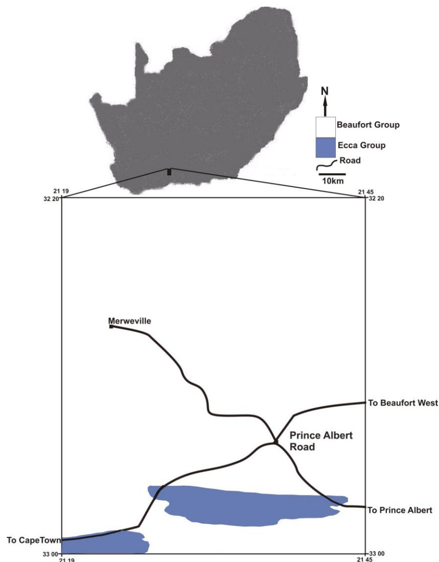
Figure 2.1: The position of the study area in the context of South Africa. The sketch is drawn from the 1:50 000 topographic maps of Dwyka, Prince Albert Road and Merweville and 1:250 000 Ladismith geological map.
