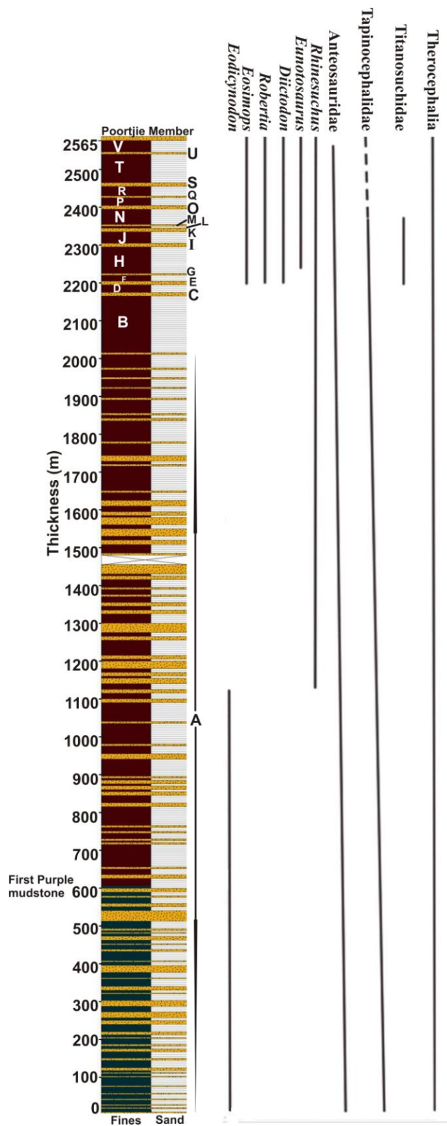
Figure 4.2: Stratigraphic section showing stratigraphic ranges of different fossil taxa in the study area. A-U represents the lithological units. Red colour denotes areas in the stratigraphic column where maroon mudrocks may occur, the green shows the portion of the stratigraphic column where no maroon mudrocks are present.
