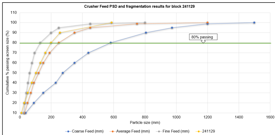
Figure 4.3: Crusher feed PSD guideline and fragmentation results for block 241129
