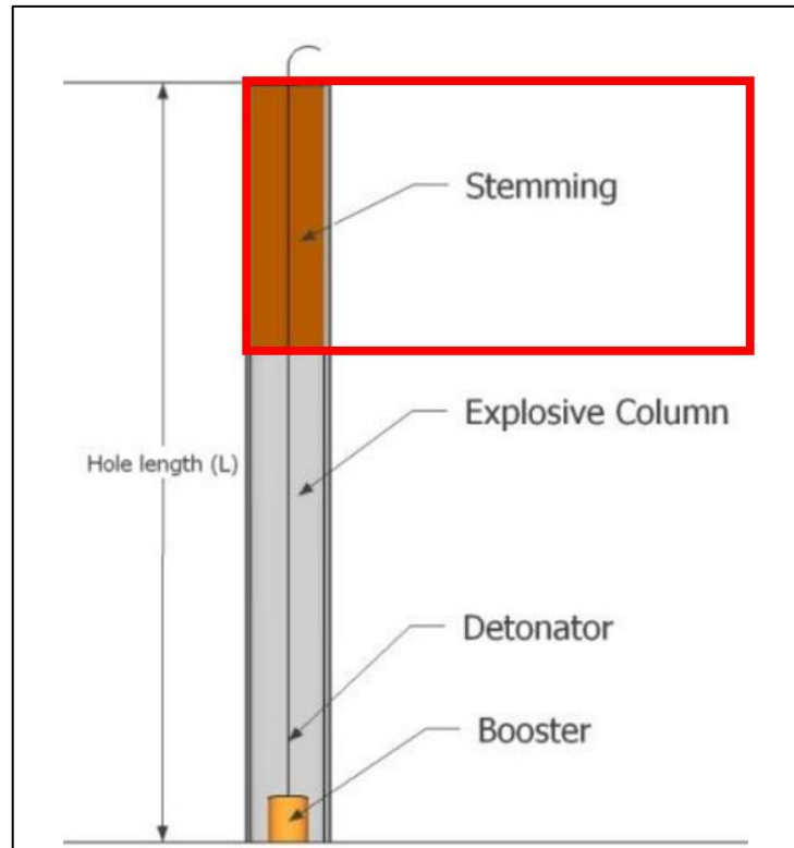
Figure 2.6: Illustration of stemming relative to an explosive column and blasthole length
