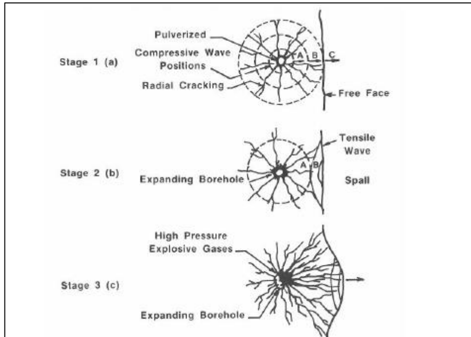
Figure 2.2: Gas expansion theory
