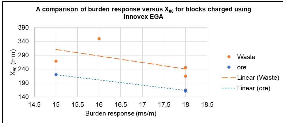
Figure 4.11: A comparison of burden response versus X_{80} for ore and waste blocks charged using Innovex EGA
