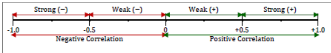
Figure 3.1: Spectrum for interpreting correlation coefficients
