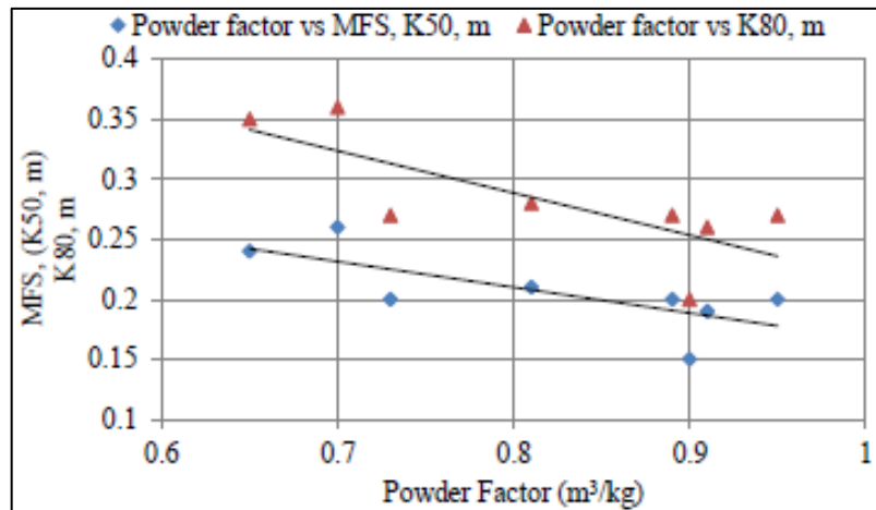
Figure 2.7: Relationship between rock fragment sizes and powder factor for a mine in India
