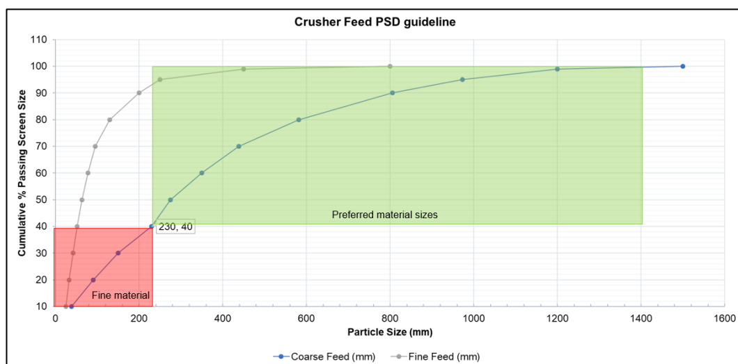
Figure 1.4: Crusher feed particle size distribution guideline
