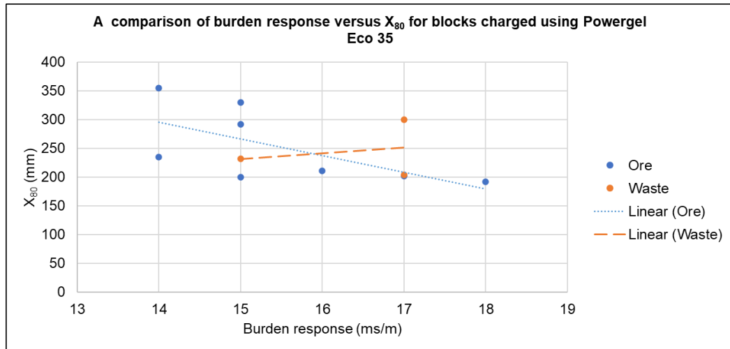
Figure 4.10: A comparison of burden response versus X_{80} for ore and waste blocks charged with Powergel Eco 35
