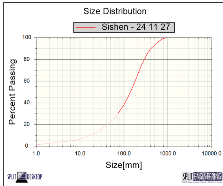
Figure 3.4: Fragmentation size distribution curve for block 241127
