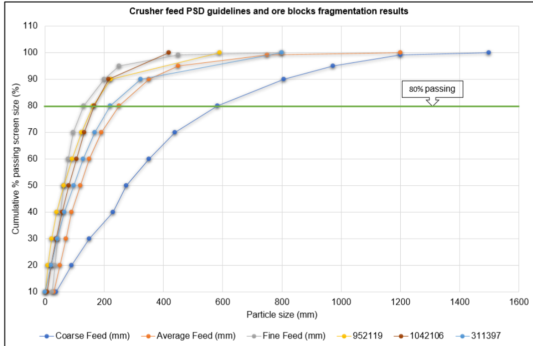
Figure 4.2: Crusher feed PSD guidelines and ore blocks fragmentation results for ore blocks charged using Innovex EGA
