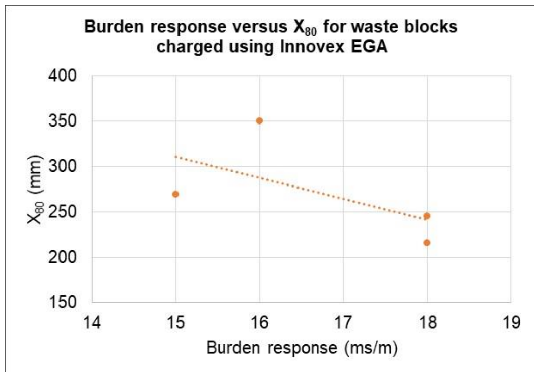
Figure 4.9: Burden response versus X 80 for waste blocks charged using Innovex EGA
