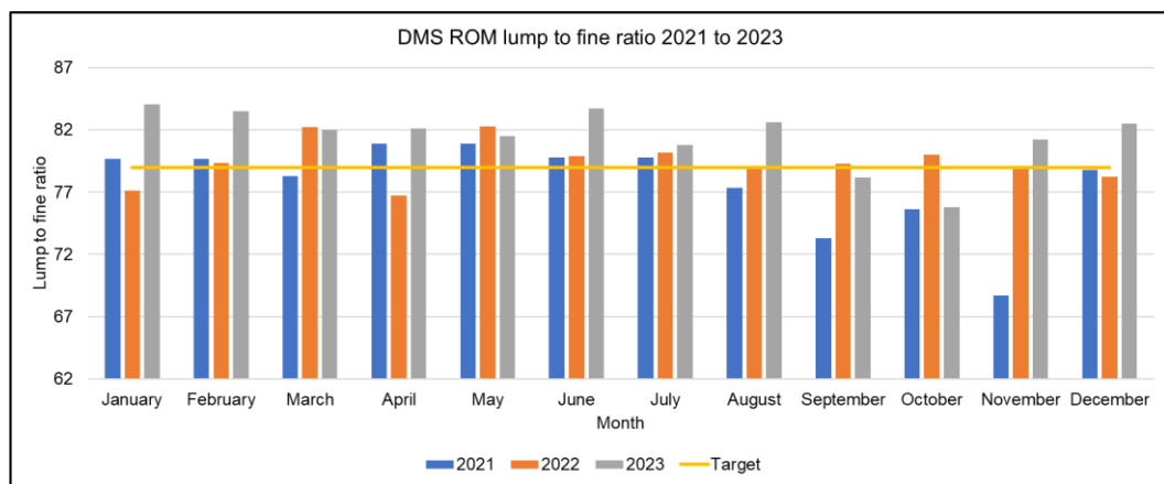
Figure 4.14: DMS ROM lump to fine 2021 to 2023
