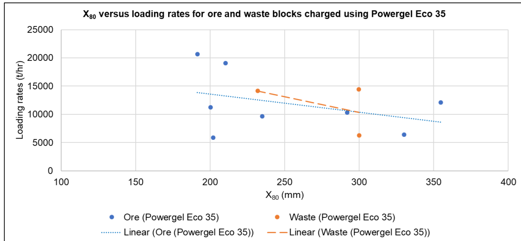
Figure 4.12: X_{80} versus loading rates for ore and waste blocks charged using Powergel Eco 35
