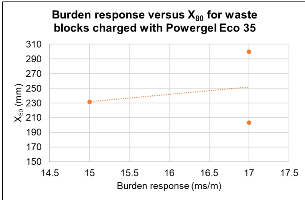
Figure 4.8: Burden response versus X_{80} for waste blocks charged using Powergel Eco 35
