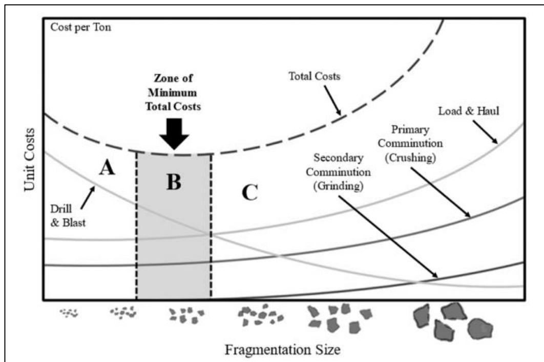
Figure 2.4: Relationship between fragmentation size and mining operational costs
