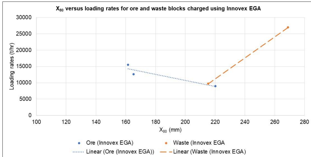
Figure 4.13: X_{80} versus loading rates for ore and waste blocks charged using Innovex EGA
