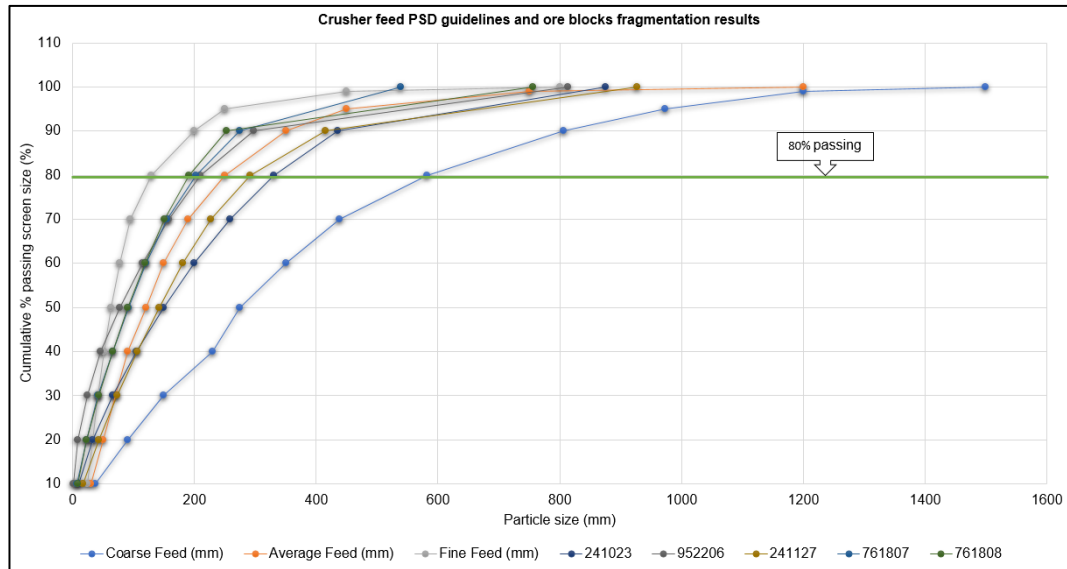
Figure 4.1: Crusher feed PSD guidelines and ore blocks fragmentation results for ore blocks charged using Powergel Eco 35
