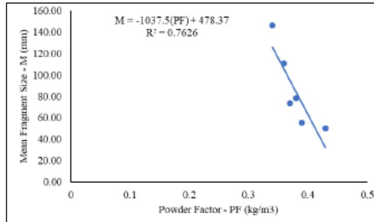
Figure 2.8: Relationship between rock fragment sizes and powder factor for a limestone quarry (Source: Shehu, et al. , 2020)
