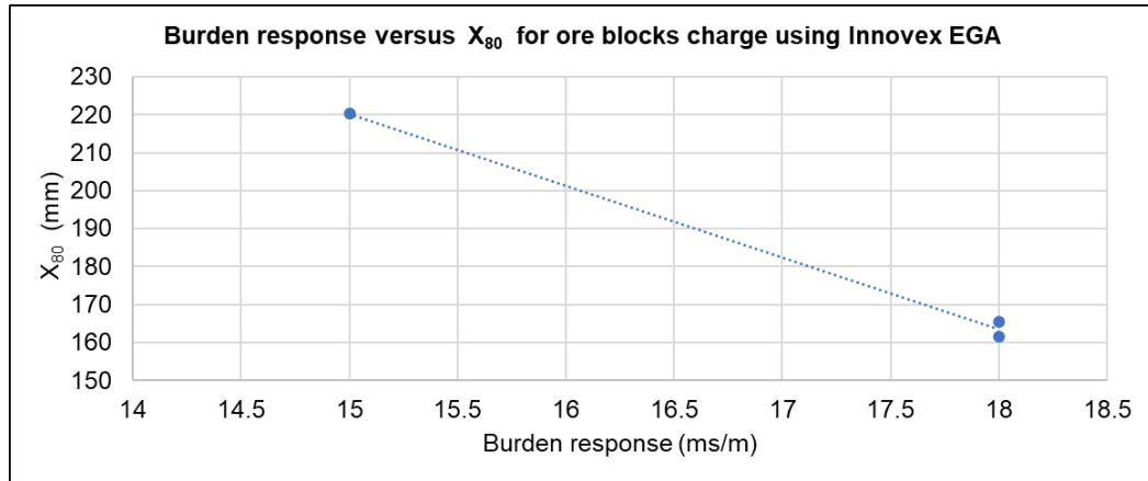
Figure 4.6: Burden response versus X_{80} for ore blocks charged with Innovex EGA
