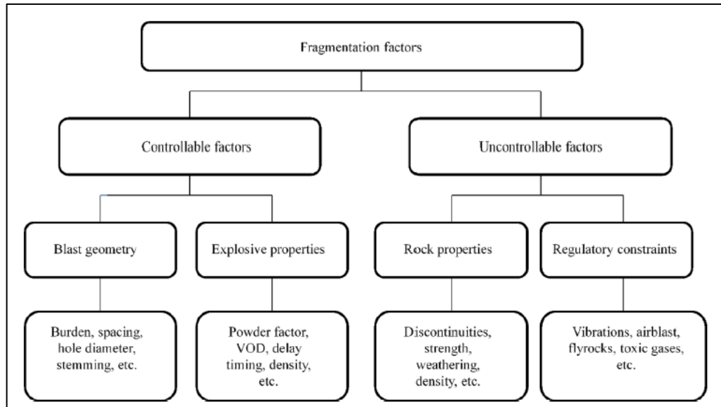
Figure 2.5: Factors that have an influence on fragmentation
