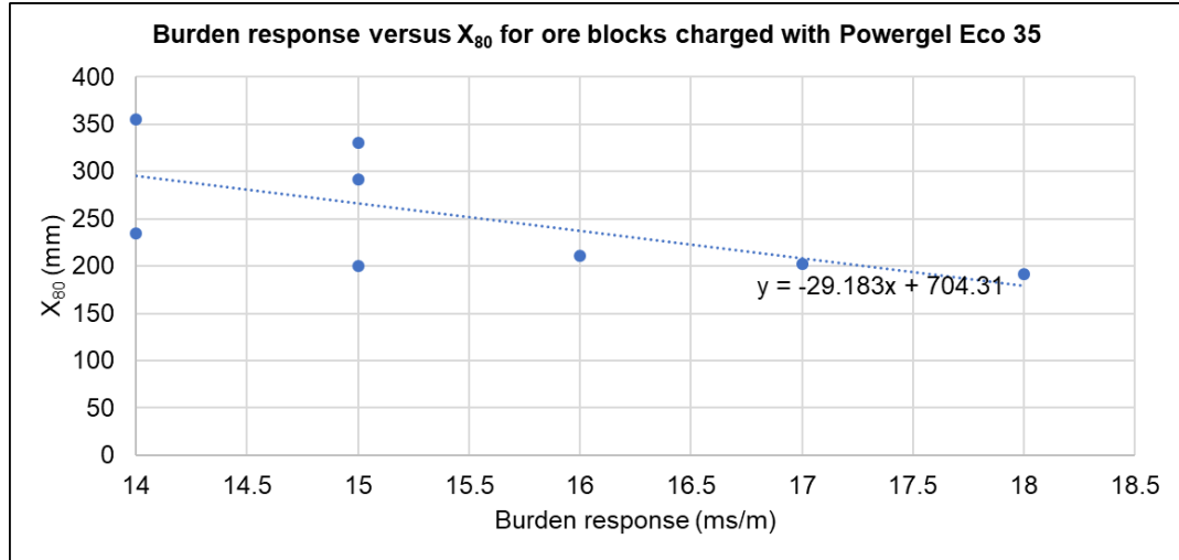
Figure 4.5: Burden response versus X_{80} for ore blocks charged using Powergel Eco 35
