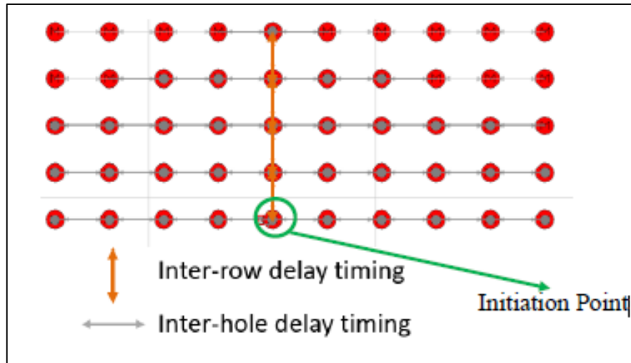
Figure 2.9: Inter-hole delay timing and inter-row delay timing
