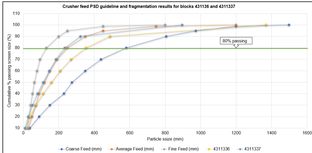
Figure 4.4: Crusher feed PSD guideline and fragmentation results for blocks 4311336 and 4311337
