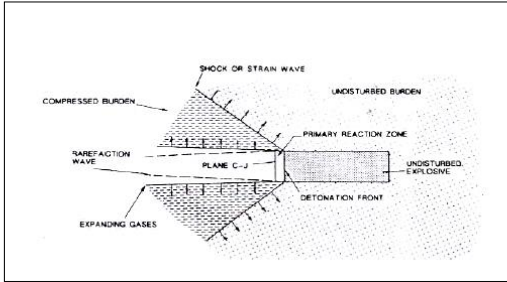
Figure 2.10: Detonation sequence showing Chapman-Jouguet Plane
