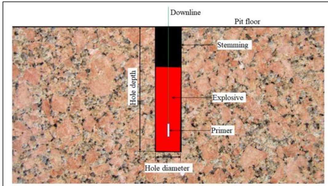
Figure 2.1: Section view illustration of a charged blasthole
