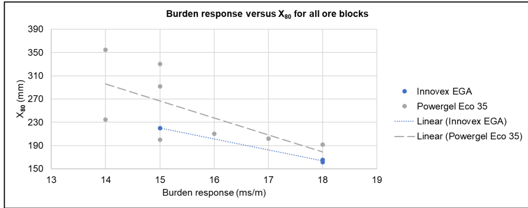
Figure 4.7: Burden response versus X_{80} for all ore blocks
