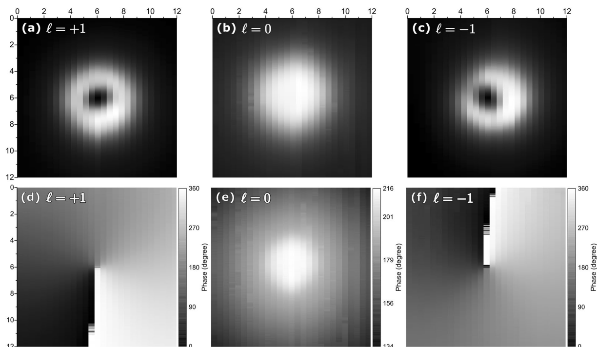
Figure 2. Intensity and phase maps of the acoustic fields generated by the 3D-printed acoustic spanner. (a–c) show the intensity maps for \ell = +1, 0, 1, -1 . The corresponding phase-maps are shown in (d–f). The x- and y-axes are measured in centimetres. Each vertical scan was taken at \approx 0.5 cm intervals.
