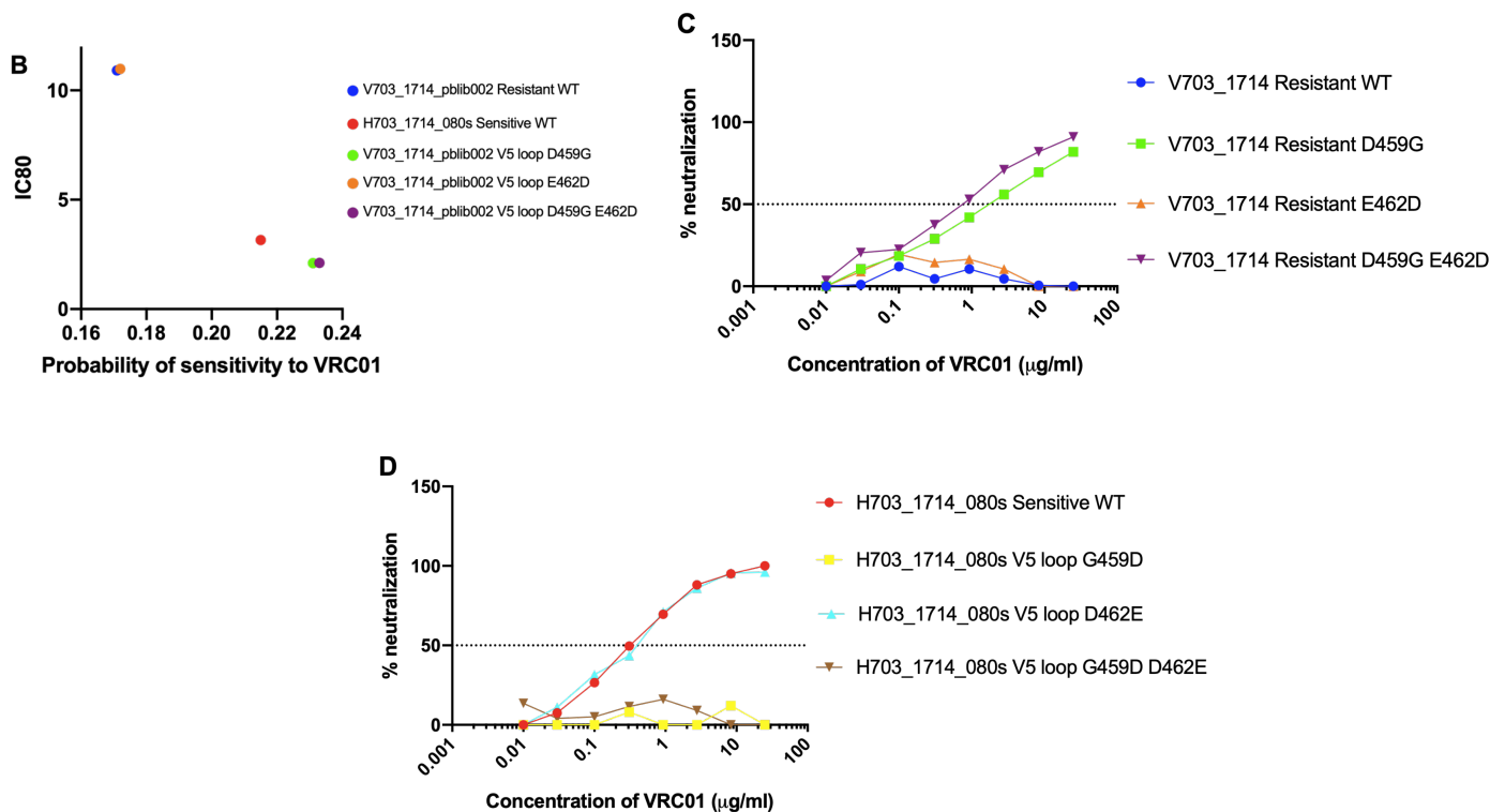
Figure 3.2.2. Results for PTID 703-1714. (A) Sequence alignment of Envs cloned from PTID 1714. Resistant WT (top) and sensitive WT (below). Regions of interest V1V2, Loop D, CD4 binding loop, CD4 contact and \beta 23 V5 loops are underlined in black. Black dots in the sensitive sequence represent an amino acid match to the resistant sequence. Dashes show a deletion in the sequence. Amino acids highlighted in grey represent mutation sites in regions responsible for
