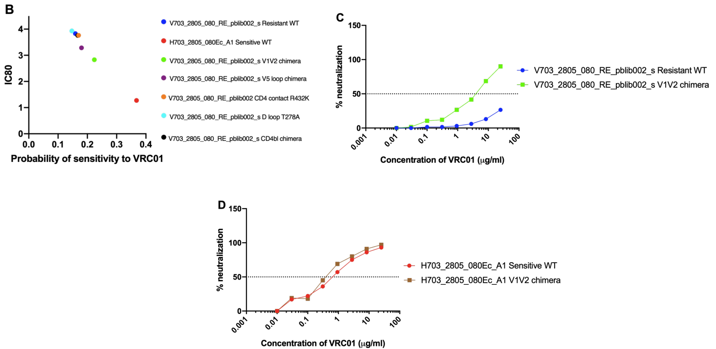
Figure 3.2.6. Results for PTID 703-2805. (A) Sequence alignment of Envs cloned from PTID 2805. Resistant WT (top) and sensitive WT (below). Regions of interest V1V2, Loop D, CD4 binding loop, CD4 contact and \beta 23 V5 loops are underlined in black. Black dots in the sensitive sequence represent an amino acid match to the resistant sequence. Dashes show a deletion in the sequence. Amino acids highlighted in blue represent PNGS that differ between sensitive and resistant viruses. The vertical grey line represents the end of gp120 and the start of gp41. (B) Correlation plots representing the machine learning-based predicted IC80 vs the predicted probability of sensitivity to VRC01 for the WTs and mutants in each set. The resistant WT is represented in blue, the sensitive WT is represented in red and the mutants are represented in
