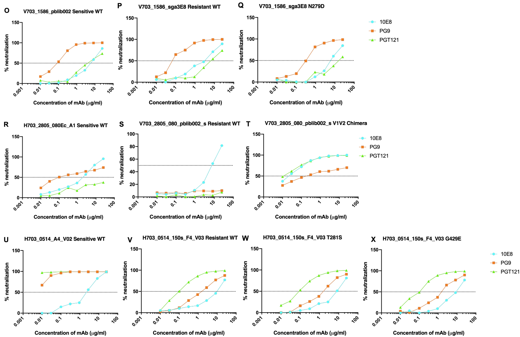
Figure 3.3.2. Overall neutralization curves of mutated viruses. Neutralization curves of (A-E) PTID 703-1714, (F-I) PTID 703-2769, (J-N) PTID 703-0510, (O-Q) PTID 703-1586, (R-T) PTID 703-2805 and (U-X) PTID 703-0514 sensitive and resistant WTs, and their respective mutants against mAbs showing the concentration of antibody needed to neutralize 50% of the virus. 10E8 in cyan, PG9 in orange and PGT121 in green.
