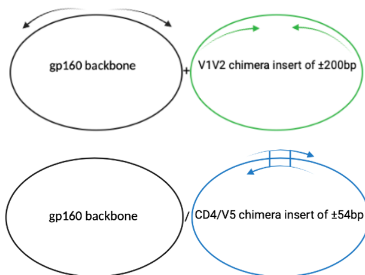
Figure 2.2. Representation of production of V1V2 and both CD4 and V5 chimeras.
