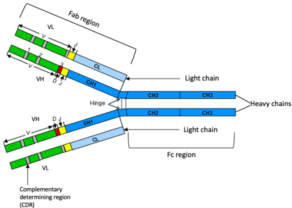
Figure 1.4. Structure of an antibody. Schematic representation showing the antibody consists of two heavy chains and two light chains. The constant regions for the heavy (CH1, CH2 and CH3) and light chains (CL) are shown in dark blue and light blue respectively, while the variable regions of the heavy (VH) and light (VL) chains, shown in green. The CDR found in the variable regions are seen by grey bars. The Fab region, consisting of the light chain, heavy chain variable region and one heavy chain constant region (CH1) and Fc region consisting of two heavy chain variable regions (CH2 & CH3) are indicated. (Adapted from Lefranc and Lefranc, 2020).
