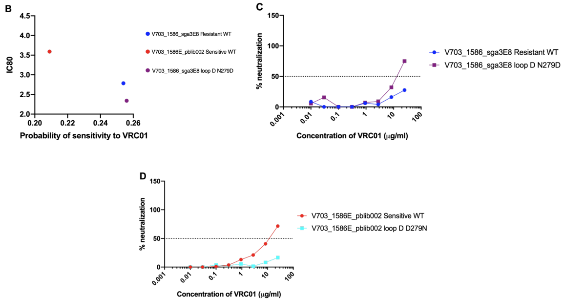
Figure 3.2.5. Results for PTID 703-1586. (A) Sequence alignment of Envs cloned from PTID 1586. Resistant WT (top) and sensitive WT (below). Regions of interest V1V2, Loop D, CD4 binding loop, CD4 contact and \beta 23 V5 loops are underlined in black. Black dots in the sensitive sequence represent an amino acid match to the resistant sequence. Dashes show a deletion in the sequence. Amino acids highlighted in grey represent the mutation site of interest in regions responsible for conferring resistance to VRC01. The vertical grey line represents the end of gp120 and the start of gp41. (B) Correlation plots representing the machine learning-based predicted IC80 vs the predicted probability of sensitivity to VRC01 for the WTs and mutants in each set. The resistant WT is represented in blue, the sensitive WT is represented in red and the mutants are represented in the remaining colours.(C) Neutralization curves of the resistant WT and mutant viruses representing the concentration of VRC01 needed to neutralize 50% of the virus. (D)
