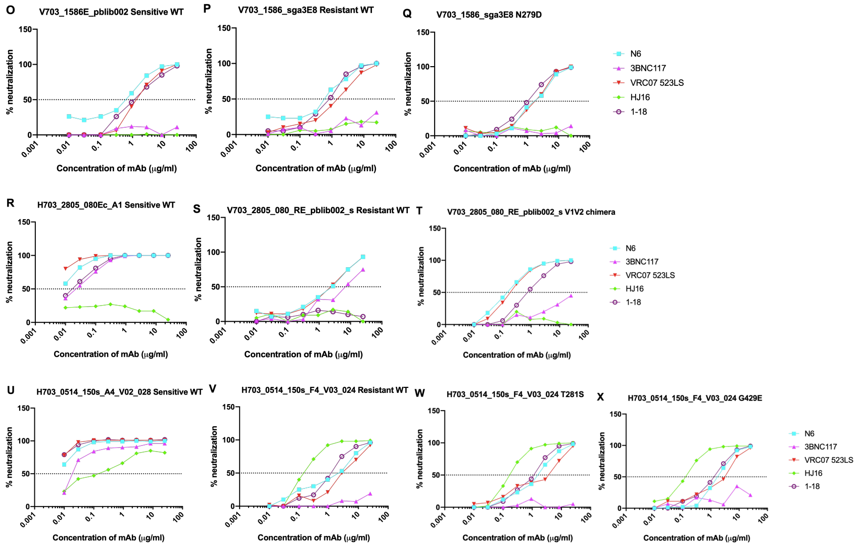
Figure 3.4.2. Neutralization curves of mutated viruses against other CD4 binding site mAbs. Neutralization curves of (A-E) PTID 703-1714, (F-I) PTID 703-2769, (J-N) PTID 703-0510, (O-Q) PTID 703-1586, (R-T) PTID 703-2805 and (U-X) PTID 703-0514 sensitive and resistant WTs, and their respective mutants against mAbs showing the concentration of antibody needed to neutralize 50% of the virus. N6 in cyan, 3BNC117 in magenta, VRC07-523 LS in red, HJ16 in green and 1-18 in purple.
