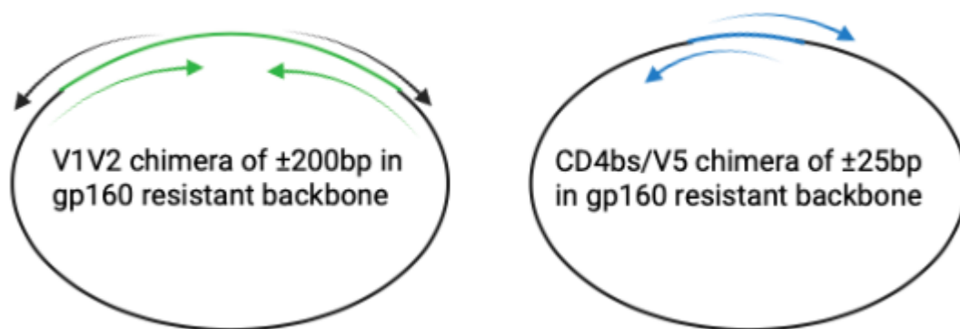
Figure 2.3. Representation of introduction of V1V2 and both CD4 and V5 chimeras in desired backbone.
