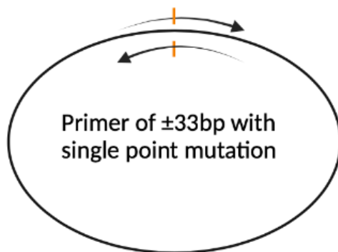
Figure 2.1. Representation of introduction of single mutations via SDM.
