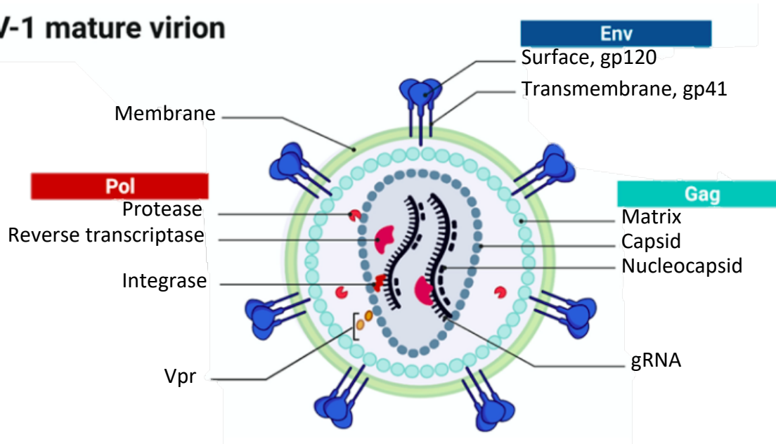
Figure 1.2. HIV-1 mature virion. Structural representation of a mature HIV-1 virion. The Env, made up of the gp120 and gp41 subunits, is embedded in the membrane. The protease and capsid are found in the matrix. The capsid contains the integrase, reverse transcriptase, viral genome and nucleocapsid. (Adapted from van Heuvel et al. , 2022).
