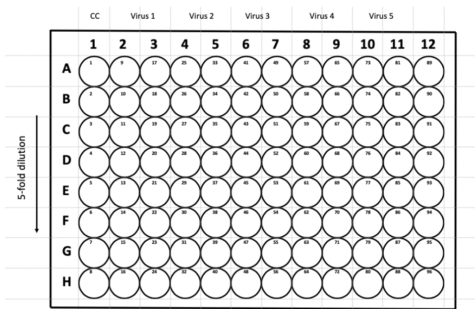
Figure 2.5. Schematic of TCID50 assay plate set-up. Column 1 is the cell control. The viruses are added in duplicate from column 2-11 along row A. A 5-fold serial dilution was made for each column from row A-H.
