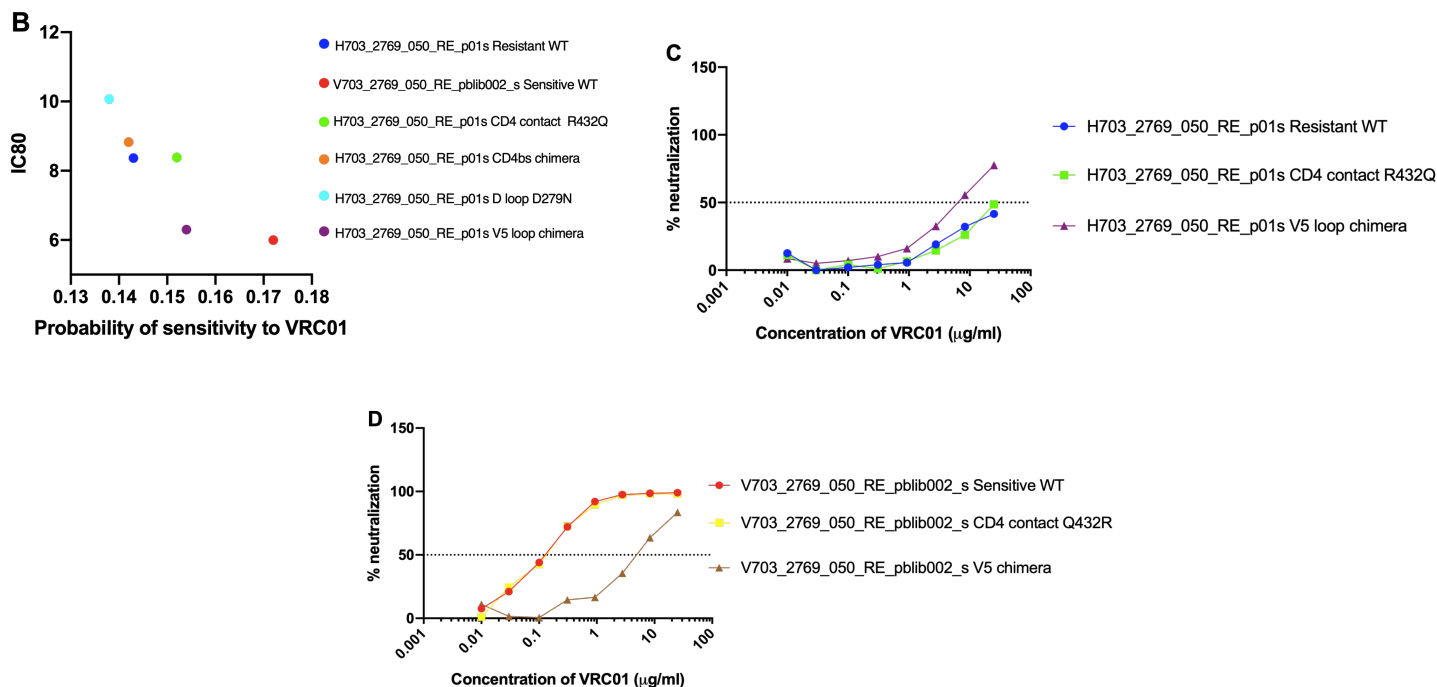
Figure 3.2.3. Results for PTID 703-2769. (A) Sequence alignment of Envs cloned from PTID 2769. Resistant WT (top) and sensitive WT (below). Regions of interest V1V2, Loop D, CD4 binding loop, CD4 contact and β23 V5 loops are underlined in black. Black dots in the sensitive sequence
