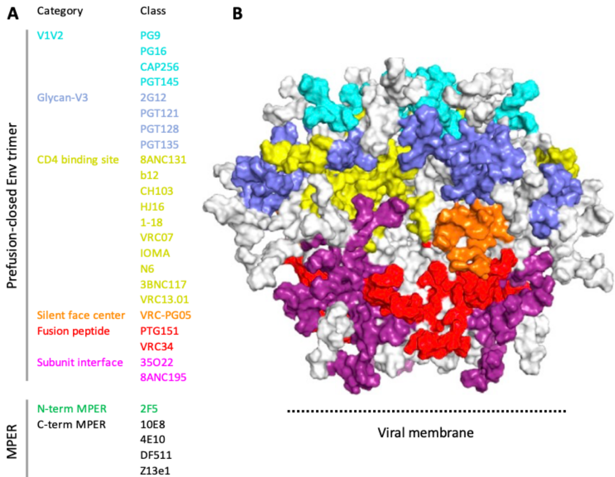
Figure 1.6. An HIV-1 viral envelope glycoprotein showing the epitopes of bNAbs. (A) The category defines the region of the Env glycoprotein that is recognised by the bNAb, and the class shows specific bNAbs coloured by epitope. (B) A visualization of the specific epitopes, corresponding to the colours seen in A, on the molecular surface of the virus. (Adapted from Kwong and Mascola, 2018).
