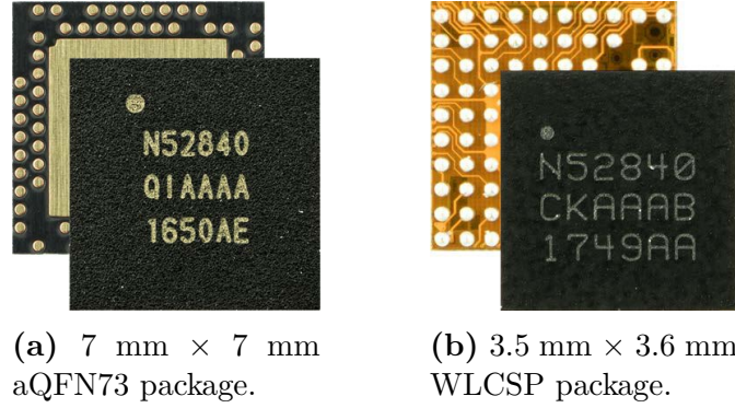
Figure 3.1: Nordic Semiconductor’s a) aQFN73 and b) WLCSP nRF52840-SoC capable of running advanced multi-protocol Bluetooth 5, Thread and ZigBee wireless technologies on a single chip [45].
