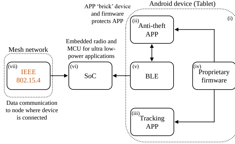
Figure 1.5: Block diagram of proposed HTEL anti-theft solution illustrating main technology systems.
