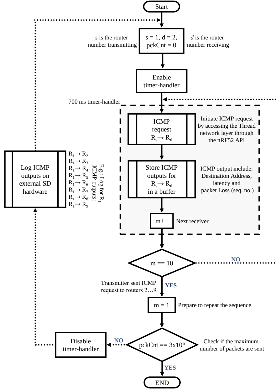
Figure 3.6: Router R_s \rightarrow R_d packet request and logging algorithm.
