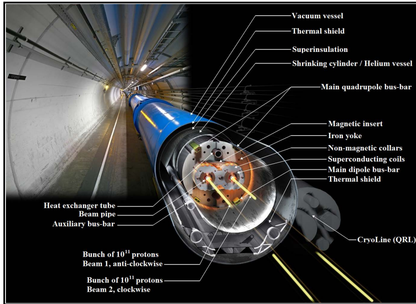
(b) Superconductor magnet electro-mechanical view.
