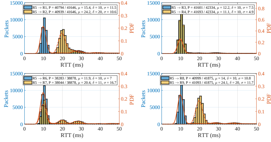
(a) Router R_5 RTT distributions within 3\sigma .
