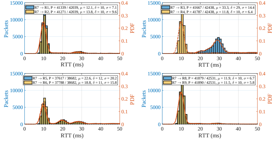
(a) Router R_7 RTT distributions within 3\sigma .
