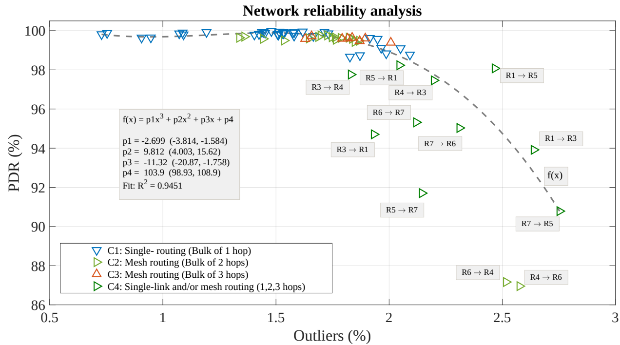
Figure 4.11: Mesh network route reliability by regression analysis.
