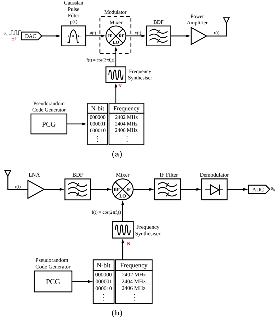
Figure 2.6: Conceptual heterodyne a) modulation of binary data s[k] to generate r(t) and b) demodulation of analog signal r(t) to generate s[k] .
