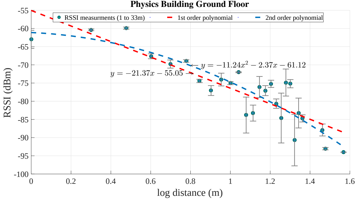
Figure 3.4: Log-distance modelling of RSSI versus \log_{10}(d) at T_x = 0 dBm.
