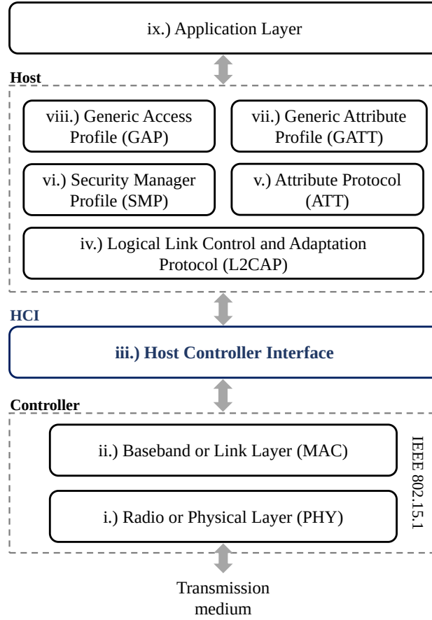
Figure 2.5: BLE protocol stack adapted from Townsend et al. [30, p.16].
