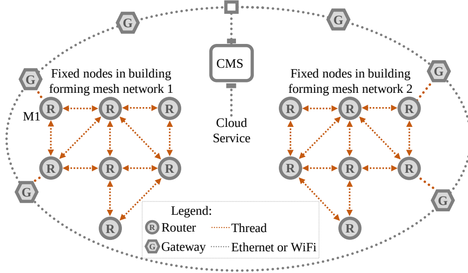
Figure 2.13: Thread network topology proposed for the HTEL anti-theft solution illustrating how multiple IEEE 802.15.4 [19] based mesh networks are connected through redundant gateways over the internet to a cloud service. The Thread end-device nodes are excluded from the network design.
