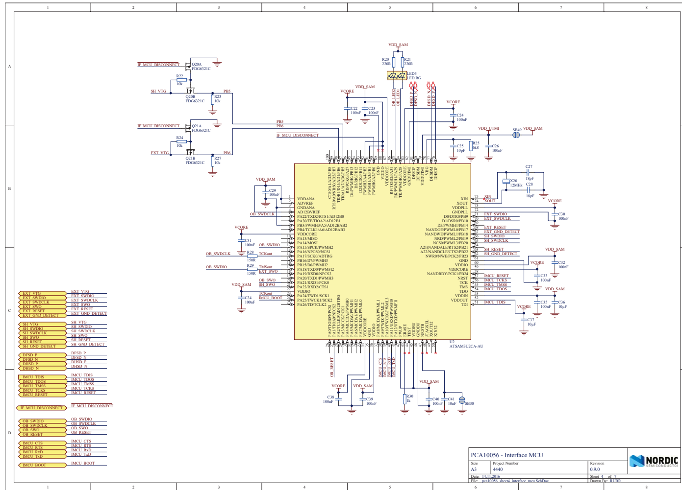
SCH II.4: PCA10056 - Interface MCU, page 4 of 7 [45].
