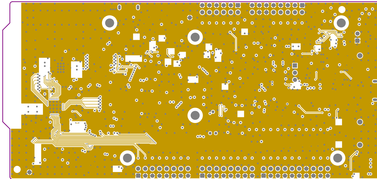
PCB II.2: nRF52840-DK mid-layer 1 [ 45 , 59 ].
