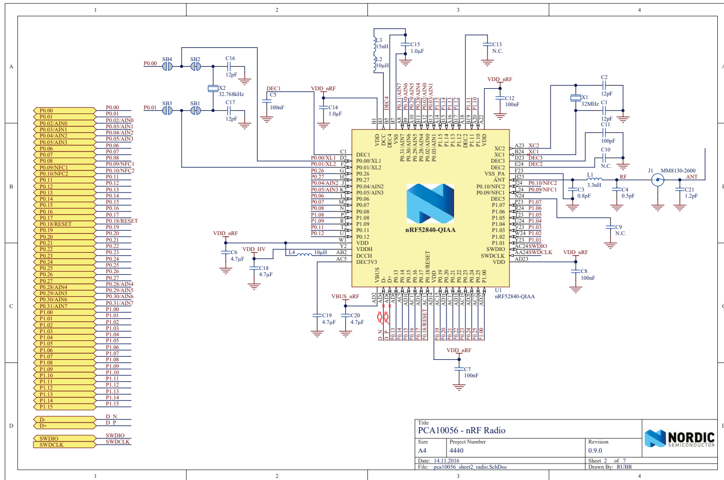
SCH II.2: PCA10056 - nRF52840 SoC, page 2 of 7 [45].
