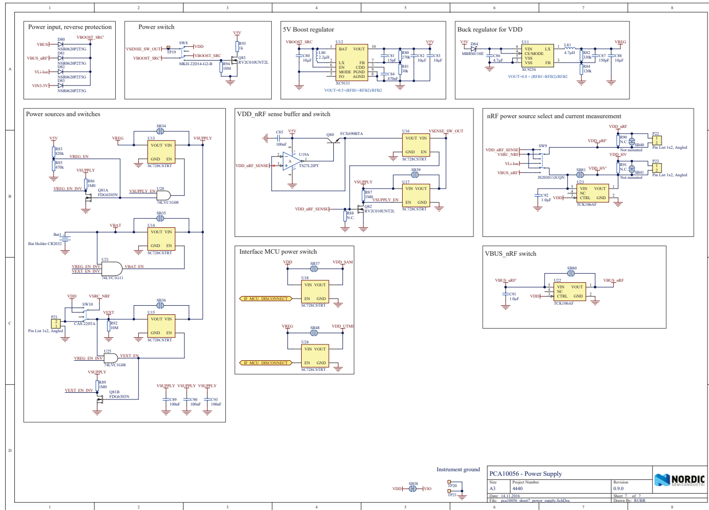
SCH II.7: PCA10056 - Power supply, page 7 of 7 [45].
