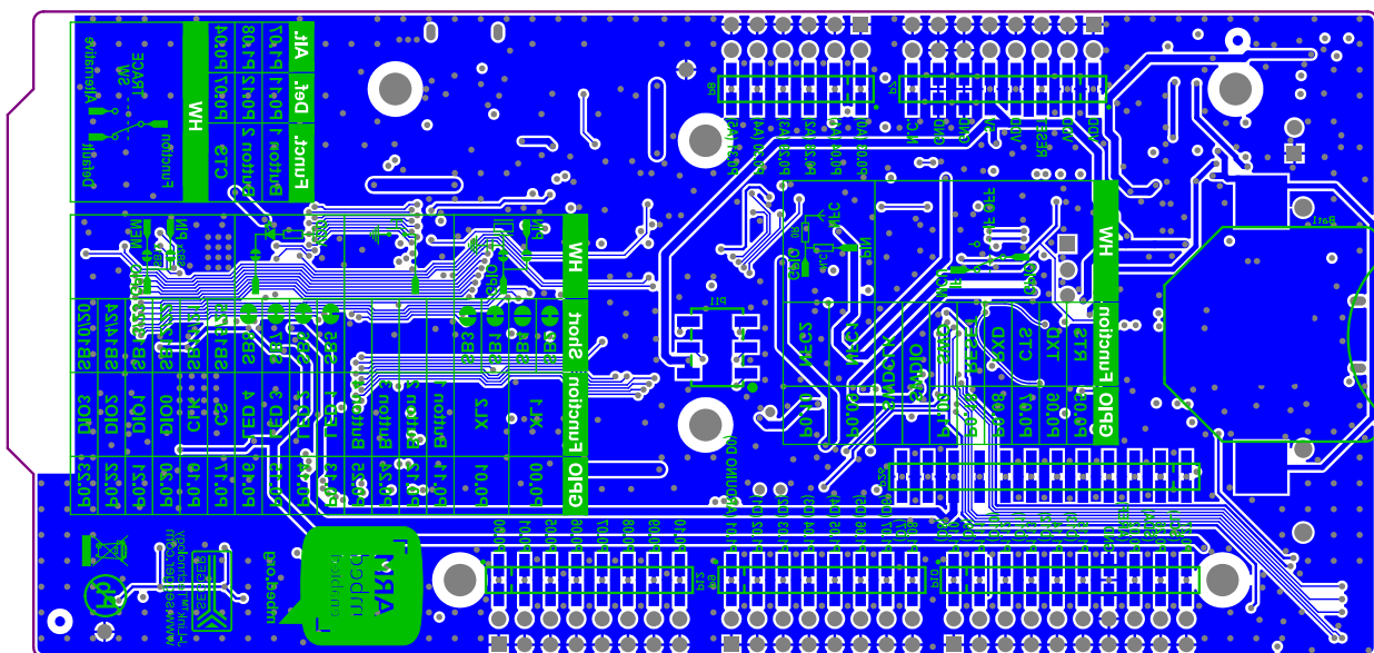
PCB II.4: nRF52840-DK bottom-layer [45, 59].
