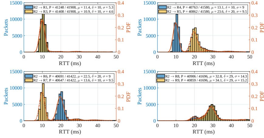
(a) Router R_2 RTT distributions within 3\sigma .
