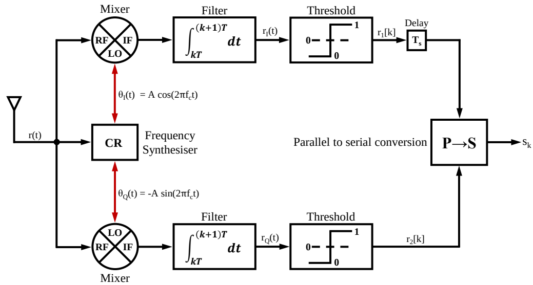
Figure 2.12: Conceptual O-QPSK demodulation modified from Xiong [32, p.181].
