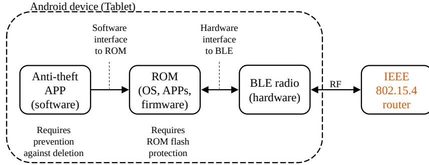
Figure 1.4: Block diagram illustrating hardware and software systems for data communications from an Android device to the nearest node in an IEEE 802.15.4 based mesh network.
