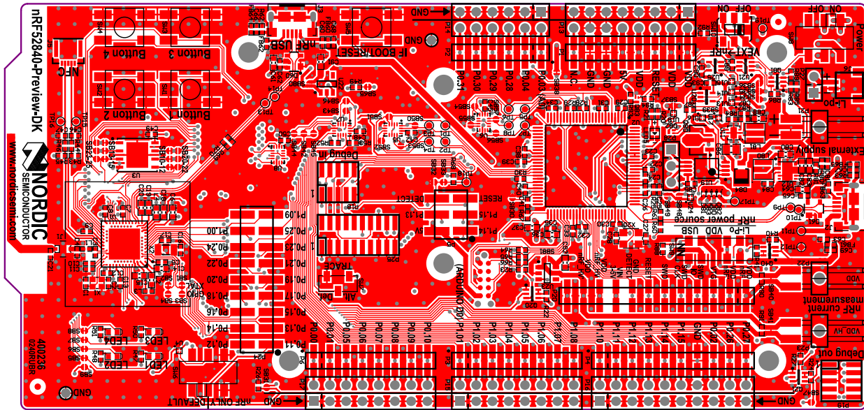
PCB II.1: nRF52840-DK top-layer [45, 59].
