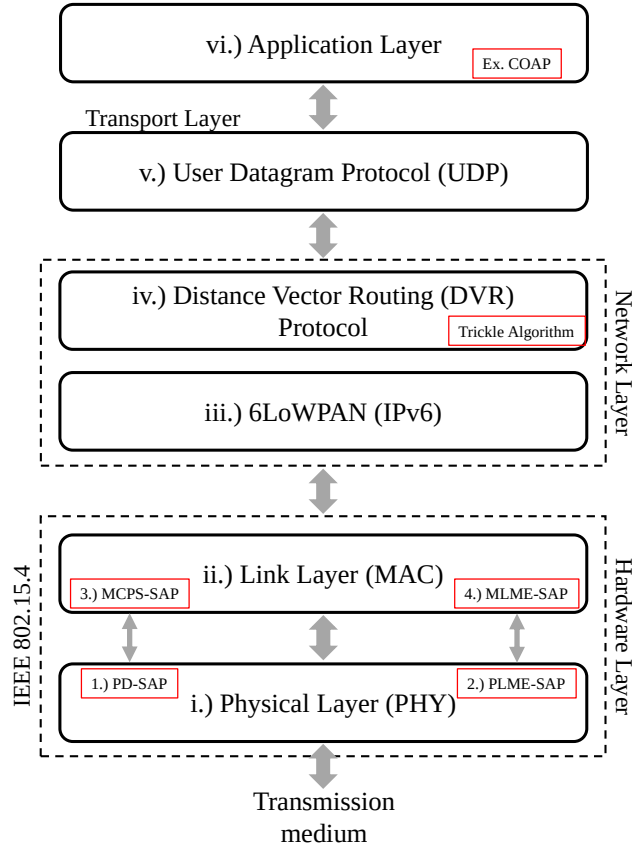
Figure 2.10: Thread protocol stack built on the IEEE 802.15.4 [19] hardware layer.
