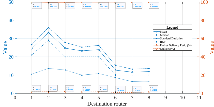
(c) Router R_9 RTT statistics and packet loss.
