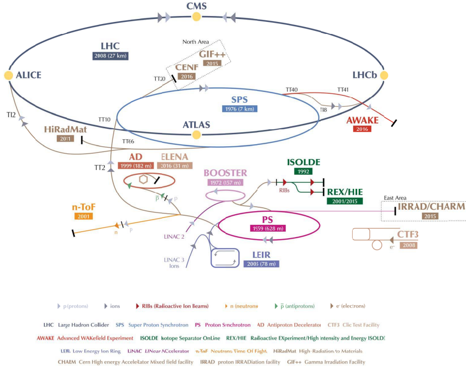
Figure 1.1: CERN's accelerator complex (Image by CERN ).
