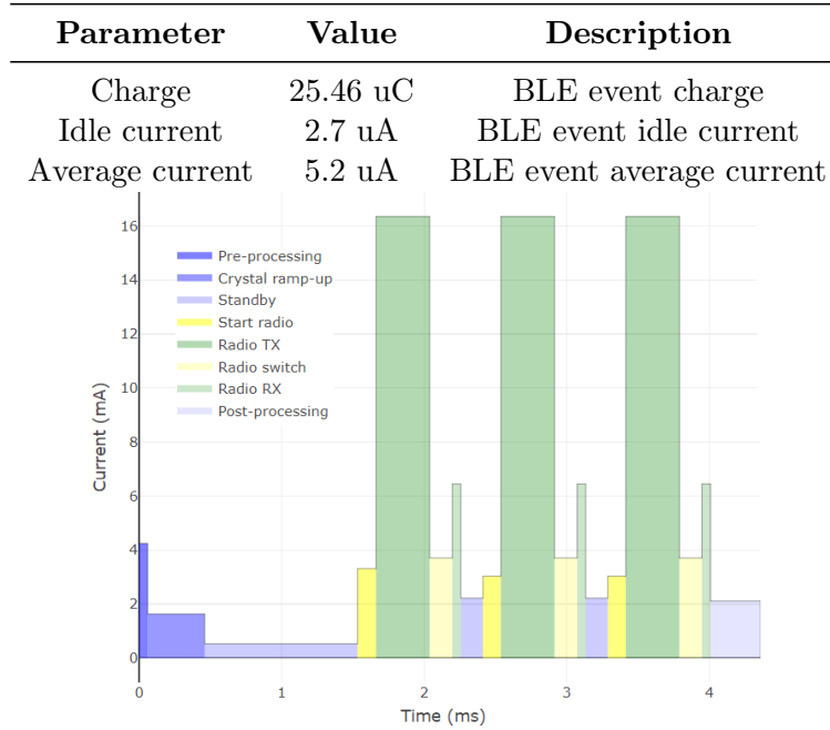
(b) nRF52840-SoC current consumption per BLE event.
