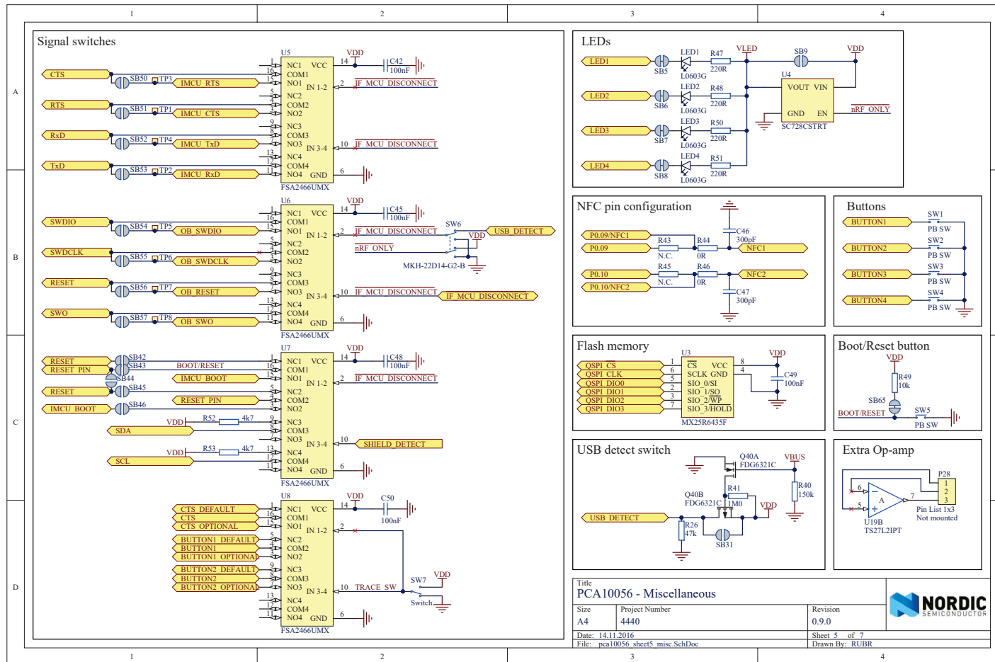
SCH II.5: PCA10056 - Miscellaneous, page 5 of 7 [45].
