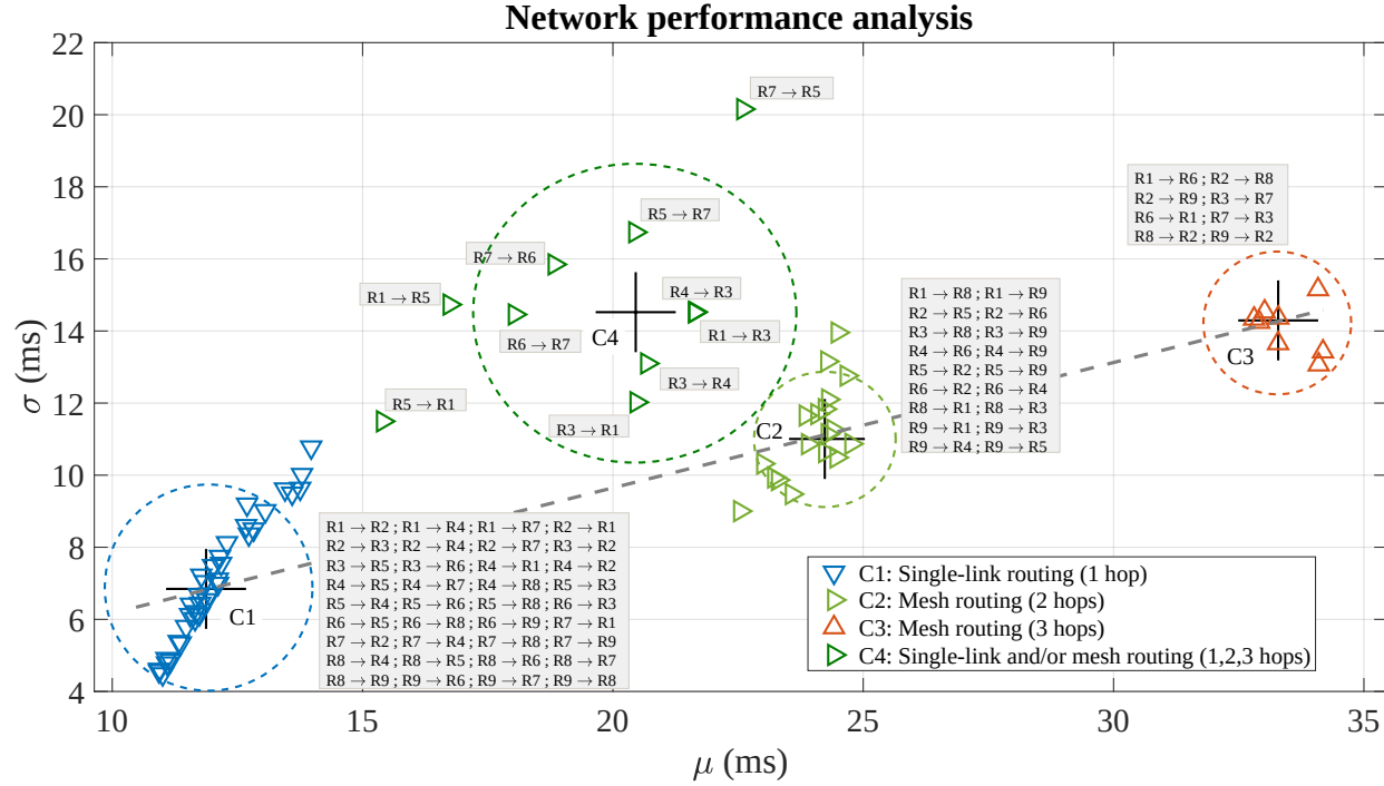
Figure 4.10: Mesh network route performance by k-means clustering analysis.
