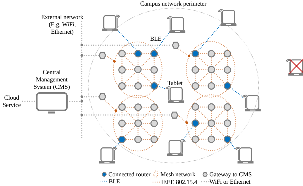
Figure 1.3: Proposed HTEL anti-theft solution where tablets connect to the nearest node based on their location in multiple mesh networks.
