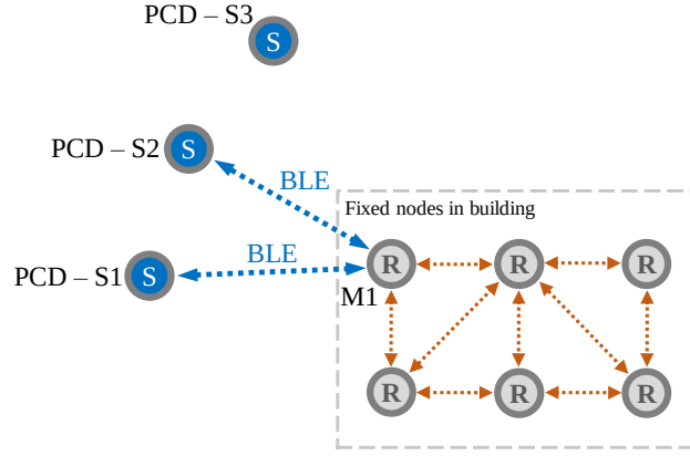
Figure 2.8: Revised BLE network topology proposed for the HTEL anti-theft solution illustrating the connection of multiple slaves nodes (PCD-S1 and PCD-S2) representing tablets to a single master node. Master nodes are configured as routers in an IEEE 802.15.4 [19] based mesh topology.
