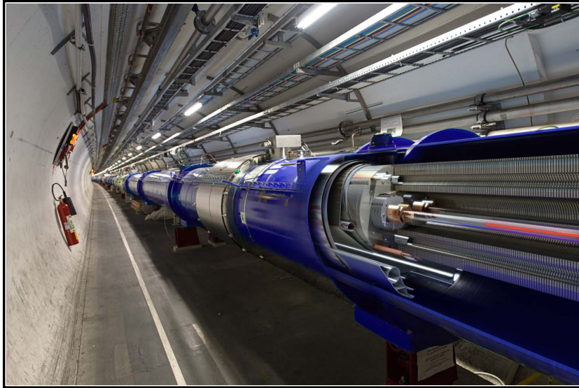
(a) Superconductor magnet located in the LHC tunnel.
