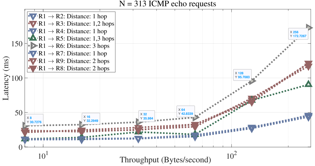
Figure 4.12: Router RTTs at various throughputs.
