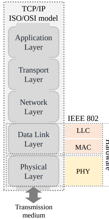
Figure 2.3: Protocol stack of TCP/IP communication system based on the OSI model illustrating the IEEE 802 hardware layer.
