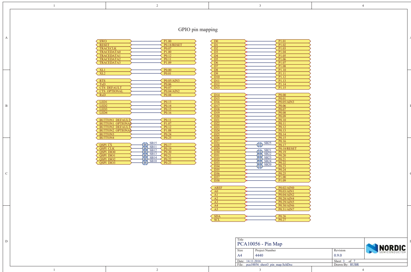
SCH II.3: PCA10056 - Pin map, page 3 of 7 [45].
