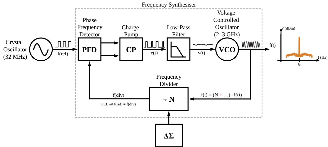
Figure 2.7: Closed-loop fractional-N phase PLL frequency synthesiser control system with \Delta\Sigma modulation modified from Lacaita et al. [33, p.14-72] and Su et al. [34, p.881].
