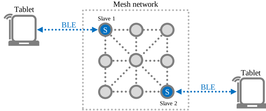
Figure 2.2: Final design concept omitting the RSIC mounted on the PCD and communicating via BLE to the nearest node in a mesh network.
