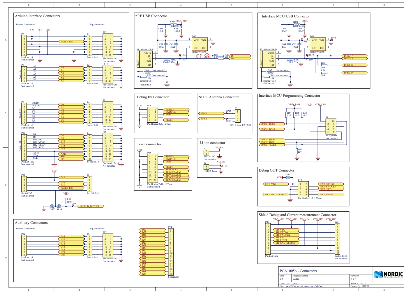
SCH II.6: PCA10056 - Connectors, page 6 of 7 [45].
