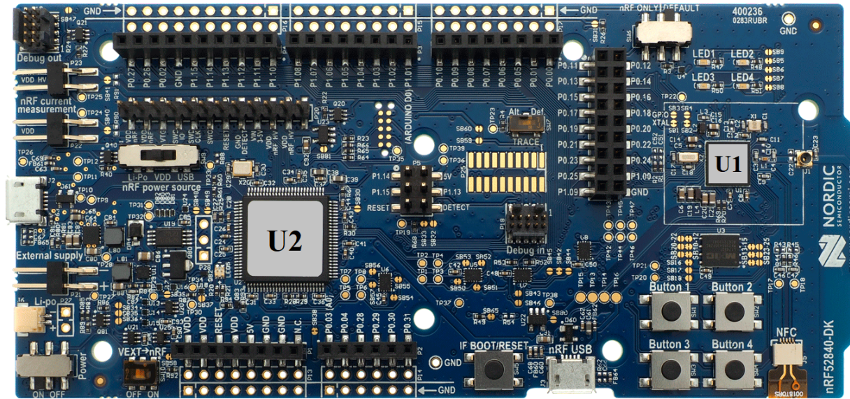
Figure 3.2: nRF52840-DK [48] utilised in the experimental study for fast prototyping and acting as a router in the Thread network. The nRF52840-SoC (labelled U1) with the passive components is mounted on the top layer located inside the square silkscreen marking. The rest of the nRF52840-DK PCB embeds an MCU (labelled U2) for programming and accessing IO ports of the nRF52840-SoC.
