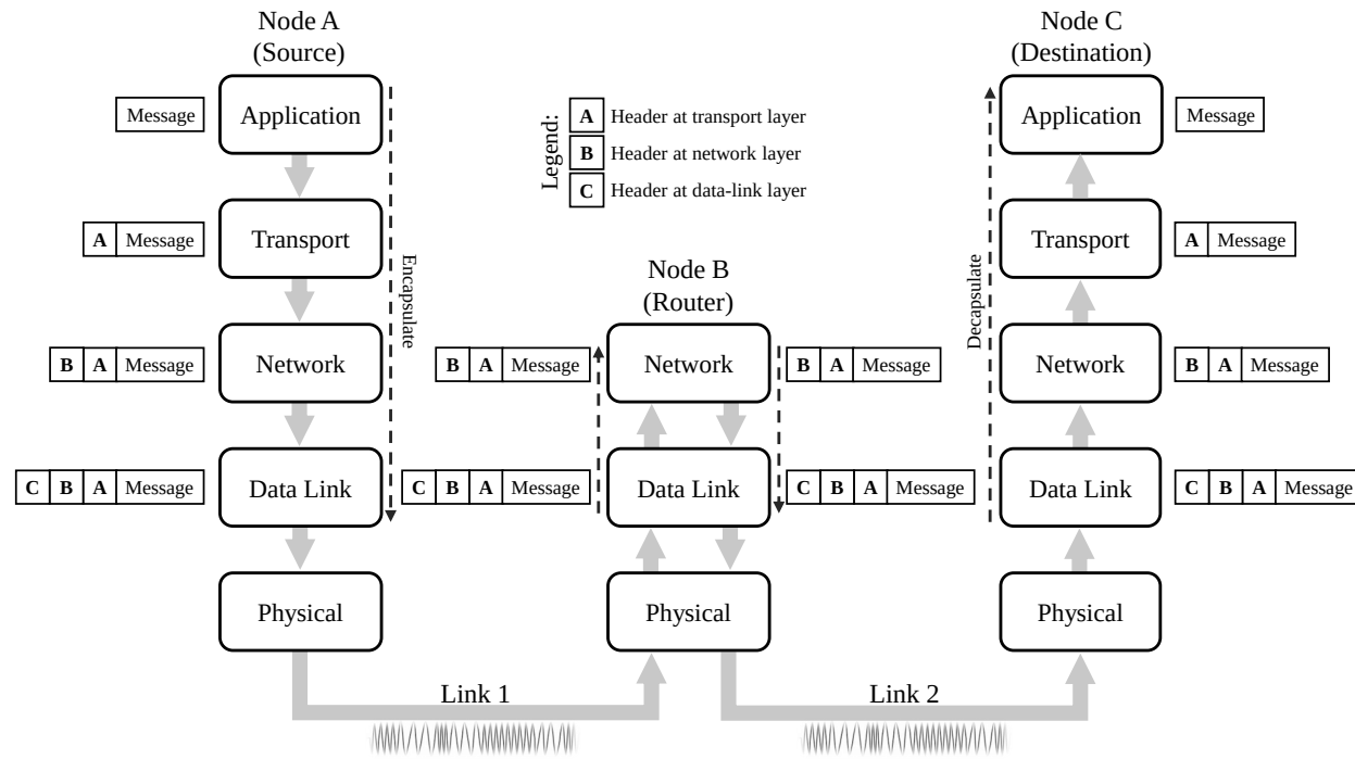
Figure 2.4: TCP/IP protocol suite adapted from Forouzan [29, p.36, 41] with the illustration of multi-hopping packet transmission over a two-hop distance using an intermediary router over two links. A packet is encapsulated from the source node and decapsulated at the receiving node.
