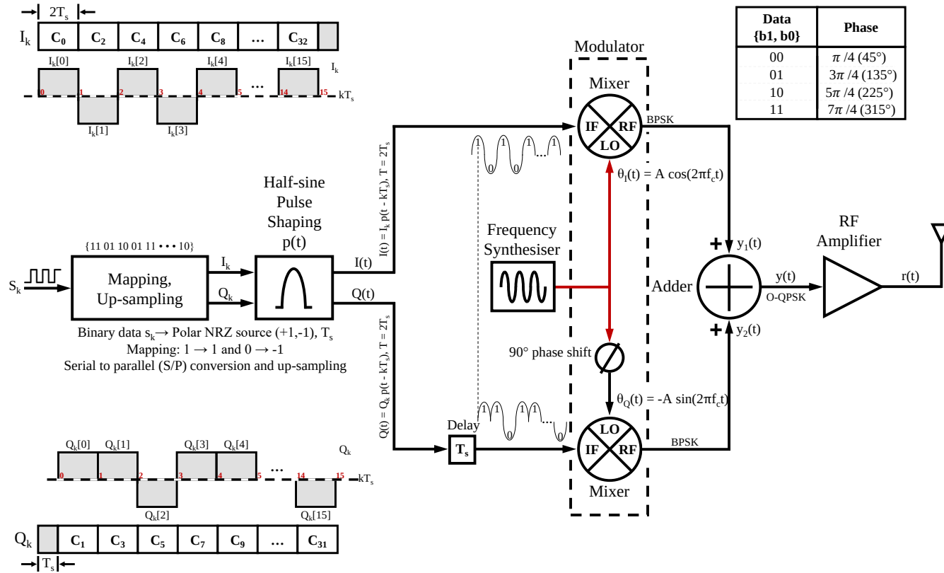
Figure 2.11: Conceptual O-QPSK modulation modified from Xiong [32, p.180].
