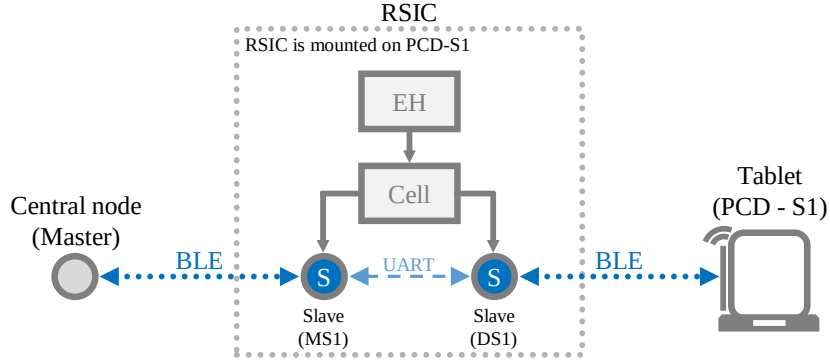
Figure 2.1: Preliminary design concept using an RSIC mounted on the PCD and communicating via BLE to a central node and tablet [20, p.2]. An energy harvester denoted by EH, provides charging capabilities to a battery cell that provides power to the slave nodes.
