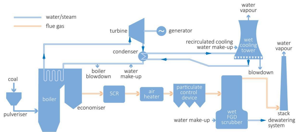
Figure 4: Schematic of a power plant showing where water is lost and added (Carpenter, 2017)
