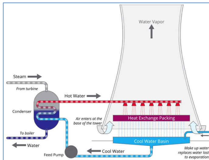
Figure 3: Typical Water Processes within a Thermal Power Plant (Reimers, 2018).
