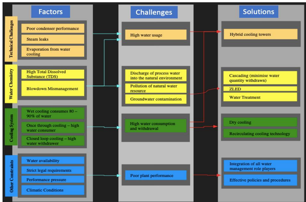
Figure 6: Conceptual Model Depicting Water Management Constraints, Challenges and Solutions
