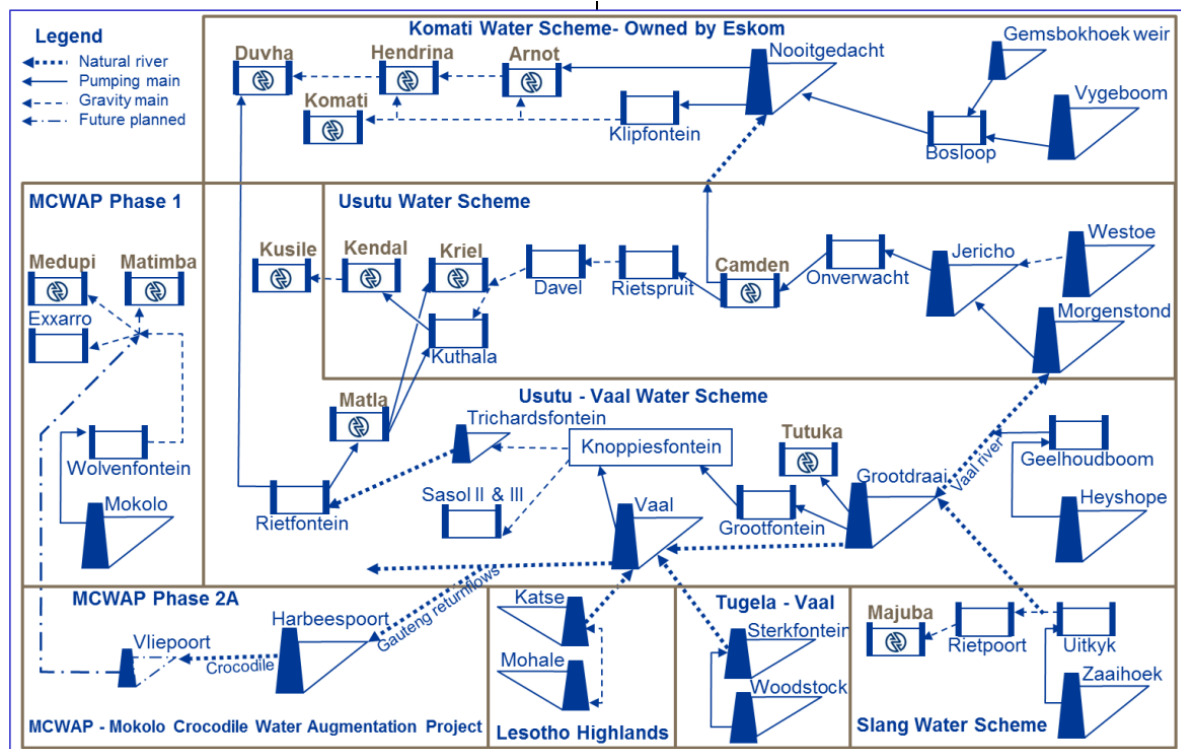
Figure 2: Interdependence of the South African energy plants' water schemes (Govender, 2018) 1
