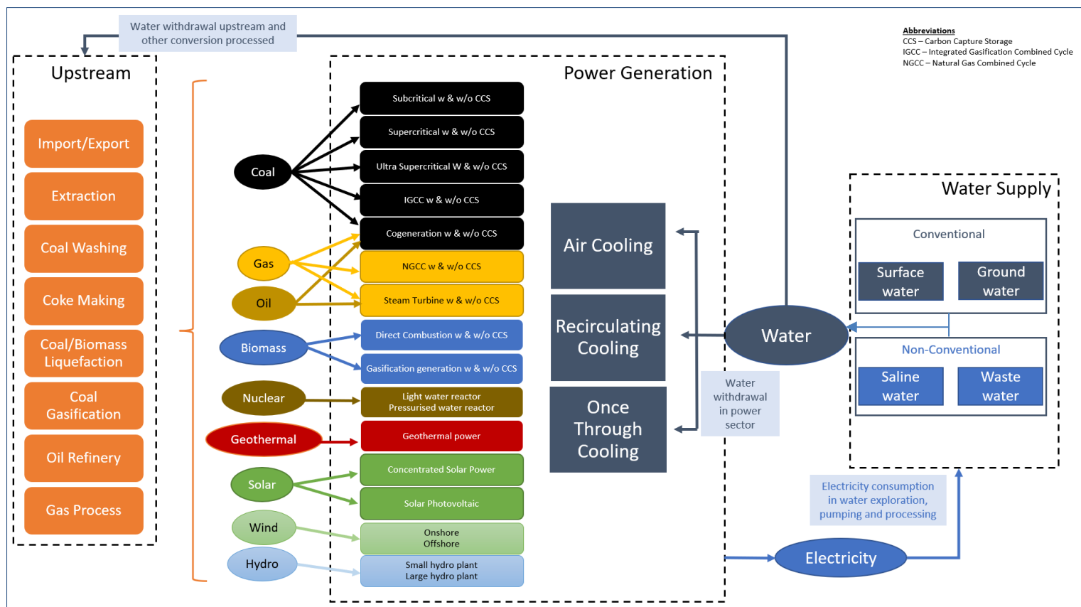
Figure 5: Water module integrated into China TIMES power and upstream sector by Huang et al. (2017)
