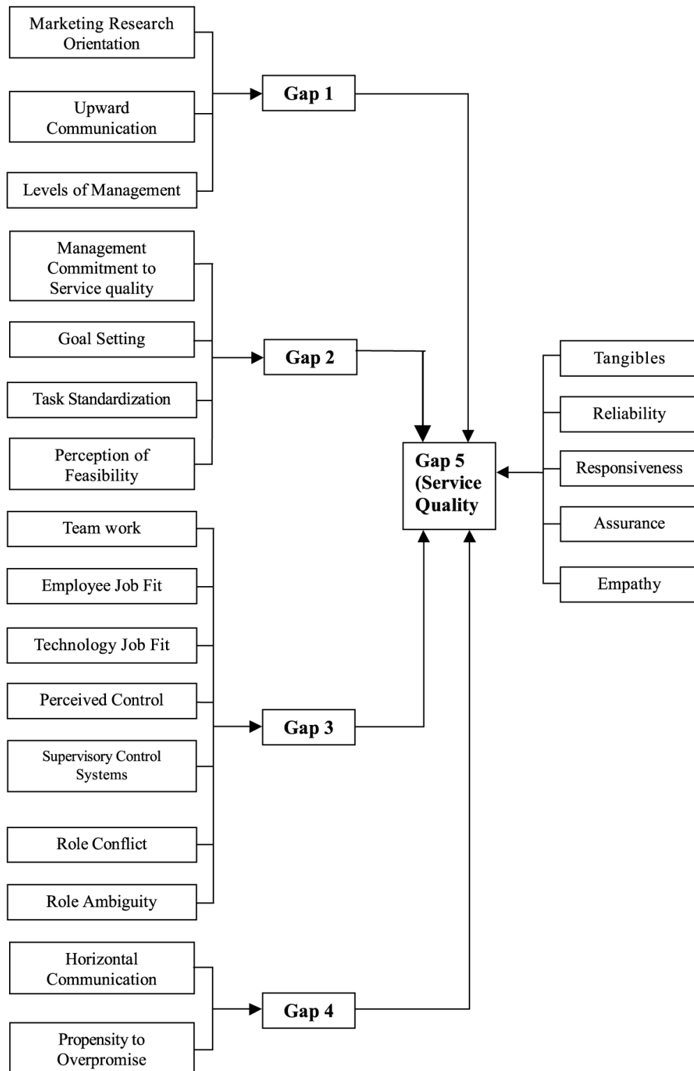
Figure 4: Improved GAPS Model
