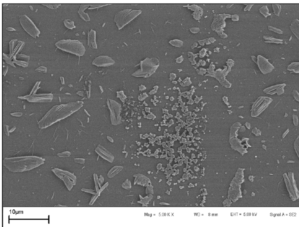
Figure 3.11 A secondary electron mode SEM micrograph of various tungsten oxide nanostructures.
