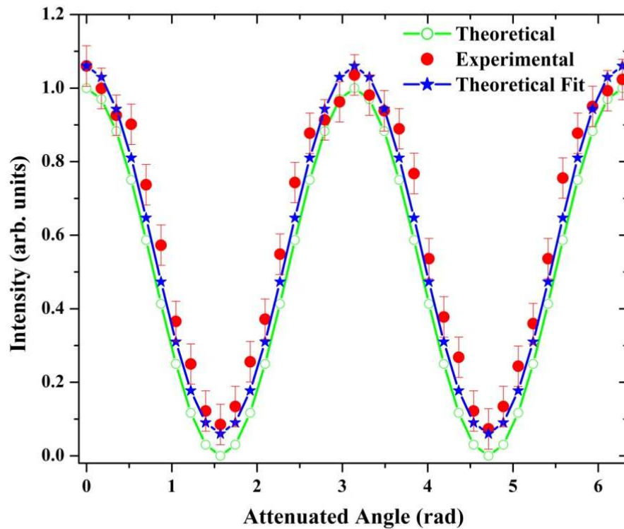
Figure 4.13 The total intensity transmission for the attenuated angles for the theoretical, normalized experimental data and the fitted theoretical curves for the experimental data of the PL6 laser.
