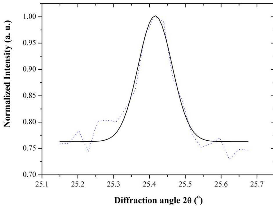
Figure 6.8 A zoomed in view of the most intense XRD peak of Figure 6.7 with a Gaussian fit to this peak. The full width at half maximum, and the angle at which the peak is most intense, are then extracted and converted to radians.
