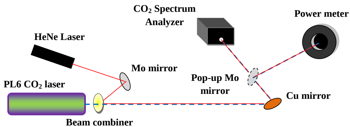
Figure 4.14 A schematic of the setup used to determine the wavelength spectrum.
