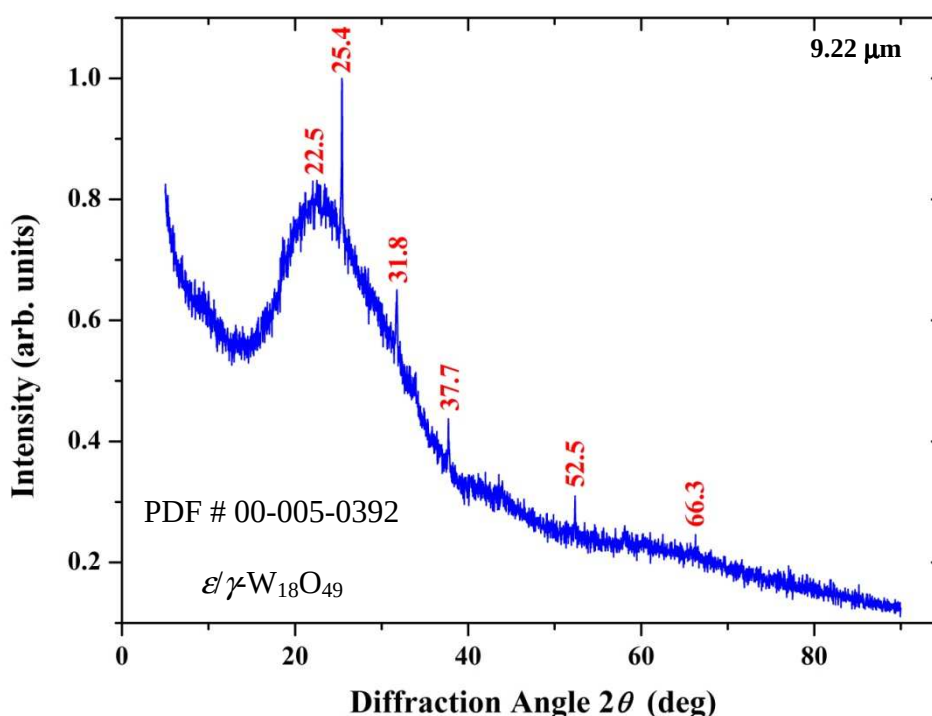
Figure 6.7 The XRD spectrum for the post-annealed sample, prepared at the 9.22 μm wavelength and 51.2 W/cm 2 power density.
