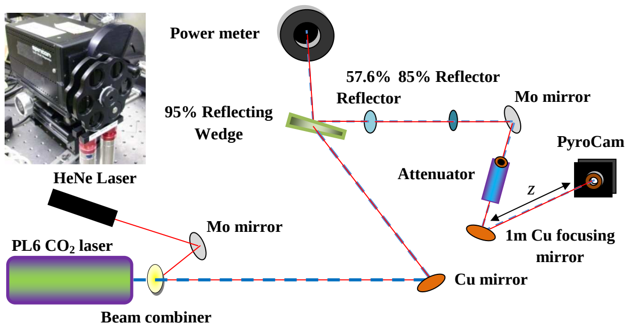
Figure 4.8 The setup used to characterize the laser beam using a pyrocam. The inset shows a picture of the pyrocam with a chopper attached to the front of it.
