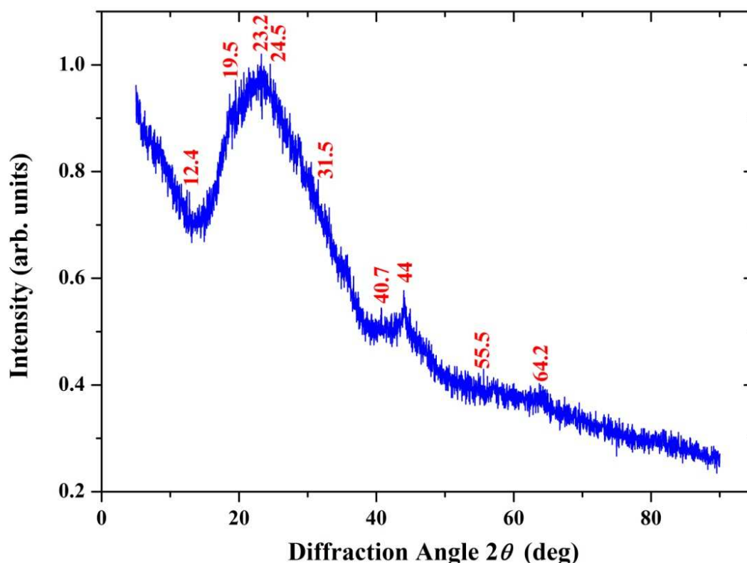
Figure 6.15 The XRD spectrum for the post-annealed sample containing the stars, slabs and the growths between the slabs.
