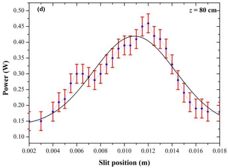
Figure 4.10 (c)-(d) Plots of the power for varying slit positions at various propagation distances between the focusing mirror and thin slit.
