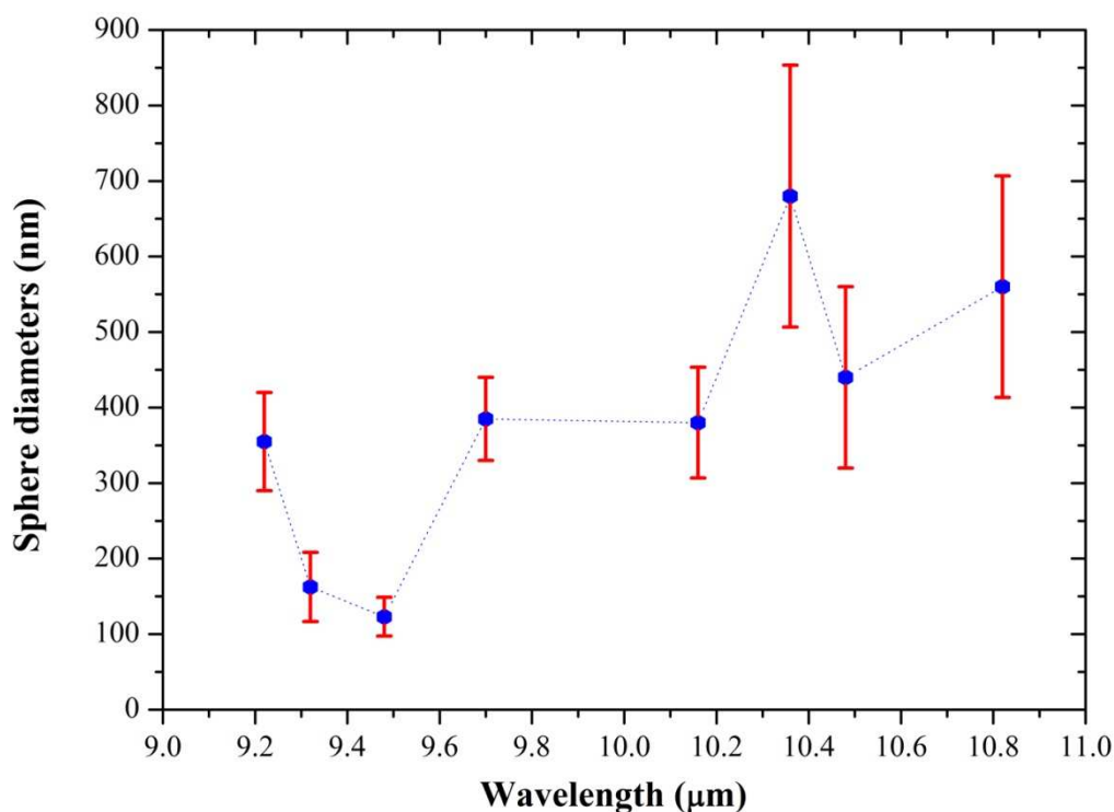
Figure 6.4 The average spherical particle sizes as a function of wavelength at the 51.2 W/cm 2 power density.
