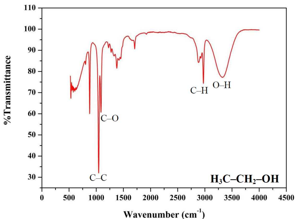
Figure 3.2 FTIR transmittance spectrum of ethanol, showing the characteristic peaks arising from the different chemical bond frequencies.
