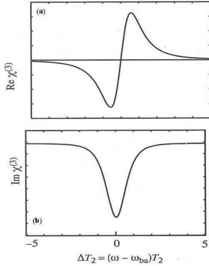
Figure A.3 (a) Real and (b) imaginary parts of the susceptibility \chi^{(3)} plotted as functions of the optical frequency \omega [86].
