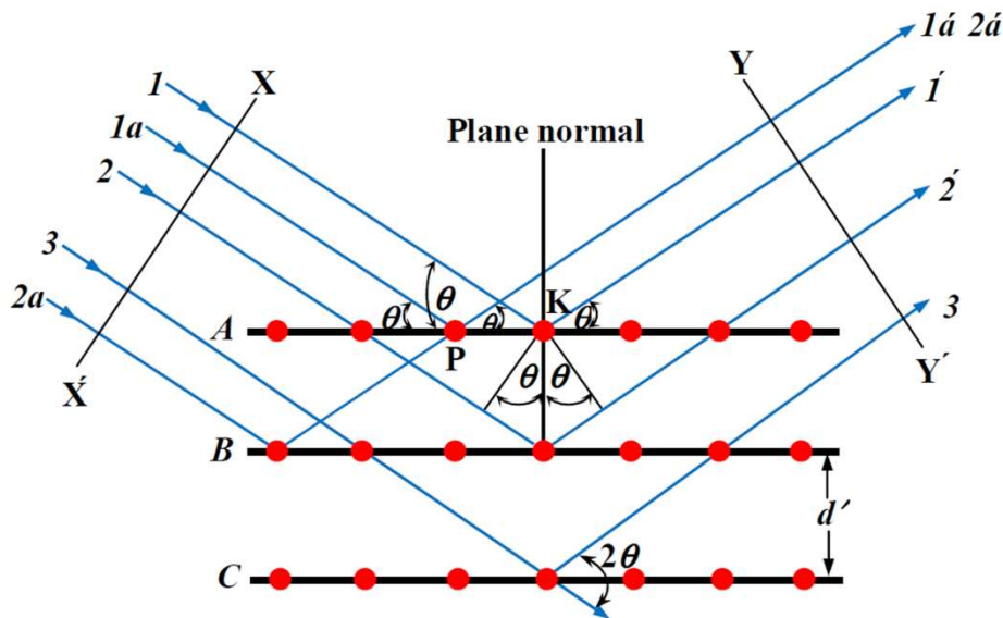
Figure 3.5 Incident x-rays diffracting off the planes in a crystal at distinct angles of \theta depending on d' [92].
