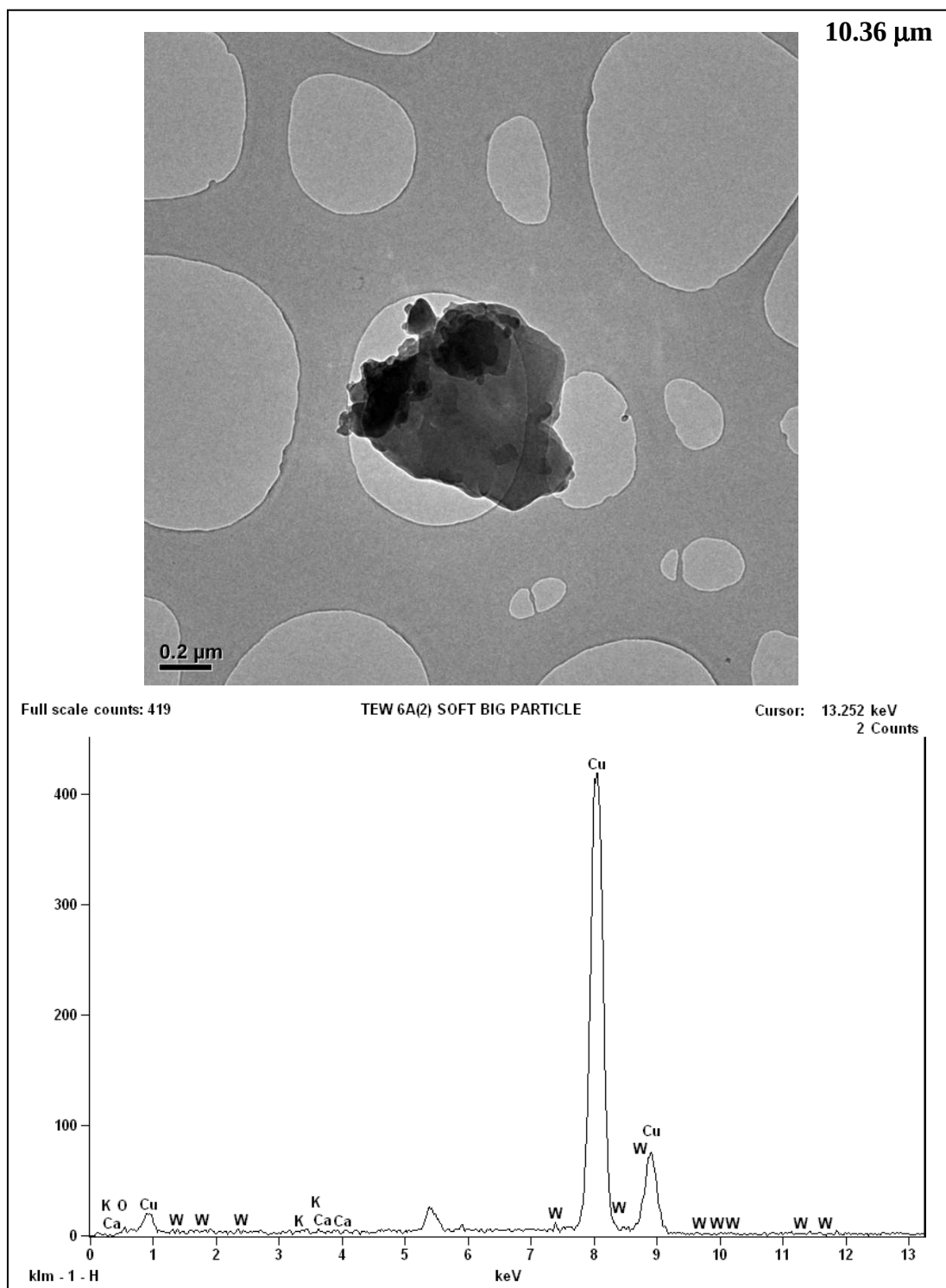
Appendix C.7 Top: A TEM micrograph showing an agglomeration of particles and Bottom: the EDX spectrum of the agglomeration.
