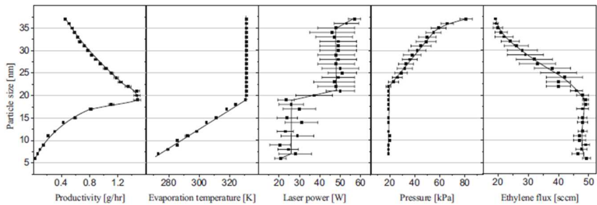
Figure 1.6 Representation of the maximum productivity predicted by the model based on aerosol theory and the experimental conditions required for the production of iron nanocrystals of a given size [79].
