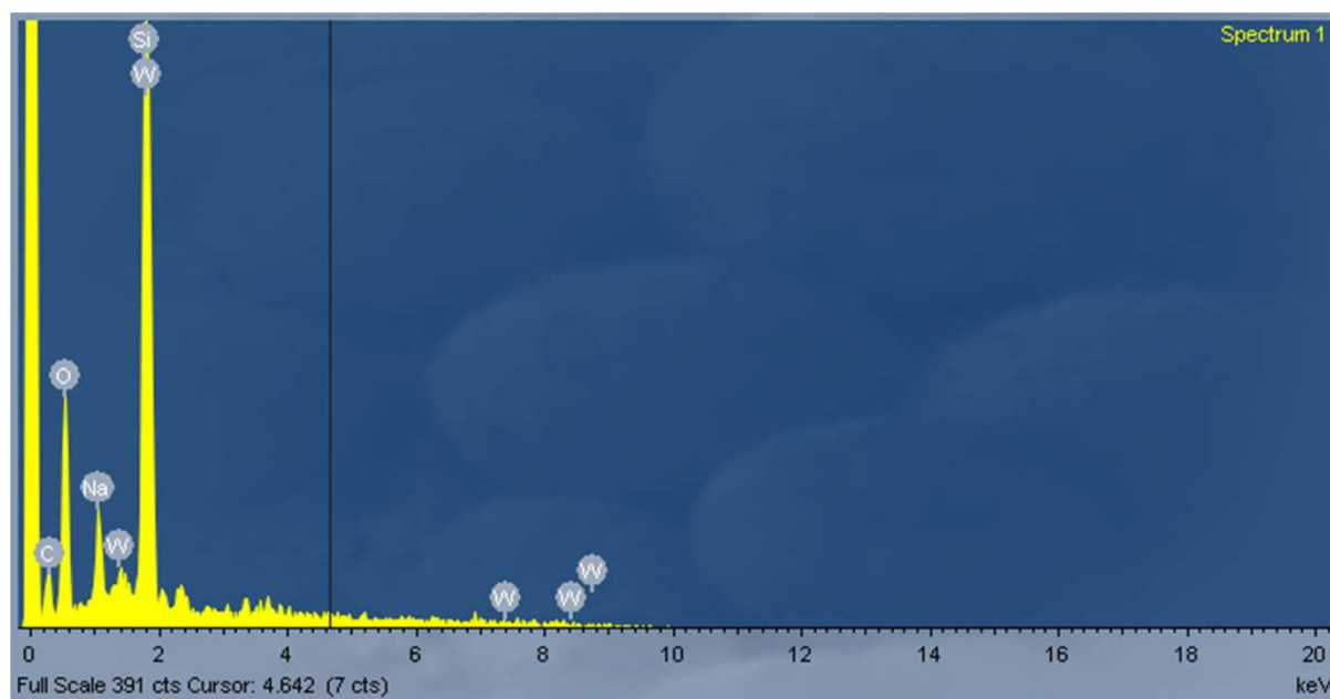
Figure 3.14 An EDX spectrum of a tungsten oxide, where the tungsten peaks are represented by W and the oxygen peak are represented by O. The carbon (C) results from carbon-coating the sample to make it conductive, and the sodium (Na) and silicon (Si) are present in the substrate.
