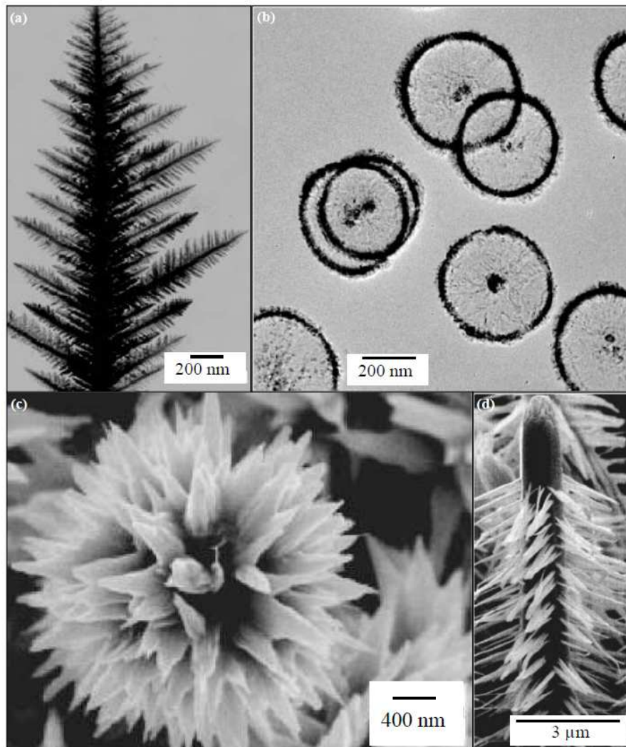
Figure 1.1 Scanning electron micrographs of less-common and hierarchical structures [27] of (a) nanopine ( \text{Fe}_2\text{O}_3 ), (b) nanowheels (Pt), (c) nanoflower (ZnO) and (d) a nanotree (ZnO).
