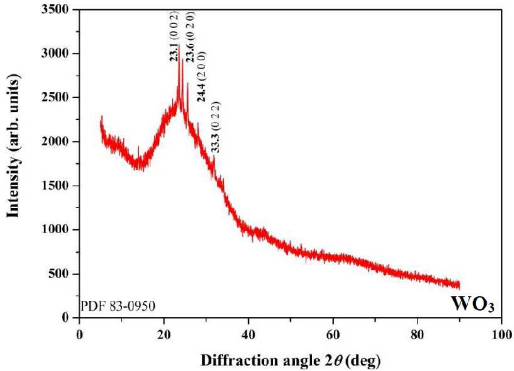
Figure 3.7 XRD diffractogram or spectrum of \text{WO}_3 , showing the characteristic diffraction angles and Miller indexes. The broad underlying peak results from the substrate on which the \text{WO}_3 sits.
