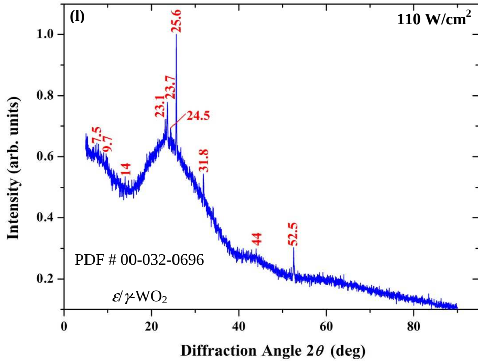
Appendix D.2 (a)-(l) The XRD spectra for the post-annealed samples, prepared at different power densities and constant wavelength of 10.6 \mu\text{m} .
