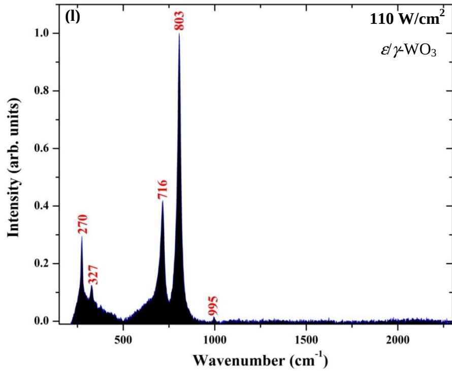
Appendix F.2 (a)-(l) The Raman spectra of the post-annealed samples, prepared at different power densities and constant wavelength of 10.6 \mu\text{m} .
