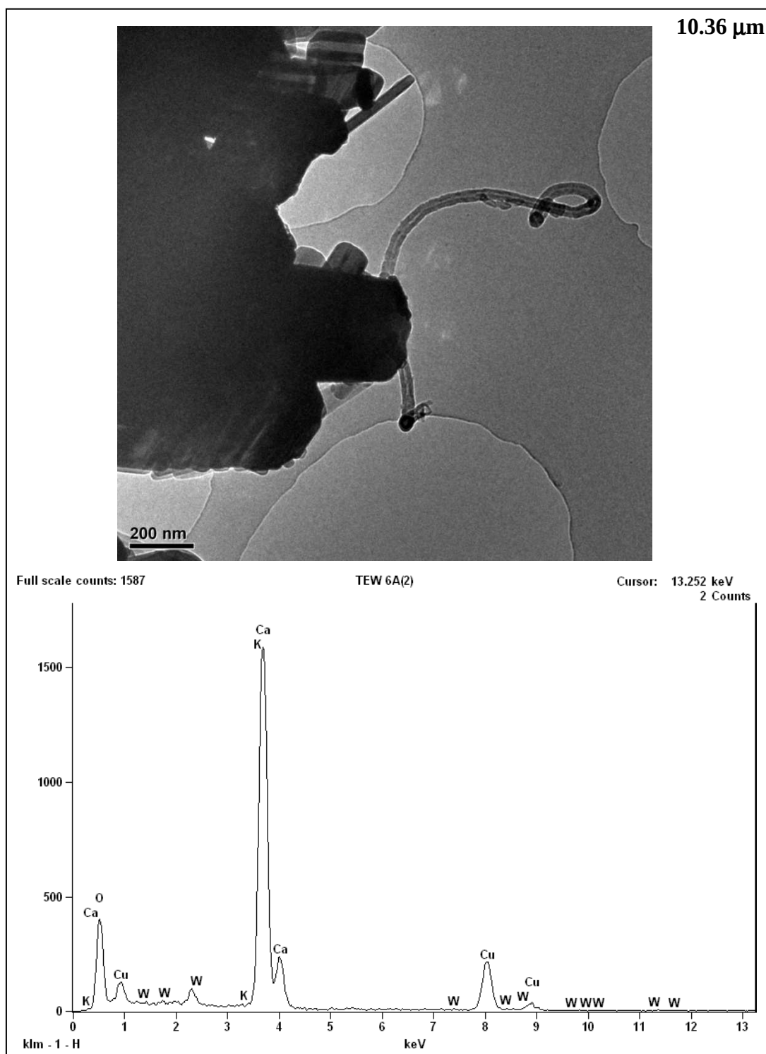
Appendix C.6 Top: A TEM micrograph showing a clump of particles and a nanotube and Bottom: the EDX spectrum of the various structures.
