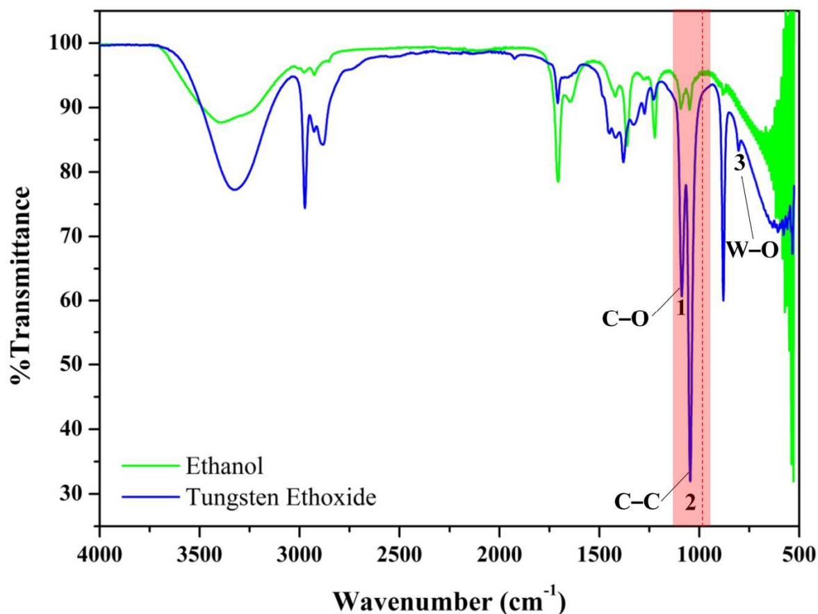
Figure 5.7 The FTIR spectrum of the tungsten ethoxide precursor (blue) and pure ethanol (green). The shaded region represents the wavelength range of the CO 2 laser and the dashed red line represents the CO 2 laser's 10.6 \mu\text{m} wavelength.
