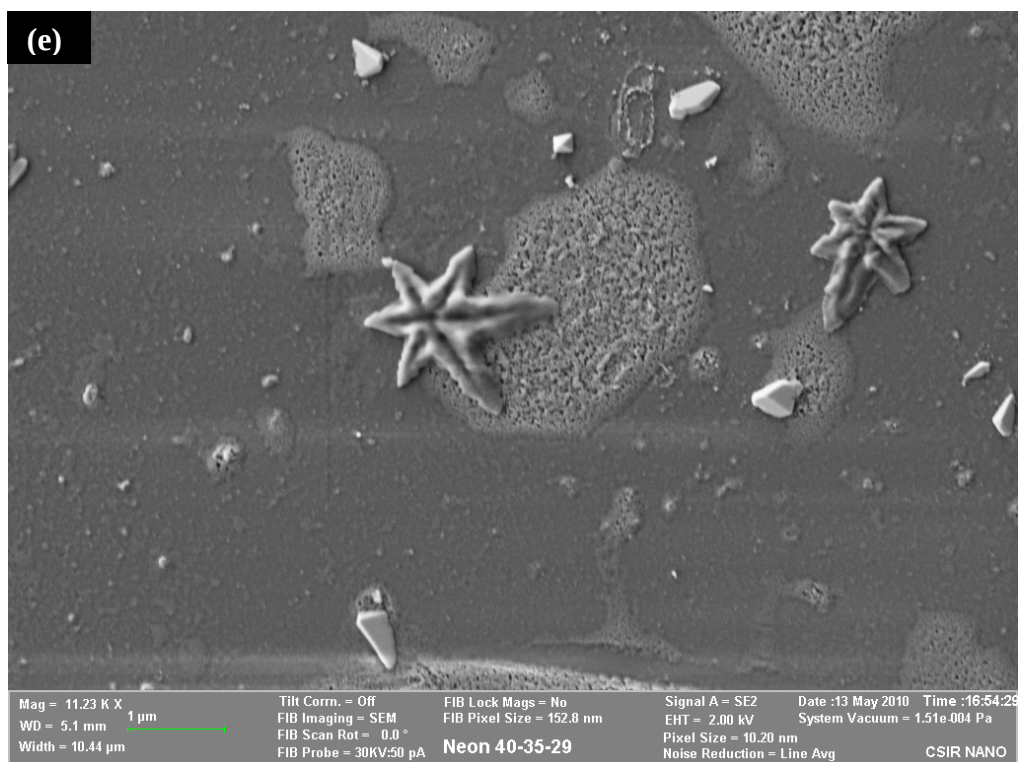
Appendix E.1 SEM micrographs of the post-annealed sample showing the stars that formed during annealing, at (a) 2000 times magnification, (b) 4500 times magnification, (c) 4740 times magnification, (d) 7490 times magnification, and (e) 11230 times magnification, prepared at the 10.6 \mu\text{m} wavelength and power density of 2.2 \text{kW}/\text{cm}^2 .
