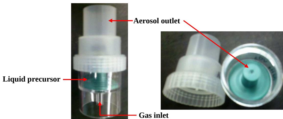
Figure 5.4 The aerosol generator holds the precursor liquid, and argon gas is passed through the bottom inlet creating a fine aerosol that emerges from the top.
