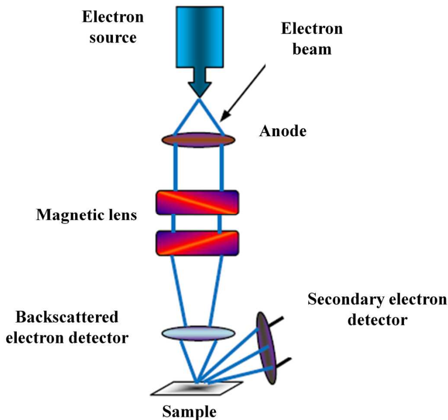
Figure 3.10 An illustration of the layout and components of a scanning electron microscope [95].
