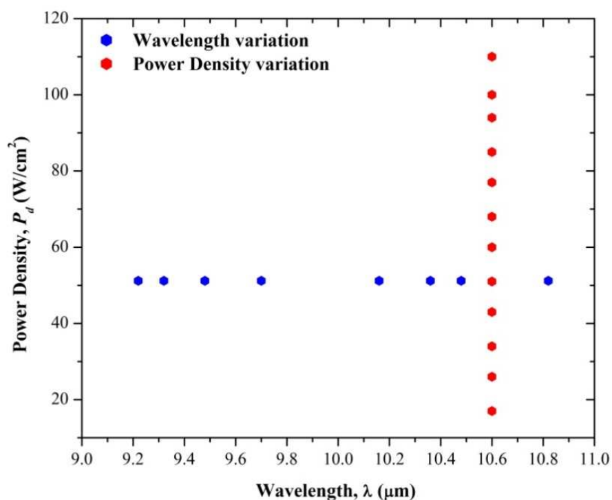
Figure 6.1 The varying laser parameters are represented by the respective points on the graph, used to investigate the effects on the morphology and chemical composition of the products.
