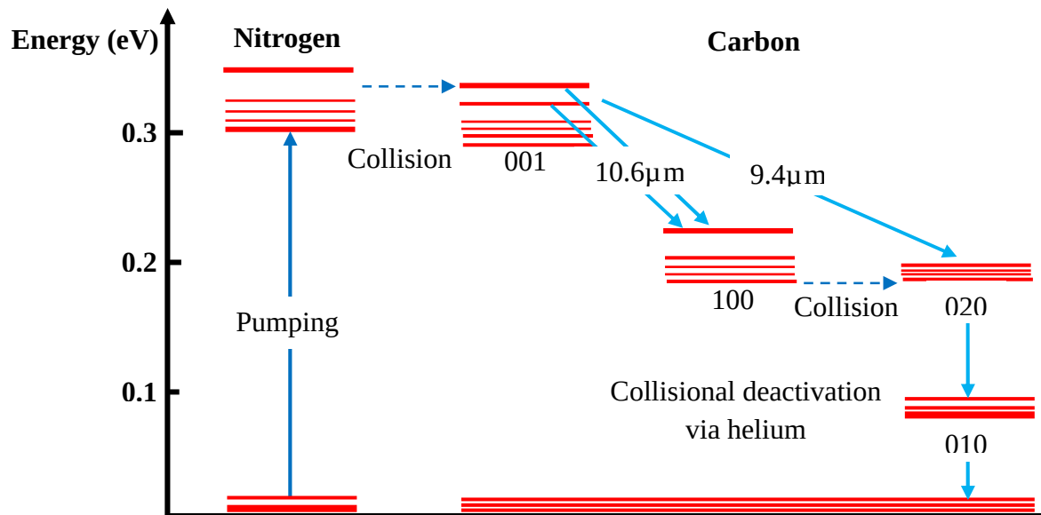
Figure 4.3 The three energy levels of the \text{CO}_2 molecule with the subdivided levels caused by rotations in the vibrating molecule and also shown here are the lasing transitions from two of the resonant modes [100].
