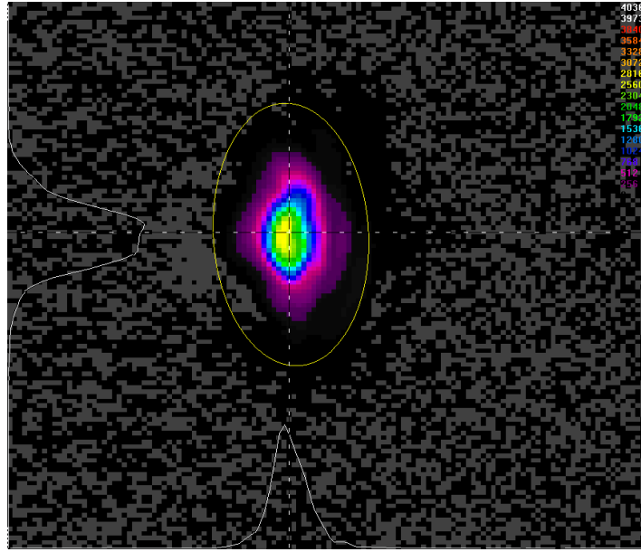
Figure 4.9 An image taken by the pyrocam showing the heat distribution of the beam by the different colours and the intensity distribution on the x and y axes are also shown.
