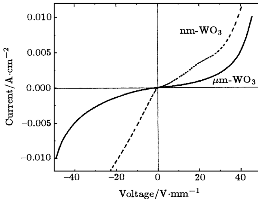
Figure 1.3 The current-voltage ( I - V ) characteristics of nanometre-sized \text{WO}_3 (nm- \text{WO}_3 ) and micrometre-sized \text{WO}_3 ( \mu\text{m} - \text{WO}_3 ) [35].
