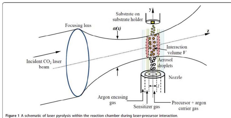
Figure 1 A schematic of laser pyrolysis within the reaction chamber during laser-precursor interaction.
