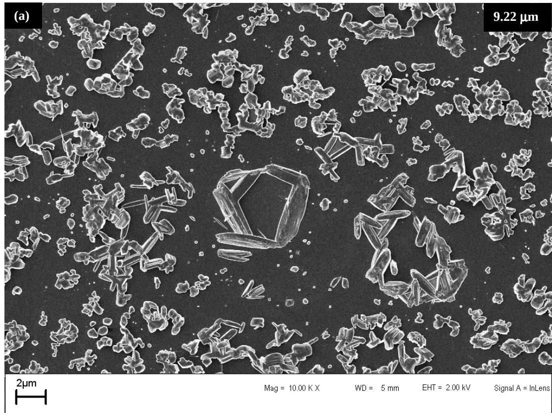
Figure 6.3 (a) The annealed sample prepared at the 9.22 \mu\text{m} wavelength and 51.2 \text{ W/cm}^2 .
