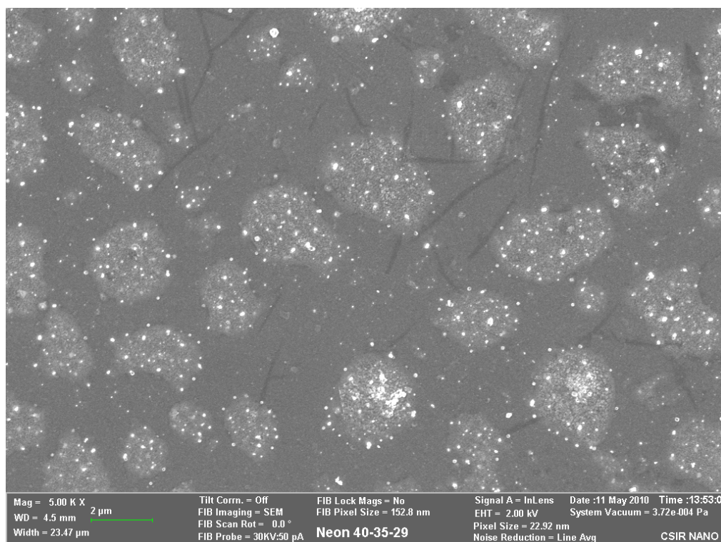
Figure 6.12 SEM micrographs of the pre-annealed sample, at 5000 times magnification, prepared at the 10.6 \mu\text{m} wavelength and power density of 2.2 \text{kW}/\text{cm}^2 .
