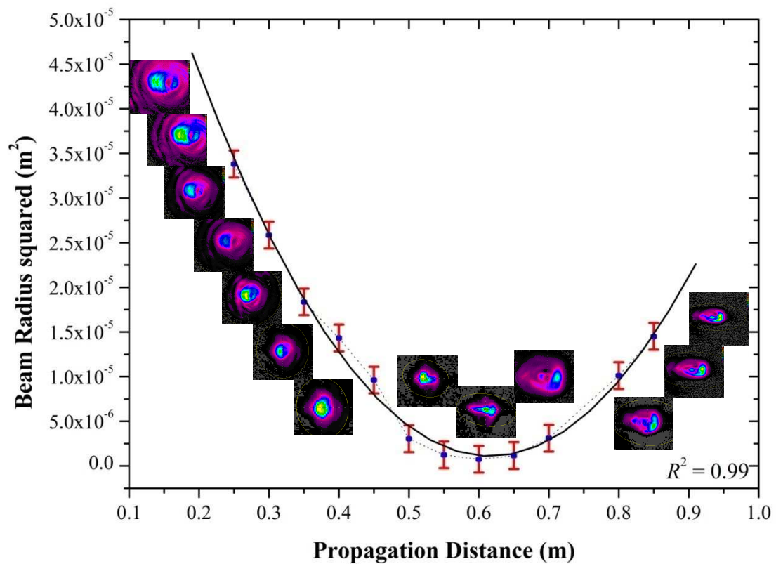
Figure 4.11 The second-order quadratic fit from the data of the pyrocam method.
