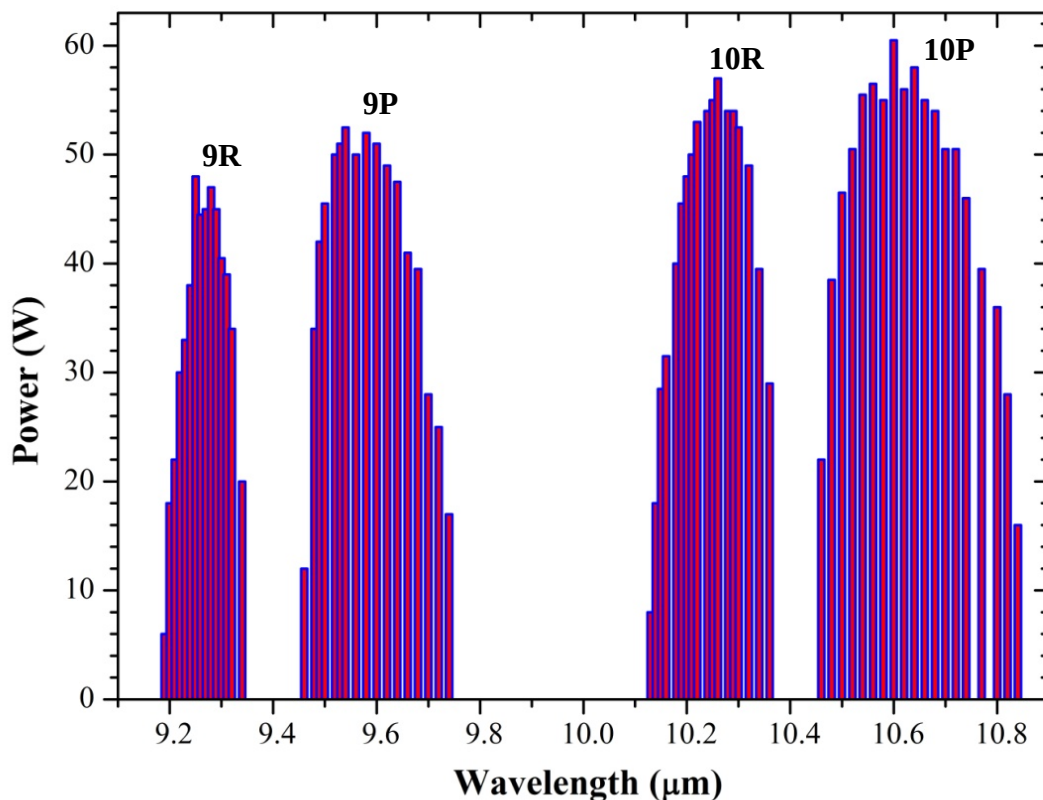
Figure 4.17 The wavelength spectrum of the PL6 CO 2 laser.
