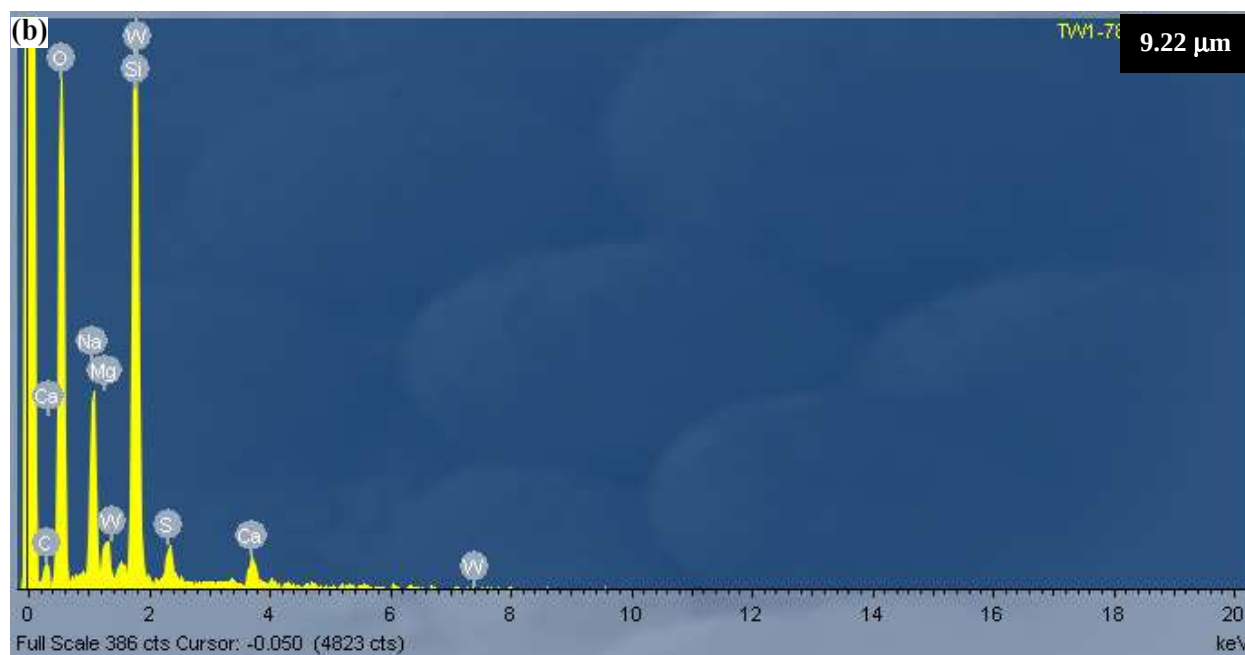
Figure 6.3 (b) The EDX spectrum on the area of the sample prepared at the 9.22 \mu\text{m} wavelength and constant power density of 51.2 \text{W}/\text{cm}^2 , which shows the presence of calcium (Ca), magnesium (Mg), carbon coating (C), sodium (Na), silicon (Si) and sulphur (S), which most probably come from the Corning glass. The oxygen (O) could have come from the substrate and the sample and tungsten (W) results from the sample.
