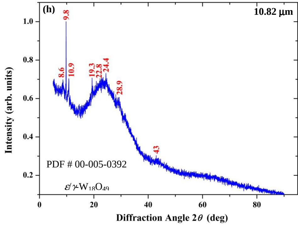
Appendix D.1 (a)-(h) The XRD spectra for the post-annealed samples, prepared at different wavelengths and constant power density of 51.2 \text{ W/cm}^2 .
