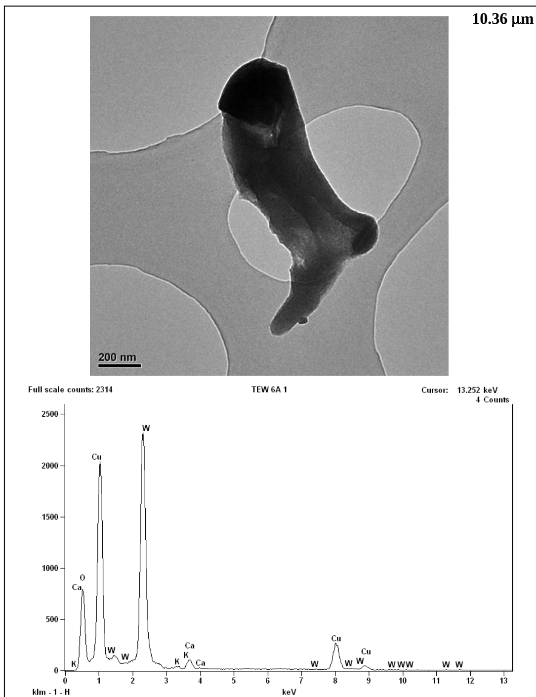
Appendix C.5 Top: A TEM micrograph showing an agglomeration of particles in the shape of a leg and Bottom: the EDX spectrum taken of the agglomerated particles.
