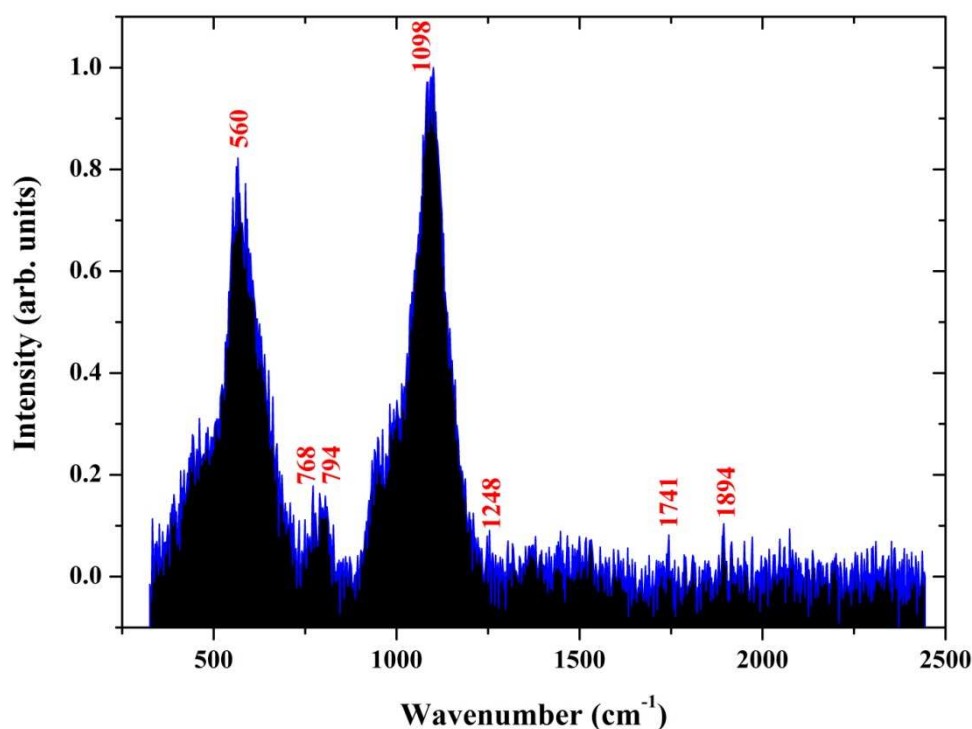
Figure 6.10 The Raman spectrum of a cleaned corning glass substrate.
