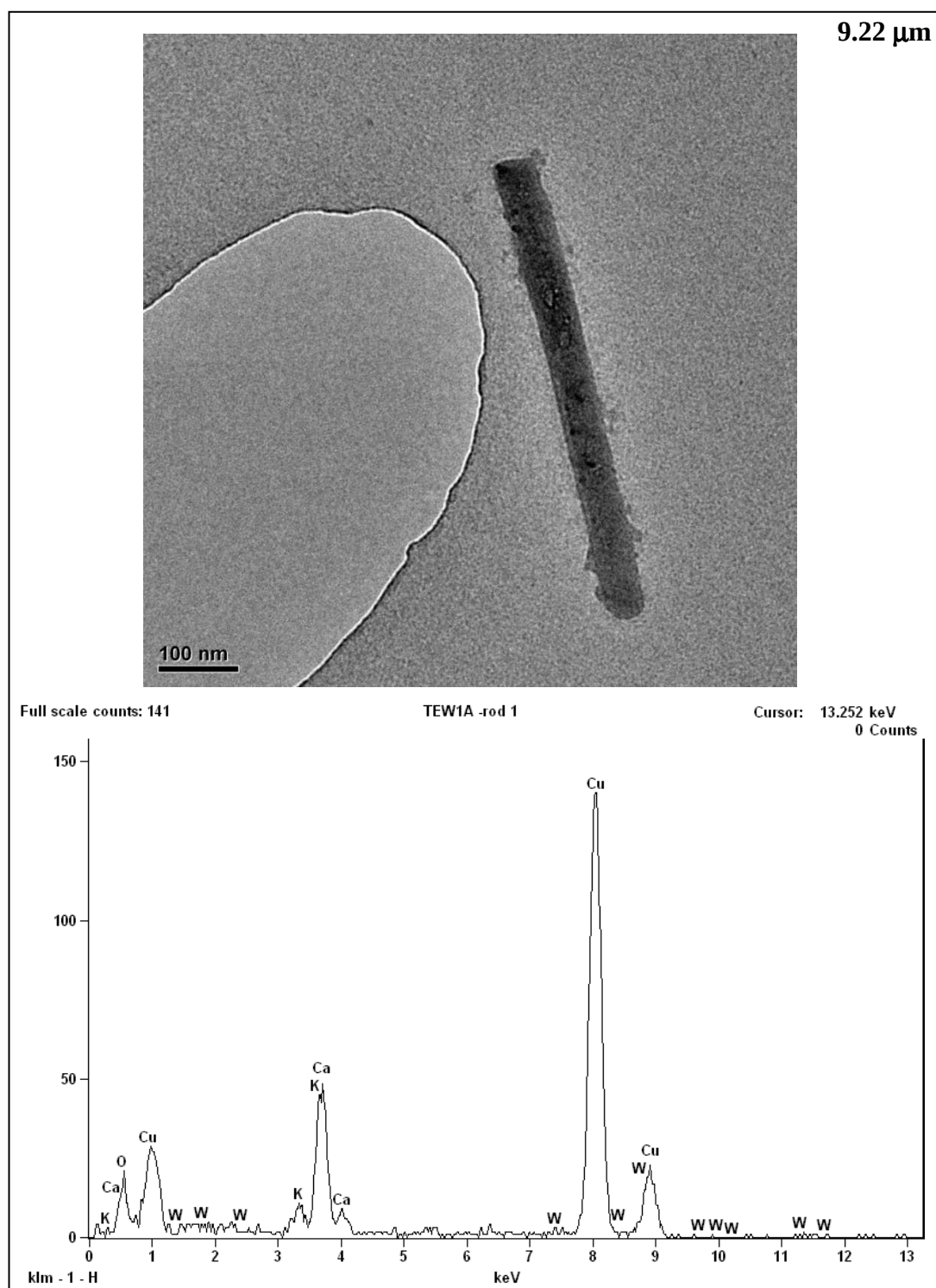
Appendix C.1 Top: A TEM micrograph showing a nanorod and Bottom: the EDX spectrum taken of the rod.
