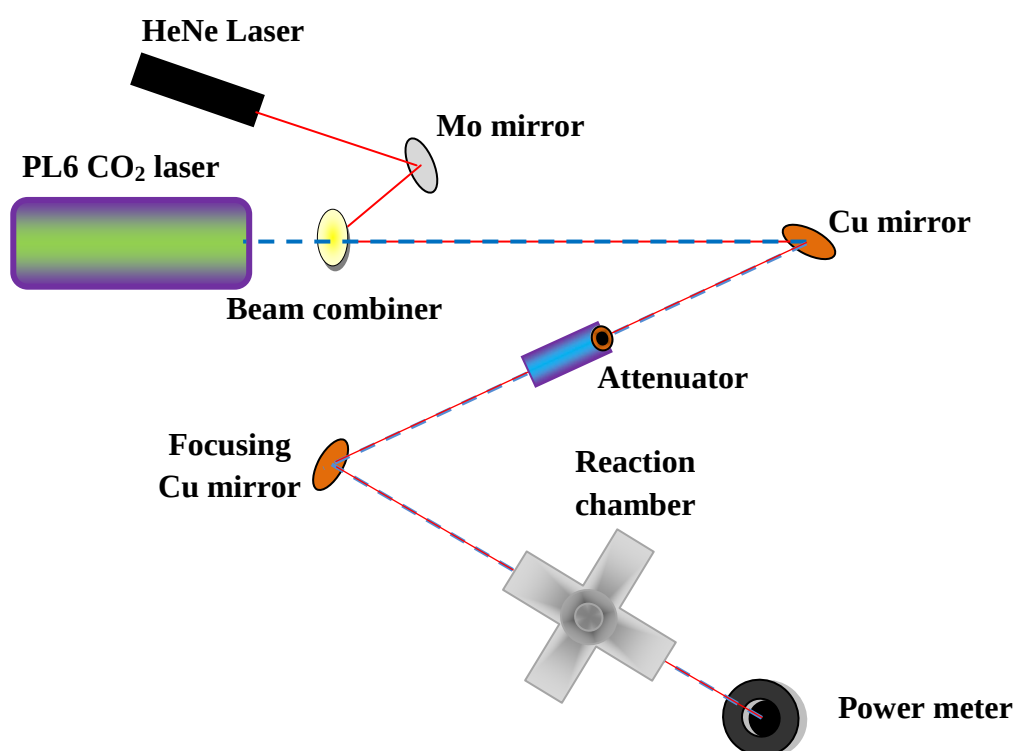
Figure 5.5 The setup used to carry out laser pyrolysis.
