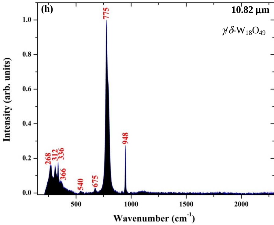
Appendix F.1 (a)-(h) The Raman spectra of the post-annealed samples, prepared at different wavelengths and constant power density of 51.2 \text{ W/cm}^2 .
