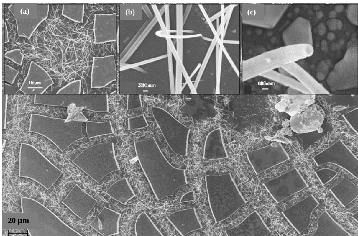
Figure 1.2 Scanning electron micrograph of post-annealed tungsten trioxide nanowires synthesized by laser pyrolysis showing a thin film that has flaked up into slabs between which are numerous nano-wires [21]. Insets: (a) shows a close look at the nanowires in between the slabs, (b) zooms in onto the nano-wire area and (c) display one nano-wire's end.
