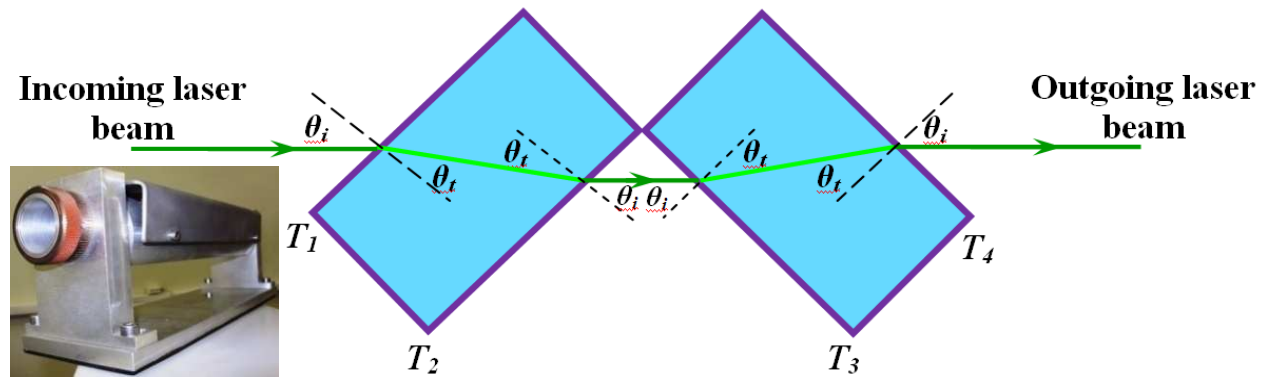
Figure 4.12 The picture shows the layout and beam propagation through the windows in an attenuator and the inset shows a home-made attenuator.
