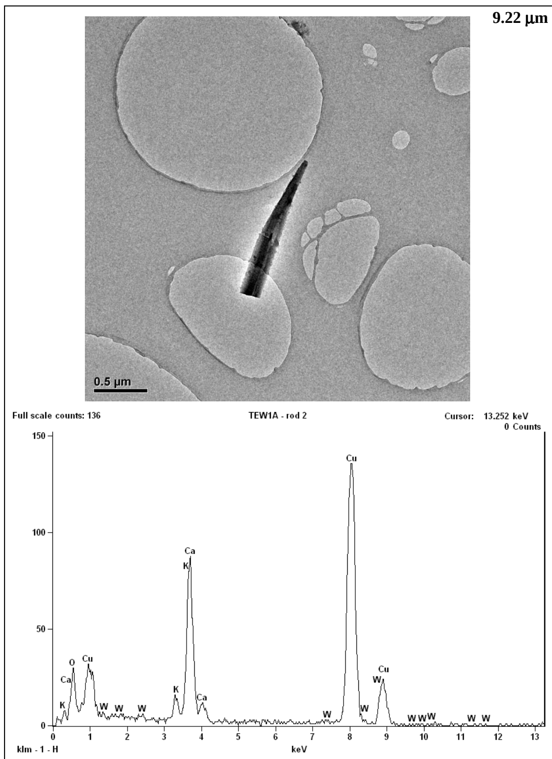
Appendix C.2 Top: A TEM micrograph showing a nanospike and Bottom: the EDX spectrum taken of the spike.
