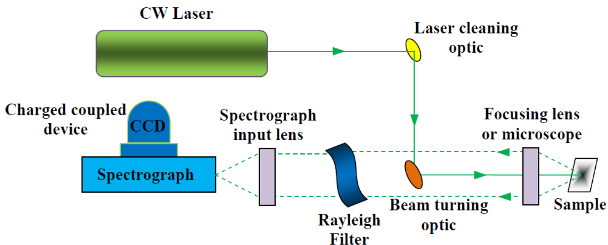
Figure 3.3 An illustration of the layout and components of a Raman spectrometer [94].
