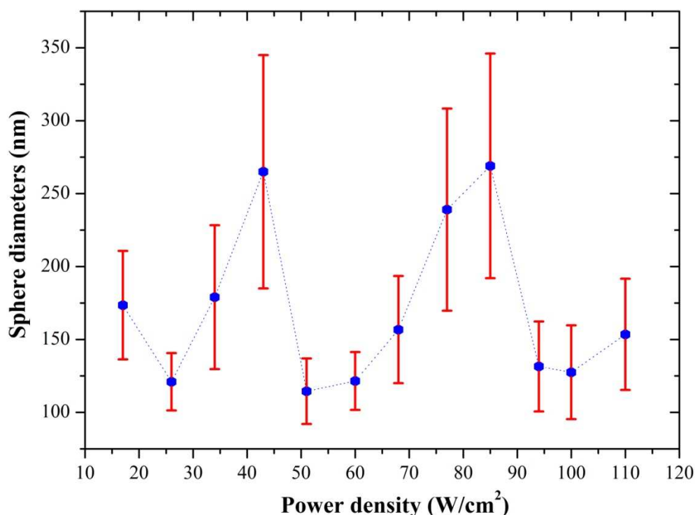
Figure 6.6 The average spherical particle sizes as a function of power density at the 10.6 \mu\text{m} wavelength
