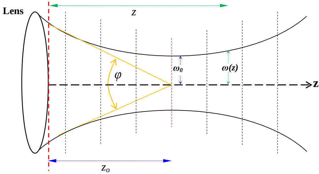
Figure 4.6 A schematic diagram of beam propagation through a lens.
