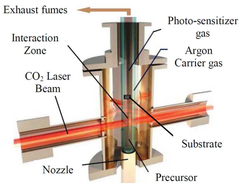
Figure 5.1 A cross-section of the reaction chamber during laser pyrolysis using the cross flow geometry [107].
