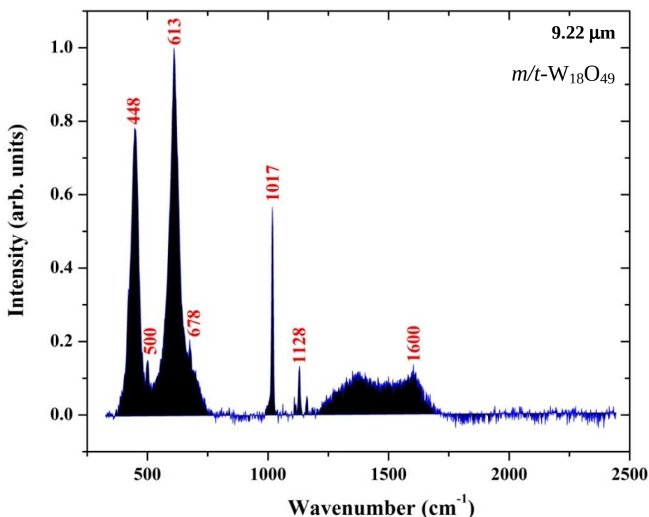
Figure 6.11 The Raman spectrum for the post-annealed sample, prepared at the 9.22 \mu\text{m} wavelength and 51.2 \text{W}/\text{cm}^2 power density.
