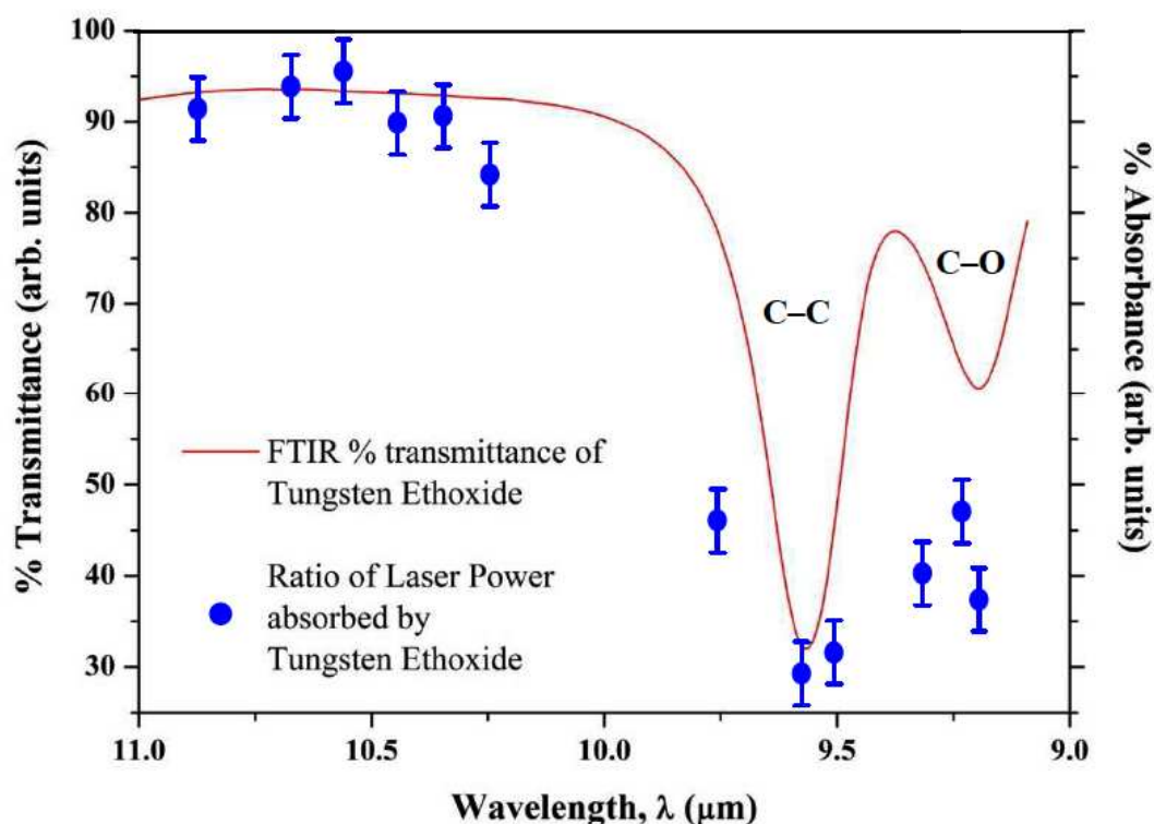
Figure 6.2 The comparison of the FTIR transmittance spectrum of the tungsten ethoxide precursor and the \text{CO}_2 laser radiation absorbance data of tungsten (VI) ethoxide as a function of wavelength.
