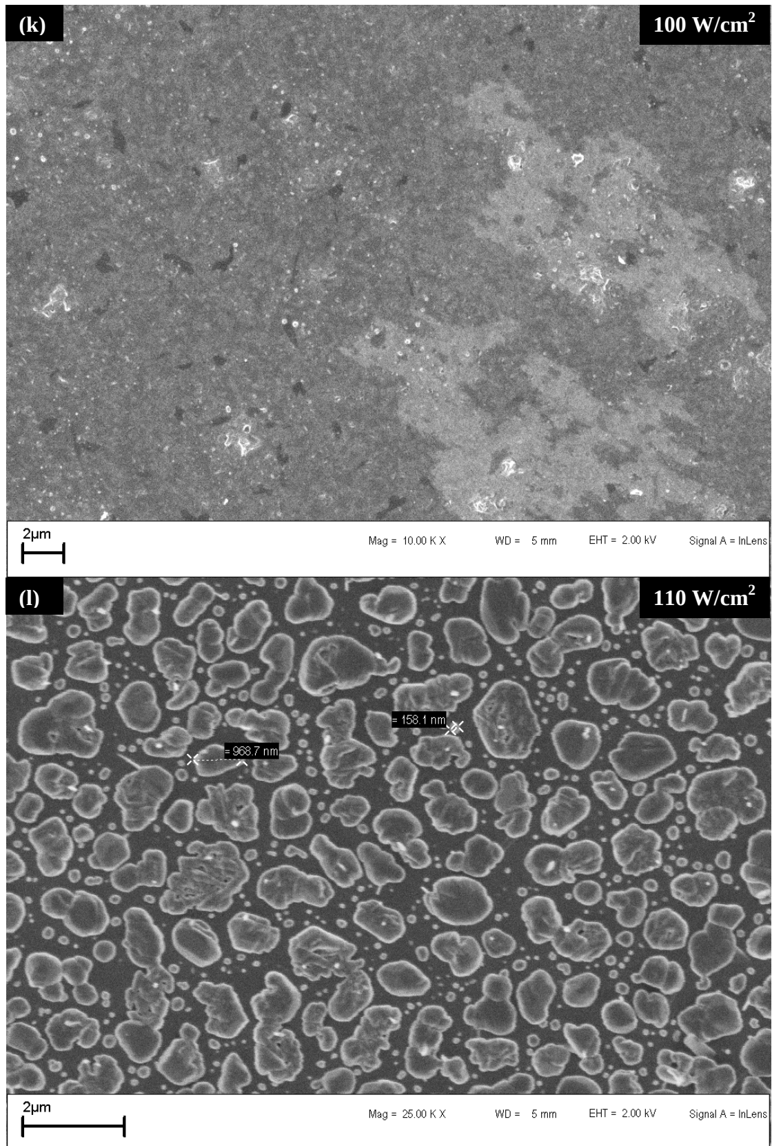
Appendix B.2 (a)-(l) The SEM micrographs for the post-annealed samples, prepared at different power densities as represented on the respective micrographs, and constant wavelength of 10.6 μm.
