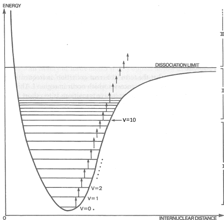
Figure 2.5 Energy levels and transitions involved in the multiphoton infrared dissociation of a diatomic molecule [89].
