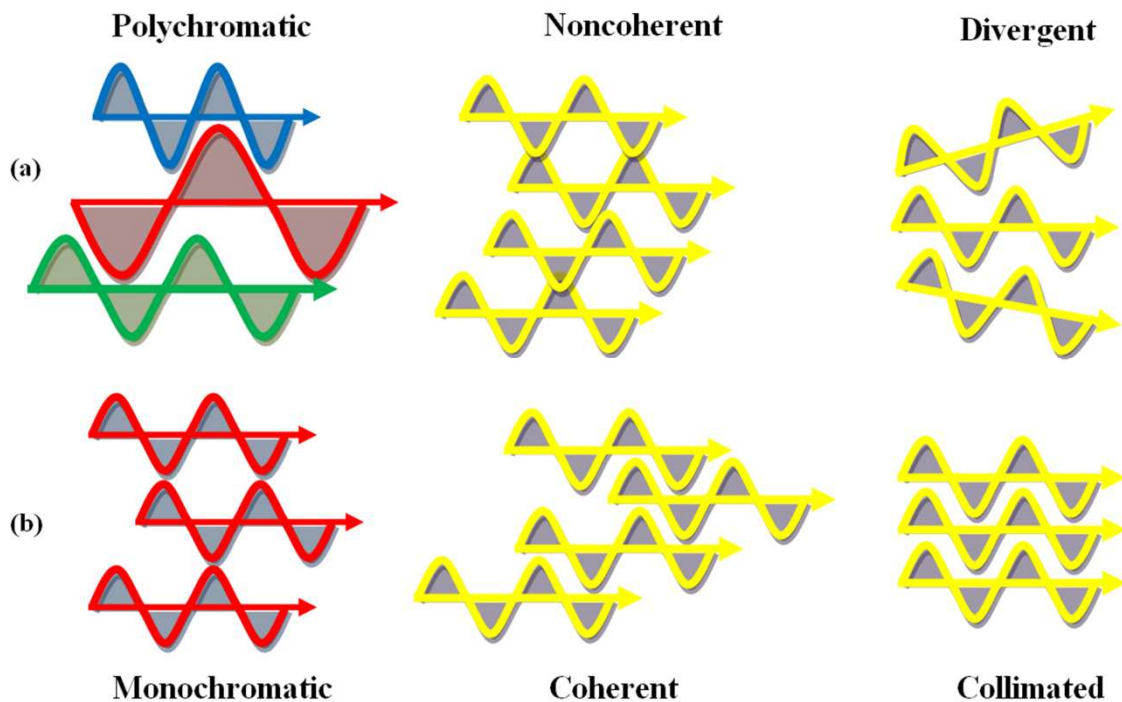
Figure 4.1 The properties that distinguish (a) white light from (b) laser light [99].
