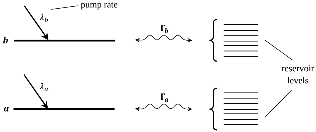
Figure 2.3 Relaxation processes of the open two-level atom [85].
