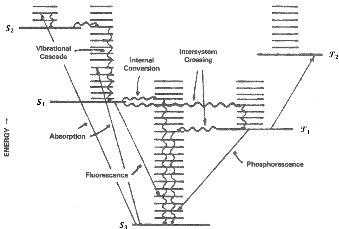
Figure 2.4 Molecular orbital energy level diagram, which shows the various photophysical processes that may be involved in a molecule [86].
