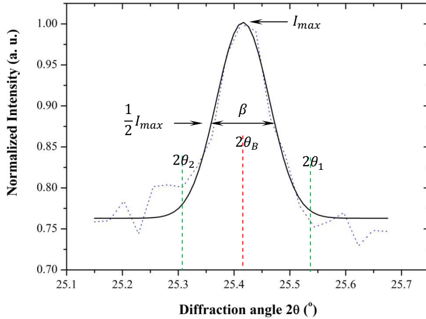
Appendix E.1 A XRD diffraction curve.
