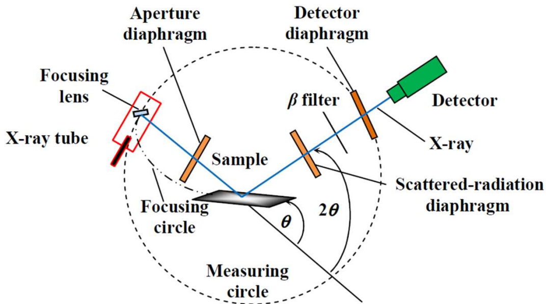
Figure 3.6 The components of a diffractometer with the beam path in the \theta/2\theta mode [97].
