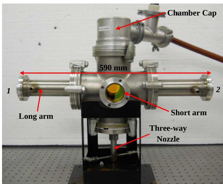
Figure 5.2 The reaction chamber inside which laser pyrolysis is carried out.
