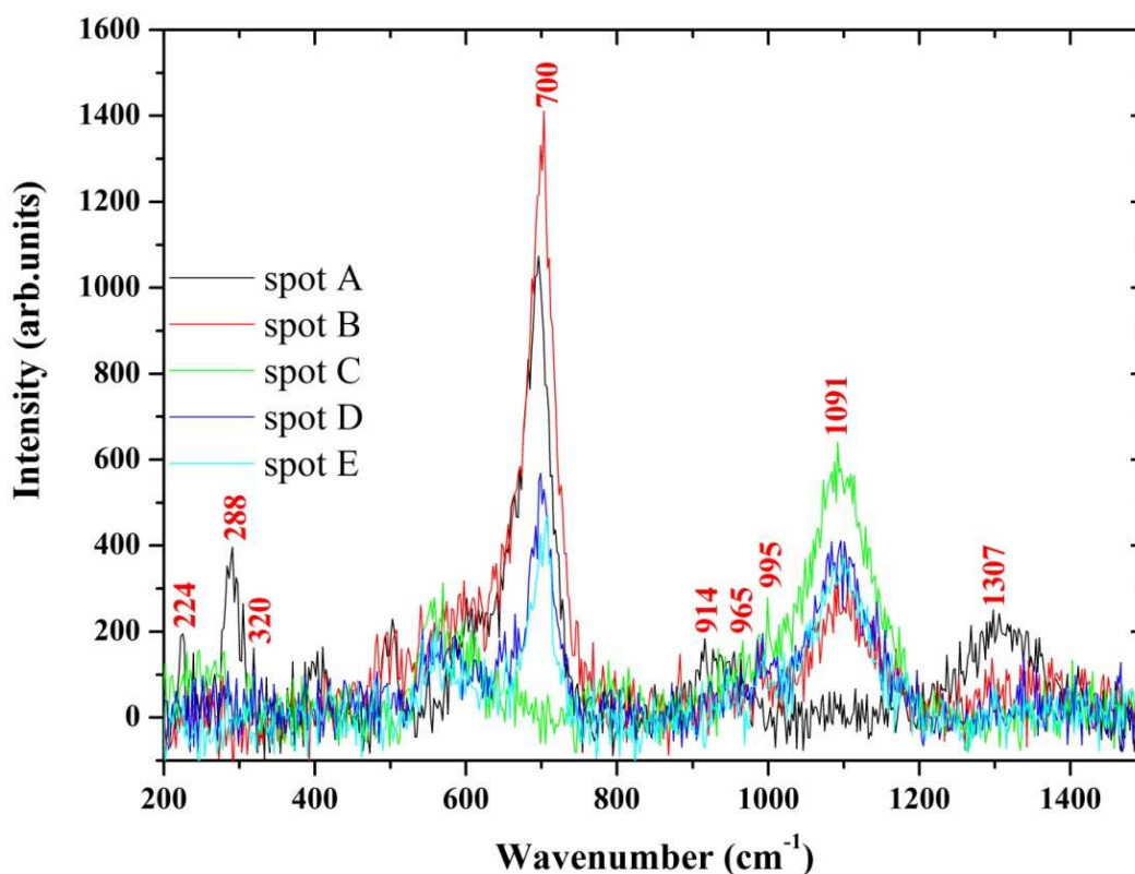
Figure 6.16 The Raman spectrum for the post-annealed sample containing the stars, slabs and the growths between the slabs.
