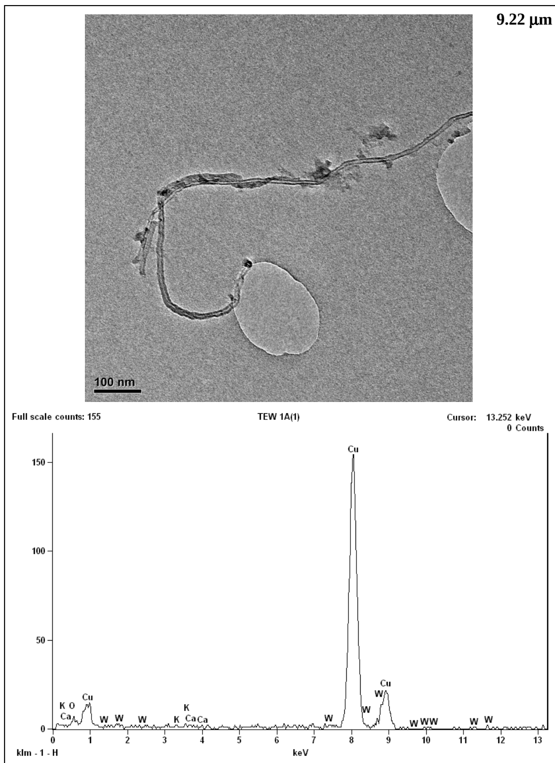
Appendix C.3 Top: A TEM micrograph showing a nanotube and Bottom: the EDX spectrum taken of the tube.
