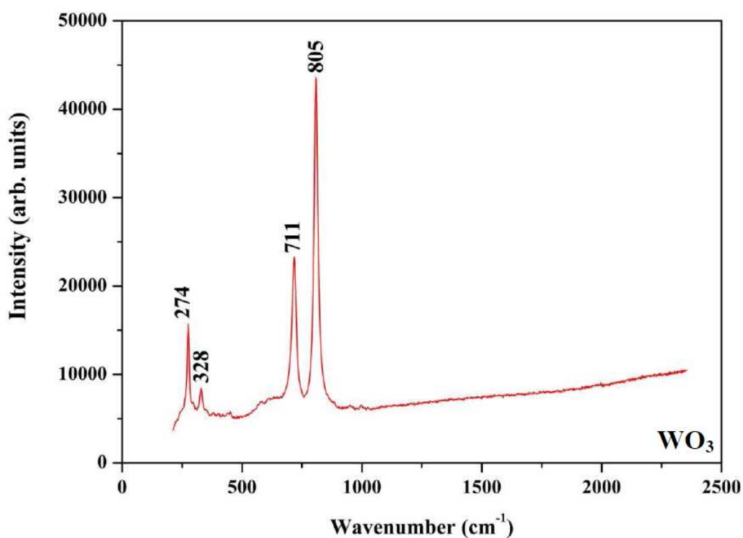
Figure 3.4 Raman spectrum of \text{WO}_3 , showing the characteristic peaks arising from the vibrational modes of the compound.
