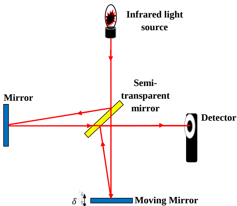
Figure 3.1 Illustration of the layout and components of an interferometer used in FTIR [90].
