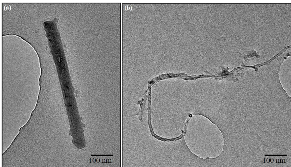
Figure 3.9 TEM micrographs of a (a) nanorod and (b) nanotube.
