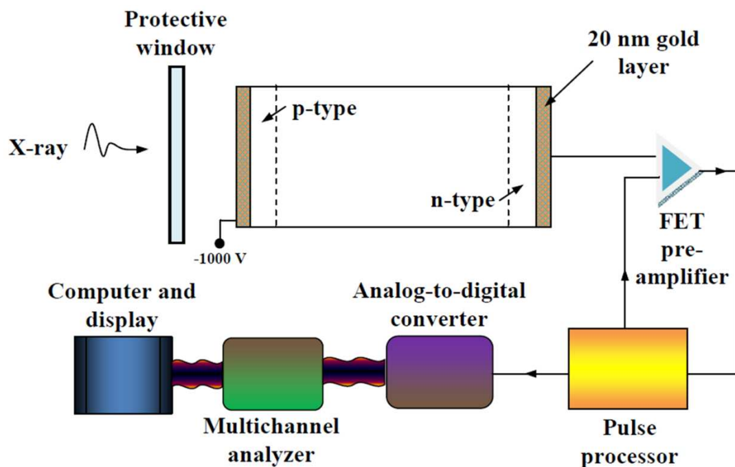
Figure 3.13 A schematic diagram of an EDX detector and its signal processing circuitry [92].
