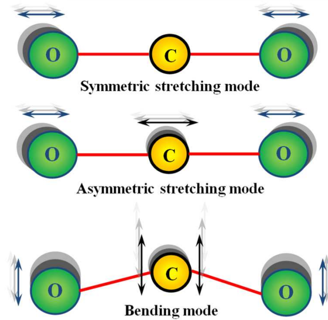
Figure 4.2 An illustration of the three possible vibrational modes of the CO 2 molecule [100].
