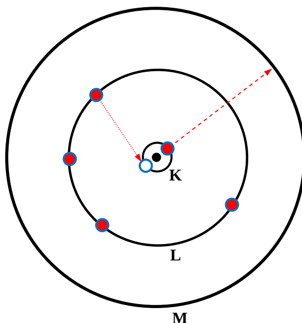
Figure 3.12 The electron orbits of an atom with the electron shells designated by K, L and M, with quantum numbers n equal to 1, 2 and 3, respectively. A K-shell electron is excited to the empty M-shell, and an L-shell electron fills the K-shell vacancy in a de-excitation process.
