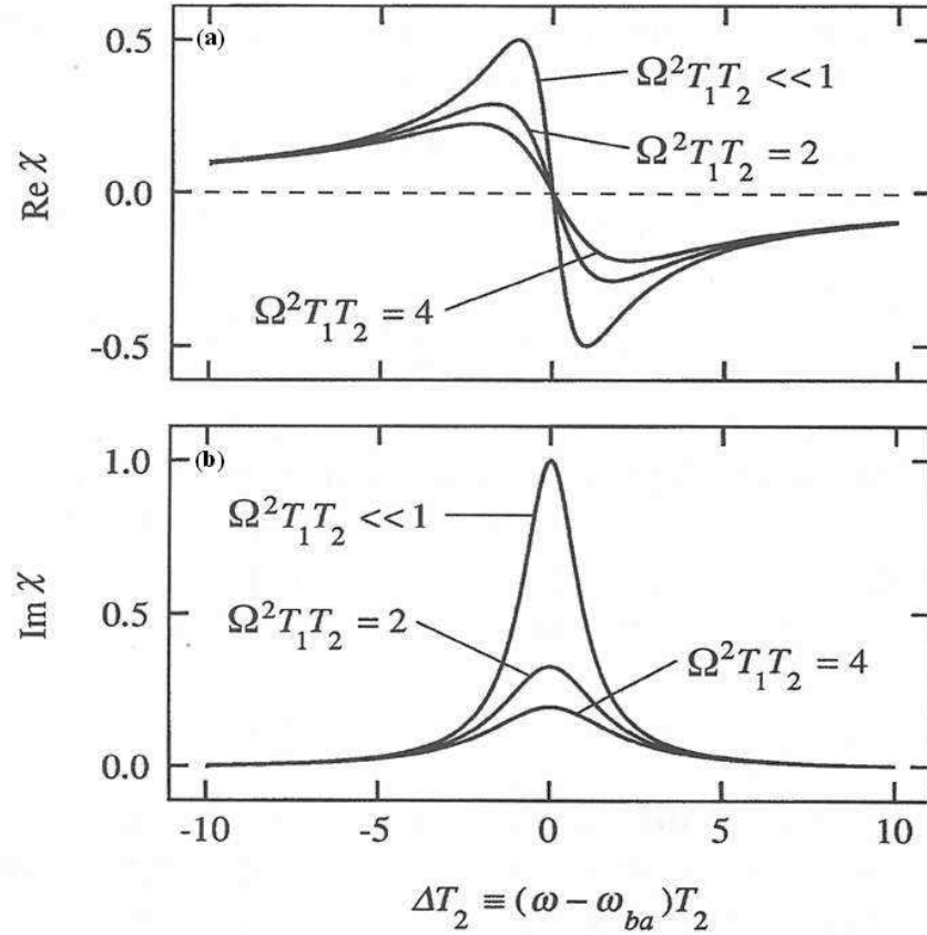
Figure A.2 (a) Real and (b) imaginary parts of the susceptibility (in units \alpha_0 c / \omega_{ba} ) plotted as functions of the optical frequency \omega for several values of the saturation parameter \Omega^2 T_1 T_2 [86].
