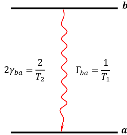
Figure 2.2 Relaxation processes of the closed two-level atom [85].
