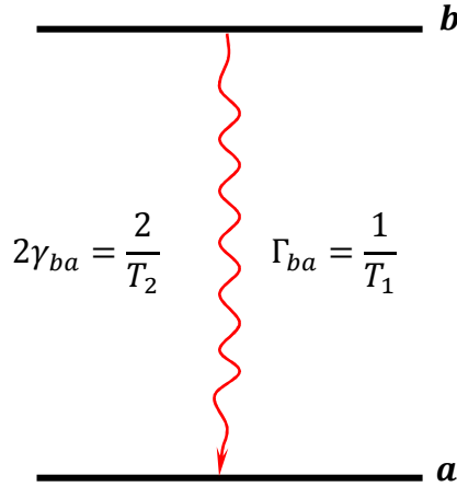
Figure A.1 Relaxation processes of the closed two-level atom [86].
