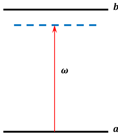
Figure 2.1 Near-resonant excitation of a two-level atom [85].
