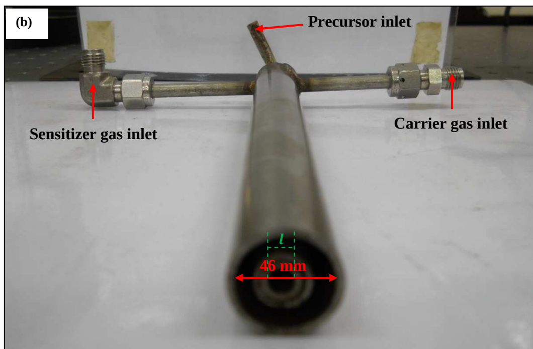
Figure 5.3 (b) A close-up of the three-way nozzle.
