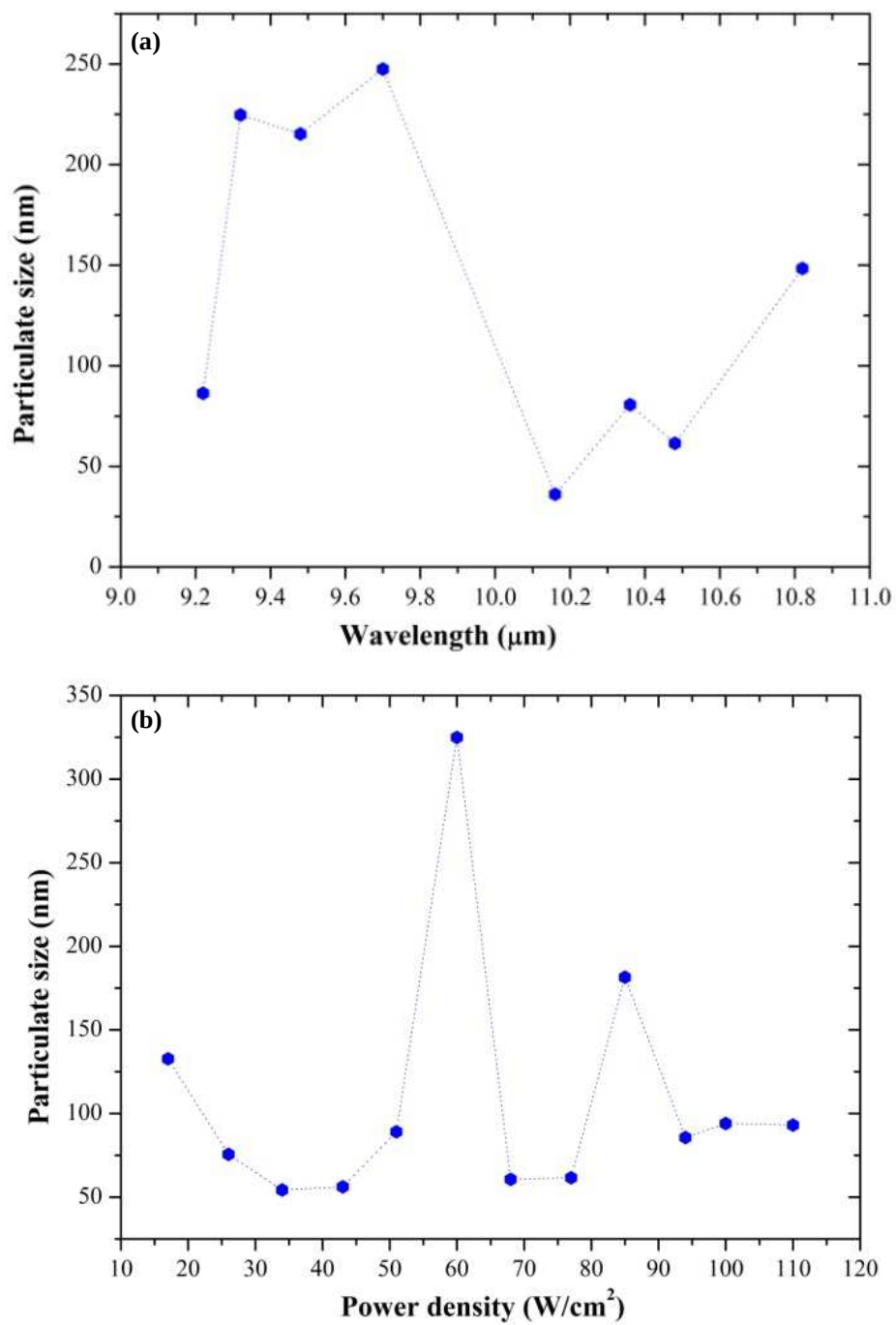
Figure 6.9 The particulate sizes for the samples shown in the SEM micrographs above, were calculated from the XRD spectra for the respective samples and Scherrer's formula, for the various (a) wavelengths at the 51.2 \text{W}/\text{cm}^2 power density and (b) power densities at the 10.6 \mu\text{m} wavelength.
