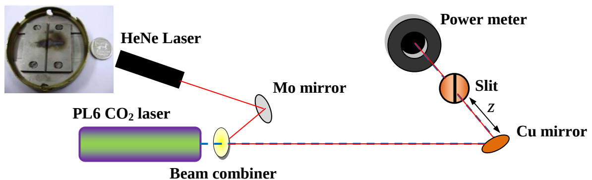
Figure 4.7 A schematic of the setup used to characterize the CO 2 laser beam using a thin slit. The inset shows the slit size relative to a South African one rand coin.
