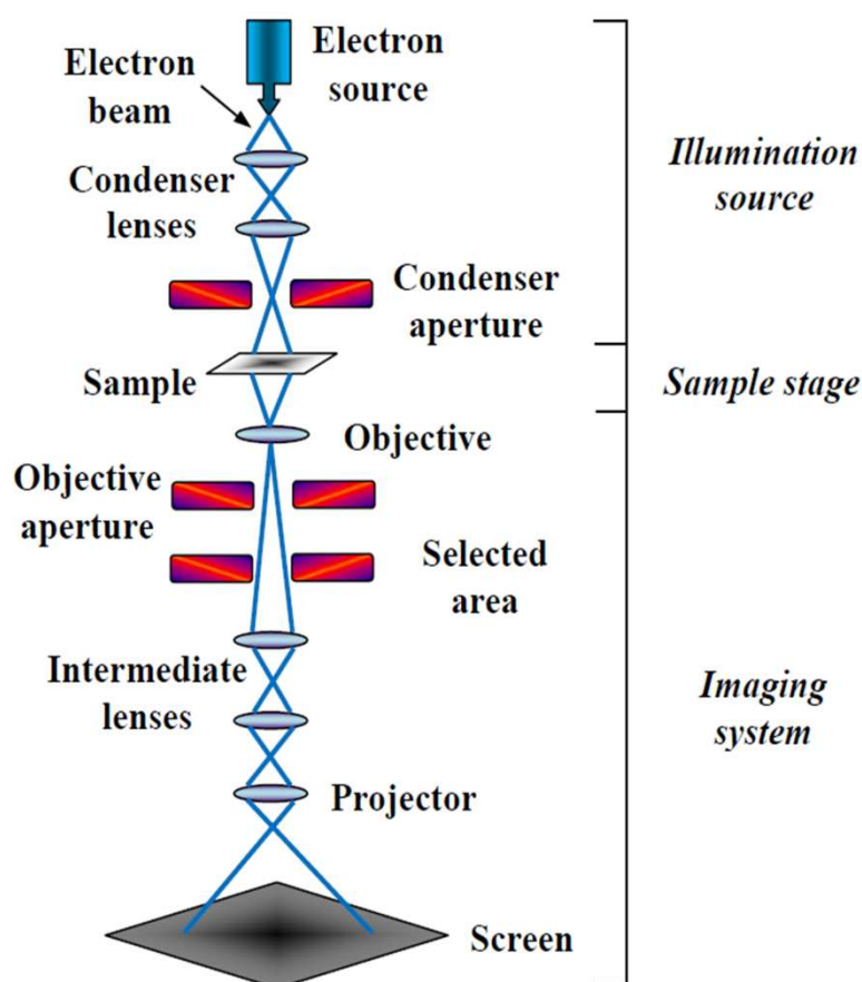
Figure 3.8 An illustration of the layout and components of a transmission electron microscope [95].
