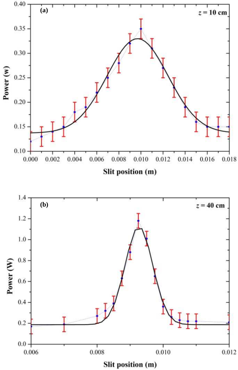
Figure 4.10 (a)-(b) Plots of the power for varying slit positions at various propagation distances between the focusing mirror and thin slit.
