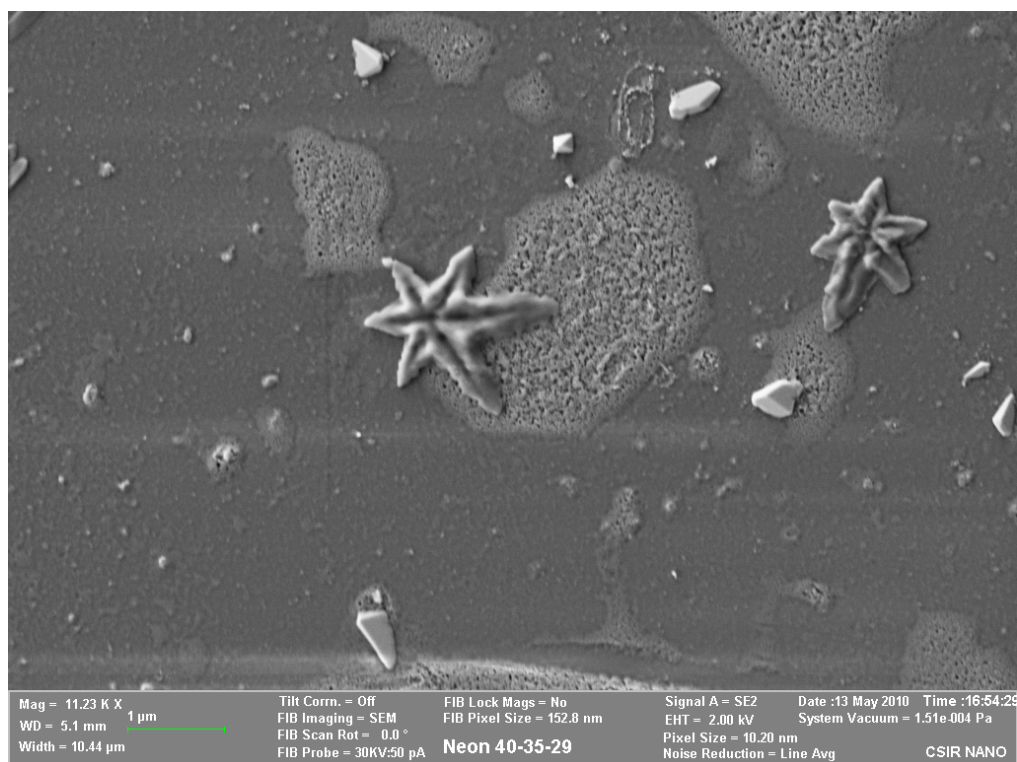
Figure 6.13 SEM micrographs ( \times 11230 ) of the post-annealed sample showing the stars that formed during annealing, prepared at the 10.6\ \mu\text{m} wavelength and power density of 2.2\ \text{kW}/\text{cm}^2 .
