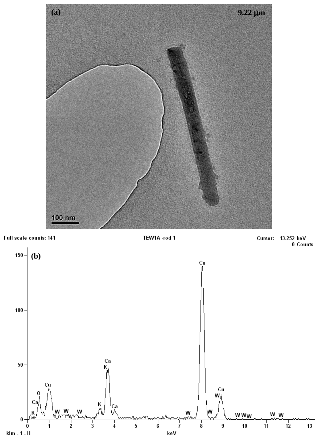
Figure 6.5 (a) A TEM micrograph showing a nanorod and (b) the EDX spectrum taken of the rod.
