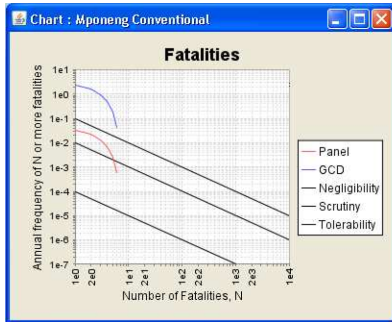
Figure 6-25: FN plot
