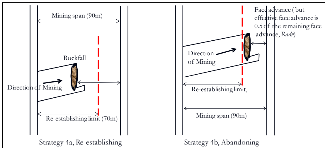
Figure 4-9: Re-establishing or abandoning criteria
