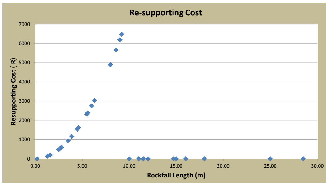
Figure 5-21:Re-supporting cost
