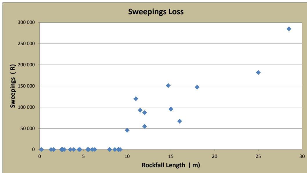
Figure 5-23: Sweepings loss
