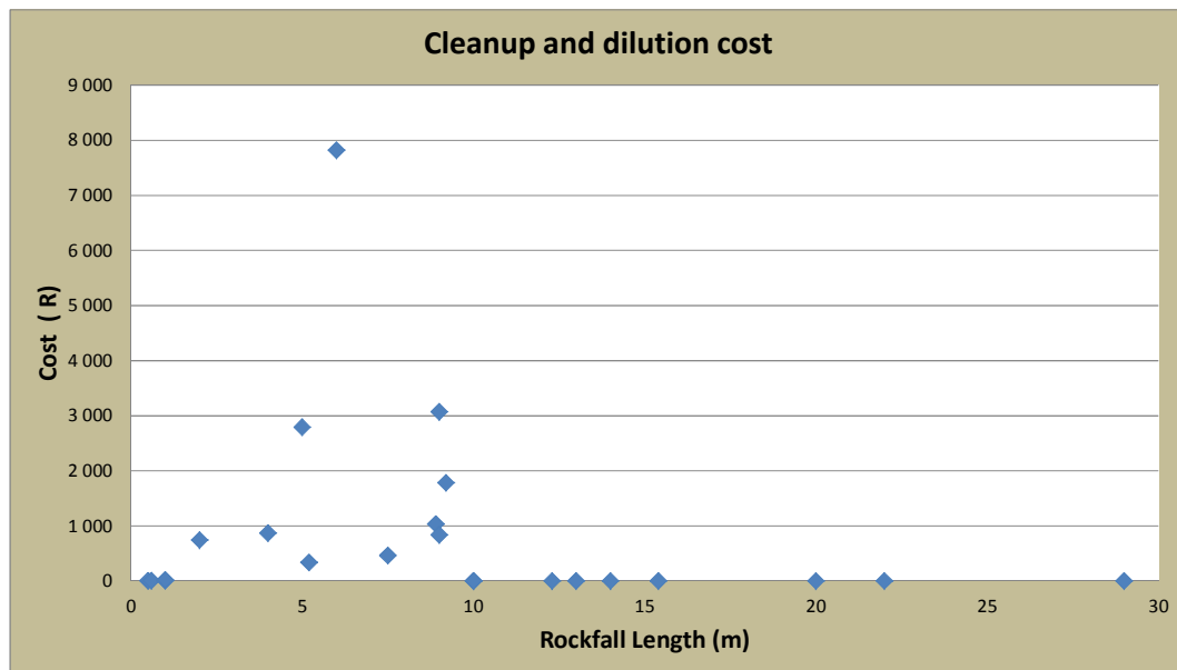
Figure 5-5: Cleanup and dilution cost
