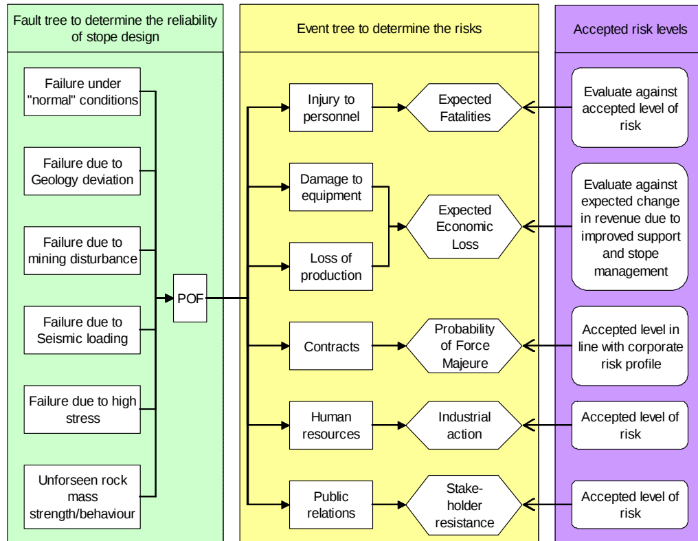
Figure 2-5: Risk evaluation process (Stacey et al, 2006)
