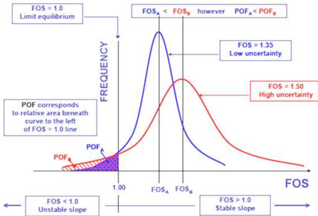
Figure 2-3: Uncertainty in slope design (after Tapia et. al 2007)
