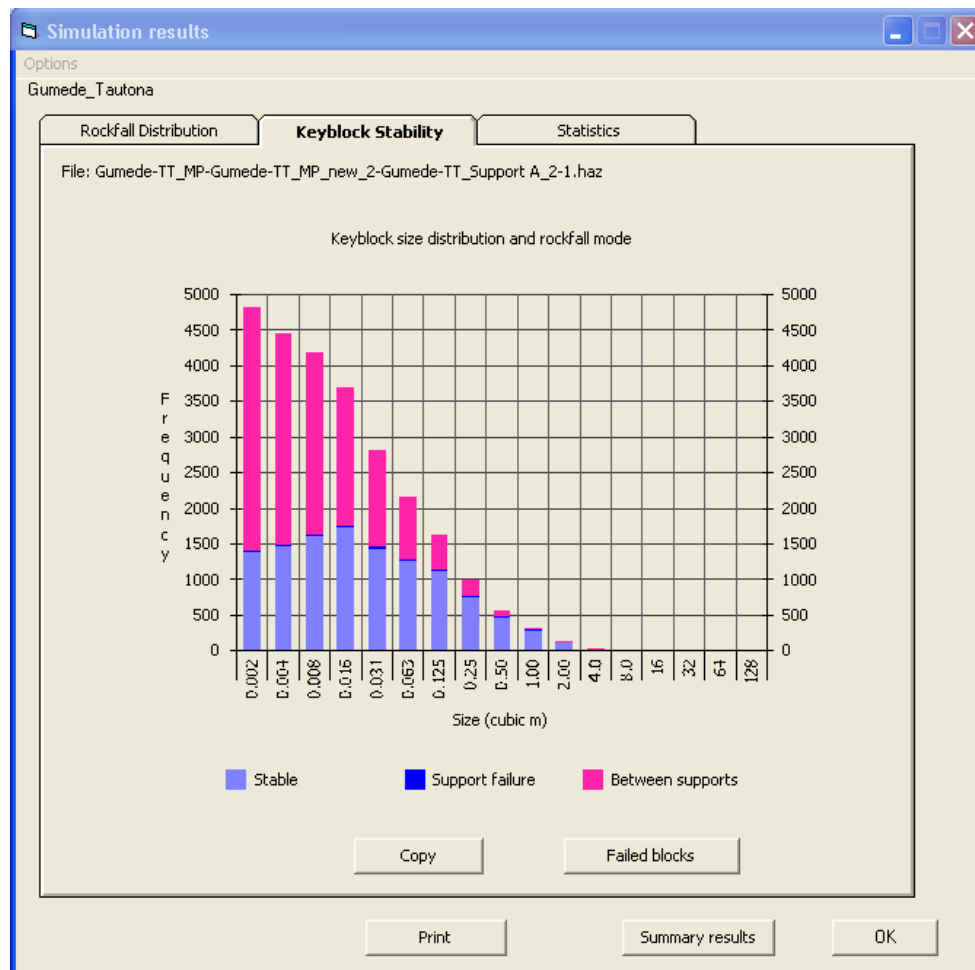
Figure 6-5: Scenario B rockfalls
