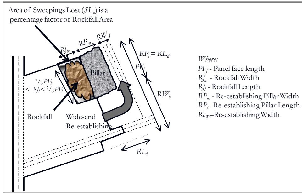
Figure 4-7: Class 3, re-establishing
