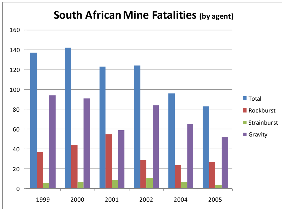
Figure 1-2: Fatal rockfall accidents analysis
