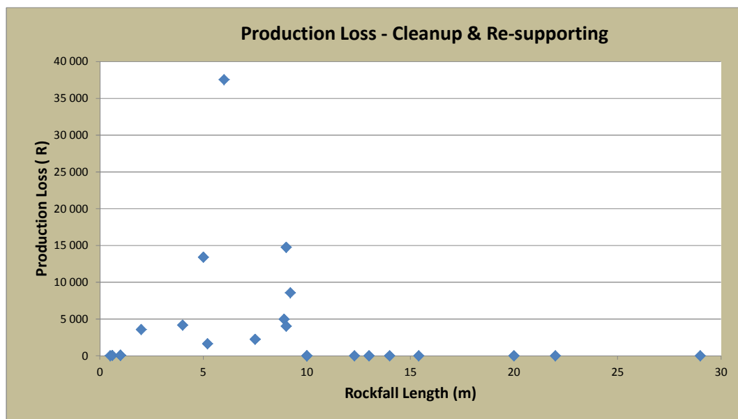
Figure 5-7: Production loss – cleanup and re-supporting
