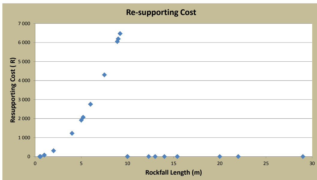
Figure 5-6: Re-supporting cost
