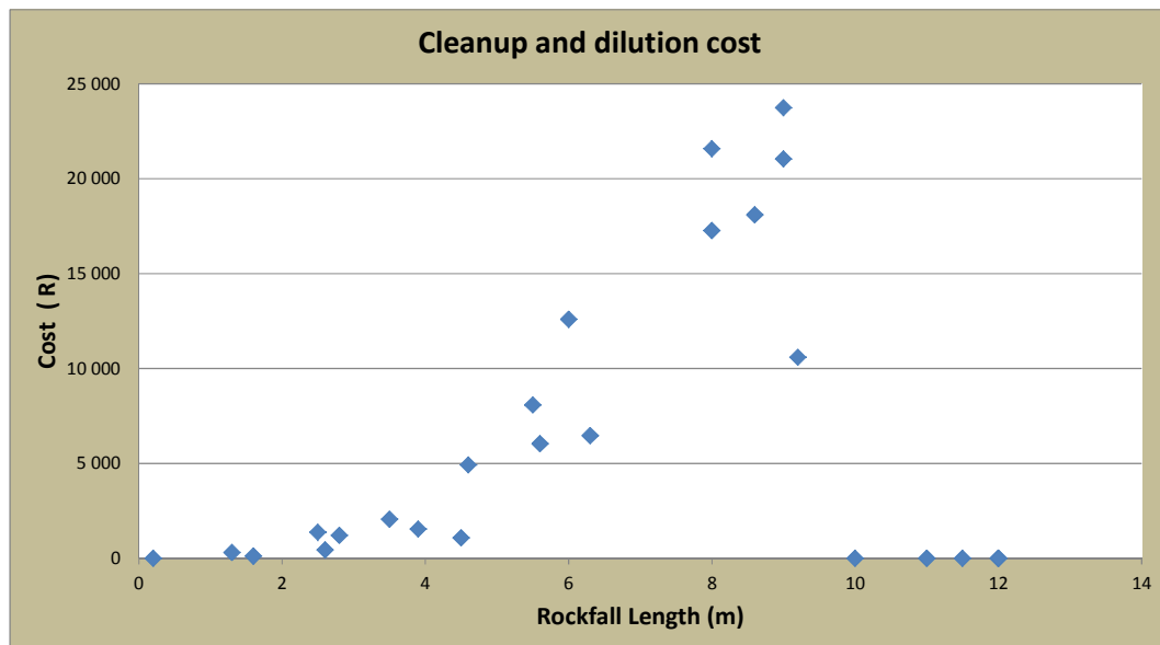
Figure 5-20: Cleanup and dilution cost curve
