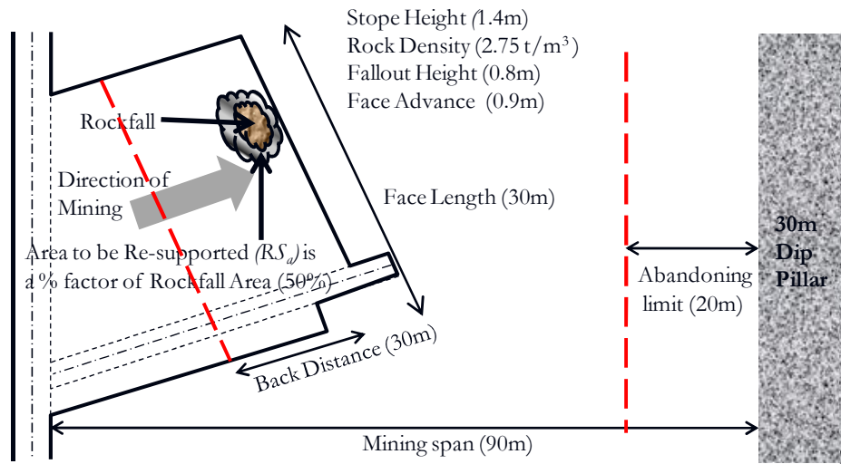
Figure 5-1: Mining parameters
