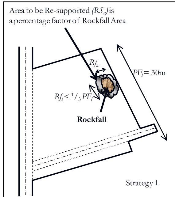
Figure 4-6: Class 2, cleanup and re-support
