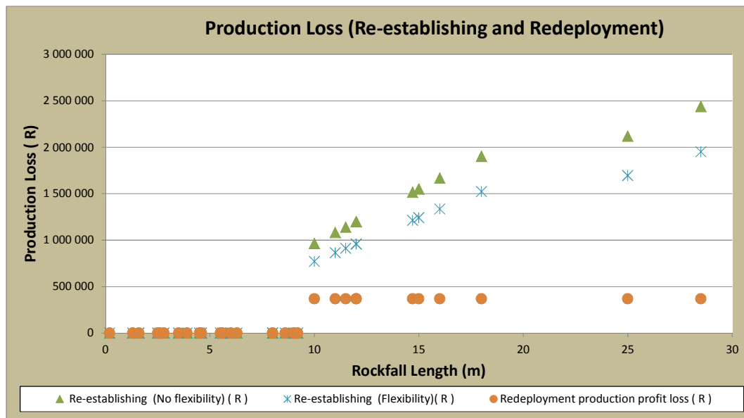
Figure 5-24: Production loss – re-establishing and redeployment
