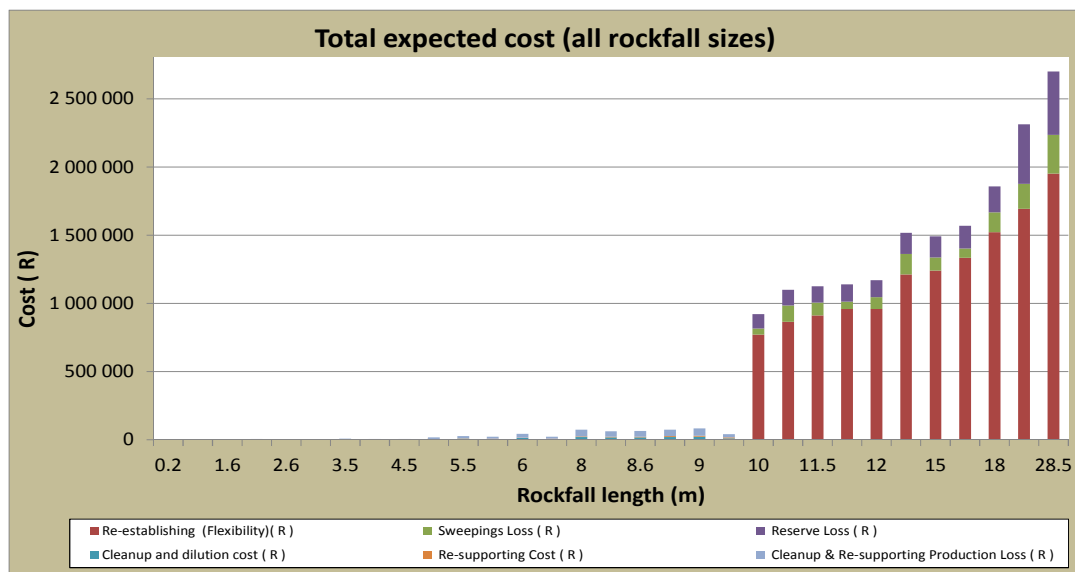
Figure 5-26: Total expected costs (all sizes)
