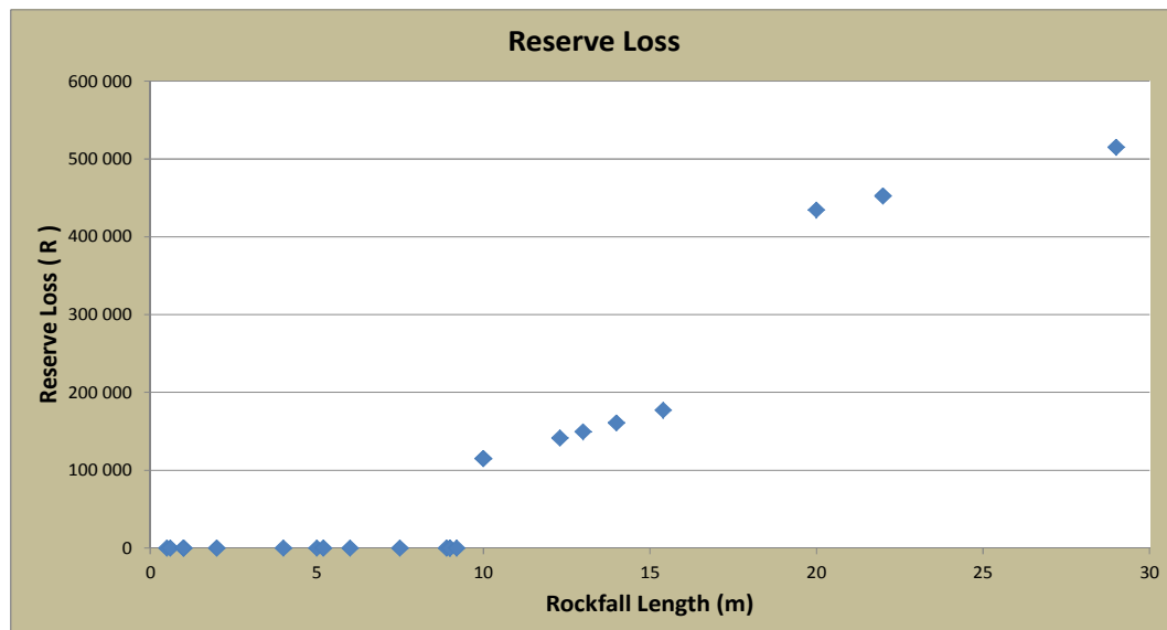
Figure 5-10: Reserve losses
