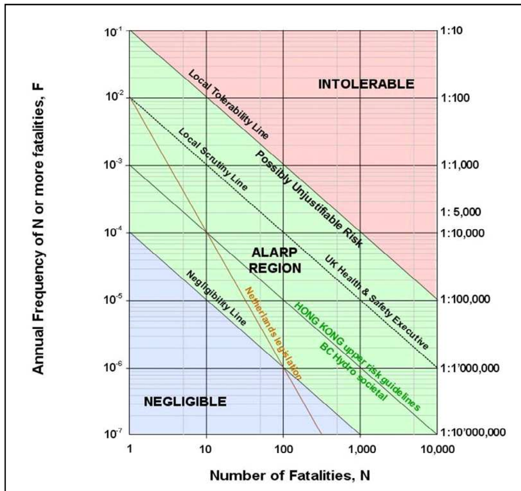
Figure 2-7: F-N Graph for bench marking safety impact (Contreras et al, 2006)
