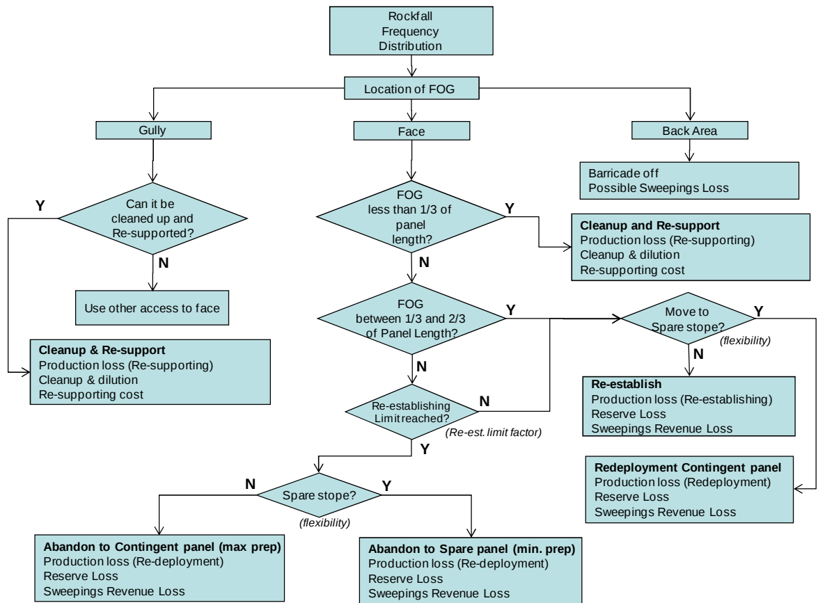
Figure 4-4: Stope damage event tree
