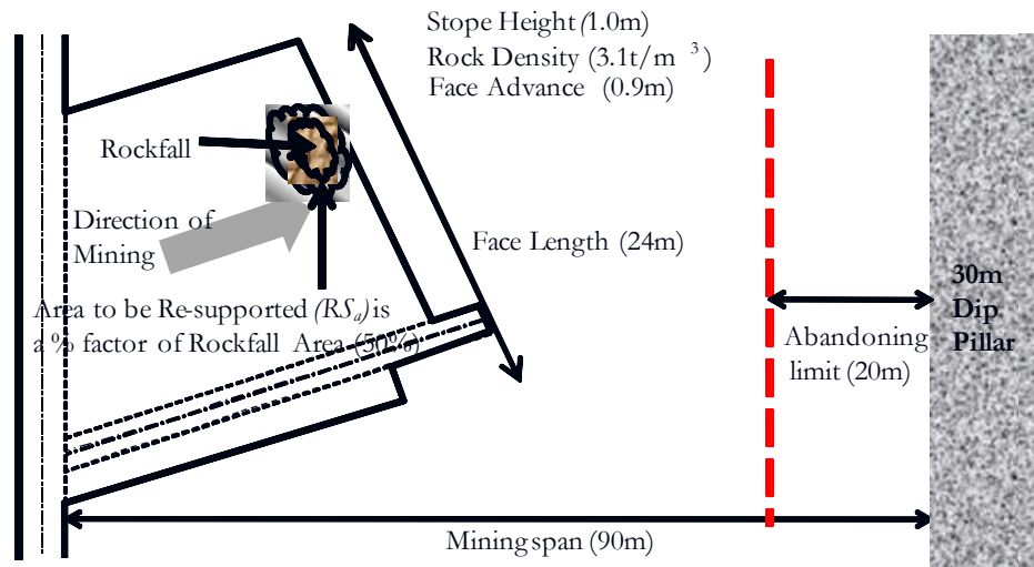
Figure 5-14: Mining parameters
