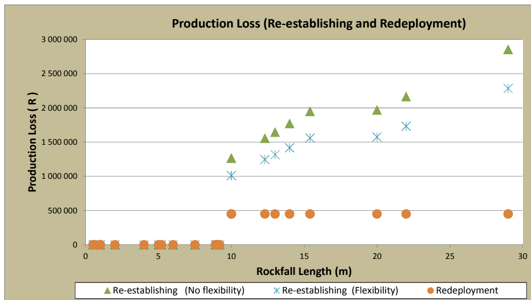
Figure 5-9: Production loss- re-establishing and redeploying
