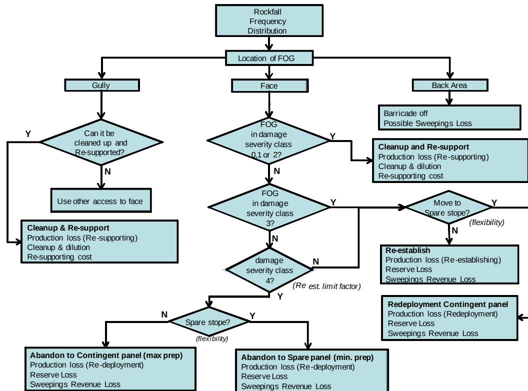
Figure 5-4: Stope damage
