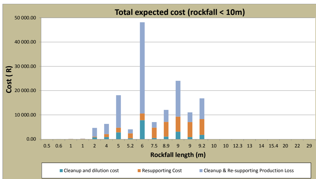
Figure 5-12: Total expected costs (rockfalls < 10m)
