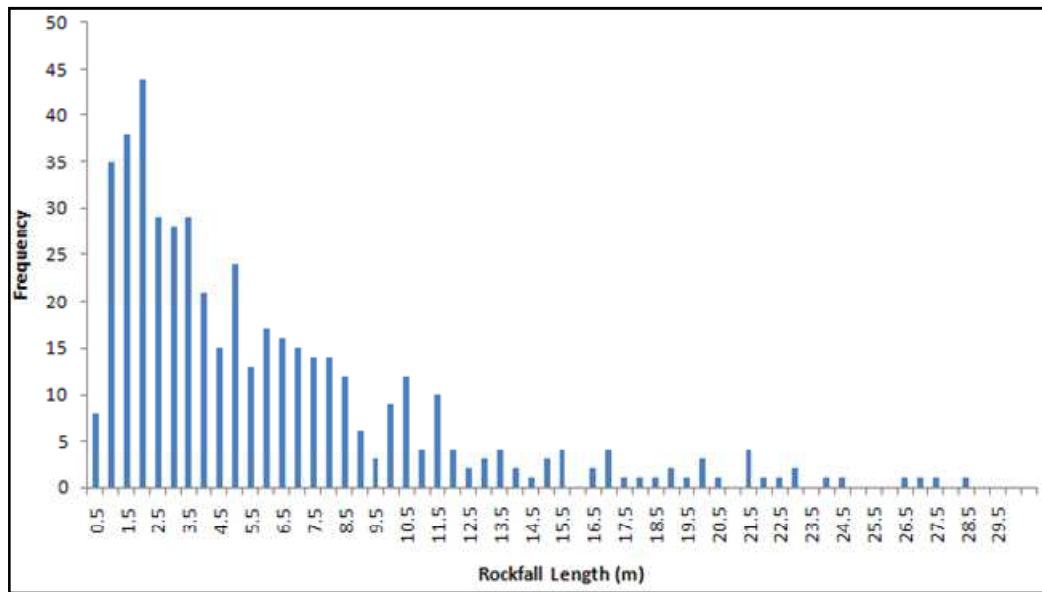
Figure 4-3: Rockfall frequency
