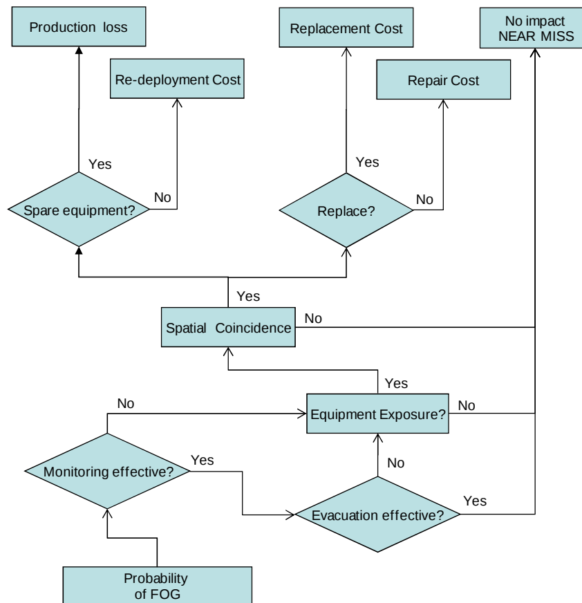
Figure 4-11: Equipment damage model event tree
