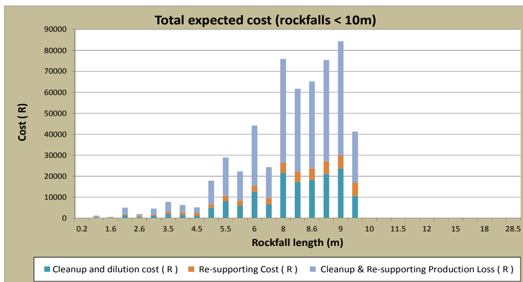
Figure 5-27: Total costs (rockfalls < 10m)
