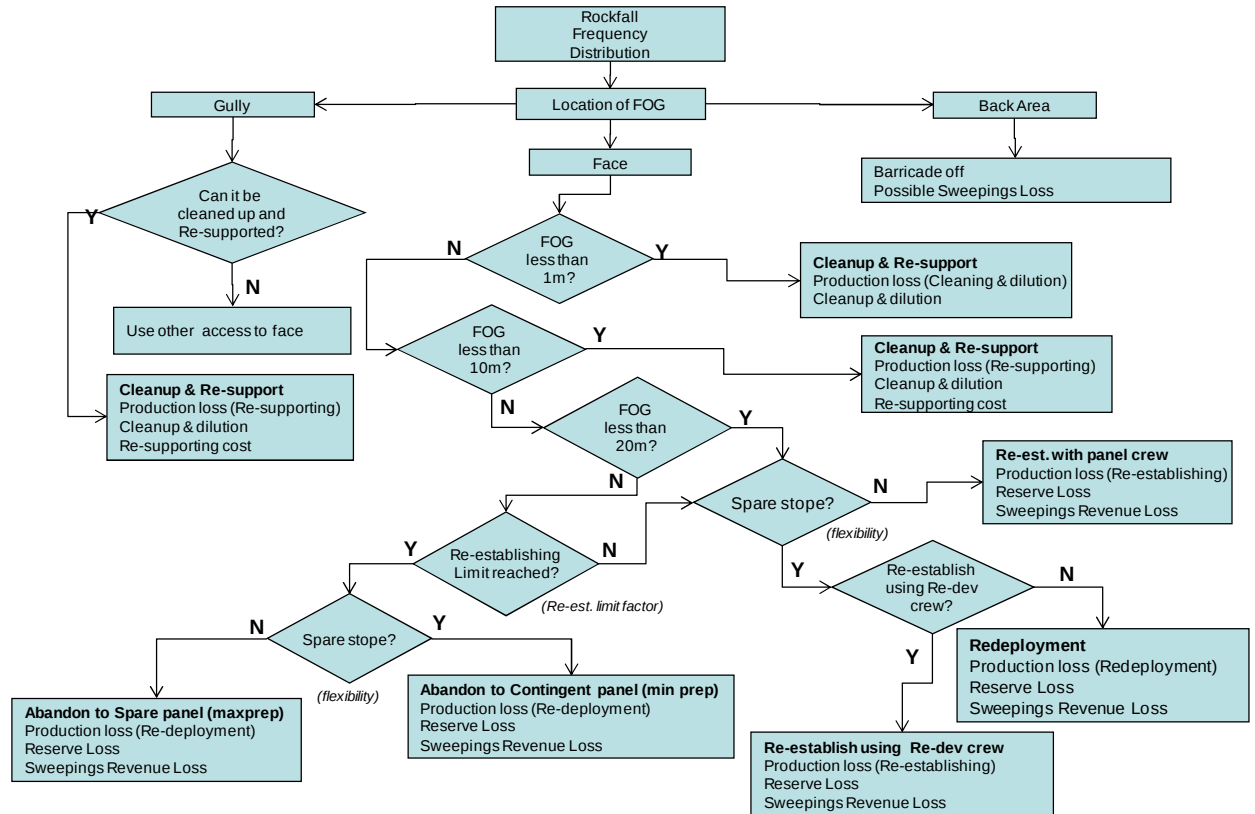
Figure 5-19: Stope damage event tree
