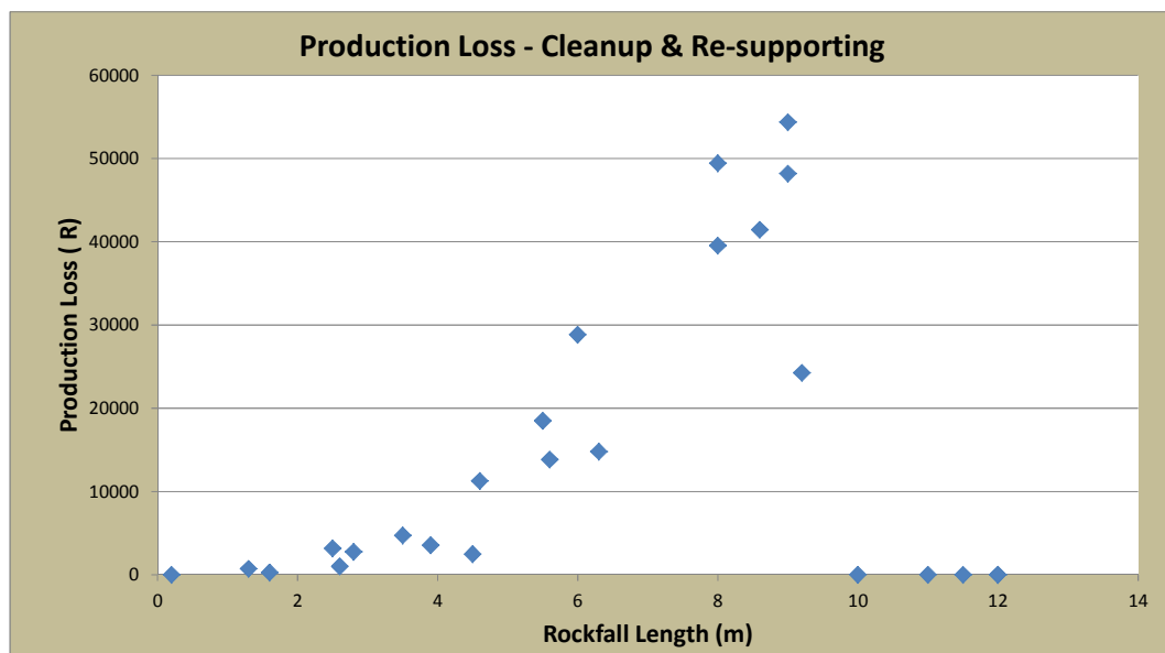
Figure 5-22: Production loss – cleanup& re-supporting
