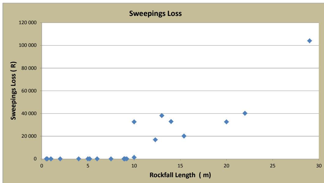
Figure 5-8: Sweepings loss
