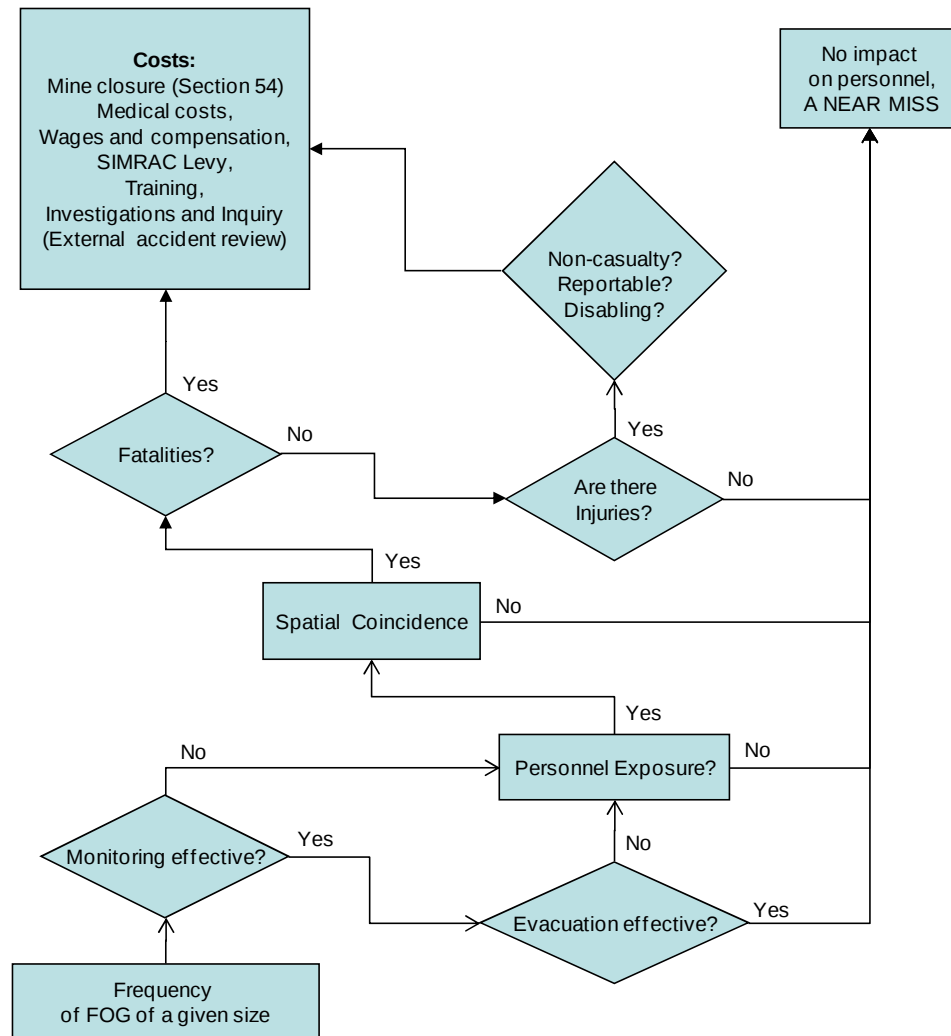
Figure 4-10: Personnel injury and fatality event tree
