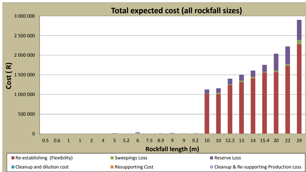
Figure 5-11: Total expected costs (all rockfall sizes)
