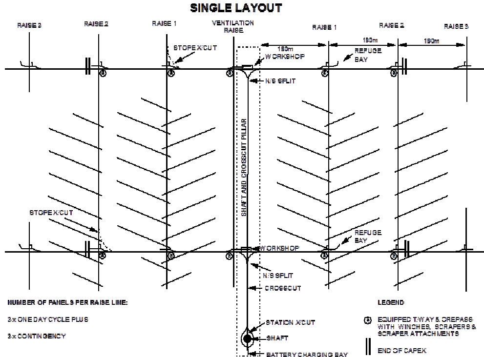
Figure 5-13: Conventional mining layout (Impala Standards, 2008)
