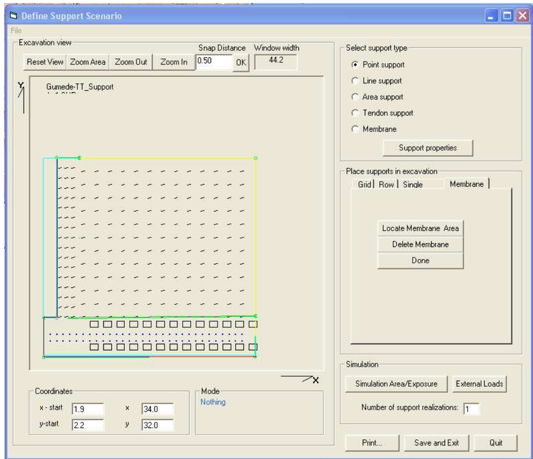
Figure 6-1: Scenario A support
