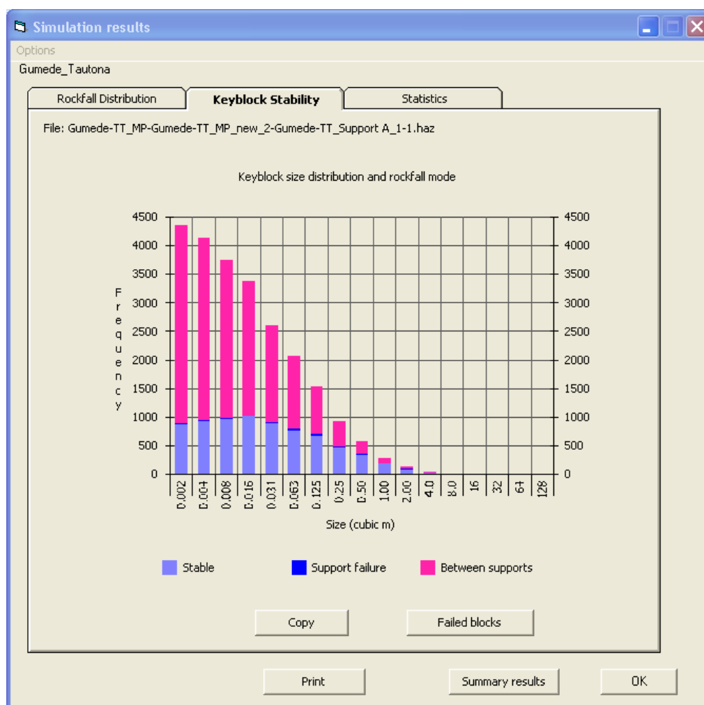
Figure 6-4: Scenario A rockfalls
