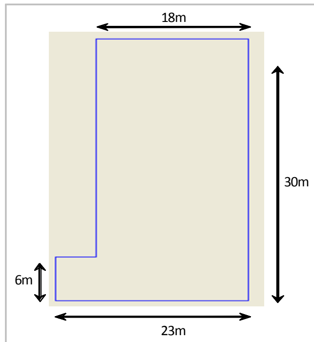
Figure 6-3: Excavation geometry
