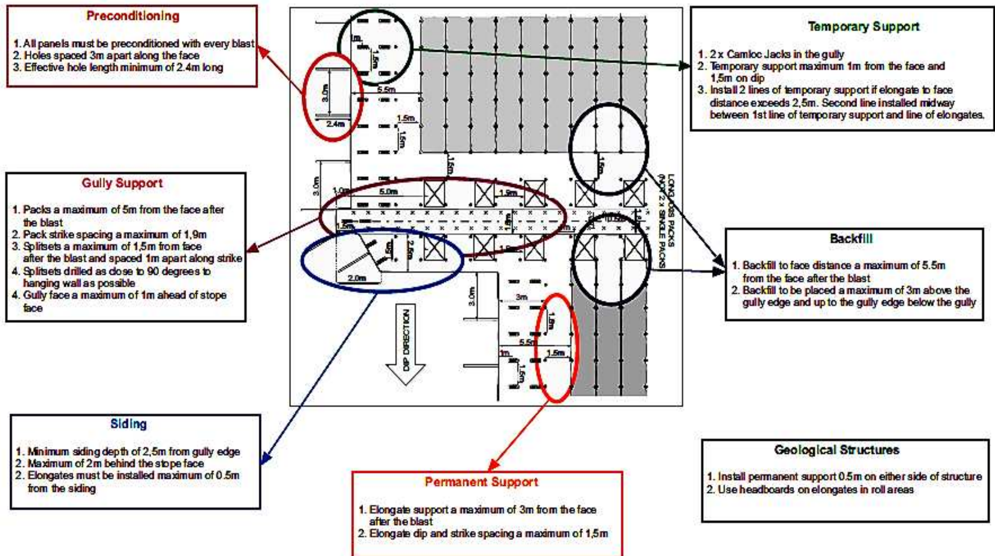
Figure 5-2: Stope support standard (Mponeng COP, 2008)
