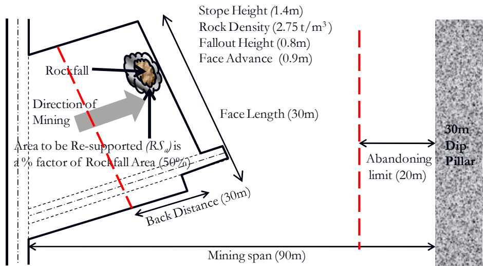
Figure 6-15: Mining parameters
