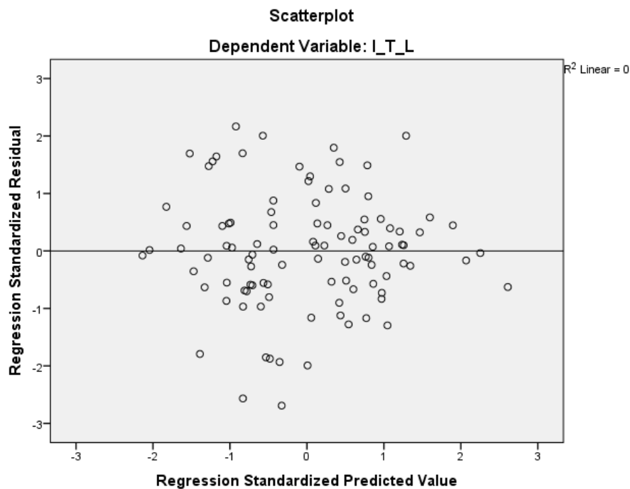
Figure 5: Homoscedasticity Diagnostic
