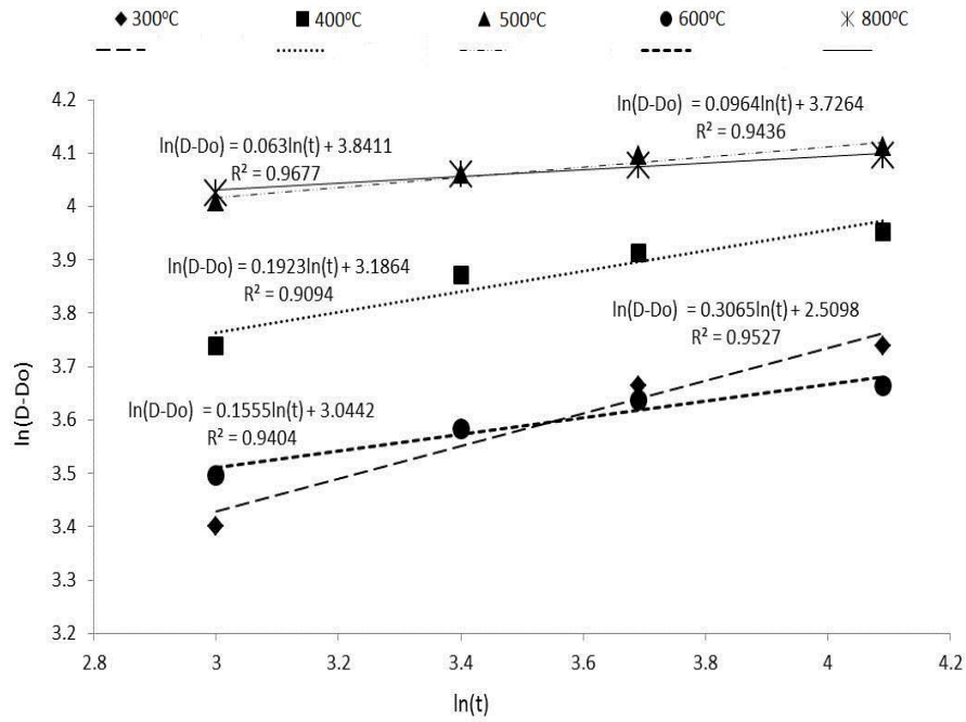
Figure 5.5: \ln(D-D_0) vs. \ln(t) for annealing the Timetal 125 style alloy at different temperatures.
