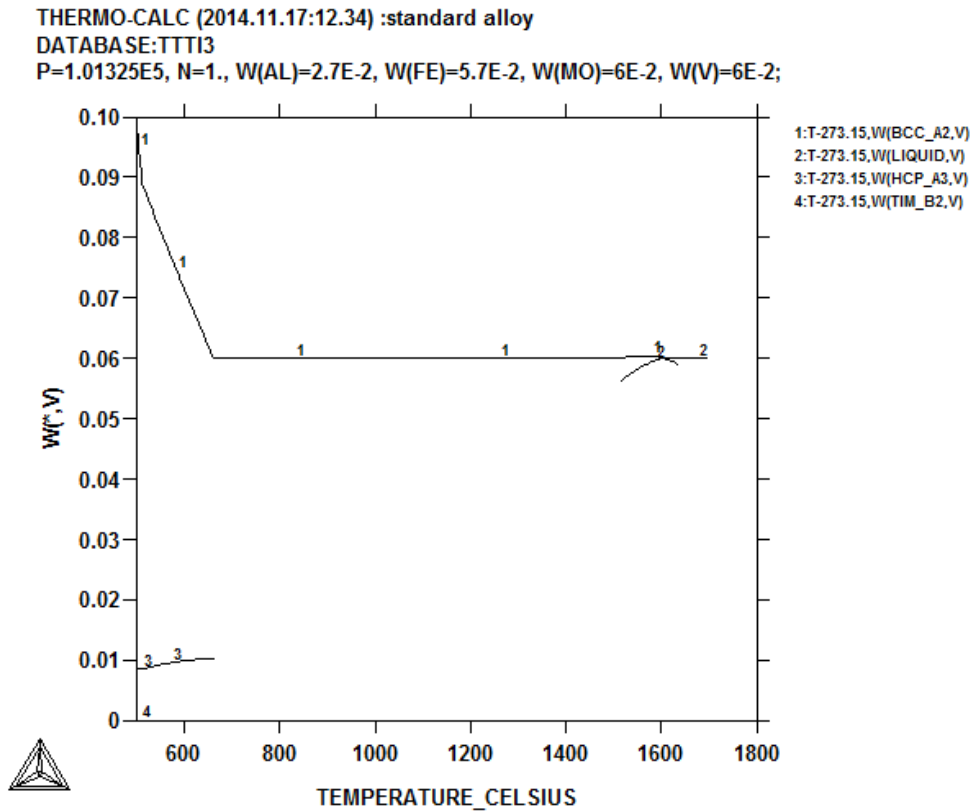
Figure 4.65: Partitioning of vanadium during equilibrium cooling of Timetal 125 calculated by Thermo-Calc using the titanium alloy database V3 (TTTI3).
