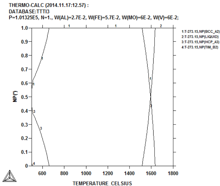
Figure 4.58: Thermo-Calc temperature-phase proportion plot of the phase composition of Timetal 125 using the titanium alloy database V3 (TTTI3).
