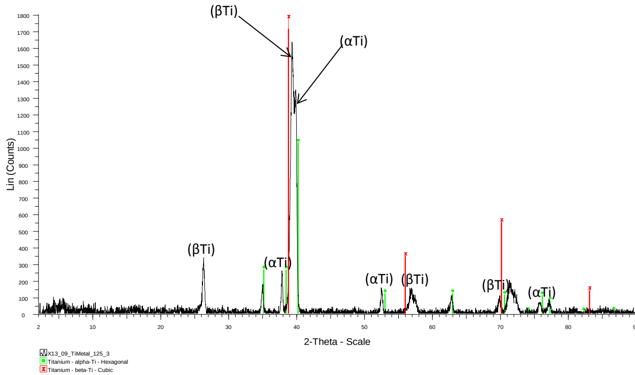
Figure 4.20: XRD pattern of the Timetal 125 style alloy in the as-cast condition.
