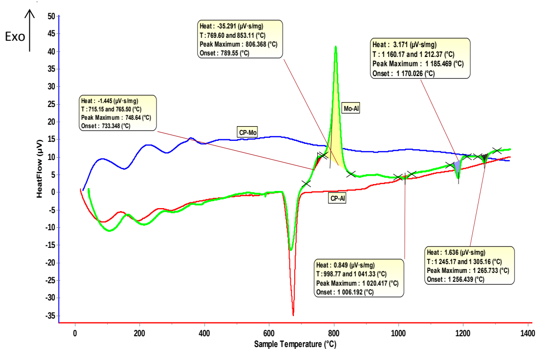
Figure 4.16: Superposed DTA scans for pure aluminium, pure molybdenum and a 50-50 wt% Al-Mo binary alloy.
