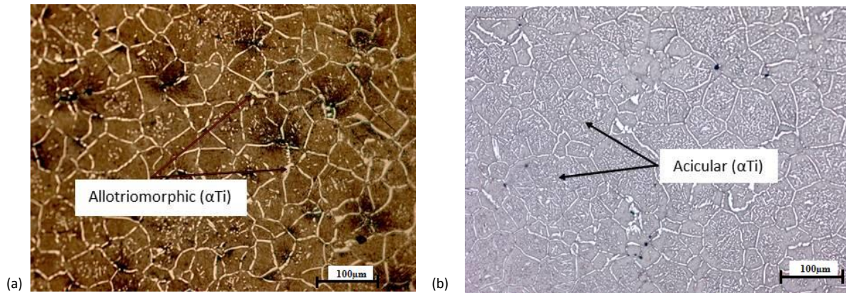
Figure 4.51: Optical micrographs of Timetal 125 after solution treatment at 900°C for 60 minutes followed by artificial ageing at 500°C for (a) 20 mins, and (b) 60 mins (micron bars = 100µm).
