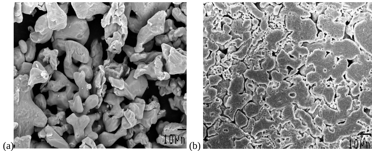
Figure 2.12: SEM micrographs of Ti-47Al after spark plasma sintering at 50MPa at a heating rate of 50°C.min -1 at (a) 400°C and (b) 900°C (Xiao et al., 2009).
