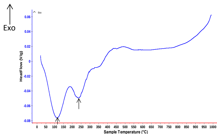
Figure 4.2: DTA scan for a blank run showing low temperature peaks due to a systematic error of the instrument.
