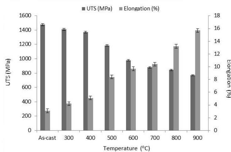
Figure 8: Ultimate tensile strength and elongation of Ti-2.7Al-5.7Fe-6Mo-6V after annealing the cast alloy at different temperatures.
