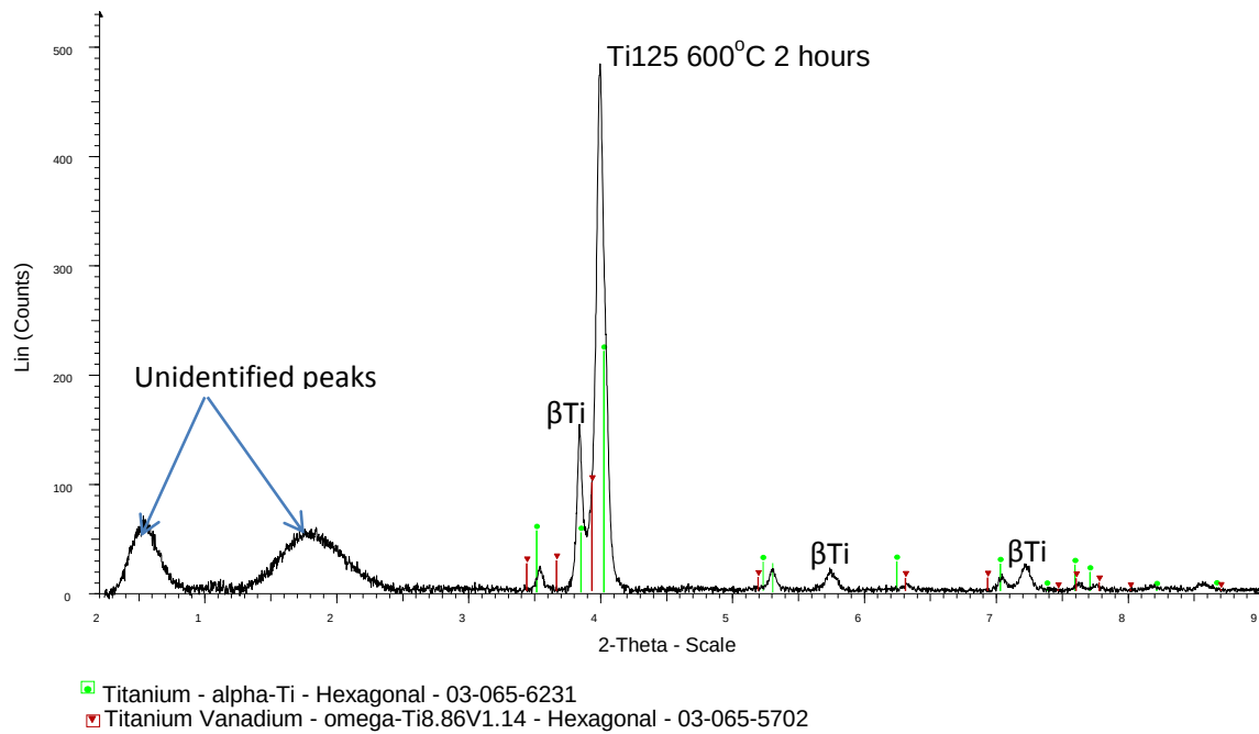
Figure 4.37: XRD pattern of the Timetal 125 style alloy annealed at 600°C for 2 hours, followed by water-quenching (2 theta in degrees).
