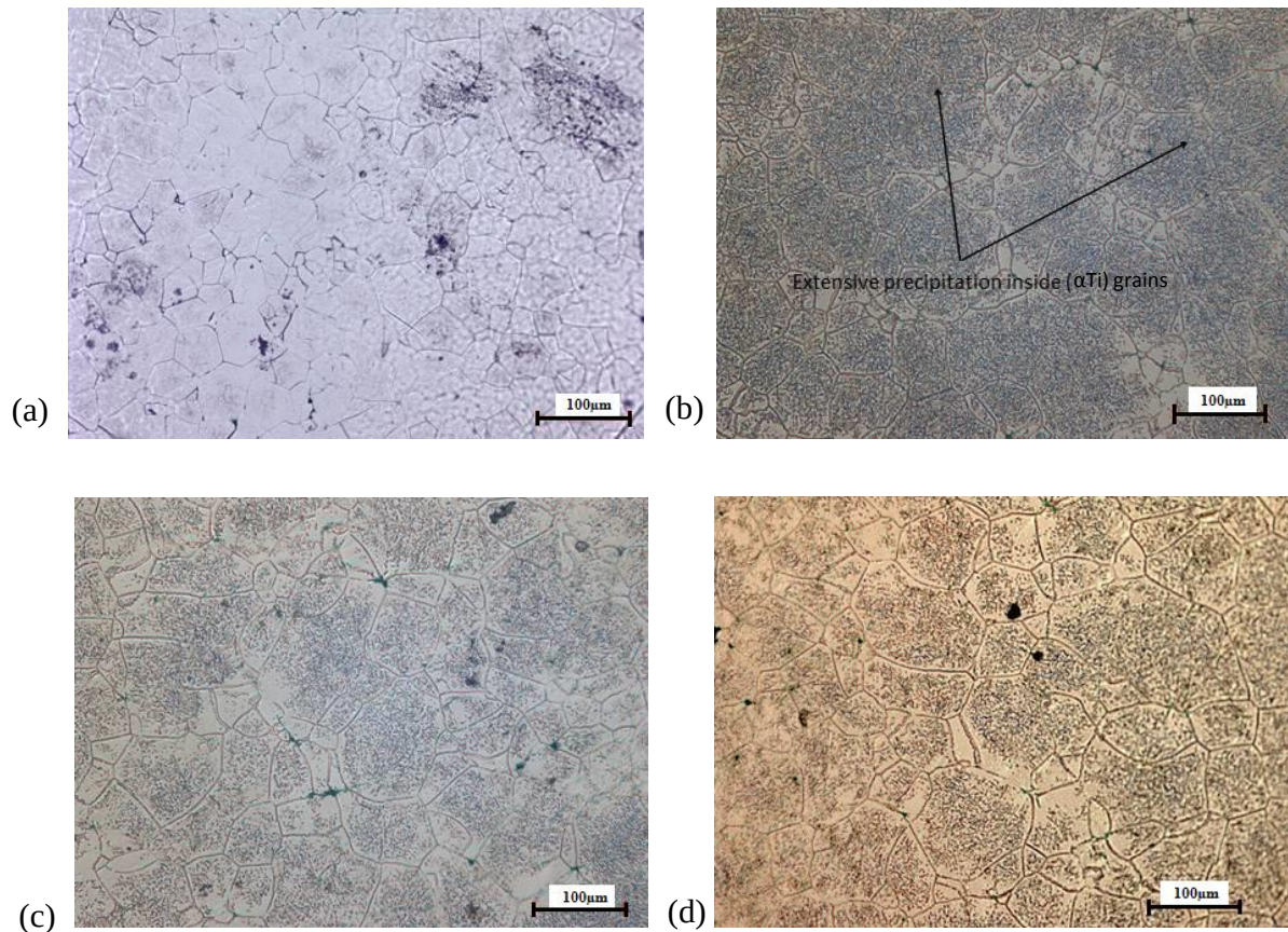
Figure 4.30: Optical micrographs of the Timetal 125 style alloy heat treated at 300°C for (a) 20 mins, (b) 30 mins, (c) 40 mins, and (d) 60 mins (all micron bars = 100μm).
