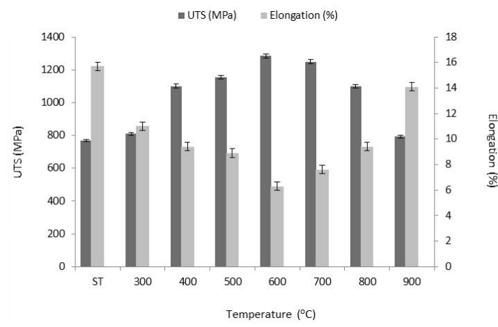
Figure 10: Ultimate tensile strength and elongation of Ti-2.7Al-5.7Fe-6Mo-6V after solution-treatment and ageing at different temperatures (ST stands for solution-treated).
