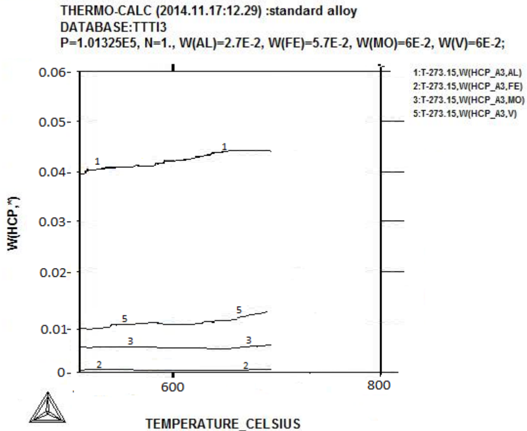
Figure 4.61: Composition of hcp Ti as function of temperature, calculated by Thermo-Calc for the Timetal 125 composition using the titanium alloy database V3 (TTTI3).
