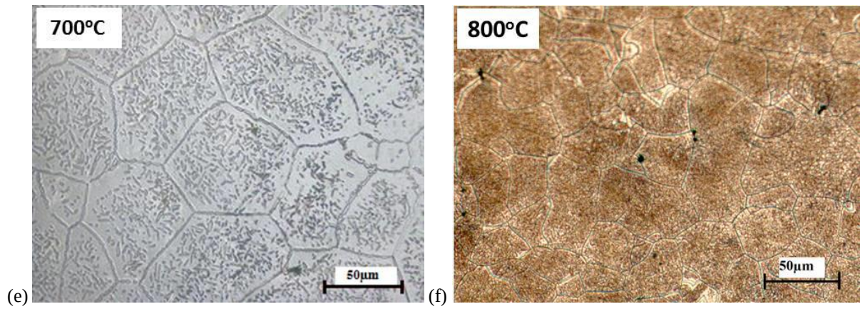
Figure 9: Optical micrographs of Ti-2.7Al-5.7Fe-6Mo-6V after solution-treatment and ageing at different temperatures for 2h.
