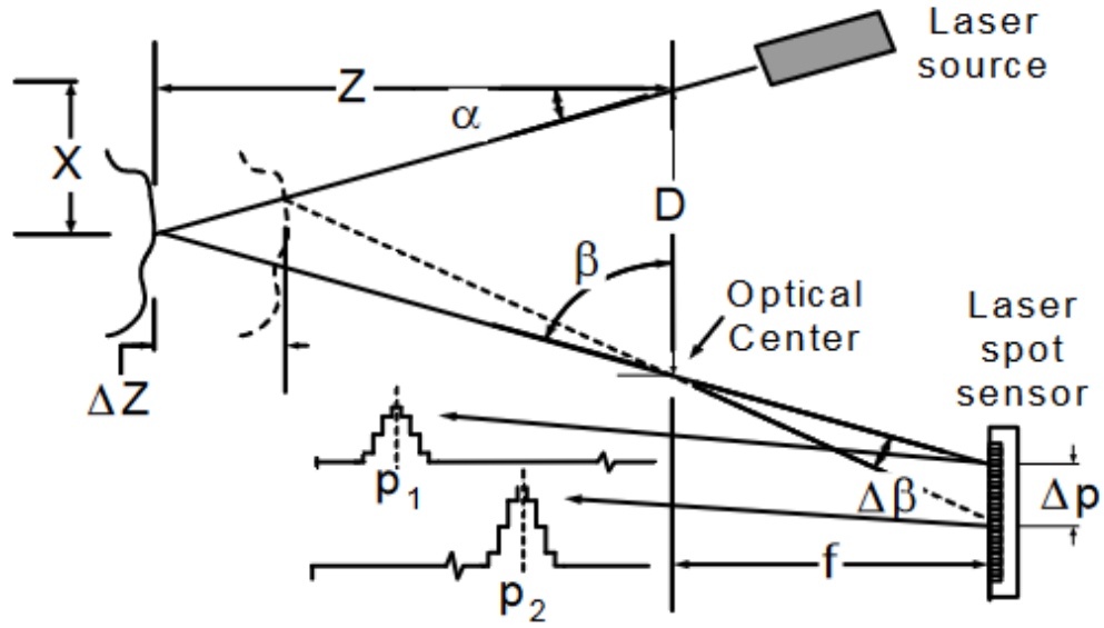
Figure 1.4: Triangulation principle using LiDAR (Beraldin, 2004).
