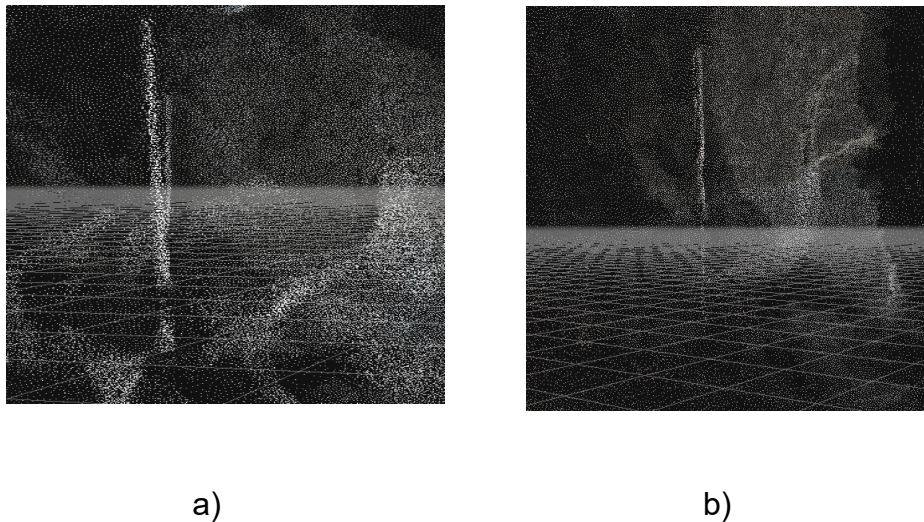
Figure 5.10: Comparison of fused LiDAR and CRP point clouds with fluorescent tube objects in a) unstructured datasets and b) structured datasets.
