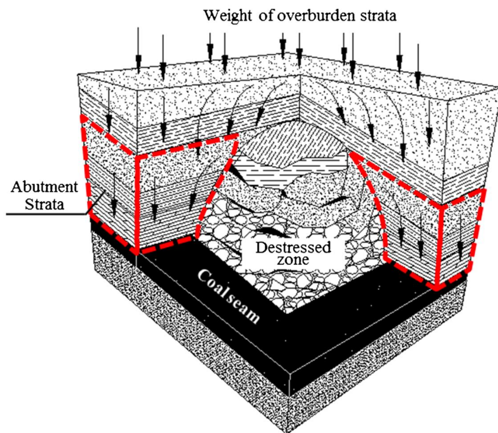
Figure 1.1: Stress transfer in a typical underground longwall mine (Li et al., 2018).
