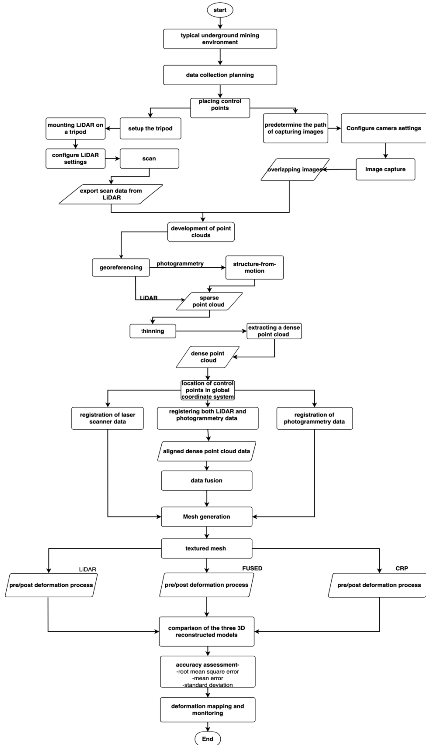
Figure 3.1: The fusion of LiDAR and CRP to reconstruct a photorealistic 3D model.
