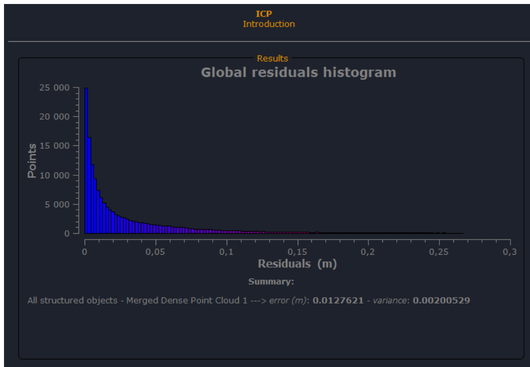
Figure 5:12: ICP global residuals graph showing the accuracy of alignment of pre-deformation and post-deformation fused point clouds.
