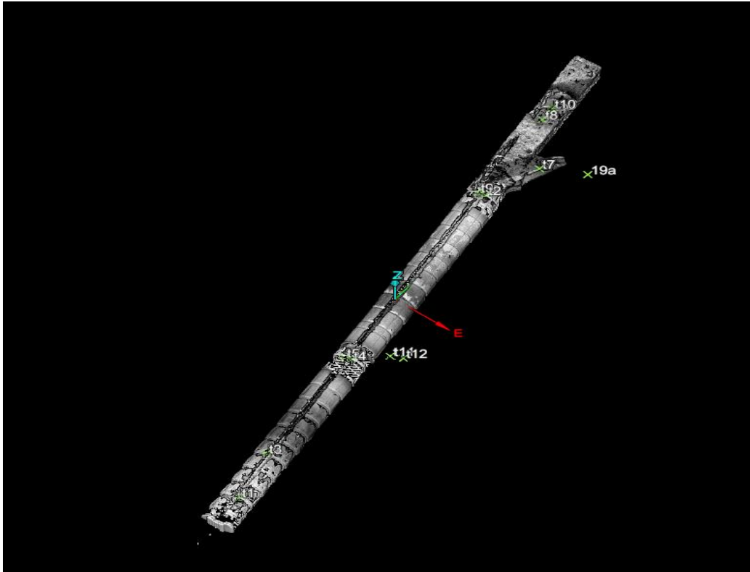
Figure 5.6: Illustration of georeferenced LiDAR point clouds with GCPs correctly positioned.
