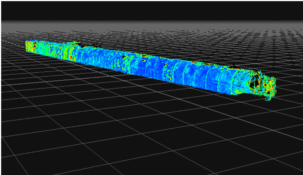
Figure 5.15: A post-deformation 3D model heat map of the Wits Mock Mine tunnel.
