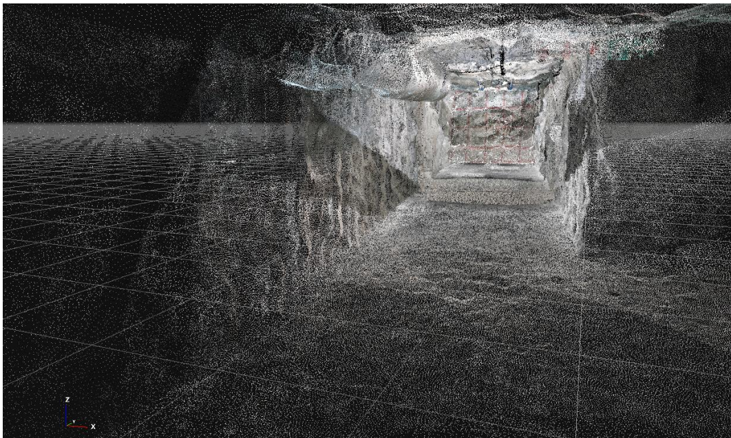
Figure 5.9: Fused 3D model from CRP and LiDAR point clouds in the pre-deformation stage.
