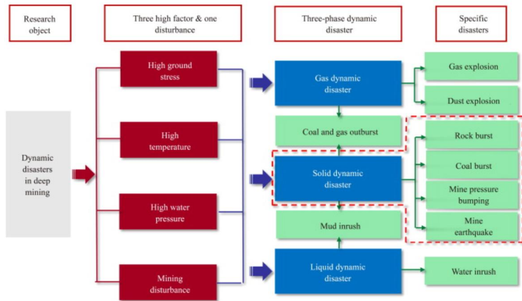
Figure 1.2 Causes and indication of main dynamic disasters in deep mines (He & Wang, 2023).
