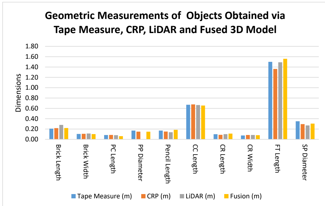
Figure 5.13: Comparison of the object dimensions obtained using a tape measure, CRP, LiDAR and fused 3D model.
