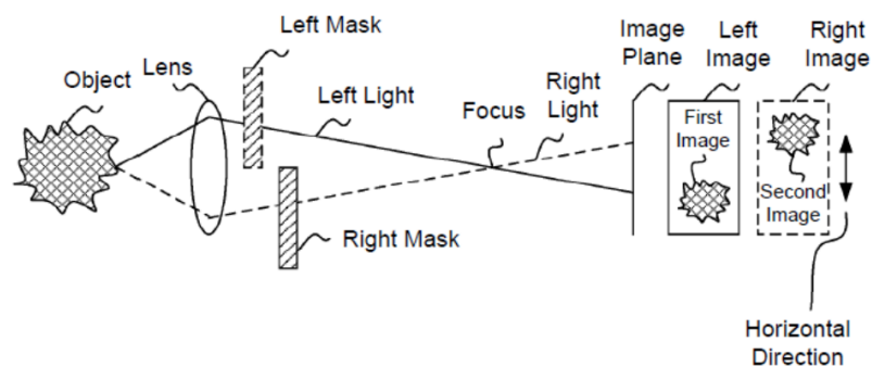
Figure 3.2: Principle of PDAF (Jutamulia, 2022).
