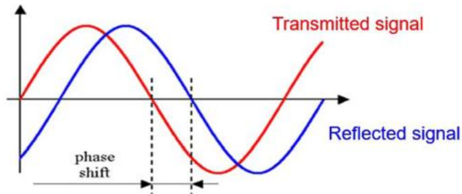
Figure 1.3: Illustration of transmitted and reflected signals using the phase shift principle of a LiDAR (Wang et al., 2020).
