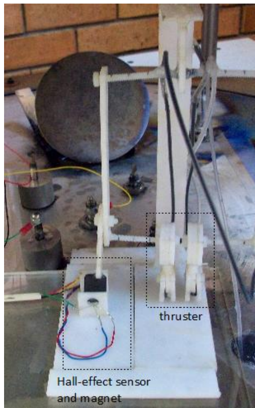
Figure 6.1: final sensor and thruster setup [25]
