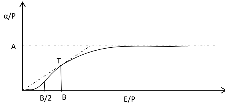
Figure 3.3: typical \frac{\alpha}{P} vs f\left(\frac{E}{P}\right) curve
