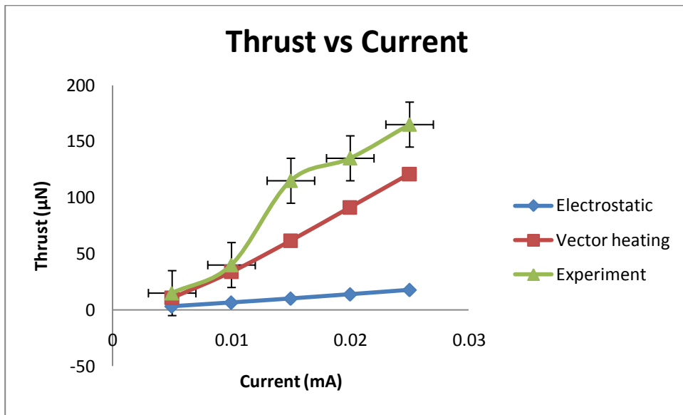
Figure 7.3: comparison of theoretical and experimental thrust
