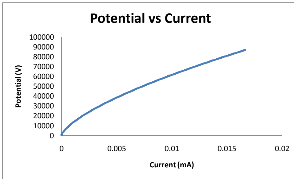
Figure 4.6: voltage as a function of the current
