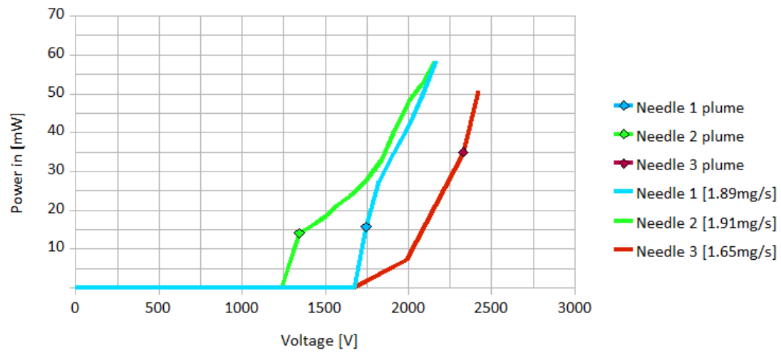
Figure 6.5: Electrical power usage for experiment 1 [25]
