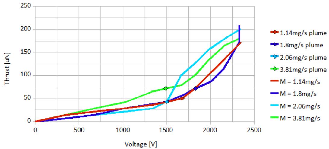
Figure 6.9: Measurements of thrust for experiment 2 [25]
