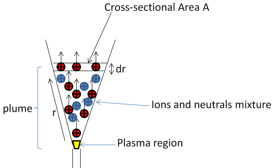
Figure 5.3: model of the plume for the thrust
