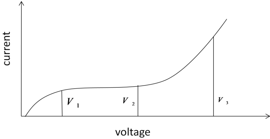
Figure 3.2: current-voltage relationship for a gas discharge process
