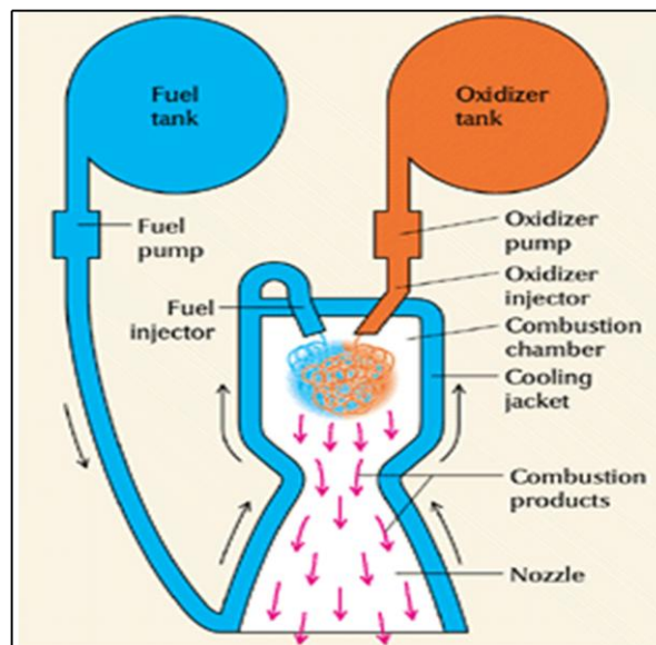
Figure 2.2: a typical liquid propellant rocket motor [14]
