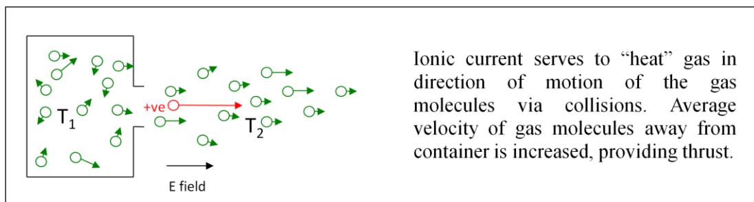
Figure 5.2: effect of the electrical energy on the molecules average velocity
