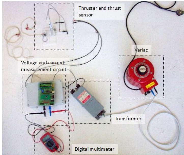
Figure 6.2: Equipment layout
