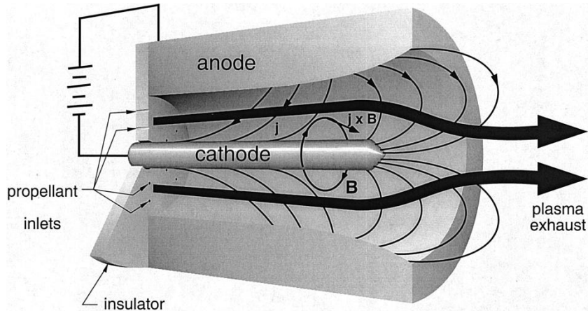
Figure 2.7: schematic of a magnetoplasmadynamic thruster. Here, gaseous propellants are introduced into the upstream portion of the channel, where after they are ionized by passage through an intense, azimuthally uniform electric arc standing in the interelectrode gap. If the arc current is high enough, its associated azimuthal magnetic field is sufficient to exert the desired axial and radial body forces on the propellant flow, directly accelerating it downstream and compressing it toward the centerline into an extremely hot plasma just beyond the cathode tip. Subsequent expansion of this plasma, along with the direct axial acceleration, yields the requisite exhaust velocity. [6]
