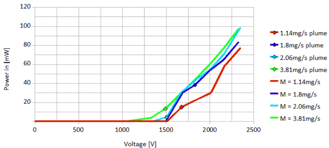
Figure 6.8: Electrical power usage for experiment 2 [25]
