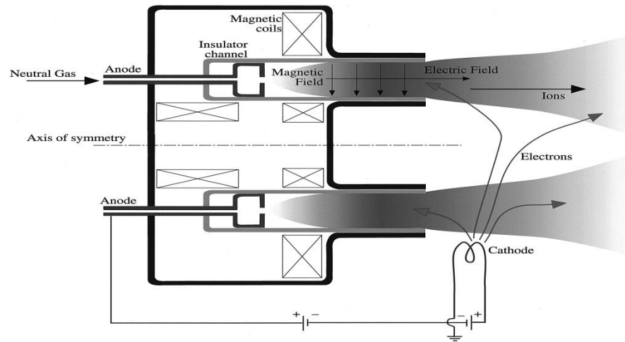
Figure 2.8: schematic of a Hall Effect thruster with an extended insulator channel (stationary plasma thruster, or SPT), showing the external cathode, the internal anode, the radial magnetic field, and typical particle trajectories [6]
