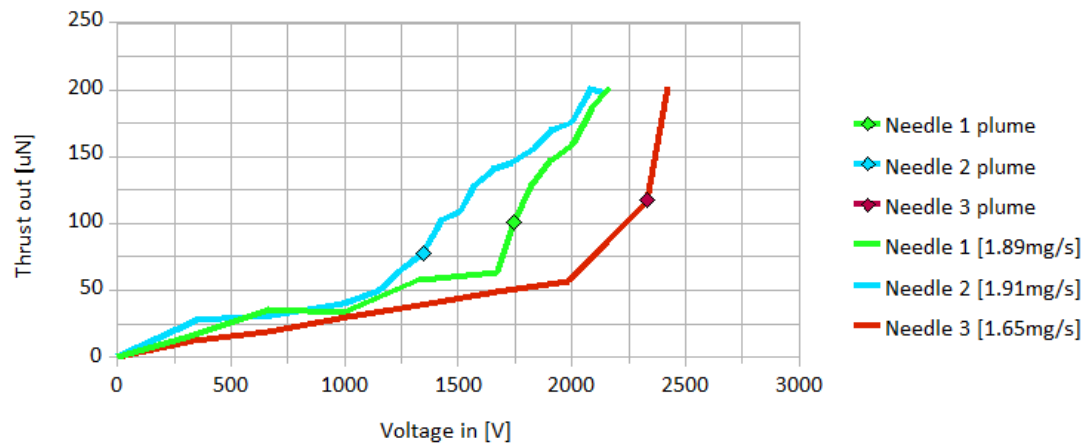
Figure 6.6: Measurements of thrust for experiment 1 [25]
