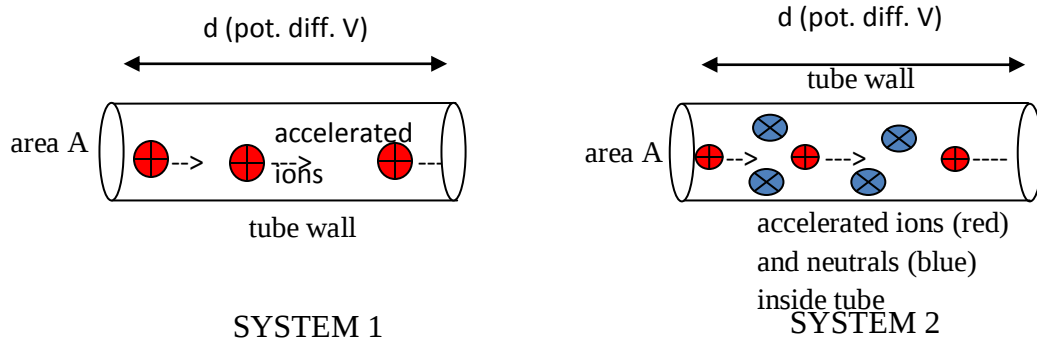
Figure 3.7: comparison of the two tubes (complete and incomplete ionization)
