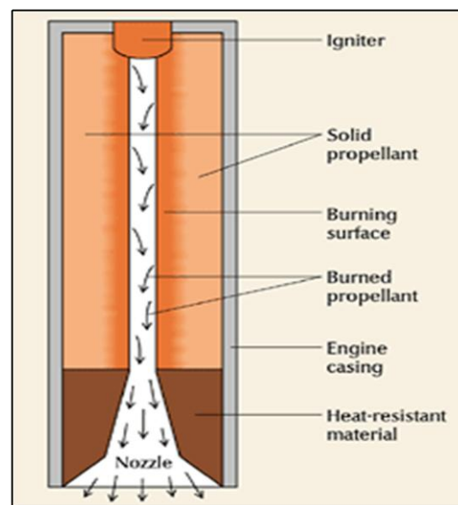
Figure 2.1: a typical solid rocket motor [14]
