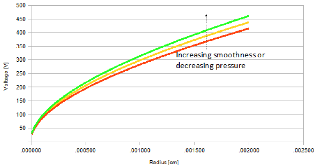
Figure 3.5: Corona onset voltage variation with electrode radius [25]
