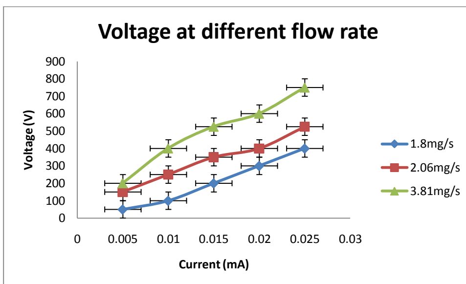
Figure 7.4: change of the potential difference with the flow rate
