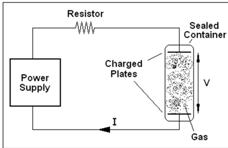
Figure 3.1: schematic of a typical gaseous discharge circuit
