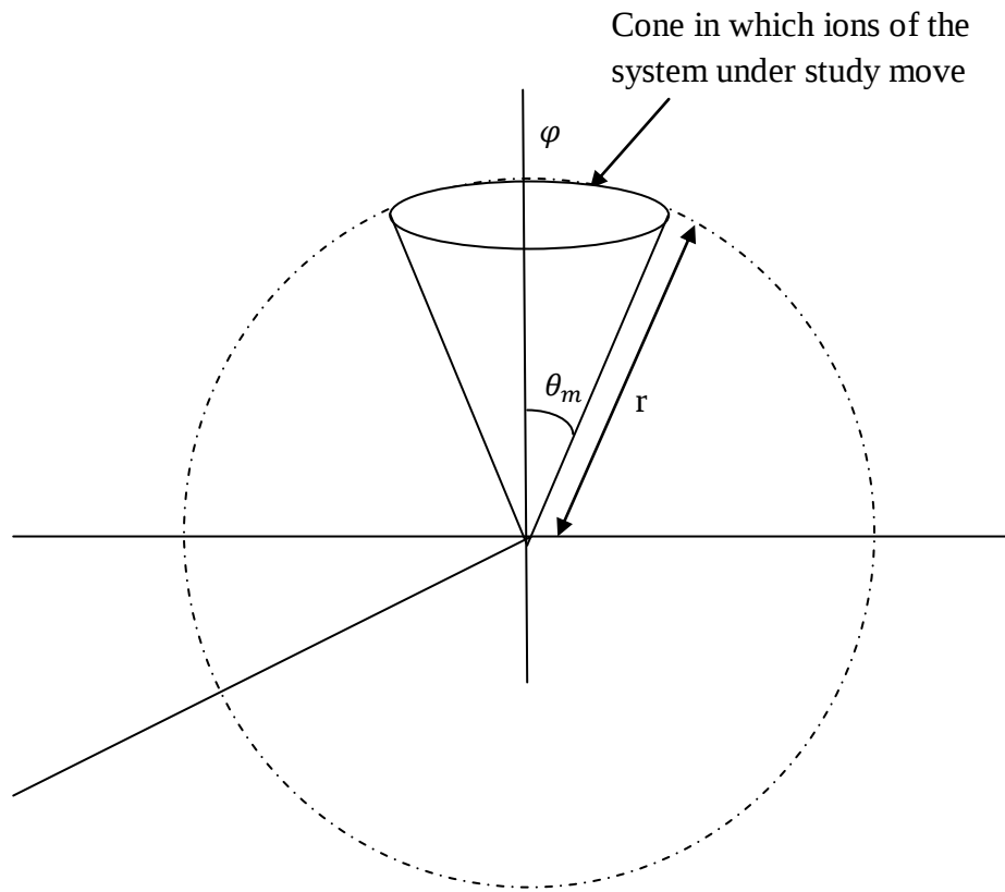
Figure 4.2: model of the plume in spherical coordinates
