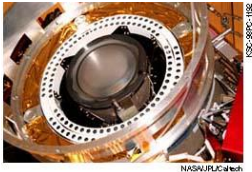
Figure 2.12: close up-view of the NSTAR ion engine [19]
