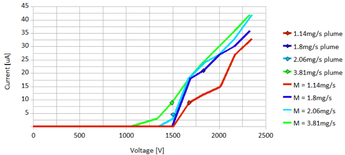
Figure 6.7: Measurements of current for experiment 2 [25]
