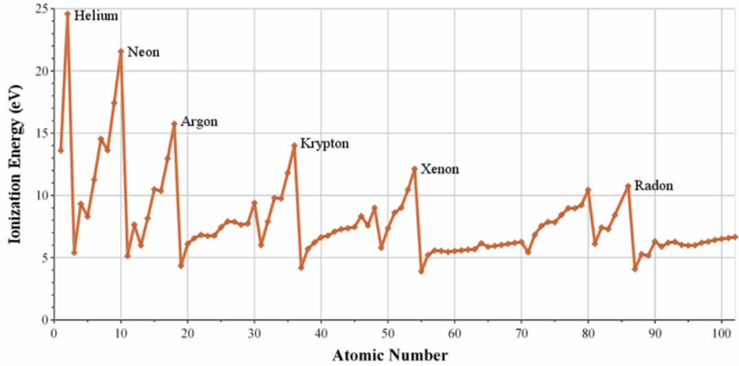
Figure 3.6: Ionization energy of different noble gases [26]
