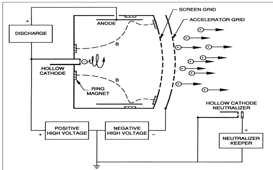
Figure 2.11: Schematic of an electron bombardment ion engine [6]
