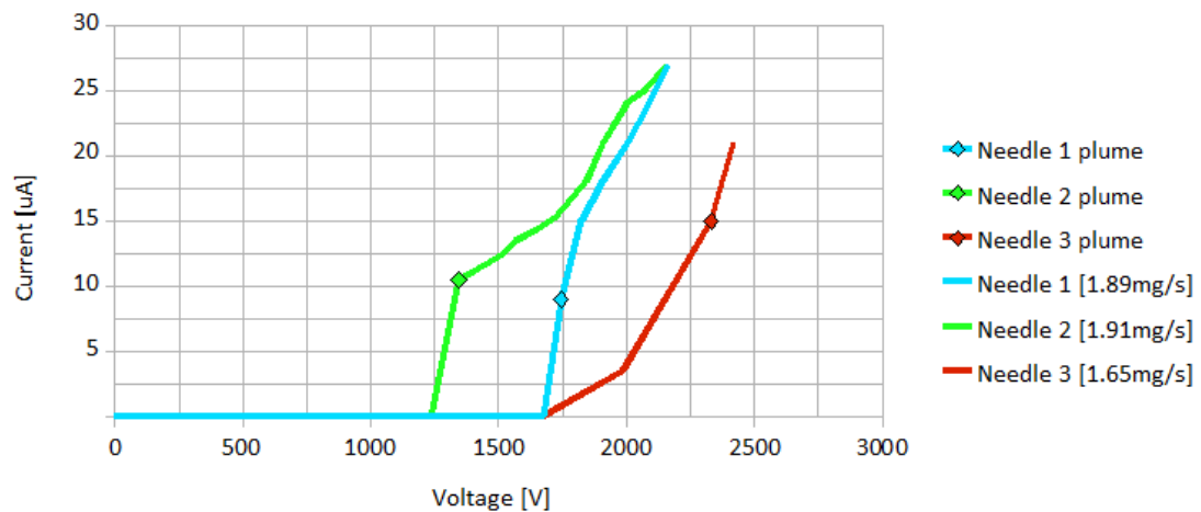
Figure 6.4: Measurements of current for experiment 1 [25]
