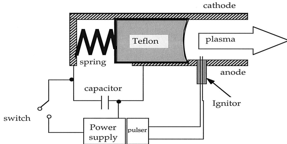
Figure 2.9: schematic of an ablative pulsed plasma thruster (APPT). The surface of a polymer block (most commonly Teflon) is successively eroded by intermittent arc pulses driven across its exposed face, and the ablated material is accelerated by a combination of thermal expansion and self-field electromagnetic forces. [6]
