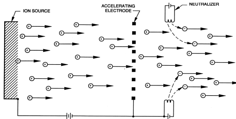
Figure 2.10: ion thruster schematic [6]
