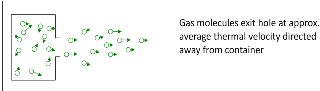
Figure 5.1: gas molecules escaping a box at approximately thermal velocity
