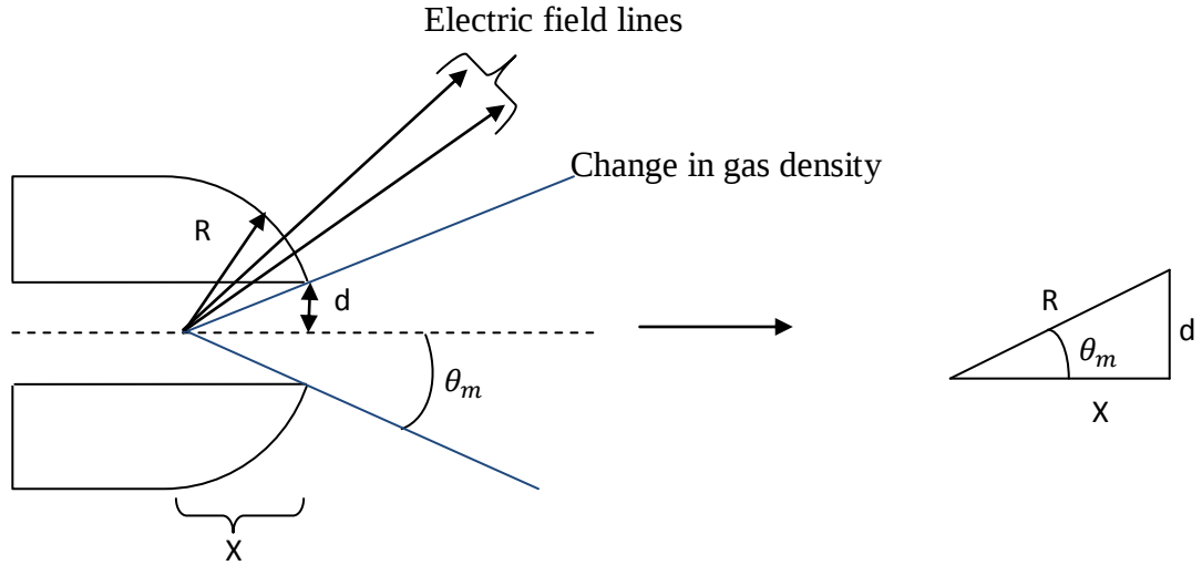
Figure 4.4: outward flux of neutral gas molecules
