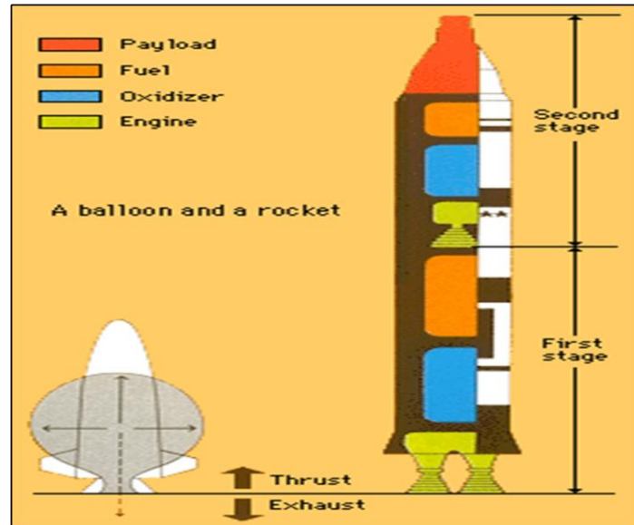
Figure 2.3: schematic of a two-stage rocket [14]
