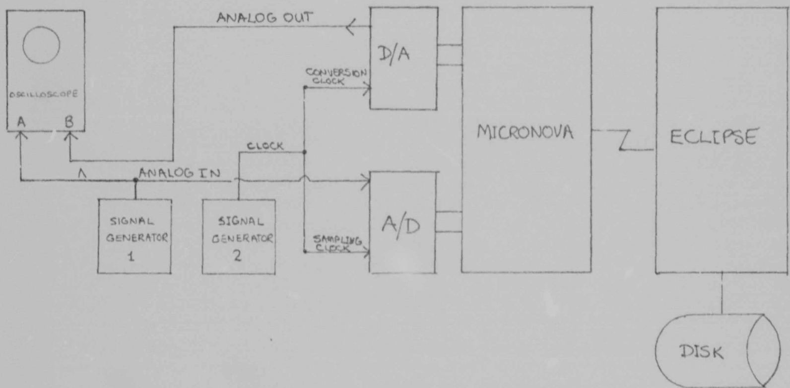
FIGURE 8 : SET-UP FOR ACCEPTANCE TESTING.
