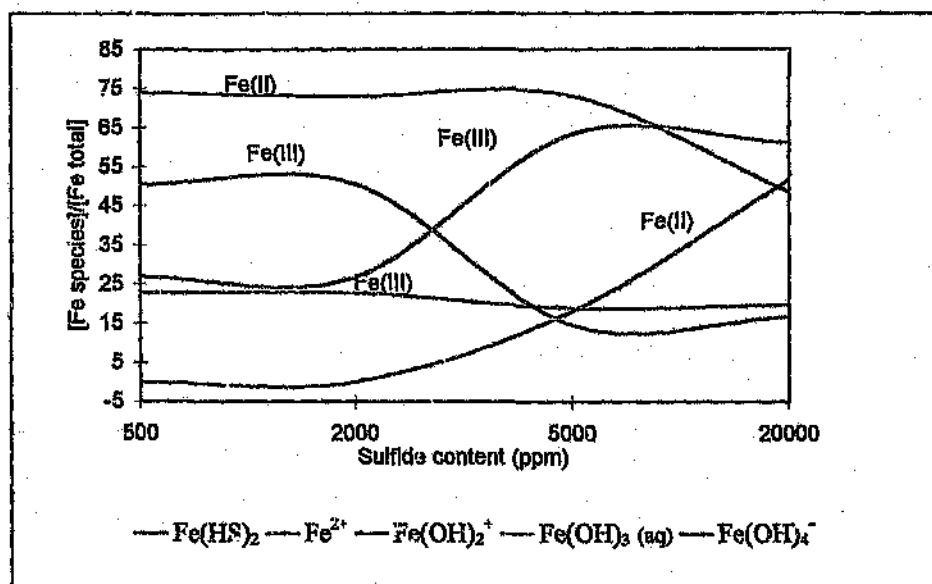
Figure 7.5: Solution speciation a at pH 6.9 as a function of sulfide content
