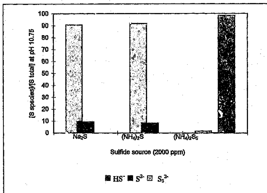
Figure 7.9: Effect of sulfide source on the distribution of sulfide species at pH 10.16
