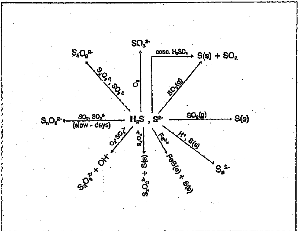
Figure 1.1: Typical decomposition routes of sulfide [9]
