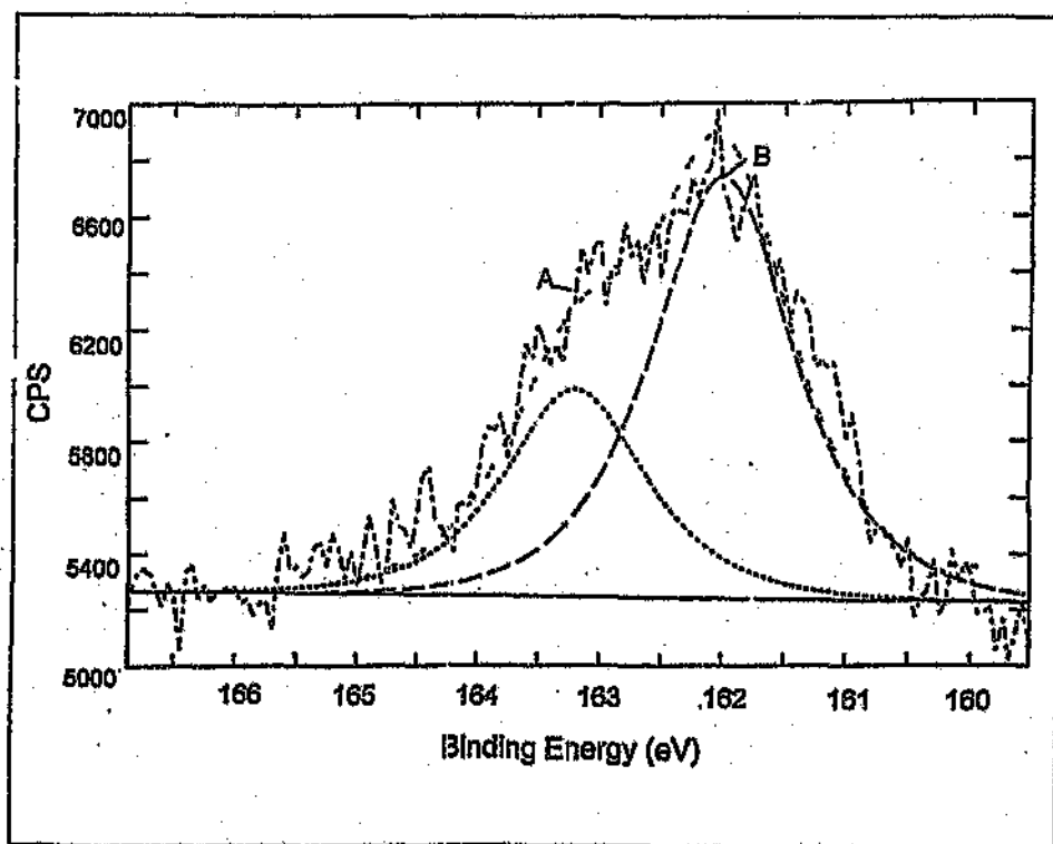
Figure 4.4: Expanded view of sulfide peak at 162 eV of catalyst in Figure 4.3a), complete with peak-fit.
