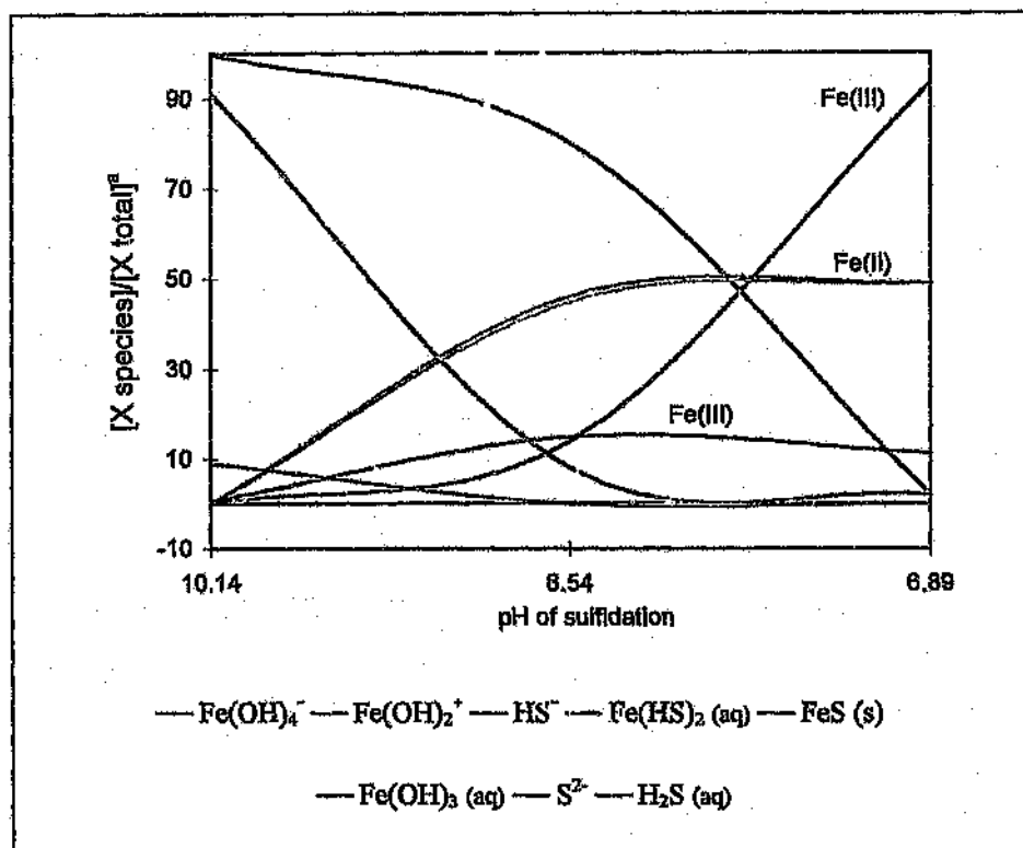
Figure 7.7: Effect of sulfidation pH on the system sulfided with 500 ppm S
