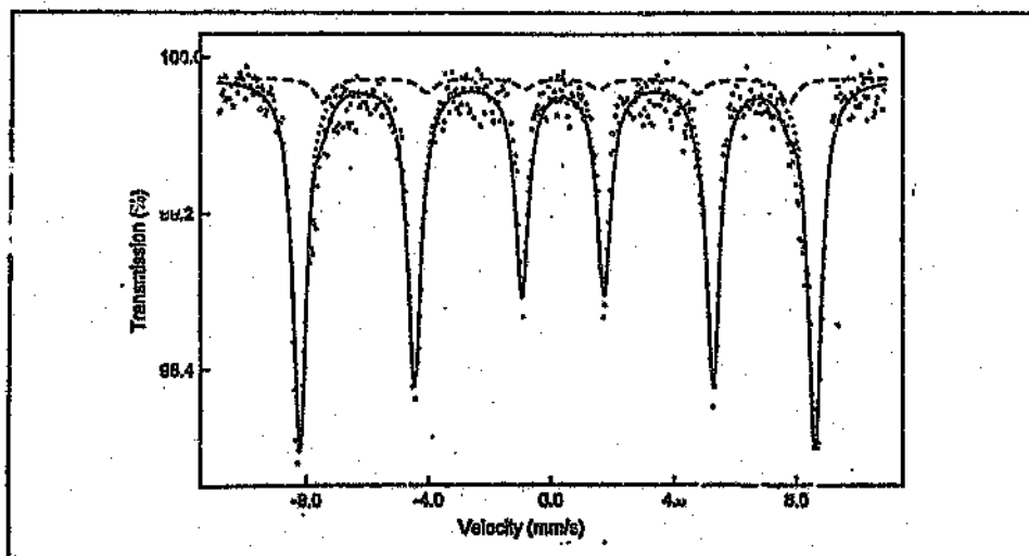
Figure 6.4: 20000 ppm polysulfided catalyst after calcination at 400^\circ\text{C}
