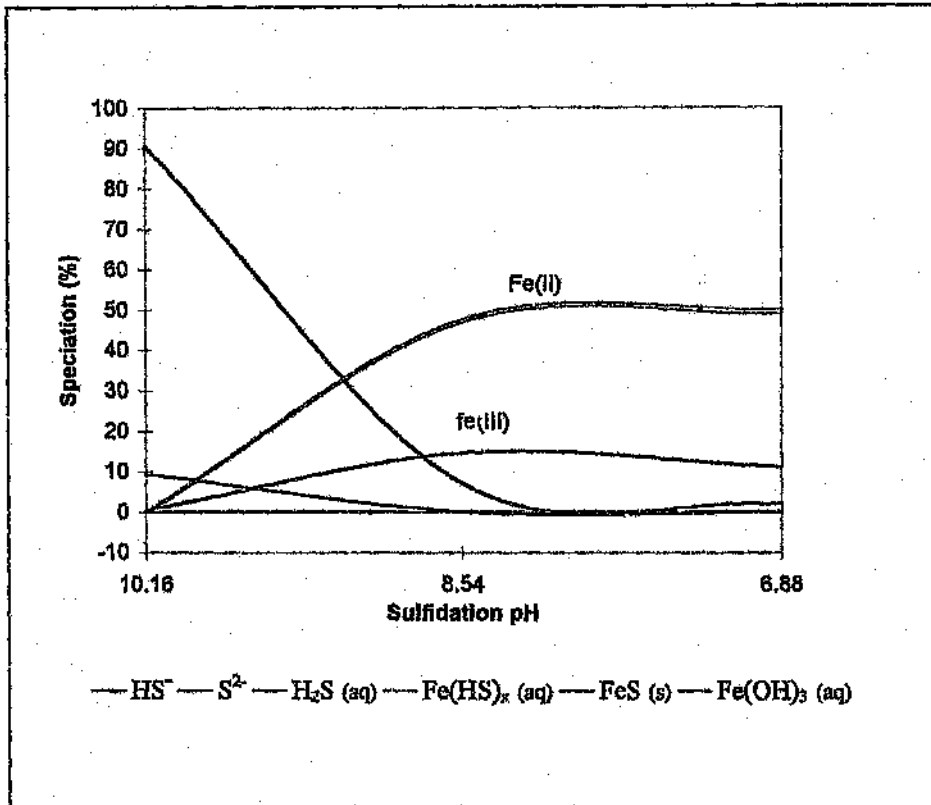
Figure 10.5: Effect of sulfidation pH on the solution speciation of a 2000 ppm \text{Na}_2\text{S} sulfided system, where sulfide species are presented as a percentage of total sulfide, and ferrous species as a percentage of total \text{Fe}^{2+} .
