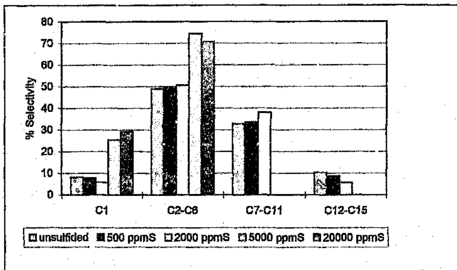
Figure 8.4: Product selectivity of catalysts sulfided in the range 500-20000 ppm S
