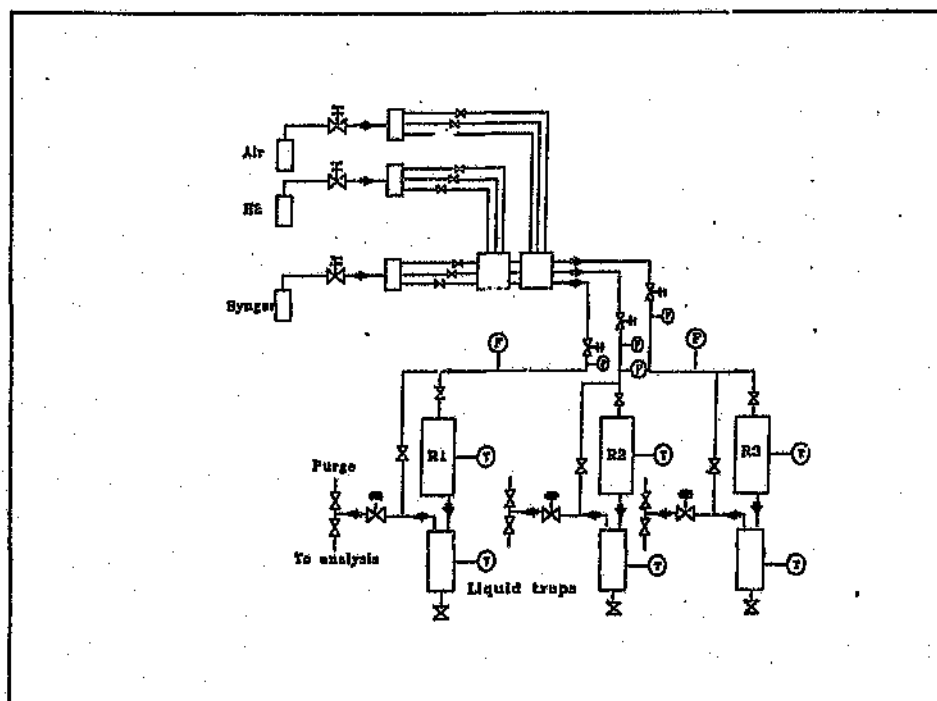
Figure 2.5: Plug Flow Reactor System for Fischer-Tropsch catalyst testing
