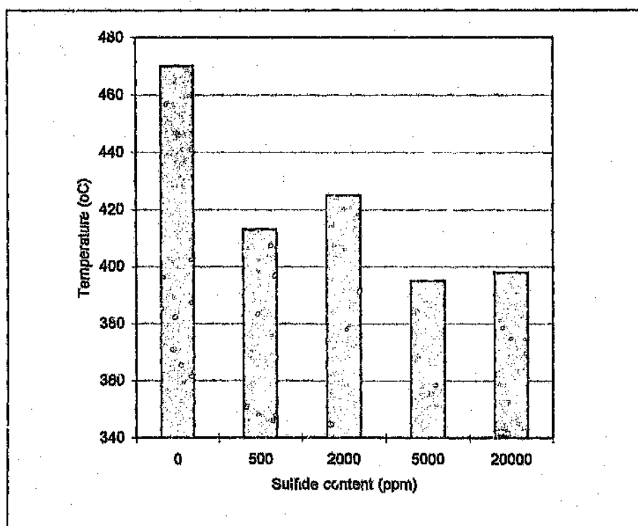
Figure 8.9: The effect of sulfide content on the reduction peak of hematite to magnetite for precipitated-iron catalysts
