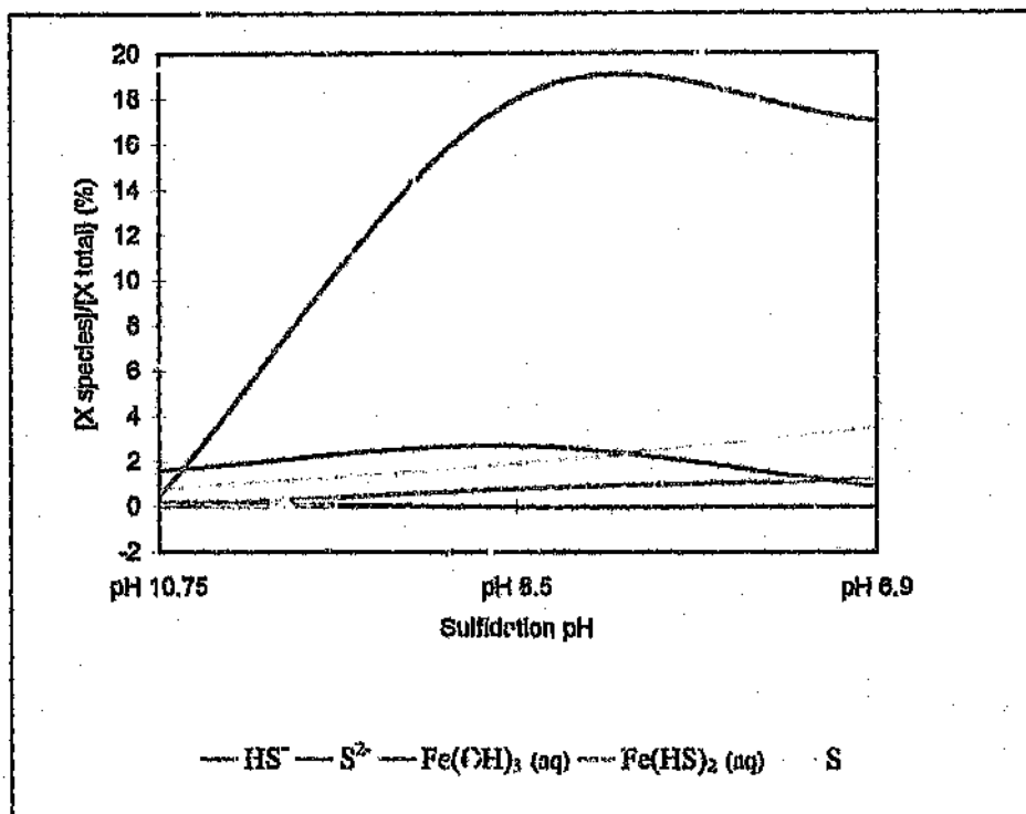
Figure 7.11: Effect of pH of polysulfide addition on sulfide solution speciation, where X refers to sulfide, or ferric
