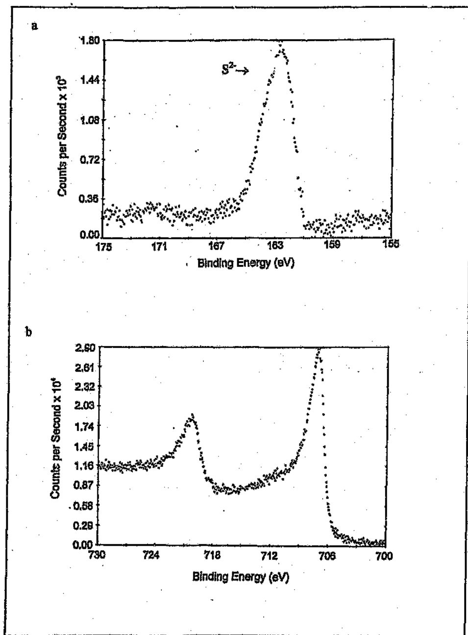
Figure 4.3: a) S (2p) core level spectrum of catalyst sulfided as in Figure 4.2, but reduced at 400°C, showing conversion of sulfate to sulfide b) Fe (2p) photopeak typical of metallic iron, formed after reduction at 400°C
