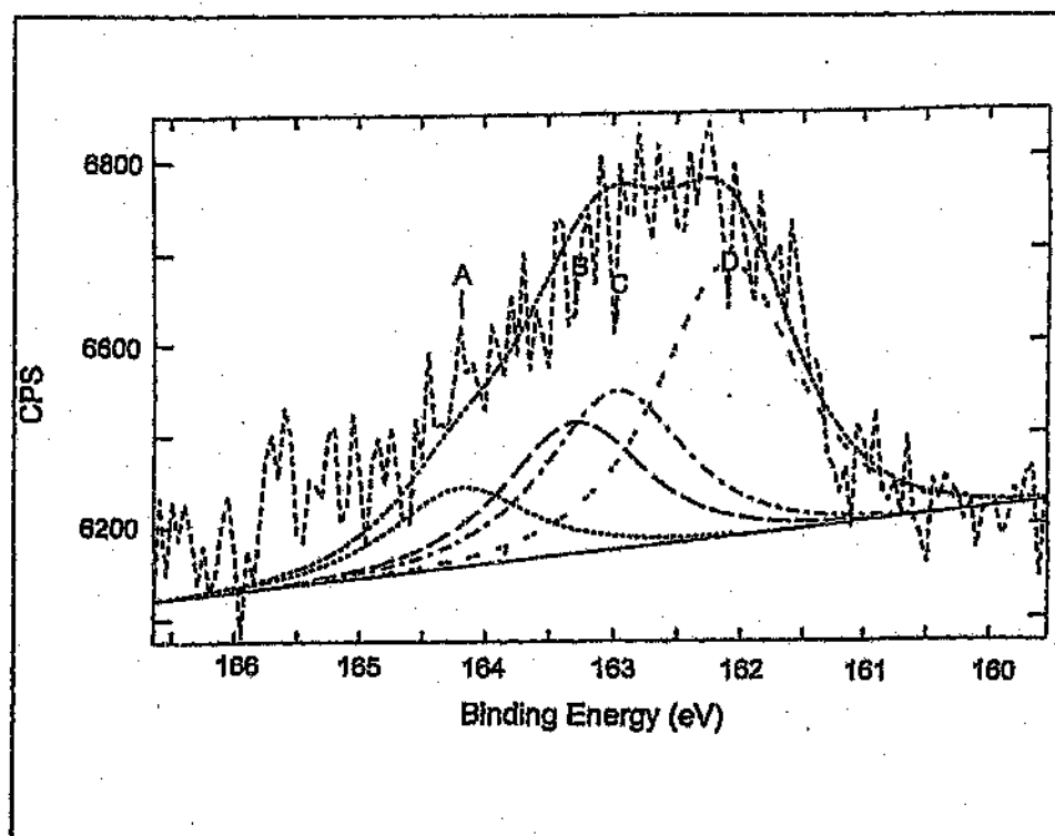
Figure 4.5: Expansion of sulfide region of polysulfided catalyst containing 20000 ppm (\text{NH}_4)_2\text{S}_3 . Lines A and C constitute one doublet used in peak-fitting, while lines B and D make up the other doublet.
