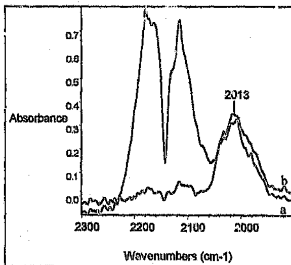
Figure 5.6: CO adsorption on a 1000 ppm S catalyst prepared by incipient wetness
