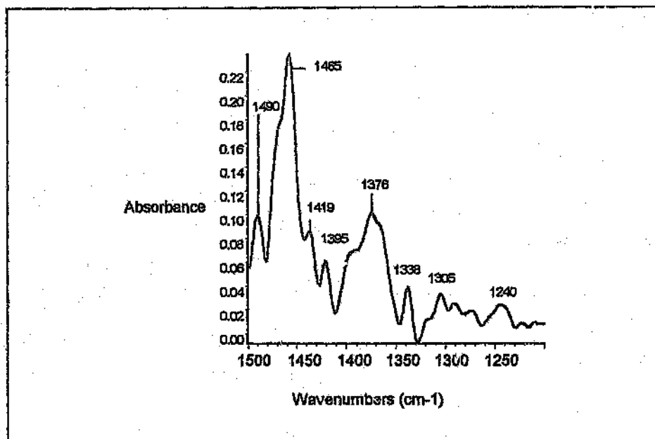
Figure 5.16: Expanded view of FT synthesis on a catalyst sulfided with 2000 ppm Na 2 S, showing 1800-1200 cm -1 region
