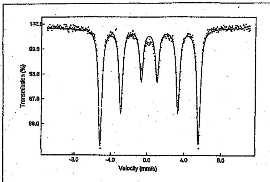
Figure 6.5: Mössbauer spectrum of spent catalyst sulfided with 5000 ppm polysulfide, recorded at 298 K
