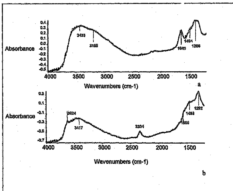
Figure 5.8: a) Catalyst sulfided with 2000 ppm \text{Na}_2\text{S} prior to calcination b) Following calcination at 400^\circ\text{C}
