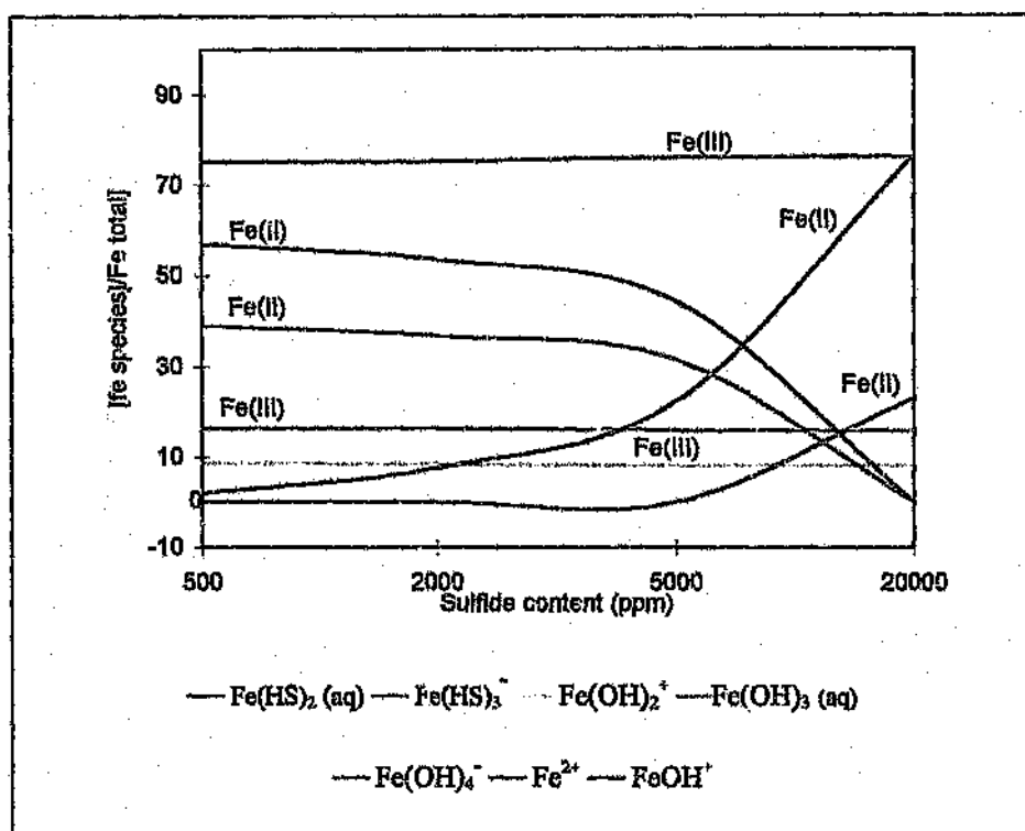
Figure 7.3: Effect of increasing sulfide addition on the solution speciation a at pH 8.5
