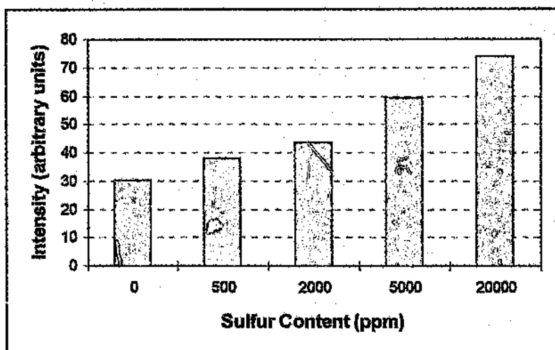
Figure 3.14: Variation in the crystallinity of iron-oxide as a function of the sulfur content
