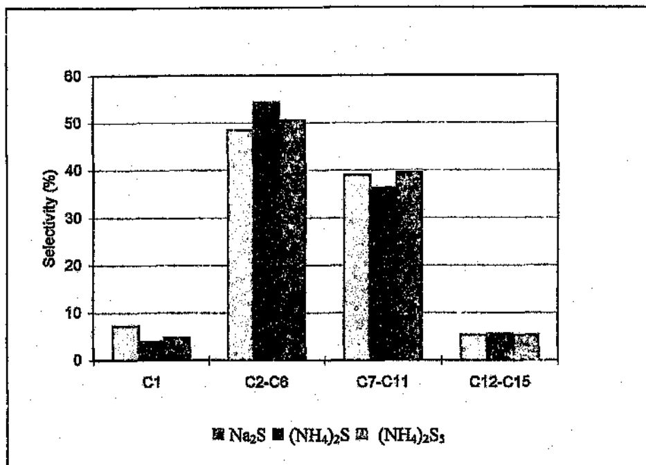
Figure 9.1: Product selectivity of catalysts sulfided using different sulfide sources
