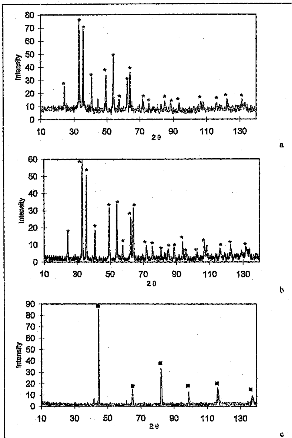
Figure 3.13: Diffraction of a catalyst sulfided with 20000 ppm (\text{NH}_4)_2\text{S}_5 at pH 6.9 a) uncalcined b) calcined c) spent where * = \text{Fe}_2\text{O}_3 ■ = \alpha\text{-Fe}
