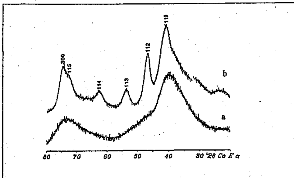
Figure 3.16: a) 2-line ferrihydrite, b) 6-line ferrihydrite [71]
