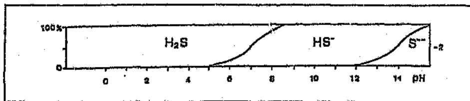
Figure 10.4: The dissociation of sulfide species as a function of pH at 25°C [204]
