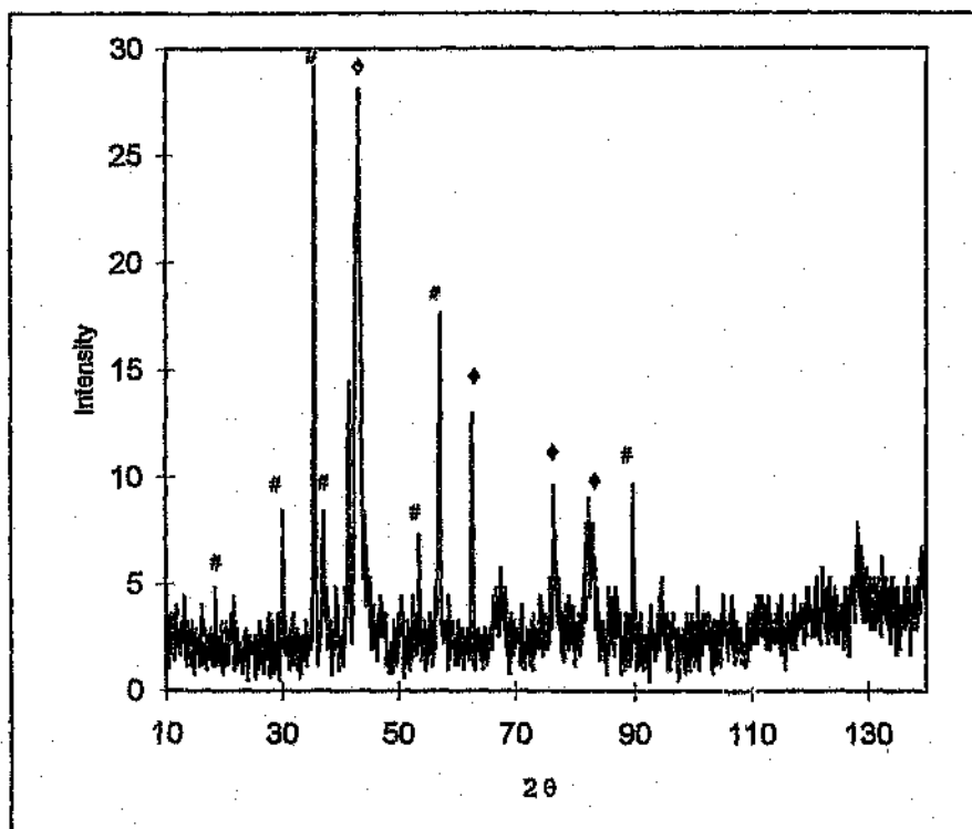
Figure 3.10: Diffractogram of a spent catalyst sulfided with 500 ppm Na 2 S at pH 6.9 where # = Fe 3 O 4 ♦ = ε-carbide
