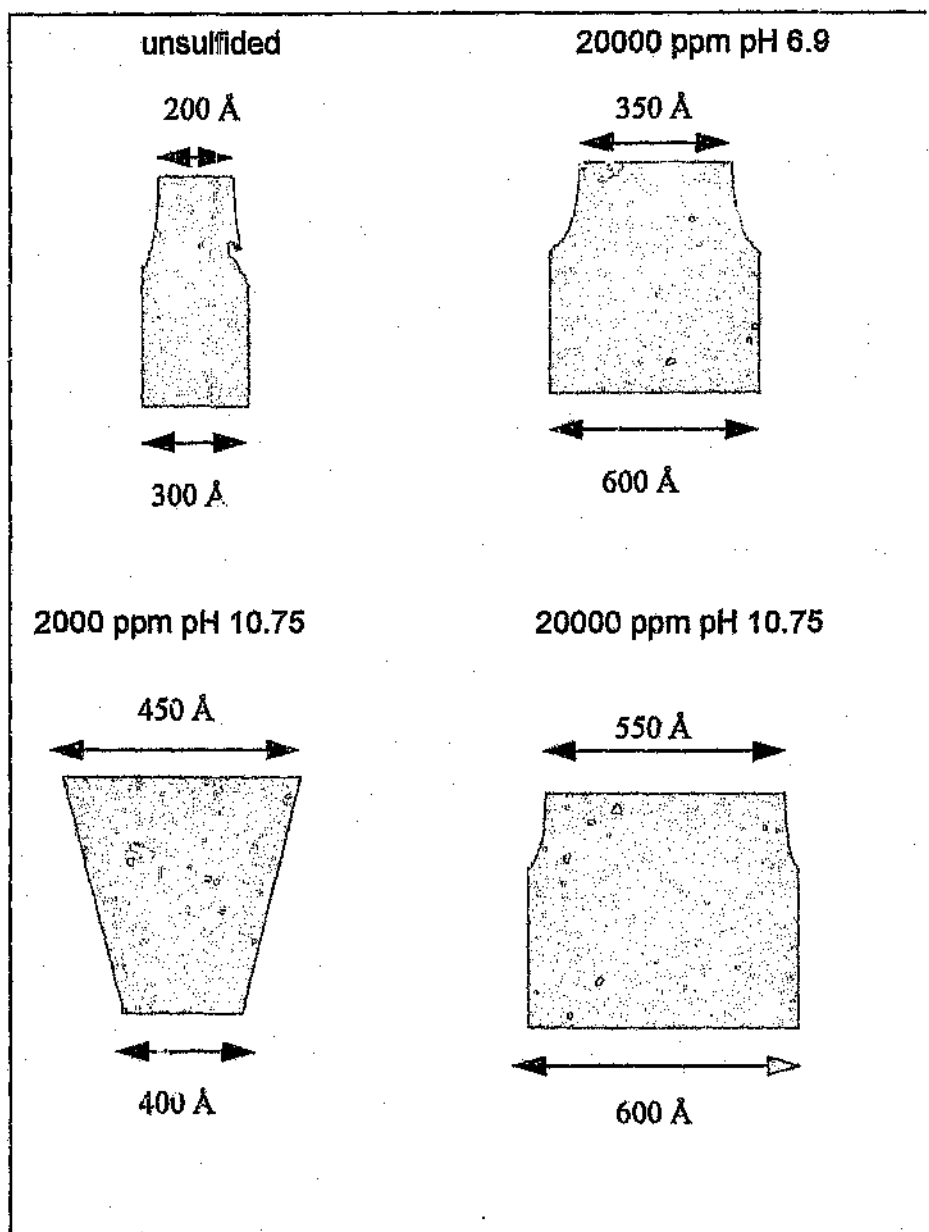
Figure 3.20: Proposed pore shapes of calcined catalysts
