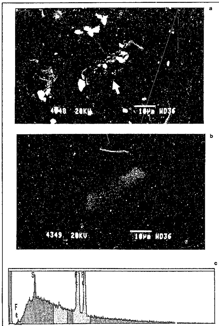
Figure 3.7: a) Micrograph of sulfur-rich region on catalyst sulfided with 20000 ppm S at 2000x magnification b) Dot density map of sulfur c) EDX analysis of sulfur rich region
