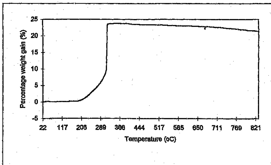
Figure 3.18: Thermogram of spent catalyst sulfided with 20000 ppm Na 2 S at pH 6.9 recorded under oxygen
