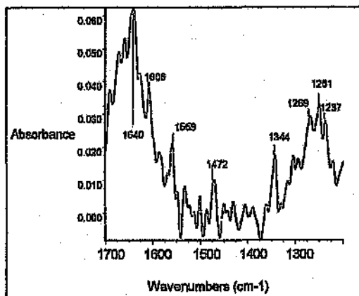
Figure 5.13: Expanded view of 1700-1200 \text{cm}^{-1} region of the DRIFTS spectrum of a catalyst sulfided with 500 ppm \text{Na}_2\text{S} recorded after CO adsorption
