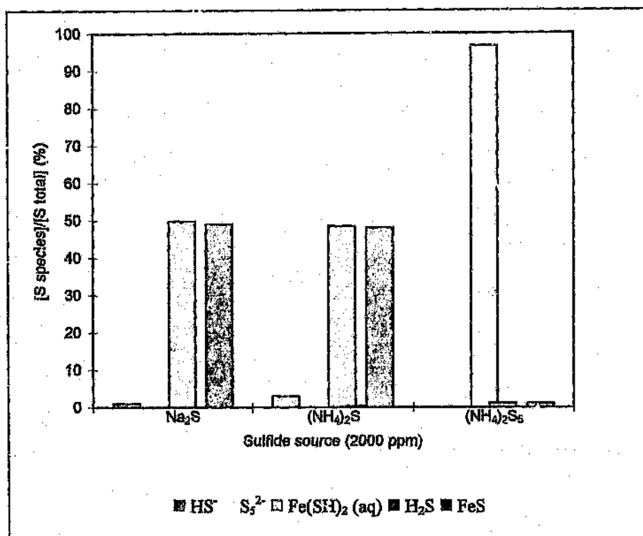
Figure 7.10: Effect of sulfide source on the distribution of sulfide species at pH 6.9
