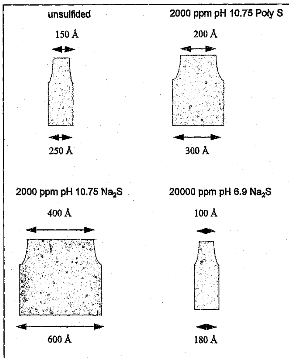
Figure 3.22: Proposed pore shapes of spent catalysts
