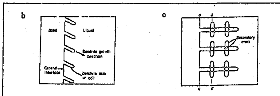
Figure 3.4: b) Representation of the first stage of dendritic growth. The temperature in the liquid drops in advance of the interface, facilitating the outward growth of the crystallites c) Secondary dendritic arms are formed when a temperature gradient exists at a point close to a primary arm and moves to a point midway from the primary arms
