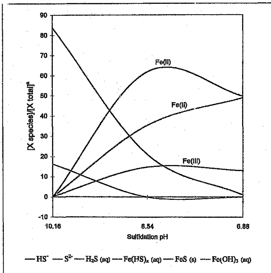
Figure 7.8: Effect of sulfidation pH on solution speciation in a system sulfided with 20000 ppm \text{Na}_2\text{S}
