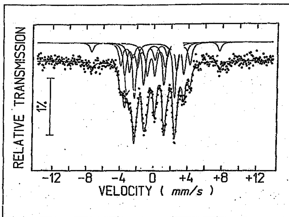
Figure 6.6: Mössbauer spectrum of a catalyst sulfided with 2000 ppm polysulfide, after FT synthesis, showing carbide formation (recorded at 298 K)
