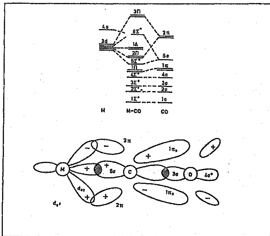
Figure 5.1: a) Molecular orbital diagram of the bonding between a metal and CO b) A schematic representation of the orbital overlap in a metal-carbonyl complex [123]
