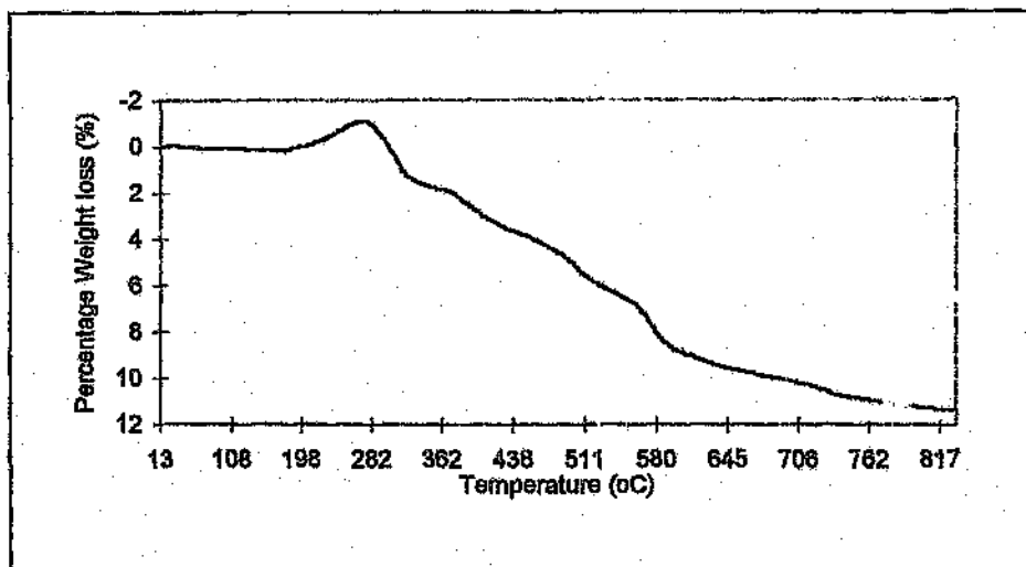
Figure 3.17: Thermogram of a spent unsulfided catalyst recorded in an oxidising atmosphere
