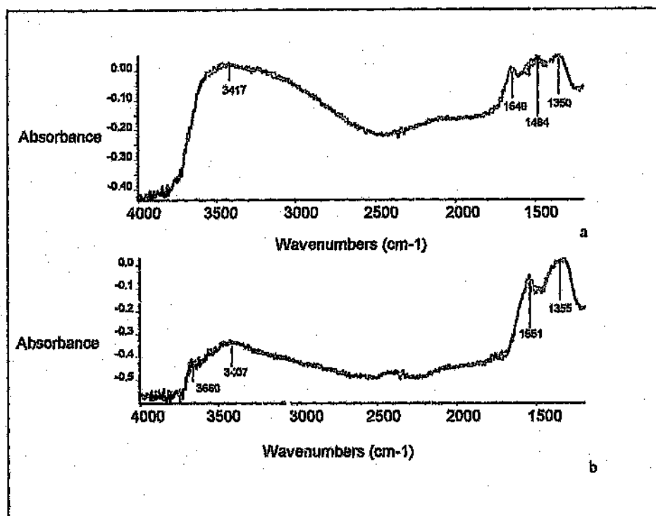
Figure 5.7: a) Unsulfided precipitated-iron catalyst prior to calcination b) After calcination at 400°C
