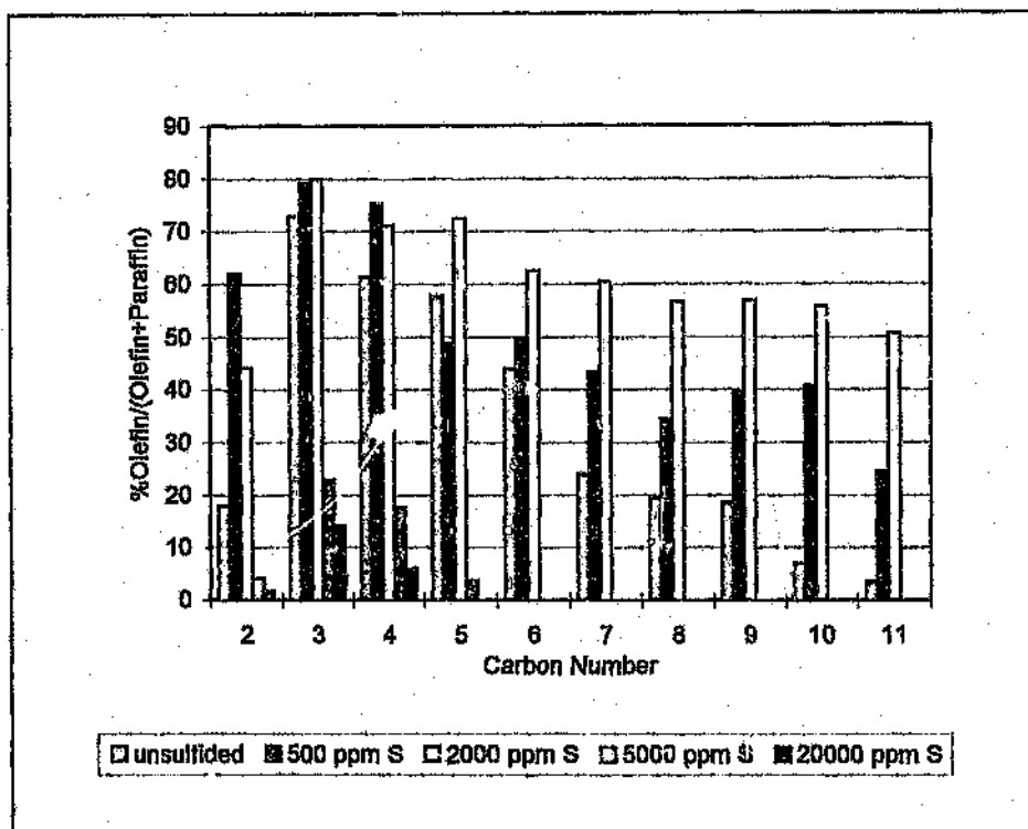
Figure 8.3: Olefinity of sulfided catalysts as a function of carbon number
