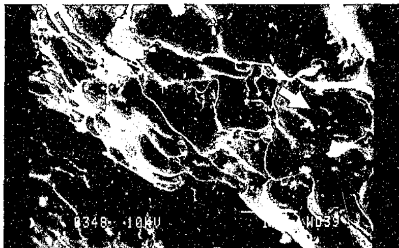
Figure 3.1a: Electron micrograph of an uncalcined, unsulfided precipitated-iron catalyst taken at 2000x magnification
