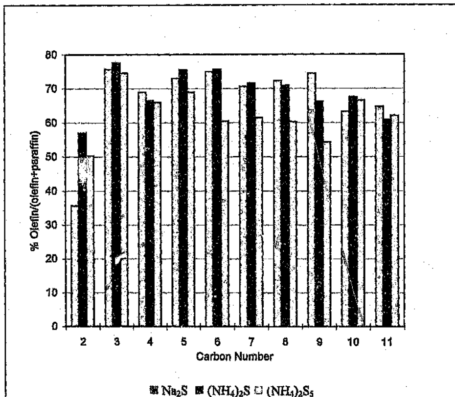
Figure 9.3: Olefinity of products obtained from catalysts sulfided using various sulfide sources
