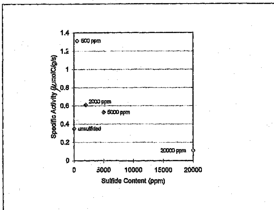
Figure 8.1: Variation of specific activity with sulfide content
