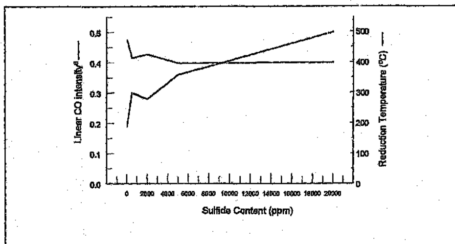
Figure 5.3: The effect of increasing levels of sulfidation on the evolution of linear carbonyl species on the surface of iron catalysts, showing correlation with extent of reduction. Catalysts were sulfided at pH 6.9 using \text{Na}_2\text{S} .
