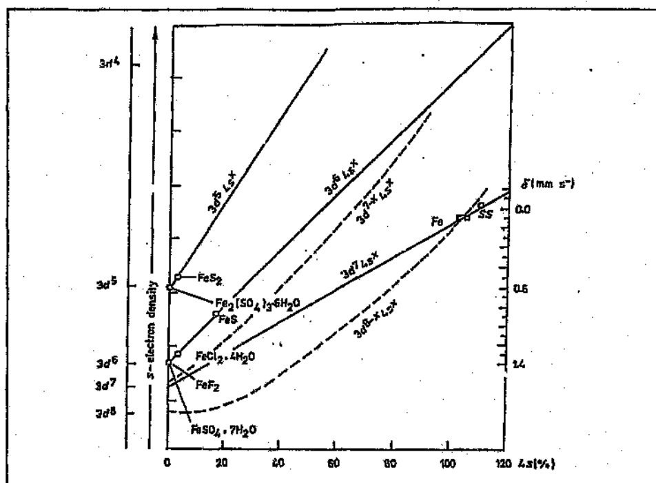
Figure 6.8: Walker Diagram of iron species showing relationship between \delta and s -electron density
