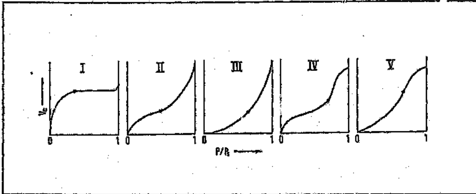
Figure 2.2: Shapes of adsorption isotherms
