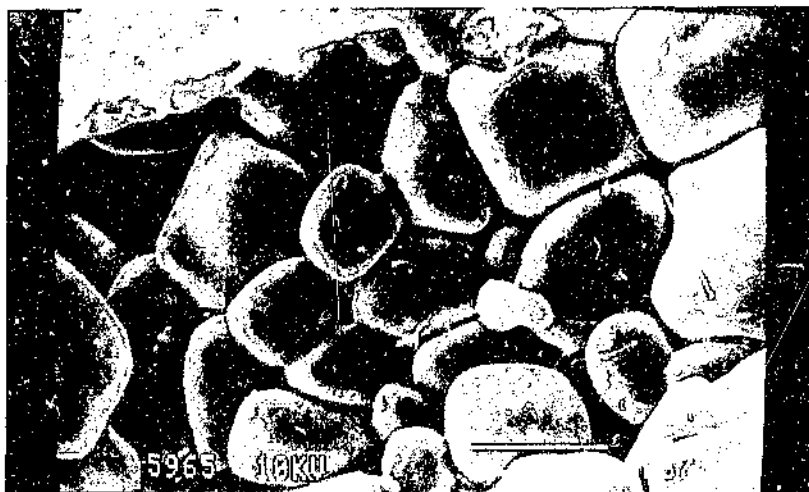
Figure 3.3a: Equiaxed crystals viewed at 2000x magnification on a catalyst sulfided with 5000 ppm S before calcination
