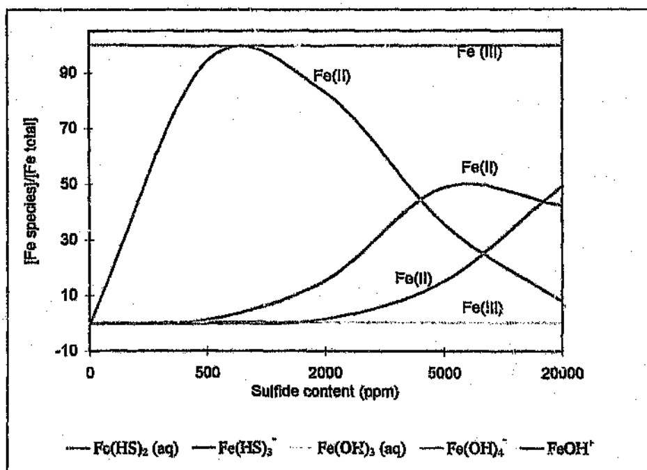
Figure 7.1: The effect of increasing levels of sulfidation on ferric and ferrous ion solution speciation* at pH 10.75:
