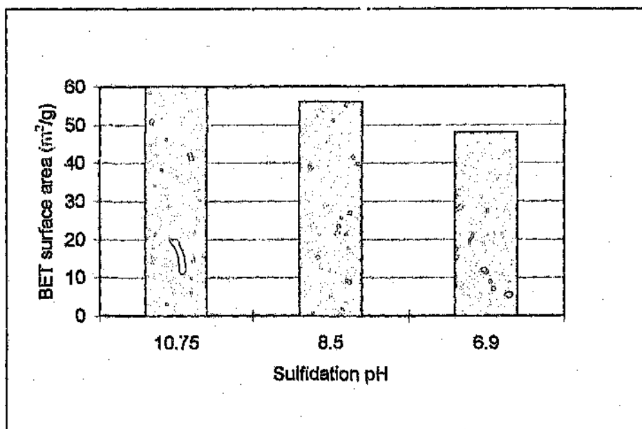
Figure 10.6: Variation in surface area with pH of uncalcined catalysts sulfided with 2000 ppm S from polysulfide
