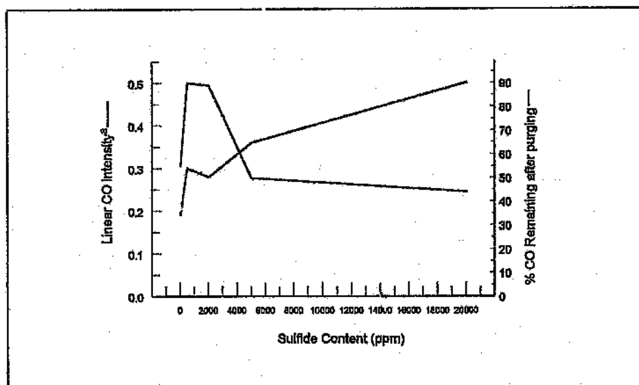
Figure 5.5: The effect of purging with nitrogen on the intensity of adsorbed linear carbonyl species as a function of sulfide content
