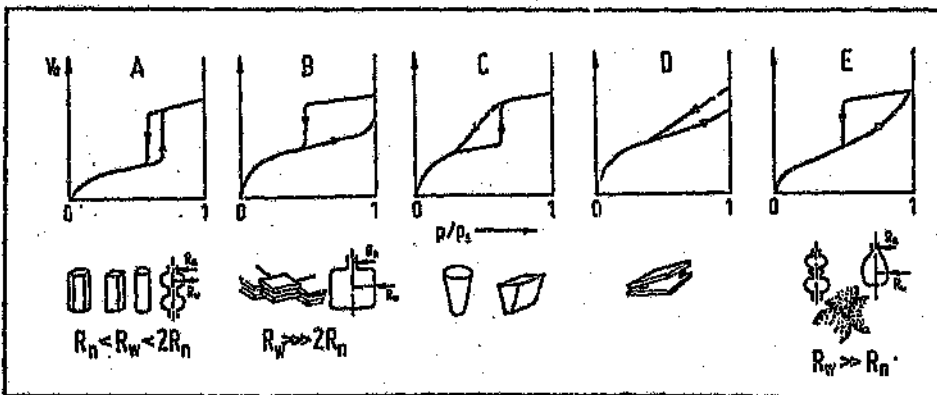
Figure 2.3: Type IV isotherms showing different hysteresis loops
