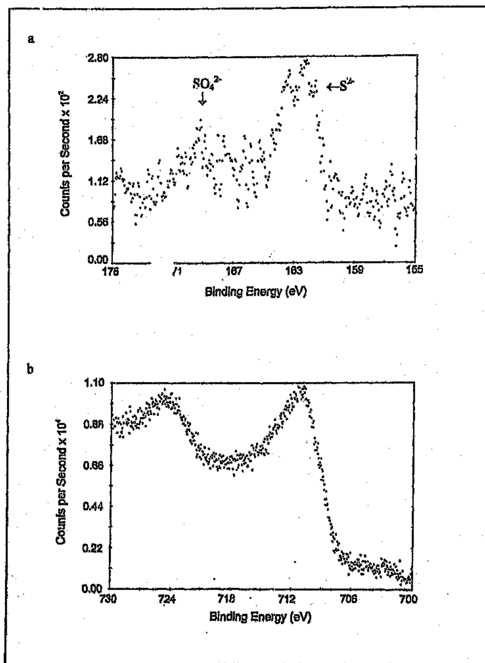
Figure 4.2: a) Evolution of sulfide (162 eV) and sulfate (168 eV) on a catalyst sulfided with 20000 ppm \text{Na}_2\text{S} , after calcination at 200^\circ\text{C} and reduction at 300^\circ\text{C} b) Fe 2p ( 3/2 ) photopeak of the same catalyst showing the presence of iron-oxide (712 eV) after hydrogen activation.
