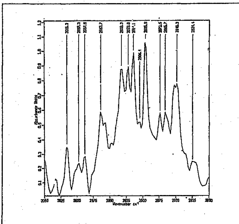
Figure 5.17: b) Highly active catalyst generated by reduction at 400°C
