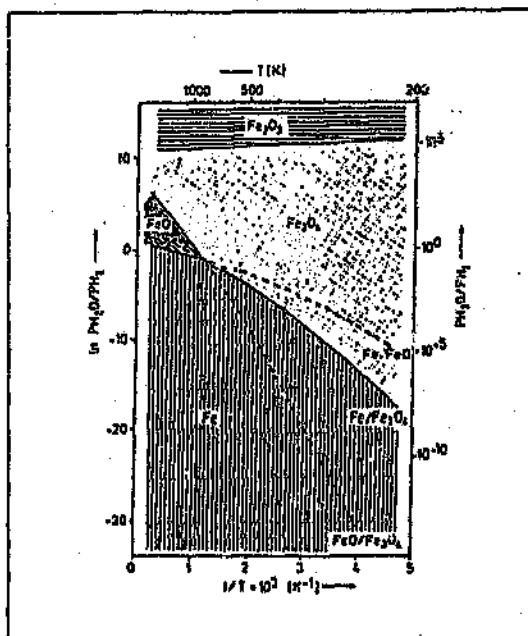
Figure 8.8: Phase Diagram of the reduction of iron oxide [52]
