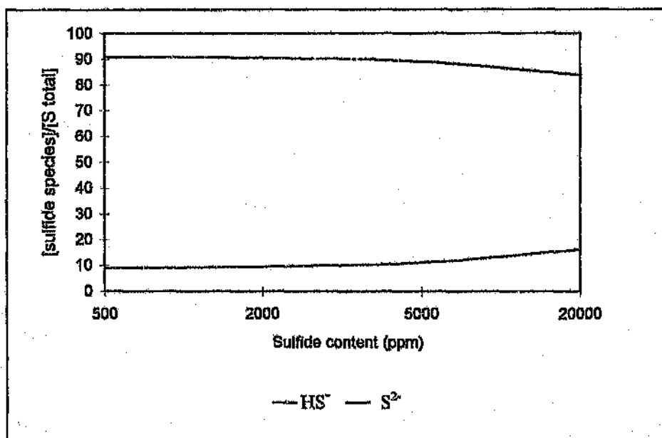
Figure 7.2: Effect of sulfidation level on the equilibrium distribution of sulfide species at pH 10.75.
