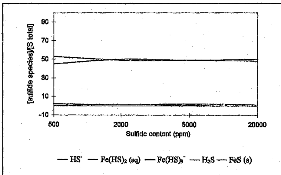
Figure 7.6: Distribution of sulfide species at pH 6.9 as a function of sulfide content
