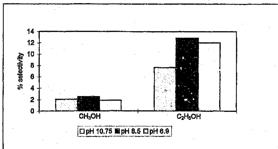
Figure 10.12: Oxygenate selectivity of catalysts sulfided at various pH values.
