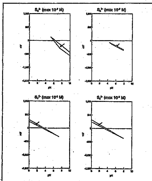
Figure 1.4: Eh-pH diagrams of polysulfides at 25°C [9]
