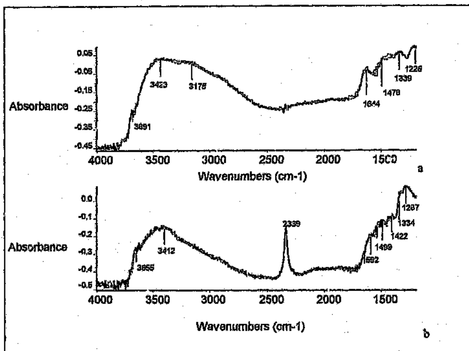
Figure 5.11: a) Infrared spectrum of uncalcined catalyst sulfided with 20000 ppm Na 2 S b) Same catalyst after calcination in air at 400°C
