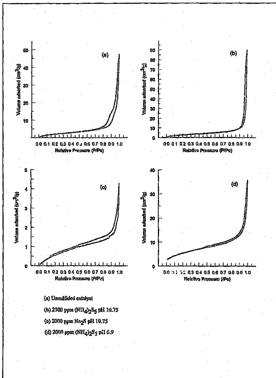
Figure 3.21a-d: Adsorption-desorption isotherms of spent catalysts
