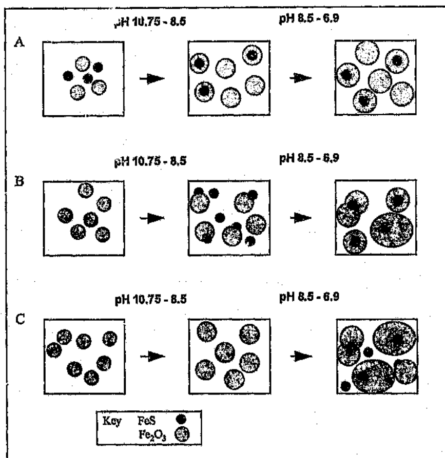
Figure 10.9: Schematic representation of the proposed model of the effect of sulfide addition on iron-oxyhydroxide crystallite growth
