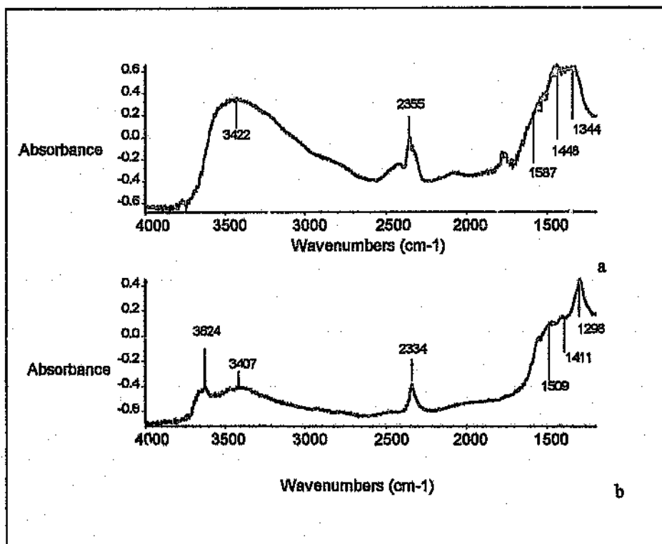
Figure 5.12: a) DRIFTS spectrum of a catalyst calcined at 200°C b) The same catalyst calcined at 400°C
