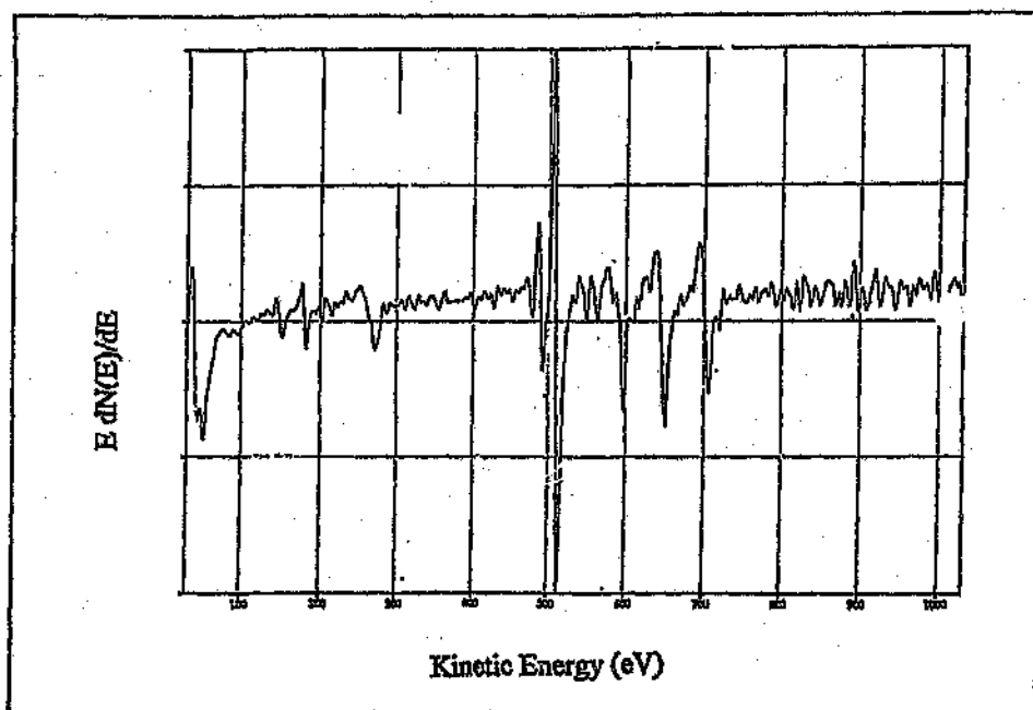
Figure 4.6: Auger electron spectrum of a calcined, reduced catalyst sulfided with 20000 ppm \text{Na}_2\text{S} at pH 10.75
