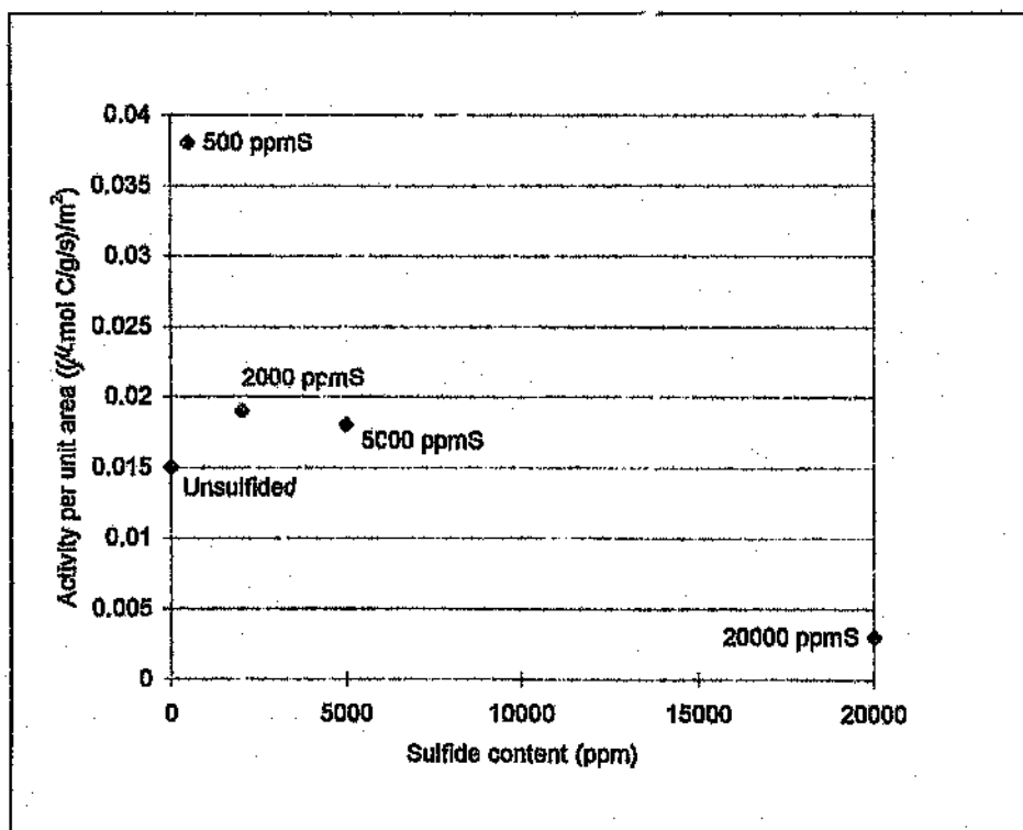
Figure 8.2: Activity per unit area of sulfided catalysts as a function of sulfide content
