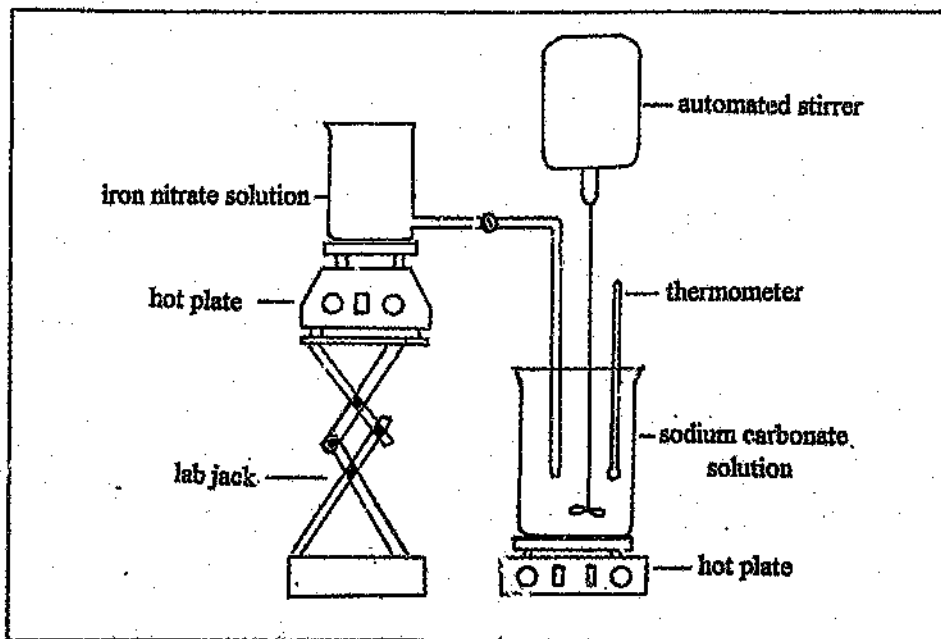
Figure 2.1: Precipitation apparatus for the preparation of iron catalysts
