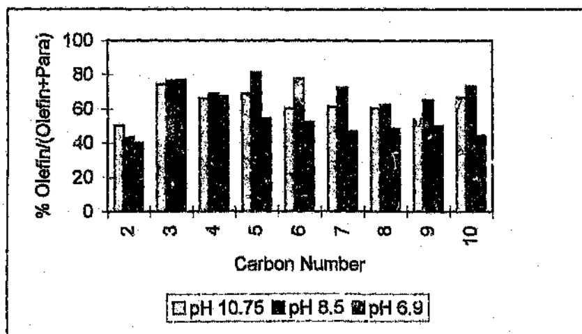
Figure 10.10: Olefin selectivity of 2000 ppm polysulfided catalysts prepared by sulfidation at pH 10.75, 8.5 and 6.9
