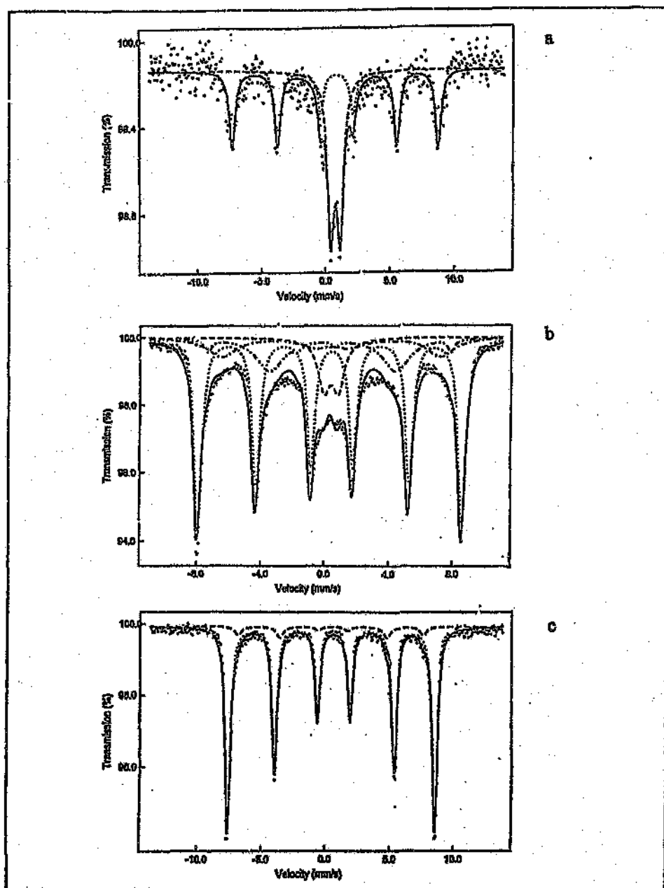
Figure 6.2: a) Uncalcined catalyst sulfided with 2000 ppm \text{Na}_2\text{S} recorded at 298 K b) Mössbauer measurement at 77 K c) After calcination at 400°C, recorded at 298 K
