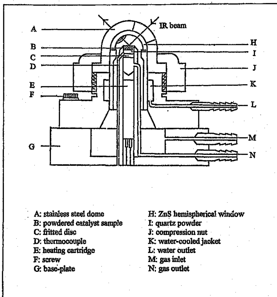
Figure 2.4: Longitudinal section through the variable temperature DRIFTS reactor cell
