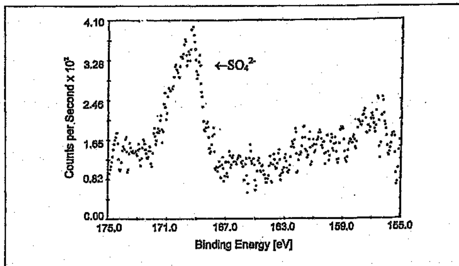
Figure 4.1: S (2p) photopeak of catalyst sulfided with 5000 ppm Na 2 S, calcined at 400°C and reduced at 300°C.
