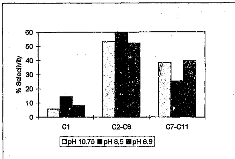
Figure 10.11: Product selectivity of catalysts sulfided at various pH values with 2000 ppm polysulfide
