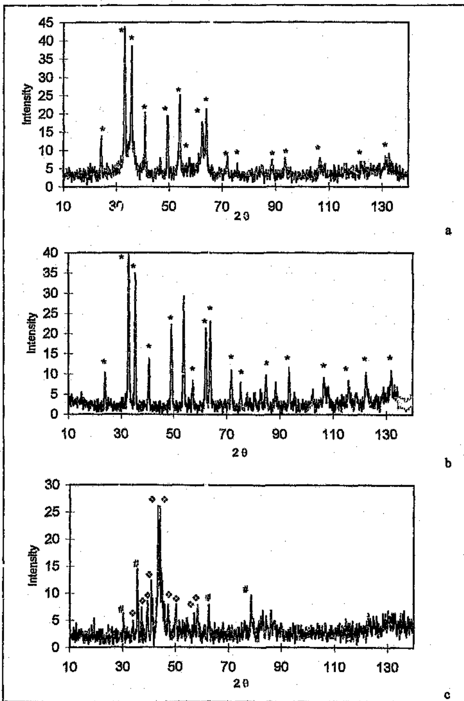
Figure 3.11: Diffractogram of catalyst sulfided with 2000 ppm \text{Na}_2\text{S} at pH 6.9 a) uncalcined b) calcined c) spent where * = \text{Fe}_2\text{O}_3 # = \text{Fe}_3\text{O}_4 \diamond = \chi -carbide
