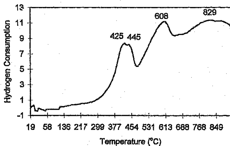
Figure 10.3: Reduction profiles of catalysts sulfided with 2000 ppm S a) Catalyst sulfided with \text{Na}_2\text{S} b) Catalyst sulfided with (\text{NH}_4)_2\text{S}
