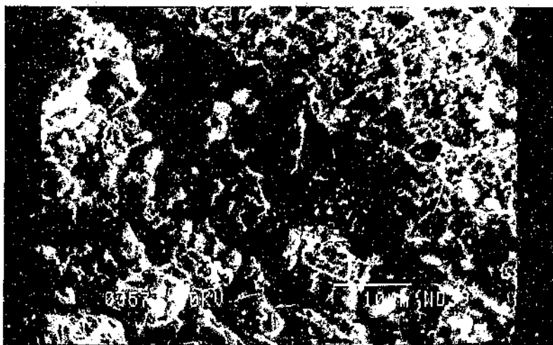
Figure 3.2b: Spent catalyst sulfided with 2000 ppm S viewed at 2000x magnification
