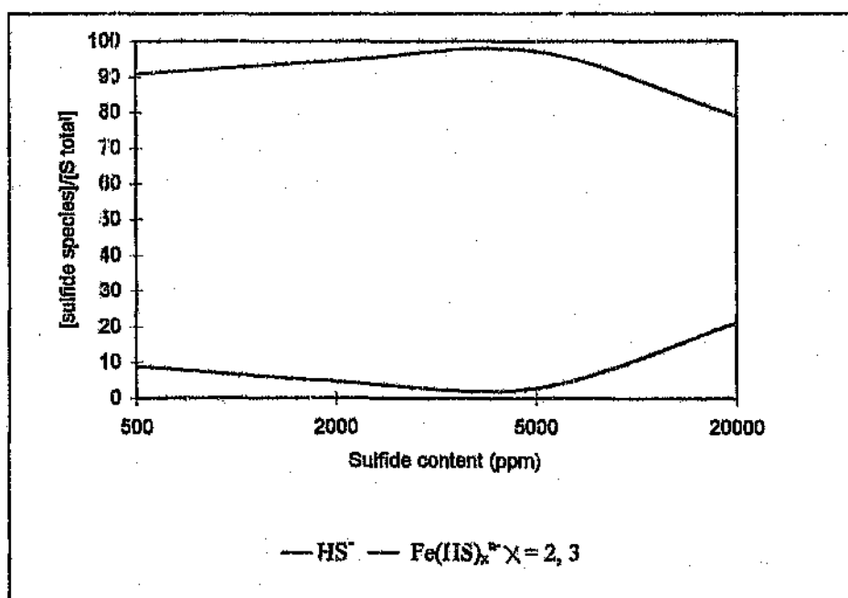
Figure 7.4: Distribution of sulfide species at pH 8.5, with increasing sulfide content
