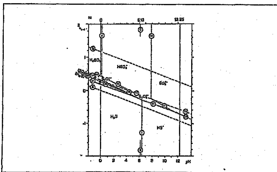
Figure 10.1: Pourbaix diagram for the S-H 2 O system at 100°C considering only sulfur, sulfides, thiosulfates, tetrathionates and sulfites (log c = 0 )
