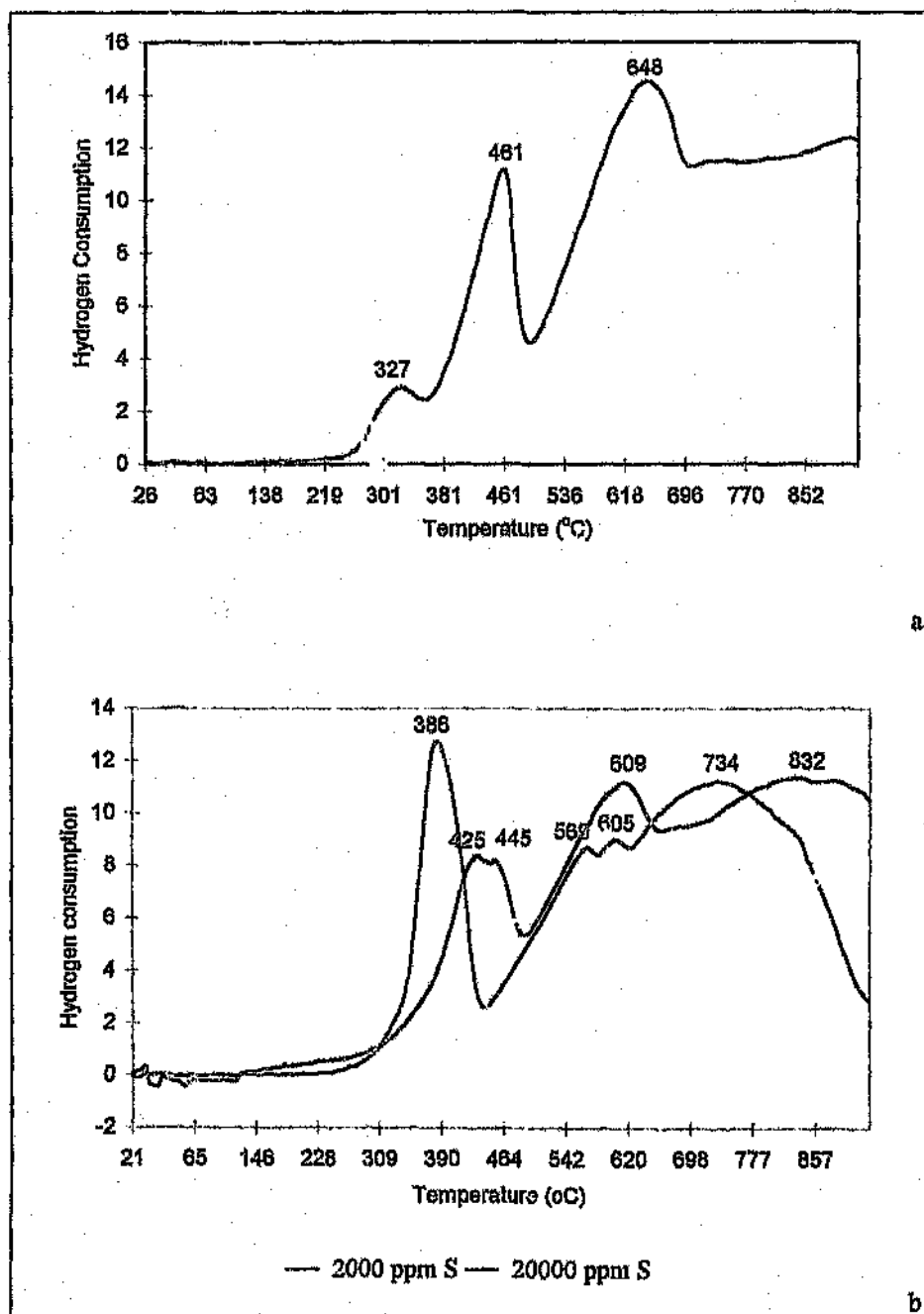
Figure 8.7: Temperature Programmed Reduction profiles of precipitated-iron catalysts: a) Unsulfided catalyst b) Catalyst sulfided with 2000 ppm S superimposed on catalyst sulfided with 20000 ppm S
