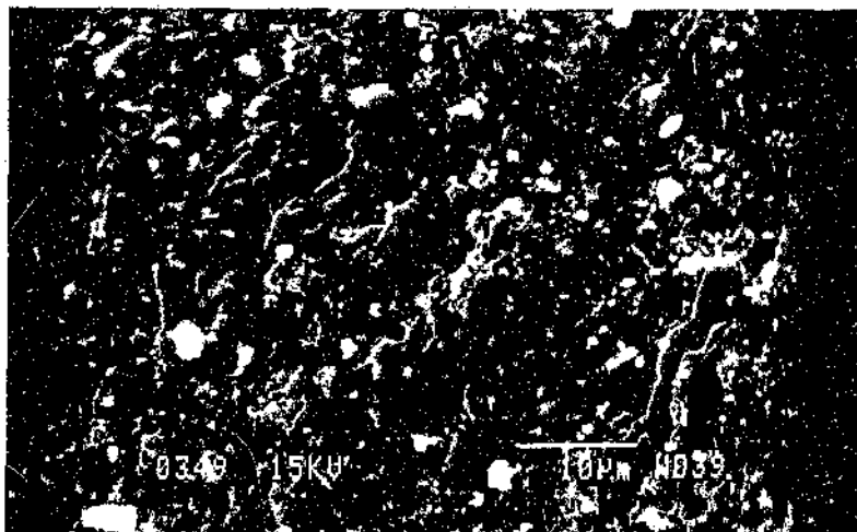
Figure 3.1b: Micrograph taken at 2000x magnification of a calcined, unsulfided precipitated-iron catalyst
