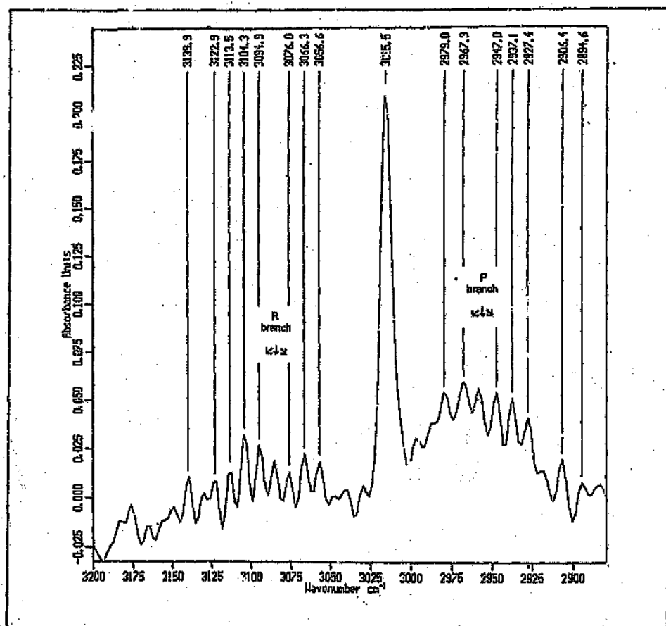
Figure 5.18: P- and R-branch band envelopes as observed on a sulfided catalyst reduced at 300°C during FT synthesis
