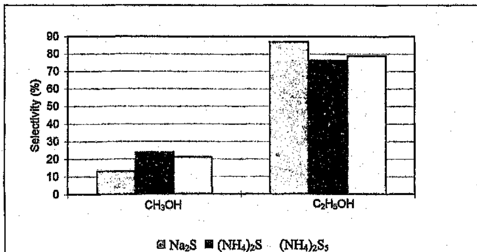
Figure 9.2: Distribution of oxygenated products for various sulfided catalysts
