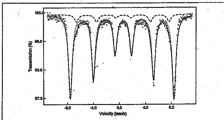
Figure 6.3: Uncalcined sample sulfided with 20000 ppm \text{Na}_2\text{S}
