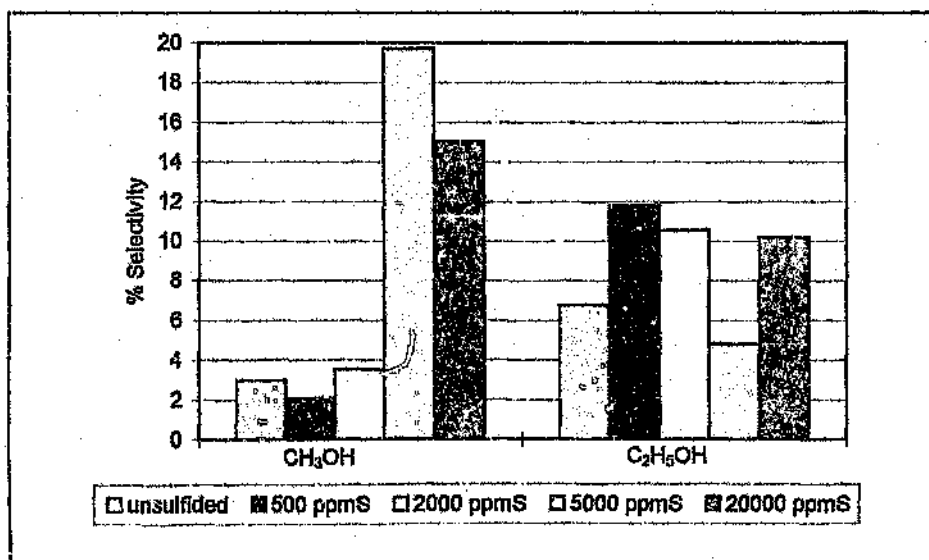
Figure 8.5: Comparison of the oxygenate selectivity of sulfided catalysts
