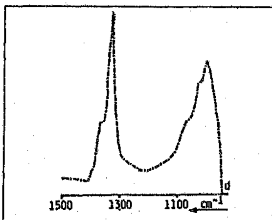
Figure 5.10: Sulfated \text{TiO}_2 after exchange with \text{H}_2^{18}\text{O} at 450^\circ\text{C} (adapted from [137])
