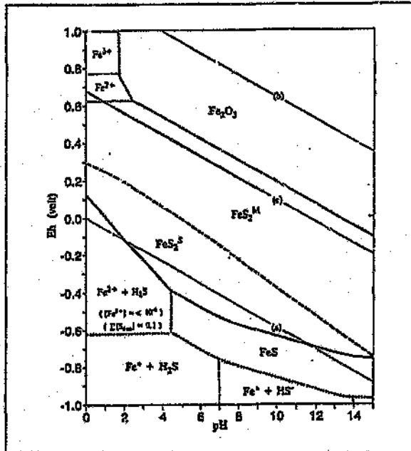
Figure 1.2: Eh-pH diagram for pyrite [10]
