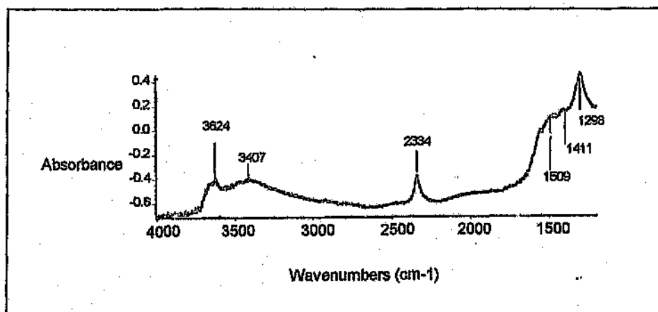
Figure 5.9: Catalyst sulfided at pH 10.75 with 2000 ppm (\text{NH}_4)_2\text{S} , after calcination at 400^\circ\text{C} , showing a sharp peak near 1300\text{ cm}^{-1}
