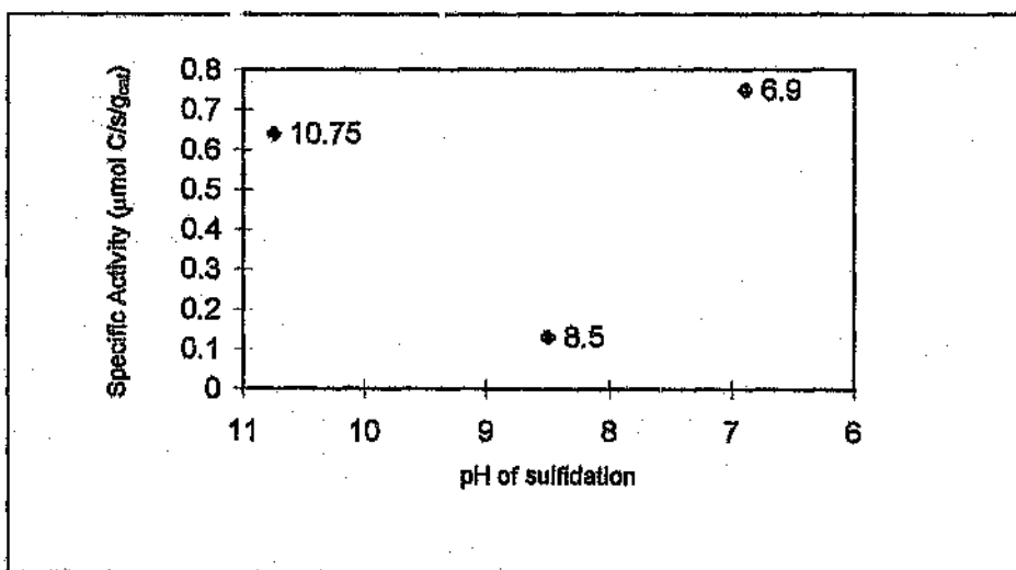
Figure 10.7: Effect of pH of sulfidation on the specific activity of catalysts sulfided with 2000 ppm polysulfide
