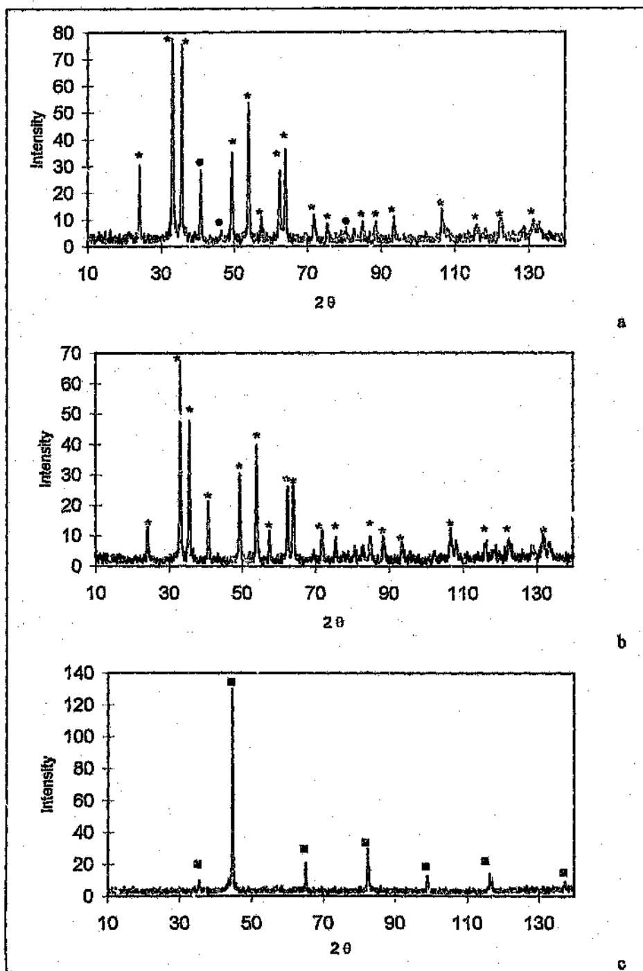
Figure 3.12: Diffractogram of catalyst sulfided with 20000 ppm \text{Na}_2\text{S} at pH 6.9 a) uncalcined b) calcined c) spent where * = \text{Fe}_2\text{O}_3 • = \text{FeS} ■ = \alpha\text{-Fe}
