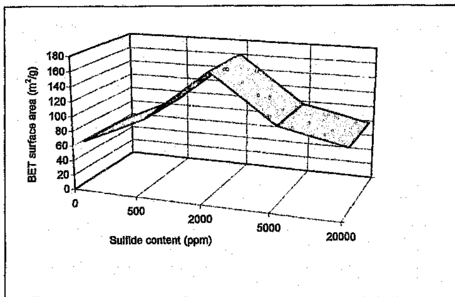
Figure 8.6: Variation of surface area with sulfide content prior to calcination.
