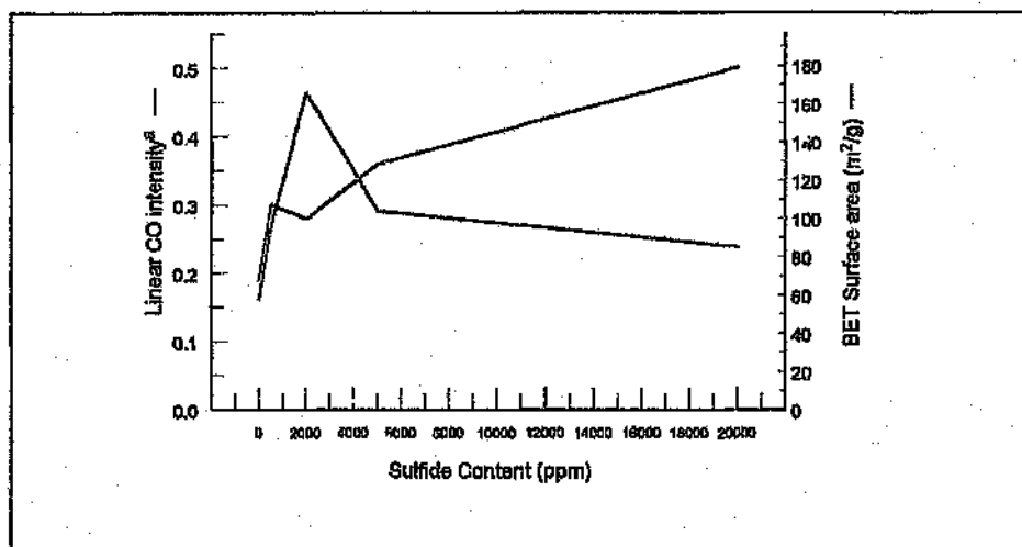
Figure 5.4: Comparison of BET surface areas and relative intensities a of linear carbonyl species adsorbed on iron catalysts as a function of sulfide content
