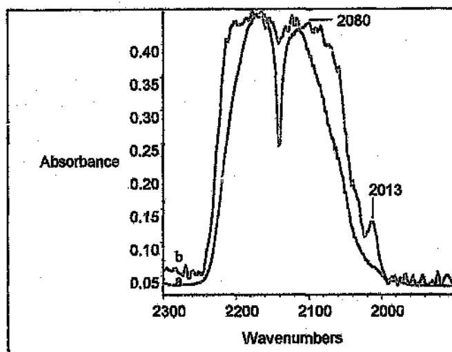
Figure 3.2: The effect of reduction temperature on the evolution of linear carbonyl species on 20000 ppm polysulfided iron catalysts a) reduced at 300°C b) reduced at 400°C
