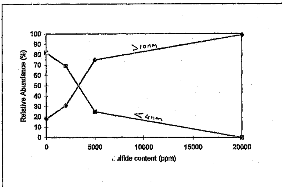
Figure 6.7: The effect of increasing sulfide content on particle size distribution of uncalcined catalysts sulfided in the range 2000-20000 ppm S at pH 6.9
