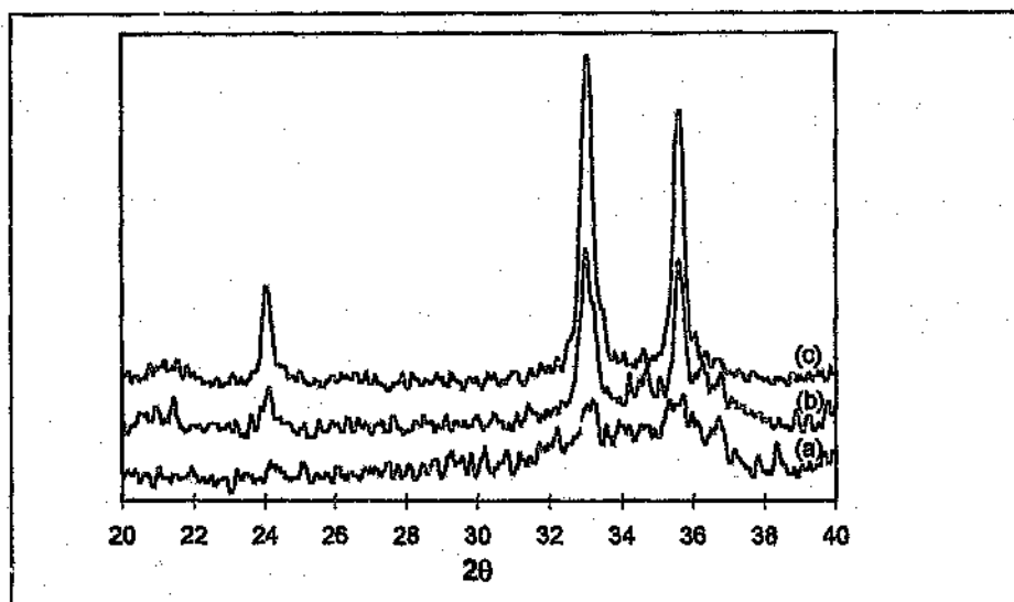
Figure 3.15: Stack-plot of diffraction patterns obtained from catalysts sulfided with 5000 ppm \text{Na}_2\text{S} a) Catalyst sulfided at pH 10.75 b) Catalyst sulfided at pH 8.5 c) Catalyst sulfided at pH 6.9
