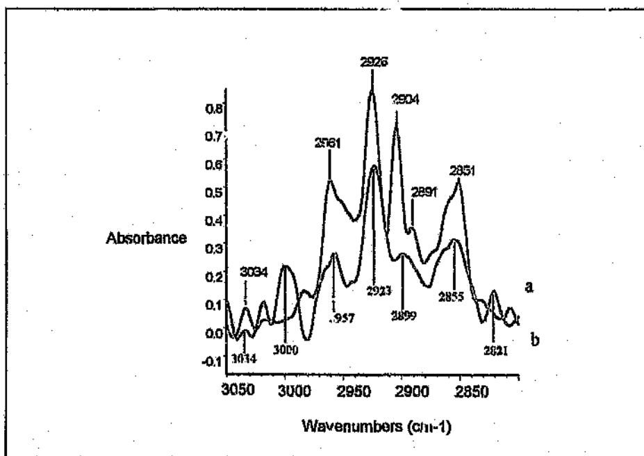
Figure 5.14: a) Hydrocarbon formation on an unsulfided iron catalyst b) Fischer-Tropsch synthesis on a catalyst sulfided with 2000 ppm \text{Na}_2\text{S} at pH 10.75
