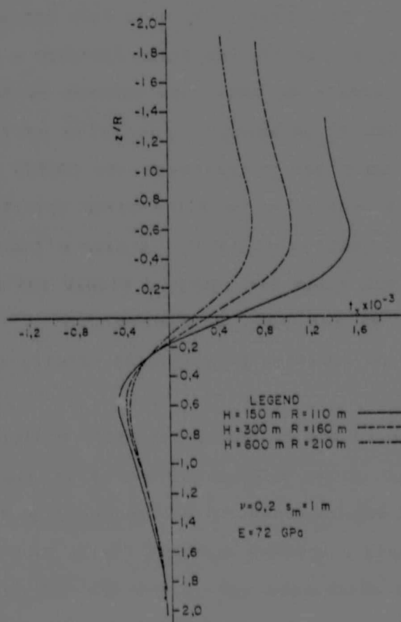
Figure 3.3 Distribution of tilt along the shaft
