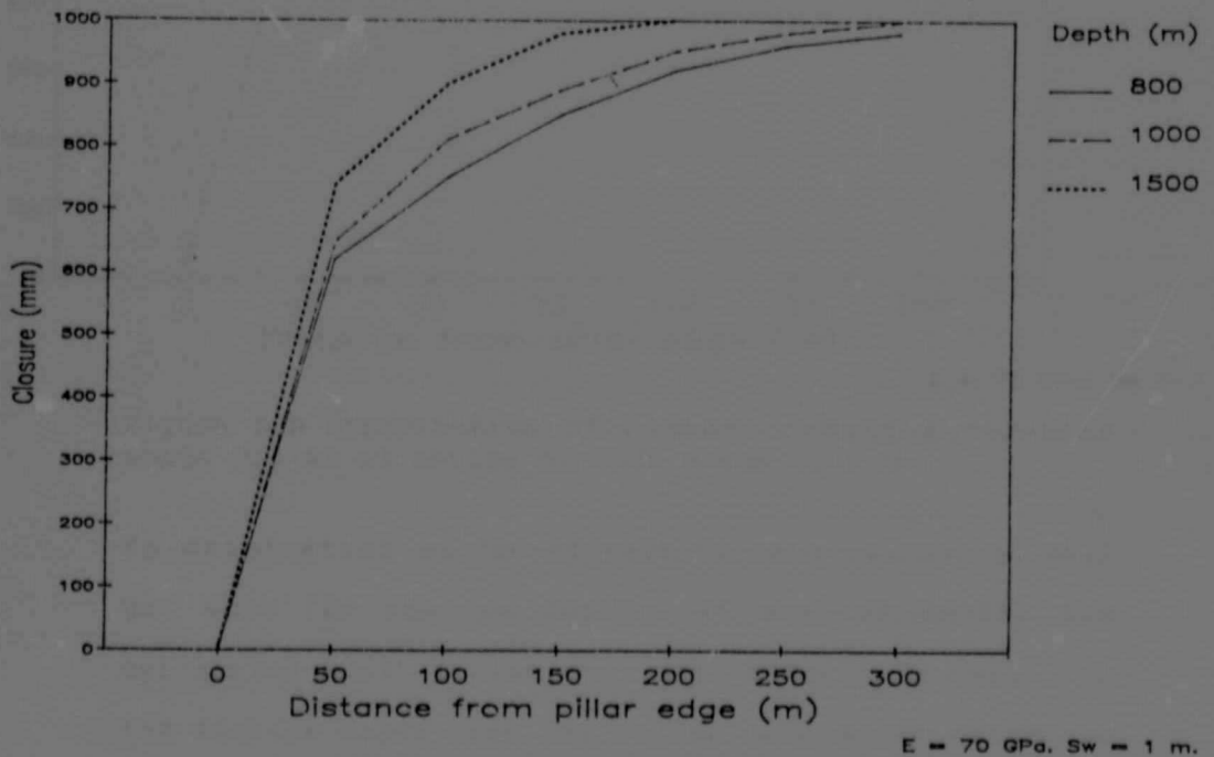
Figure 3.4 Distribution of closure around circular shaft pillars at depths of 800 m, 1000 m and 1500 m.
