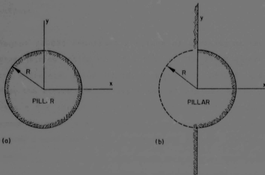
Figure 2.1 Most adverse geometries with respect to vertical strain and stress (a), tilt (b).
