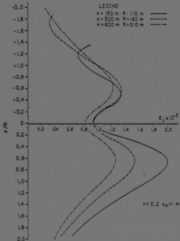
Figure 3.2 Distribution of vertical induced strain along the shaft
