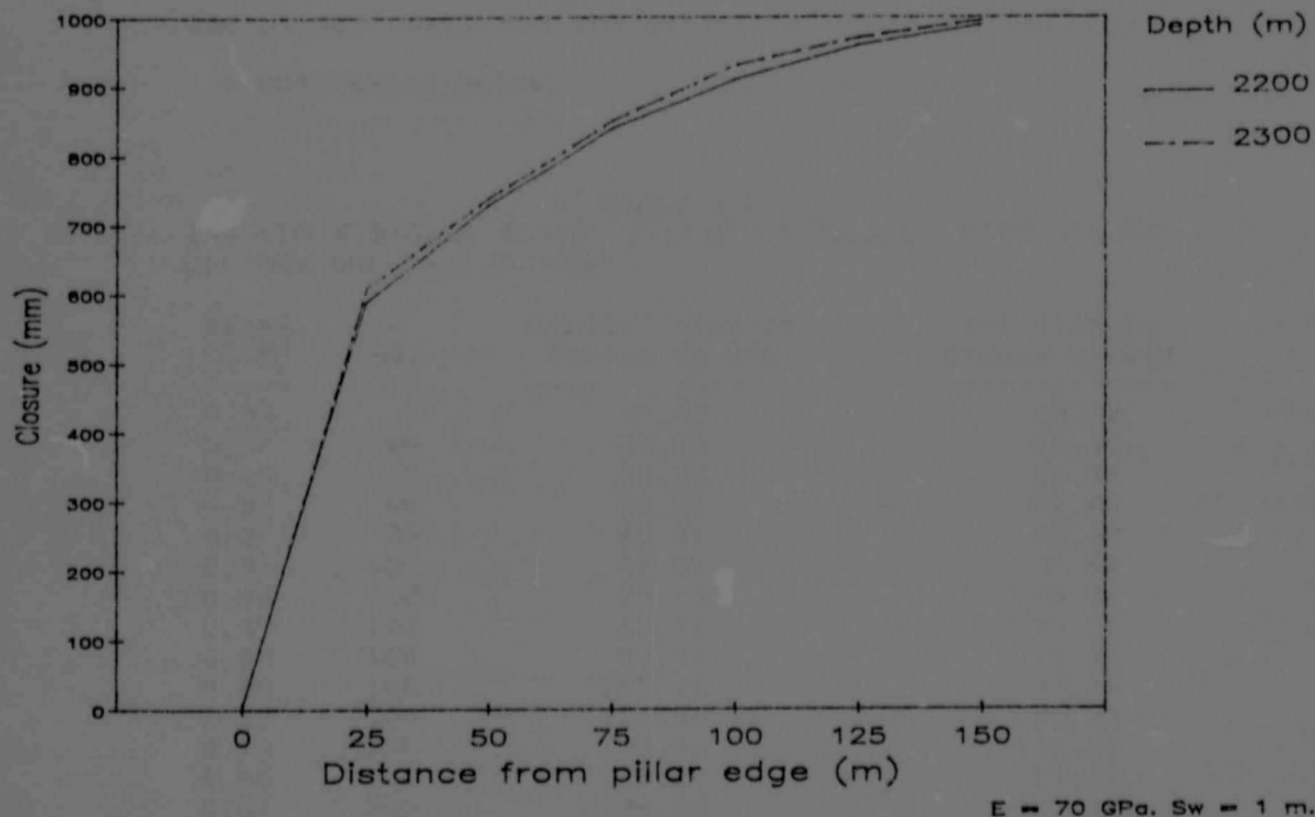
Figure 3.5 Distribution of closure around a circular shaft pillar at depths of 2200 m and 2300 m.
