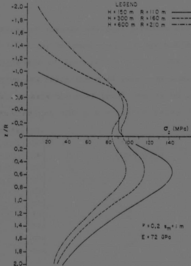
Figure 3.1 Distribution of induced vertical stress along the shaft
