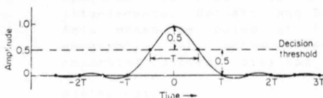
Fig 3.3 Pulse shape with raised cosine spectrum
