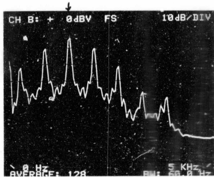
Fig 4.6 Photograph of spectrum of FSK signal modulated with 1:1 mark:space ratio data at 600 Hz. The centre frequency of 1487.5 Hz is arrowed. Note the sidebands at intervals of 600 Hz. The spectrum has been averaged over 128 samples.
