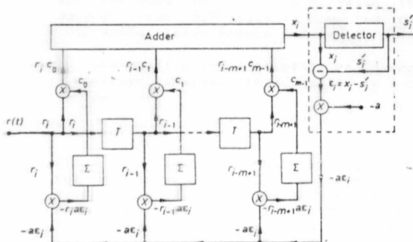
Fig 3.4 Structure of Linear Adaptive Equaliser
