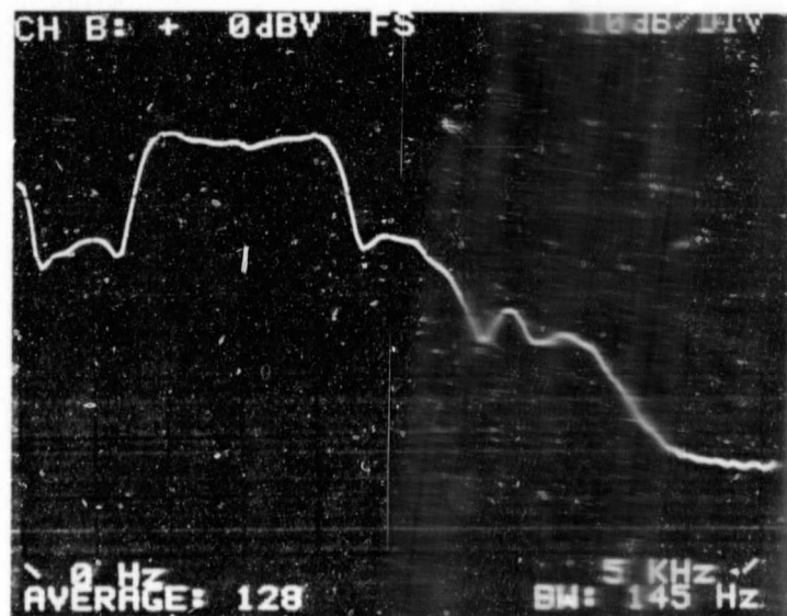
Fig 4.7 Photograph of spectrum of FSK signal modulated by 2047 bit pseudo-random data averaged over 128 samples. Note that the main portion signal lies in the region f_c \pm 600 Hz. See also section 4.5.1.
