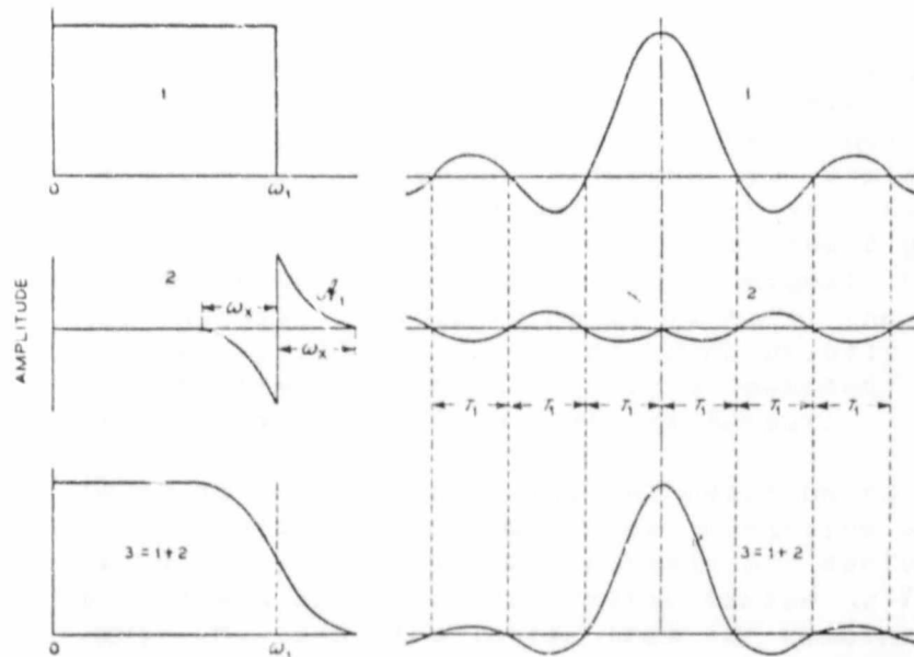
Fig 2.2 Idealised transmission characteristic with gradual cut-off, 3, obtained by superposition of characteristic with sharp cut-off, 1, and characteristic, 2, with odd symmetry about \omega_1 .
