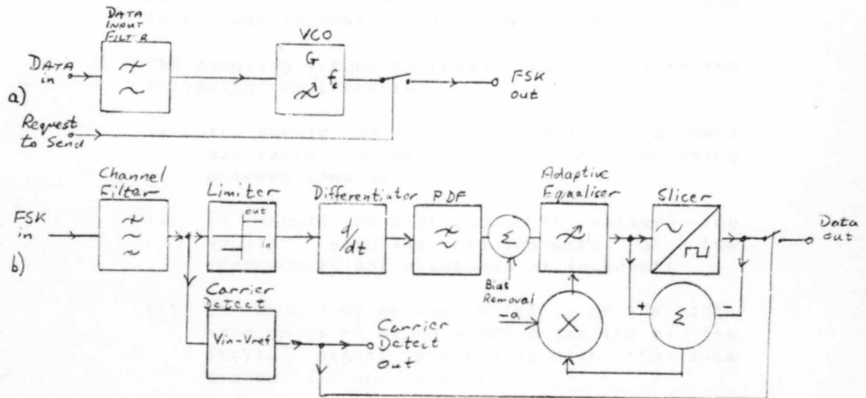
Fig 4.1 Modem Block Diagram a) Transmitter Section; b) Receiver Section
