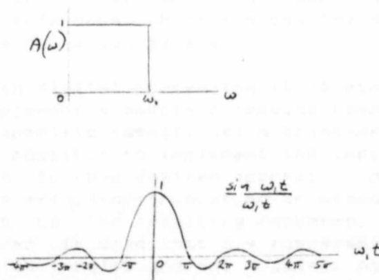
Fig 3.2 Ideal low-pass filter and its impulse response
