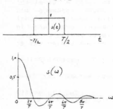
Fig 3.1 Rectangular pulse and its Fourier Transform
