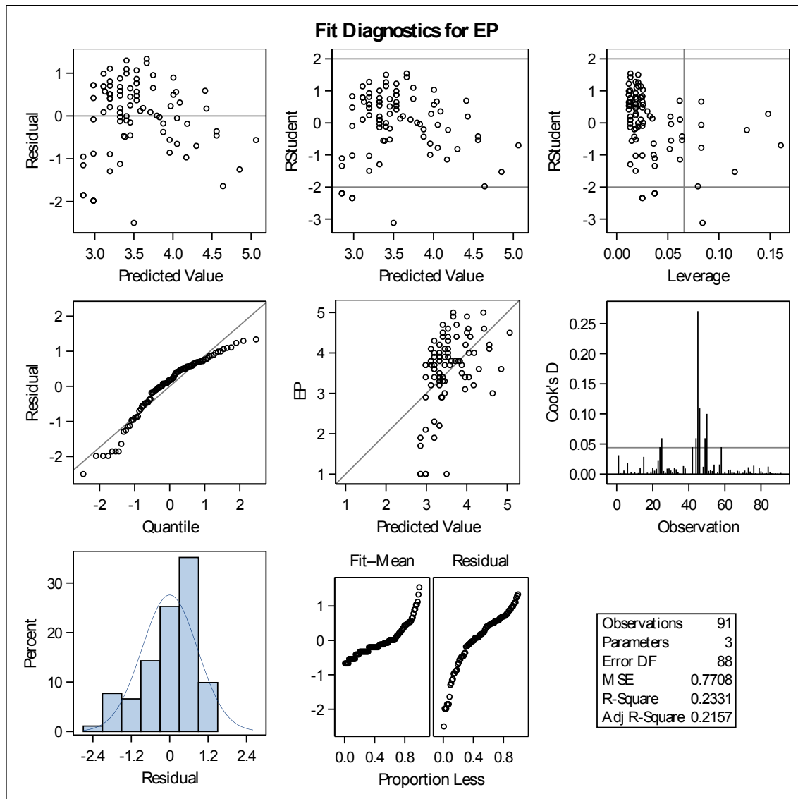
Figure 4-12: Fit diagnostic for the regression model using a combined enterprise performance and enterprise control factors
