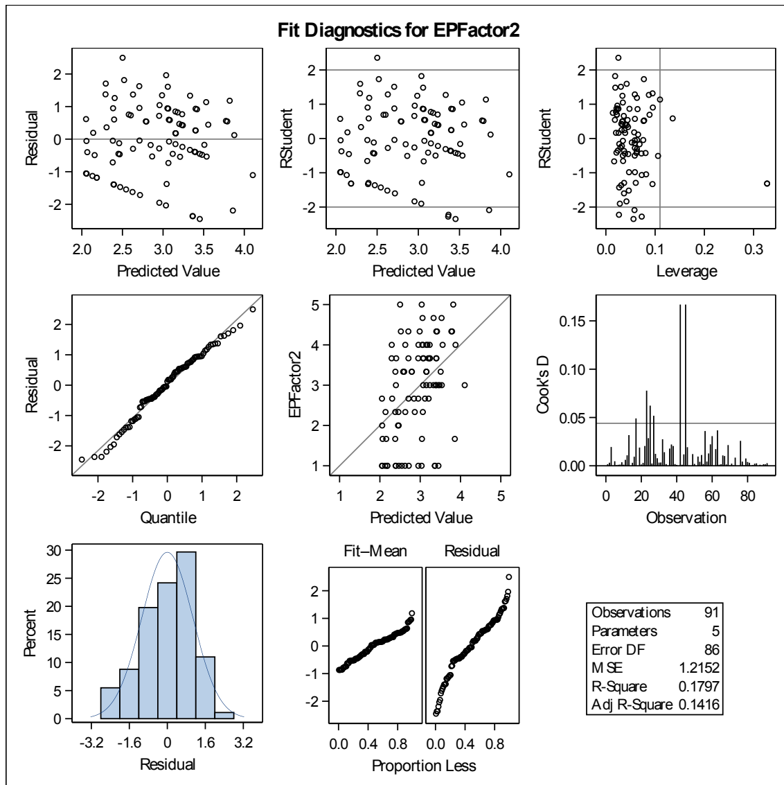
Figure A-2: Fit diagnostic for the regression model between enterprise performance factor 2 and motivation factors
