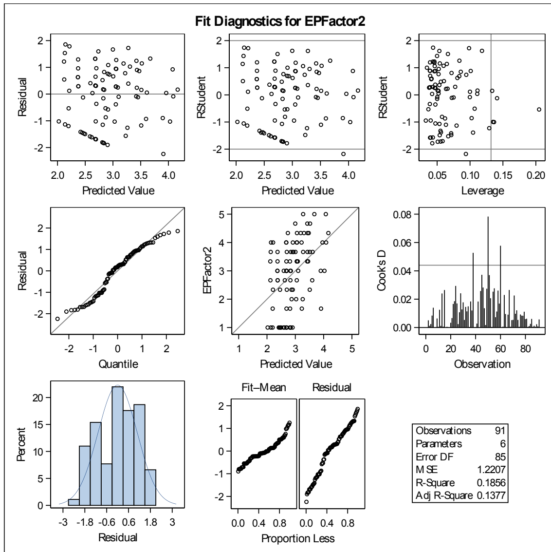
Figure A-5: Fit diagnostic for the regression model between enterprise performance factor 2 and individual control factors
