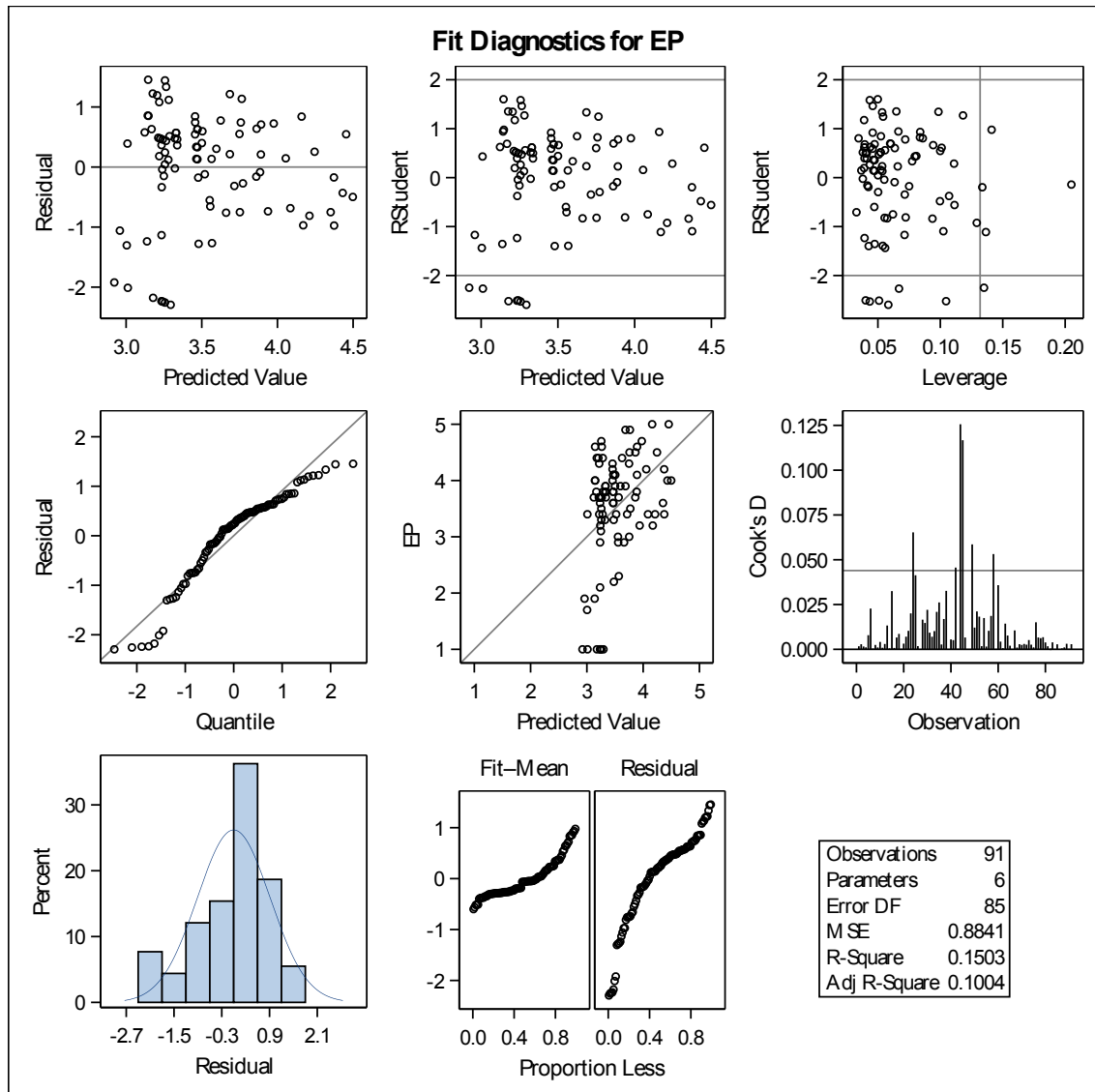
Figure 4-11: Fit diagnostic for the regression model using a combined enterprise performance and individual control factors
