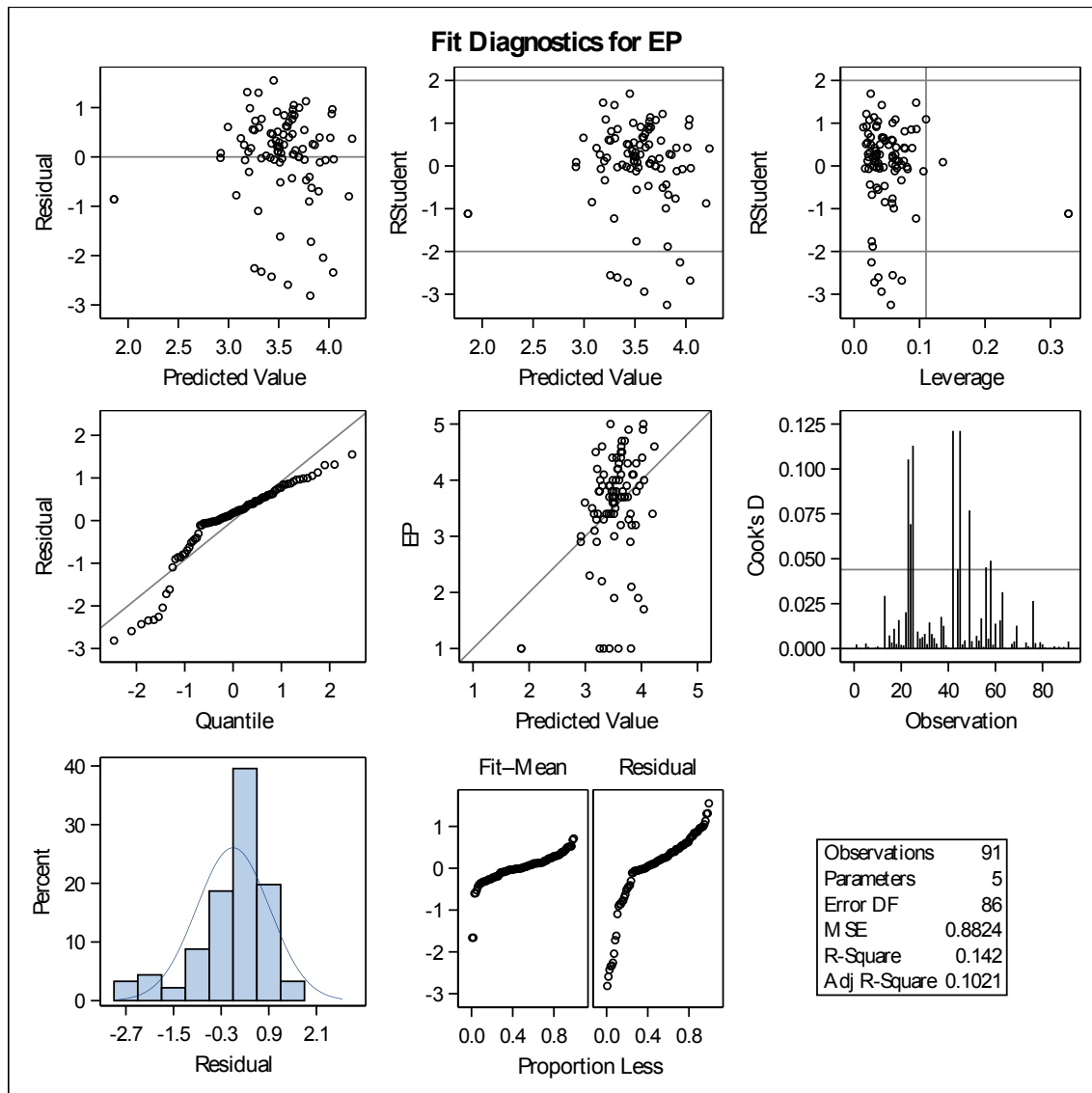
Figure 4-10: Fit diagnostic for the regression model using a combined enterprise performance
