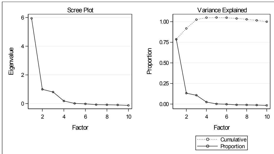
Figure 4-7: Scree plot from EFA of the enterprise performance scale
