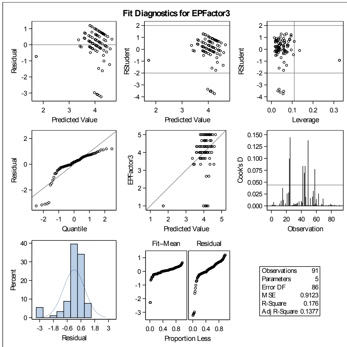
Figure A-3: Fit diagnostic for the regression model between enterprise performance factor 3 and motivation factors
