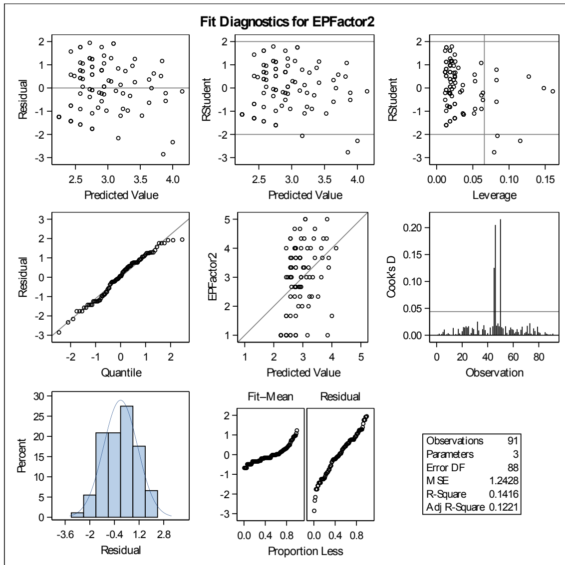
Figure A-8: Fit diagnostic for the regression model between enterprise performance factor 2 and enterprise control factors
