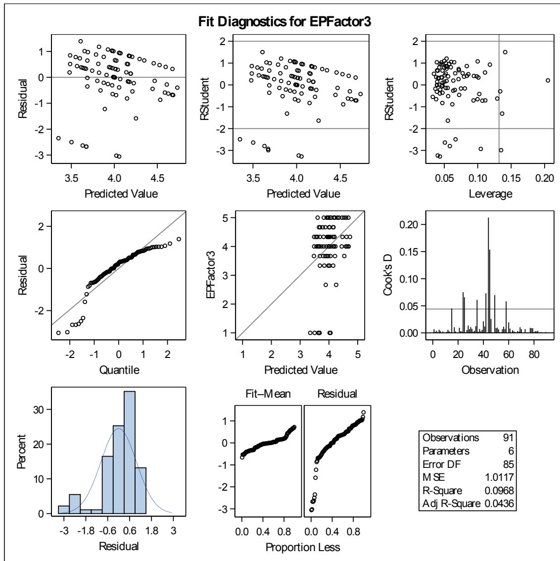
Figure A-6: Fit diagnostic for the regression model between enterprise performance factor 3 and individual control factors
