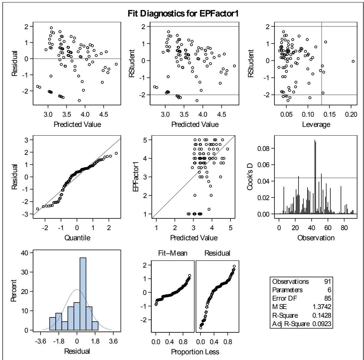
Figure A-4: Fit diagnostic for the regression model between enterprise performance factor 1 and individual control factors
